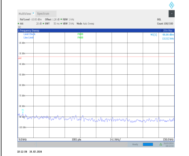
1-N12-15-15-M-1-DFT-PI2BPSK-Inner_1RB_Left-1 @ 1-0.009-0.15-Ant1-0.01--86.86--33-PASS
