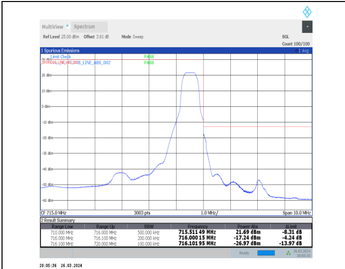
1-N12-15-15-H-2-DFT-PI2BPSK-Edge_1RB_Right-1@78-Ant1-1--PASS-see graph
