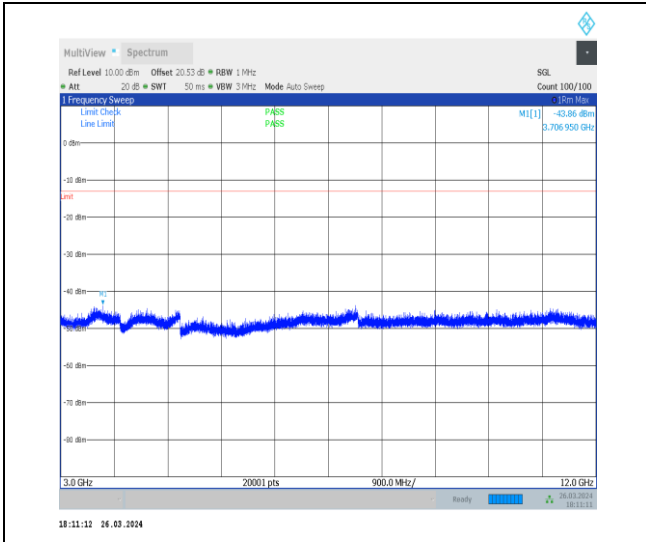
1-N12-15-15-L-1-DFT-PI2BPSK-Inner_1RB_Left-1 @ 1-3000-12000-Ant1-3706.95--43.86--13-PASS
