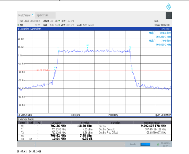
1-N12-15-10-M-9-CP-256QAM-Outer_Full-52@0-Ant 1-9.292-10.040-≤10-PASS
