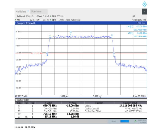
1-N12-15-15-M-6-CP-QPSK-Outer_Full-79@0-Ant1 14.116-15.180-≤15-PASS
