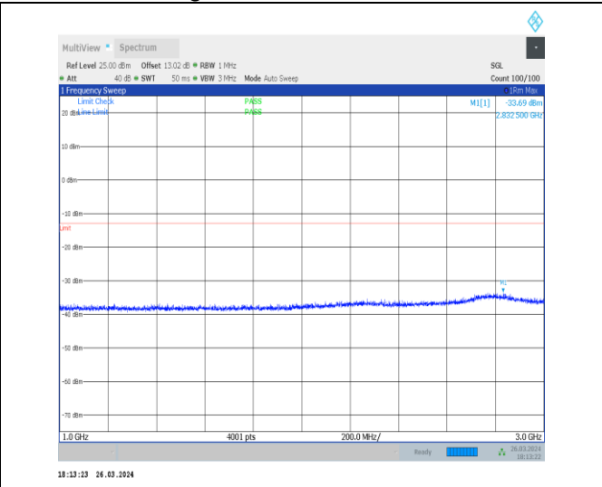
1-N12-15-15-M-1-DFT-PI2BPSK-Inner_1RB_Left-1 @ 1-1000-3000-Ant1-2832.50--33.69--13-PASS
