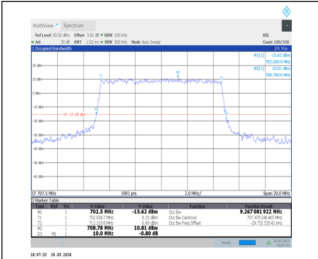
1-N12-15-10-M-8-CP-64QAM-Outer_Full-52@0-Ant 1-9.267-10.000-≤10-PASS
