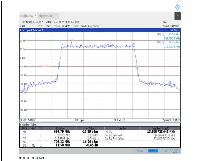
1-N12-15-15-M-3-DFT-16QAM-Outer_Full-75@0-Ant 1-13.507-14.580-≤15-PASS
