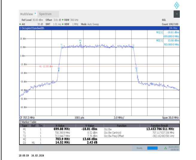
1-N12-15-15-M-5-DFT-256QAM-Outer_Full-75@0-A nt1-13.454-14.520-≤15-PASS
