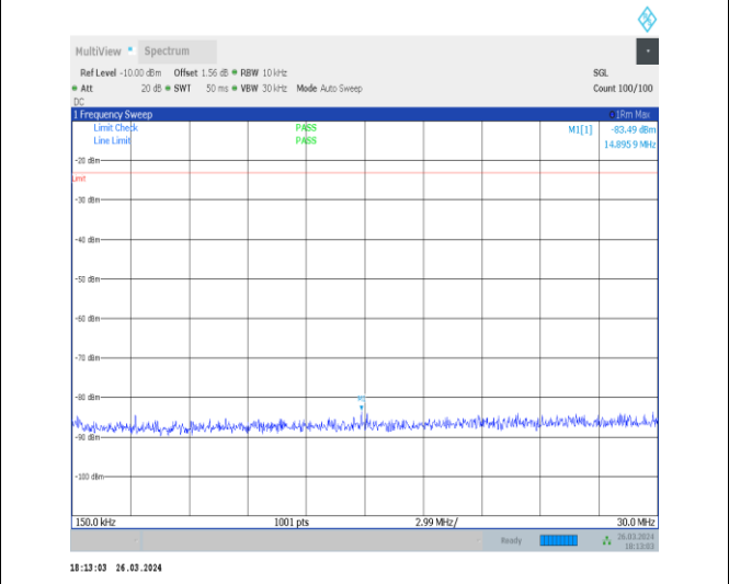
1-N12-15-15-M-1-DFT-PI2BPSK-Inner_1RB_Left-1 @ 1-0.15-30-Ant1-14.90--83.49--23-PASS
