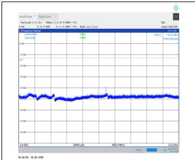
1-N12-15-15-H-1-DFT-PI2BPSK-Inner_1RB_Left-1 @1-3000-12000-Ant1-7904.55--43.18--13-PASS
