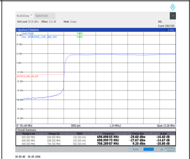
1-N12-15-10-L-6-CP-QPSK-Outer_Full-52@0-Ant1-1--PASS-see graph
