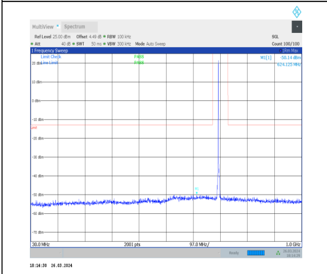
1-N12-15-15-H-1-DFT-PI2BPSK-Inner_1RB_Left-1 @ 1-30-1000-Ant1-624.13--50.14--13-PASS
