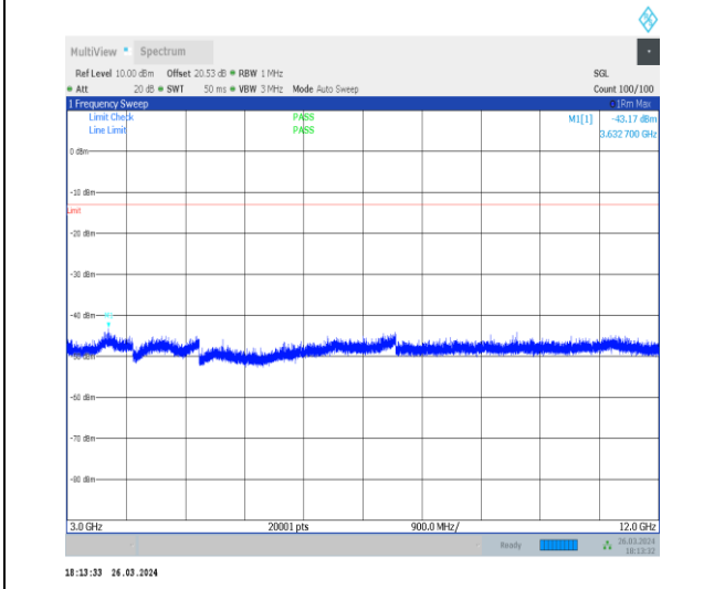
1-N12-15-15-M-1-DFT-PI2BPSK-Inner_1RB_Left-1 @ 1-3000-12000-Ant1-3632.70--43.17--13-PASS
