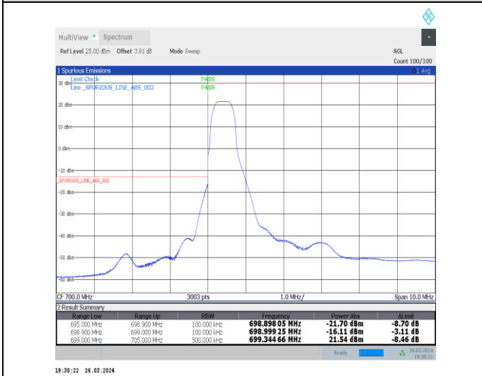
1-N12-15-10-L-4-CP-QPSK-Edge_1RB_Left-1@0-Ant1-1--PASS-see graph
