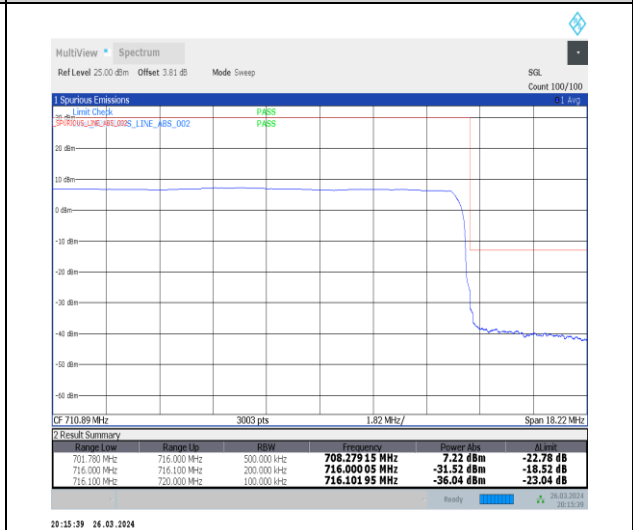
1-N12-15-15-H-6-CP-QPSK-Outer_Full-79@0-Ant1-1--PASS-see graph
