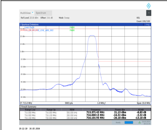
1-N12-15-15-H-5-CP-QPSK-Edge_1RB_Right-1@78-Ant1-1--PASS-see graph
