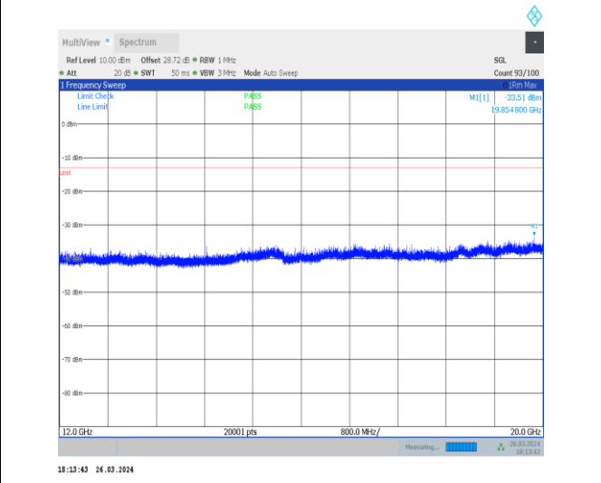
1-N12-15-15-M-1-DFT-PI2BPSK-Inner_1RB_Left-1 @ 1-12000-20000-Ant1-19854.80--33.51--13-PASS
