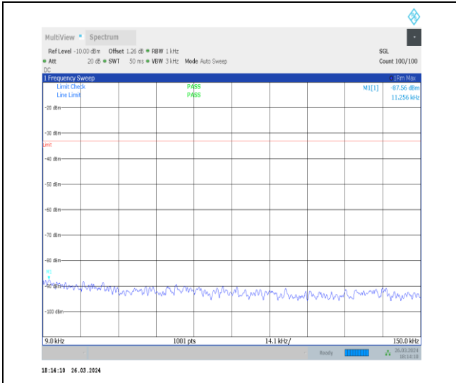
1-N12-15-15-H-1-DFT-PI2BPSK-Inner_1RB_Left-1 @ 1-0.009-0.15-Ant1-0.01--87.56--33-PASS
