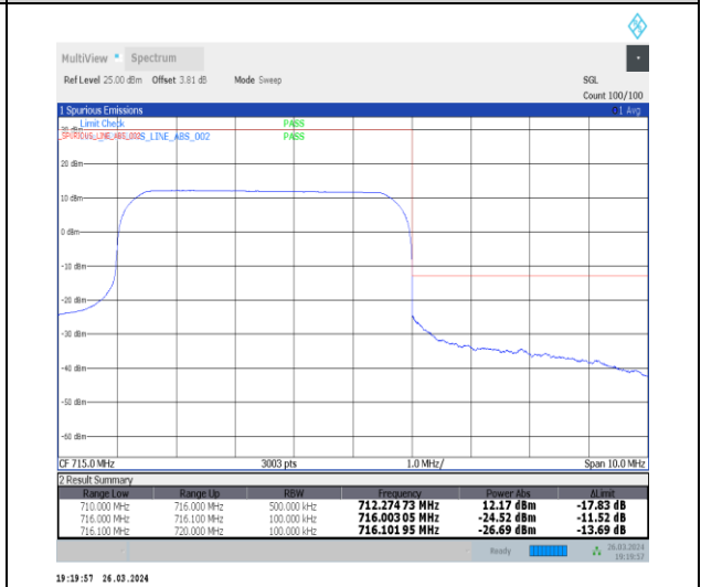
1-N12-15-5-H-6-CP-QPSK-Outer_Full-25@0-Ant1-1--PASS-see graph
