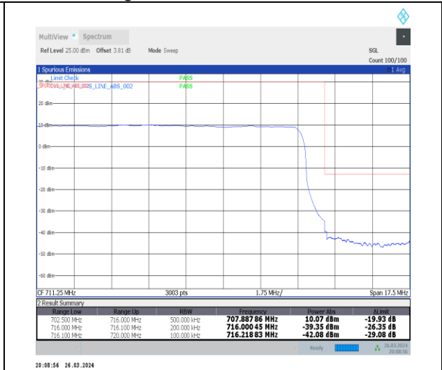
1-N12-15-15-H-3-DFT-PI2BPSK-Outer_Full-75@0-Ant1-1--PASS-see graph
