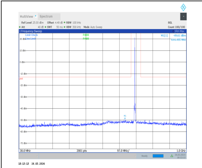
1-N12-15-15-M-1-DFT-PI2BPSK-Inner_1RB_Left-1 @ 1-30-1000-Ant1-644.50--49.61--13-PASS
