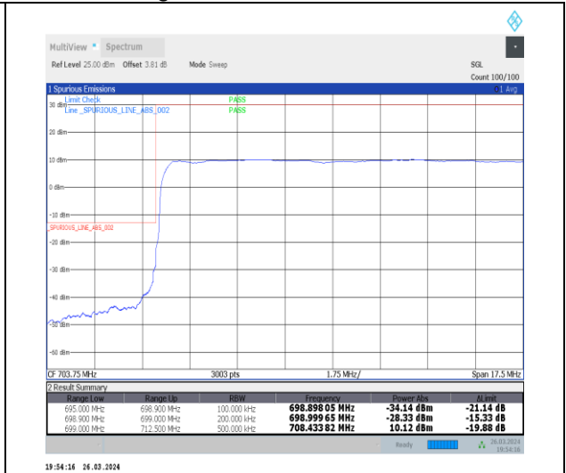
1-N12-15-15-L-3-DFT-PI2BPSK-Outer_Full-75@0-Ant1-1--PASS-see graph
