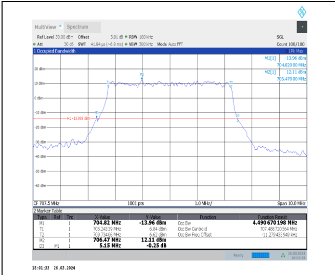
1-N12-15-5-M-5-DFT-256QAM-Outer_Full-25@0-Ant 1-4.491-5.150-≤5-PASS
