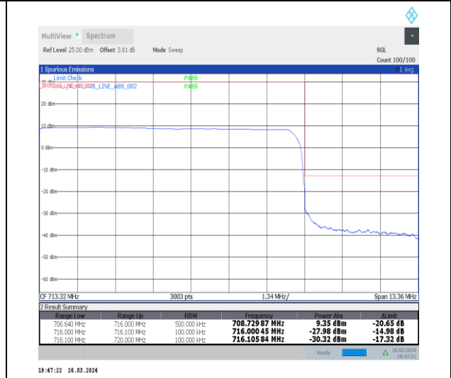
1-N12-15-10-H-6-CP-QPSK-Outer_Full-52@0-Ant1-1--PASS-see graph
