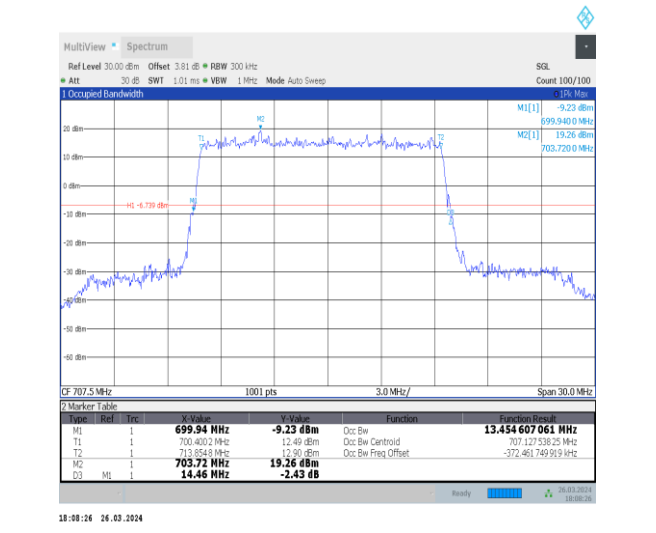
1-N12-15-15-M-2-DFT-PI2BPSK-Outer_Full-75@0-A nt1-13.455-14.460-≤15-PASS
