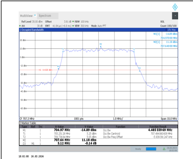
1-N12-15-5-M-9-CP-256QAM-Outer_Full-25@0-Ant 1-4.486-5.120-≤5-PASS
