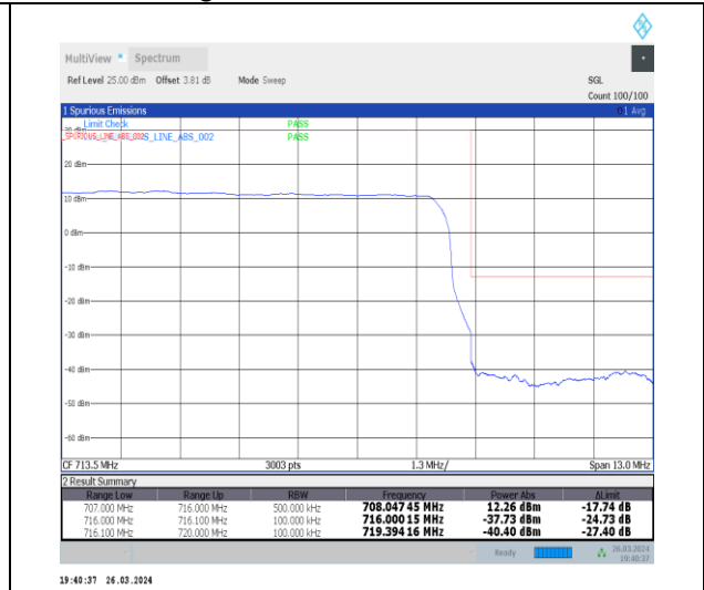
1-N12-15-10-H-3-DFT-PI2BPSK-Outer_Full-50@0-Ant1-1--PASS-see graph
