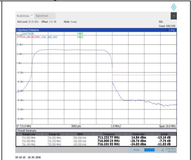
1-N12-15-5-H-3-DFT-PI2BPSK-Outer_Full-25@0-Ant1-1--PASS-see graph
