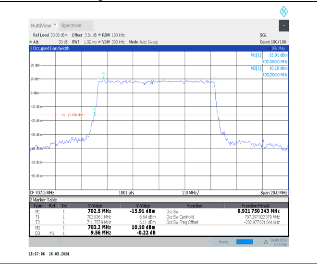
1-N12-15-10-M-5-DFT-256QAM-Outer_Full-50@0-A nt1-8.922-9.560-≤10-PASS
