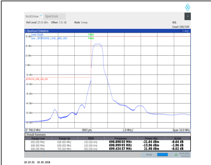
1-N12-15-10-L-1-DFT-PI2BPSK-Edge_1RB_Left-1@0-Ant1-1--PASS-see graph
