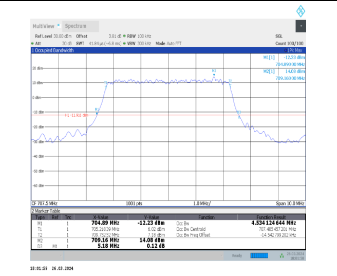
1-N12-15-5-M-8-CP-64QAM-Outer_Full-25@0-Ant1- 4.534-5.180-≤5-PASS
