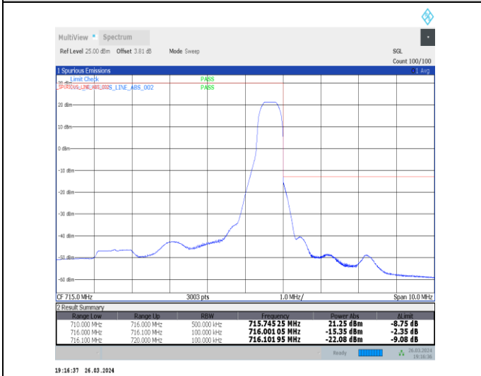
1-N12-15-5-H-5-CP-QPSK-Edge_1RB_Right-1@24-Ant1-1--PASS-see graph
