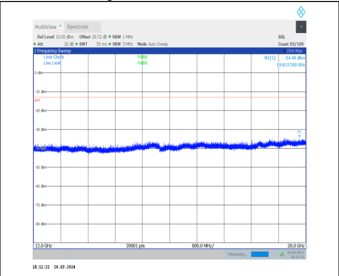
1-N12-15-15-L-1-DFT-PI2BPSK-Inner_1RB_Left-1 @ 1-12000-20000-Ant1-19813.20--34.48--13-PASS
