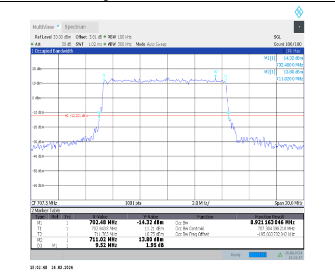
1-N12-15-10-M-1-DFT-QPSK-Outer_Full-50@0-Ant1 -8.921-9.520-≤10-PASS
