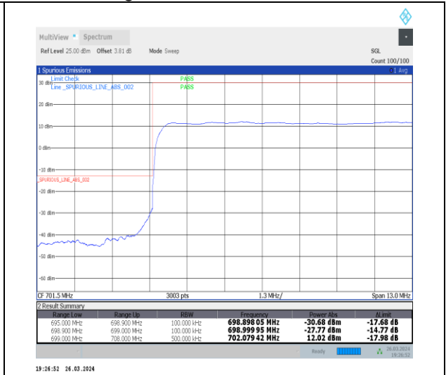
1-N12-15-10-L-3-DFT-PI2BPSK-Outer_Full-50@0-Ant1-1--PASS-see graph
