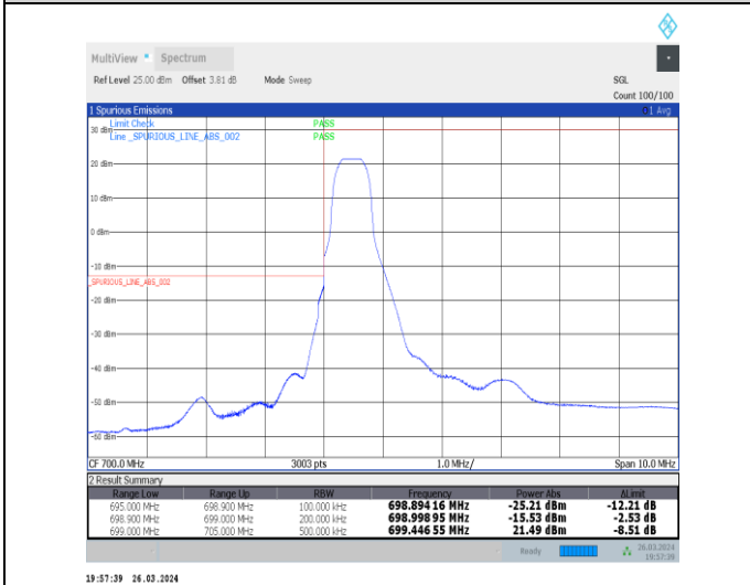
1-N12-15-15-L-4-CP-QPSK-Edge_1RB_Left-1@0-Ant1-1--PASS-see graph
