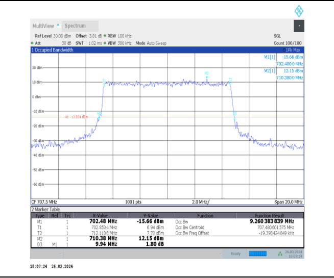
1-N12-15-10-M-7-CP-16QAM-Outer_Full-52@0-Ant1 -9.26-9.940-≤10-PASS
