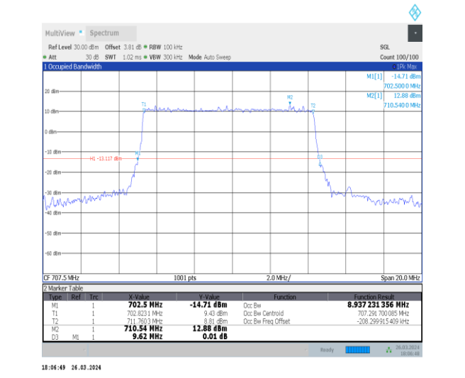
1-N12-15-10-M-3-DFT-16QAM-Outer_Full-50@0-Ant 1-8.937-9.620-≤10-PASS
