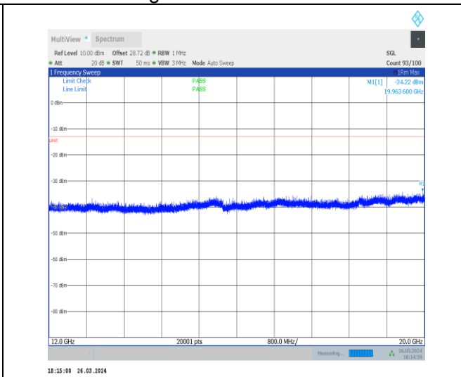
1-N12-15-15-H-1-DFT-PI2BPSK-Inner_1RB_Left-1 @ 1-12000-20000-Ant1-19963.60--34.22--13-PASS
