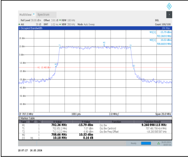
1-N12-15-10-M-6-CP-QPSK-Outer_Full-52@0-Ant1 9.261-10.180-≤10-PASS
