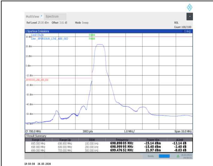
1-N12-15-15-L-1-DFT-PI2BPSK-Edge_1RB_Left-1@0-Ant1-1--PASS-see graph
