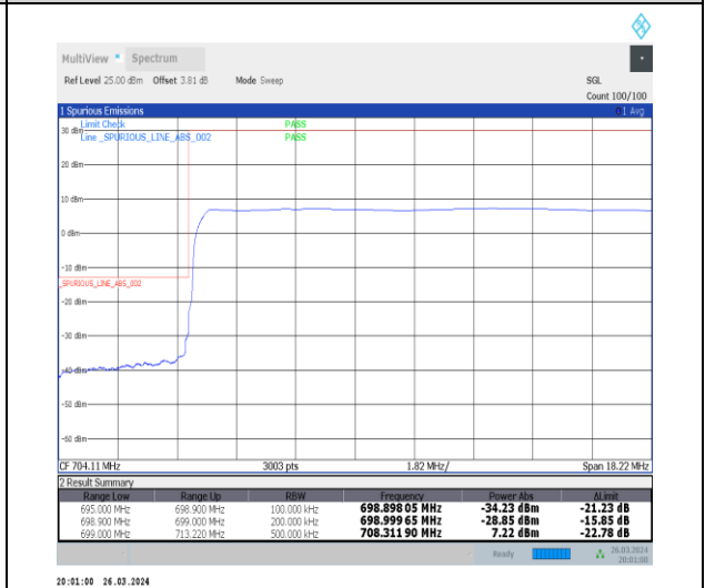
1-N12-15-15-L-6-CP-QPSK-Outer_Full-79@0-Ant1-1--PASS-see graph
