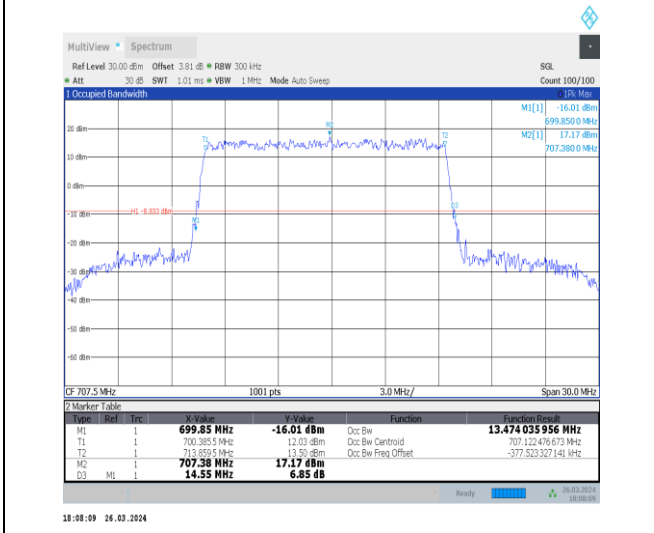
1-N12-15-15-M-1-DFT-QPSK-Outer_Full-75@0-Ant1 -13.474-14.550-≤15-PASS
