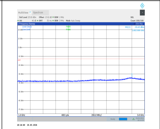
1-N12-15-15-H-1-DFT-PI2BPSK-Inner_1RB_Left-1 @ 1-1000-3000-Ant1-2802.00--33.42--13-PASS
