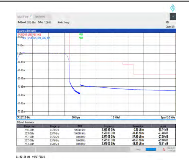
1-N7-15-5-H-6-CP-QPSK-Outer_Full-25@0-Ant1-1--PASS-see graph
