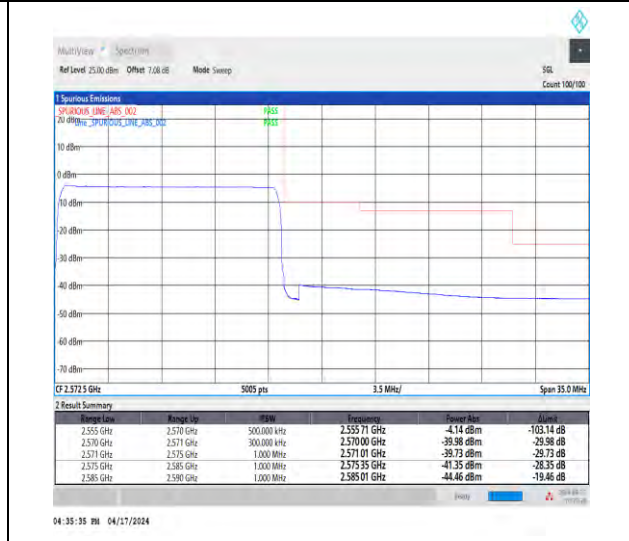
1-N7-15-15-H-6-CP-QPSK-Outer_Full-79@0-Ant1 -1--PASS-see graph
