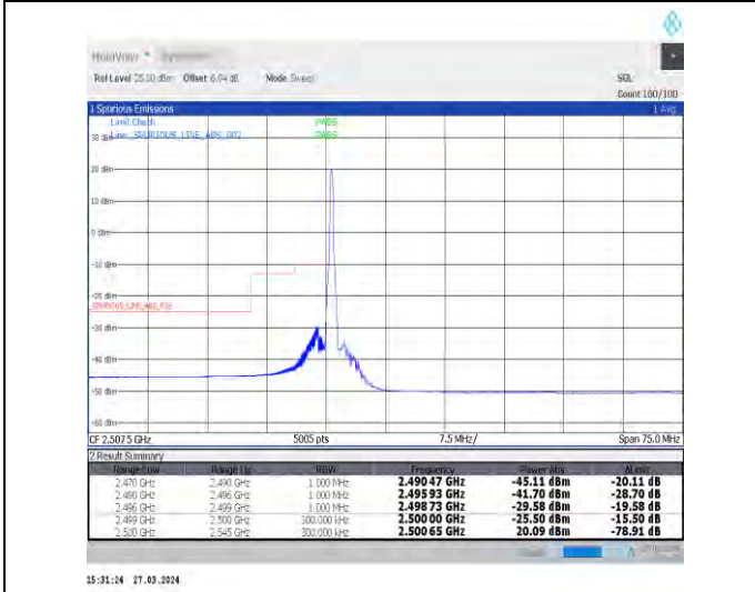
1-N7-15-30-L-4-CP-QPSK-Edge_1RB_Left-1@0-Ant1-1--PASS-see graph
