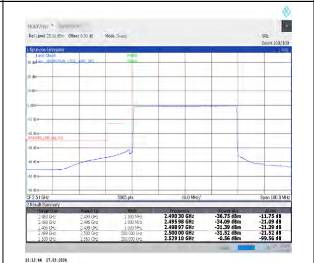
1-N7-15-40-L-6-CP-QPSK-Outer_Full-216@0-Ant1-1--PASS-see graph
