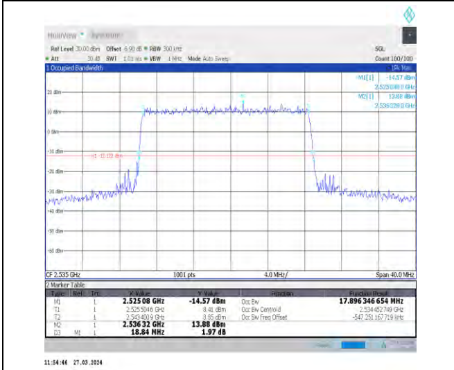
1-N7-15-20-M-4-DFT-64QAM-Outer_Full-100@0-Ant 1-17.896-18.840-≤20-PASS
