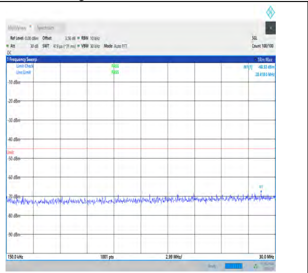
1-N7-15-40-H-1-DFT-PI2BPSK-Inner_1RB_Left-1@ -0.15-30-Ant1-29.79--68.53--45-PASS
