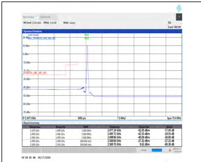
1-N7-15-30-L-1-DFT-PI2BPSK-Edge_1RB_Left-1@0-Ant1-1--PASS-see graph
