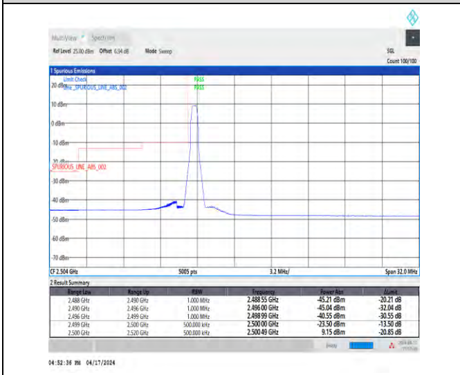
1-N7-15-20-L-4-CP-QPSK-Edge_1RB_Left-1@0-Ant1-1--PASS-see graph
