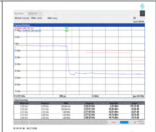
1-N7-15-20-H-3-DFT-PI2BPSK-Outer_Full-100@0 -Ant1-1--PASS-see graph
