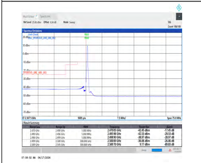
1-N7-15-30-L-4-CP-QPSK-Edge_1RB_Left-1@0-Ant1-1--PASS-see graph
