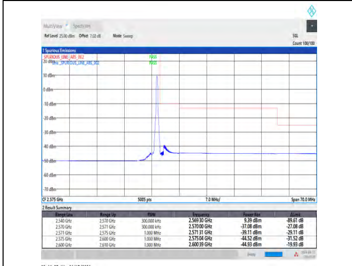
1-N7-15-30-H-5-CP-QPSK-Edge_1RB_Right-1@159-Ant1-1--PASS-see graph
