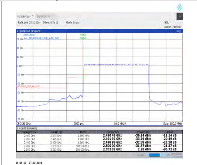
1-N7-15-40-L-3-DFT-PI2BPSK-Outer_Full-216@0 -Ant1-1--PASS-see graph
