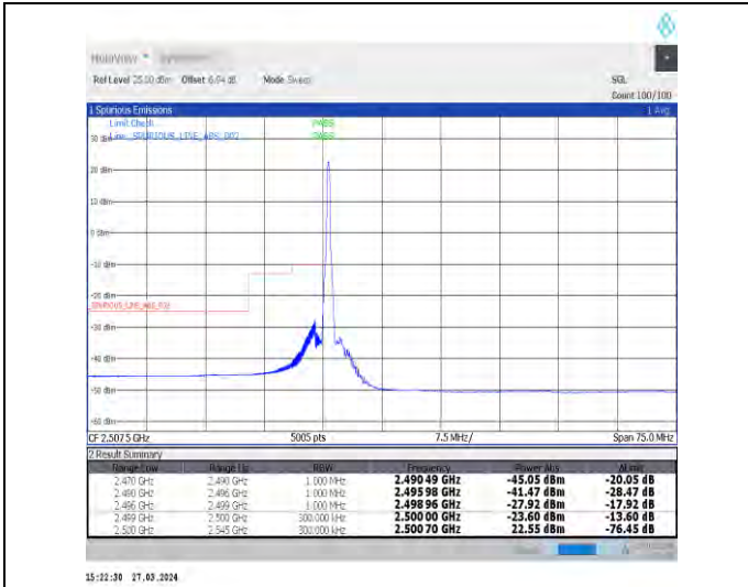
1-N7-15-30-L-1-DFT-PI2BPSK-Edge_1RB_Left-1@0-A nt1-1--PASS-see graph
