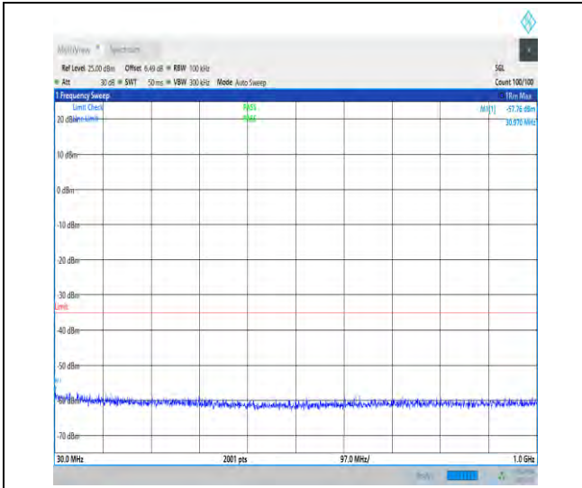
1-N7-15-40-M-1-DFT-PI2BPSK-Inner_1RB_Left-1@ 1-30-1000-Ant1-30.00--57.76--35-PASS
