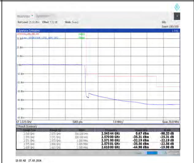
1-N7-15-30-H-6-CP-QPSK-Outer_Full-160@0-Ant 1-1--PASS-see graph
