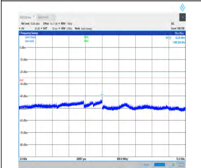
1-N7-15-40-M-1-DFT-PI2BPSK-Inner_1RB_Left-1@ 1-3000-12000-Ant1-7449.60--42.29--25-PASS
