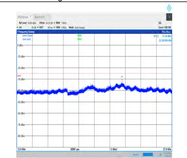
1-N7-15-40-L-1-DFT-PI2BPSK-Inner_1RB_Left-1@1- 12000-27000-Ant1-22217.00--31.25--25-PASS
