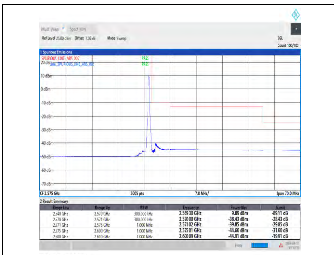
1-N7-15-30-H-2-DFT-PI2BPSK-Edge_1RB_Right-1@159-Ant1-1--PASS-see graph
