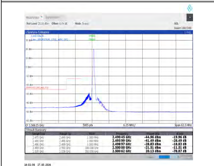
1-N7-15-25-L-4-CP-QPSK-Edge_1RB_Left-1@0-Ant1-1--PASS-see graph
