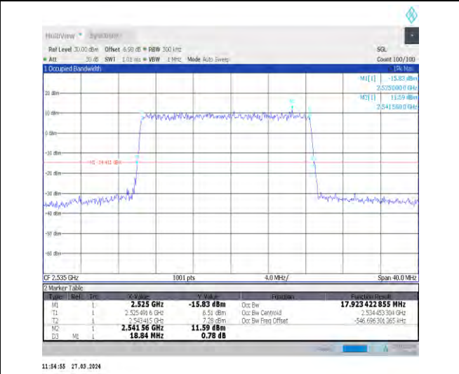
1-N7-15-20-M-5-DFT-256QAM-Outer_Full-100@0-A nt1-17.923-18.840-≤20-PASS
