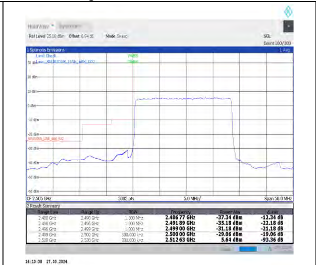
1-N7-15-20-L-3-DFT-PI2BPSK-Outer_Full-100@0 -Ant1-1--PASS-see graph
