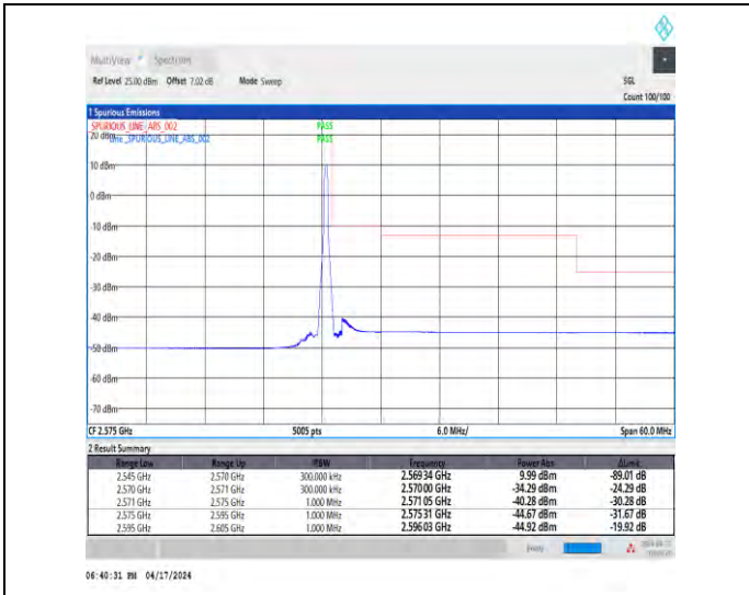
1-N7-15-25-H-2-DFT-PI2BPSK-Edge_1RB_Right-1@1 32-Ant1-1--PASS-see graph
