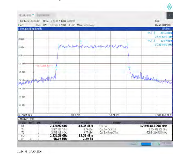
1-N7-15-20-M-3-DFT-16QAM-Outer_Full-100@0-Ant 1-17.895-18.920-≤20-PASS
