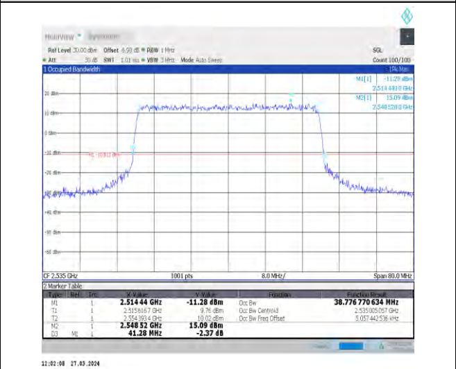
1-N7-15-40-M-6-CP-QPSK-Outer_Full-216@0-Ant1 38.777-41.280-≤40-PASS
