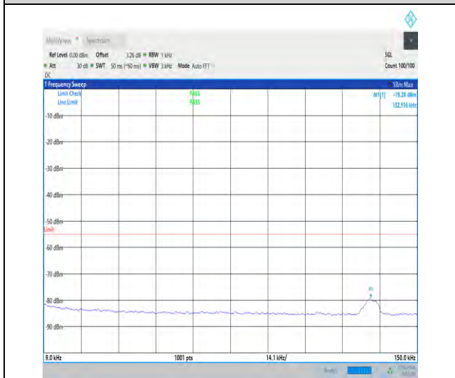
1-N7-15-40-M-1-DFT-PI2BPSK-Inner_1RB_Left-1@ 1-0.009-0.15-Ant1-0.13--79.28--55-PASS
