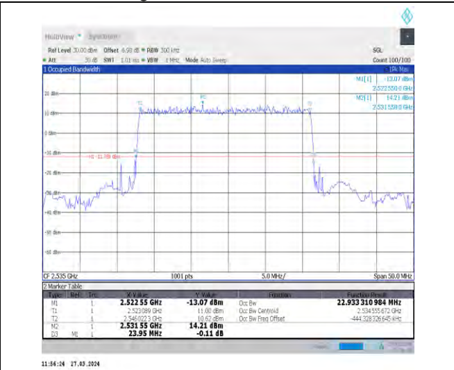
1-N7-15-25-M-2-DFT-PI2BPSK-Outer_Full-128@0-Ant1 nt1-22.933-23.950-≤25-PASS
