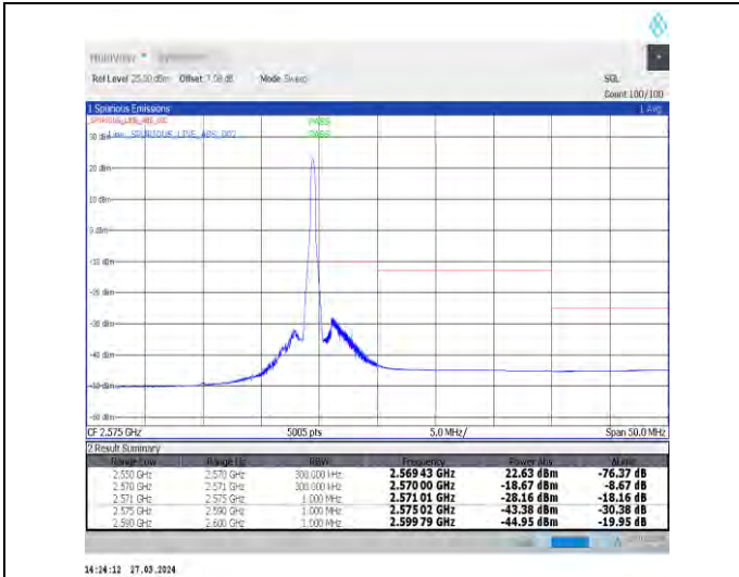
1-N7-15-20-H-2-DFT-PI2BPSK-Edge_1RB_Right-1@105-Ant1-1--PASS-see graph
