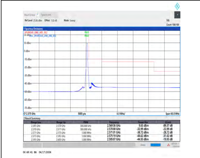
1-N7-15-25-H-5-CP-QPSK-Edge_1RB_Right-1@132-A nt1-1--PASS-see graph
