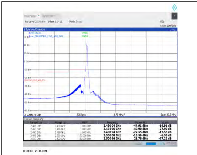
1-N7-15-15-L-1-DFT-PI2BPSK-Edge_1RB_Left-1@0-A nt1-1--PASS-see graph
