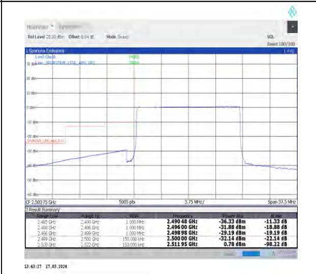
1-N7-15-15-L-6-CP-QPSK-Outer_Full-79@0-Ant1-1--PASS-see graph
