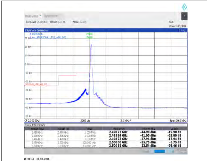
1-N7-15-20-L-1-DFT-PI2BPSK-Edge_1RB_Left-1@0-A nt1-1--PASS-see graph
