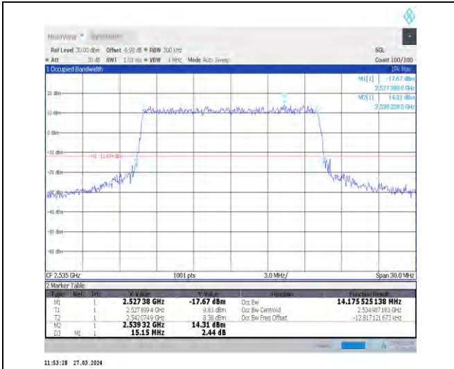
1-N7-15-15-M-7-CP-16QAM-Outer_Full-79@0-Ant1-14.176-15.150-≤15-PASS
