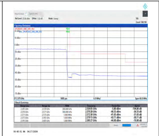
1-N7-15-25-H-3-DFT-PI2BPSK-Outer_Full-128@0 -Ant1-1--PASS-see graph
