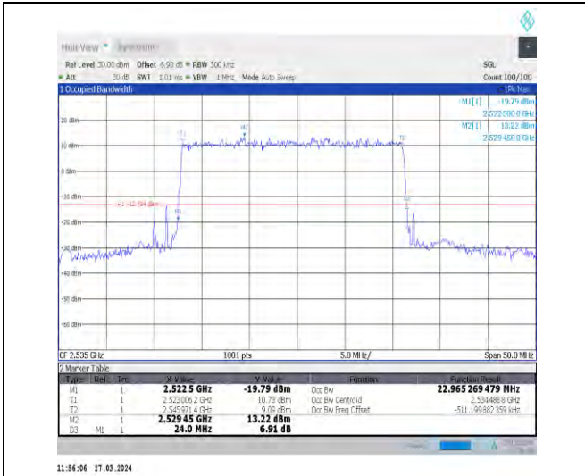
1-N7-15-25-M-1-DFT-QPSK-Outer_Full-128@0-Ant1 -22.965-24.000-≤25-PASS
