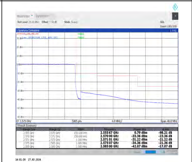
1-N7-15-15-H-6-CP-QPSK-Outer_Full-79@0-Ant1-1--PASS-see graph
