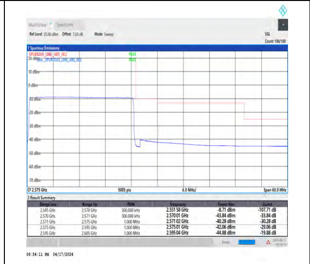
1-N7-15-25-H-6-CP-QPSK-Outer_Full-133@0-Ant 1-1--PASS-see graph
