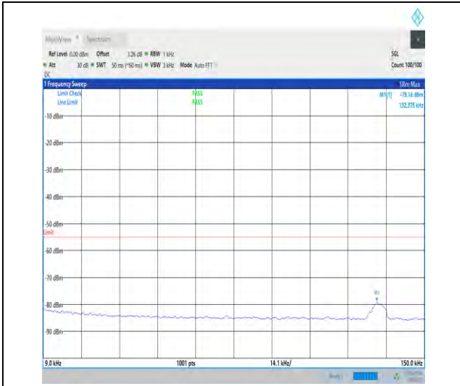
1-N7-15-40-H-1-DFT-PI2BPSK-Inner_1RB_Left-1@ 1-0.009-0.15-Ant1-0.13--79.16--55-PASS
