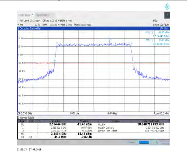
1-N7-15-40-M-8-CP-64QAM-Outer_Full-216@0-Ant1 -38.849-41.200-≤40-PASS
