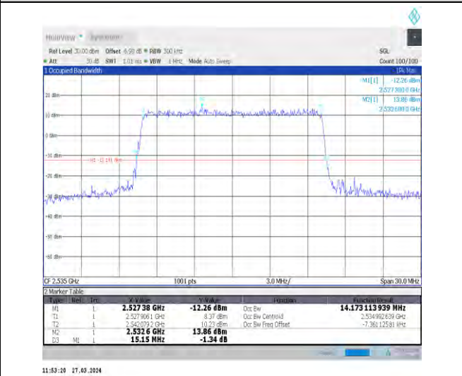
1-N7-15-15-M-6-CP-QPSK-Outer_Full-79@0-Ant1-1 4.173-15.150-≤15-PASS
