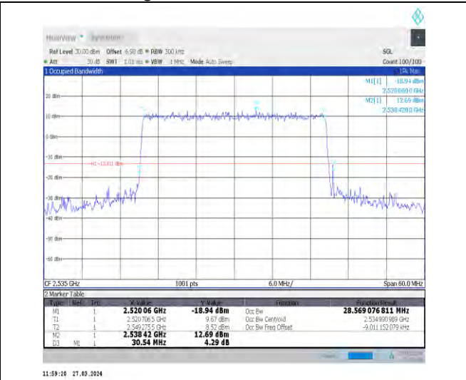
1-N7-15-30-M-1-DFT-QPSK-Outer_Full-160@0-Ant1 -28.57-30.540-≤30-PASS
