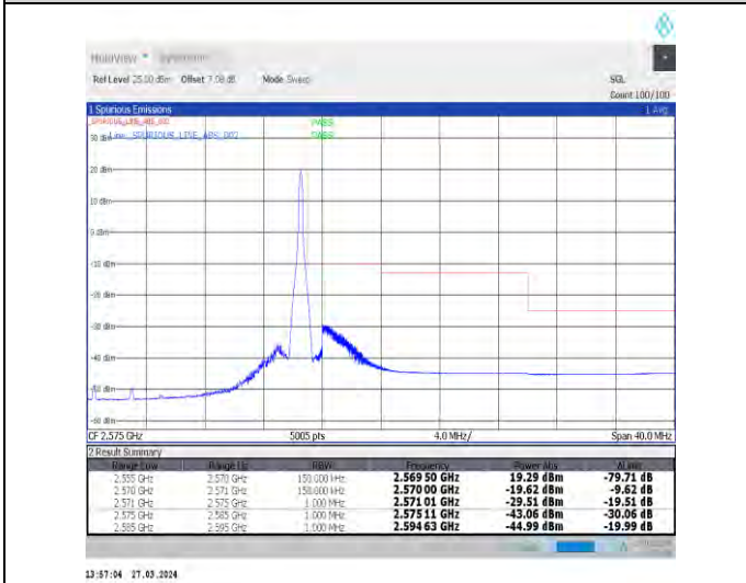
1-N7-15-15-H-5-CP-QPSK-Edge_1RB_Right-1@78-Ant1-1--PASS-see graph
