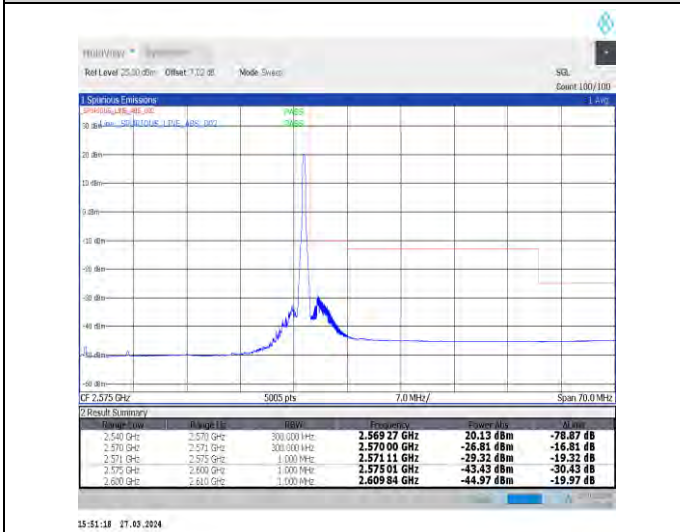
1-N7-15-30-H-5-CP-QPSK-Edge_1RB_Right-1@159-A nt1-1--PASS-see graph
