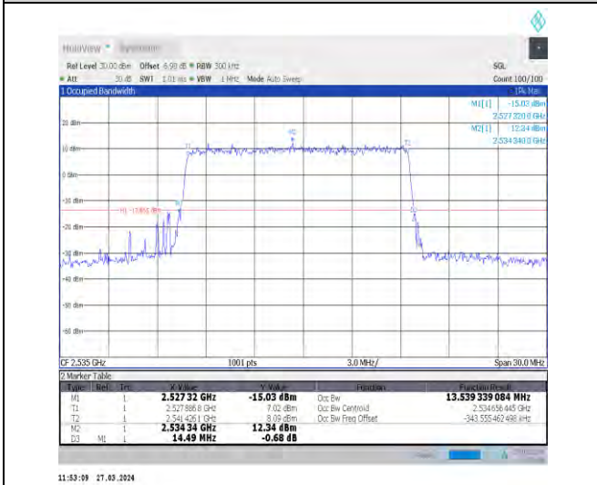
1-N7-15-15-M-5-DFT-256QAM-Outer_Full-75@0-Ant 1-13.539-14.490-≤15-PASS
