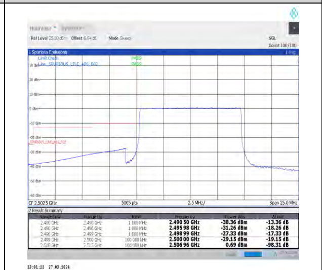
1-N7-15-10-L-6-CP-QPSK-Outer_Full-52@0-Ant1-1--PASS-see graph
