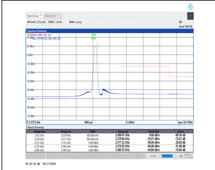
1-N7-15-15-H-5-CP-QPSK-Edge_1RB_Right-1@78-An t1-1--PASS-see graph
