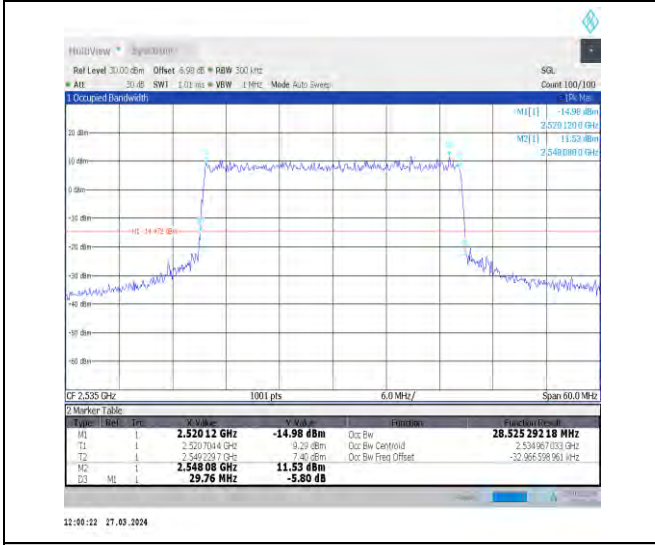
1-N7-15-30-M-6-CP-QPSK-Outer_Full-160@0-Ant1- 28.524-29.760-≤30-PASS
