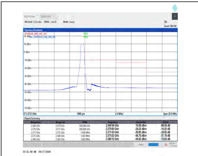
1-N7-15-10-H-2-DFT-PI2BPSK-Edge_1RB_Right-1@5 1-Ant1-1--PASS-see graph
