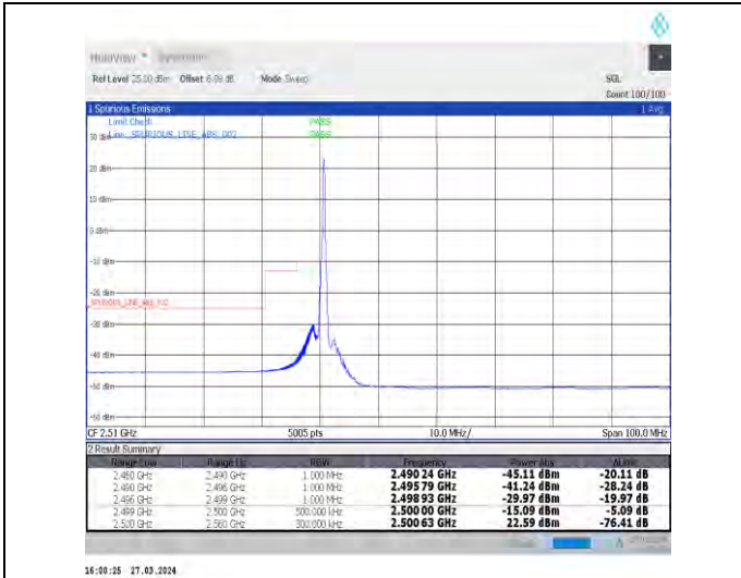
1-N7-15-40-L-1-DFT-PI2BPSK-Edge_1RB_Left-1@0-A nt1-1--PASS-see graph
