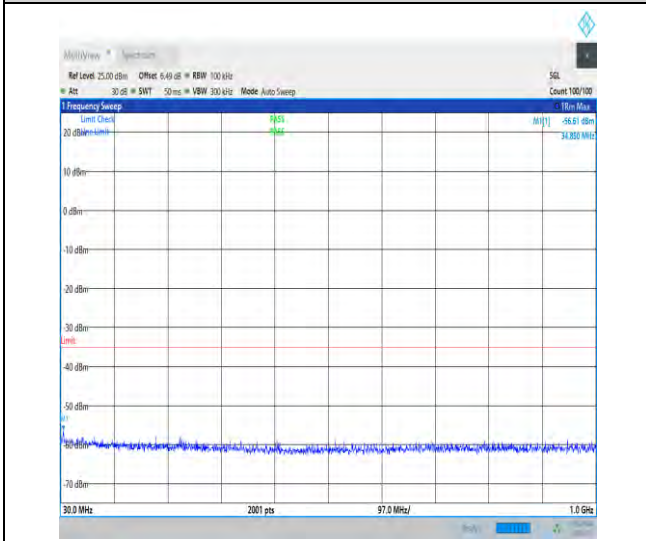
1-N7-15-40-H-1-DFT-PI2BPSK-Inner_1RB_Left-1@ 1-30-1000-Ant1-33.40--56.61--35-PASS
