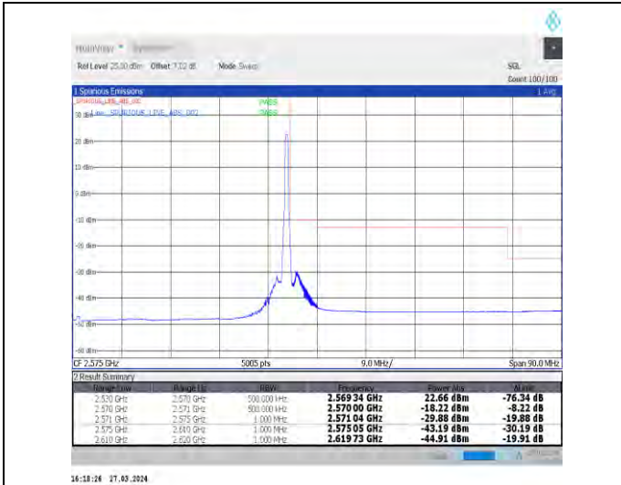
1-N7-15-40-H-2-DFT-PI2BPSK-Edge_1RB_Right-1@2 15-Ant1-1--PASS-see graph
