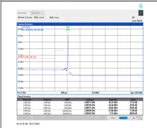
1-N7-15-40-L-4-CP-QPSK-Edge_1RB_Left-1@0-Ant1-1--PASS-see graph
