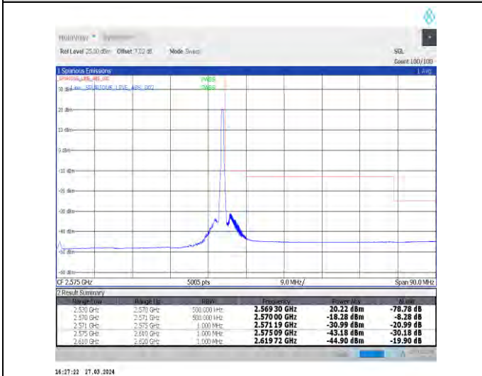
1-N7-15-40-H-5-CP-QPSK-Edge_1RB_Right-1@215-A nt1-1--PASS-see graph
