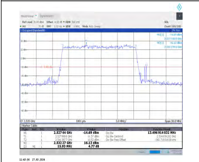
1-N7-15-15-M-1-DFT-QPSK-Outer_Full-75@0-Ant1-13.497-15.930-≤15-PASS
