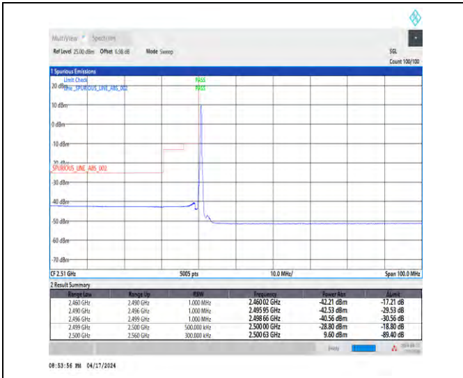
1-N7-15-40-L-1-DFT-PI2BPSK-Edge_1RB_Left-1@0-Ant1-1--PASS-see graph
