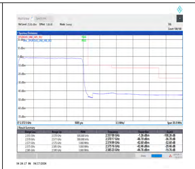
1-N7-15-15-H-3-DFT-PI2BPSK-Outer_Full-75@0- Ant1-1--PASS-see graph
