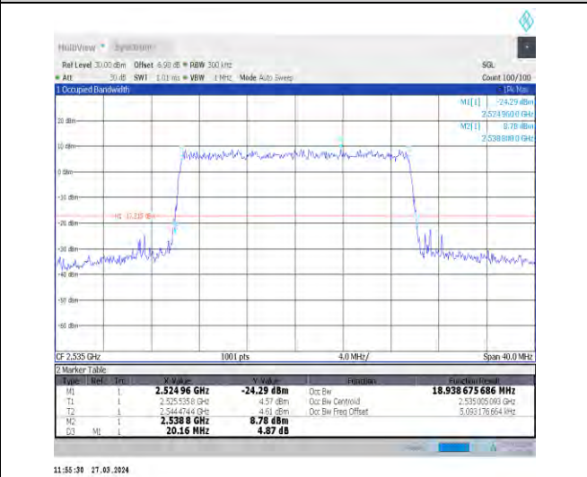
1-N7-15-20-M-9-CP-256QAM-Outer_Full-106@0-Ant1-18.939-20.160-≤20-PASS
