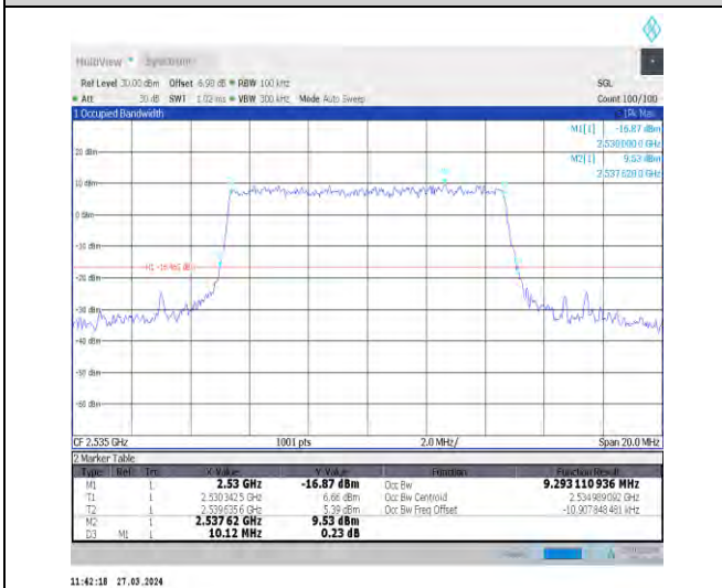
1-N7-15-10-M-6-CP-QPSK-Outer_Full-52@0-Ant1-9. 293-10.120-≤10-PASS
