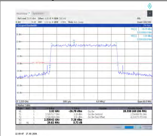
1-N7-15-30-M-9-CP-256QAM-Outer_Full-160@0-Ant1 1-28.559-29.820-≤30-PASS
