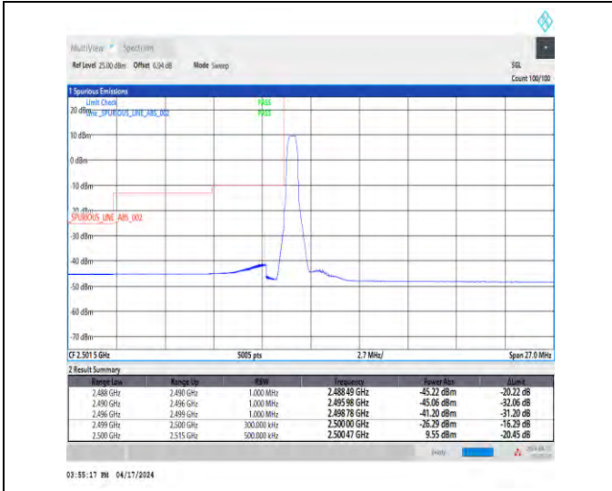
1-N7-15-15-L-1-DFT-PI2BPSK-Edge_1RB_Left-1@0-Ant1-1--PASS-see graph
