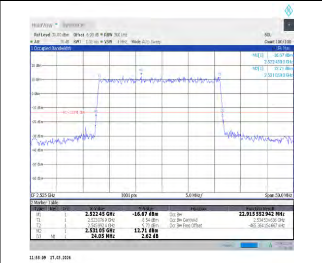
1-N7-15-25-M-4-DFT-64QAM-Outer_Full-128@0-Ant1 1-22.916-24.050-≤25-PASS
