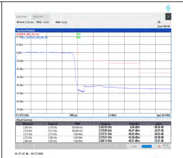
1-N7-15-10-H-3-DFT-PI2BPSK-Outer_Full-50@0-Ant1-1--PASS-see graph
