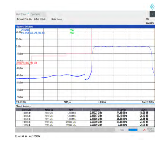
1-N7-15-10-L-3-DFT-PI2BPSK-Outer_Full-50@0-Ant1-1--PASS-see graph
