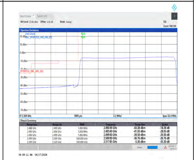
1-N7-15-20-L-6-CP-QPSK-Outer_Full-106@0-Ant1-1--PASS-see graph
