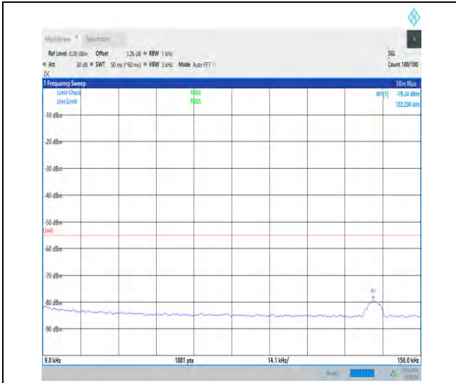
1-N7-15-40-H-1-DFT-PI2BPSK-Inner_1RB_Left-1@ 1-0.009-0.15-Ant1-0.13--79.24--55-PASS
