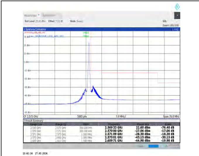
1-N7-15-30-H-2-DFT-PI2BPSK-Edge_1RB_Right-1@1 59-Ant1-1--PASS-see graph
