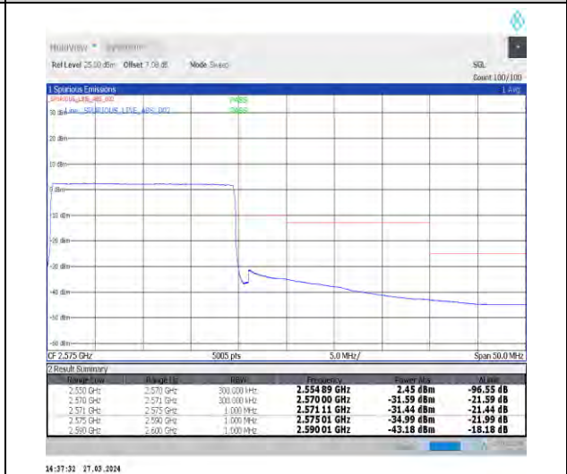
1-N7-15-20-H-6-CP-QPSK-Outer_Full-106@0-Ant1-1--PASS-see graph
