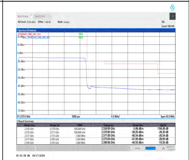
1-N7-15-20-H-6-CP-QPSK-Outer_Full-106@0-Ant 1-1--PASS-see graph
