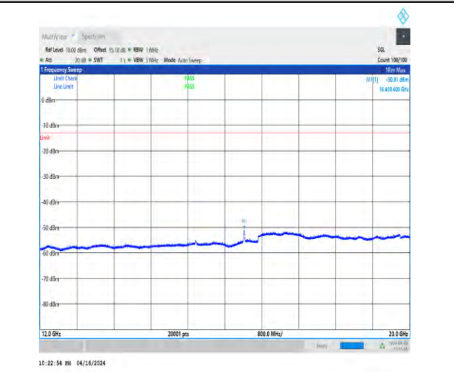
1-N5-15-20-M-1-DFT-QPSK-Edge_1RB_Left-1@0-12 000-20000-Ant1-16418.40--50.81--13-PASS
