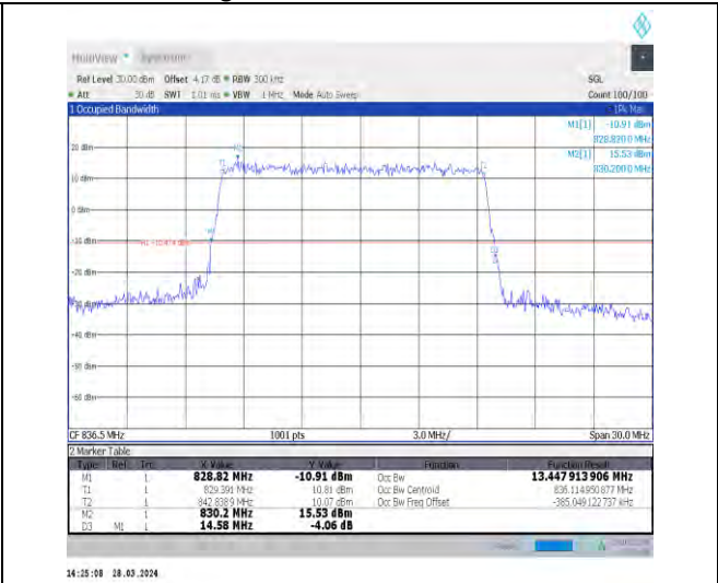
1-N5-15-15-M-4-DFT-64QAM-Outer_Full-75@0-Ant1 -13.448-14.580-≤15-PASS
