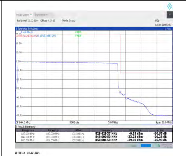
1-N5-15-20-H-6-CP-QPSK-Outer_Full-106@0-Ant1-1--PASS-see graph
