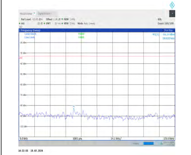
1-N5-15-20-H-1-DFT-PI2BPSK-Inner_1RB_Left-1@1 -0.009-0.15-Ant1-0.06--84.14--33-PASS
