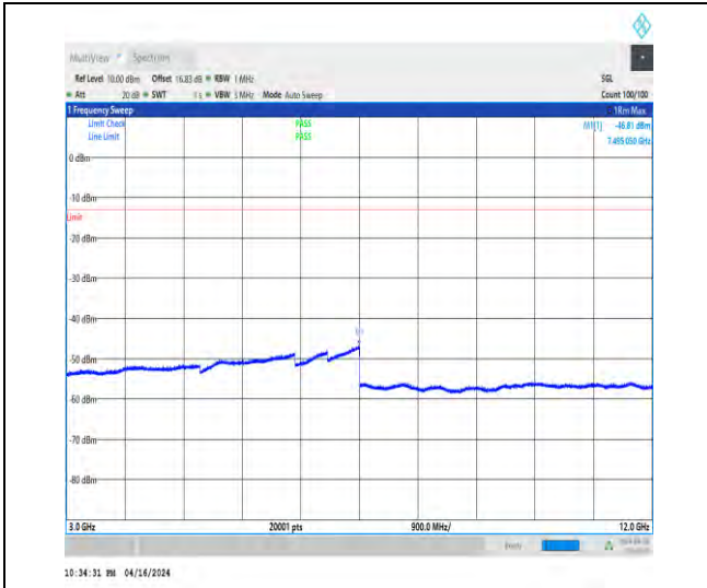
1-N5-15-20-H-1-DFT-QPSK-Edge_1RB_Left-1@0-3 000-12000-Ant1-7495.05--46.81--13-PASS
