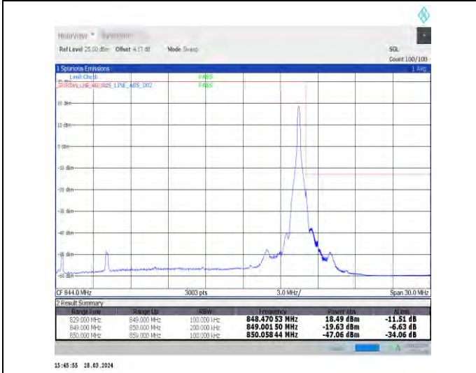
1-N5-15-20-H-5-CP-QPSK-Edge_1RB_Right-1@105-Ant1-1--PASS-see graph
