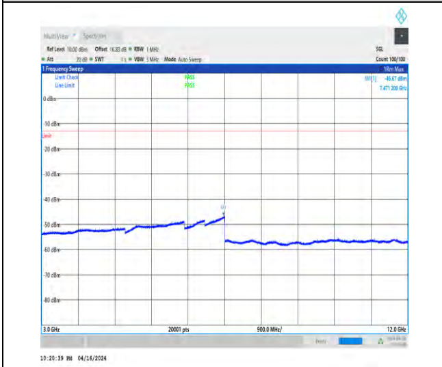
1-N5-15-20-M-1-DFT-QPSK-Edge_1RB_Left-1@0-3 000-12000-Ant1-7471.20--46.67--13-PASS
