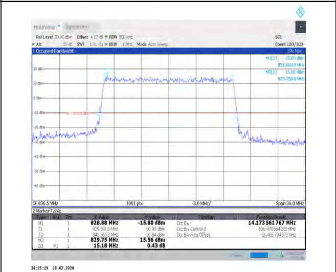
1-N5-15-15-M-6-CP-QPSK-Outer_Full-79@0-Ant1-1 4.174-15.180-≤15-PASS
