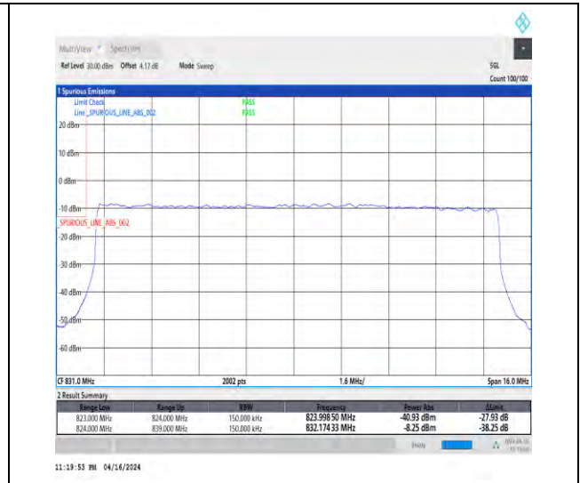
1-N5-15-15-L-3-DFT-PI2BPSK-Outer_Full-75@0-Ant1-1-seegraph-PASS-see graph
