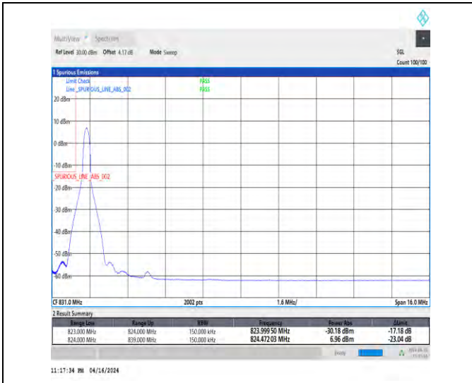
1-N5-15-15-L-1-DFT-PI2BPSK-Edge_1RB_Left-1@0-Ant1-1-seegraph-PASS-see graph
