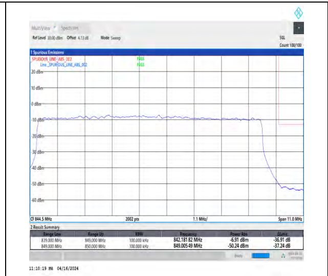
1-N5-15-10-H-3-DFT-PI2BPSK-Outer_Full-50@0-Ant1-1-seegraph-PASS-see graph
