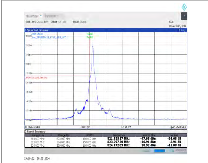
1-N5-15-15-L-4-CP-QPSK-Edge_1RB_Left-1@0-Ant1-1--PASS-see graph
