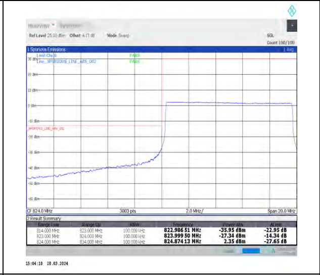
1-N5-15-10-L-6-CP-QPSK-Outer_Full-52@0-Ant1-1--PASS-see graph
