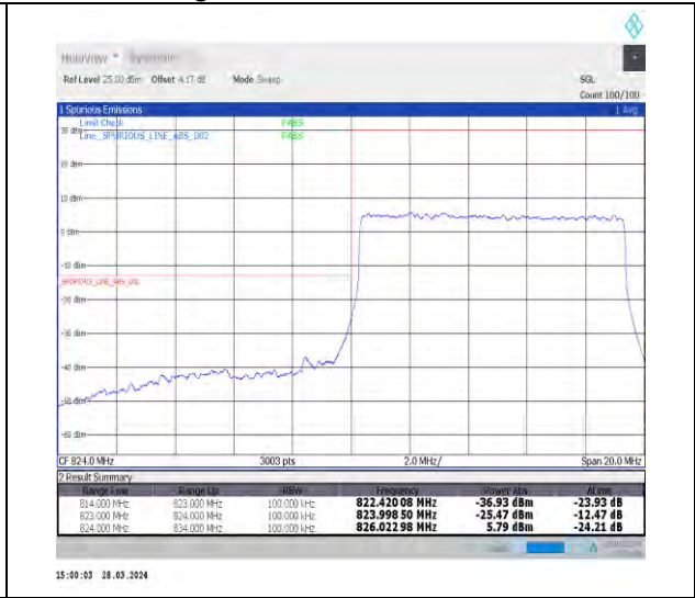
1-N5-15-10-L-3-DFT-PI2BPSK-Outer_Full-50@0-A nt1-1--PASS-see graph
