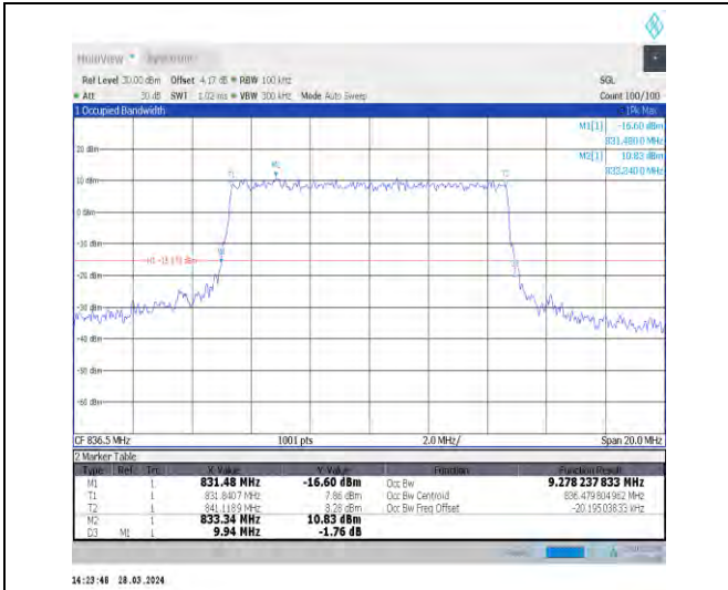
1-N5-15-10-M-8-CP-64QAM-Outer_Full-52@0-Ant1-9.278-9.940-≤10-PASS
