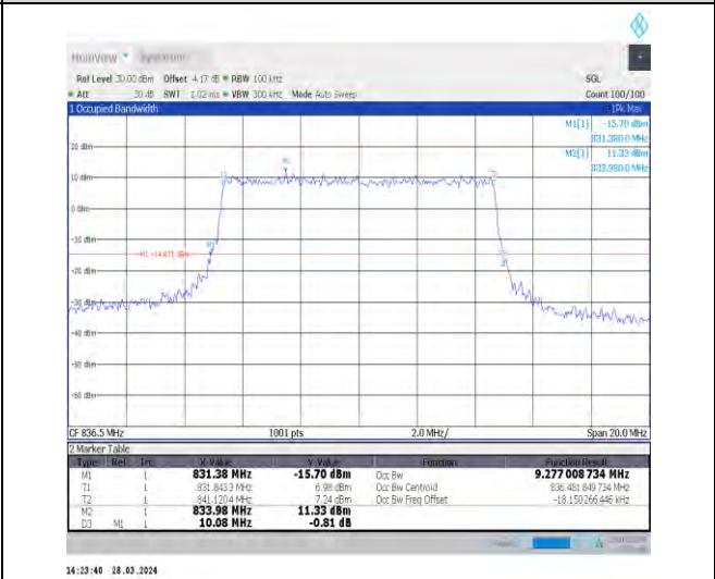
1-N5-15-10-M-7-CP-16QAM-Outer_Full-52@0-Ant1- 9.277-10.080-≤10-PASS
