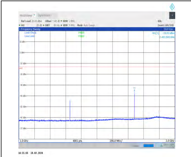
1-N5-15-20-M-1-DFT-PI2BPSK-Inner_1RB_Left-1@ 1-1000-3000-Ant1-2481.50--35.93--13-PASS
