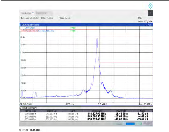
1-N5-15-15-H-5-CP-QPSK-Edge_1RB_Right-1@78-Ant1-1--PASS-see graph
