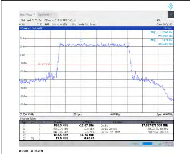
1-N5-15-20-M-4-DFT-64QAM-Outer_Full-100@0-Ant 1-17.918-19.000-≤20-PASS
