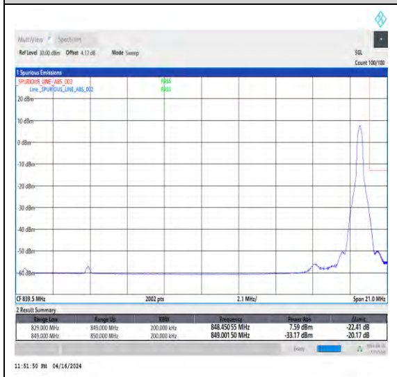
1-N5-15-20-H-5-CP-QPSK-Edge_1RB_Right-1@105-Ant1-1-seegraph-PASS-see graph
