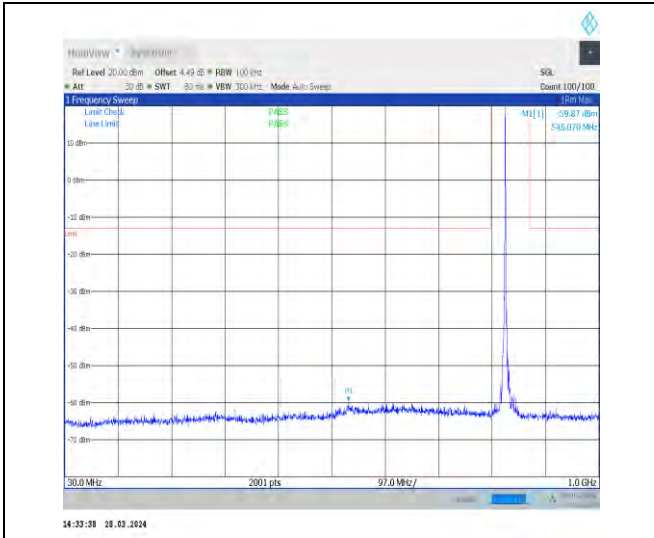
1-N5-15-20-H-1-DFT-PI2BPSK-Inner_1RB_Left-1@1 -30-1000-Ant1-545.07--59.87--13-PASS
