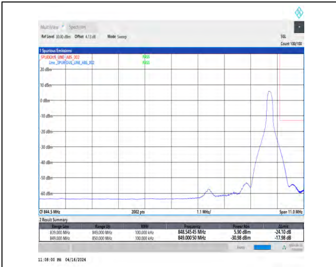
1-N5-15-10-H-2-DFT-PI2BPSK-Edge_1RB_Right-1@5-Ant1-1-seegraph-PASS-see graph
