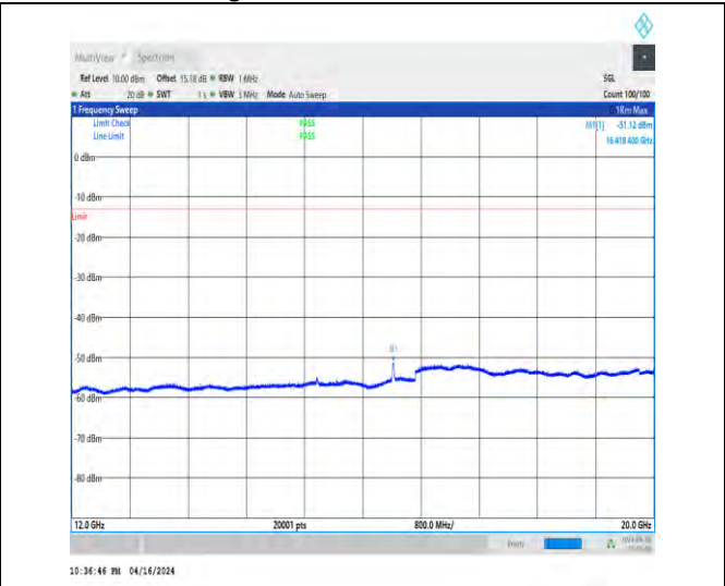
1-N5-15-20-H-1-DFT-QPSK-Edge_1RB_Left-1@0-12 000-20000-Ant1-16418.40--51.12--13-PASS
