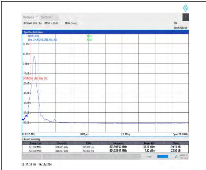
1-N5-15-20-L-1-DFT-PI2BPSK-Edge_1RB_Left-1@0-Ant1-1-seegraph-PASS-see graph
