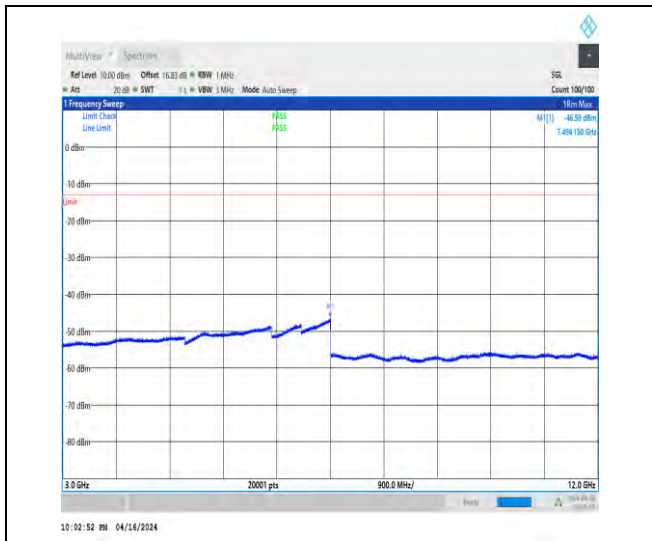
1-N5-15-20-L-1-DFT-QPSK-Edge_1RB_Left-1@0-3 000-12000-Ant1-7494.15--46.59--13-PASS
