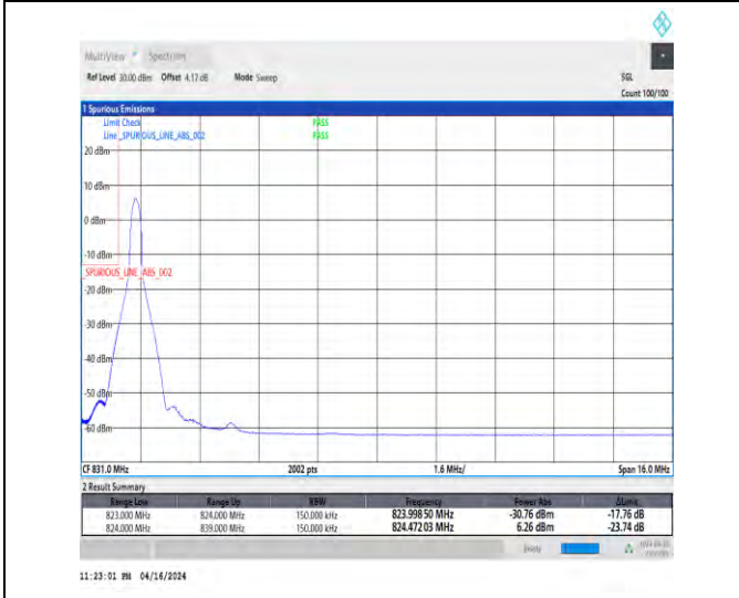
1-N5-15-15-L-4-CP-QPSK-Edge_1RB_Left-1@0-Ant1-1-seegraph-PASS-see graph
