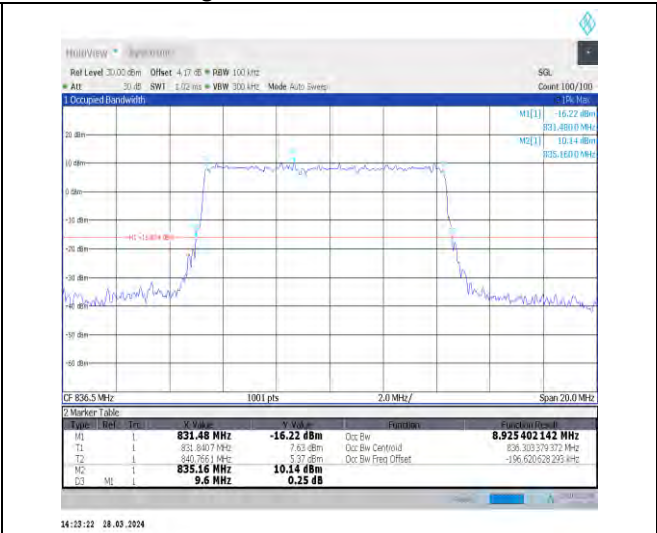
1-N5-15-10-M-5-DFT-256QAM-Outer_Full-50@0-Ant 1-8.925-9.600-≤10-PASS
