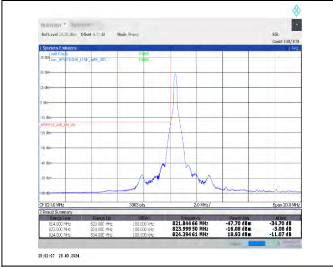
1-N5-15-10-L-4-CP-QPSK-Edge_1RB_Left-1@0-Ant1-1--PASS-see graph
