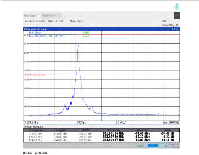
1-N5-15-20-L-4-CP-QPSK-Edge_1RB_Left-1@0-Ant1-1--PASS-see graph
