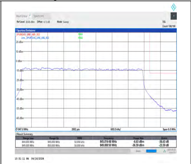
1-N5-15-5-H-3-DFT-PI2BPSK-Outer_Full-25@0-Ant1-1-see graph-PASS-see graph
