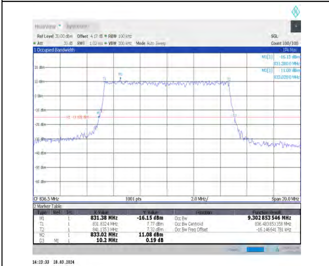
1-N5-15-10-M-6-CP-QPSK-Outer_Full-52@0-Ant1-9. 303-10.200-≤10-PASS
