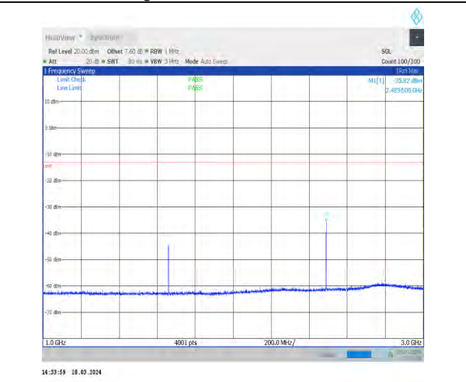
1-N5-15-20-H-1-DFT-PI2BPSK-Inner_1RB_Left-1@1 -1000-3000-Ant1-2489.50--35.82--13-PASS
