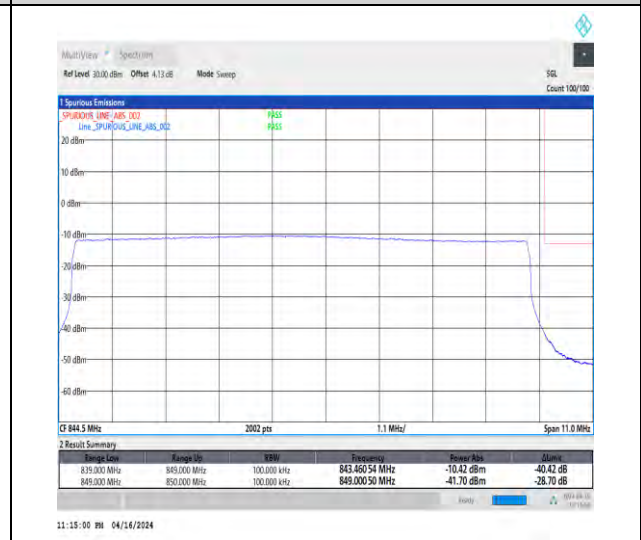
1-N5-15-10-H-6-CP-QPSK-Outer_Full-52@0-Ant1-1-seegraph-PASS-see graph
