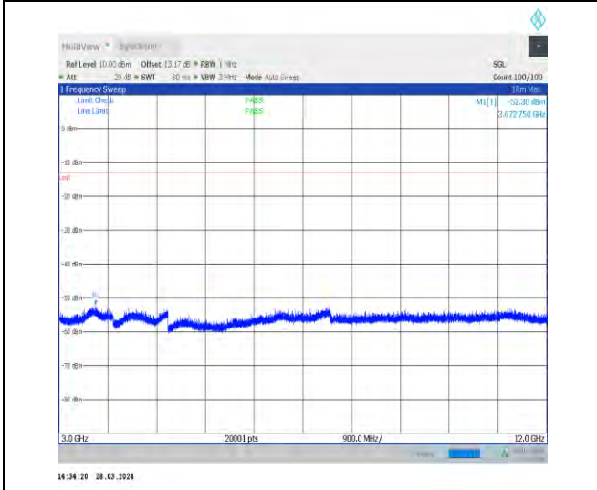
1-N5-15-20-H-1-DFT-PI2BPSK-Inner_1RB_Left-1@1 -3000-12000-Ant1-3672.75--52.30--13-PASS
