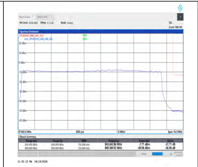
1-N5-15-15-H-3-DFT-PI2BPSK-Outer_Full-75@0-Ant1-1-seegraph-PASS-see graph
