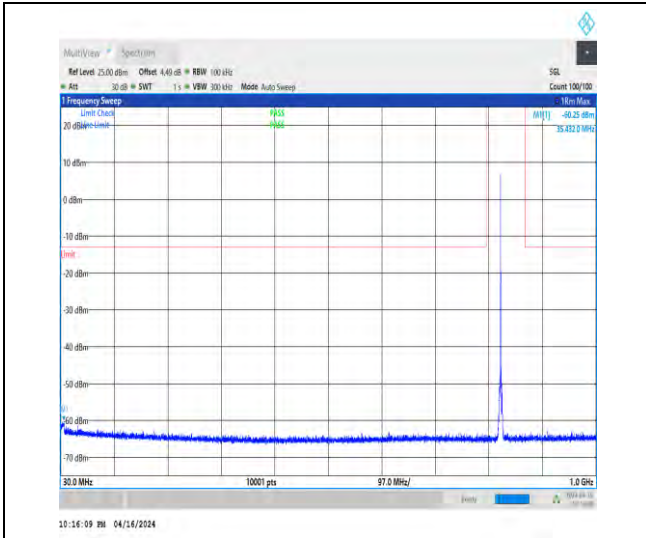
1-N5-15-20-M-1-DFT-QPSK-Edge_1RB_Left-1@0-3 0-1000-Ant1-35.43--60.25--13-PASS
