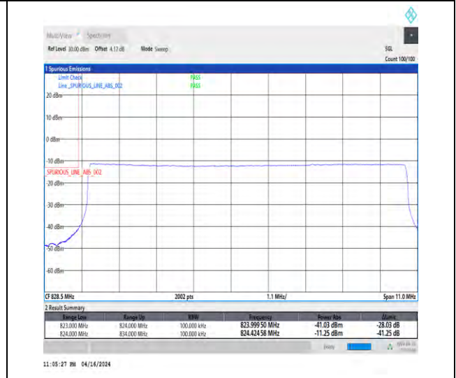
1-N5-15-10-L-6-CP-QPSK-Outer_Full-52@0-Ant1-1-seegraph-PASS-see graph
