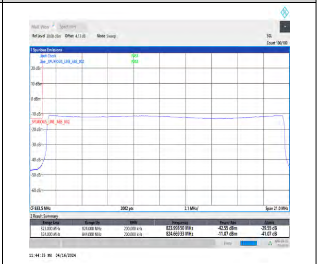
1-N5-15-20-L-6-CP-QPSK-Outer_Full-106@0-Ant1-1-seegraph-PASS-see graph
