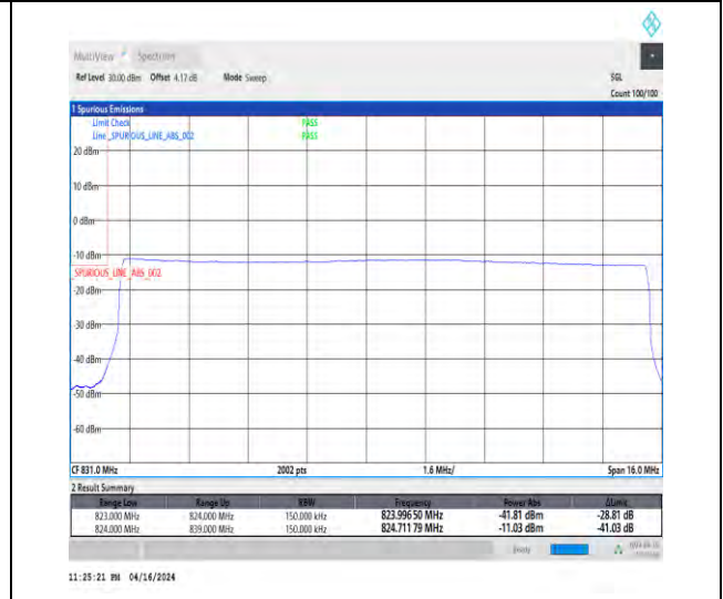
1-N5-15-15-L-6-CP-QPSK-Outer_Full-79@0-Ant1-1-seegraph-PASS-see graph
