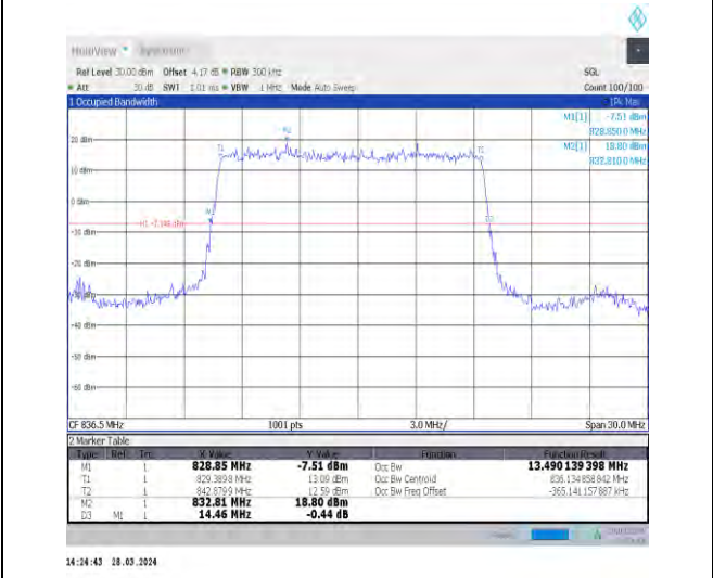
1-N5-15-15-M-2-DFT-PI2BPSK-Outer_Full-75@0-Ant1-13.492-14.550-≤15-PASS
