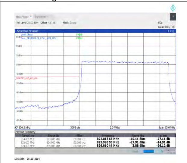
1-N5-15-15-L-3-DFT-PI2BPSK-Outer_Full-75@0-Ant1-1--PASS-see graph
