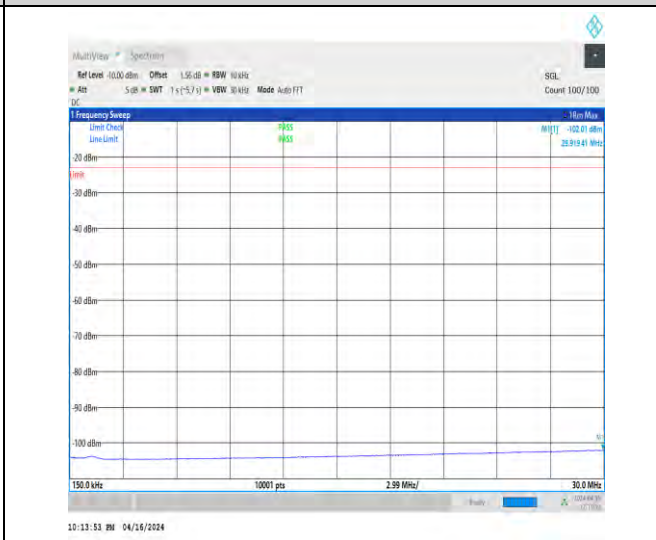
1-N5-15-20-M-1-DFT-QPSK-Edge_1RB_Left-1@0-0. 15-30-Ant1-29.92--102.01--23-PASS
