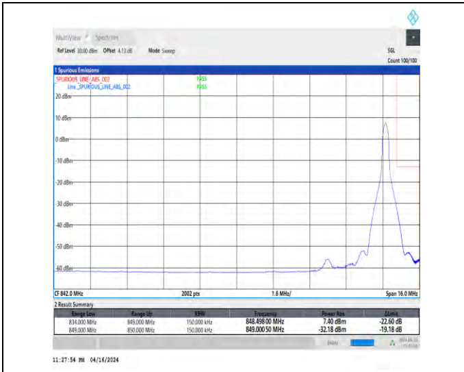
1-N5-15-15-H-2-DFT-PI2BPSK-Edge_1RB_Right-1@7-8-Ant1-1-seegraph-PASS-see graph
