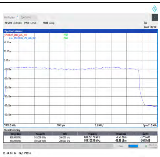
1-N5-15-20-H-3-DFT-PI2BPSK-Outer_Full-100@0-Ant1-1-seegraph-PASS-see graph
