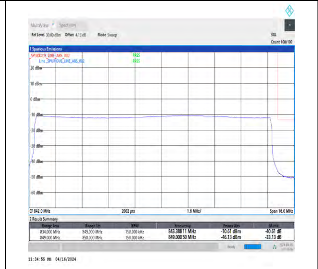
1-N5-15-15-H-6-CP-QPSK-Outer_Full-79@0-Ant1-1-seegraph-PASS-see graph
