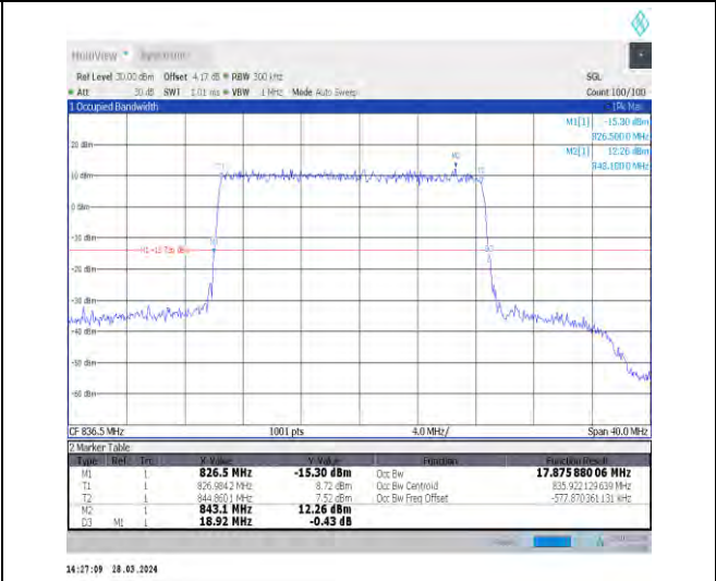
1-N5-15-20-M-5-DFT-256QAM-Outer_Full-100@0-A nt1-17.876-18.920-≤20-PASS
