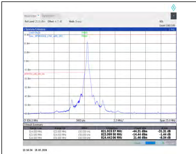
1-N5-15-15-L-1-DFT-PI2BPSK-Edge_1RB_Left-1@0-Ant1-1--PASS-see graph
