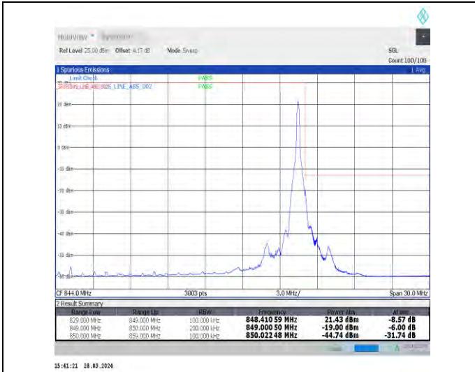
1-N5-15-20-H-2-DFT-PI2BPSK-Edge_1RB_Right-1@105-Ant1-1--PASS-see graph
