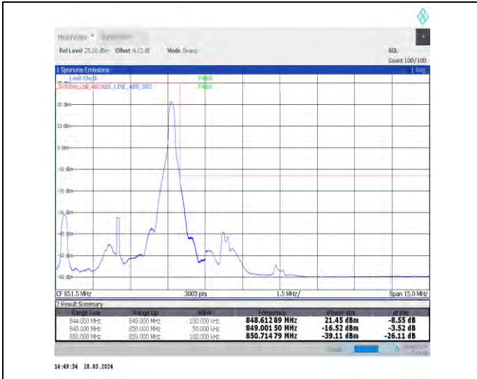
1-N5-15-5-H-2-DFT-PI2BPSK-Edge_1RB_Right-1@24-Ant1-1--PASS-see graph
