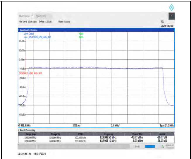
1-N5-15-20-L-3-DFT-PI2BPSK-Outer_Full-100@0-Ant1-1-seegraph-PASS-see graph
