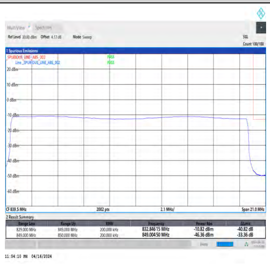
1-N5-15-20-H-6-CP-QPSK-Outer_Full-106@0-Ant1-1-seegraph-PASS-see graph
