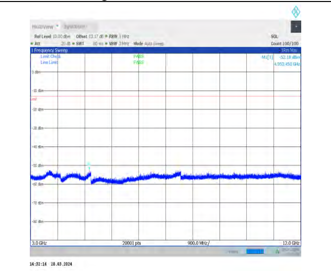
1-N5-15-20-M-1-DFT-PI2BPSK-Inner_1RB_Left-1@ 1-3000-12000-Ant1-4953.45--52.18--13-PASS
