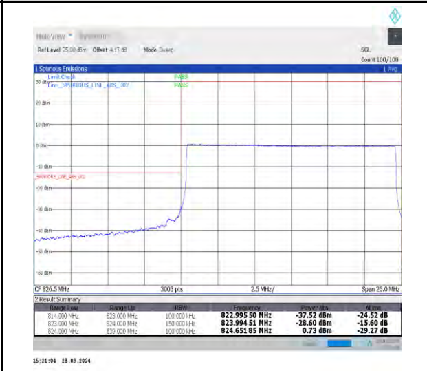
1-N5-15-15-L-6-CP-QPSK-Outer_Full-79@0-Ant1-1--PASS-see graph
