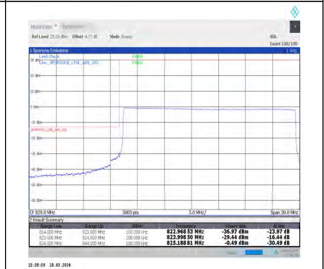
1-N5-15-20-L-6-CP-QPSK-Outer_Full-106@0-Ant 1-1--PASS-see graph
