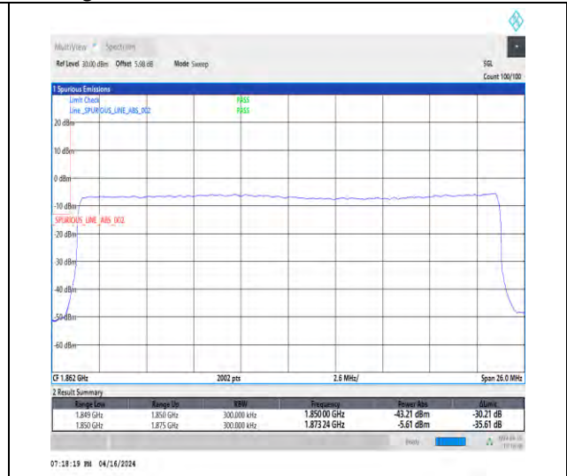
1-N2-15-25-L-3-DFT-PI2BPSK-Outer_Full-128@0-Ant1-1-seegraph-PASS-see graph
