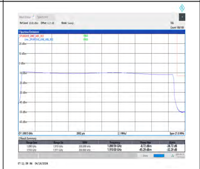
1-N2-15-20-H-6-CP-QPSK-Outer_Full-106@0-Ant1-1-seegraph-PASS-see graph
