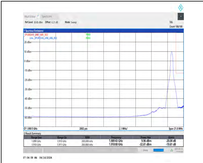
1-N2-15-20-H-2-DFT-PI2BPSK-Edge_1RB_Right-1@105-Ant1-1-seegraph-PASS-see graph
