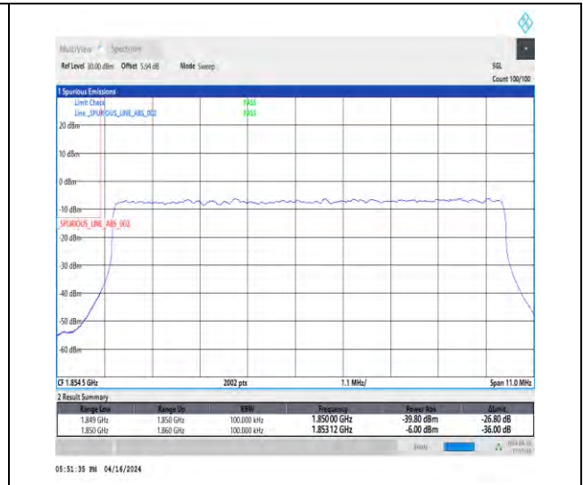
1-N2-15-10-L-3-DFT-PI2BPSK-Outer_Full-50@0-Ant1-1-seegraph-PASS-see graph
