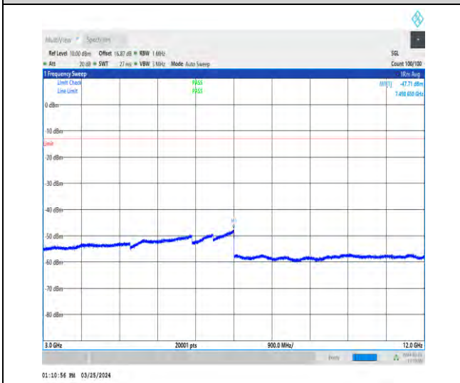
1-N2-15-40-M-1-DFT-PI2BPSK-Inner_1RB_Left-1@ 1-3000-12000-Ant1-7493.70--47.71--13-PASS
