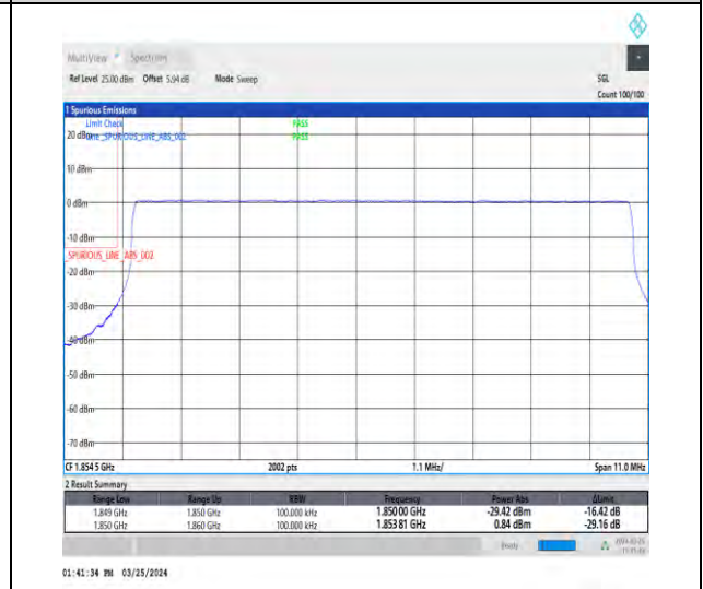
1-N2-15-10-L-6-CP-QPSK-Outer_Full-52@0-Ant1-1-seegraph-PASS-see graph
