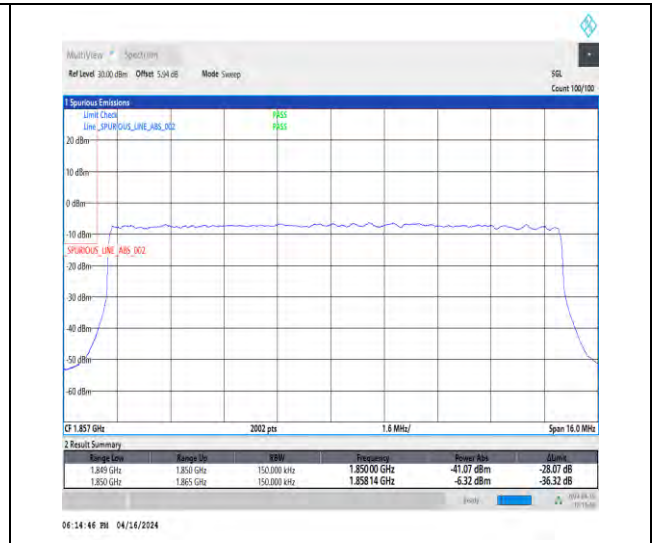
1-N2-15-15-L-3-DFT-PI2BPSK-Outer_Full-75@0-Ant1-1-seegraph-PASS-see graph
