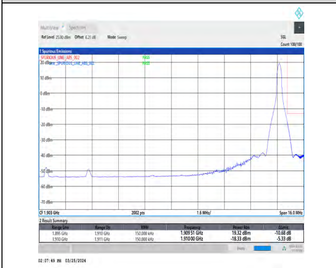
1-N2-15-15-H-5-CP-QPSK-Edge_1RB_Right-1@78-Ant1-1-seegraph-PASS-see graph
