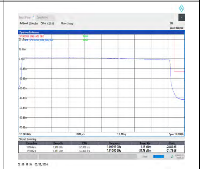
1-N2-15-15-H-6-CP-QPSK-Outer_Full-79@0-Ant1-1-seegraph-PASS-see graph
