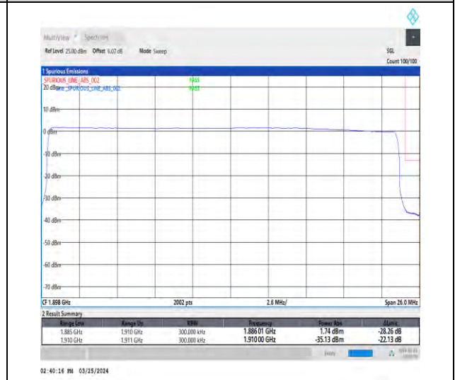
1-N2-15-25-H-6-CP-QPSK-Outer_Full-133@0-Ant 1-1-seegraph-PASS-see graph
