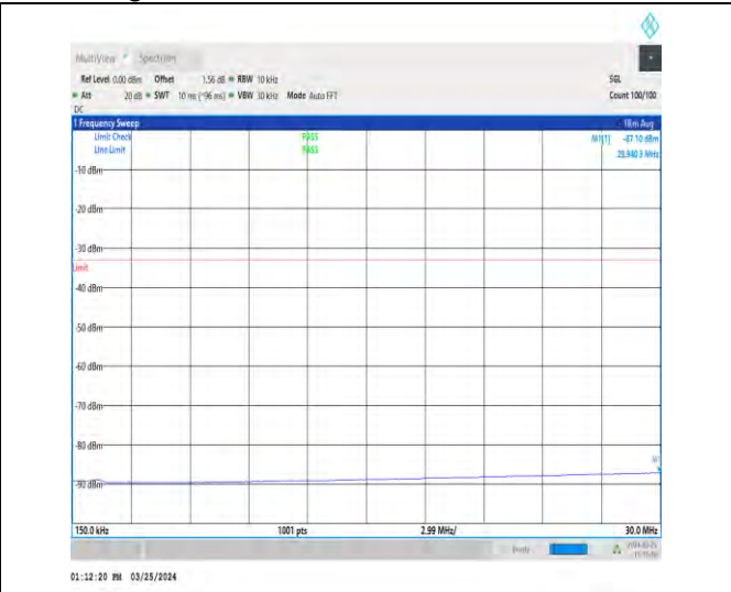
1-N2-15-40-H-1-DFT-PI2BPSK-Inner_1RB_Left-1@ -0.15-30-Ant1-29.94--87.10--33-PASS
