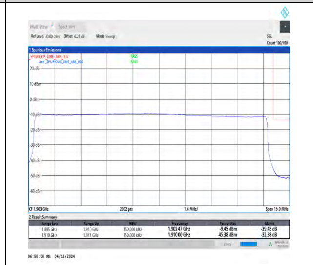
1-N2-15-15-H-6-CP-QPSK-Outer_Full-79@0-Ant1-1-seegraph-PASS-see graph
