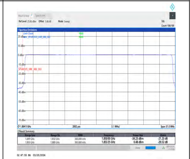
1-N2-15-30-L-6-CP-QPSK-Outer_Full-160@0-Ant1-1-seegraph-PASS-see graph
