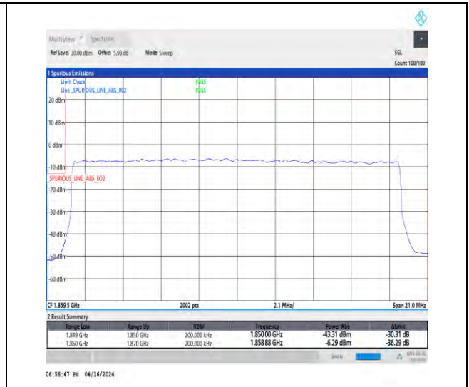
1-N2-15-20-L-3-DFT-PI2BPSK-Outer_Full-100@0-Ant1-1-seegraph-PASS-see graph
