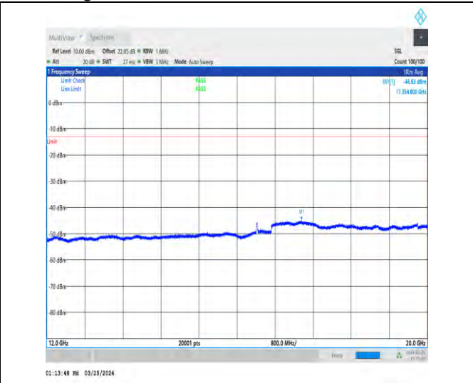
1-N2-15-40-H-1-DFT-PI2BPSK-Inner_1RB_Left-1@ -12000-20000-Ant1-17354.80--44.93--13-PASS
