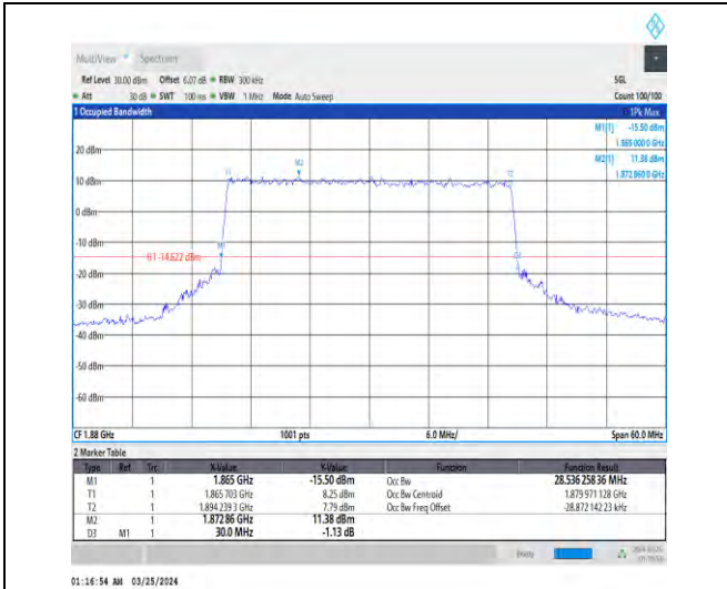
1-N2-15-30-M-8-CP-64QAM-Outer_Full-160@0-Ant1 -28.536-30.000-≤30-PASS
