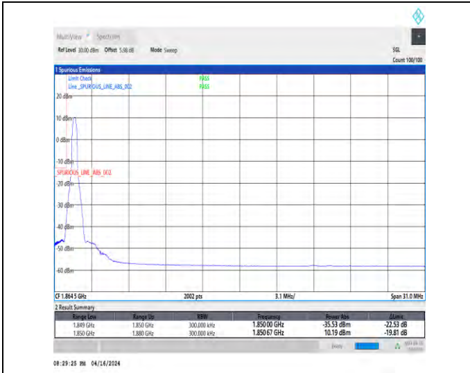
1-N2-15-30-L-1-DFT-PI2BPSK-Edge_1RB_Left-1@0-A nt1-1-seegraph-PASS-see graph
