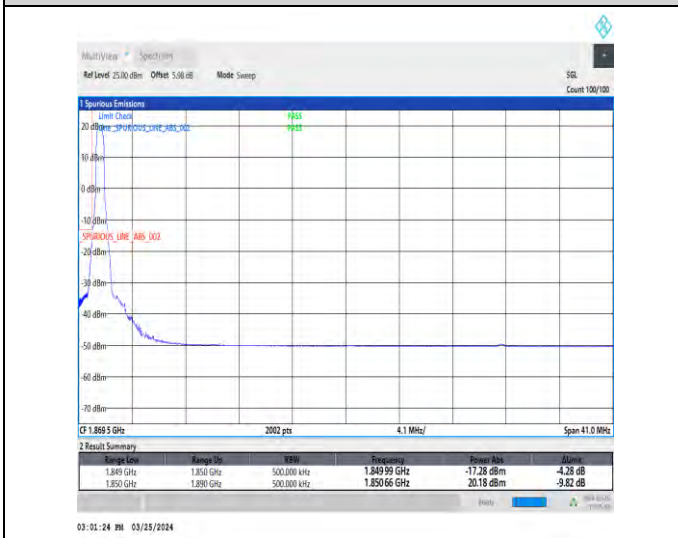
1-N2-15-40-L-4-CP-QPSK-Edge_1RB_Left-1@0-Ant1-1-seegraph-PASS-see graph
