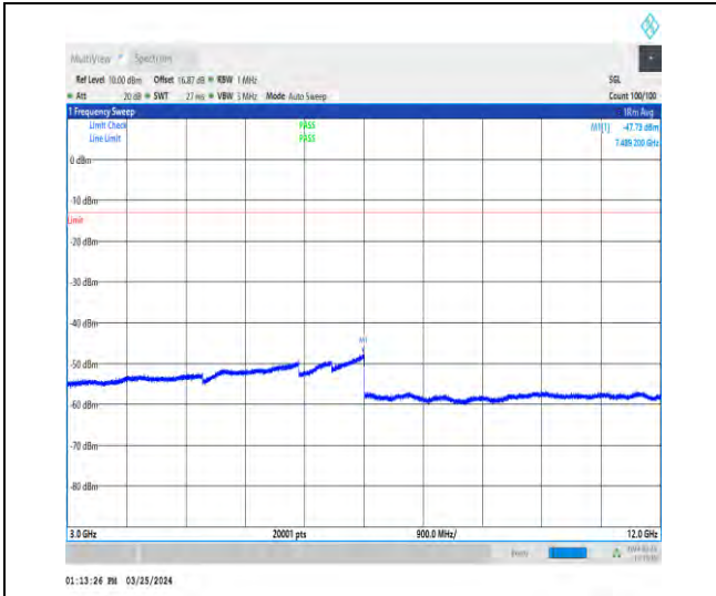
1-N2-15-40-H-1-DFT-PI2BPSK-Inner_1RB_Left-1@ 1-3000-12000-Ant1-7489.20--47.73--13-PASS
