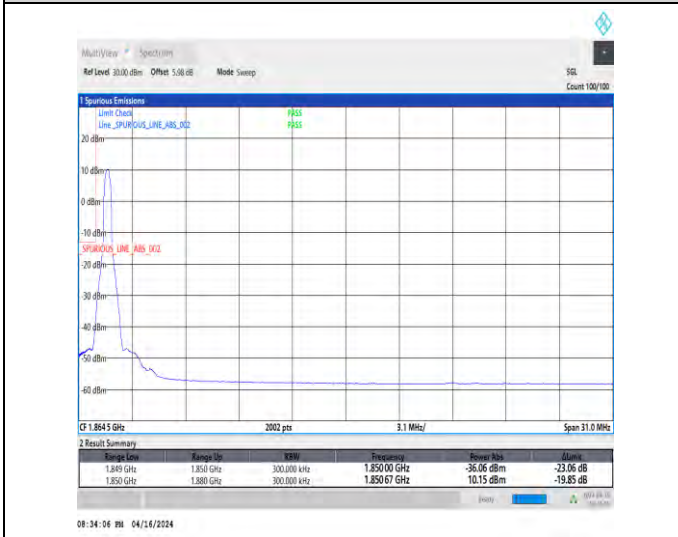
1-N2-15-30-L-4-CP-QPSK-Edge_1RB_Left-1@0-Ant1-1-seegraph-PASS-see graph
