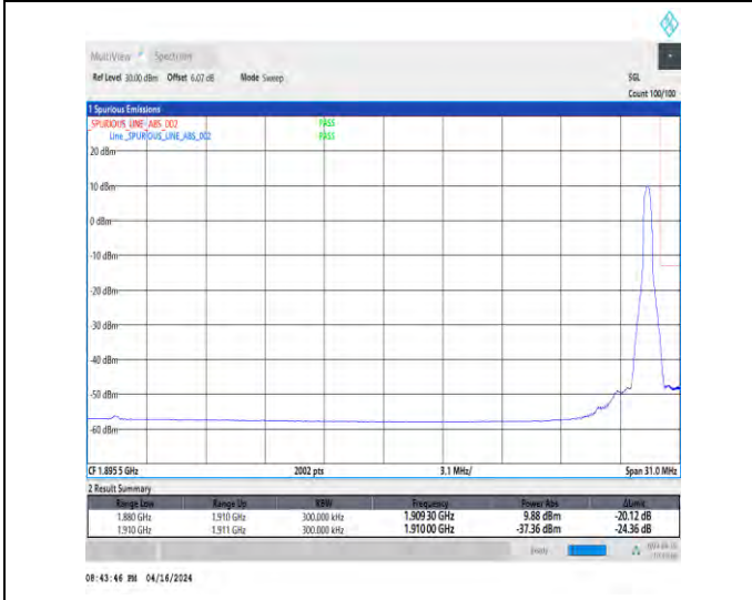
1-N2-15-30-H-5-CP-QPSK-Edge_1RB_Right-1@159-Ant1-1-seegraph-PASS-see graph
