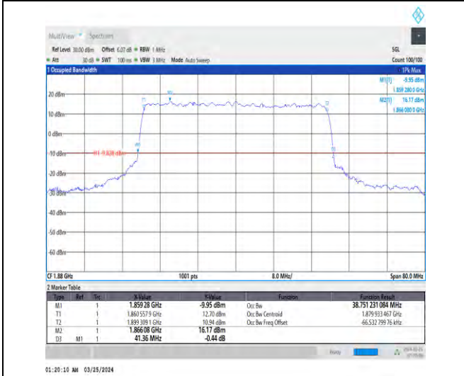
1-N2-15-40-M-7-CP-16QAM-Outer_Full-216@0-Ant1 -38.751-41.360-≤40-PASS
