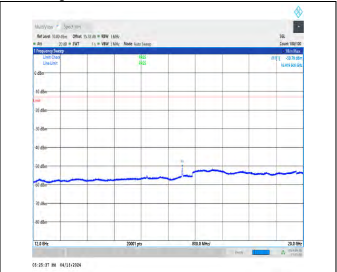
1-N2-15-40-H-1-DFT-QPSK-Edge_1RB_Left-1@0-12 000-20000-Ant1-16419.60--50.78--13-PASS
