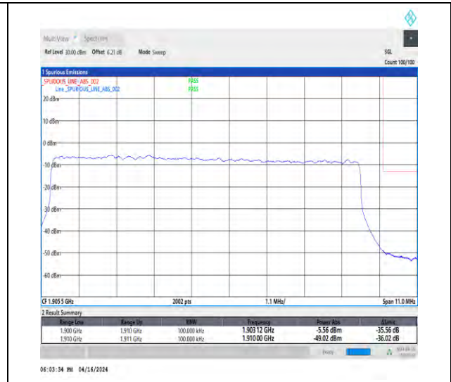
1-N2-15-10-H-3-DFT-PI2BPSK-Outer_Full-50@0- Ant1-1-seegraph-PASS-see graph
