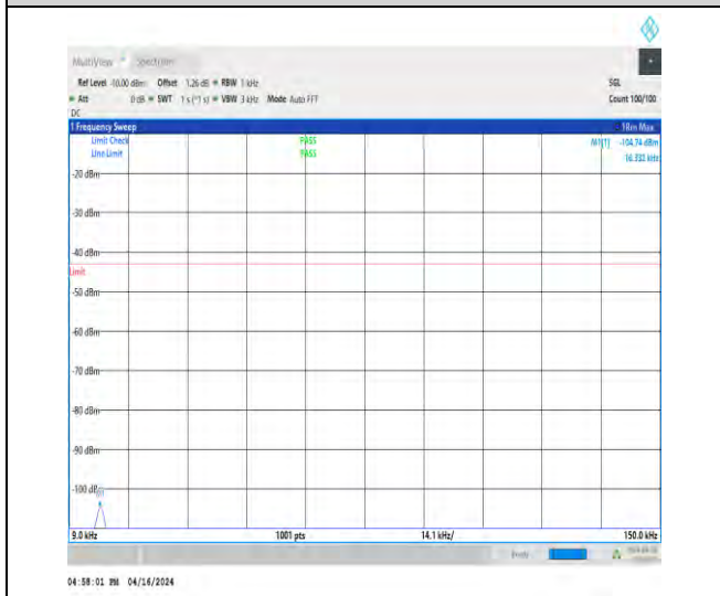
1-N2-15-40-M-1-DFT-QPSK-Edge_1RB_Left-1@0-0 .009-0.15-Ant1-0.02--104.74--43-PASS
