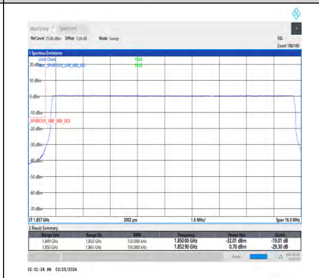
1-N2-15-15-L-6-CP-QPSK-Outer_Full-79@0-A nt1-1-seegraph-PASS-see graph
