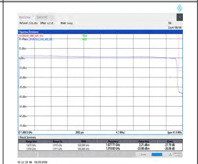
1-N2-15-40-H-6-CP-QPSK-Outer_Full-216@0-Ant 1-1-seegraph-PASS-see graph
