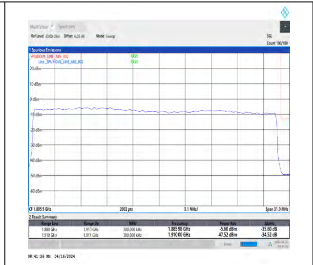
1-N2-15-30-H-3-DFT-PI2BPSK-Outer_Full-160@0-Ant1-1-seegraph-PASS-see graph
