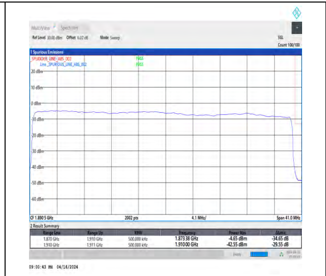
1-N2-15-40-H-3-DFT-PI2BPSK-Outer_Full-216@0-Ant1-1-seegraph-PASS-see graph
