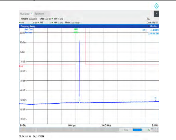
1-N2-15-40-M-1-DFT-QPSK-Edge_1RB_Left-1@0-10 00-3000-Ant1-2949.60--51.29--13-PASS
