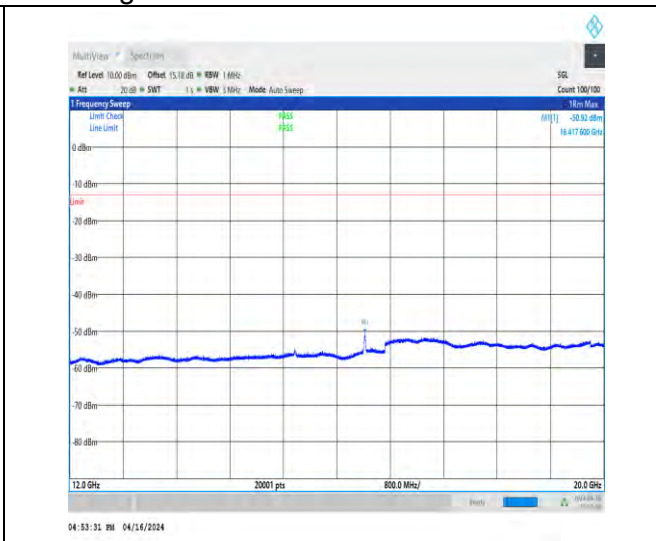
1-N2-15-40-L-1-DFT-QPSK-Edge_1RB_Left-1@0-12 000-20000-Ant1-16417.60--50.92--13-PASS
