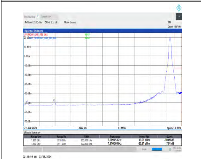
1-N2-15-20-H-5-CP-QPSK-Edge_1RB_Right-1@105-Ant1-1-seegraph-PASS-see graph
