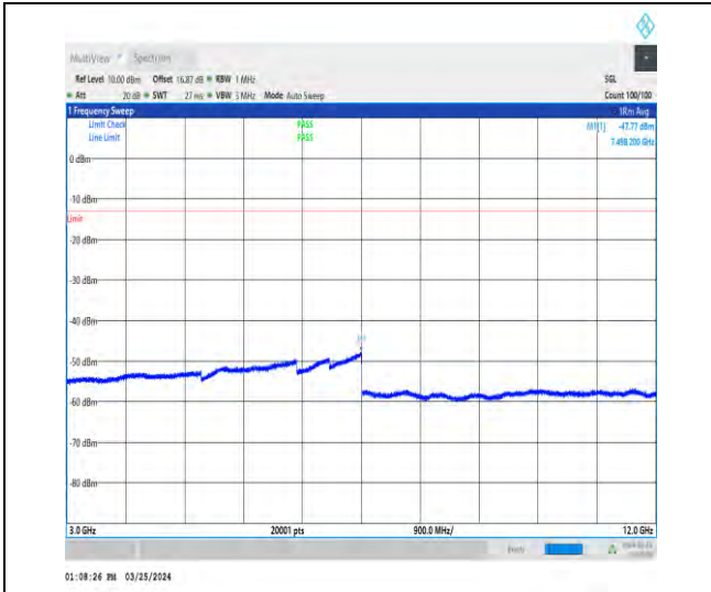
1-N2-15-40-L-1-DFT-PI2BPSK-Inner_1RB_Left-1@ 1-3000-12000-Ant1-7428.45--47.77--13-PASS
