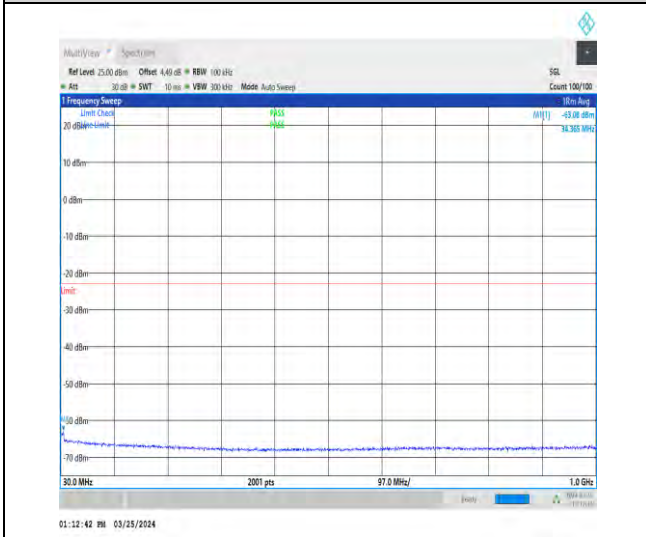
1-N2-15-40-H-1-DFT-PI2BPSK-Inner_1RB_Left-1@ 1-30-1000-Ant1-34.37--63.08--23-PASS
