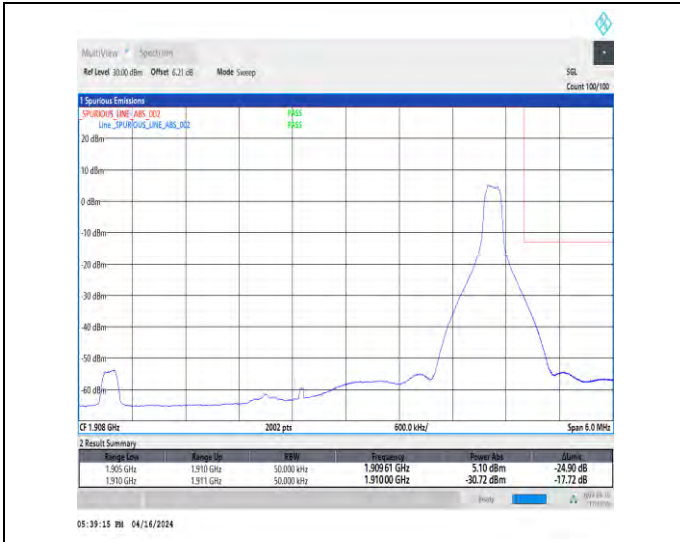
1-N2-15-5-H-2-DFT-PI2BPSK-Edge_1RB_Right-1@24-Ant1-1-see graph-PASS-see graph
