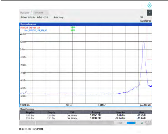
1-N2-15-25-H-5-CP-QPSK-Edge_1RB_Right-1@132-Ant1-1-seegraph-PASS-see graph
