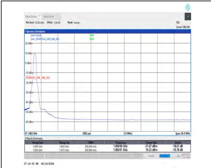
1-N2-15-25-L-1-DFT-PI2BPSK-Edge_1RB_Left-1@0-Ant1-1-seegraph-PASS-see graph
