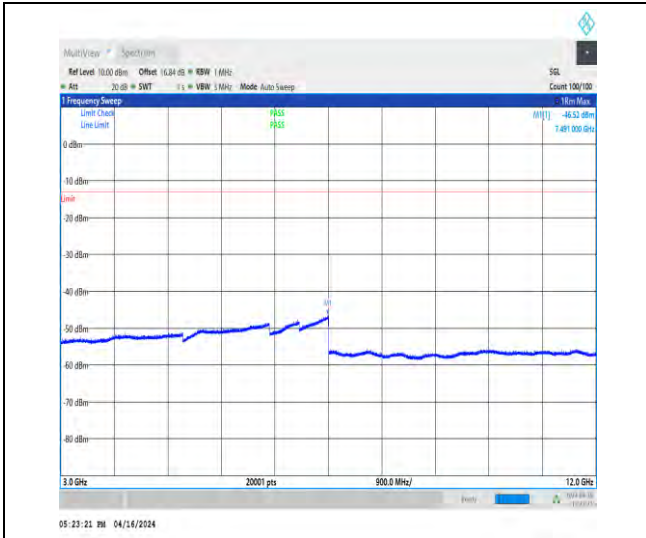
1-N2-15-40-H-1-DFT-QPSK-Edge_1RB_Left-1@0-3 000-12000-Ant1-7491.00--46.52--13-PASS
