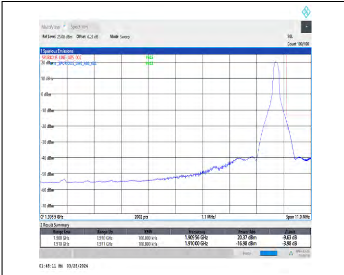
1-N2-15-10-H-2-DFT-PI2BPSK-Edge_1RB_Right-1@5 1-Ant1-1-seegraph-PASS-see graph
