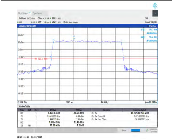
1-N2-15-40-M-9-CP-256QAM-Outer_Full-216@0-Ant 1-38.782-41.280-≤40-PASS
