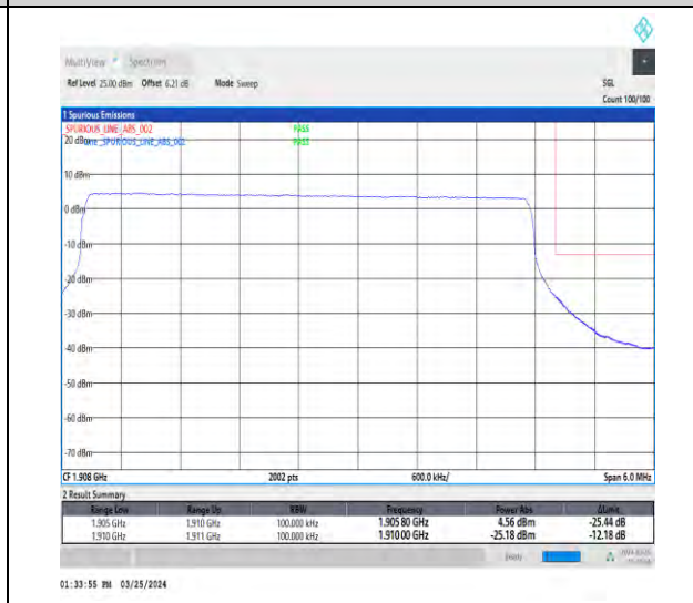
1-N2-15-5-H-6-CP-QPSK-Outer_Full-25@0-Ant1-1-see graph-PASS-see graph
