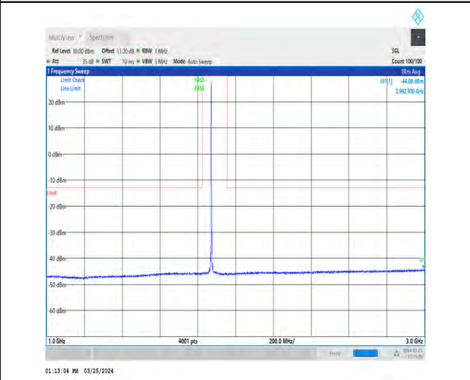
1-N2-15-40-H-1-DFT-PI2BPSK-Inner_1RB_Left-1@ -1000-3000-Ant1-2992.50--44.08--13-PASS
