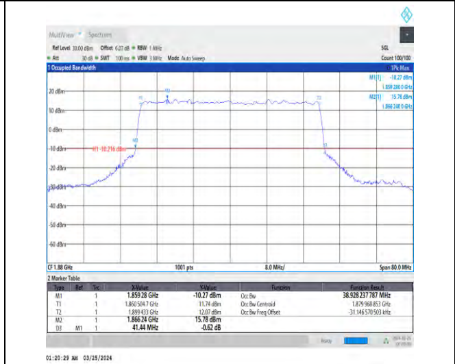
1-N2-15-40-M-8-CP-64QAM-Outer_Full-216@0-Ant1 -38.928-41.440-≤40-PASS
