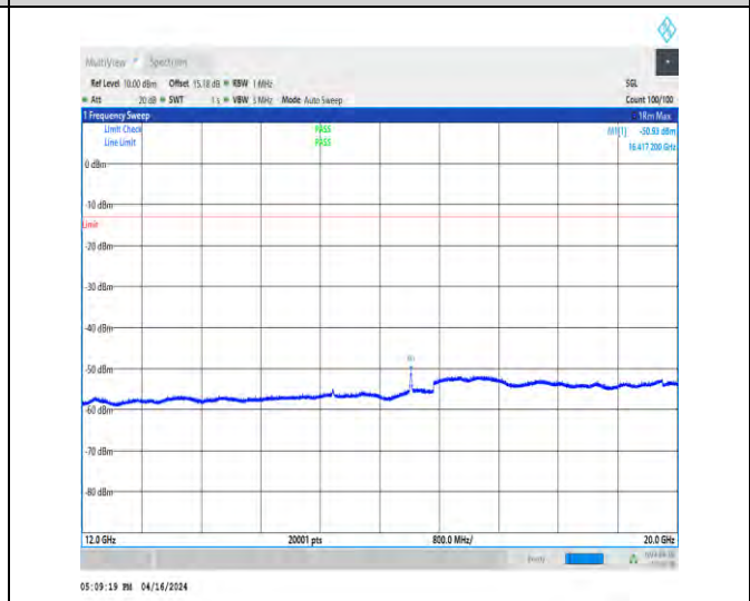
1-N2-15-40-M-1-DFT-QPSK-Edge_1RB_Left-1@0-12 000-20000-Ant1-16417.20--50.93--13-PASS
