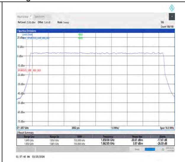
1-N2-15-15-L-3-DFT-PI2BPSK-Outer_Full-75@0-A nt1-1-seegraph-PASS-see graph
