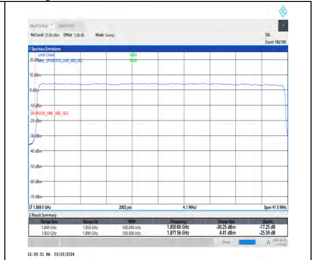
1-N2-15-40-L-3-DFT-PI2BPSK-Outer_Full-216@0-Ant1-1-seegraph-PASS-see graph
