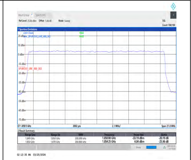
1-N2-15-20-L-3-DFT-PI2BPSK-Outer_Full-100@0-A Ant1-1-seegraph-PASS-see graph
