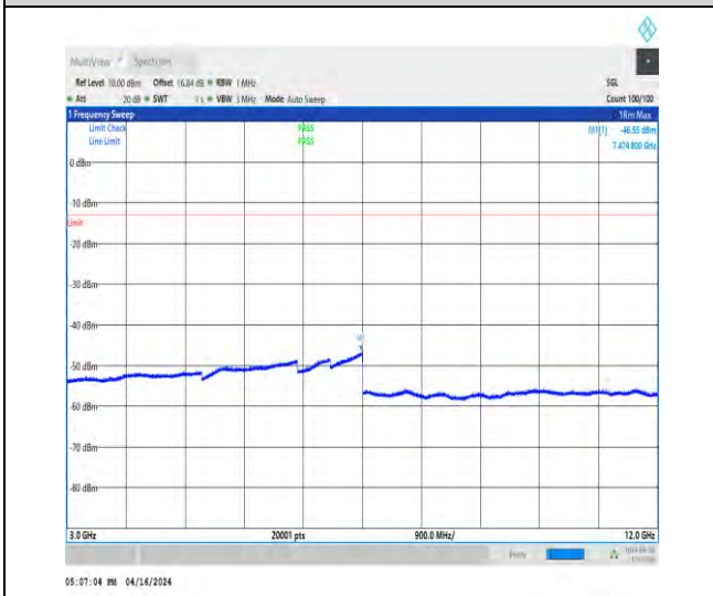
1-N2-15-40-M-1-DFT-QPSK-Edge_1RB_Left-1@0-3 000-12000-Ant1-7474.80--46.55--13-PASS
