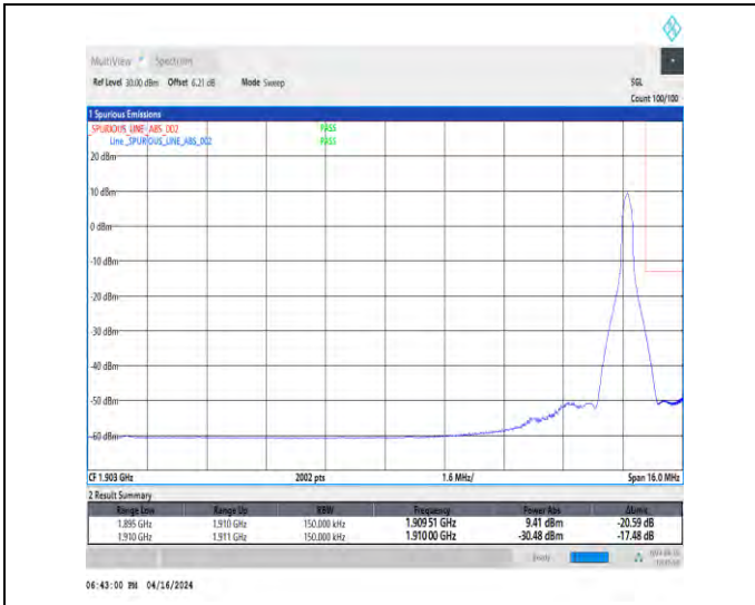
1-N2-15-15-H-2-DFT-PI2BPSK-Edge_1RB_Right-1@7-8-Ant1-1-seegraph-PASS-see graph
