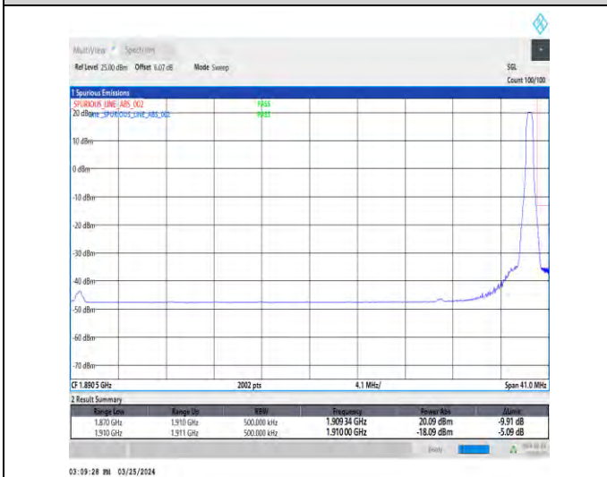
1-N2-15-40-H-5-CP-QPSK-Edge_1RB_Right-1@215-A nt1-1-seegraph-PASS-see graph
