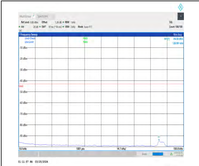
1-N2-15-40-H-1-DFT-PI2BPSK-Inner_1RB_Left-1@ 1-0.009-0.15-Ant1-0.13--94.50--43-PASS
