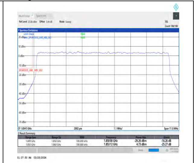
1-N2-15-10-L-3-DFT-PI2BPSK-Outer_Full-50@0-Ant1-1-seegraph-PASS-see graph
