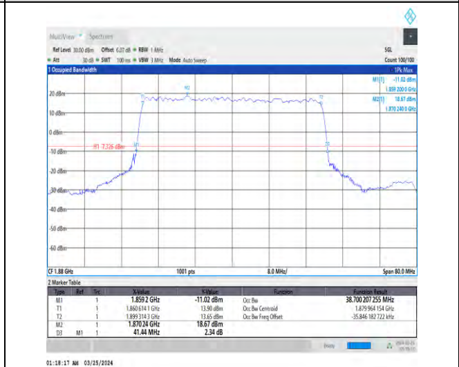
1-N2-15-40-M-2-DFT-PI2BPSK-Outer_Full-216@0-Ant1 -38.7-41.440-≤40-PASS
