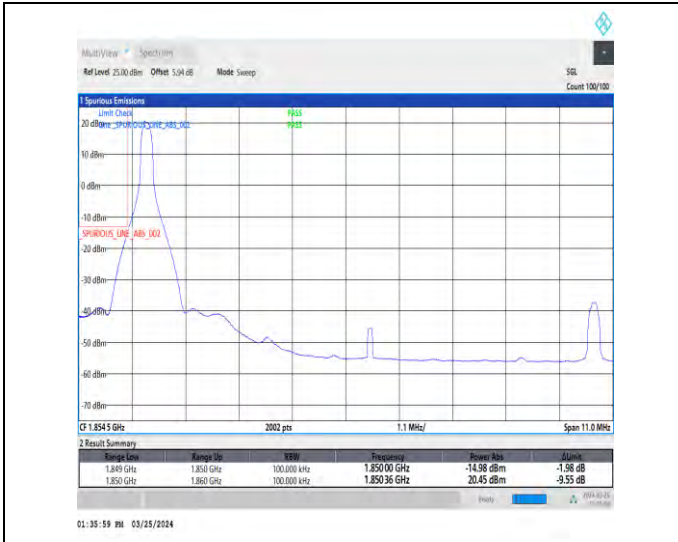
1-N2-15-10-L-1-DFT-PI2BPSK-Edge_1RB_Left-1@0-Ant1-1-seegraph-PASS-see graph
