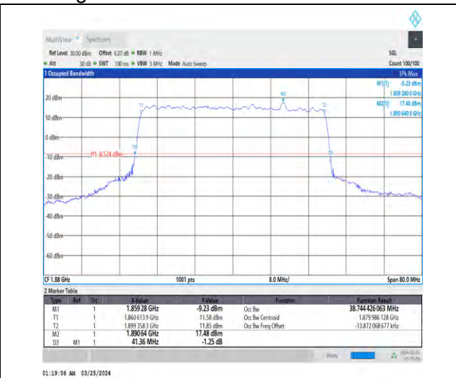
1-N2-15-40-M-4-DFT-64QAM-Outer_Full-216@0-Ant 1-38.744-41.360-≤40-PASS
