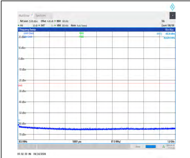
1-N2-15-40-M-1-DFT-QPSK-Edge_1RB_Left-1@0-3 0-1000-Ant1-35.53--60.34--23-PASS
