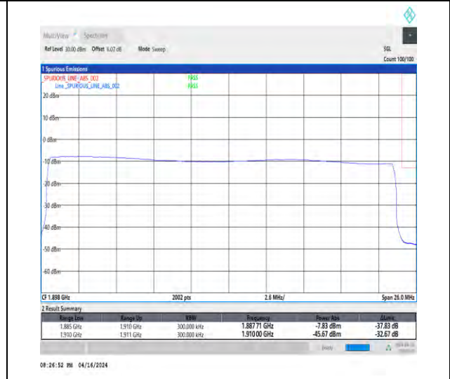
1-N2-15-25-H-6-CP-QPSK-Outer_Full-133@0-Ant1-1-seegraph-PASS-see graph
