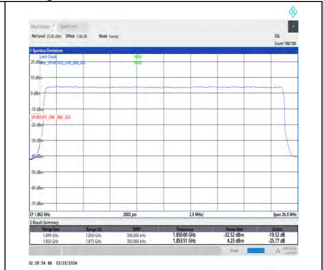
1-N2-15-25-L-3-DFT-PI2BPSK-Outer_Full-128@0-Ant1-1-seegraph-PASS-see graph
