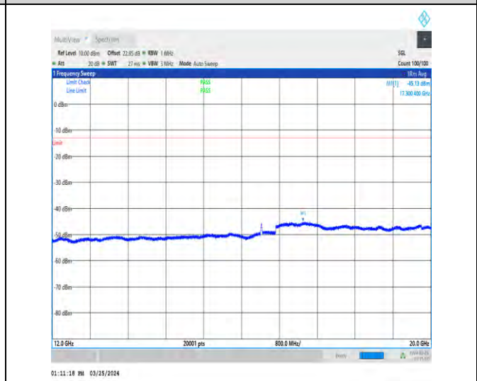
1-N2-15-40-M-1-DFT-PI2BPSK-Inner_1RB_Left-1@ -12000-20000-Ant1-17460.40--45.13--13-PASS
