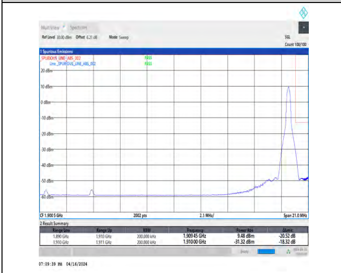
1-N2-15-20-H-5-CP-QPSK-Edge_1RB_Right-1@105-Ant1-1-seegraph-PASS-see graph
