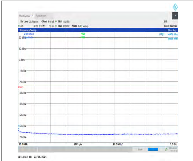
1-N2-15-40-M-1-DFT-PI2BPSK-Inner_1RB_Left-1@ 1-30-1000-Ant1-34.37--63.56--23-PASS
