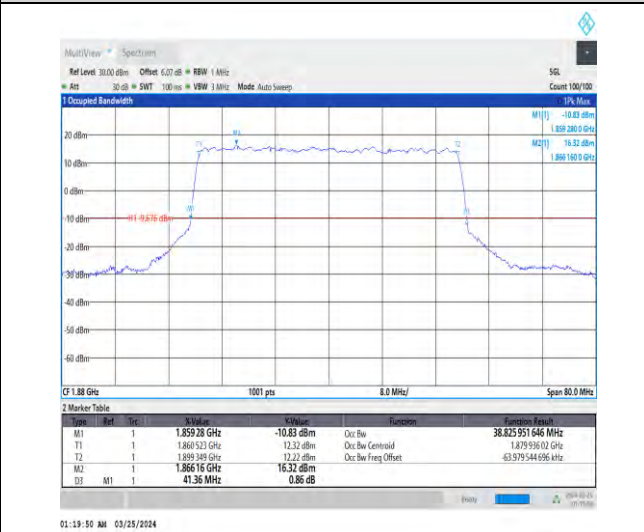
1-N2-15-40-M-6-CP-QPSK-Outer_Full-216@0-Ant1 38.826-41.360-≤40-PASS
