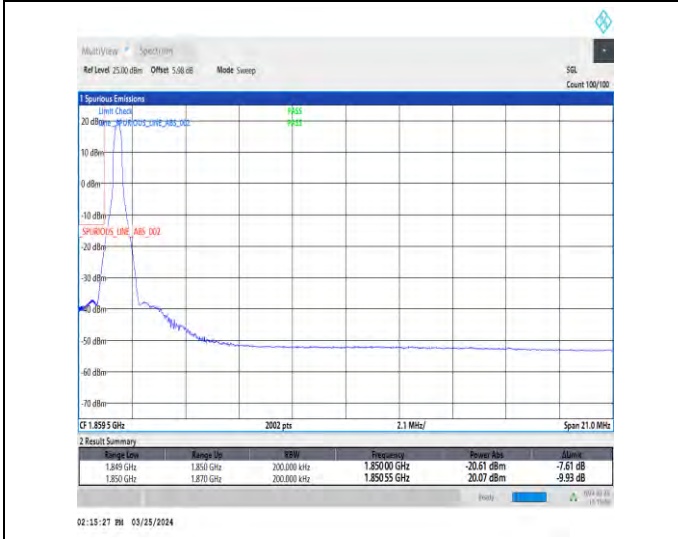
1-N2-15-20-L-4-CP-QPSK-Edge_1RB_Left-1@0-Ant1-1-seegraph-PASS-see graph
