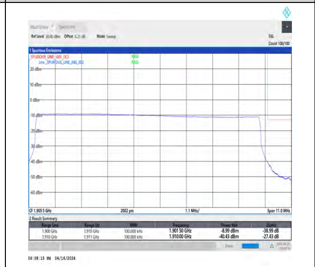
1-N2-15-10-H-6-CP-QPSK-Outer_Full-52@0-Ant1 -1-seegraph-PASS-see graph
