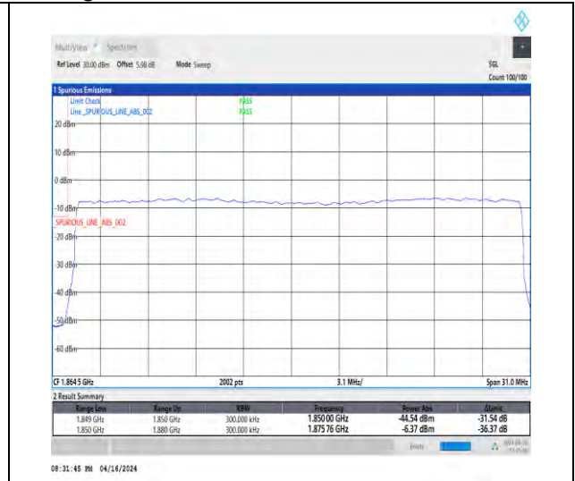
1-N2-15-30-L-3-DFT-PI2BPSK-Outer_Full-160@0-A Ant1-1-seegraph-PASS-see graph
