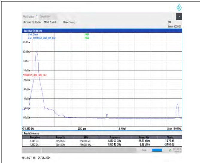
1-N2-15-15-L-1-DFT-PI2BPSK-Edge_1RB_Left-1@0-Ant1-1-seegraph-PASS-see graph
