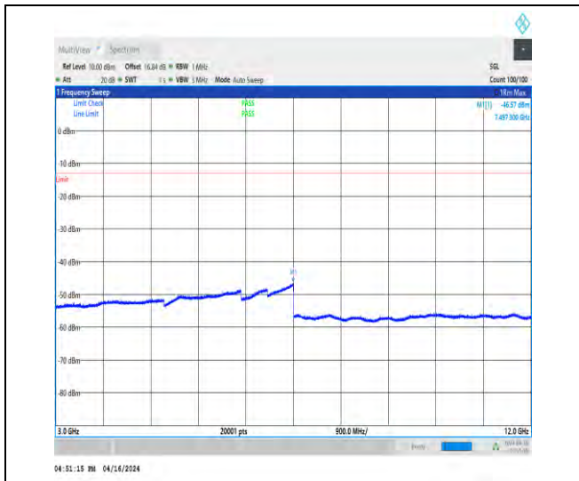
1-N2-15-40-L-1-DFT-QPSK-Edge_1RB_Left-1@0-3 000-12000-Ant1-7497.30--46.57--13-PASS
