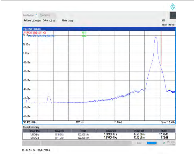
1-N2-15-10-H-5-CP-QPSK-Edge_1RB_Right-1@51-An t1-1-seegraph-PASS-see graph
