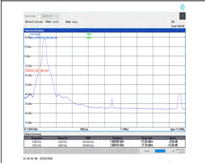
1-N2-15-10-L-4-CP-QPSK-Edge_1RB_Left-1@0-Ant1-1-seegraph-PASS-see graph
