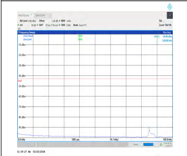
1-N2-15-40-M-1-DFT-PI2BPSK-Inner_1RB_Left-1@ 1-0.009-0.15-Ant1-0.13--93.96--43-PASS
