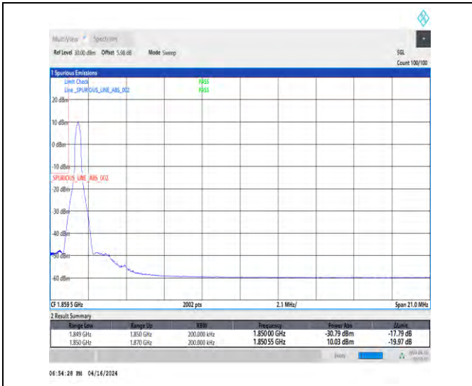
1-N2-15-20-L-1-DFT-PI2BPSK-Edge_1RB_Left-1@0-Ant1-1-seegraph-PASS-see graph
