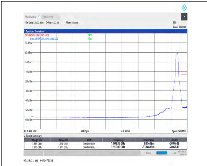
1-N2-15-25-H-2-DFT-PI2BPSK-Edge_1RB_Right-1@132-Ant1-1-seegraph-PASS-see graph
