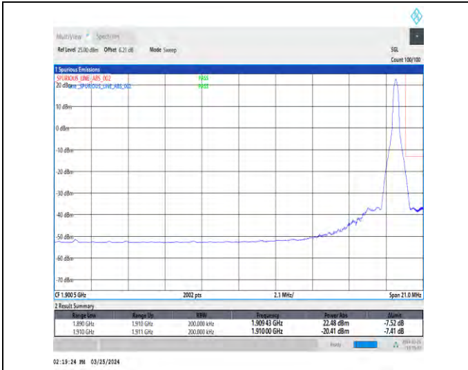
1-N2-15-20-H-2-DFT-PI2BPSK-Edge_1RB_Right-1@105-Ant1-1-seegraph-PASS-see graph
