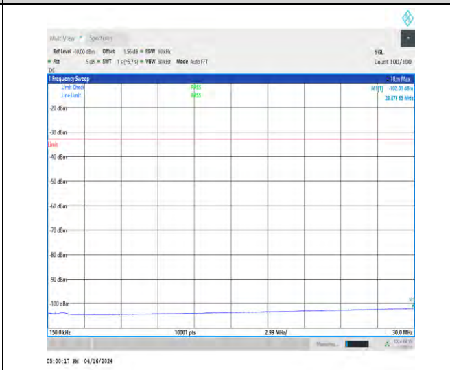
1-N2-15-40-M-1-DFT-QPSK-Edge_1RB_Left-1@0-0. 15-30-Ant1-29.87--102.01--33-PASS
