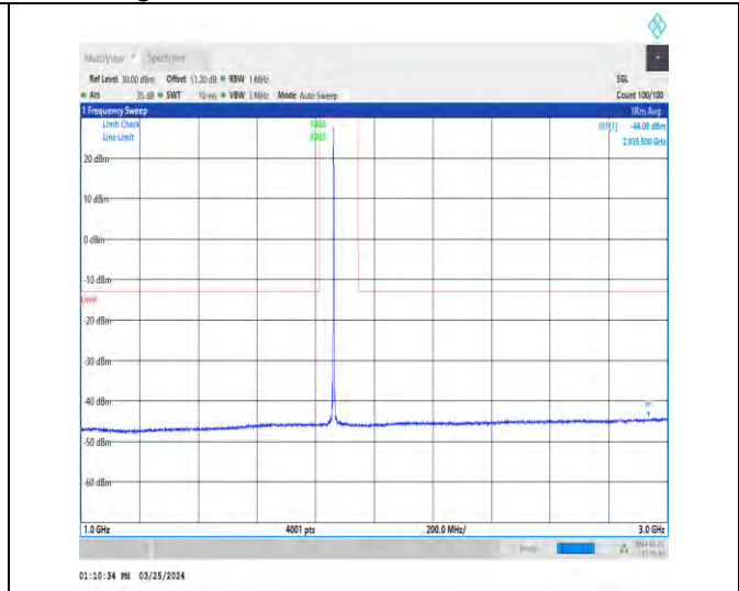
1-N2-15-40-M-1-DFT-PI2BPSK-Inner_1RB_Left-1@ -1000-3000-Ant1-2960.50--44.09--13-PASS
