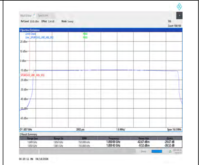
1-N2-15-15-L-6-CP-QPSK-Outer_Full-79@0-Ant1-1-seegraph-PASS-see graph
