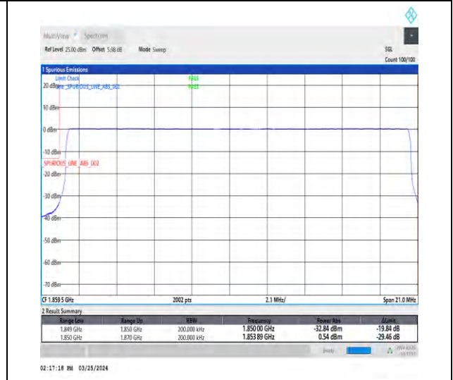
1-N2-15-20-L-6-CP-QPSK-Outer_Full-106@0-Ant1-1-seegraph-PASS-see graph
