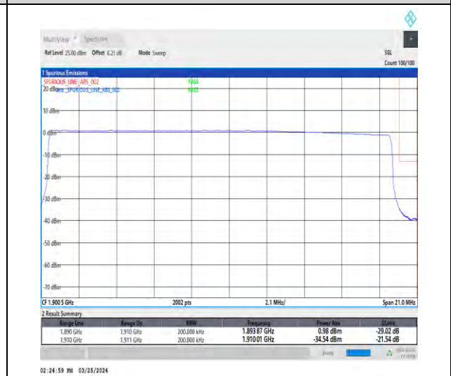
1-N2-15-20-H-6-CP-QPSK-Outer_Full-106@0-Ant1-1-seegraph-PASS-see graph
