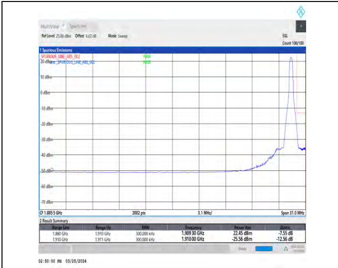
1-N2-15-30-H-2-DFT-PI2BPSK-Edge_1RB_Right-1@159-Ant1-1-seegraph-PASS-see graph
