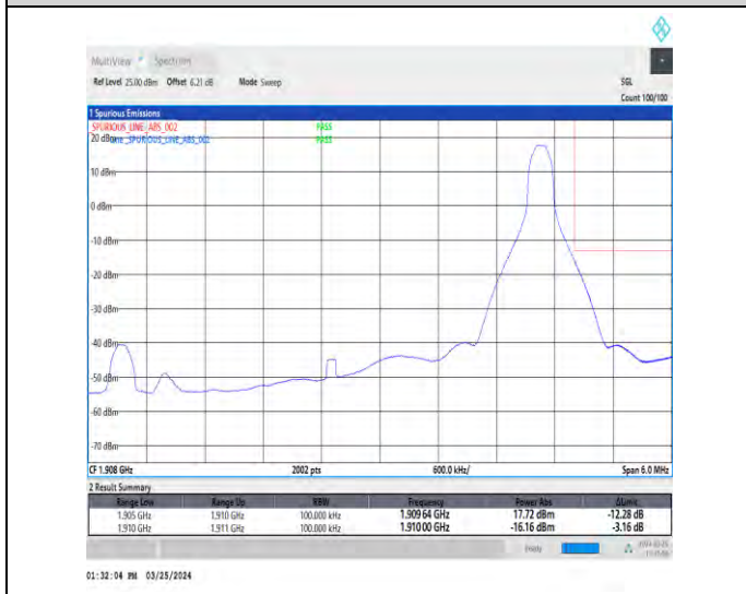
1-N2-15-5-H-5-CP-QPSK-Edge_1RB_Right-1@24-Ant1-1-see graph-PASS-see graph
