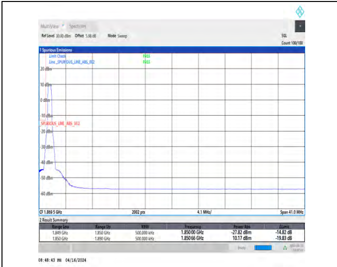
1-N2-15-40-L-1-DFT-PI2BPSK-Edge_1RB_Left-1@0-Ant1-1-seegraph-PASS-see graph
