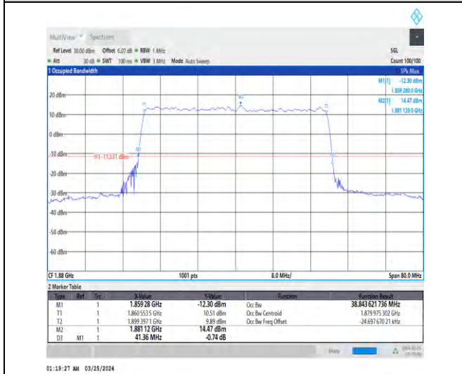
1-N2-15-40-M-5-DFT-256QAM-Outer_Full-216@0-A nt1-38.844-41.360-≤40-PASS
