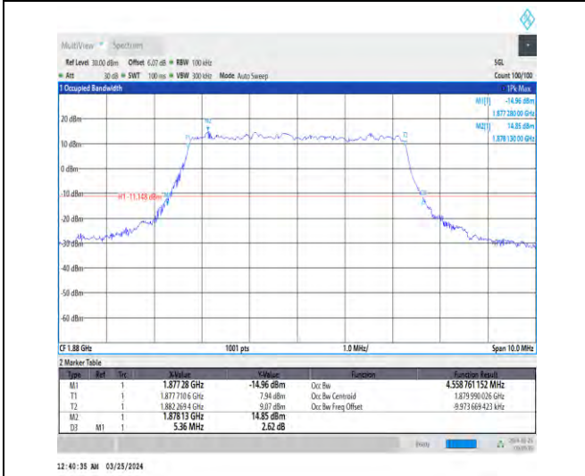
1-N2-15-5-M-7-CP-16QAM-Outer_Full-25@0-Ant1-4 .559-5.360-≤5-PASS
