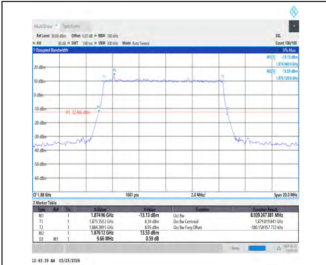
1-N2-15-10-M-4-DFT-64QAM-Outer_Full-50@0-Ant1 -8.939-9.660-≤10-PASS
