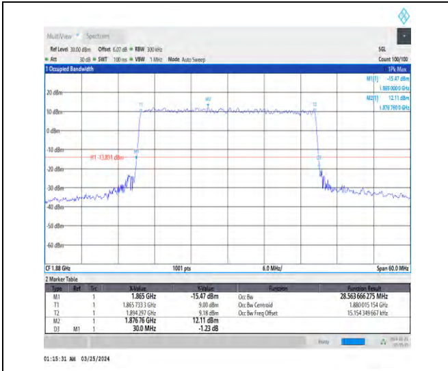
1-N2-15-30-M-4-DFT-64QAM-Outer_Full-160@0-Ant 1-28.564-30.000-≤30-PASS
