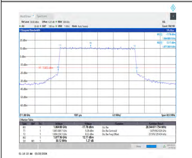
1-N2-15-30-M-6-CP-QPSK-Outer_Full-160@0-Ant1 28.545-30.120-≤30-PASS
