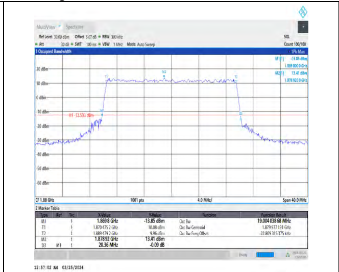
1-N2-15-20-M-7-CP-16QAM-Outer_Full-106@0-Ant1-19.004-20.360-<=20-PASS
