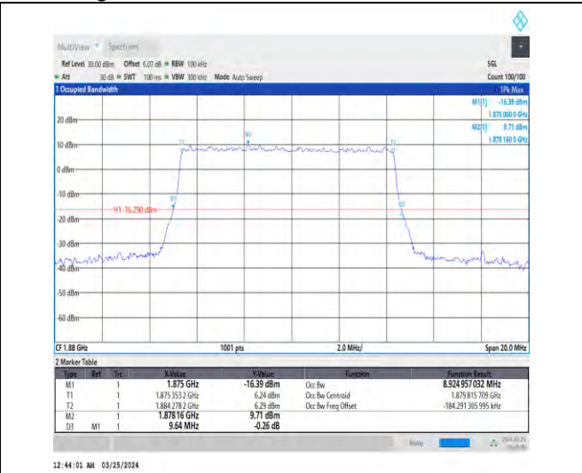
1-N2-15-10-M-5-DFT-256QAM-Outer_Full-50@0-Ant 1-8.925-9.640-≤10-PASS
