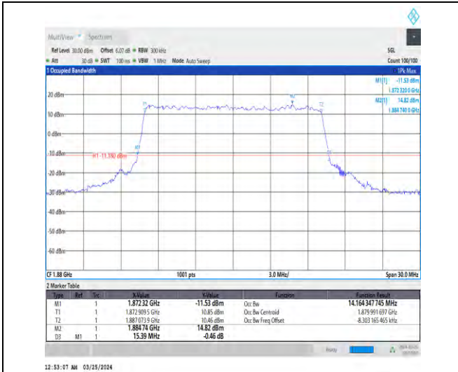
1-N2-15-15-M-7-CP-16QAM-Outer_Full-79@0-Ant1-14.164-15.390-≤15-PASS
