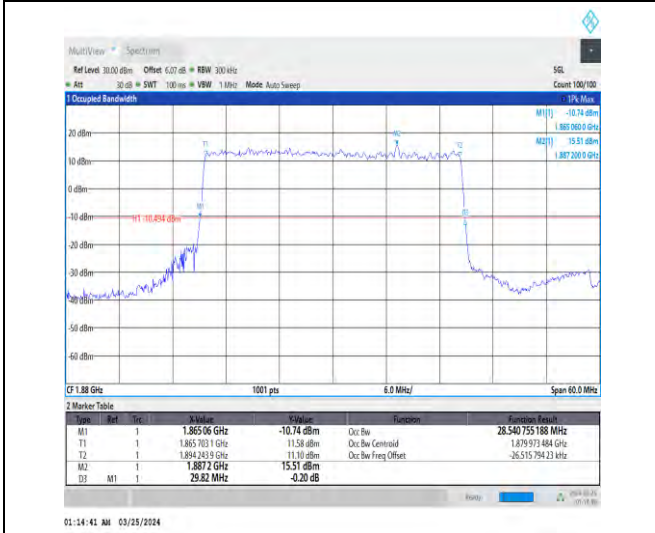
1-N2-15-30-M-2-DFT-PI2BPSK-Outer_Full-160@0-A nt1-28.541-29.820-≤30-PASS
