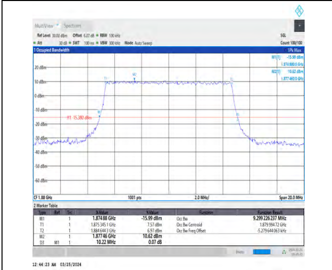
1-N2-15-10-M-6-CP-QPSK-Outer_Full-52@0-Ant1-9. 299-10.220-≤10-PASS
