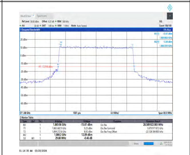
1-N2-15-30-M-7-CP-16QAM-Outer_Full-160@0-Ant1 -28.59-29.880-≤30-PASS
