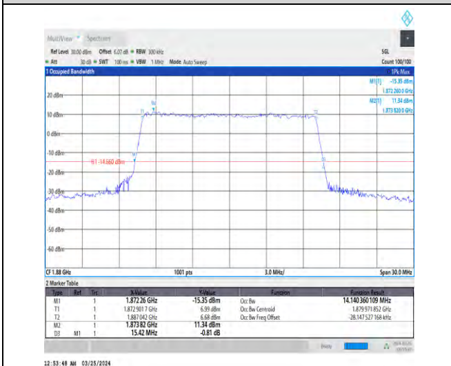
1-N2-15-15-M-9-CP-256QAM-Outer_Full-79@0-Ant1-14.14-15.420-≤15-PASS
