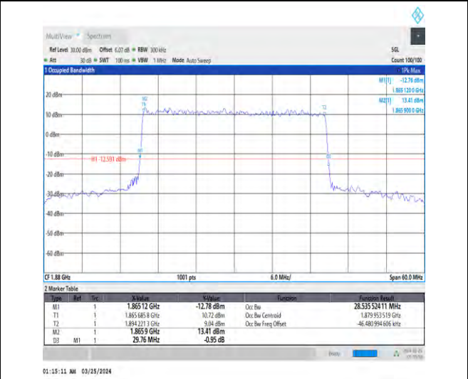
1-N2-15-30-M-3-DFT-16QAM-Outer_Full-160@0-Ant 1-28.536-29.760-≤30-PASS
