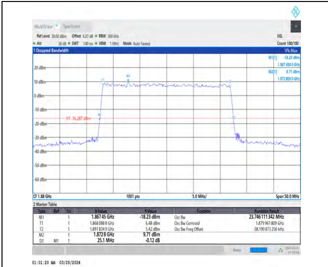
1-N2-15-25-M-9-CP-256QAM-Outer_Full-133@0-Ant 1-23.746-25.100-≤25-PASS
