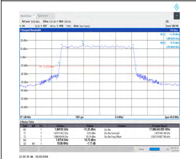
1-N2-15-20-M-4-DFT-64QAM-Outer_Full-100@0-Ant 1-17.887-19.080-≤20-PASS
