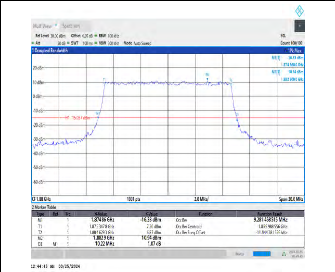
1-N2-15-10-M-7-CP-16QAM-Outer_Full-52@0-Ant1-9. 9.281-10.220-≤10-PASS
