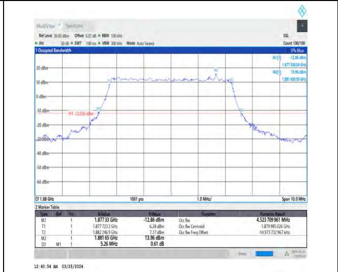
1-N2-15-5-M-8-CP-64QAM-Outer_Full-25@0-Ant1-4 .524-5.260-≤5-PASS
