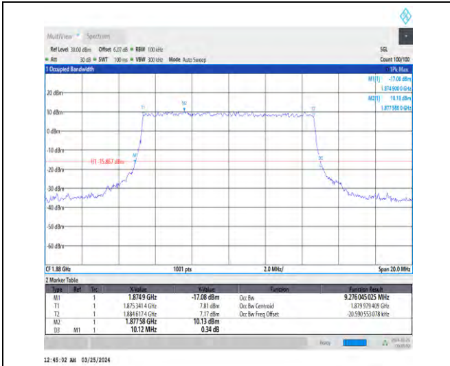
1-N2-15-10-M-8-CP-64QAM-Outer_Full-52@0-Ant1-9.276-10.120-≤10-PASS
