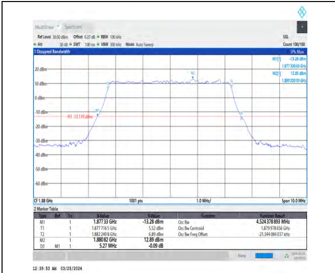
1-N2-15-5-M-5-DFT-256QAM-Outer_Full-25@0-Ant1 -4.524-5.270-≤5-PASS
