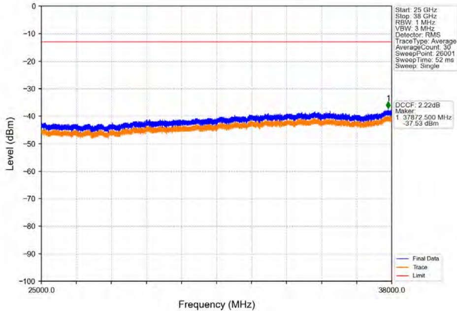
Band43d_15MHz_QPSK_LCH_3707.5MHz_RB_75_0_NTNV
