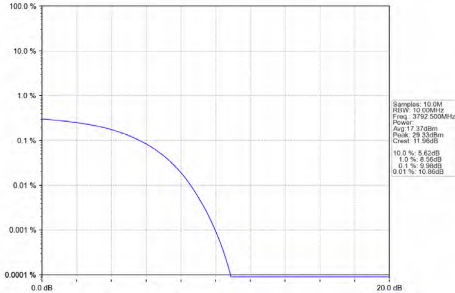
Band43d_15MHz_64QAM_HCH_3792.5MHz_RB_75_0_NTNV
