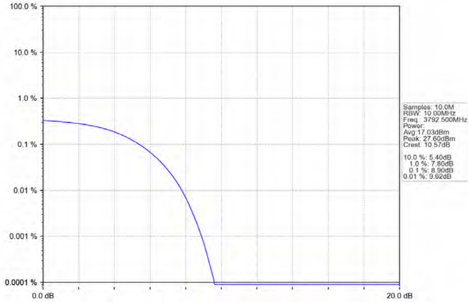
Band43d_15MHz_QPSK_HCH_3792.5MHz_RB_75_0_NTNV
