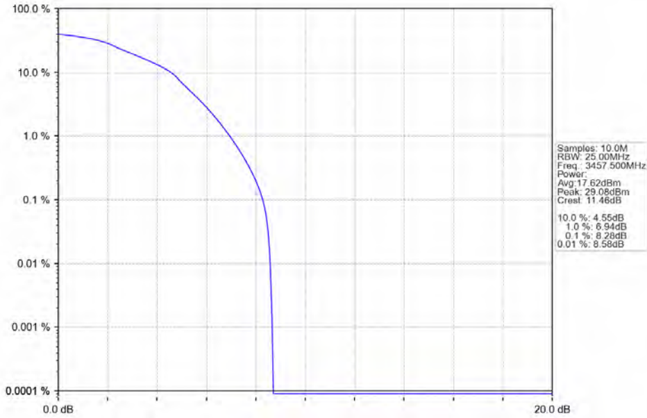
Band42a 15MHz 64QAM LCH 3457.5MHz RB 75 0 NTN
