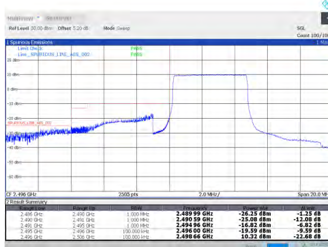
Band41-5MHz-QPSK-39675-25RB#0
