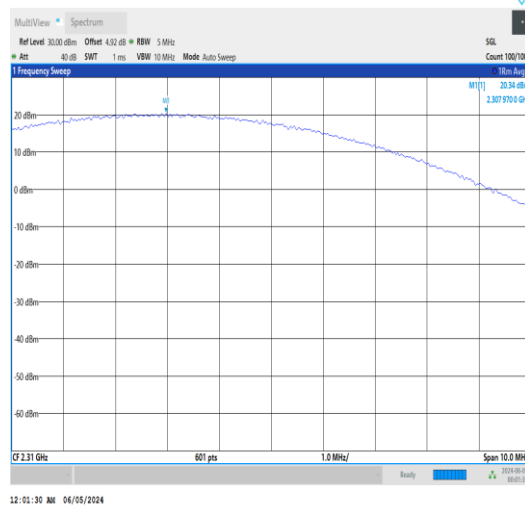
Band30-5MHz-QPSK-27710-1RB#0-PASS
