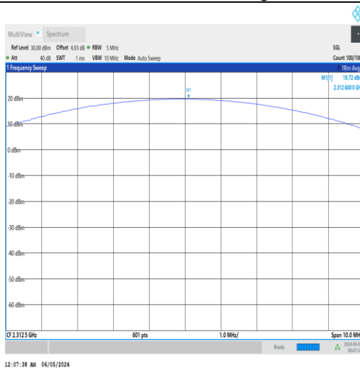
Band30-5MHz-QPSK-27735-12RB#6-PASS
