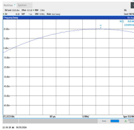
Band30-5MHz-QPSK-27735-1RB#24-PASS
