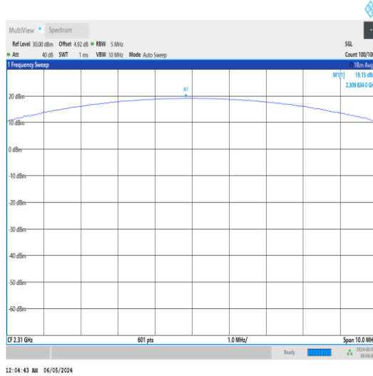
Band30-5MHz-QPSK-27710-25RB#0-PASS
