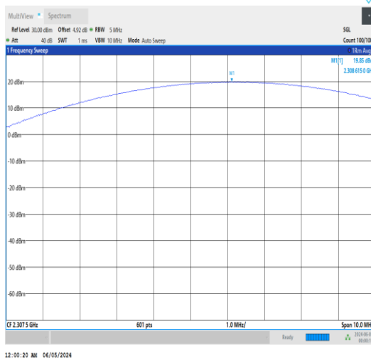
Band30-5MHz-QPSK-27685-12RB#13-PASS
