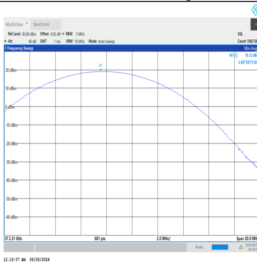
Band30-10MHz-QPSK-27710-25RB#0-PASS
