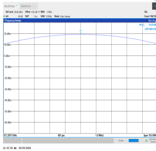
Band30-5MHz-QPSK-27685-25RB#0-PASS
