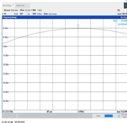
Band30-5MHz-QPSK-27735-12RB#13-PASS
