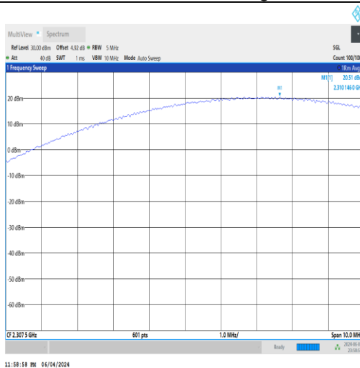
Band30-5MHz-QPSK-27685-1RB#24-PASS
