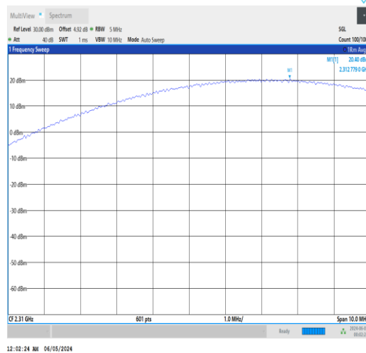
Band30-5MHz-QPSK-27710-1RB#24-PASS
