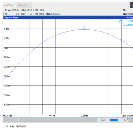
Band30-10MHz-QPSK-27710-25RB#25-PASS
