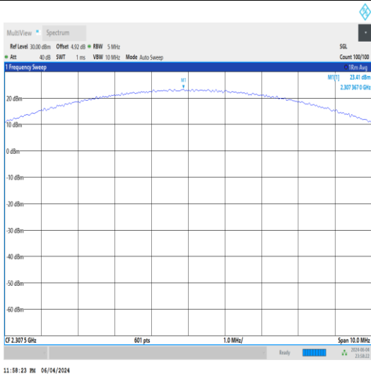
Band30-5MHz-QPSK-27685-1RB#12-PASS
