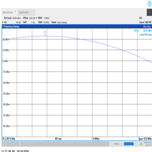
Band30-5MHz-QPSK-27685-1RB#0-PASS
