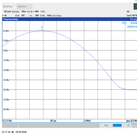
Band30-10MHz-QPSK-27710-1RB#0-PASS
