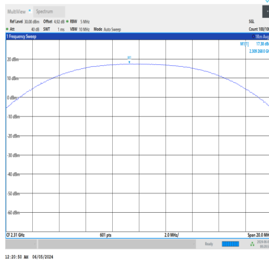
Band30-10MHz-QPSK-27710-50RB#0-PASS
