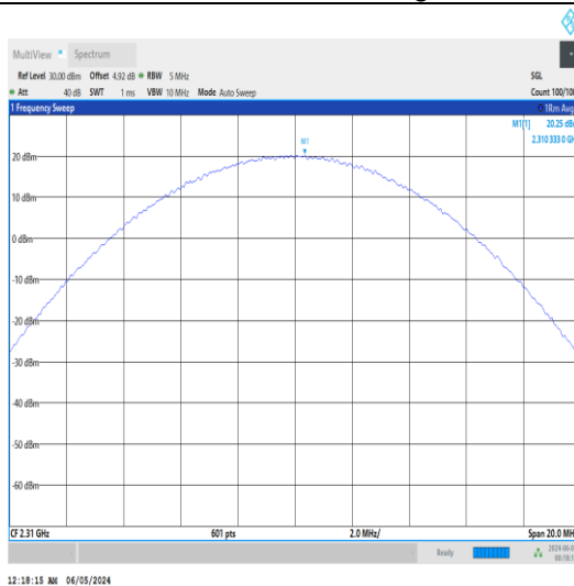
Band30-10MHz-QPSK-27710-1RB#24-PASS
