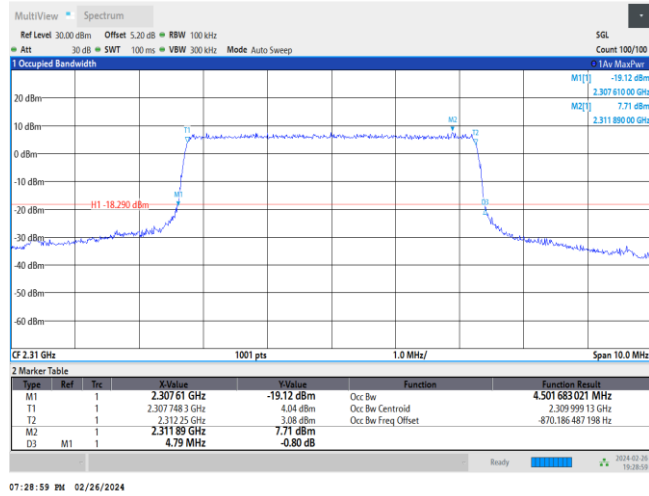
Band30-5MHz-16QAM-27710-25RB#0
