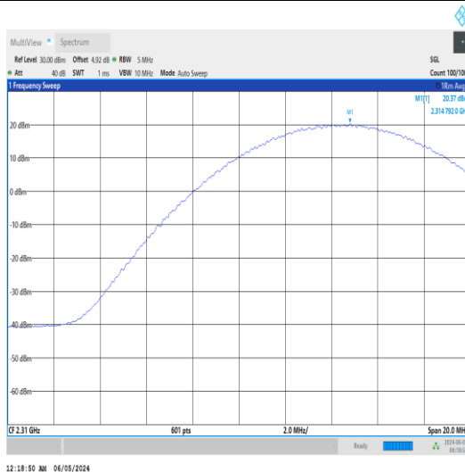
Band30-10MHz-QPSK-27710-1RB#49-PASS
