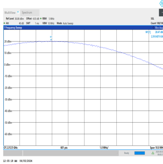
Band30-5MHz-QPSK-27735-1RB#0-PASS
