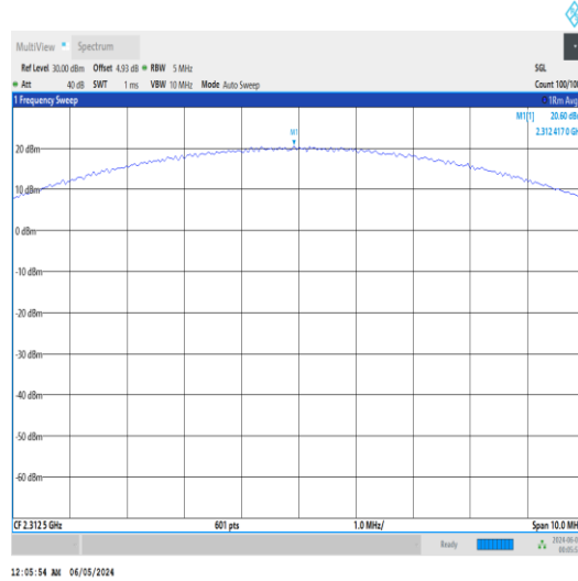
Band30-5MHz-QPSK-27735-1RB#12-PASS
