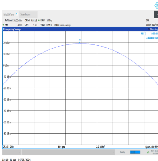
Band30-10MHz-QPSK-27710-25RB#12-PASS
