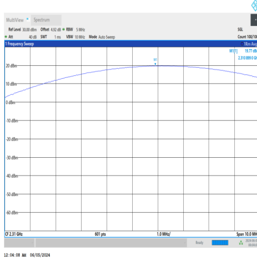
Band30-5MHz-QPSK-27710-12RB#13-PASS
