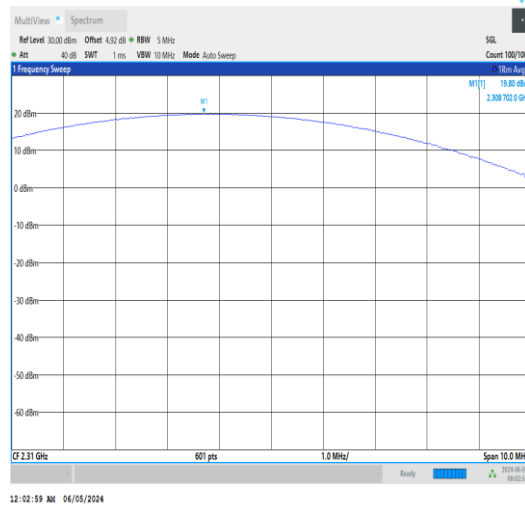
Band30-5MHz-QPSK-27710-12RB#0-PASS
