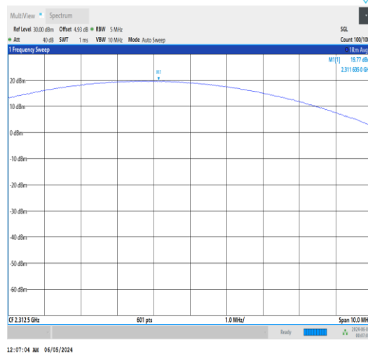
Band30-5MHz-QPSK-27735-12RB#0-PASS
