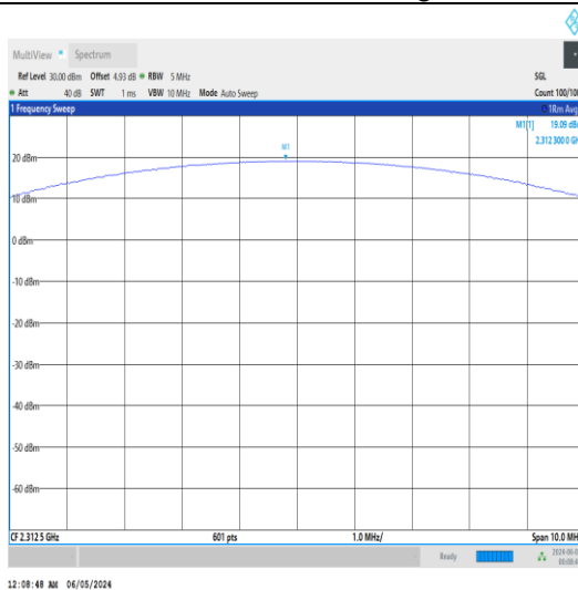
Band30-5MHz-QPSK-27735-25RB#0-PASS
