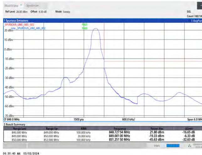
Band26-1.4MHz-QPSK-27033-6RB#0
