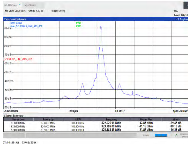
Band26-10MHz-QPSK-26840-50RB#0
