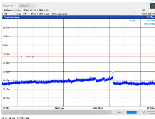
Band26-15MHz-QPSK-26965-1RB#0-Range4:1000~10000MHz
