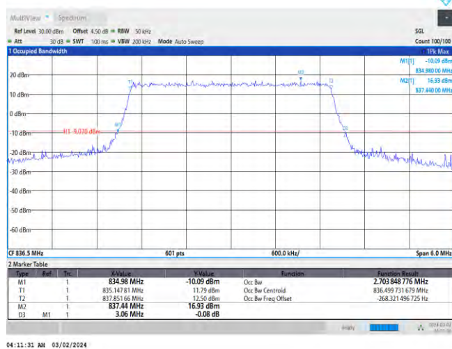
Band26-3MHz-64QAM-26915-15RB#0
