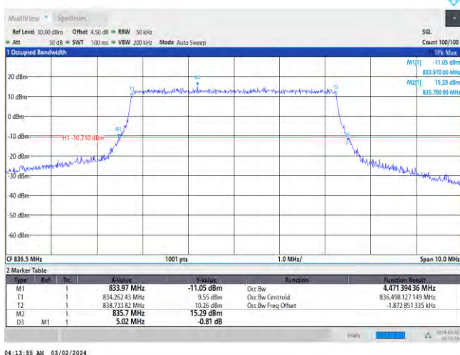
Band26-5MHz-64QAM-26915-25RB#0
