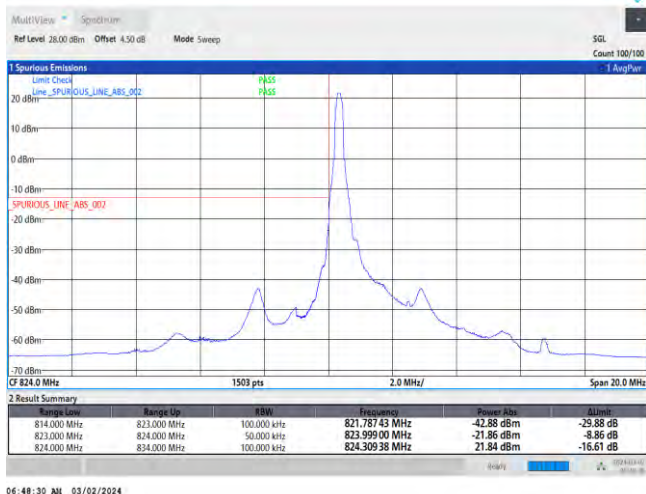
Band26-5MHz-QPSK-26815-25RB#0
