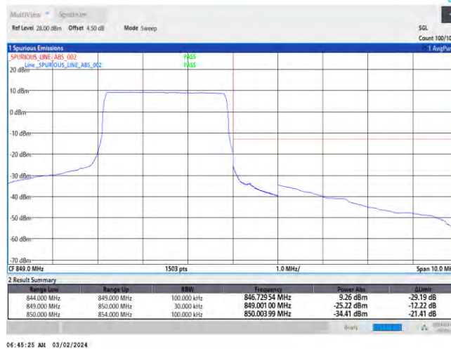
Band26-5MHz-QPSK-26815-1RB#0
