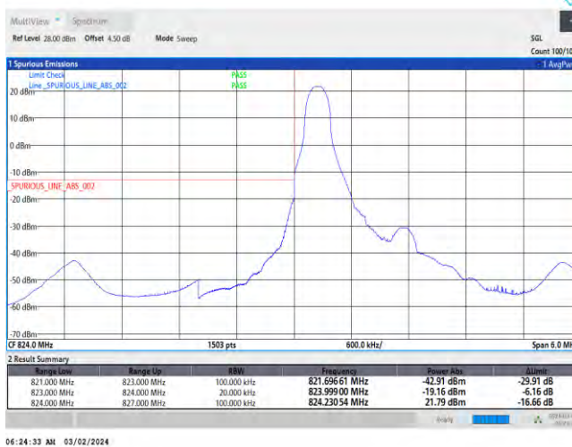
Band26-1.4MHz-QPSK-26797-6RB#0
