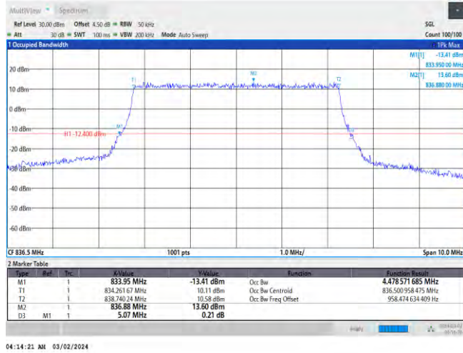
Band26-5MHz-256QAM-26915-25RB#0
