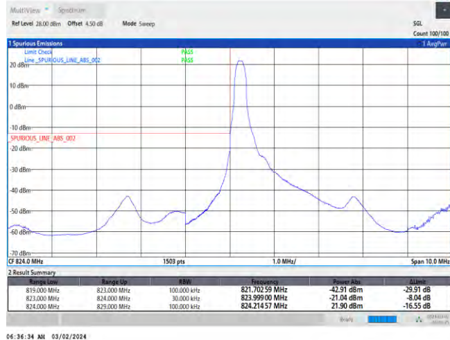
Band26-3MHz-QPSK-26805-15RB#0
