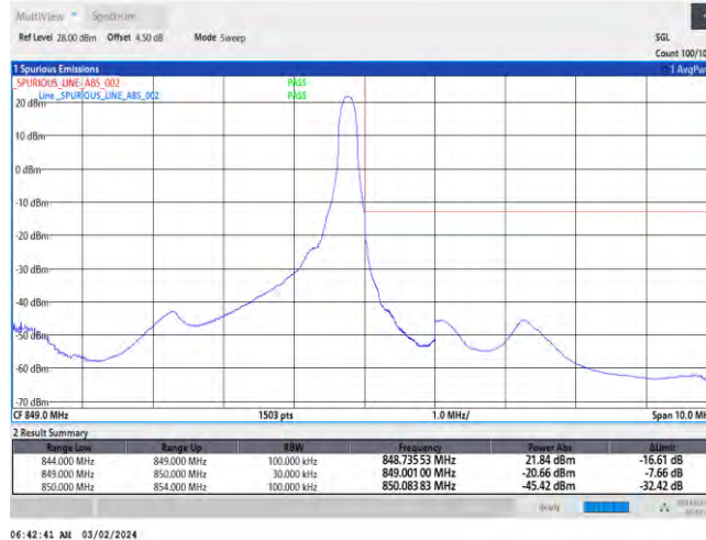
Band26-3MHz-QPSK-27025-15RB#0
