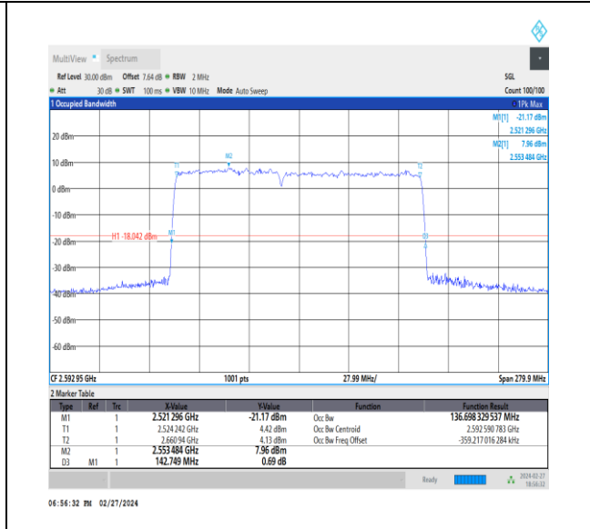
NTNV_CA_n41C_PC3_30+30_60+80_M+M_Ant1_TID4_1_#1
