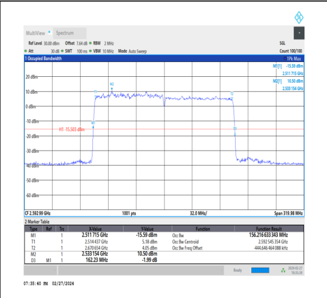
NTNV_CA_n41C_PC3_30+30_80+80_M+M_Ant1_TID8_1_#1
