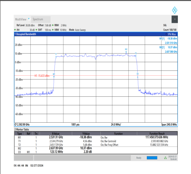
NTVN_CA_n41C_PC3_30+30_60+60_M+M_Ant1_TID5_1_#1
