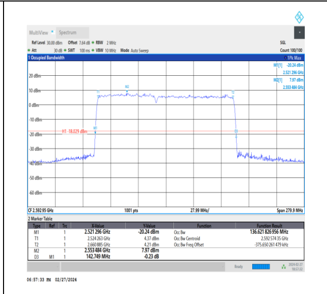
NTNV_CA_n41C_PC3_30+30_60+80_M+M_Ant1_TID8_1_#1
