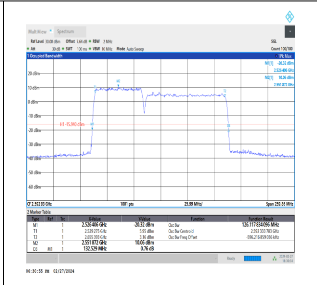
NTNV_CA_n41C_PC3_30+30_50+80_M+M_Ant1_TID3_1_#1
