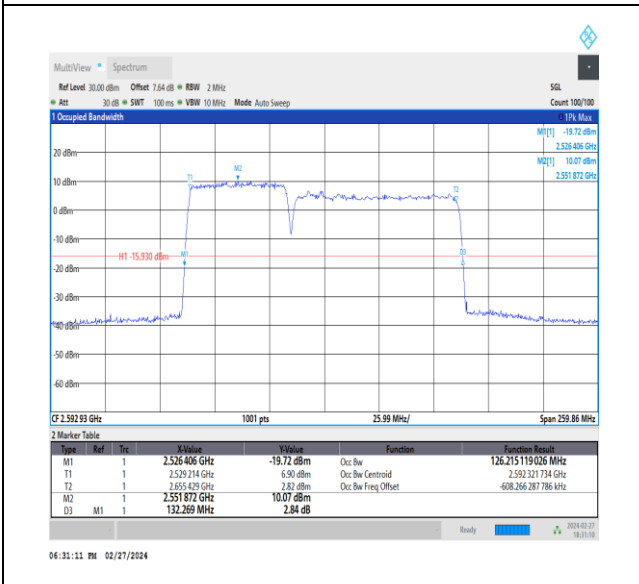
NTNV_CA_n41C_PC3_30+30_50+80_M+M_Ant1_TID4_1_#1
