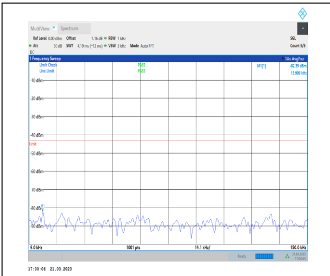
1-N78-3700-3800-30-100-H-1-DFT-QPSK-Edge_1R B_Left-1@0-0.009-0.15-Ant0-0.02--82.39--43-PASS
