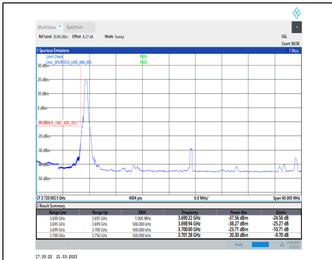
1-N78-3700-3800-30-50-L-4-CP-QPSK-Edge_1RB_Lef t-1@0-Ant0-1--PASS-see graph
