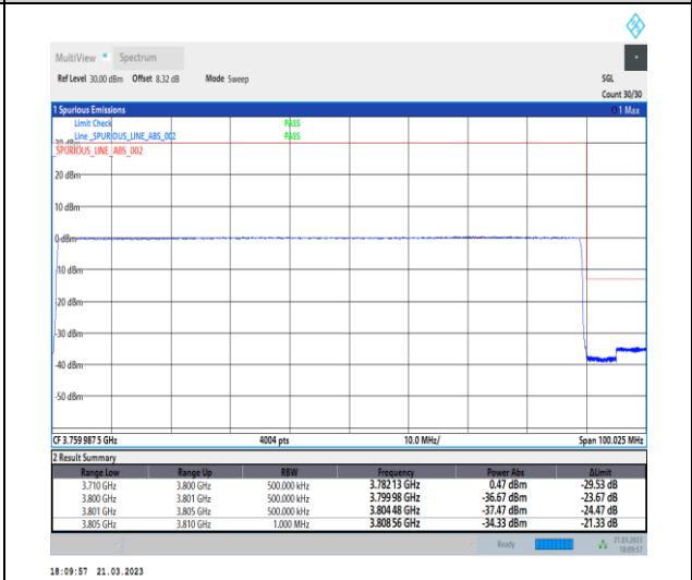
1-N78-3700-3800-30-90-H-6-CP-QPSK-Outer_Full -245@0-Ant0-1--PASS-see graph
