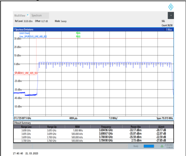
1-N78-3700-3800-30-60-L-6-CP-QPSK-Outer_Full -162@0-Ant0-1--PASS-see graph
