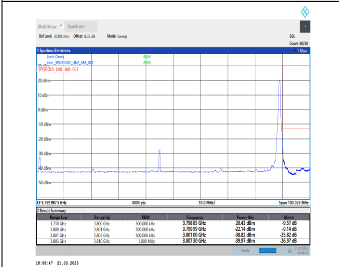
1-N78-3700-3800-30-90-H-5-CP-QPSK-Edge_1RB_Ri ght-1@244-Ant0-1--PASS-see graph
