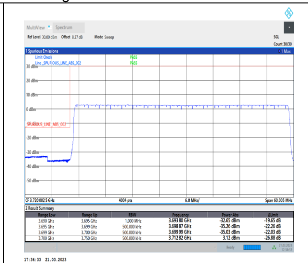
1-N78-3700-3800-30-50-L-6-CP-QPSK-Outer_Full -133@0-Ant0-1--PASS-see graph
