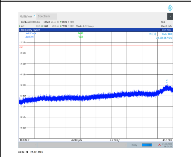
1-N78-3700-3800-30-100-M-1-DFT-QPSK-Edge_1R B_Left-1@0-18000-40000-Ant0-18000.00--38.63--13- PASS
