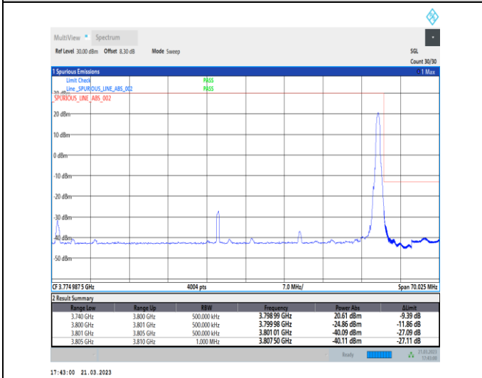
1-N78-3700-3800-30-60-H-5-CP-QPSK-Edge_1RB_Ri ght-1@161-Ant0-1--PASS-see graph
