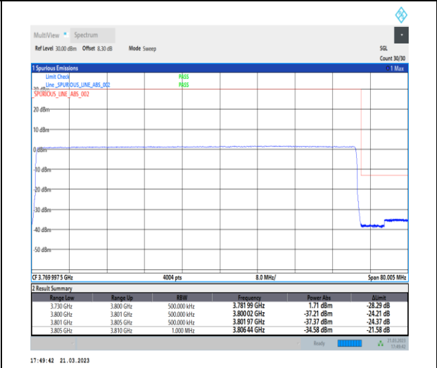
1-N78-3700-3800-30-70-H-6-CP-QPSK-Outer_Full -189@0-Ant0-1--PASS-see graph
