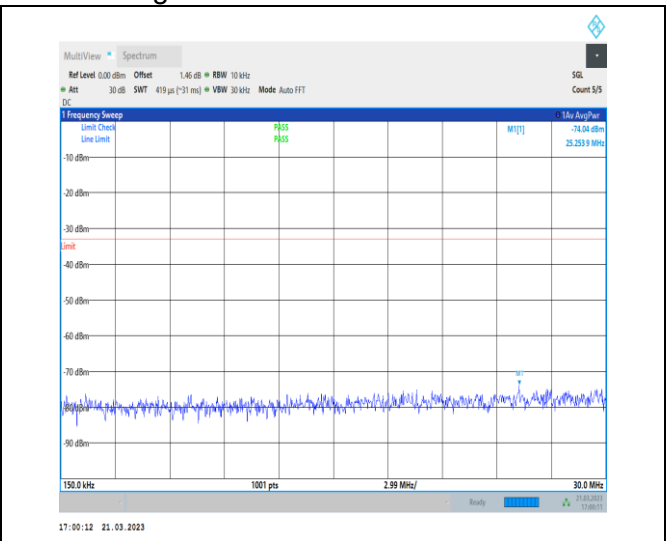
1-N78-3700-3800-30-100-H-1-DFT-QPSK-Edge_1RB _Left-1@0-0.15-30-Ant0-25.25--74.04--33-PASS
