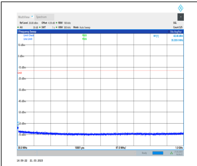
1-N78-3700-3800-30-100-M-1-DFT-QPSK-Edge_1R B_Left-1@0-30-1000-Ant0-35.34--62.46--13-PASS
