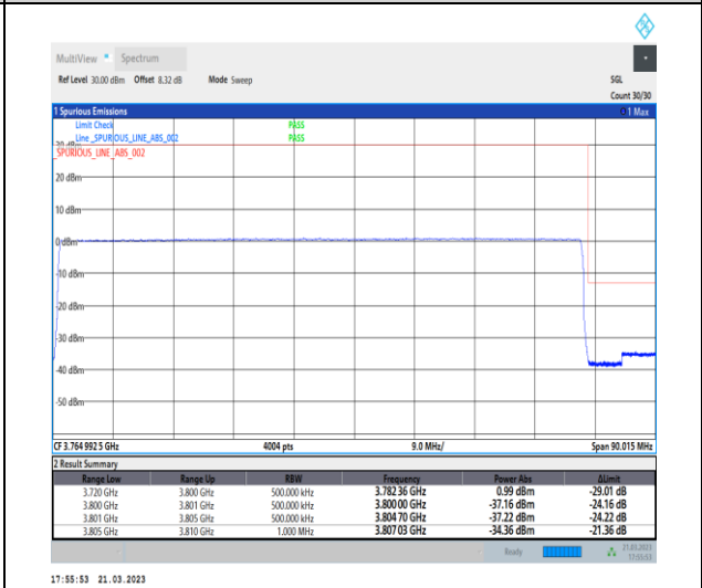
1-N78-3700-3800-30-80-H-6-CP-QPSK-Outer_Full -217@0-Ant0-1--PASS-see graph
