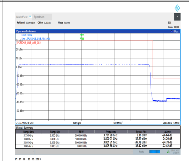
1-N78-3700-3800-30-50-H-6-CP-QPSK-Outer_Full -133@0-Ant0-1--PASS-see graph
