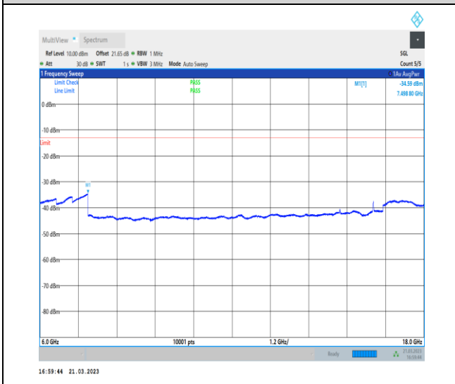
1-N78-3700-3800-30-100-M-1-DFT-QPSK-Edge_1R B_Left-1@0-6000-18000-Ant0-7498.80--34.59--13-P ASS
