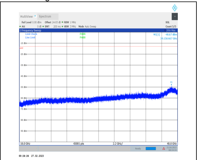
1-N78-3700-3800-30-100-H-1-DFT-QPSK-Edge_1RB _Left-1@0-18000-40000-Ant0-18000.00--38.50--13-P ASS
