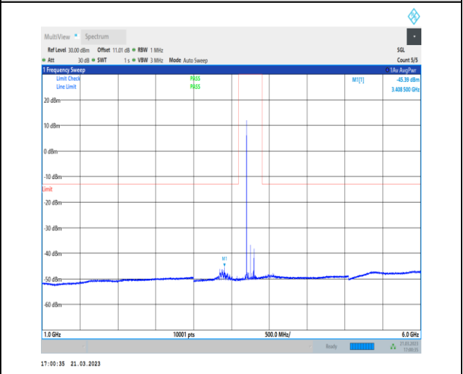
1-N78-3700-3800-30-100-H-1-DFT-QPSK-Edge_1RB _Left-1@0-1000-6000-Ant0-3408.50--45.39--13-PASS
