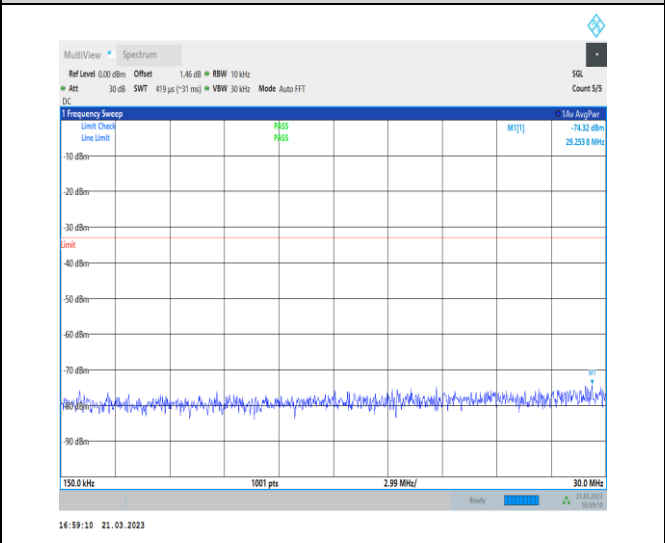
1-N78-3700-3800-30-100-M-1-DFT-QPSK-Edge_1R B_Left-1@0-0.15-30-Ant0-29.25--74.32--33-PASS
