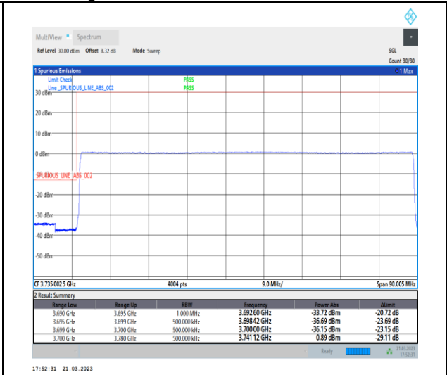
1-N78-3700-3800-30-80-L-6-CP-QPSK-Outer_Full -217@0-Ant0-1--PASS-see graph
