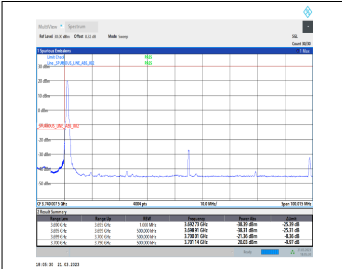
1-N78-3700-3800-30-90-L-4-CP-QPSK-Edge_1RB_Lef t-1@0-Ant0-1--PASS-see graph
