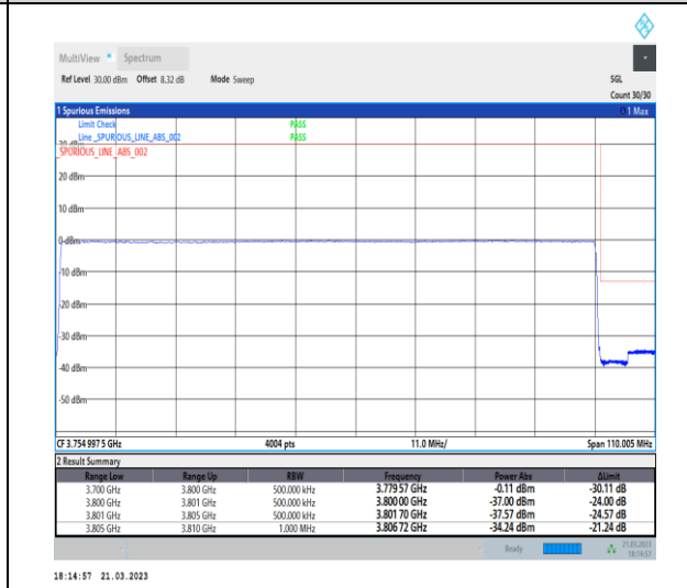
1-N78-3700-3800-30-100-H-6-CP-QPSK-Outer_F ull-273@0-Ant0-1--PASS-see graph
