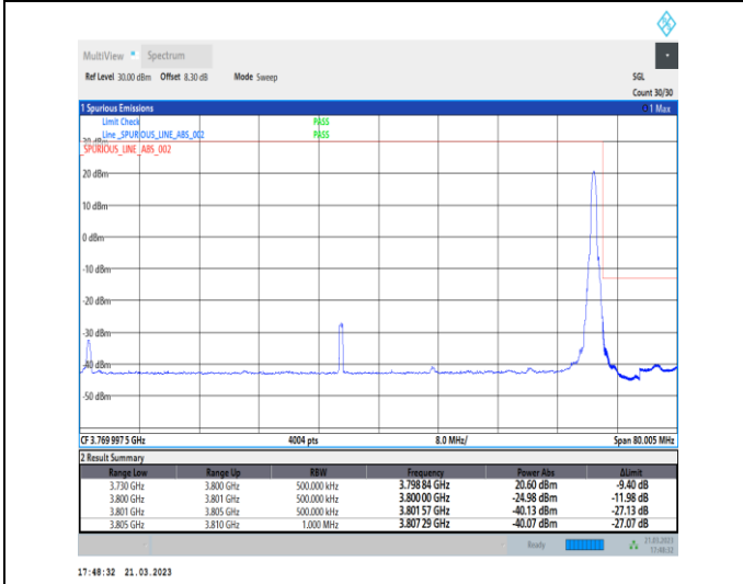
1-N78-3700-3800-30-70-H-5-CP-QPSK-Edge_1RB_Ri ght-1@188-Ant0-1--PASS-see graph
