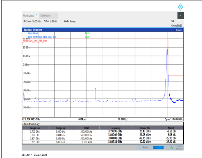
1-N78-3700-3800-30-100-H-5-CP-QPSK-Edge_1RB_R ight-1@272-Ant0-1--PASS-see graph
