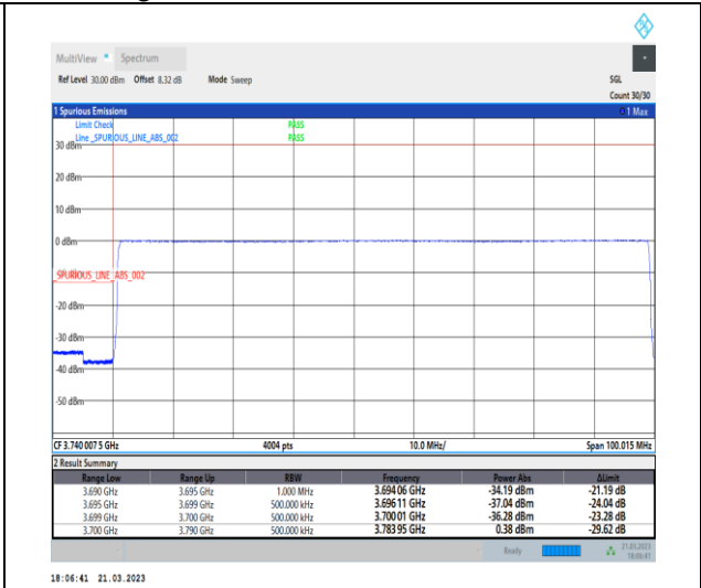
1-N78-3700-3800-30-90-L-6-CP-QPSK-Outer_Full -245@0-Ant0-1--PASS-see graph
