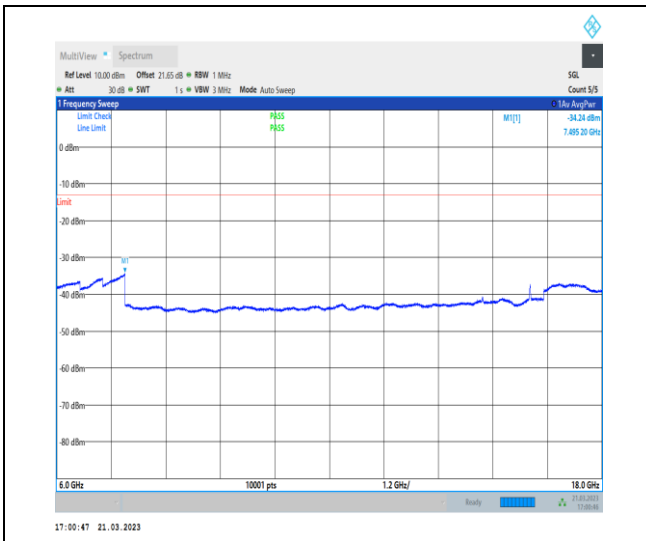
1-N78-3700-3800-30-100-H-1-DFT-QPSK-Edge_1R B_Left-1@0-6000-18000-Ant0-7495.20--34.24--13-P ASS
