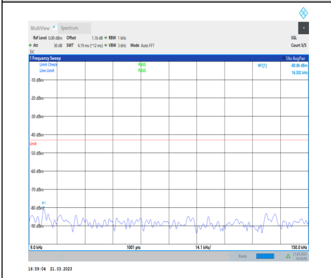
1-N78-3700-3800-30-100-M-1-DFT-QPSK-Edge_1R B_Left-1@0-0.009-0.15-Ant0-0.02--80.86--43-PASS
