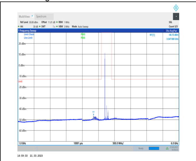
1-N78-3700-3800-30-100-M-1-DFT-QPSK-Edge_1R B_Left-1@0-1000-6000-Ant0-3347.00--46.15--13-PA SS
