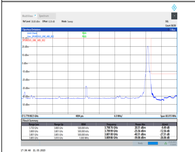
1-N78-3700-3800-30-50-H-5-CP-QPSK-Edge_1RB_Ri ght-1@132-Ant0-1--PASS-see graph
