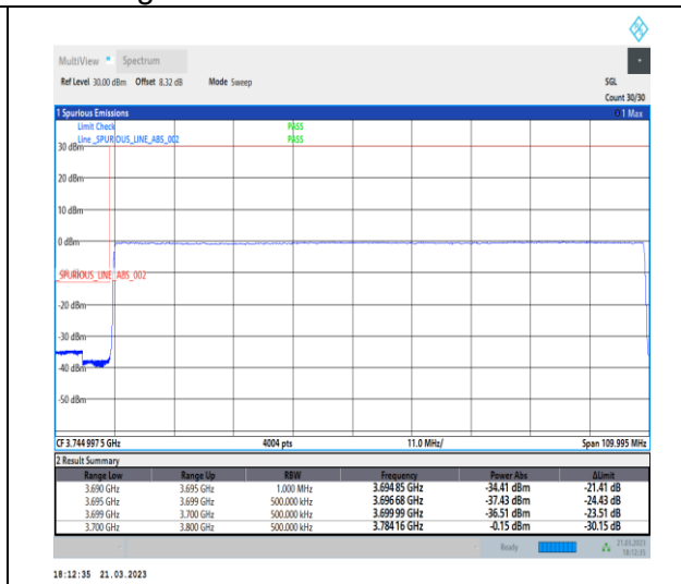
1-N78-3700-3800-30-100-L-6-CP-QPSK-Outer_Fu II-273@0-Ant0-1--PASS-see graph
