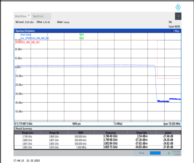
1-N78-3700-3800-30-60-H-6-CP-QPSK-Outer_Full -162@0-Ant0-1--PASS-see graph
