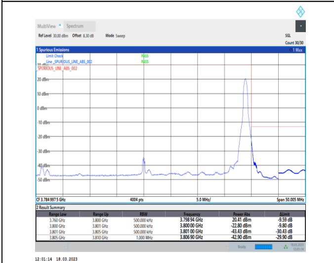
1-N78-3700-3800-30-40-H-5-CP-QPSK-Edge_1RB_Right-1@105-Ant0-1--PASS-see graph
