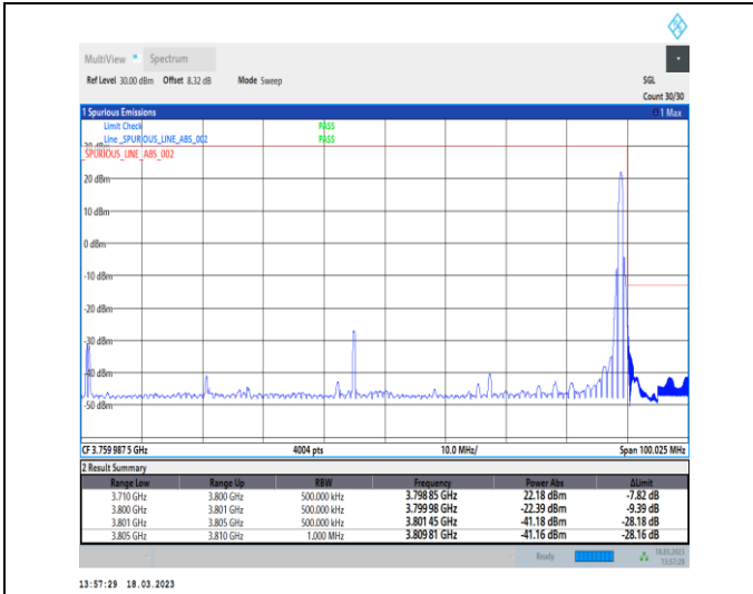
1-N78-3700-3800-30-90-H-2-DFT-PI2BPSK-Edge_1R_B_Right-1@244-Ant0-1--PASS-see graph
