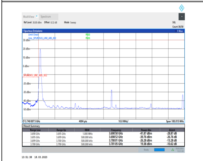
1-N78-3700-3800-30-90-L-4-CP-QPSK-Edge_1RB_Lef t-1@0-Ant0-1--PASS-see graph
