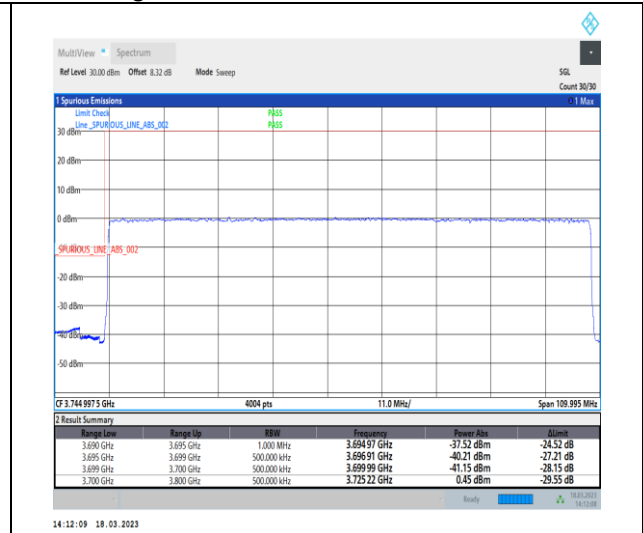
1-N78-3700-3800-30-100-L-3-DFT-PI2BPSK-Outer_Full-270@0-Ant0-1--PASS-see graph
