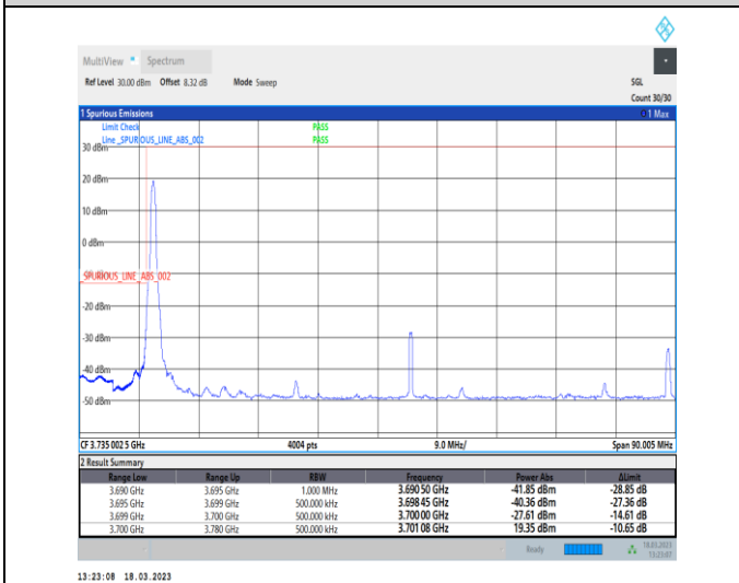
1-N78-3700-3800-30-80-L-4-CP-QPSK-Edge_1RB_Lef t-1@0-Ant0-1--PASS-see graph
