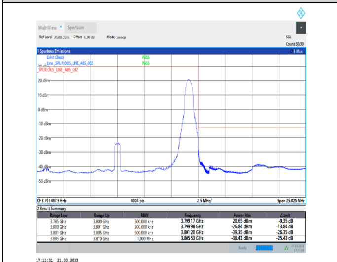
1-N78-3700-3800-30-15-H-5-CP-QPSK-Edge_1RB_Ri ght-1@37-Ant0-1--PASS-see graph
