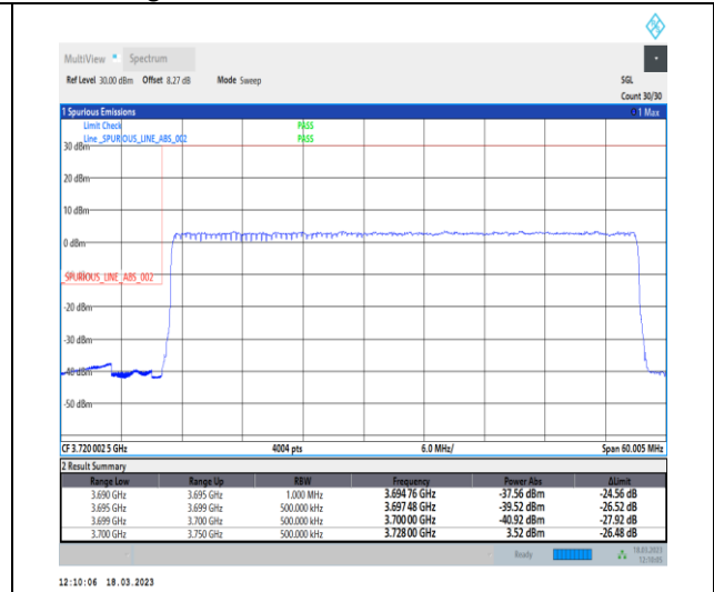
1-N78-3700-3800-30-50-L-3-DFT-PI2BPSK-Outer _Full-128@0-Ant0-1--PASS-see graph
