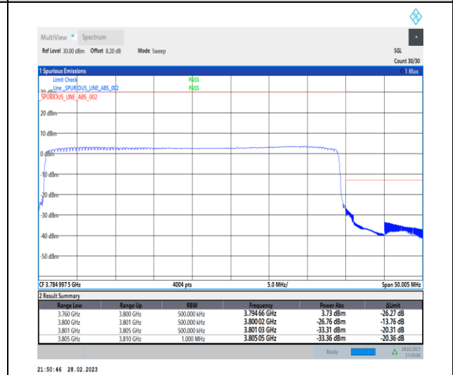
1-N78-3700-3800-30-40-H-6-CP-QPSK-Outer_Full-106@0-Ant0-1--PASS-see graph
