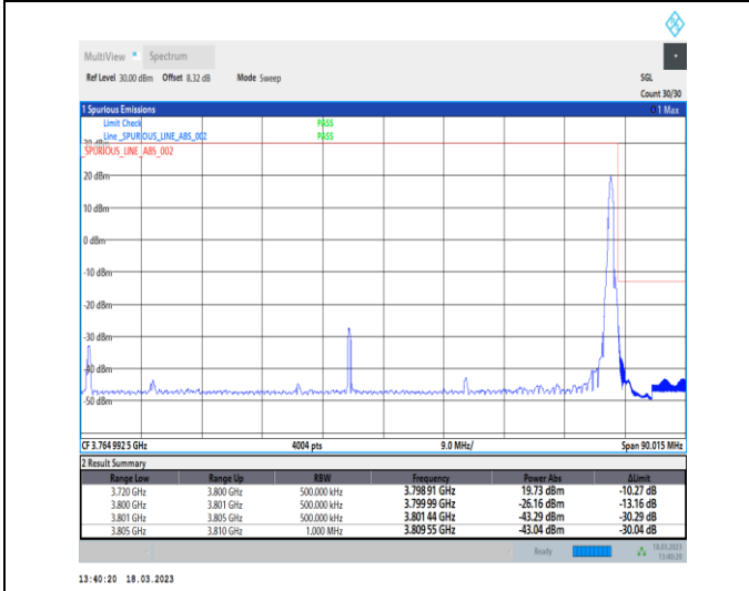
1-N78-3700-3800-30-80-H-5-CP-QPSK-Edge_1RB_Right-1@216-Ant0-1--PASS-see graph
