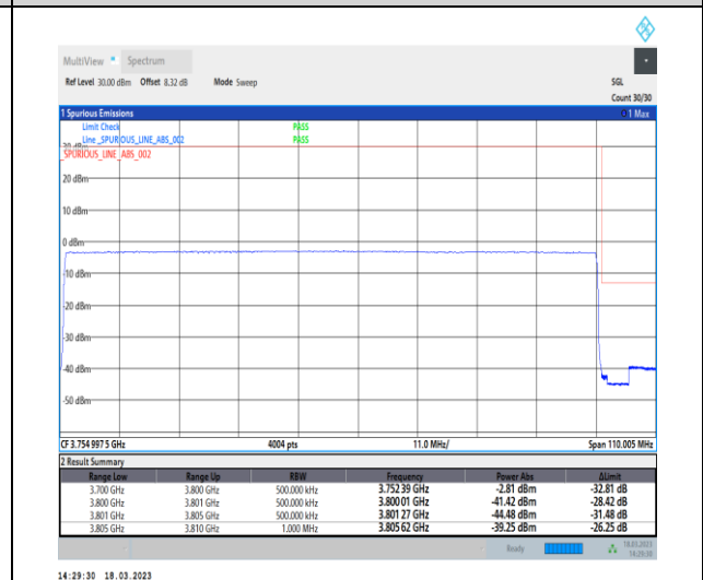
1-N78-3700-3800-30-100-H-6-CP-QPSK-Outer_Full-273@0-Ant0-1--PASS-see graph
