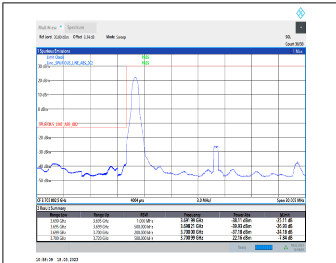
1-N78-3700-3800-30-20-L-1-DFT-PI2BPSK-Edge_1RB _Left-1@0-Ant0-1--PASS-see graph
