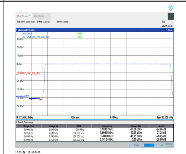
1-N78-3700-3800-30-50-L-6-CP-QPSK-Outer_Full -133@0-Ant0-1--PASS-see graph
