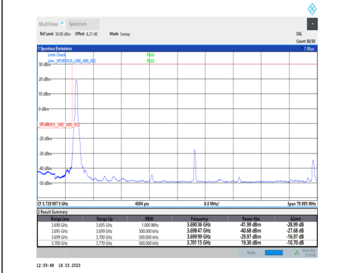
1-N78-3700-3800-30-70-L-4-CP-QPSK-Edge_1RB_Lef t-1@0-Ant0-1--PASS-see graph
