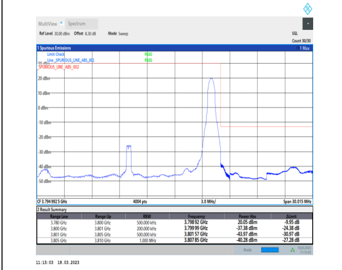
1-N78-3700-3800-30-20-H-5-CP-QPSK-Edge_1RB_Right-1@50-Ant0-1--PASS-see graph
