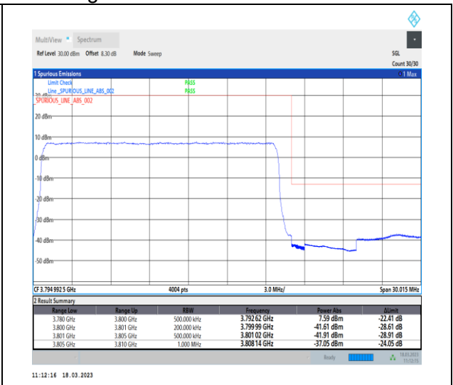
1-N78-3700-3800-30-20-H-3-DFT-PI2BPSK-Outer_Full-50@0-Ant0-1--PASS-see graph
