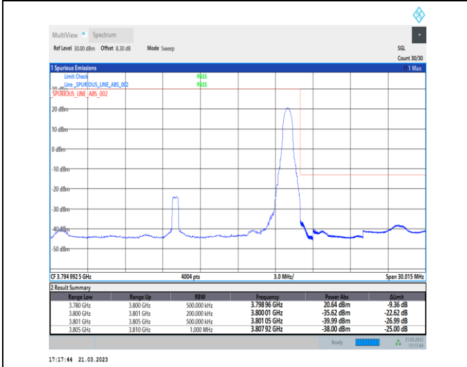
1-N78-3700-3800-30-20-H-5-CP-QPSK-Edge_1RB_Ri ght-1@50-Ant0-1--PASS-see graph
