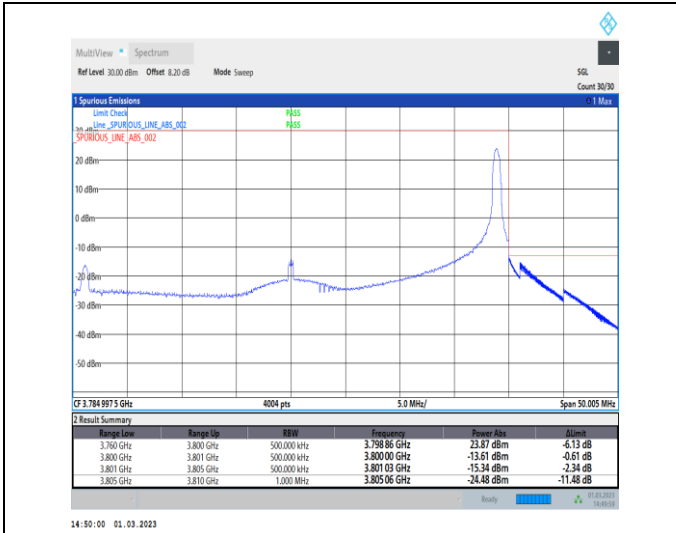
1-N78-3700-3800-30-40-H-2-DFT-PI2BPSK-Edge_1R_B_Right-1@105-Ant0-1--PASS-see graph
