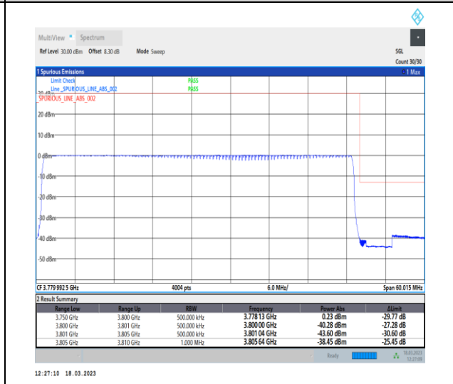
1-N78-3700-3800-30-50-H-6-CP-QPSK-Outer_Full-133@0-Ant0-1--PASS-see graph
