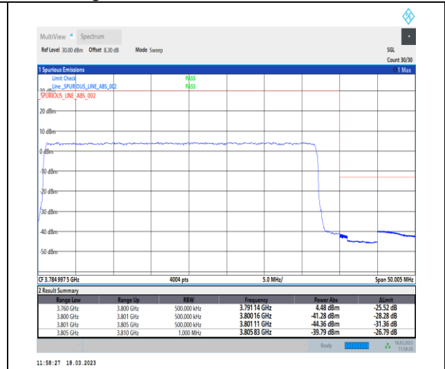
1-N78-3700-3800-30-40-H-3-DFT-PI2BPSK-Outer_Full-100@0-Ant0-1--PASS-see graph
