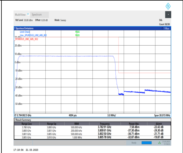
1-N78-3700-3800-30-20-H-6-CP-QPSK-Outer_Full -51@0-Ant0-1--PASS-see graph
