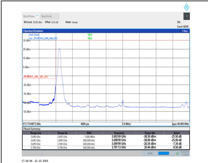
1-N78-3700-3800-30-40-L-4-CP-QPSK-Edge_1RB_Lef t-1@0-Ant0-1--PASS-see graph
