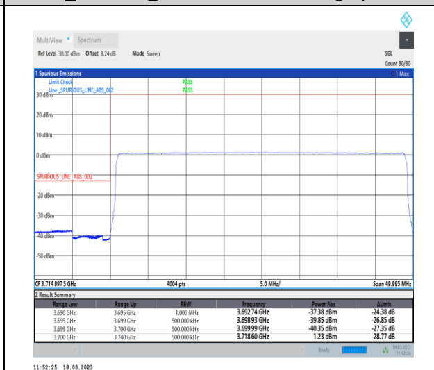
1-N78-3700-3800-30-40-L-6-CP-QPSK-Outer_Full -106@0-Ant0-1--PASS-see graph
