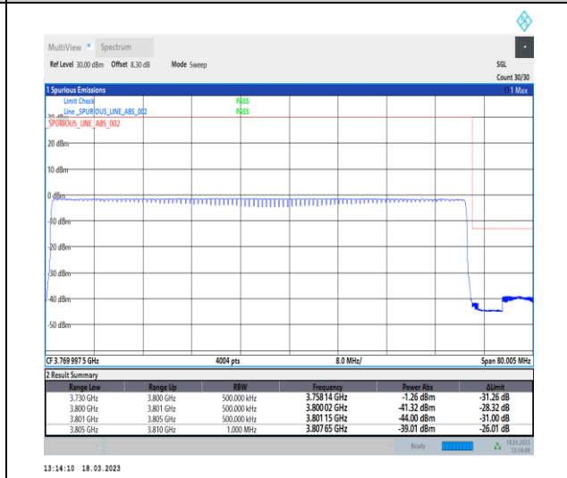
1-N78-3700-3800-30-70-H-6-CP-QPSK-Outer_Full-189@0-Ant0-1--PASS-see graph
