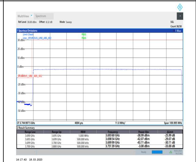
1-N78-3700-3800-30-100-L-6-CP-QPSK-Outer_Full-273@0-Ant0-1--PASS-see graph
