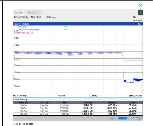
1-N78-3700-3800-30-60-H-6-CP-QPSK-Outer_Full-162@0-Ant0-1--PASS-see graph
