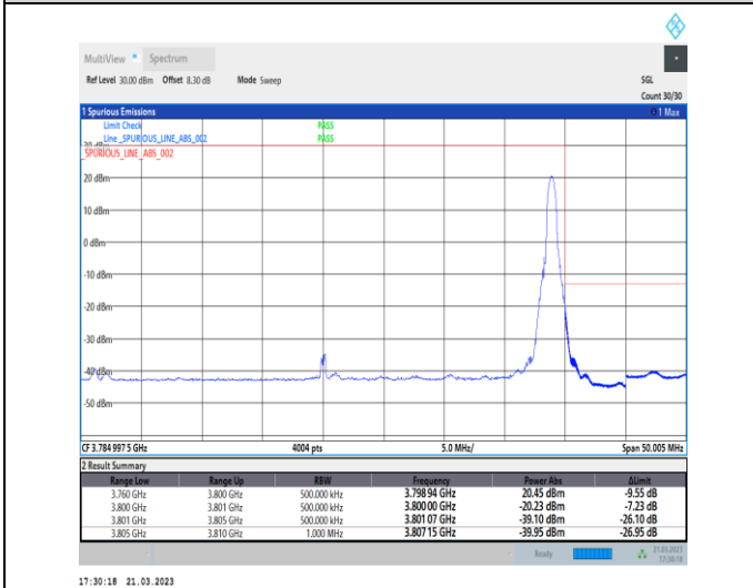
1-N78-3700-3800-30-40-H-5-CP-QPSK-Edge_1RB_Ri ght-1@105-Ant0-1--PASS-see graph
