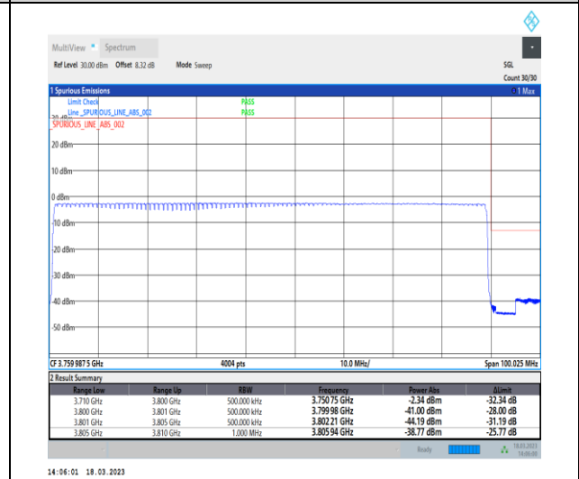
1-N78-3700-3800-30-90-H-6-CP-QPSK-Outer_Full-245@0-Ant0-1--PASS-see graph
