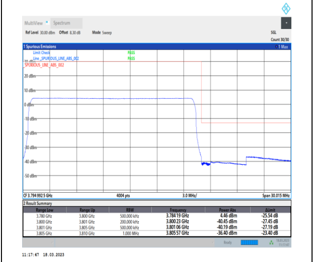
1-N78-3700-3800-30-20-H-6-CP-QPSK-Outer_Full-51@0-Ant0-1--PASS-see graph
