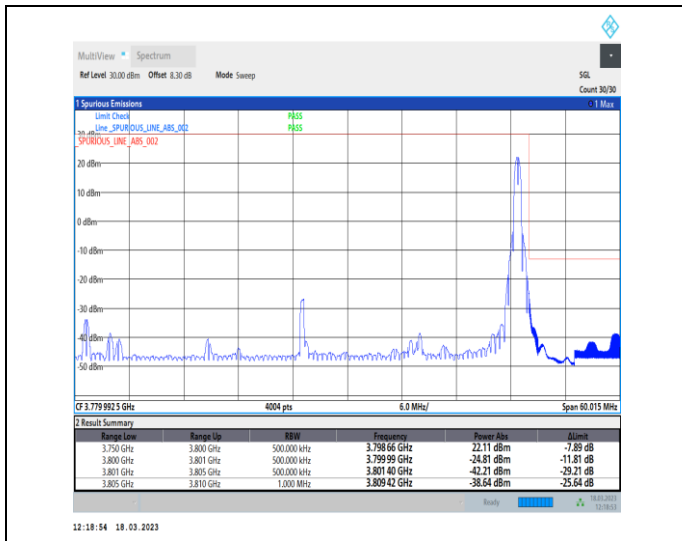
1-N78-3700-3800-30-50-H-2-DFT-PI2BPSK-Edge_1R_B_Right-1@132-Ant0-1--PASS-see graph
