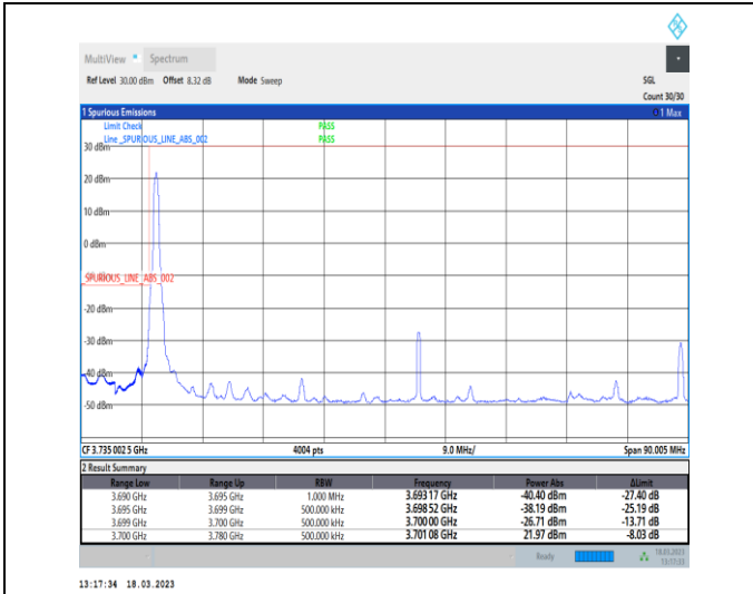
1-N78-3700-3800-30-80-L-1-DFT-PI2BPSK-Edge_1RB_Left-1@0-Ant0-1--PASS-see graph
