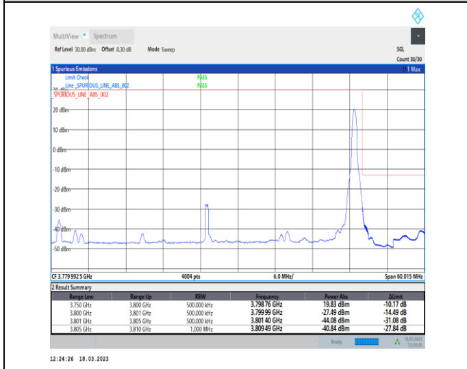
1-N78-3700-3800-30-50-H-5-CP-QPSK-Edge_1RB_Right-1@132-Ant0-1--PASS-see graph
