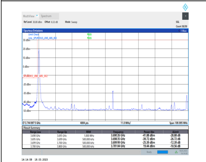
1-N78-3700-3800-30-100-L-4-CP-QPSK-Edge_1RB_Left-1@0-Ant0-1--PASS-see graph
