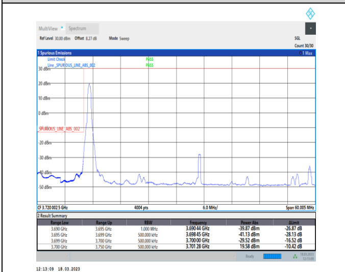
1-N78-3700-3800-30-50-L-4-CP-QPSK-Edge_1RB_Lef t-1@0-Ant0-1--PASS-see graph
