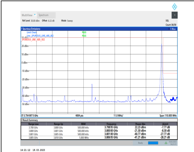
1-N78-3700-3800-30-100-H-2-DFT-PI2BPSK-Edge_1R_B_Right-1@272-Ant0-1--PASS-see graph
