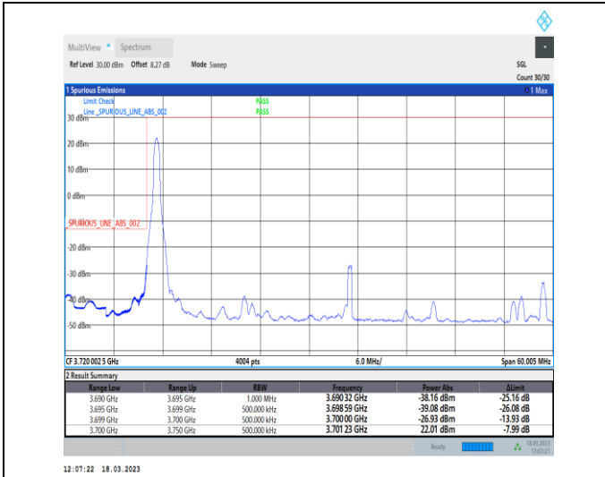
1-N78-3700-3800-30-50-L-1-DFT-PI2BPSK-Edge_1RB _Left-1@0-Ant0-1--PASS-see graph
