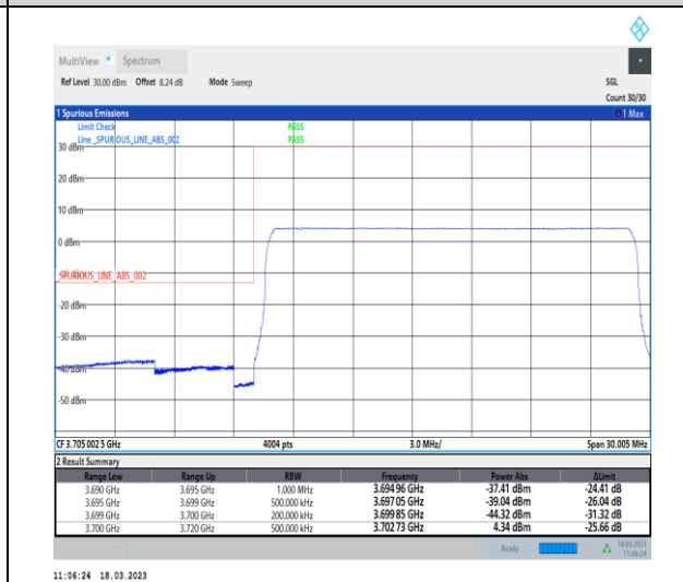
1-N78-3700-3800-30-20-L-6-CP-QPSK-Outer_Full -51@0-Ant0-1--PASS-see graph
