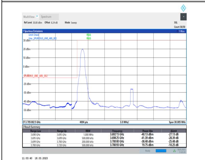
1-N78-3700-3800-30-20-L-4-CP-QPSK-Edge_1RB_Lef t-1@0-Ant0-1--PASS-see graph
