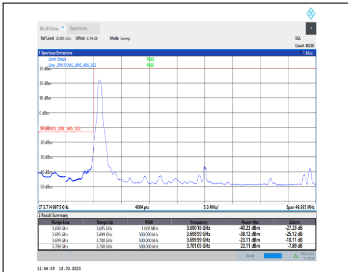
1-N78-3700-3800-30-40-L-1-DFT-PI2BPSK-Edge_1RB _Left-1@0-Ant0-1--PASS-see graph
