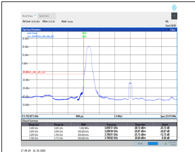
1-N78-3700-3800-30-15-L-4-CP-QPSK-Edge_1RB_Lef t-1@0-Ant0-1--PASS-see graph
