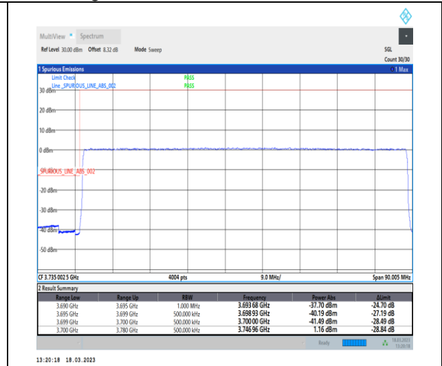
1-N78-3700-3800-30-80-L-3-DFT-PI2BPSK-Outer_Full-216@0-Ant0-1--PASS-see graph
