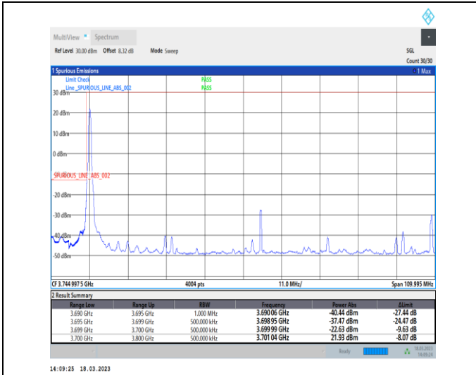
1-N78-3700-3800-30-100-L-1-DFT-PI2BPSK-Edge_1R_B_Left-1@0-Ant0-1--PASS-see graph
