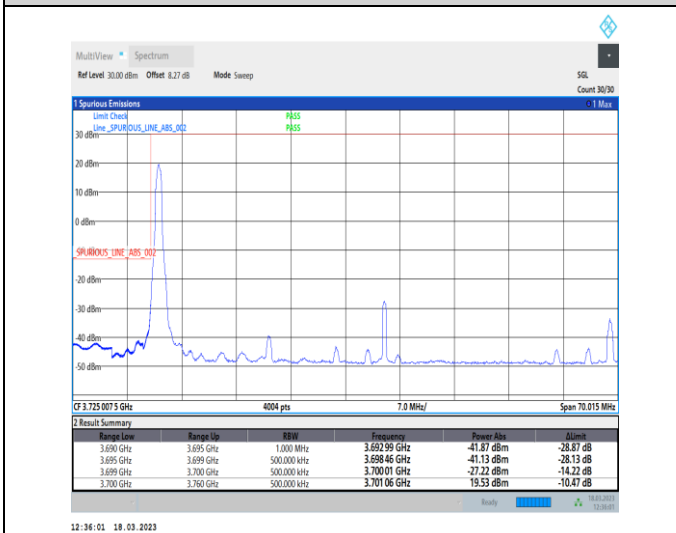
1-N78-3700-3800-30-60-L-4-CP-QPSK-Edge_1RB_Lef t-1@0-Ant0-1--PASS-see graph
