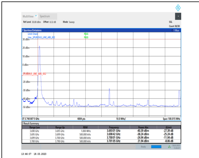
1-N78-3700-3800-30-90-L-1-DFT-PI2BPSK-Edge_1RB _Left-1@0-Ant0-1--PASS-see graph
