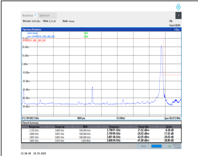
1-N78-3700-3800-30-80-H-2-DFT-PI2BPSK-Edge_1R_B_Right-1@216-Ant0-1--PASS-see graph
