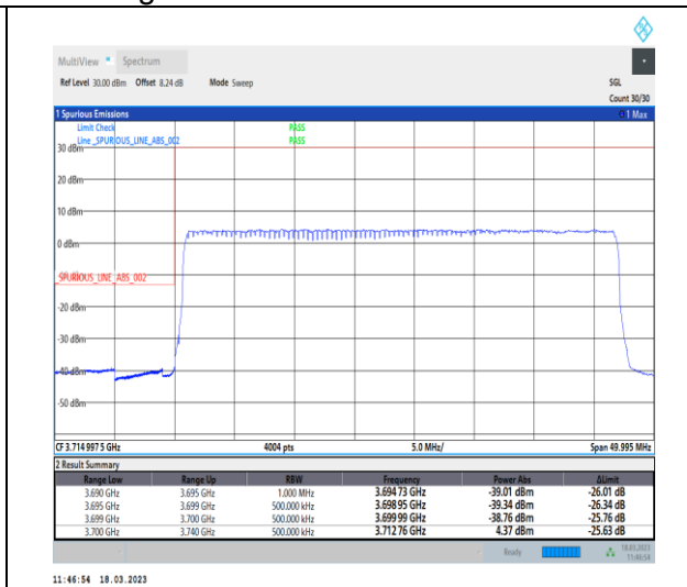
1-N78-3700-3800-30-40-L-3-DFT-PI2BPSK-Outer _Full-100@0-Ant0-1--PASS-see graph
