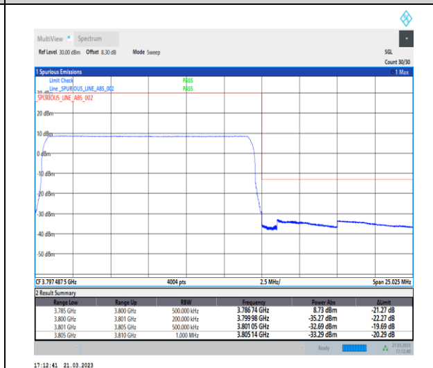
1-N78-3700-3800-30-15-H-6-CP-QPSK-Outer_Full -38@0-Ant0-1--PASS-see graph
