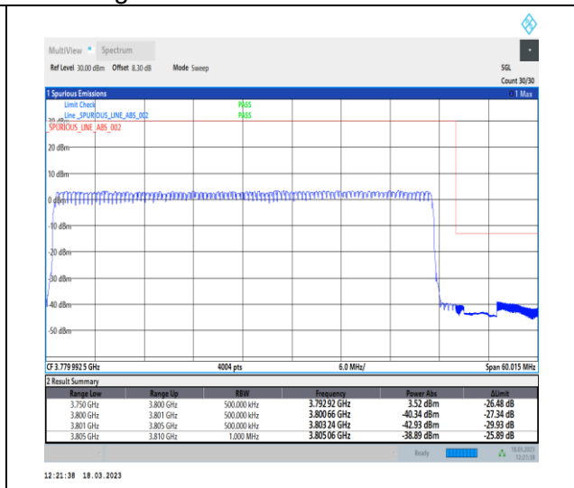
1-N78-3700-3800-30-50-H-3-DFT-PI2BPSK-Outer_Full-128@0-Ant0-1--PASS-see graph
