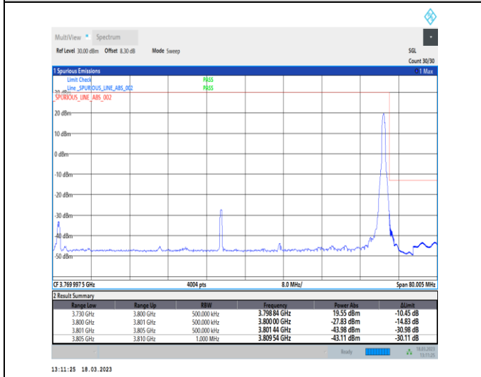
1-N78-3700-3800-30-70-H-5-CP-QPSK-Edge_1RB_Right-1@188-Ant0-1--PASS-see graph
