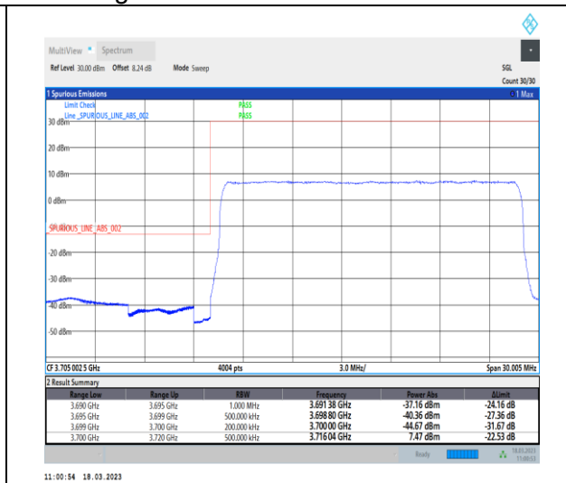
1-N78-3700-3800-30-20-L-3-DFT-PI2BPSK-Outer _Full-50@0-Ant0-1--PASS-see graph
