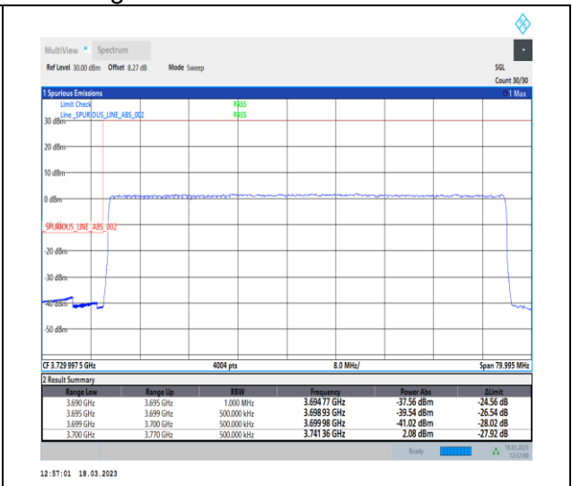
1-N78-3700-3800-30-70-L-3-DFT-PI2BPSK-Outer_Full-180@0-Ant0-1--PASS-see graph
