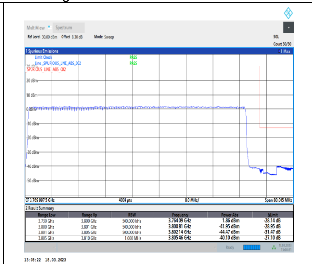
1-N78-3700-3800-30-70-H-3-DFT-PI2BPSK-Outer_Full-180@0-Ant0-1--PASS-see graph
