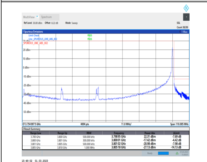
1-N78-3700-3800-30-100-H-5-CP-QPSK-Edge_1RB_Right-1@272-Ant0-1--PASS-see graph
