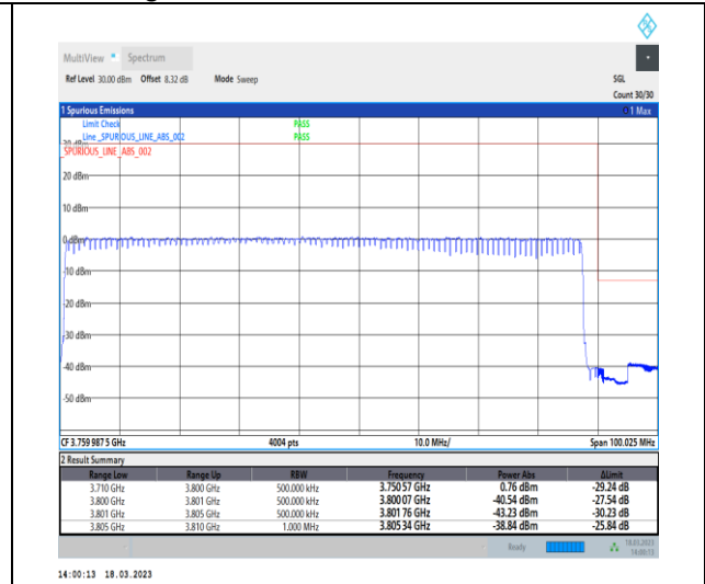
1-N78-3700-3800-30-90-H-3-DFT-PI2BPSK-Outer_Full-240@0-Ant0-1--PASS-see graph
