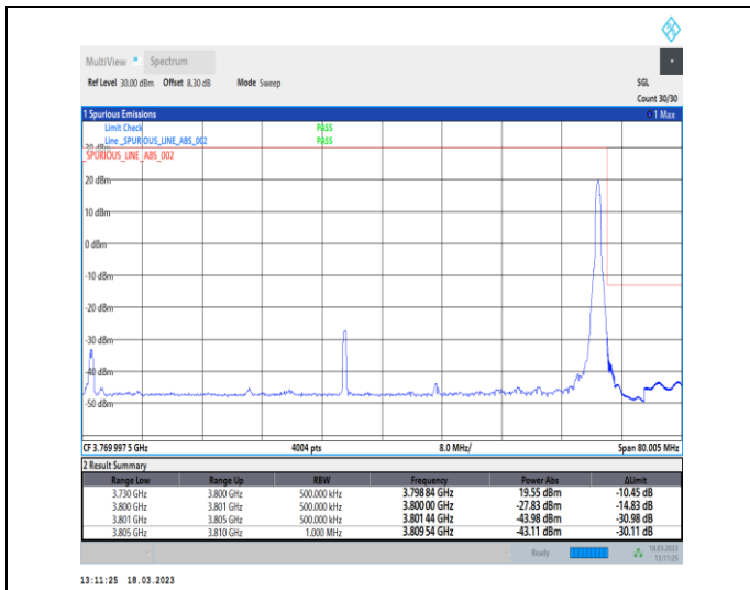
1-N78-3700-3800-30-70-H-2-DFT-PI2BPSK-Edge_1R_B_Right-1@188-Ant0-1--PASS-see graph
