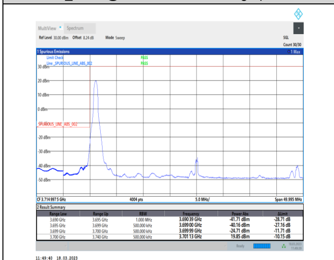
1-N78-3700-3800-30-40-L-4-CP-QPSK-Edge_1RB_Lef t-1@0-Ant0-1--PASS-see graph
