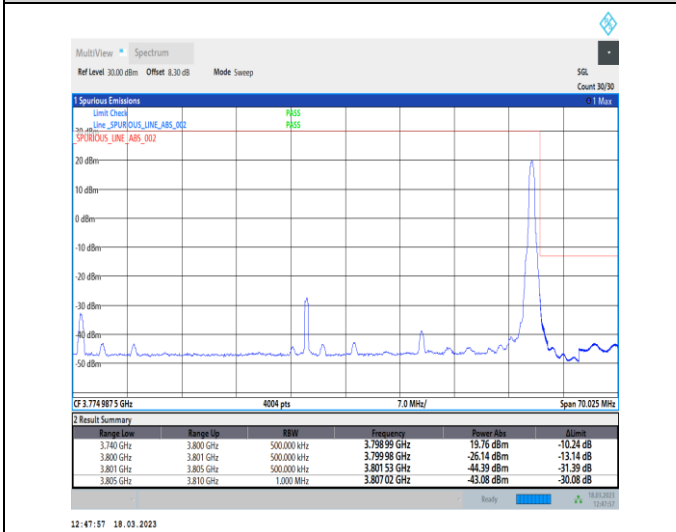
1-N78-3700-3800-30-60-H-5-CP-QPSK-Edge_1RB_Right-1@161-Ant0-1--PASS-see graph
