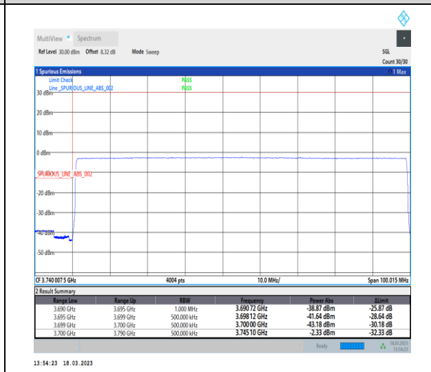
1-N78-3700-3800-30-90-L-6-CP-QPSK-Outer_Full -245@0-Ant0-1--PASS-see graph
