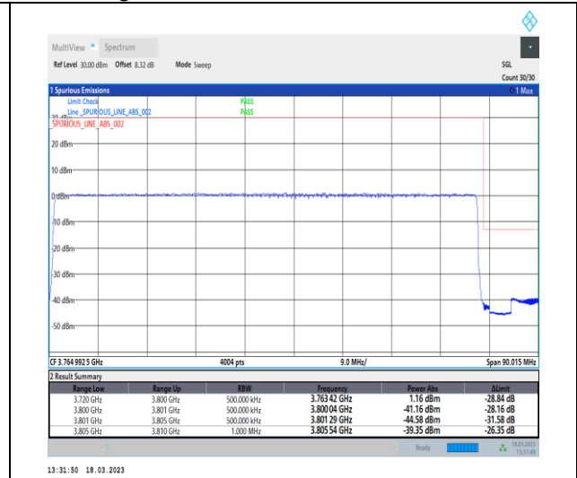
1-N78-3700-3800-30-80-H-3-DFT-PI2BPSK-Outer_Full-216@0-Ant0-1--PASS-see graph
