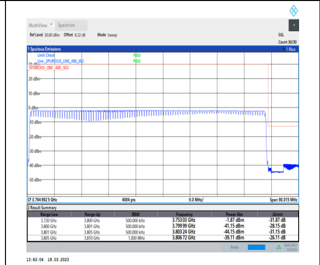
1-N78-3700-3800-30-80-H-6-CP-QPSK-Outer_Full-217@0-Ant0-1--PASS-see graph
