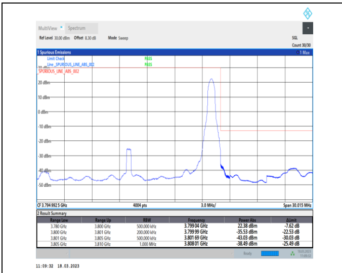
1-N78-3700-3800-30-20-H-2-DFT-PI2BPSK-Edge_1R_B_Right-1@50-Ant0-1--PASS-see graph
