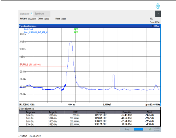
1-N78-3700-3800-30-20-L-4-CP-QPSK-Edge_1RB_Lef t-1@0-Ant0-1--PASS-see graph
