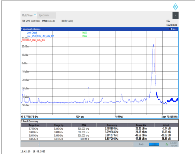
1-N78-3700-3800-30-60-H-2-DFT-PI2BPSK-Edge_1R_B_Right-1@161-Ant0-1--PASS-see graph
