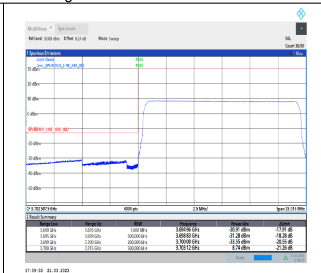
1-N78-3700-3800-30-15-L-6-CP-QPSK-Outer_Full -38@0-Ant0-1--PASS-see graph
