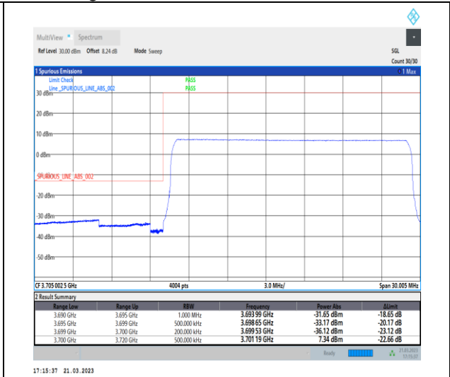
1-N78-3700-3800-30-20-L-6-CP-QPSK-Outer_Full -51@0-Ant0-1--PASS-see graph
