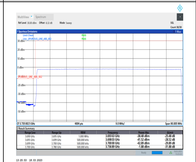
1-N78-3700-3800-30-80-L-6-CP-QPSK-Outer_Full -217@0-Ant0-1--PASS-see graph
