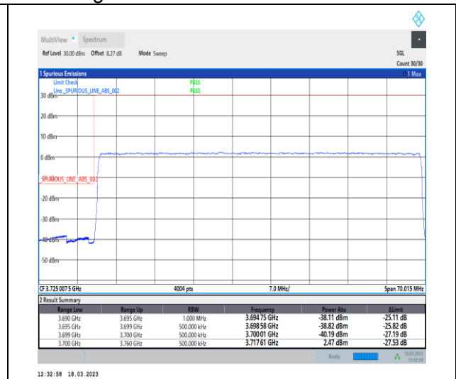
1-N78-3700-3800-30-60-L-3-DFT-PI2BPSK-Outer _Full-162@0-Ant0-1--PASS-see graph
