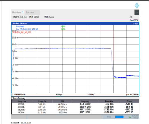
1-N78-3700-3800-30-40-H-6-CP-QPSK-Outer_Full -106@0-Ant0-1--PASS-see graph
