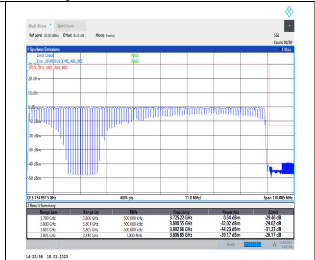
1-N78-3700-3800-30-100-H-3-DFT-PI2BPSK-Outer_Full-270@0-Ant0-1--PASS-see graph
