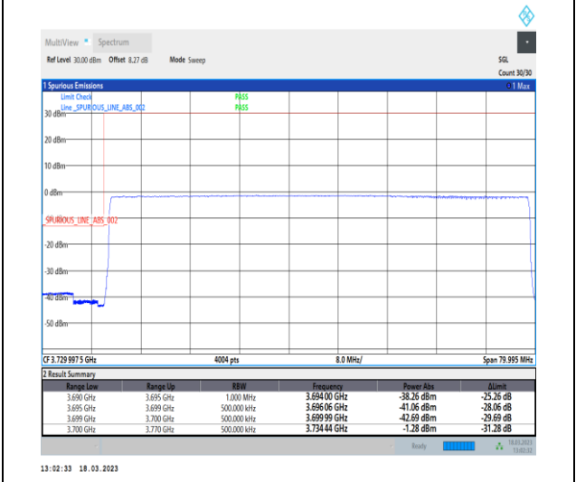
1-N78-3700-3800-30-70-L-6-CP-QPSK-Outer_Full -189@0-Ant0-1--PASS-see graph
