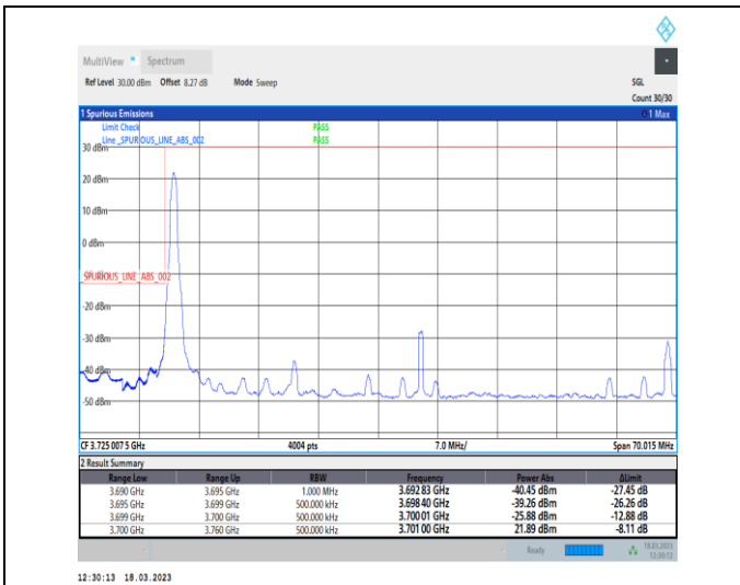
1-N78-3700-3800-30-60-L-1-DFT-PI2BPSK-Edge_1RB _Left-1@0-Ant0-1--PASS-see graph
