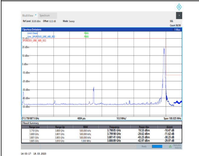
1-N78-3700-3800-30-90-H-5-CP-QPSK-Edge_1RB_Right-1@244-Ant0-1--PASS-see graph
