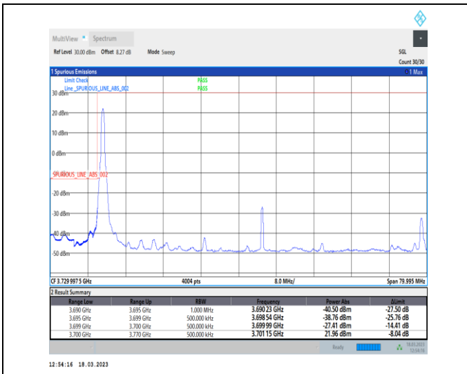
1-N78-3700-3800-30-70-L-1-DFT-PI2BPSK-Edge_1RB_Left-1@0-Ant0-1--PASS-see graph
