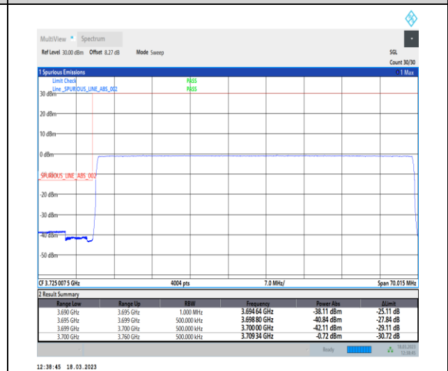
1-N78-3700-3800-30-60-L-6-CP-QPSK-Outer_Full -162@0-Ant0-1--PASS-see graph
