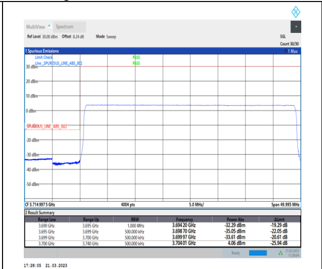
1-N78-3700-3800-30-40-L-6-CP-QPSK-Outer_Full -106@0-Ant0-1--PASS-see graph
