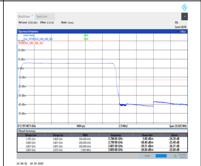
1-N78-3700-3800-30-15-H-6-CP-QPSK-Outer_Full-38@0-Ant0-1--PASS-see graph
