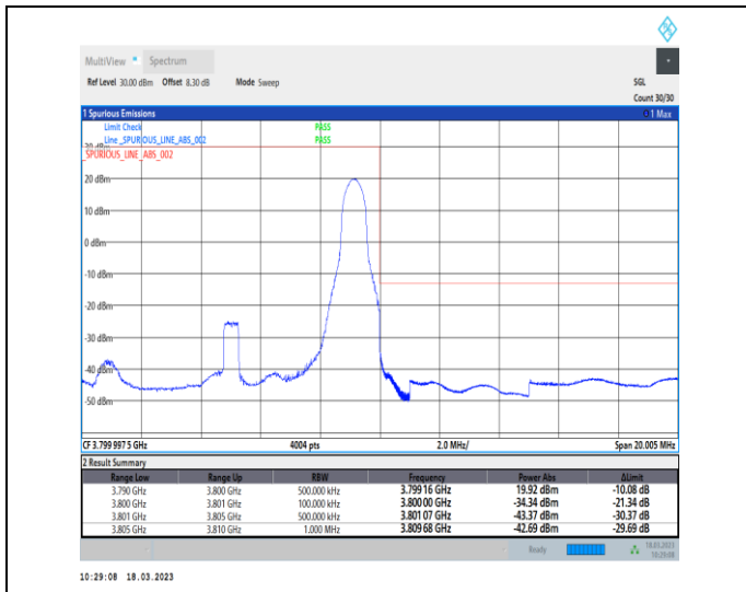
1-N78-3700-3800-30-10-H-2-DFT-PI2BPSK-Edge_1R_B_Right-1@23-Ant0-1--PASS-see graph
