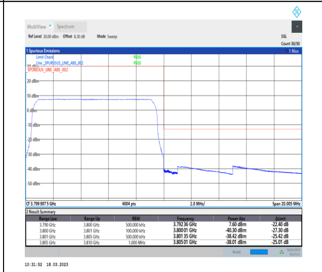
1-N78-3700-3800-30-10-H-6-CP-QPSK-Outer_Full-24@0-Ant0-1--PASS-see graph
