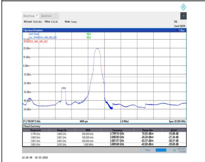
1-N78-3700-3800-30-10-H-5-CP-QPSK-Edge_1RB_Right-1@23-Ant0-1--PASS-see graph
