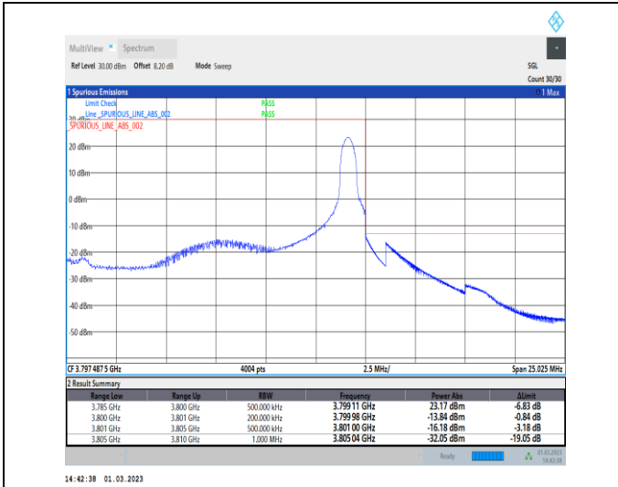
1-N78-3700-3800-30-15-H-2-DFT-PI2BPSK-Edge_1R_B_Right-1@37-Ant0-1--PASS-see graph
