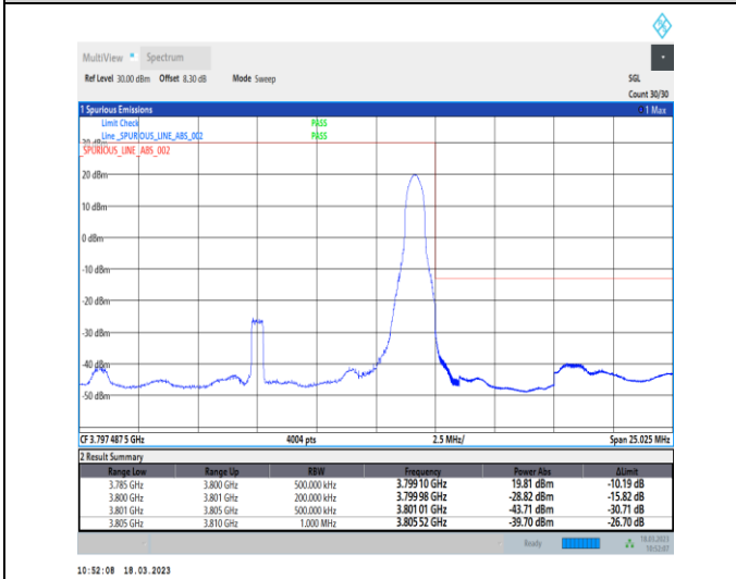
1-N78-3700-3800-30-15-H-5-CP-QPSK-Edge_1RB_Right-1@37-Ant0-1--PASS-see graph
