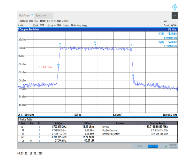
1-N78-3700-3800-30-40-L-3-DFT-16QAM-Outer_Full -100@0-Ant0-35.715-37.360-≤40-PASS
