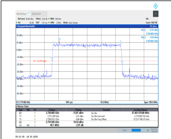
1-N78-3700-3800-30-50-H-6-CP-QPSK-Outer_Full-1 33@0-Ant0-47.401-49.100-≤50-PASS
