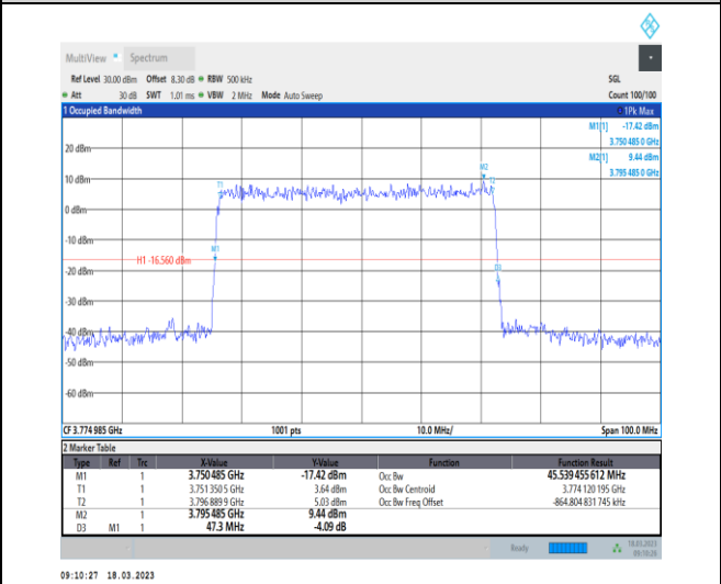
1-N78-3700-3800-30-50-H-5-DFT-256QAM-Outer_Full-128@0-Ant0-45.539-47.300-≤50-PASS
