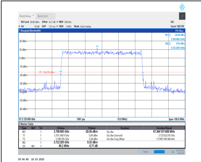
1-N78-3700-3800-30-50-L-8-CP-64QAM-Outer_Full-133@0-Ant0-47.364-49.200-≤50-PASS
