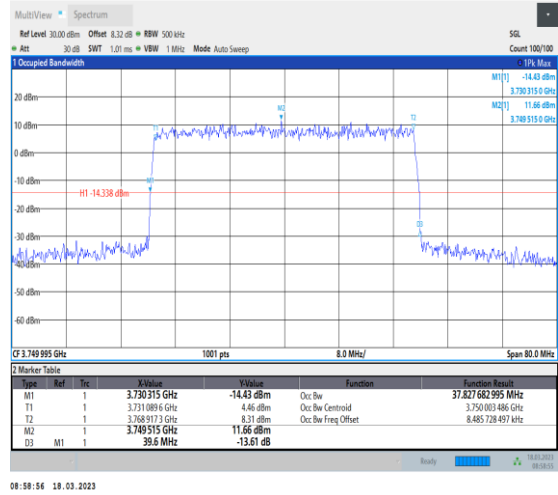
1-N78-3700-3800-30-40-M-7-CP-16QAM-Outer_Full-106@0-Ant0-37.828-39.600-≤40-PASS
