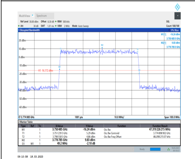
1-N78-3700-3800-30-50-H-8-CP-64QAM-Outer_Full-133@0-Ant0-47.319-49.200-≤50-PASS
