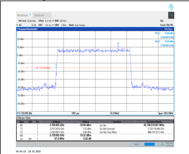
1-N78-3700-3800-30-50-L-5-DFT-256QAM-Outer_Full-128@0-Ant0-45.747-47.400-≤50-PASS
