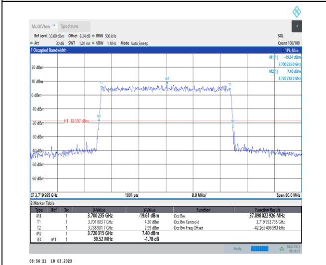
1-N78-3700-3800-30-40-L-9-CP-256QAM-Outer_Full-106@0-Ant0-37.898-39.520-≤40-PASS
