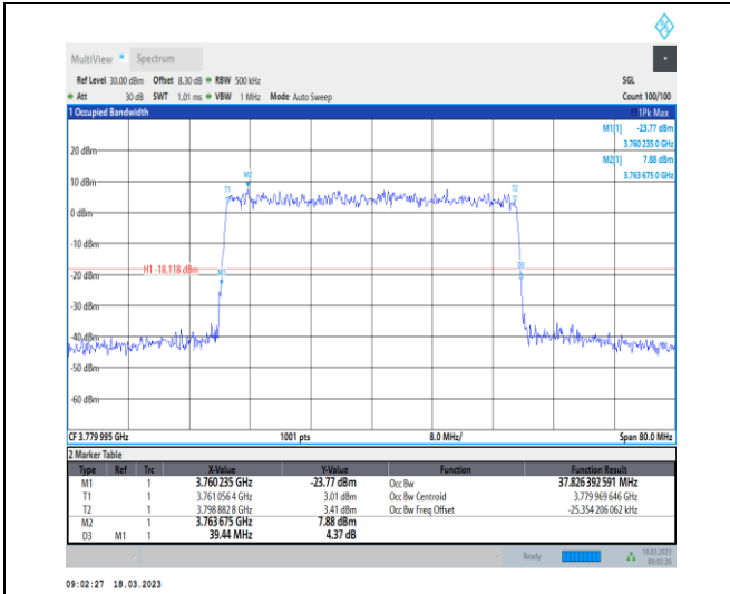
1-N78-3700-3800-30-40-H-9-CP-256QAM-Outer_Ful I-106@0-Ant0-37.826-39.440-≤40-PASS
