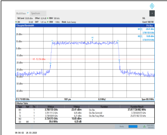
1-N78-3700-3800-30-40-L-7-CP-16QAM-Outer_Full-106@0-Ant0-37.818-39.600-≤40-PASS
