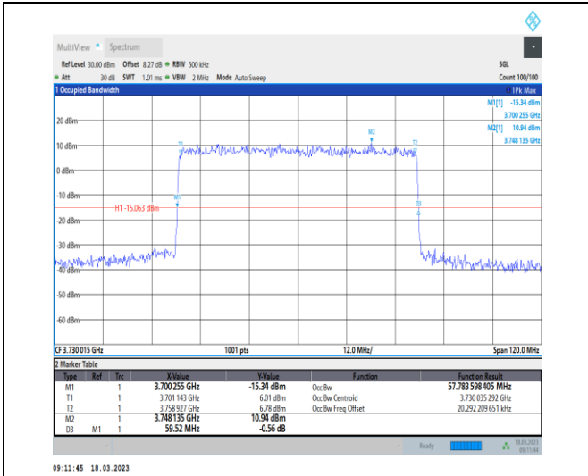
1-N78-3700-3800-30-60-L-1-DFT-QPSK-Outer_Full-162@0-Ant0-57.784-59.520-≤60-PASS
