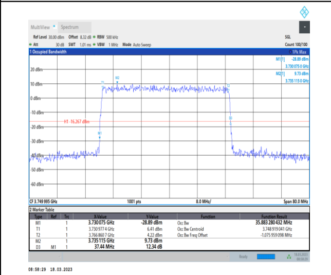
1-N78-3700-3800-30-40-M-5-DFT-256QAM-Outer_Full-100@0-Ant0-35.883-37.440-≤40-PASS
