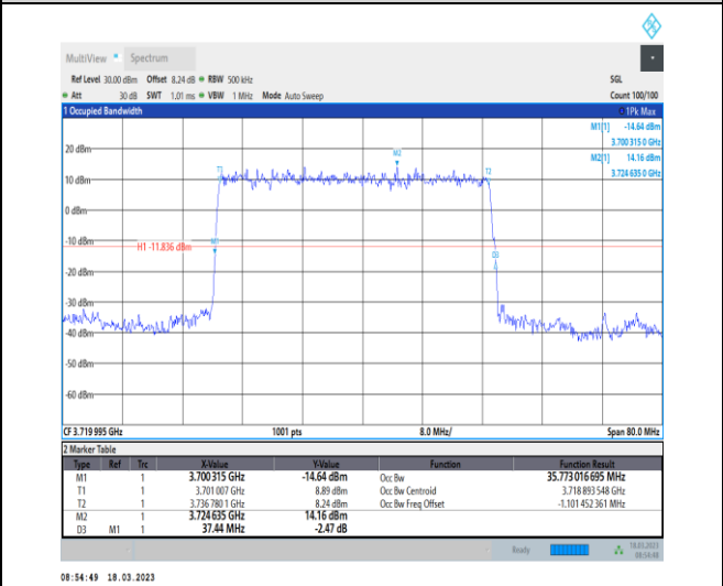
1-N78-3700-3800-30-40-L-2-DFT-PI2BPSK-Outer_Full-100@0-Ant0-35.773-37.440-≤40-PASS
