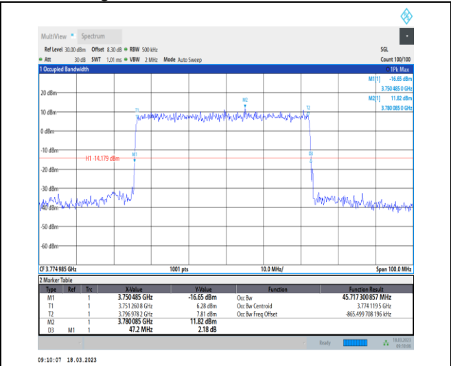
1-N78-3700-3800-30-50-H-3-DFT-16QAM-Outer_Full-128@0-Ant0-45.717-47.200-≤50-PASS
