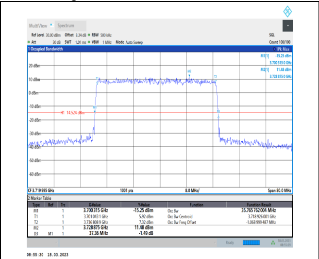
1-N78-3700-3800-30-40-L-4-DFT-64QAM-Outer_Full -100@0-Ant0-35.766-37.360-≤40-PASS
