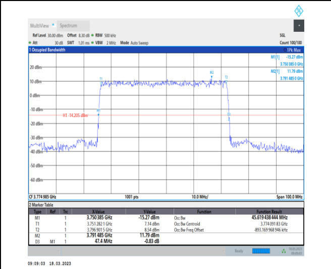
1-N78-3700-3800-30-50-H-1-DFT-QPSK-Outer_Full-128@0-Ant0-45.619-47.400-≤50-PASS
