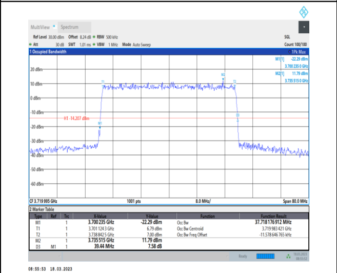
1-N78-3700-3800-30-40-L-6-CP-QPSK-Outer_Full-1 06@0-Ant0-37.718-39.440-≤40-PASS
