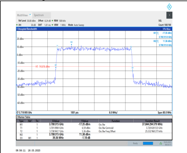
1-N78-3700-3800-30-40-L-8-CP-64QAM-Outer_Full-106@0-Ant0-37.844-39.360-≤40-PASS
