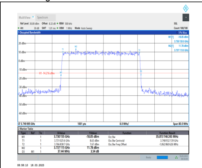
1-N78-3700-3800-30-40-M-3-DFT-16QAM-Outer_Full-100@0-Ant0-35.813-37.440-≤40-PASS
