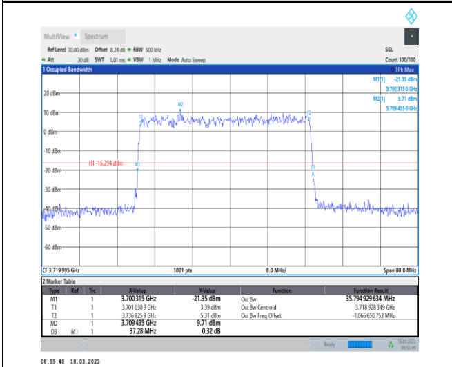
1-N78-3700-3800-30-40-L-5-DFT-256QAM-Outer_Fu II-100@0-Ant0-35.795-37.280-≤40-PASS
