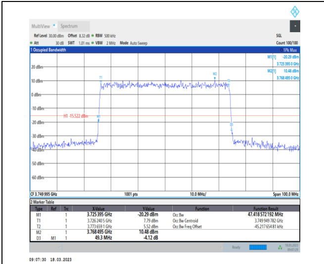
1-N78-3700-3800-30-50-M-7-CP-16QAM-Outer_Full-133@0-Ant0-47.419-49.300-≤50-PASS
