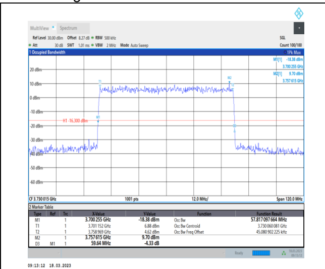
1-N78-3700-3800-30-60-L-6-CP-QPSK-Outer_Full-1 62@0-Ant0-57.817-59.640-≤60-PASS
