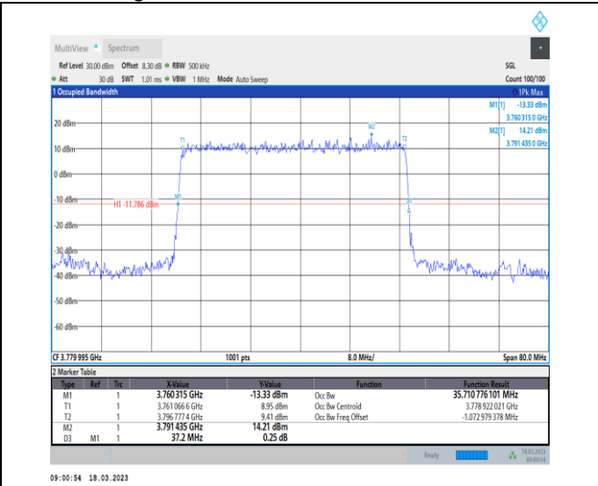
1-N78-3700-3800-30-40-H-2-DFT-PI2BPSK-Outer_Full-100@0-Ant0-35.711-37.200-≤40-PASS
