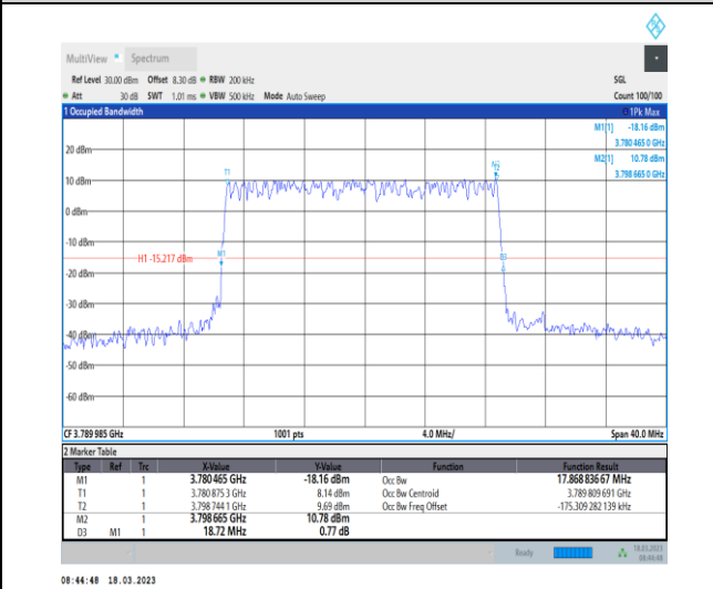
1-N78-3700-3800-30-20-H-4-DFT-64QAM-Outer_Full-50@0-Ant0-17.869-18.720-≤20-PASS
