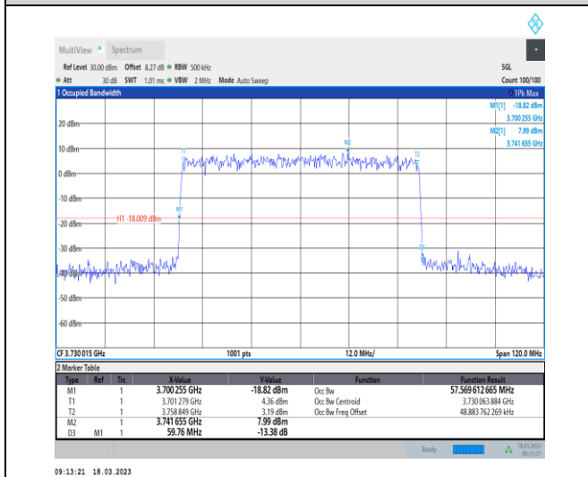
1-N78-3700-3800-30-60-L-7-CP-16QAM-Outer_Full-162@0-Ant0-57.57-59.760-≤60-PASS
