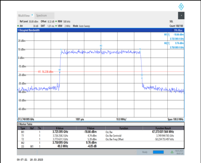
1-N78-3700-3800-30-50-M-6-CP-QPSK-Outer_Full-133@0-Ant0-47.373-49.300-≤50-PASS
