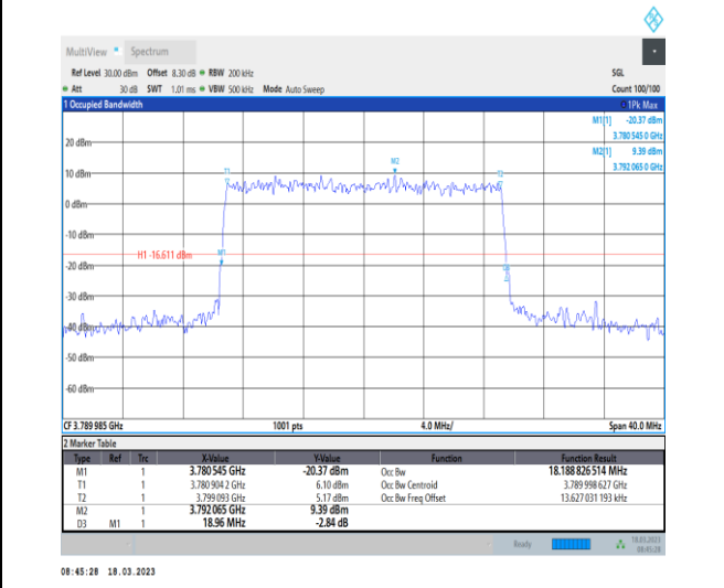
1-N78-3700-3800-30-20-H-8-CP-64QAM-Outer_Full-51@0-Ant0-18.189-18.960-≤20-PASS
