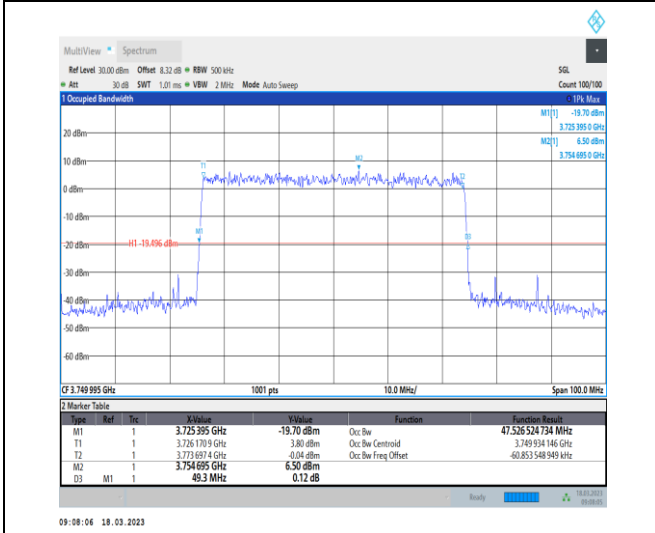
1-N78-3700-3800-30-50-M-9-CP-256QAM-Outer_Ful-1-133@0-Ant0-47.527-49.300-≤50-PASS
