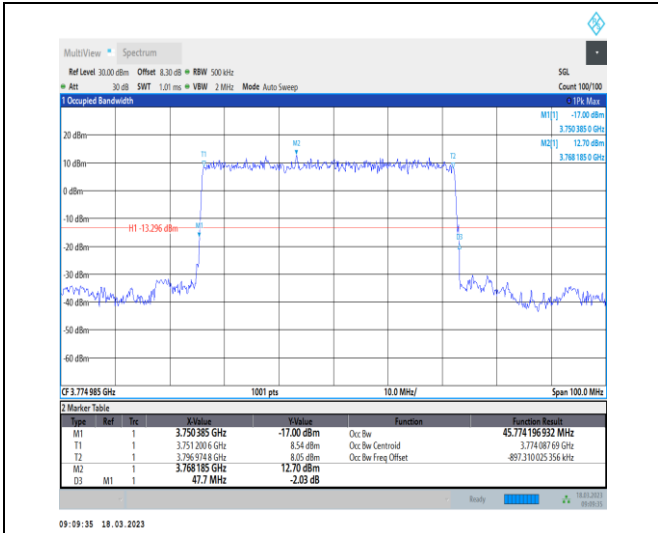
1-N78-3700-3800-30-50-H-2-DFT-PI2BPSK-Outer_Full-128@0-Ant0-45.774-47.700-≤50-PASS
