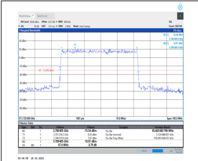
1-N78-3700-3800-30-50-L-4-DFT-64QAM-Outer_Full -128@0-Ant0-45.664-47.400-≤50-PASS
