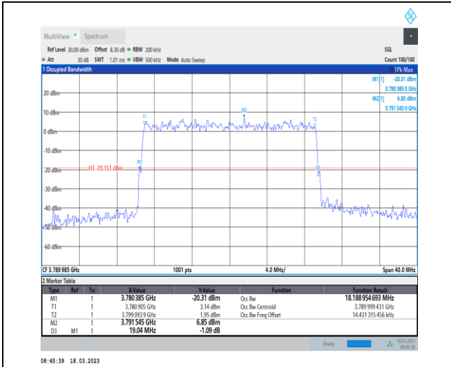
1-N78-3700-3800-30-20-H-9-CP-256QAM-Outer_Ful I-51@0-Ant0-18.189-19.040-≤20-PASS
