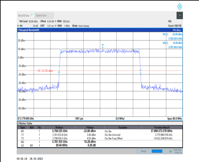
1-N78-3700-3800-30-40-H-8-CP-64QAM-Outer_Full-106@0-Ant0-37.89-39.440-≤40-PASS
