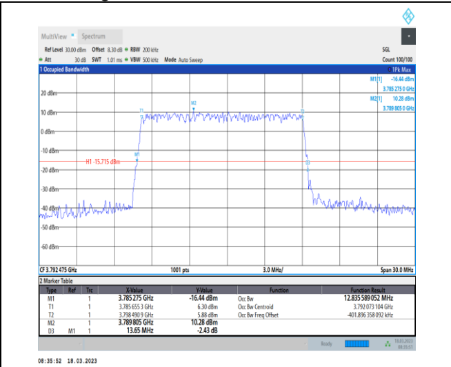
1-N78-3700-3800-30-15-H-5-DFT-256QAM-Outer_Full-I-36@0-Ant0-12.836-13.650-≤15-PASS
