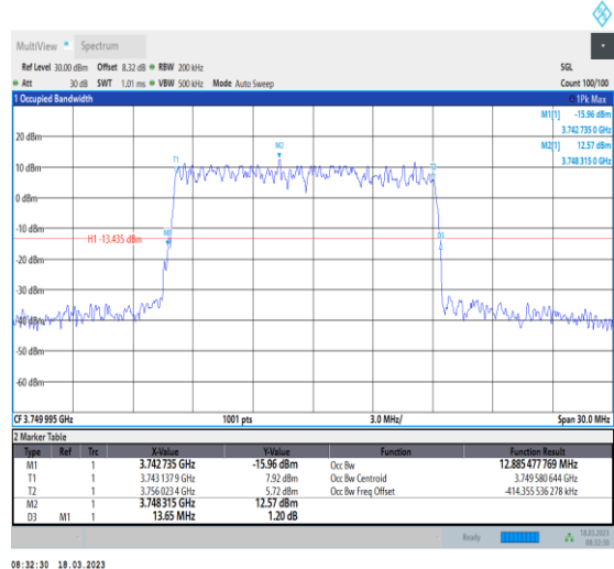
1-N78-3700-3800-30-15-M-4-DFT-64QAM-Outer_Full-36@0-Ant0-12.885-13.650-≤15-PASS
