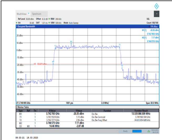
1-N78-3700-3800-30-15-M-9-CP-256QAM-Outer_Ful I-38@0-Ant0-13.535-14.460-≤15-PASS
