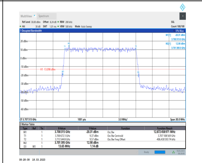
1-N78-3700-3800-30-15-L-1-DFT-QPSK-Outer_Full-36@0-Ant0-12.872-13.650-≤15-PASS
