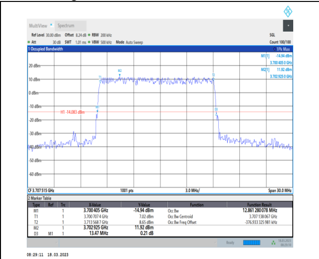
1-N78-3700-3800-30-15-L-3-DFT-16QAM-Outer_Full-36@0-Ant0-12.861-13.470-≤15-PASS
