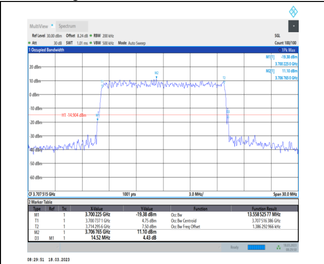
1-N78-3700-3800-30-15-L-7-CP-16QAM-Outer_Full-38@0-Ant0-13.559-14.520-≤15-PASS
