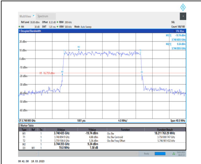
1-N78-3700-3800-30-20-M-6-CP-QPSK-Outer_Full-5 1@0-Ant0-18.212-19.000-≤20-PASS
