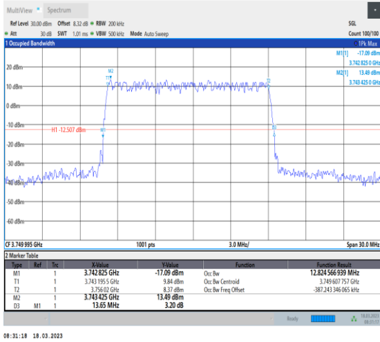
1-N78-3700-3800-30-15-M-1-DFT-QPSK-Outer_Full-36@0-Ant0-12.825-13.650-≤15-PASS
