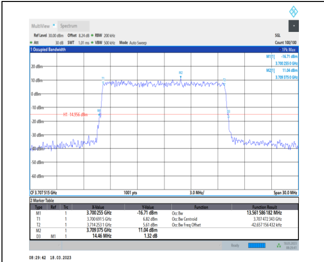
1-N78-3700-3800-30-15-L-6-CP-QPSK-Outer_Full-38@0-Ant0-13.562-14.460-≤15-PASS
