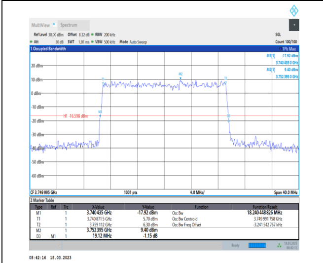
1-N78-3700-3800-30-20-M-8-CP-64QAM-Outer_Full-51@0-Ant0-18.24-19.120-≤20-PASS
