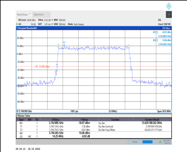
1-N78-3700-3800-30-15-M-8-CP-64QAM-Outer_Full-38@0-Ant0-13.62-14.250-≤15-PASS
