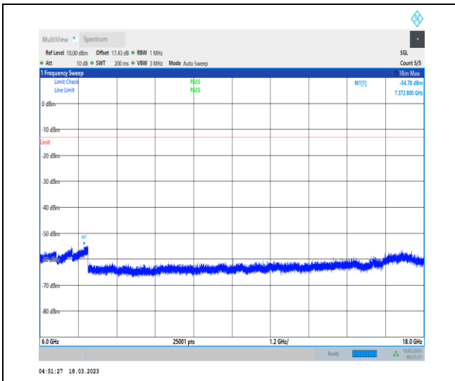
1-N78-3450-3550-30-100-H-1-DFT-PI2BPSK-Inner_1RB_Left-1@1-6000-18000-Ant0-7372.80--54.78--1 3-PASS
