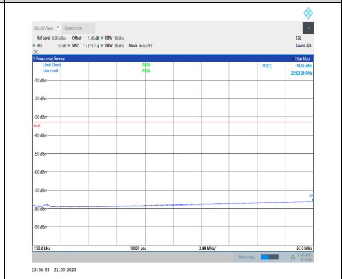
1-N78-3450-3550-30-100-H-1-DFT-QPSK-Edge_1R B_Left-1@0-0.15-30-Ant0-29.93--76.36--33-PASS
