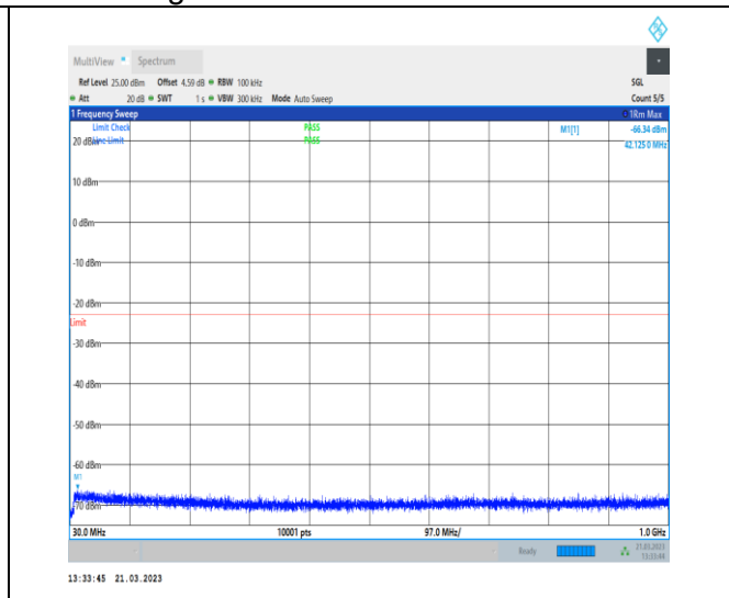
1-N78-3450-3550-30-100-M-1-DFT-QPSK-Edge_1R B_Left-1@0-30-1000-Ant0-42.13--66.34--23-PASS
