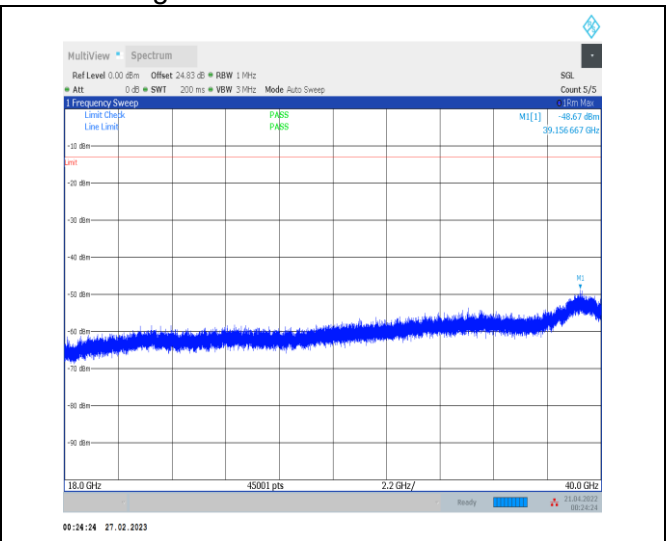
1-N78-3450-3550-30-100-H-1-DFT-PI2BPSK-Inner_1RB_Left-1@1-18000-40000-Ant0-18000.00--59.03--1 3-PASS
