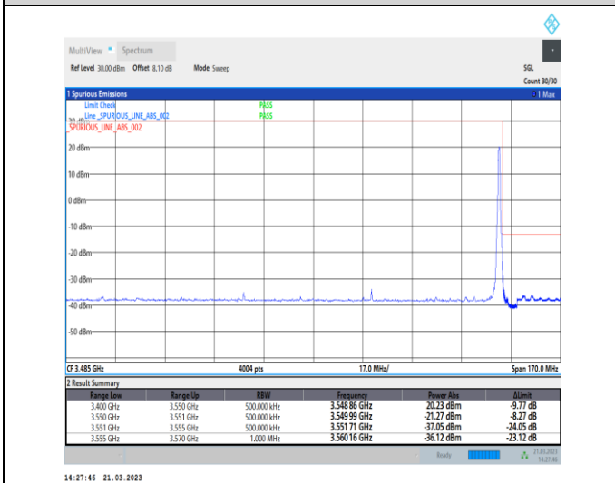
1-N78-3450-3550-30-90-H-5-CP-QPSK-Edge_1RB_Ri ght-1@244-Ant0-1--PASS-see graph
