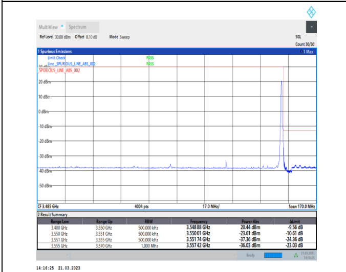
1-N78-3450-3550-30-70-H-5-CP-QPSK-Edge_1RB_Ri ght-1@188-Ant0-1--PASS-see graph
