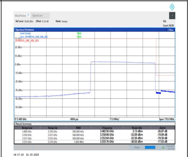
1-N78-3450-3550-30-70-H-6-CP-QPSK-Outer_Full -189@0-Ant0-1--PASS-see graph
