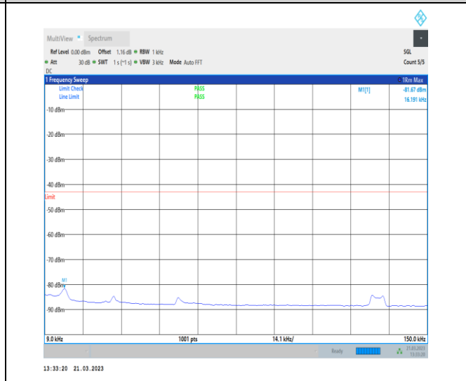
1-N78-3450-3550-30-100-M-1-DFT-QPSK-Edge_1R B_Left-1@0-0.009-0.15-Ant0-0.02--81.67--43-PASS
