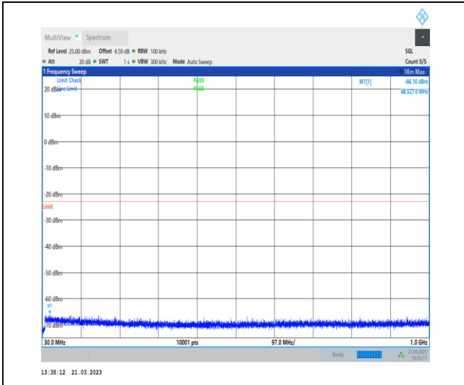
1-N78-3450-3550-30-100-H-1-DFT-QPSK-Edge_1R B_Left-1@0-30-1000-Ant0-48.53--66.10--23-PASS
