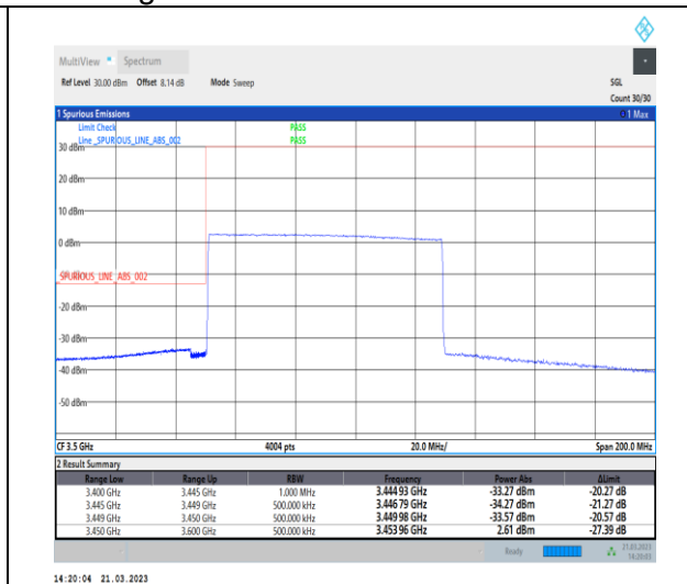
1-N78-3450-3550-30-80-L-6-CP-QPSK-Outer_Full -217@0-Ant0-1--PASS-see graph
