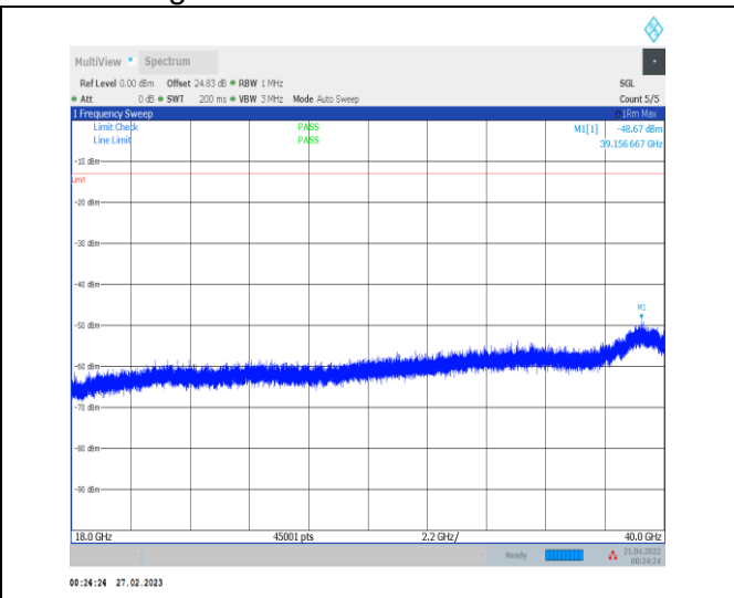
1-N78-3450-3550-30-100-L-1-DFT-PI2BPSK-Inner_1RB_Left-1@1-18000-40000-Ant0-18000.00--58.72--1 3-PASS
