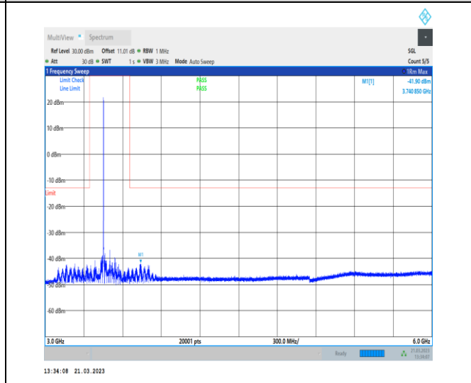
1-N78-3450-3550-30-100-M-1-DFT-QPSK-Edge_1R B_Left-1@0-3000-6000-Ant0-3740.85--41.90--13-PA
