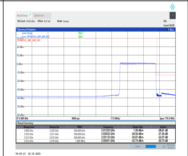
1-N78-3450-3550-30-40-H-6-CP-QPSK-Outer_Full-106@0-Ant0-1--PASS-see graph
