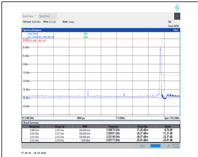
1-N78-3450-3550-30-80-H-2-DFT-PI2BPSK-Edge_1R_B_Right-1@216-Ant0-1--PASS-see graph
