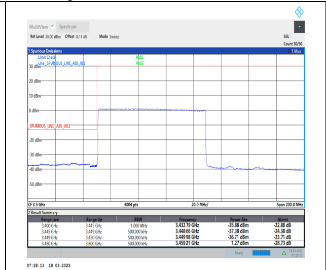
1-N78-3450-3550-30-80-L-3-DFT-PI2BPSK-Outer _Full-216@0-Ant0-1--PASS-see graph
