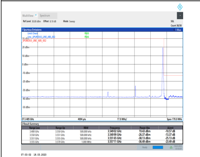
1-N78-3450-3550-30-60-H-5-CP-QPSK-Edge_1RB_Right-1@161-Ant0-1--PASS-see graph
