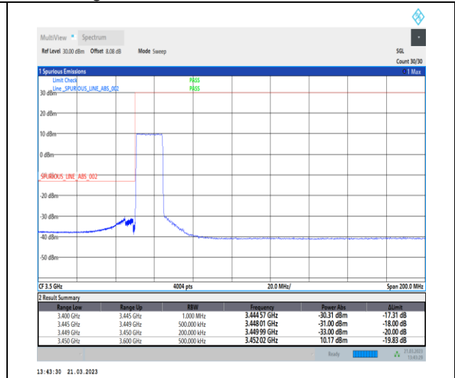
1-N78-3450-3550-30-15-L-6-CP-QPSK-Outer_Full -38@0-Ant0-1--PASS-see graph
