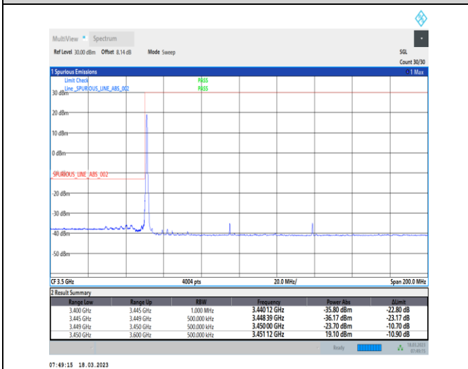
1-N78-3450-3550-30-90-L-4-CP-QPSK-Edge_1RB_Lef t-1@0-Ant0-1--PASS-see graph
