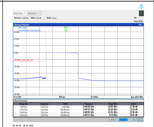
1-N78-3450-3550-30-50-L-6-CP-QPSK-Outer_Full -133@0-Ant0-1--PASS-see graph
