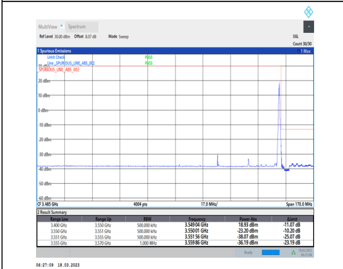
1-N78-3450-3550-30-40-H-5-CP-QPSK-Edge_1RB_Right-1@105-Ant0-1--PASS-see graph
