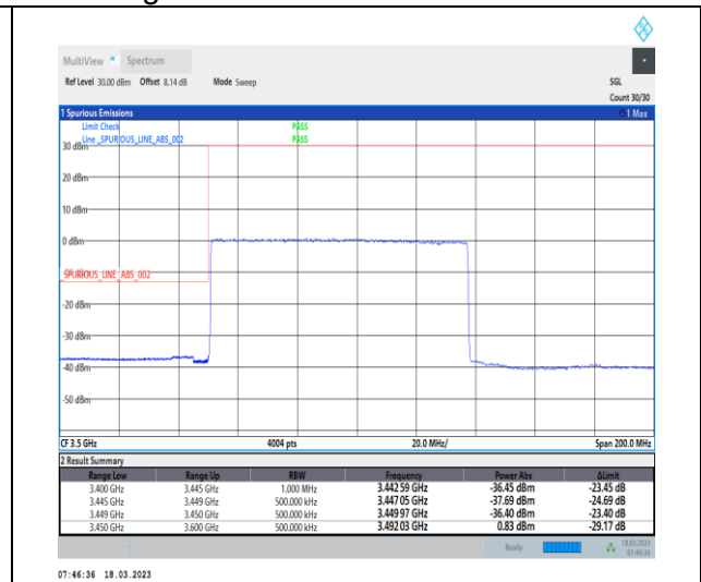
1-N78-3450-3550-30-90-L-3-DFT-PI2BPSK-Outer _Full-240@0-Ant0-1--PASS-see graph
