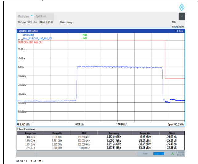
1-N78-3450-3550-30-90-H-3-DFT-PI2BPSK-Outer_Full-240@0-Ant0-1--PASS-see graph
