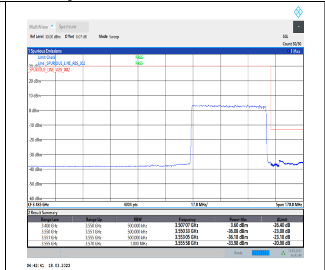
1-N78-3450-3550-30-50-H-3-DFT-PI2BPSK-Outer_Full-128@0-Ant0-1--PASS-see graph
