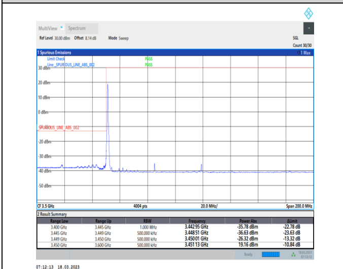
1-N78-3450-3550-30-70-L-4-CP-QPSK-Edge_1RB_Lef t-1@0-Ant0-1--PASS-see graph
