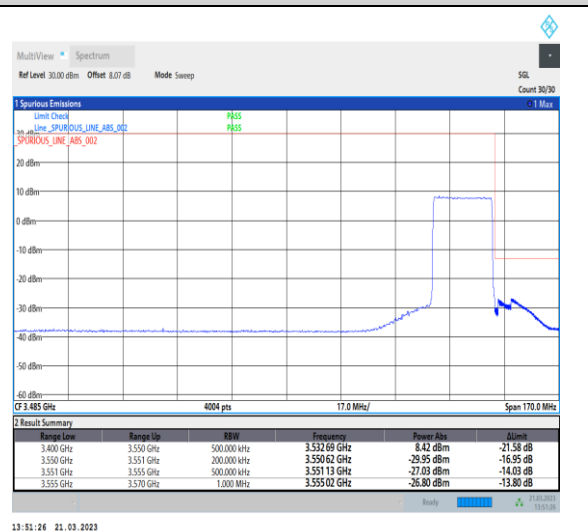
1-N78-3450-3550-30-20-H-6-CP-QPSK-Outer_Full -51@0-Ant0-1--PASS-see graph
