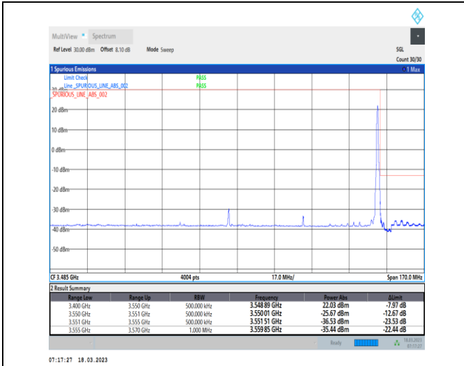
1-N78-3450-3550-30-70-H-2-DFT-PI2BPSK-Edge_1R_B_Right-1@188-Ant0-1--PASS-see graph
