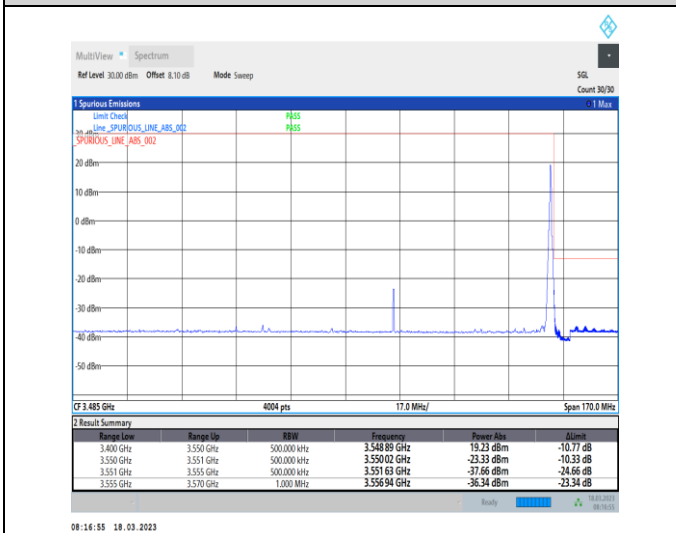
1-N78-3450-3550-30-100-H-5-CP-QPSK-Edge_1RB_Right-1@272-Ant0-1--PASS-see graph
