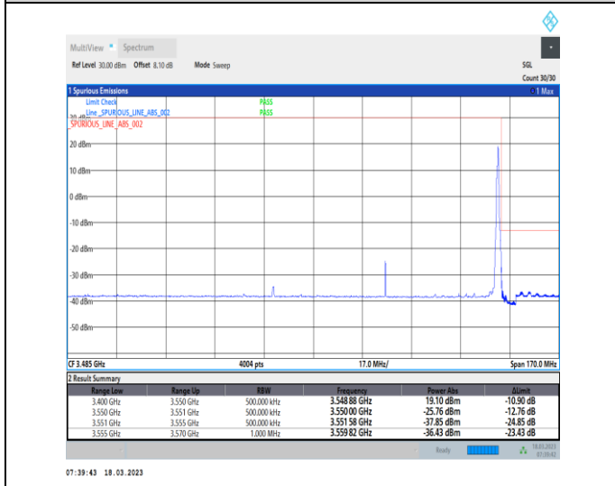
1-N78-3450-3550-30-80-H-5-CP-QPSK-Edge_1RB_Right-1@216-Ant0-1--PASS-see graph
