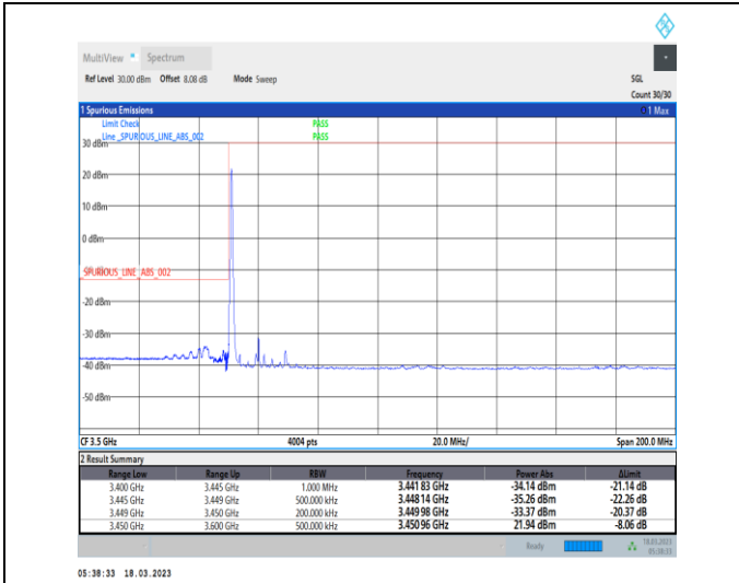
1-N78-3450-3550-30-20-L-1-DFT-PI2BPSK-Edge_1RB _Left-1@0-Ant0-1--PASS-see graph
