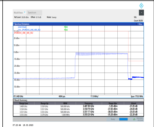
1-N78-3450-3550-30-70-H-6-CP-QPSK-Outer_Full-189@0-Ant0-1--PASS-see graph
