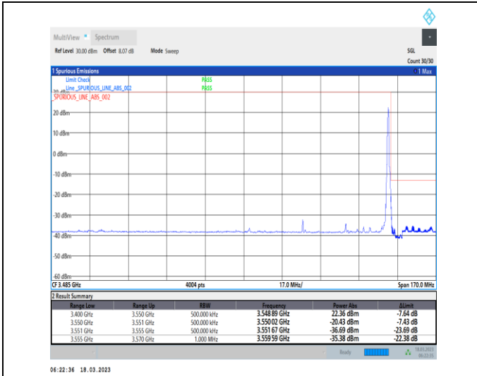
1-N78-3450-3550-30-40-H-2-DFT-PI2BPSK-Edge_1R_B_Right-1@105-Ant0-1--PASS-see graph
