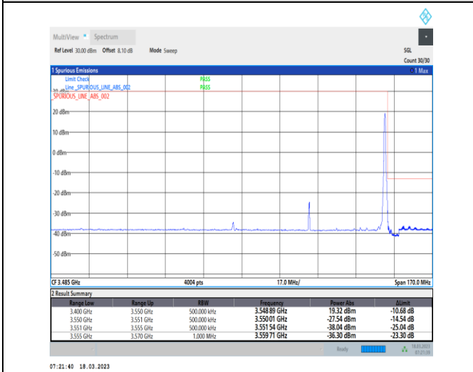
1-N78-3450-3550-30-70-H-5-CP-QPSK-Edge_1RB_Right-1@188-Ant0-1--PASS-see graph
