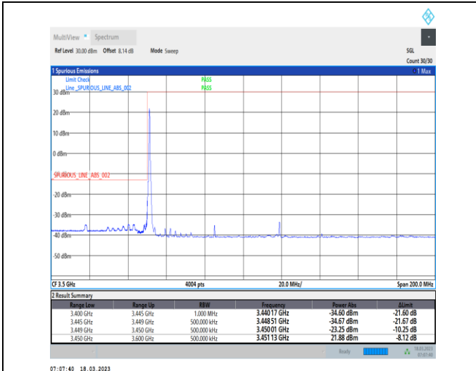
1-N78-3450-3550-30-70-L-1-DFT-PI2BPSK-Edge_1RB _Left-1@0-Ant0-1--PASS-see graph
