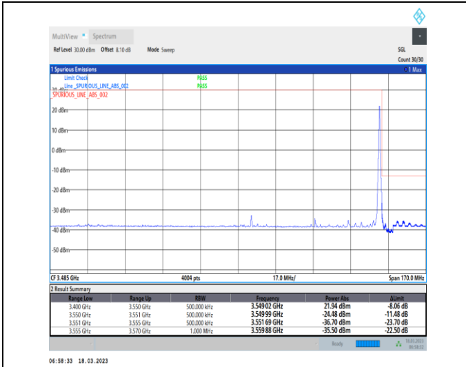
1-N78-3450-3550-30-60-H-2-DFT-PI2BPSK-Edge_1R_B_Right-1@161-Ant0-1--PASS-see graph
