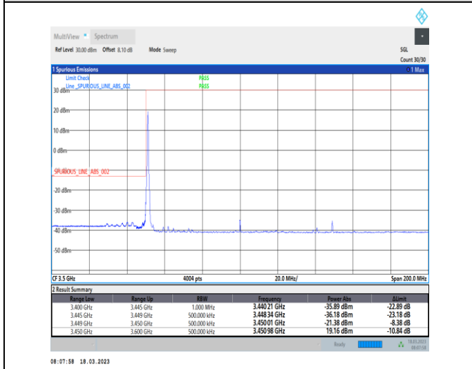
1-N78-3450-3550-30-100-L-4-CP-QPSK-Edge_1RB_Left-1@0-Ant0-1--PASS-see graph
