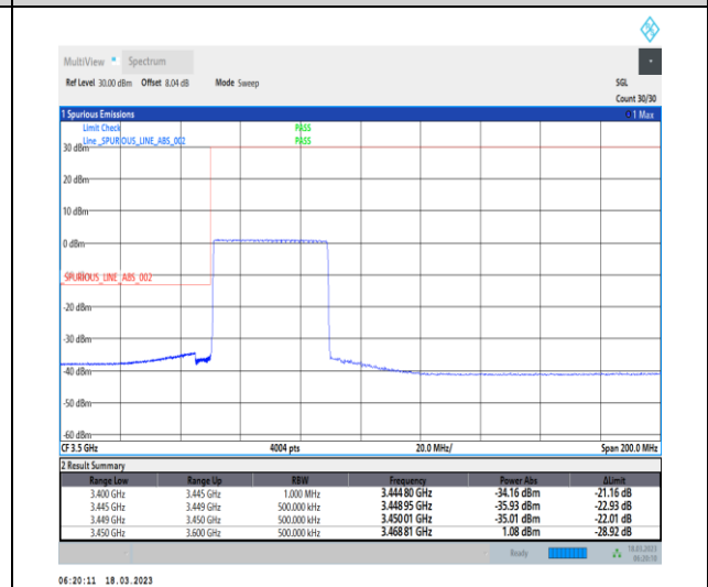
1-N78-3450-3550-30-40-L-6-CP-QPSK-Outer_Full -106@0-Ant0-1--PASS-see graph
