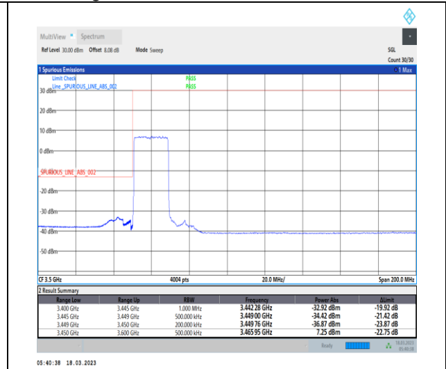
1-N78-3450-3550-30-20-L-3-DFT-PI2BPSK-Outer _Full-50@0-Ant0-1--PASS-see graph
