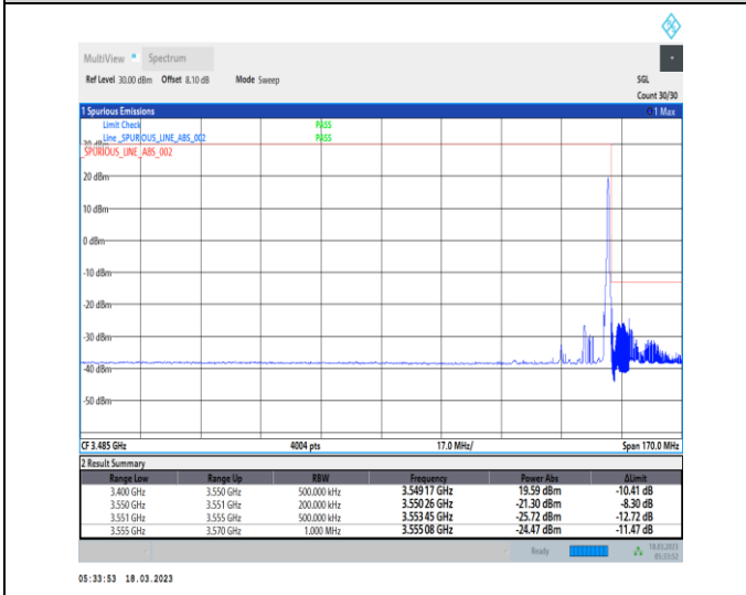
1-N78-3450-3550-30-15-H-5-CP-QPSK-Edge_1RB_Right-1@37-Ant0-1--PASS-see graph
