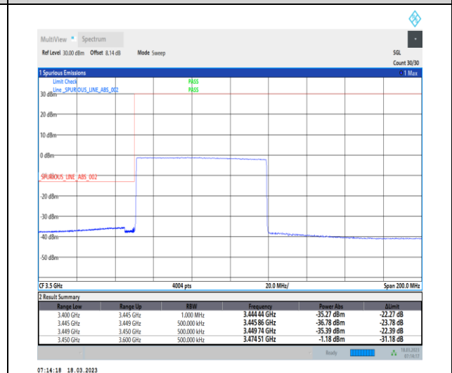
1-N78-3450-3550-30-70-L-6-CP-QPSK-Outer_Full -189@0-Ant0-1--PASS-see graph
