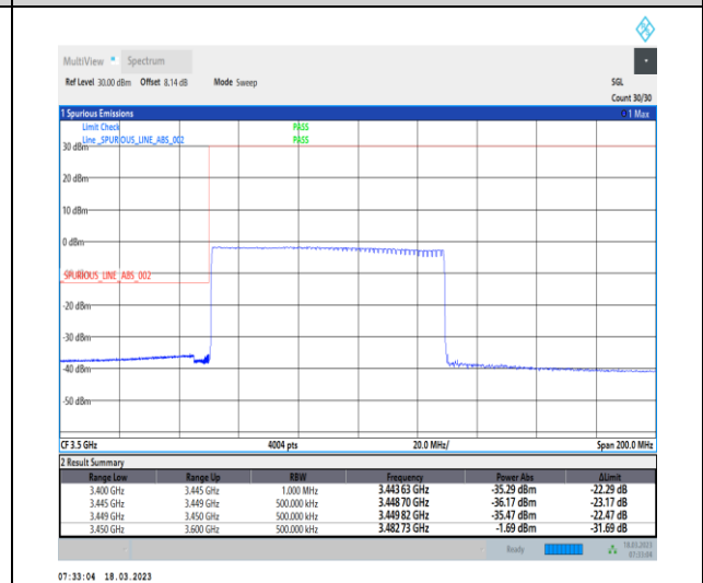
1-N78-3450-3550-30-80-L-6-CP-QPSK-Outer_Full -217@0-Ant0-1--PASS-see graph
