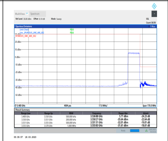
1-N78-3450-3550-30-15-H-6-CP-QPSK-Outer_Full-38@0-Ant0-1--PASS-see graph
