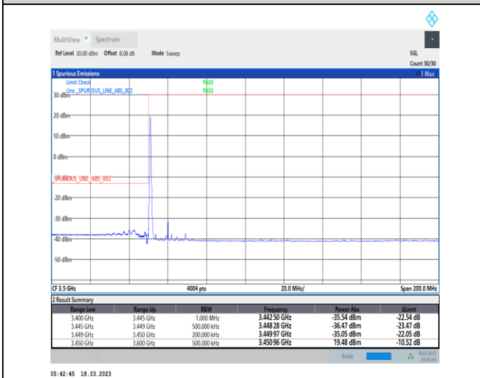
1-N78-3450-3550-30-20-L-4-CP-QPSK-Edge_1RB_Lef t-1@0-Ant0-1--PASS-see graph
