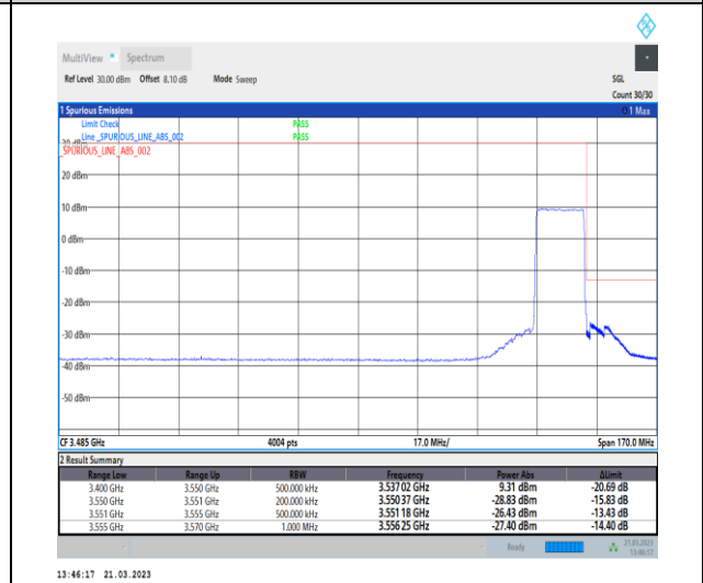
1-N78-3450-3550-30-15-H-6-CP-QPSK-Outer_Full -38@0-Ant0-1--PASS-see graph
