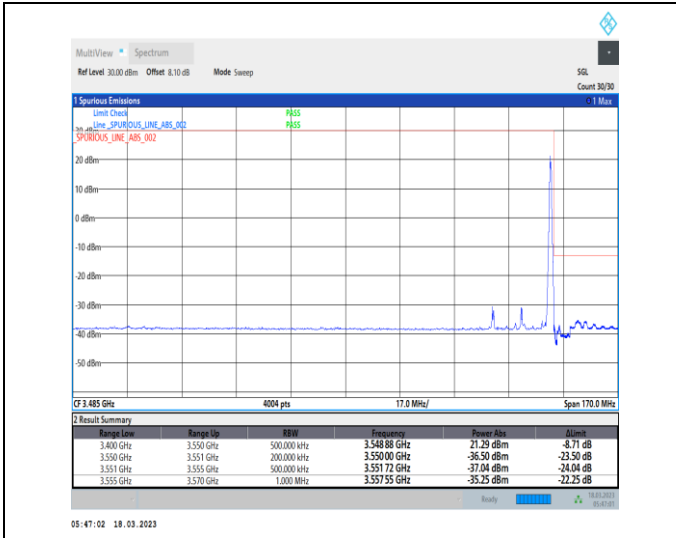
1-N78-3450-3550-30-20-H-2-DFT-PI2BPSK-Edge_1R_B_Right-1@50-Ant0-1--PASS-see graph
