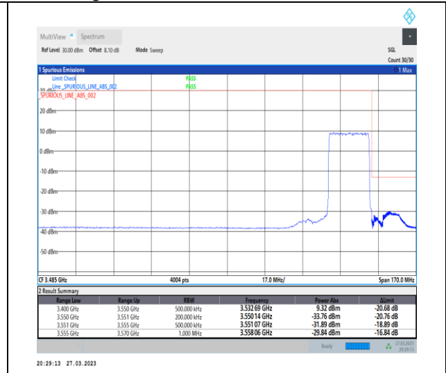
1-N78-3450-3550-30-20-H-3-DFT-PI2BPSK-Outer_Full-50@0-Ant0-1--PASS-see graph
