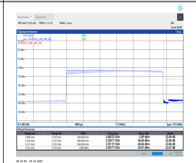
1-N78-3450-3550-30-100-H-6-CP-QPSK-Outer_Full-273@0-Ant0-1--PASS-see graph
