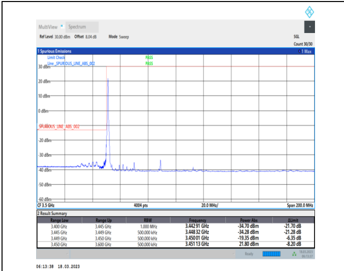
1-N78-3450-3550-30-40-L-1-DFT-PI2BPSK-Edge_1RB _Left-1@0-Ant0-1--PASS-see graph
