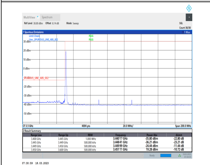
1-N78-3450-3550-30-80-L-4-CP-QPSK-Edge_1RB_Lef t-1@0-Ant0-1--PASS-see graph
