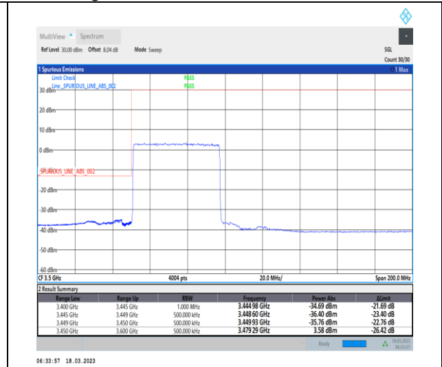
1-N78-3450-3550-30-50-L-3-DFT-PI2BPSK-Outer _Full-128@0-Ant0-1--PASS-see graph
