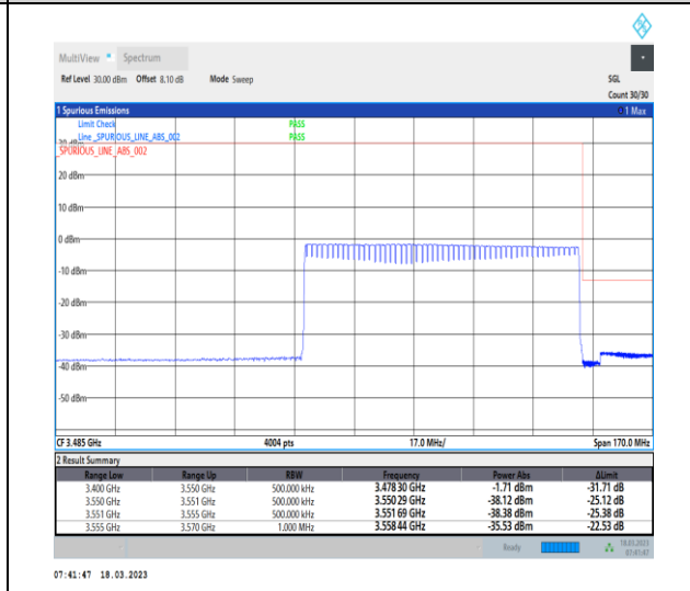
1-N78-3450-3550-30-80-H-6-CP-QPSK-Outer_Full-217@0-Ant0-1--PASS-see graph
