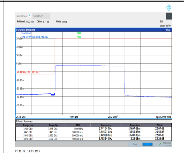
1-N78-3450-3550-30-90-L-6-CP-QPSK-Outer_Full -245@0-Ant0-1--PASS-see graph
