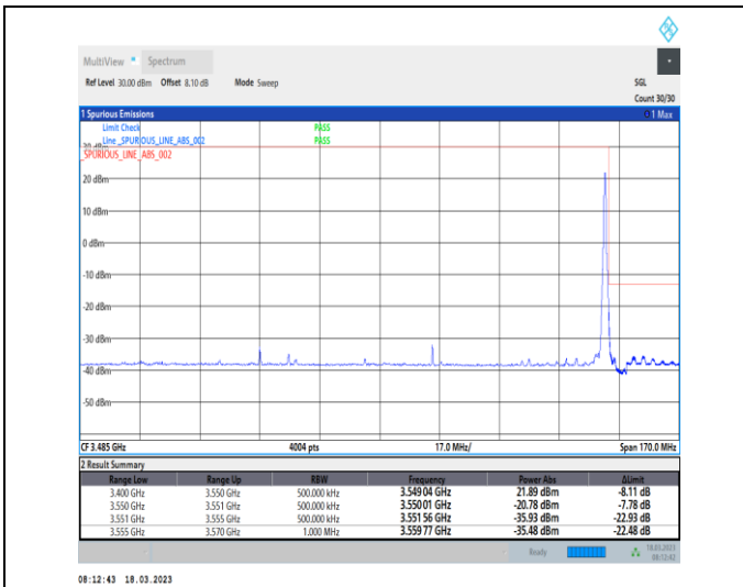
1-N78-3450-3550-30-100-H-2-DFT-PI2BPSK-Edge_1R_B_Right-1@272-Ant0-1--PASS-see graph
