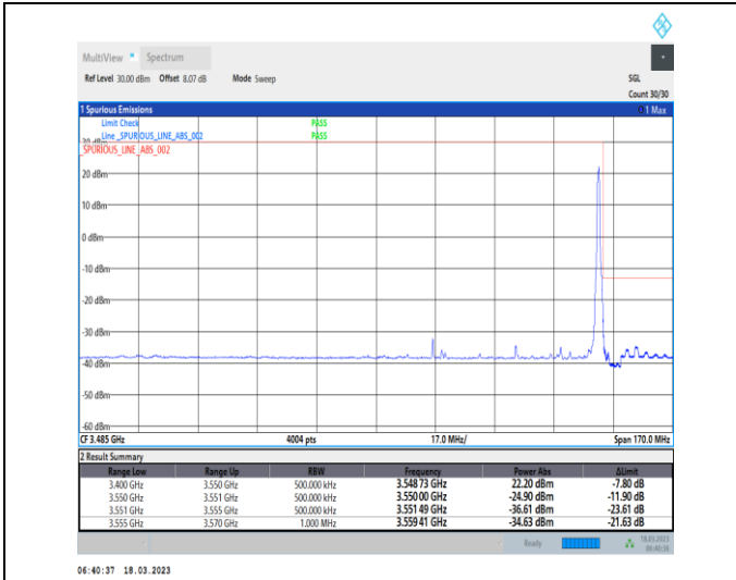
1-N78-3450-3550-30-50-H-2-DFT-PI2BPSK-Edge_1R_B_Right-1@132-Ant0-1--PASS-see graph
