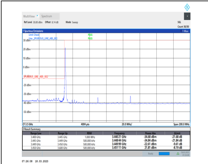
1-N78-3450-3550-30-80-L-1-DFT-PI2BPSK-Edge_1RB _Left-1@0-Ant0-1--PASS-see graph
