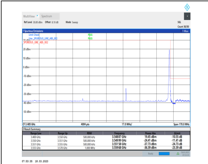
1-N78-3450-3550-30-90-H-2-DFT-PI2BPSK-Edge_1R_B_Right-1@244-Ant0-1--PASS-see graph
