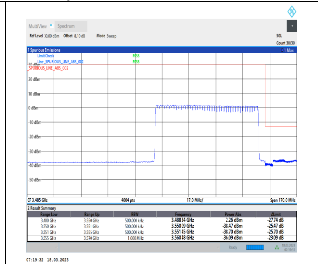
1-N78-3450-3550-30-70-H-3-DFT-PI2BPSK-Outer_Full-180@0-Ant0-1--PASS-see graph
