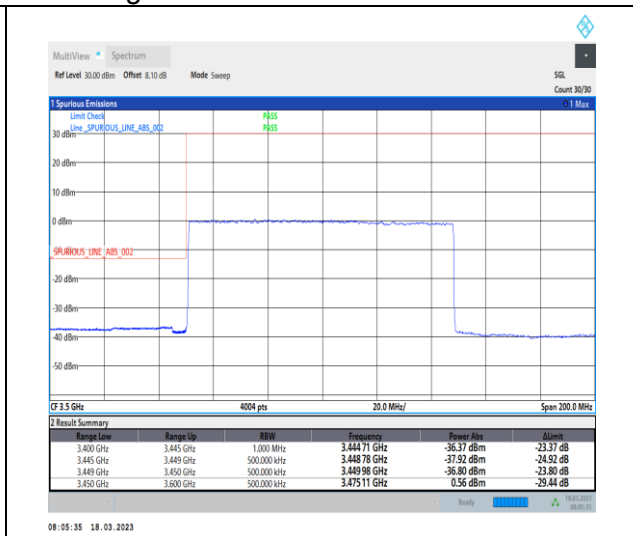
1-N78-3450-3550-30-100-L-3-DFT-PI2BPSK-Outer_Full-270@0-Ant0-1--PASS-see graph
