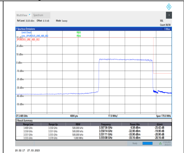
1-N78-3450-3550-30-60-H-3-DFT-PI2BPSK-Outer_Full-162@0-Ant0-1--PASS-see graph
