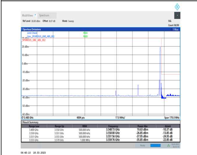
1-N78-3450-3550-30-50-H-5-CP-QPSK-Edge_1RB_Right-1@132-Ant0-1--PASS-see graph
