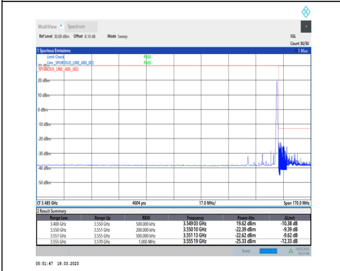
1-N78-3450-3550-30-20-H-5-CP-QPSK-Edge_1RB_Right-1@50-Ant0-1--PASS-see graph
