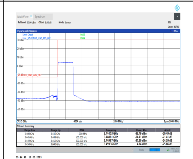
1-N78-3450-3550-30-20-L-6-CP-QPSK-Outer_Full -51@0-Ant0-1--PASS-see graph
