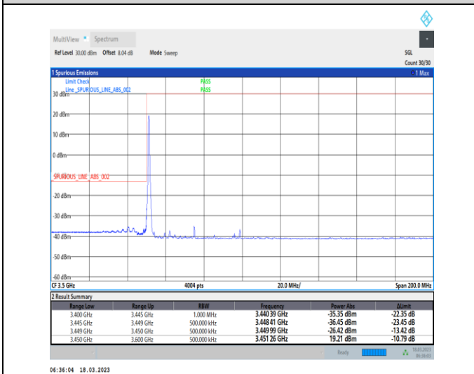
1-N78-3450-3550-30-50-L-4-CP-QPSK-Edge_1RB_Lef t-1@0-Ant0-1--PASS-see graph
