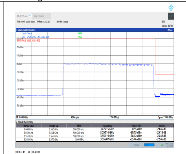
1-N78-3450-3550-30-100-H-3-DFT-PI2BPSK-Outer_Full-270@0-Ant0-1--PASS-see graph
