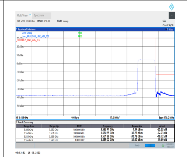
1-N78-3450-3550-30-20-H-6-CP-QPSK-Outer_Full-51@0-Ant0-1--PASS-see graph
