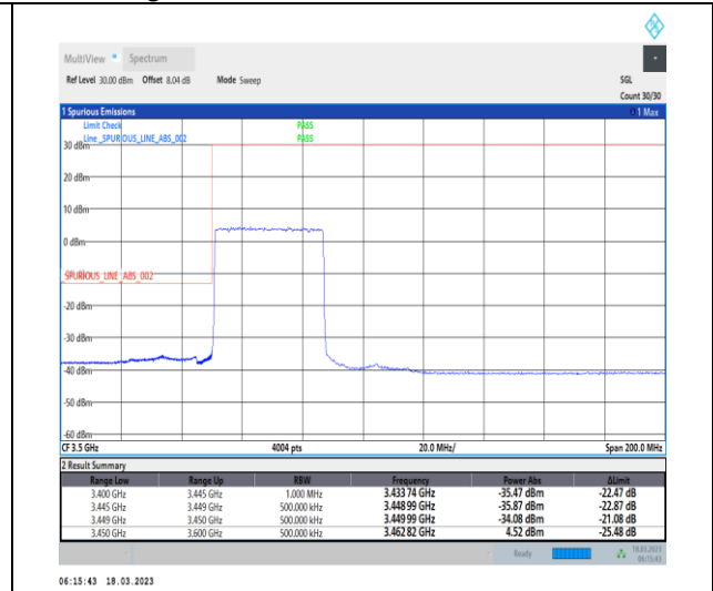
1-N78-3450-3550-30-40-L-3-DFT-PI2BPSK-Outer _Full-100@0-Ant0-1--PASS-see graph
