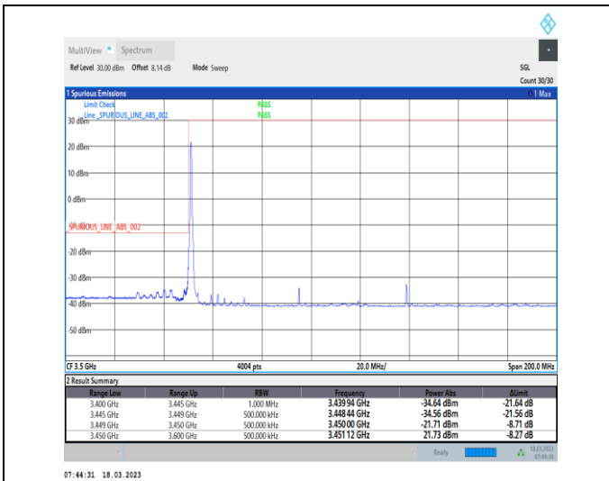
1-N78-3450-3550-30-90-L-1-DFT-PI2BPSK-Edge_1RB _Left-1@0-Ant0-1--PASS-see graph
