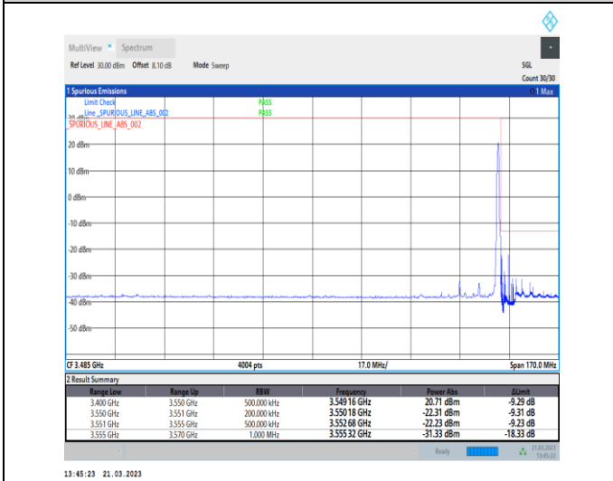
1-N78-3450-3550-30-15-H-5-CP-QPSK-Edge_1RB_Ri ght-1@37-Ant0-1--PASS-see graph
