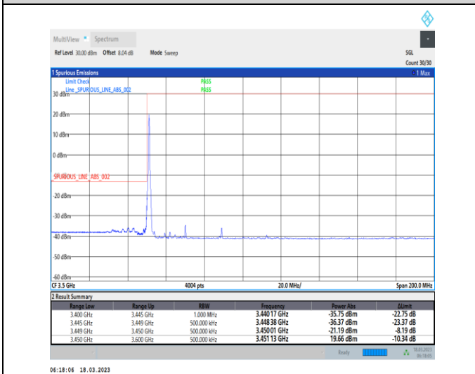
1-N78-3450-3550-30-40-L-4-CP-QPSK-Edge_1RB_Lef t-1@0-Ant0-1--PASS-see graph
