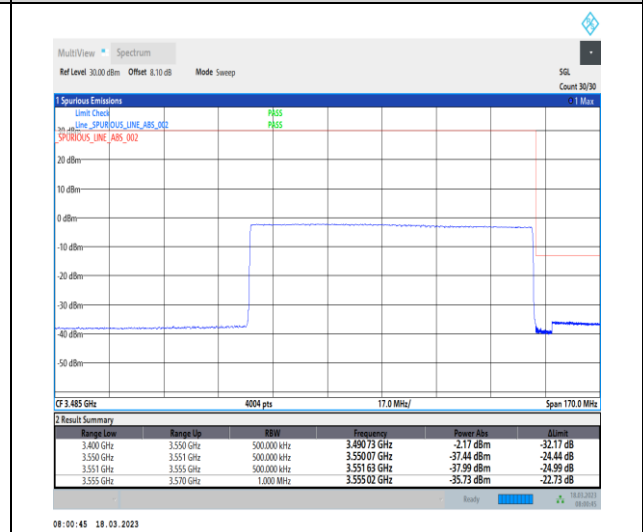
1-N78-3450-3550-30-90-H-6-CP-QPSK-Outer_Full-245@0-Ant0-1--PASS-see graph
