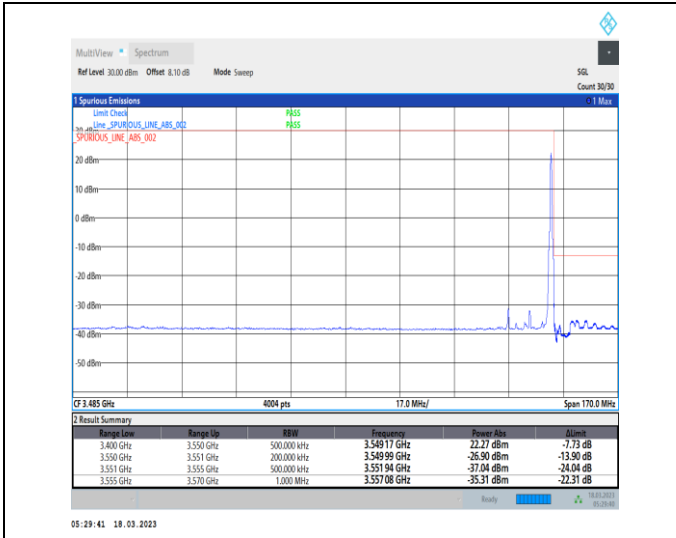
1-N78-3450-3550-30-15-H-2-DFT-PI2BPSK-Edge_1R_B_Right-1@37-Ant0-1--PASS-see graph
