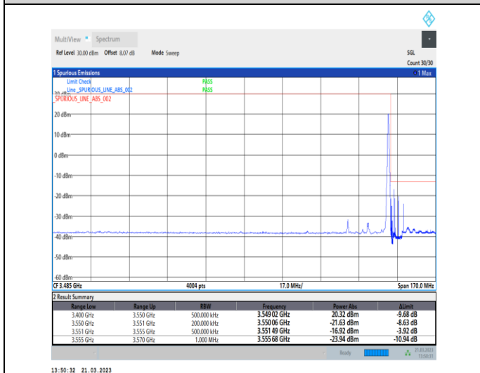
1-N78-3450-3550-30-20-H-5-CP-QPSK-Edge_1RB_Ri ght-1@50-Ant0-1--PASS-see graph
