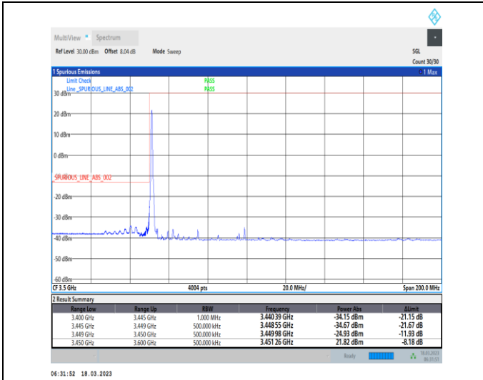
1-N78-3450-3550-30-50-L-1-DFT-PI2BPSK-Edge_1RB _Left-1@0-Ant0-1--PASS-see graph
