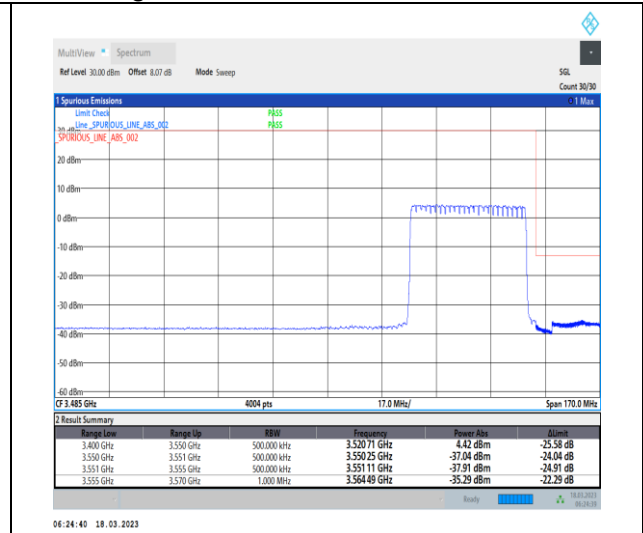
1-N78-3450-3550-30-40-H-3-DFT-PI2BPSK-Outer_Full-100@0-Ant0-1--PASS-see graph
