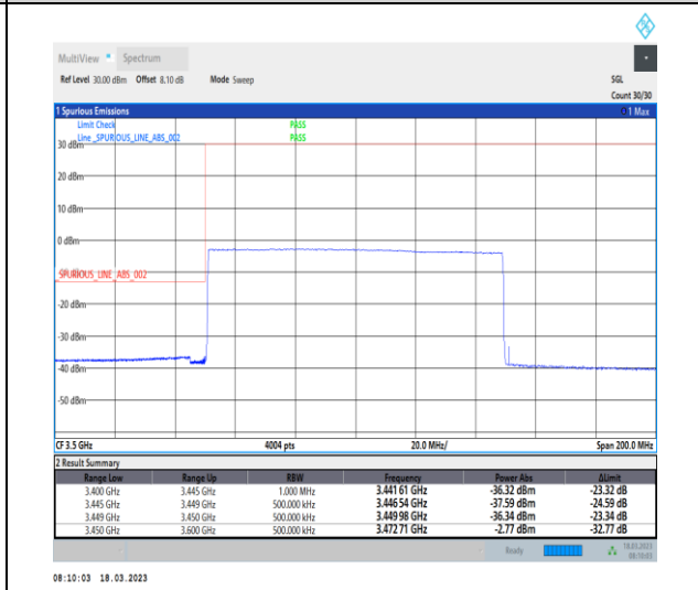
1-N78-3450-3550-30-100-L-6-CP-QPSK-Outer_Full-273@0-Ant0-1--PASS-see graph
