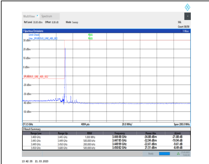
1-N78-3450-3550-30-15-L-4-CP-QPSK-Edge_1RB_Lef t-1@0-Ant0-1--PASS-see graph
