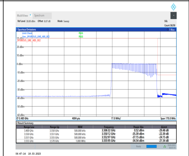
1-N78-3450-3550-30-50-H-6-CP-QPSK-Outer_Full-133@0-Ant0-1--PASS-see graph
