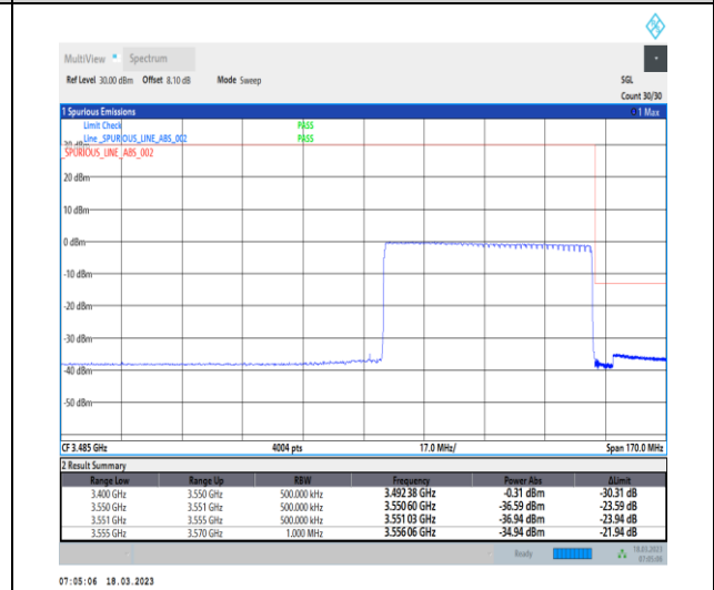
1-N78-3450-3550-30-60-H-6-CP-QPSK-Outer_Full-162@0-Ant0-1--PASS-see graph
