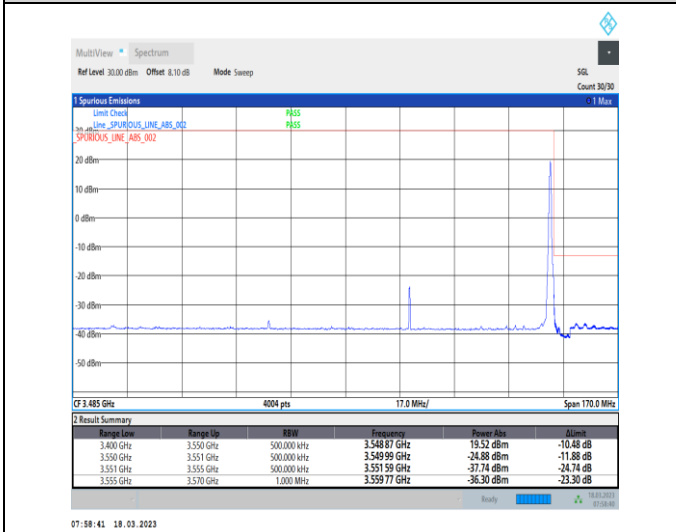
1-N78-3450-3550-30-90-H-5-CP-QPSK-Edge_1RB_Right-1@244-Ant0-1--PASS-see graph
