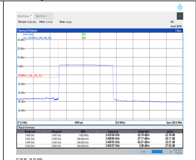
1-N78-3450-3550-30-70-L-3-DFT-PI2BPSK-Outer _Full-180@0-Ant0-1--PASS-see graph
