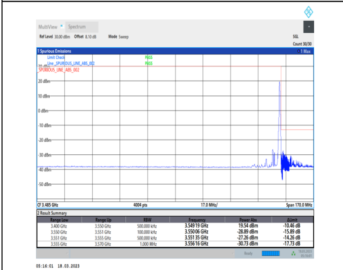
1-N78-3450-3550-30-10-H-5-CP-QPSK-Edge_1RB_Right-1@23-Ant0-1--PASS-see graph
