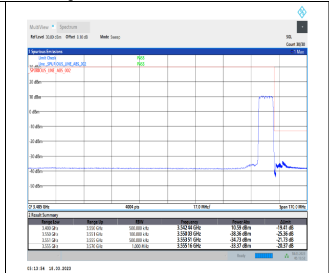
1-N78-3450-3550-30-10-H-3-DFT-PI2BPSK-Outer_Full-24@0-Ant0-1--PASS-see graph
