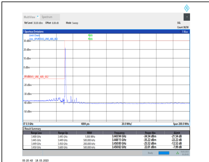
1-N78-3450-3550-30-15-L-1-DFT-PI2BPSK-Edge_1RB_Left-1@0-Ant0-1--PASS-see graph
