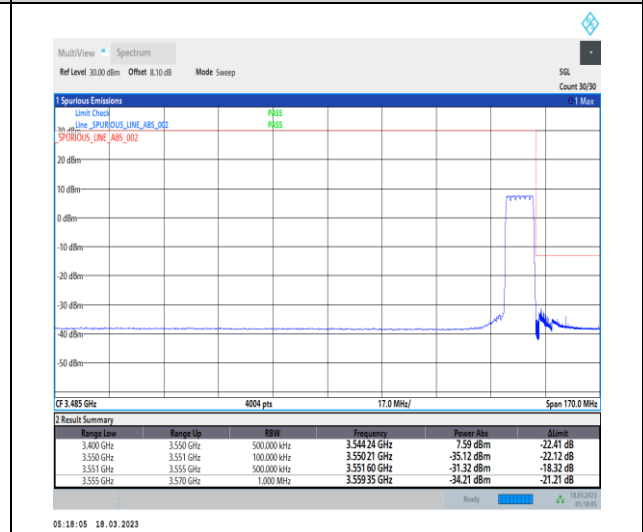
1-N78-3450-3550-30-10-H-6-CP-QPSK-Outer_Full-24@0-Ant0-1--PASS-see graph
