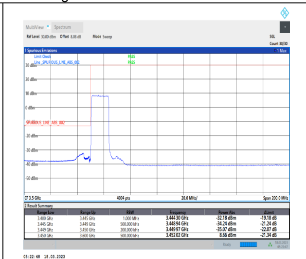
1-N78-3450-3550-30-15-L-3-DFT-PI2BPSK-Outer_Full-36@0-Ant0-1--PASS-see graph
