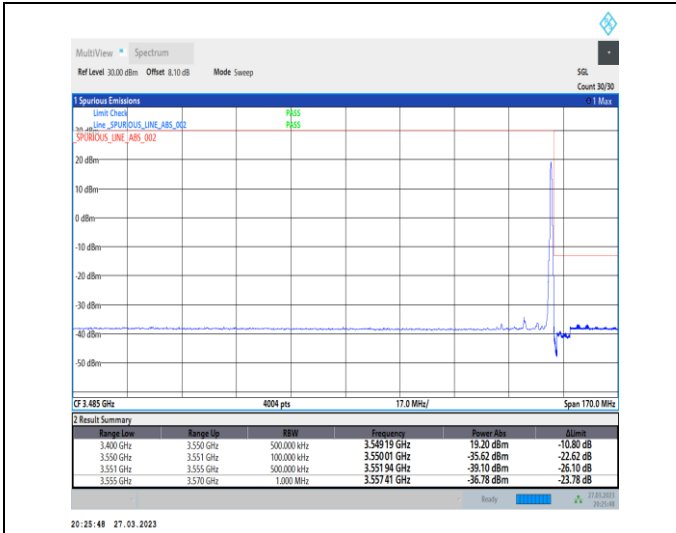
1-N78-3450-3550-30-10-H-2-DFT-PI2BPSK-Edge_1R_B_Right-1@23-Ant0-1--PASS-see graph
