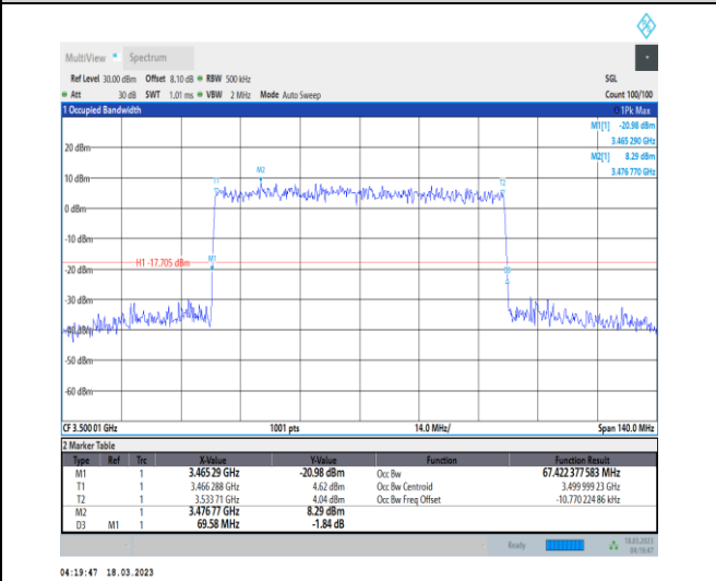
1-N78-3450-3550-30-70-M-8-CP-64QAM-Outer_Full-189@0-Ant0-67.422-69.580-≤70-PASS
