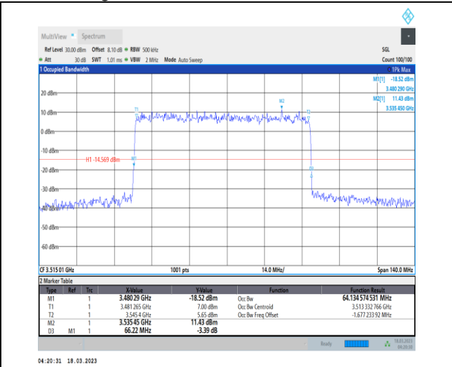
1-N78-3450-3550-30-70-H-1-DFT-QPSK-Outer_Full 180@0-Ant0-64.135-66.220-≤70-PASS
