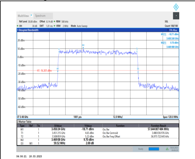
1-N78-3450-3550-30-60-L-6-CP-QPSK-Outer_Full-62@0-Ant0-57.644-59.520-≤60-PASS
