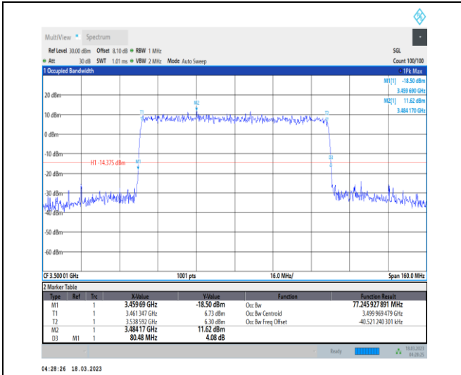
1-N78-3450-3550-30-80-M-6-CP-QPSK-Outer_Full-2 17@0-Ant0-77.246-80.480-≤80-PASS
