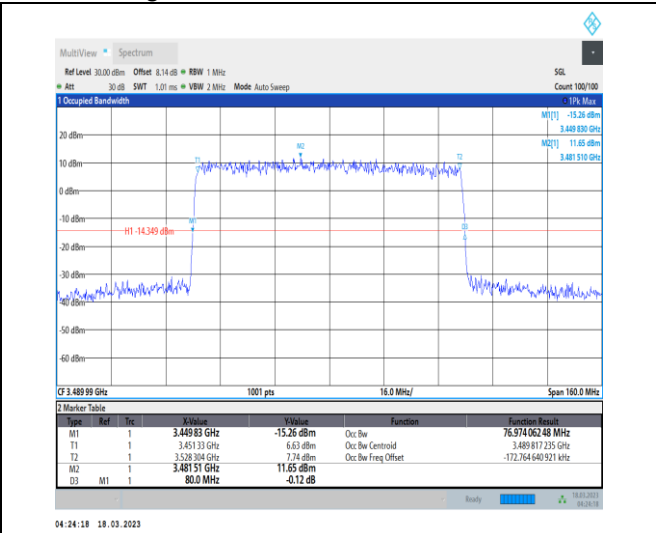
1-N78-3450-3550-30-80-L-4-DFT-64QAM-Outer_Full -216@0-Ant0-76.974-80.000-≤80-PASS
