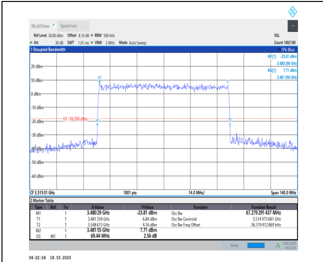
1-N78-3450-3550-30-70-H-8-CP-64QAM-Outer_Full-189@0-Ant0-67.279-69.440-≤70-PASS
