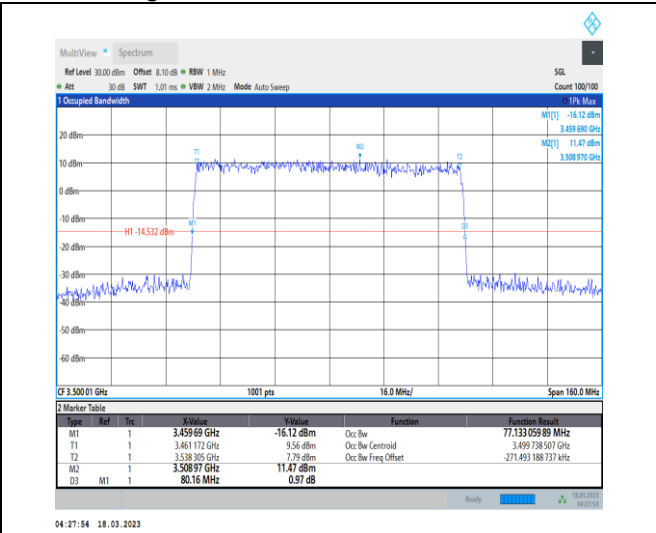
1-N78-3450-3550-30-80-M-3-DFT-16QAM-Outer_Full-216@0-Ant0-77.133-80.160-≤80-PASS
