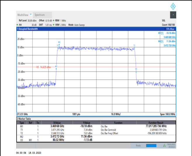
1-N78-3450-3550-30-80-H-4-DFT-64QAM-Outer_Full-216@0-Ant0-77.017-80.320-≤80-PASS
