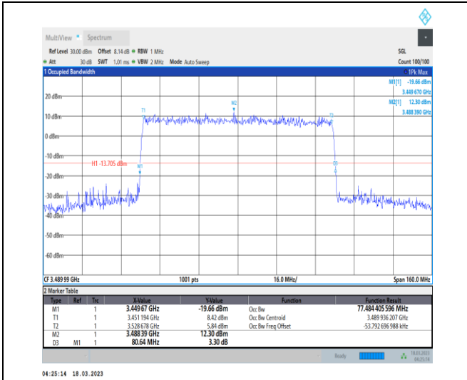
1-N78-3450-3550-30-80-L-7-CP-16QAM-Outer_Full-217@0-Ant0-77.484-80.640-≤80-PASS
