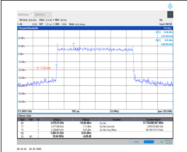
1-N78-3450-3550-30-60-M-6-CP-QPSK-Outer_Full-1 62@0-Ant0-57.756-59.640-≤60-PASS
