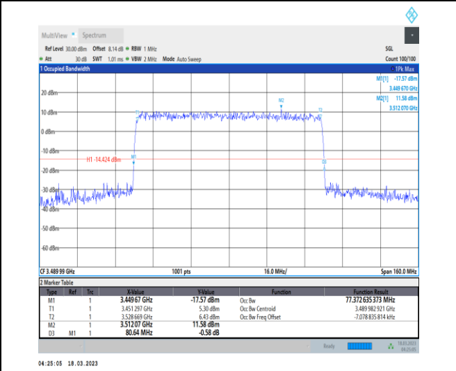
1-N78-3450-3550-30-80-L-6-CP-QPSK-Outer_Full-2 17@0-Ant0-77.373-80.640-≤80-PASS
