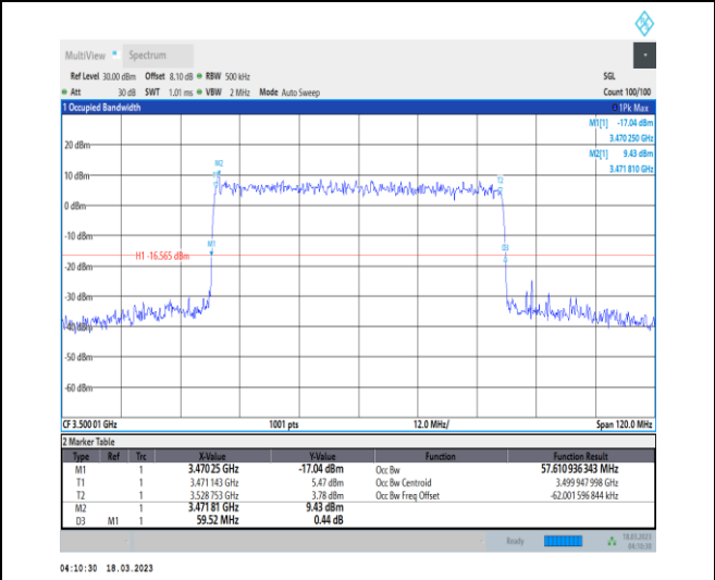
1-N78-3450-3550-30-60-M-7-CP-16QAM-Outer_Full -162@0-Ant0-57.611-59.520-≤60-PASS
