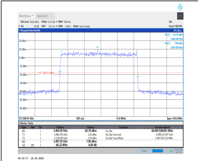
1-N78-3450-3550-30-70-M-5-DFT-256QAM-Outer_Full-180@0-Ant0-64.094-66.220-≤70-PASS
