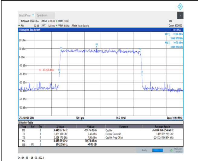
1-N78-3450-3550-30-80-L-5-DFT-256QAM-Outer_Fu ll-216@0-Ant0-76.835-80.320-≤80-PASS
