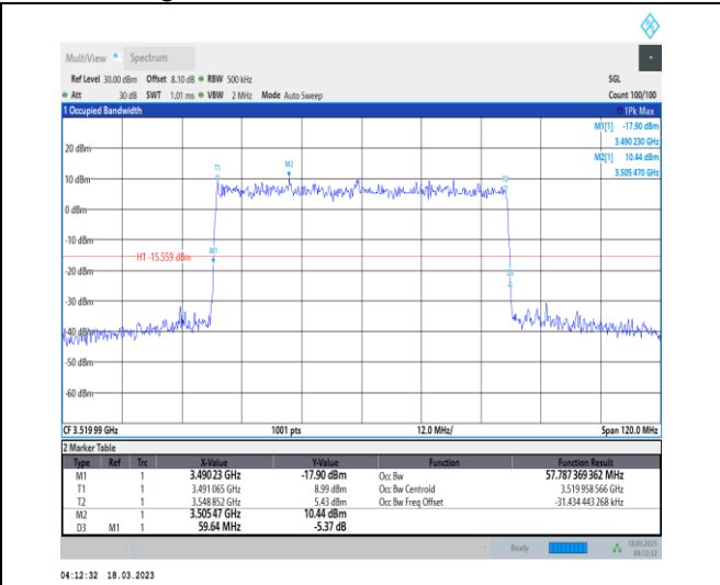
1-N78-3450-3550-30-60-H-4-DFT-64QAM-Outer_Ful I-162@0-Ant0-57.787-59.640-≤60-PASS
