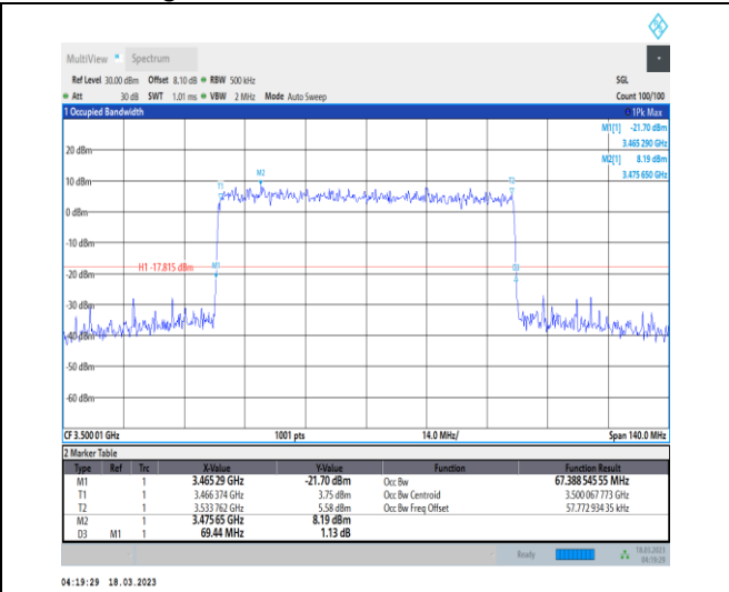
1-N78-3450-3550-30-70-M-6-CP-QPSK-Outer_Full-189@0-Ant0-67.389-69.440-≤70-PASS
