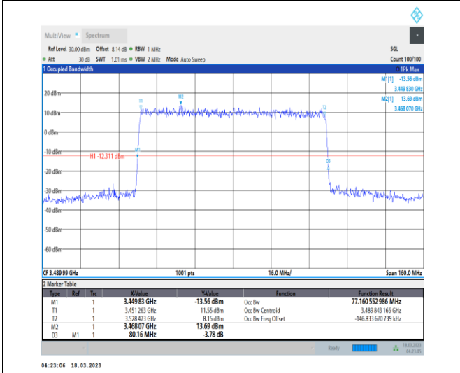
1-N78-3450-3550-30-80-L-1-DFT-QPSK-Outer_Full-216@0-Ant0-77.161-80.160-≤80-PASS
