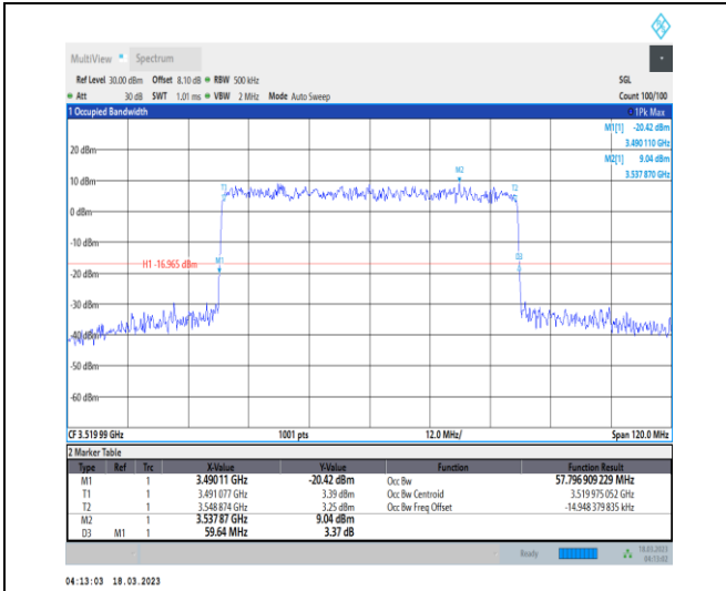
1-N78-3450-3550-30-60-H-7-CP-16QAM-Outer_Full-162@0-Ant0-57.797-59.640-≤60-PASS
