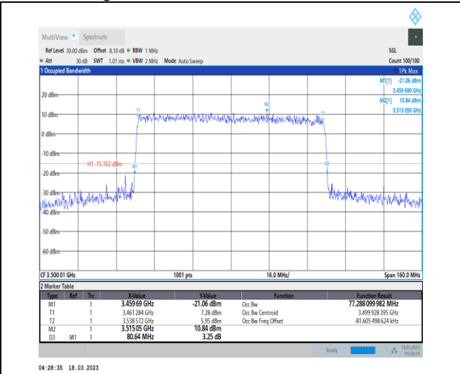
1-N78-3450-3550-30-80-M-7-CP-16QAM-Outer_Full-217@0-Ant0-77.288-80.640-≤80-PASS
