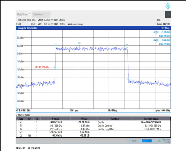
1-N78-3450-3550-30-70-H-3-DFT-16QAM-Outer_Full 180@0-Ant0-64.228-66.500-≤70-PASS
