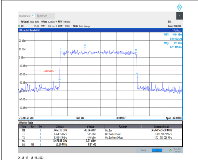
1-N78-3450-3550-30-70-L-4-DFT-64QAM-Outer_Full-180@0-Ant0-64.261-66.360-≤70-PASS
