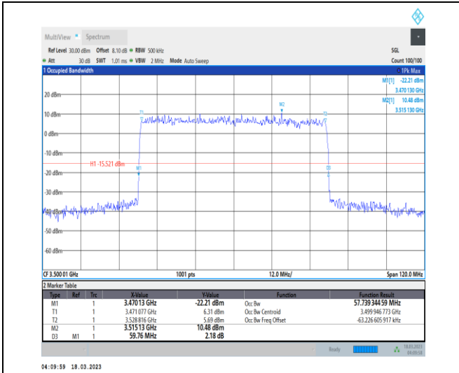
1-N78-3450-3550-30-60-M-4-DFT-64QAM-Outer_Ful I-162@0-Ant0-57.739-59.760-≤60-PASS
