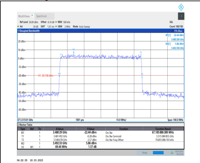
1-N78-3450-3550-30-70-H-9-CP-256QAM-Outer_Full-189@0-Ant0-67.186-69.440-≤70-PASS
