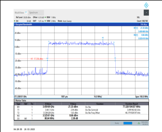
1-N78-3450-3550-30-80-M-9-CP-256QAM-Outer_Full-217@0-Ant0-77.328-80.640-≤80-PASS
