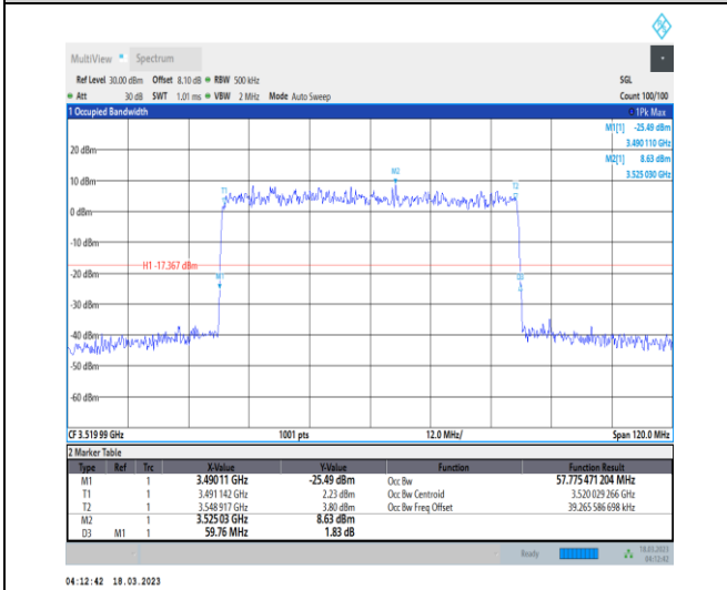
1-N78-3450-3550-30-60-H-5-DFT-256QAM-Outer_Full-162@0-Ant0-57.775-59.760-≤60-PASS
