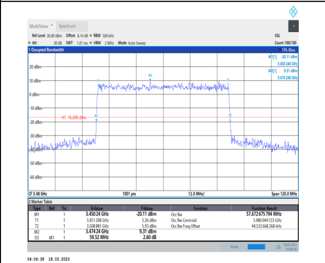
1-N78-3450-3550-30-60-L-8-CP-64QAM-Outer_Full-162@0-Ant0-57.673-59.520-≤60-PASS
