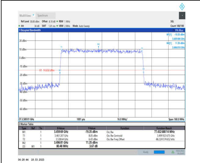
1-N78-3450-3550-30-80-M-8-CP-64QAM-Outer_Full-217@0-Ant0-77.433-80.480-≤80-PASS
