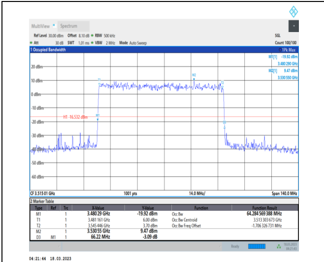
1-N78-3450-3550-30-70-H-4-DFT-64QAM-Outer_Ful I-180@0-Ant0-64.285-66.220-≤70-PASS
