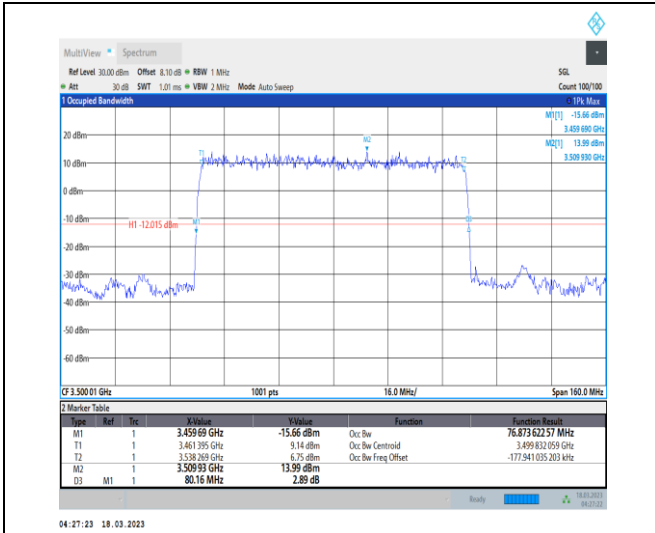
1-N78-3450-3550-30-80-M-2-DFT-PI2BPSK-Outer_Full-216@0-Ant0-76.874-80.160-≤80-PASS
