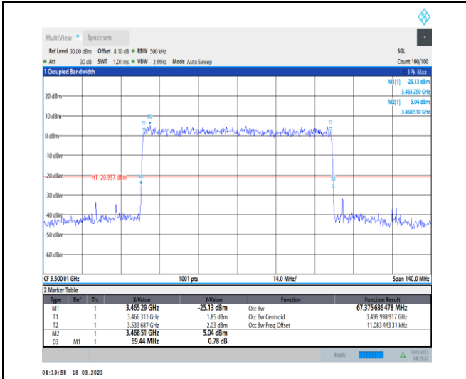
1-N78-3450-3550-30-70-M-9-CP-256QAM-Outer_Ful I-189@0-Ant0-67.376-69.440-≤70-PASS
