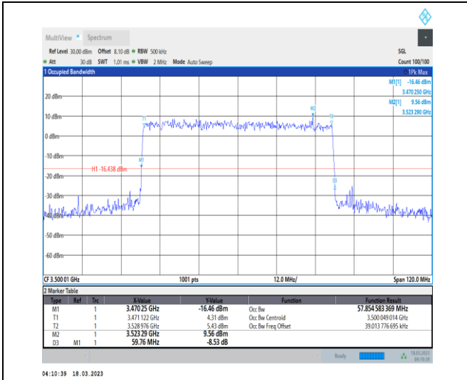
1-N78-3450-3550-30-60-M-8-CP-64QAM-Outer_Full-162@0-Ant0-57.855-59.760-≤60-PASS
