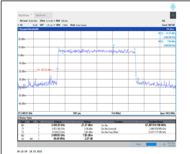
1-N78-3450-3550-30-70-L-6-CP-QPSK-Outer_Full-1 89@0-Ant0-67.387-69.440-≤70-PASS
