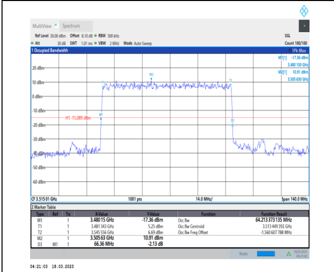
1-N78-3450-3550-30-70-H-2-DFT-PI2BPSK-Outer_Full 180@0-Ant0-64.213-66.360-≤70-PASS
