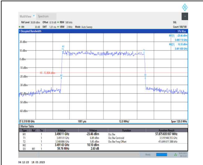
1-N78-3450-3550-30-60-H-3-DFT-16QAM-Outer_Ful I-162@0-Ant0-57.876-59.760-≤60-PASS
