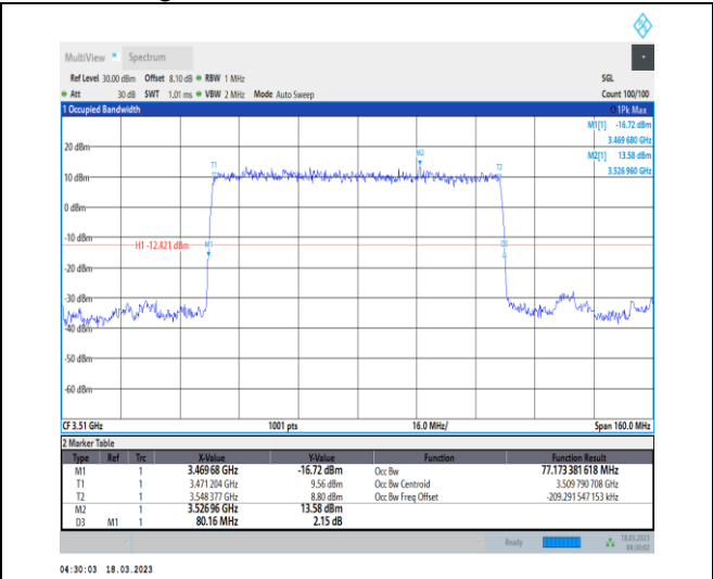
1-N78-3450-3550-30-80-H-2-DFT-PI2BPSK-Outer_Full-216@0-Ant0-77.173-80.160-≤80-PASS
