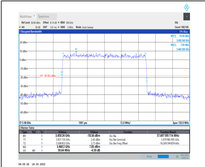
1-N78-3450-3550-30-60-L-5-DFT-256QAM-Outer_Fu II-162@0-Ant0-57.698-59.640-≤60-PASS
