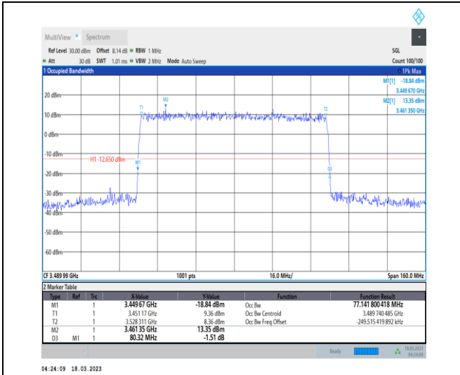
1-N78-3450-3550-30-80-L-3-DFT-16QAM-Outer_Full -216@0-Ant0-77.142-80.320-≤80-PASS
