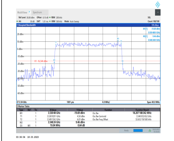
1-N78-3450-3550-30-20-H-7-CP-16QAM-Outer_Full-51@0-Ant0-18.207-19.040-≤20-PASS
