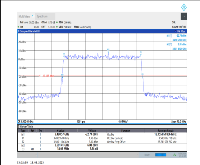
1-N78-3450-3550-30-20-M-9-CP-256QAM-Outer_Fu II-51@0-Ant0-18.156-18.960-≤20-PASS
