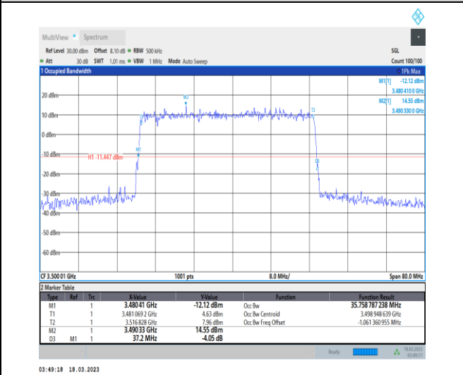
1-N78-3450-3550-30-40-M-1-DFT-QPSK-Outer_Full-100@0-Ant0-35.759-37.200-≤40-PASS
