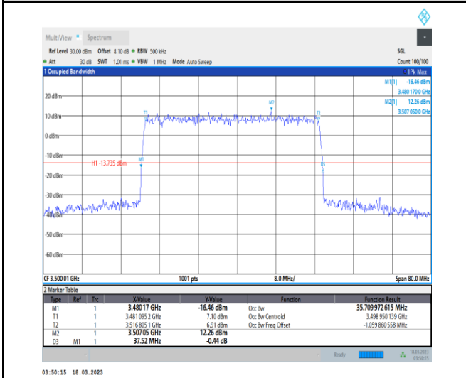
1-N78-3450-3550-30-40-M-4-DFT-64QAM-Outer_Full-100@0-Ant0-35.71-37.520-≤40-PASS
