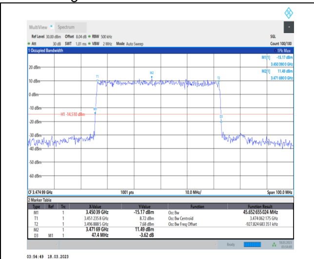
1-N78-3450-3550-30-50-L-1-DFT-QPSK-Outer_Full-128@0-Ant0-45.653-47.400-≤50-PASS
