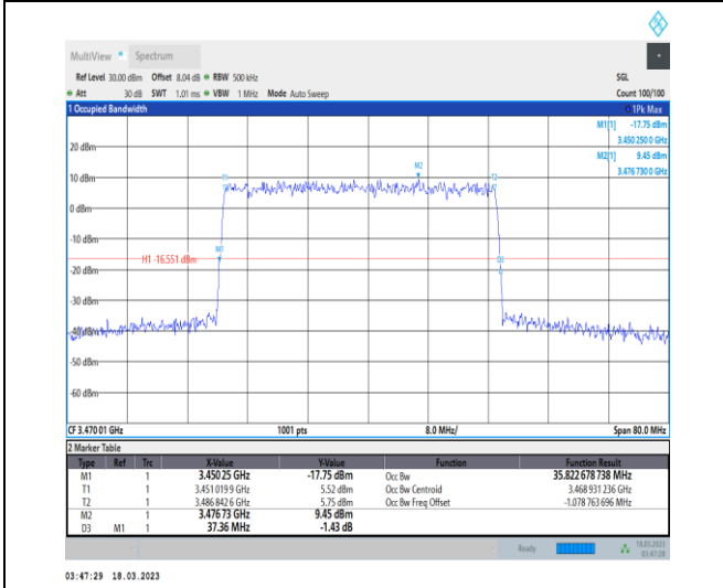
1-N78-3450-3550-30-40-L-5-DFT-256QAM-Outer_Fu II-100@0-Ant0-35.823-37.360-≤40-PASS
