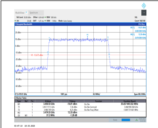
1-N78-3450-3550-30-40-L-3-DFT-16QAM-Outer_Full -100@0-Ant0-35.657-37.200-≤40-PASS
