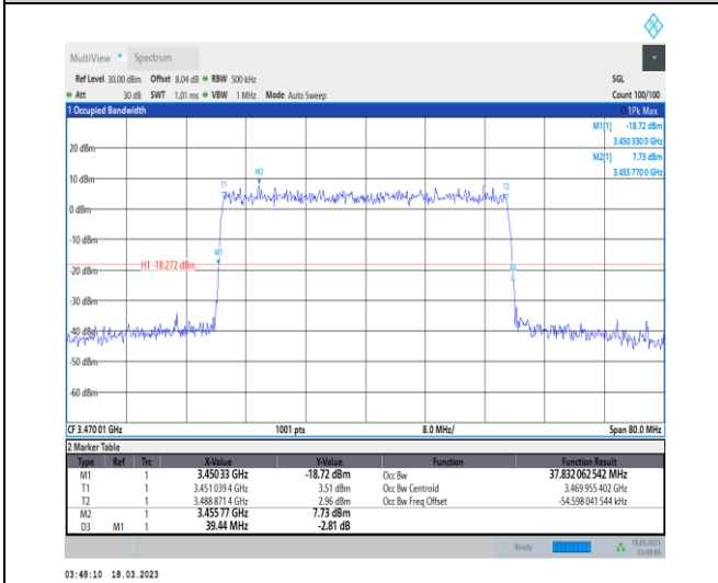
1-N78-3450-3550-30-40-L-9-CP-256QAM-Outer_Full-106@0-Ant0-37.832-39.440-≤40-PASS
