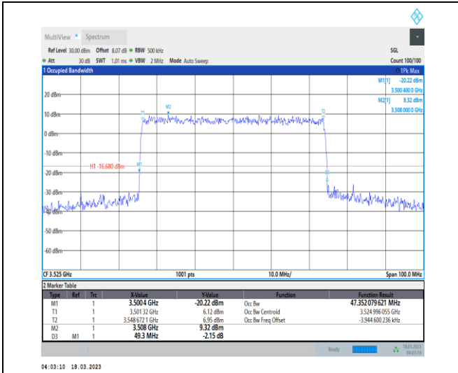
1-N78-3450-3550-30-50-H-6-CP-QPSK-Outer_Full-1 33@0-Ant0-47.352-49.300-≤50-PASS
