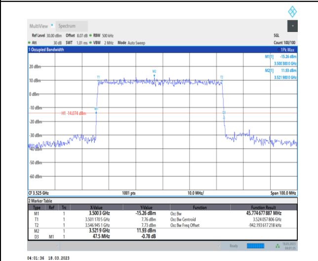
1-N78-3450-3550-30-50-H-1-DFT-QPSK-Outer_Full-128@0-Ant0-45.775-47.500-≤50-PASS
