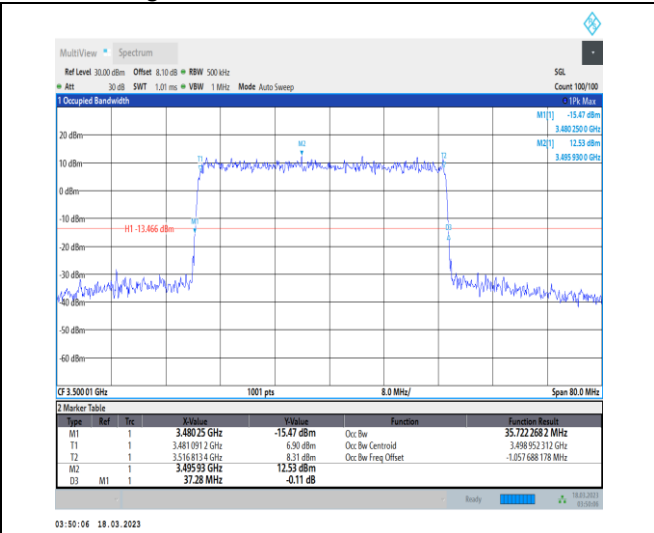
1-N78-3450-3550-30-40-M-3-DFT-16QAM-Outer_Full-100@0-Ant0-35.722-37.280-≤40-PASS
