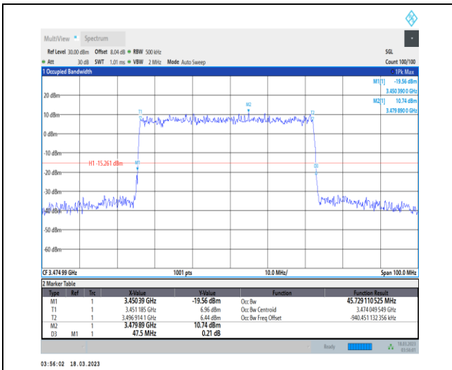
1-N78-3450-3550-30-50-L-4-DFT-64QAM-Outer_Full -128@0-Ant0-45.729-47.500-≤50-PASS
