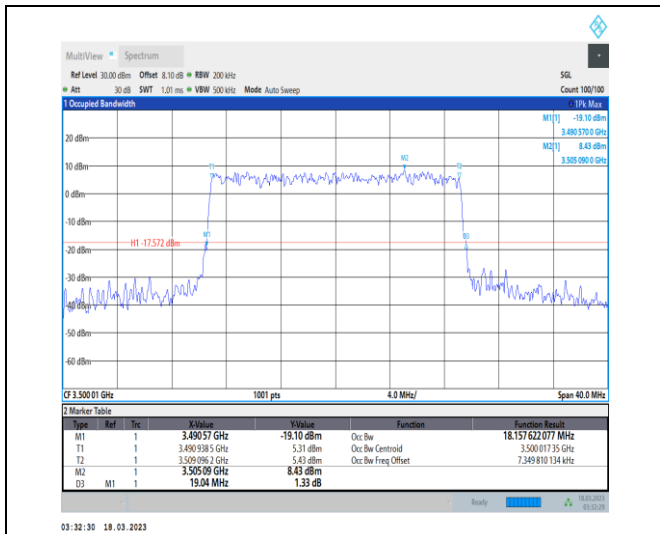
1-N78-3450-3550-30-20-M-6-CP-QPSK-Outer_Full-5 1@0-Ant0-18.158-19.040-≤20-PASS
