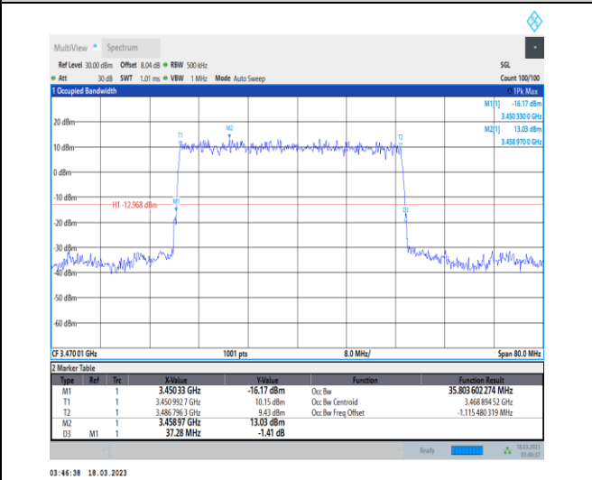
1-N78-3450-3550-30-40-L-2-DFT-PI2BPSK-Outer_Full-100@0-Ant0-35.804-37.280-≤40-PASS
