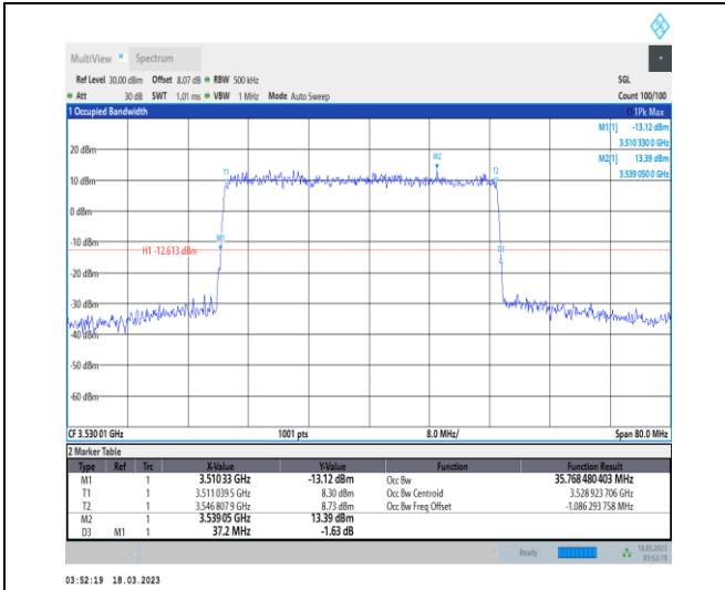
1-N78-3450-3550-30-40-H-1-DFT-QPSK-Outer_Full-100@0-Ant0-35.768-37.200-≤40-PASS
