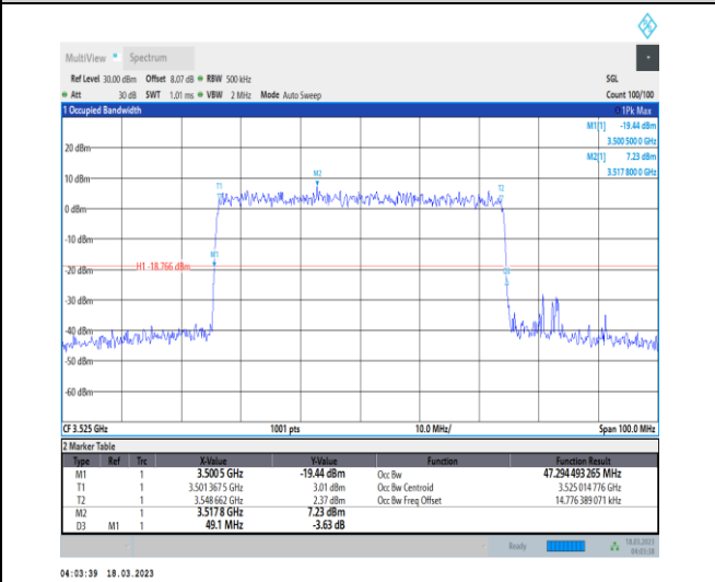
1-N78-3450-3550-30-50-H-9-CP-256QAM-Outer_Full-133@0-Ant0-47.294-49.100-≤50-PASS
