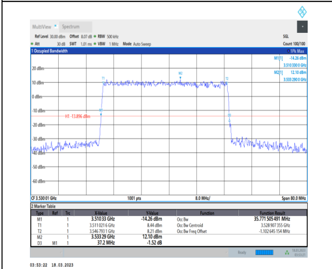
1-N78-3450-3550-30-40-H-3-DFT-16QAM-Outer_Full-100@0-Ant0-35.772-37.200-≤40-PASS
