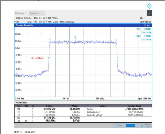
1-N78-3450-3550-30-60-L-2-DFT-PI2BPSK-Outer_Full-162@0-Ant0-57.886-59.880-≤60-PASS
