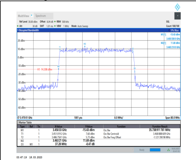
1-N78-3450-3550-30-40-L-4-DFT-64QAM-Outer_Full -100@0-Ant0-35.739-37.280-≤40-PASS
