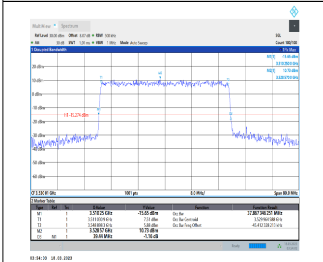
1-N78-3450-3550-30-40-H-7-CP-16QAM-Outer_Full-106@0-Ant0-37.867-39.440-≤40-PASS
