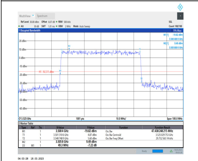
1-N78-3450-3550-30-50-H-8-CP-64QAM-Outer_Full-133@0-Ant0-47.438-49.300-≤50-PASS
