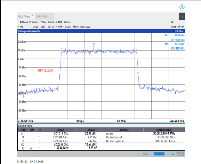
1-N78-3450-3550-30-40-H-4-DFT-64QAM-Outer_Full-100@0-Ant0-35.682-37.440-≤40-PASS
