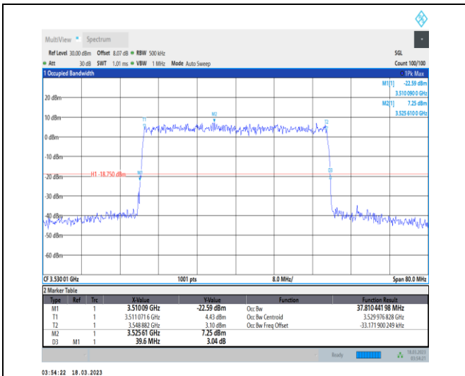
1-N78-3450-3550-30-40-H-9-CP-256QAM-Outer_Ful I-106@0-Ant0-37.81-39.600-≤40-PASS
