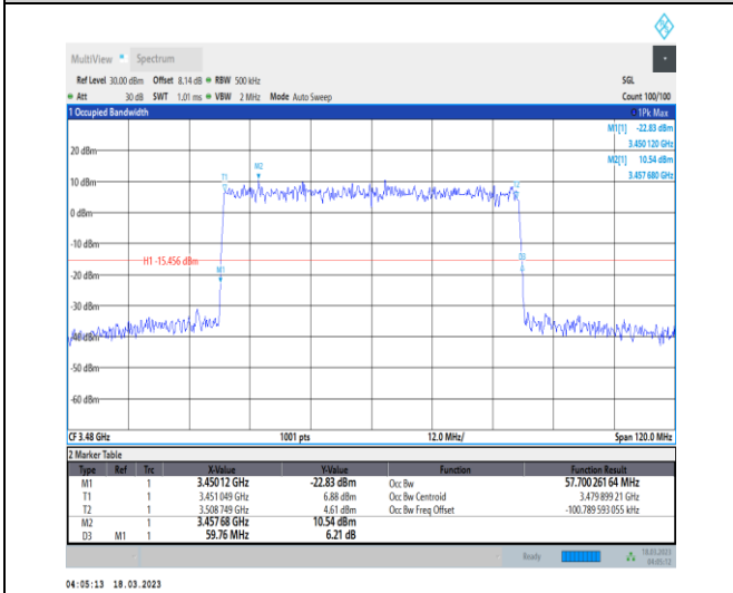
1-N78-3450-3550-30-60-L-3-DFT-16QAM-Outer_Full-162@0-Ant0-57.7-59.760-≤60-PASS
