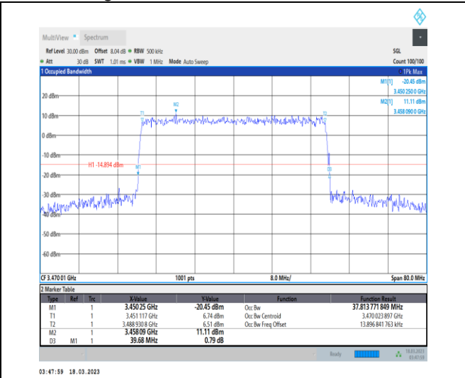
1-N78-3450-3550-30-40-L-8-CP-64QAM-Outer_Full-106@0-Ant0-37.814-39.680-≤40-PASS
