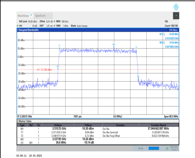
1-N78-3450-3550-30-40-H-8-CP-64QAM-Outer_Full-106@0-Ant0-37.945-39.600-≤40-PASS
