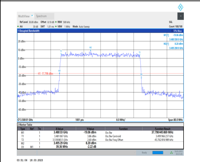
1-N78-3450-3550-30-40-M-9-CP-256QAM-Outer_Full-106@0-Ant0-37.798-39.360-≤40-PASS
