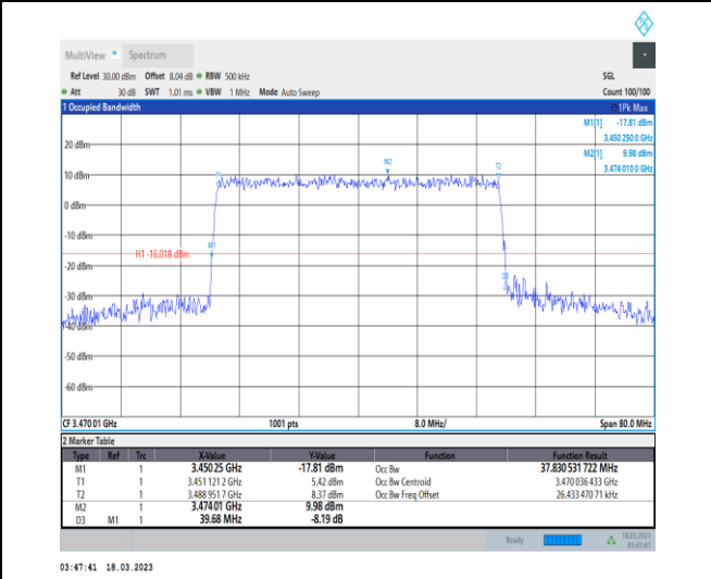
1-N78-3450-3550-30-40-L-6-CP-QPSK-Outer_Full-1 06@0-Ant0-37.831-39.680-≤40-PASS
