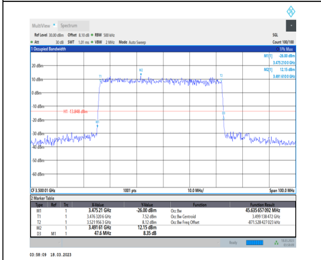
1-N78-3450-3550-30-50-M-1-DFT-QPSK-Outer_Full-128@0-Ant0-45.636-47.600-≤50-PASS
