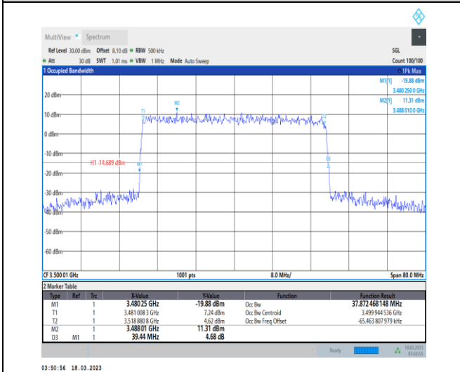
1-N78-3450-3550-30-40-M-8-CP-64QAM-Outer_Full-106@0-Ant0-37.872-39.440-≤40-PASS
