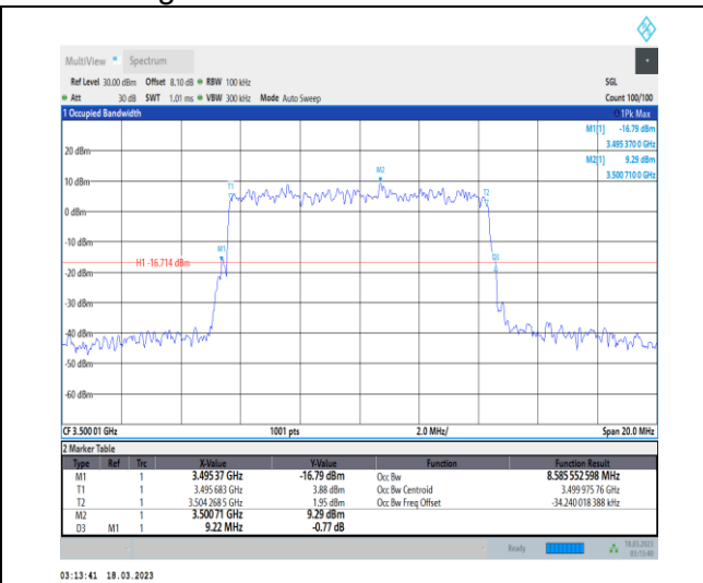
1-N78-3450-3550-30-10-M-5-DFT-256QAM-Outer_Full-24@0-Ant0-8.586-9.220-≤10-PASS
