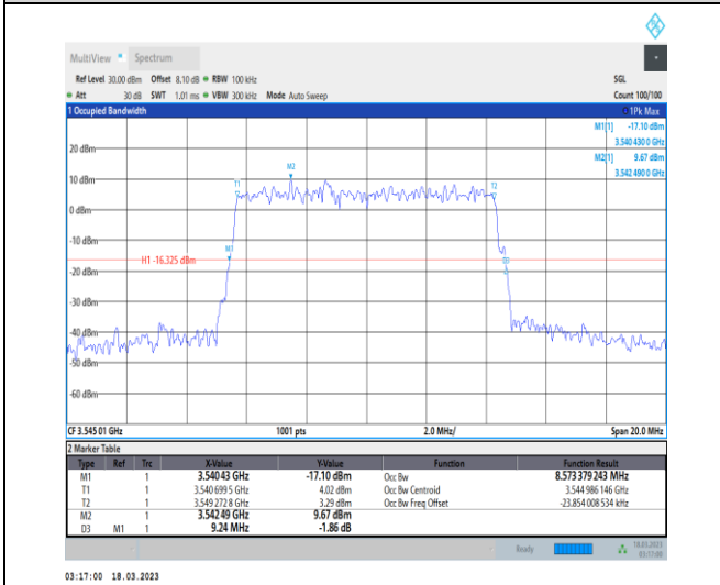
1-N78-3450-3550-30-10-H-5-DFT-256QAM-Outer_Full-24@0-Ant0-8.573-9.240-≤10-PASS
