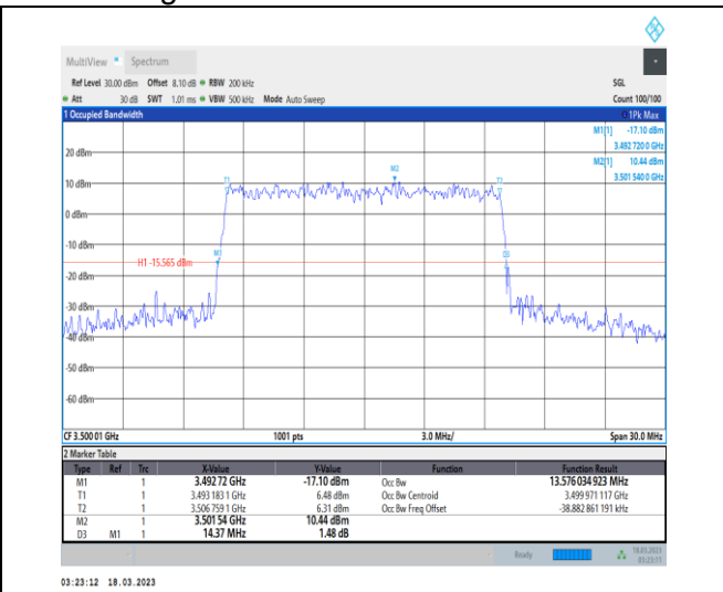
1-N78-3450-3550-30-15-M-6-CP-QPSK-Outer_Full-38@0-Ant0-13.576-14.370-≤15-PASS
