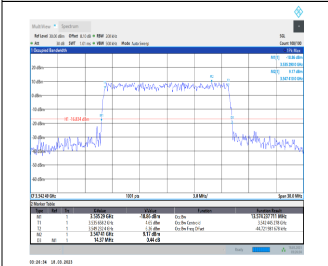
1-N78-3450-3550-30-15-H-6-CP-QPSK-Outer_Full-I-38@0-Ant0-13.574-14.370-≤15-PASS
