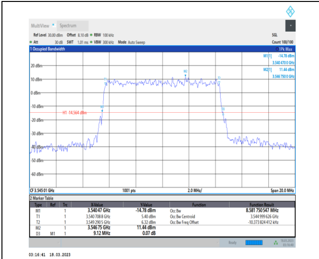
1-N78-3450-3550-30-10-H-3-DFT-16QAM-Outer_Full-24@0-Ant0-8.582-9.120-≤10-PASS
