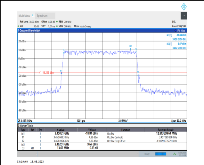
1-N78-3450-3550-30-15-L-5-DFT-256QAM-Outer_Full-36@0-Ant0-12.813-13.620-≤15-PASS
