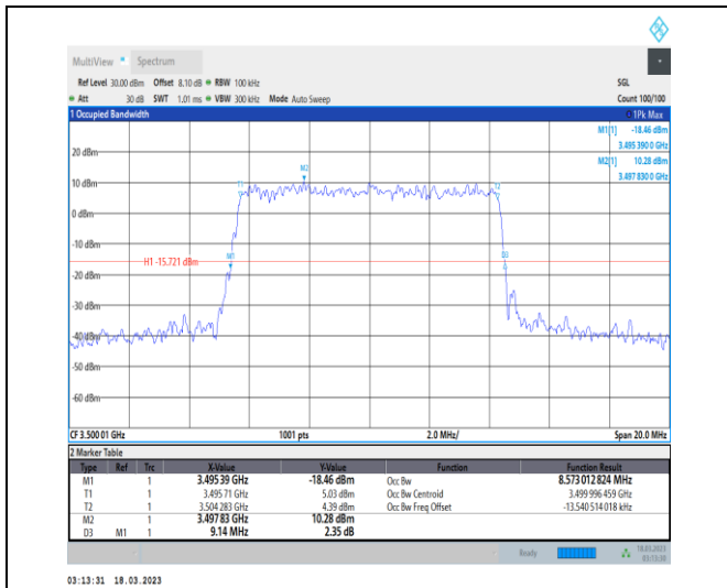
1-N78-3450-3550-30-10-M-4-DFT-64QAM-Outer_Ful I-24@0-Ant0-8.573-9.140-≤10-PASS
