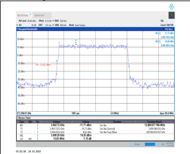
1-N78-3450-3550-30-15-M-2-DFT-PI2BPSK-Outer_Full-36@0-Ant0-12.893-13.650-≤15-PASS
