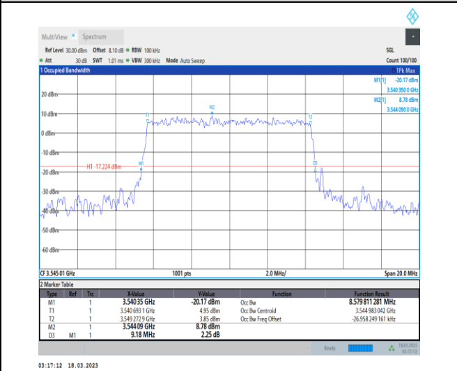
1-N78-3450-3550-30-10-H-6-CP-QPSK-Outer_Full-24@0-Ant0-8.58-9.180-≤10-PASS
