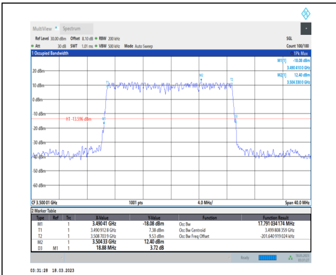
1-N78-3450-3550-30-20-M-2-DFT-PI2BPSK-Outer_Full-50@0-Ant0-17.791-18.880-≤20-PASS
