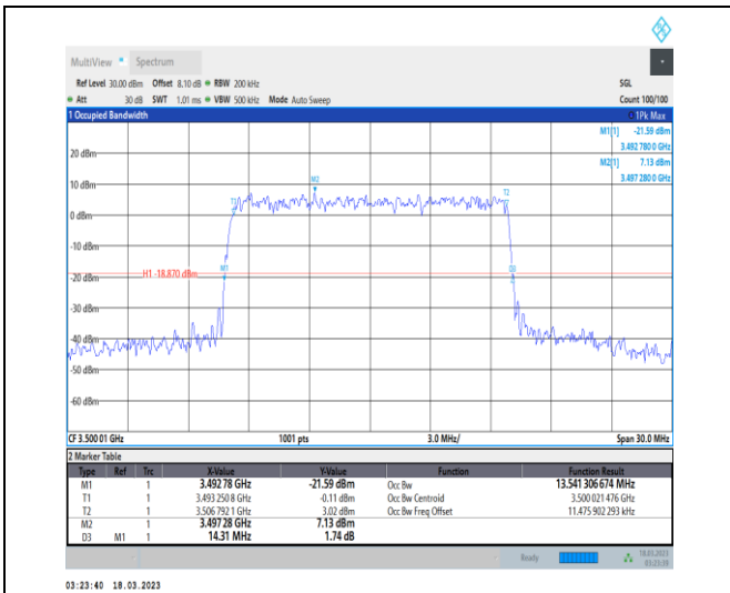
1-N78-3450-3550-30-15-M-9-CP-256QAM-Outer_Ful I-38@0-Ant0-13.541-14.310-≤15-PASS
