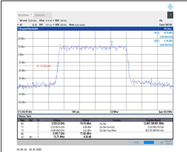
1-N78-3450-3550-30-15-H-4-DFT-64QAM-Outer_Full-I-36@0-Ant0-12.841-13.710-≤15-PASS
