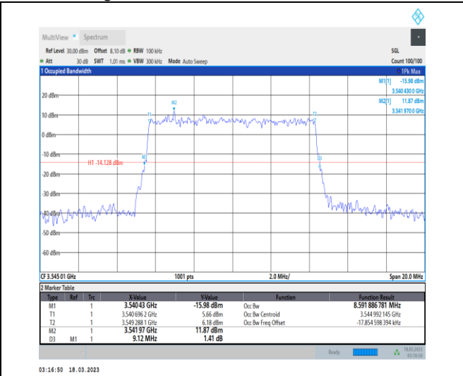
1-N78-3450-3550-30-10-H-4-DFT-64QAM-Outer_Full-24@0-Ant0-8.592-9.120-≤10-PASS
