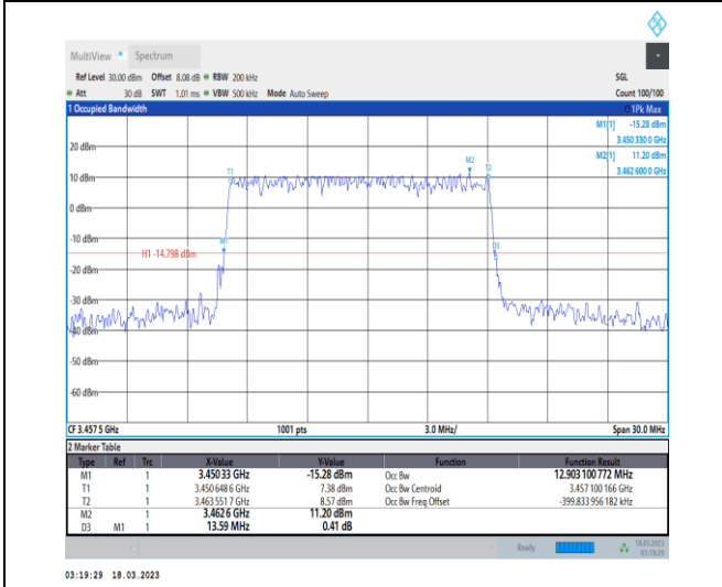
1-N78-3450-3550-30-15-L-4-DFT-64QAM-Outer_Full-36@0-Ant0-12.903-13.590-≤15-PASS
