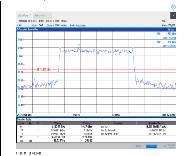
1-N78-3450-3550-30-20-L-8-CP-64QAM-Outer_Full-51@0-Ant0-18.213-19.120-≤20-PASS
