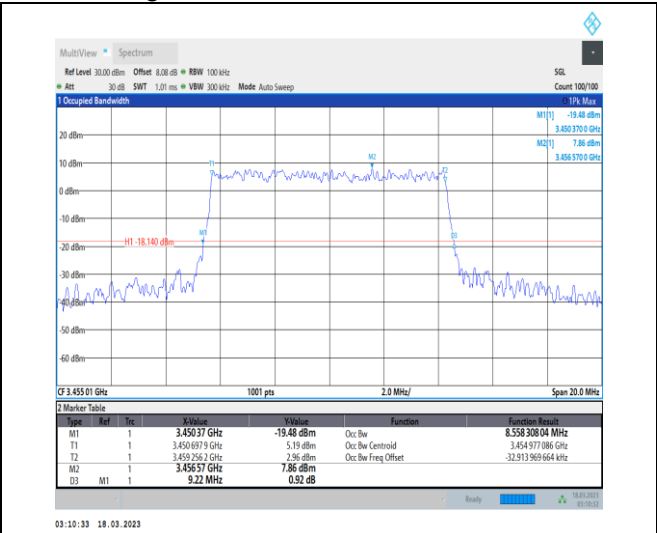
1-N78-3450-3550-30-10-L-6-CP-QPSK-Outer_Full-2 4@0-Ant0-8.558-9.220-≤10-PASS
