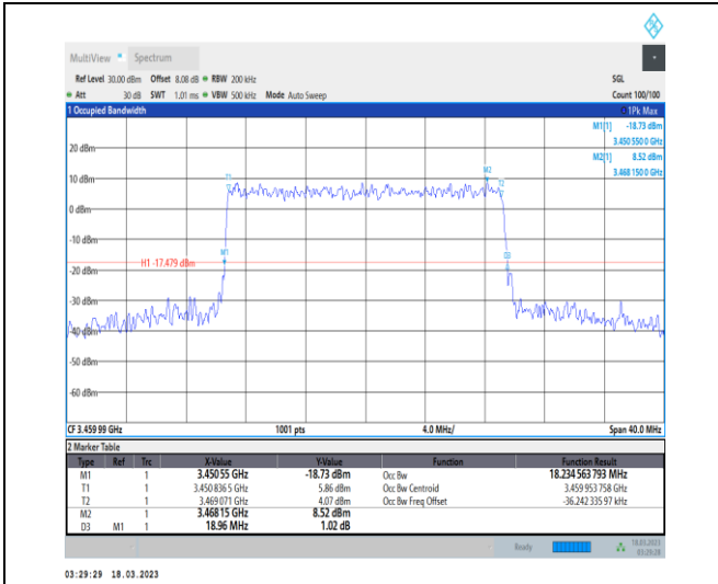
1-N78-3450-3550-30-20-L-7-CP-16QAM-Outer_Full-51@0-Ant0-18.235-18.960-≤20-PASS
