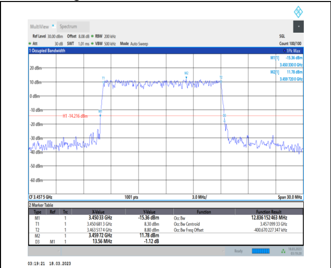
1-N78-3450-3550-30-15-L-3-DFT-16QAM-Outer_Full-36@0-Ant0-12.836-13.560-≤15-PASS
