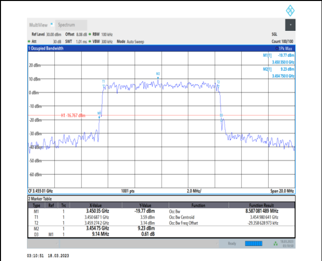
1-N78-3450-3550-30-10-L-8-CP-64QAM-Outer_Full-24@0-Ant0-8.587-9.140-≤10-PASS
