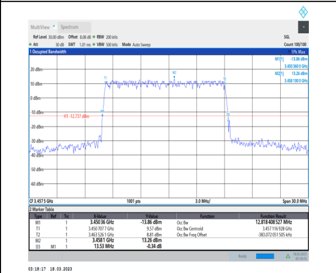
1-N78-3450-3550-30-15-L-1-DFT-QPSK-Outer_Full-36@0-Ant0-12.818-13.530-≤15-PASS
