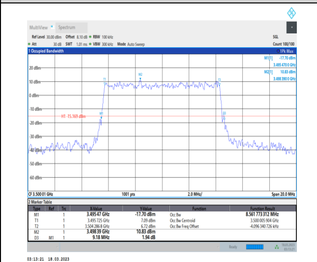
1-N78-3450-3550-30-10-M-3-DFT-16QAM-Outer_Full -24@0-Ant0-8.562-9.180-≤10-PASS
