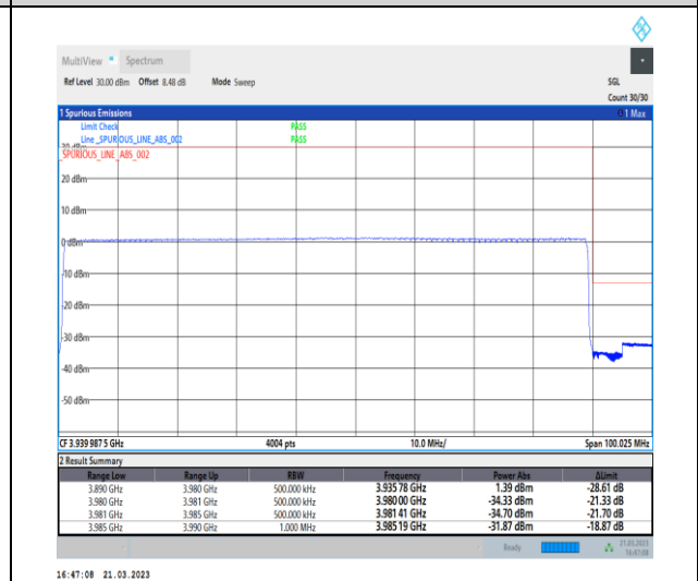
1-N77-3700-3980-30-90-H-6-CP-QPSK-Outer_Full -245@0-Ant0-1--PASS-see graph
