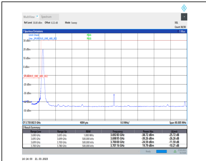
1-N77-3700-3980-30-80-L-4-CP-QPSK-Edge_1RB_Lef t-1@0-Ant0-1--PASS-see graph
