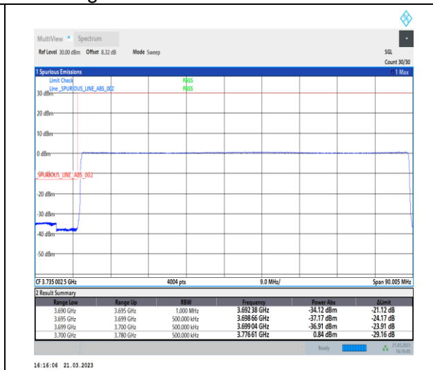
1-N77-3700-3980-30-80-L-6-CP-QPSK-Outer_Full -217@0-Ant0-1--PASS-see graph
