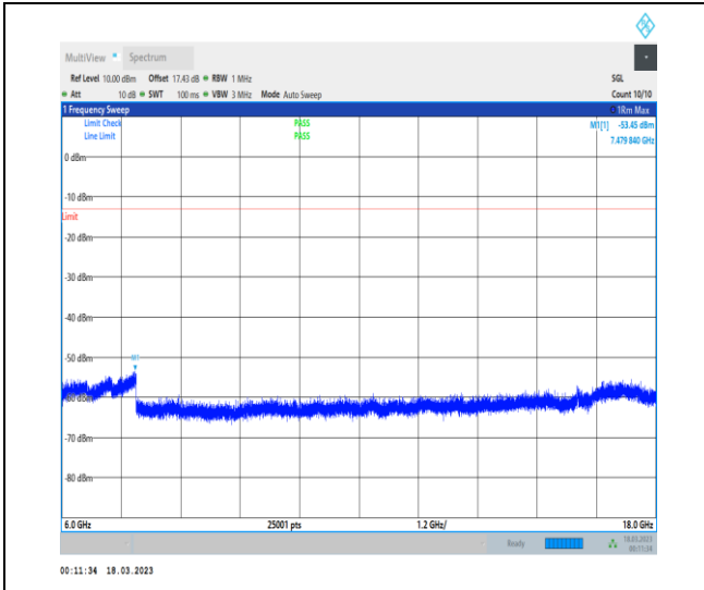
1-N77-3700-3980-30-100-L-1-DFT-PI2BPSK-Inner_1RB_Left-1@1-6000-18000-Ant0-7479.84--53.45--1 3-PASS
