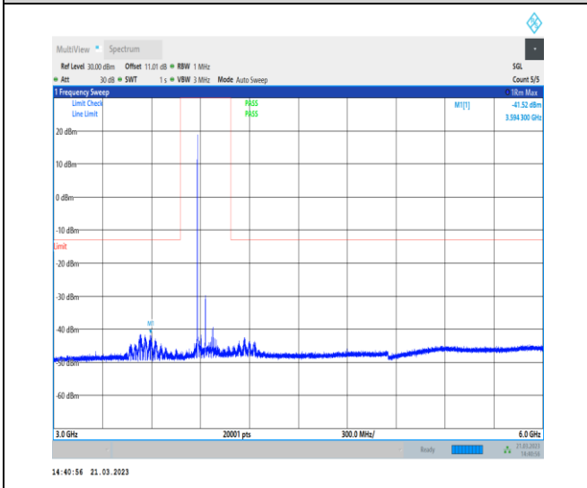
1-N77-3700-3980-30-100-H-1-DFT-QPSK-Edge_1R B_Left-1@0-3000-6000-Ant0-3594.30--41.52--13-PA SS
