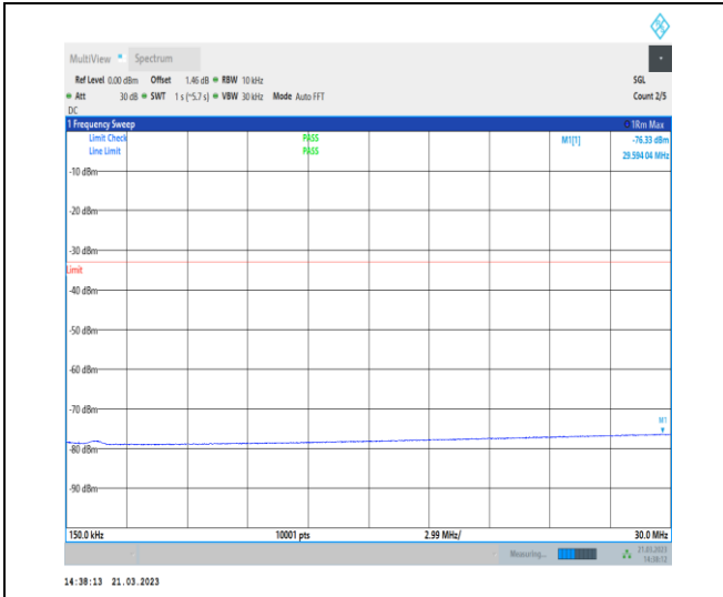
1-N77-3700-3980-30-100-M-1-DFT-QPSK-Edge_1R B_Left-1@0-0.15-30-Ant0-29.59--76.33--33-PASS
