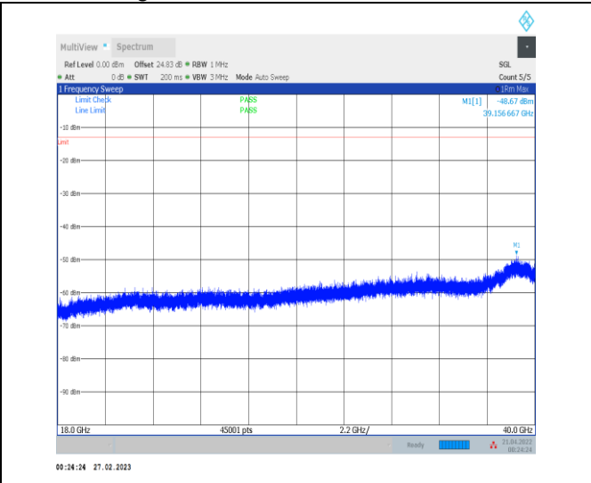
1-N77-3700-3980-30-100-L-1-DFT-PI2BPSK-Inner_1RB_Left-1@1-18000-40000-Ant0-18000.00--57.13--1 3-PASS
