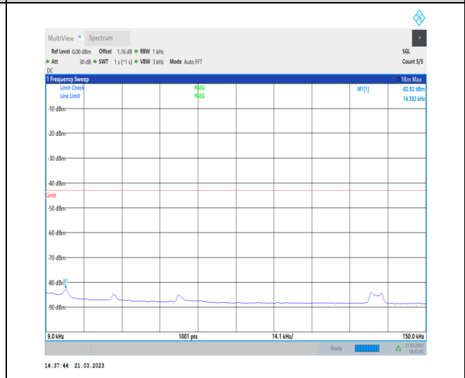
1-N77-3700-3980-30-100-M-1-DFT-QPSK-Edge_1R B_Left-1@0-0.009-0.15-Ant0-0.02--82.92--43-PASS
