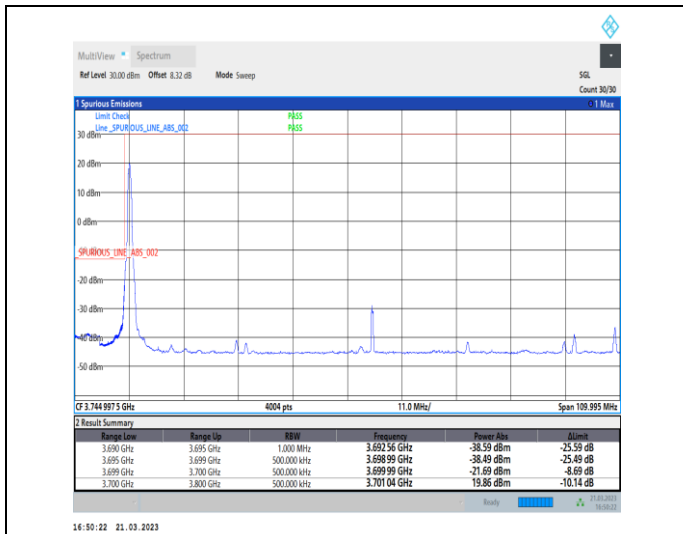
1-N77-3700-3980-30-100-L-4-CP-QPSK-Edge_1RB_L eft-1@0-Ant0-1--PASS-see graph
