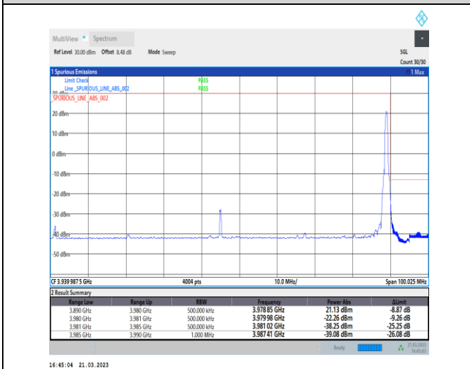
1-N77-3700-3980-30-90-H-5-CP-QPSK-Edge_1RB_Ri ght-1@244-Ant0-1--PASS-see graph
