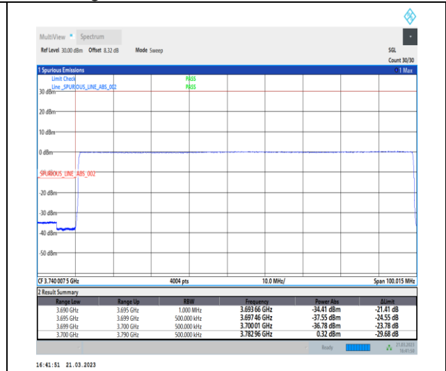
1-N77-3700-3980-30-90-L-6-CP-QPSK-Outer_Full -245@0-Ant0-1--PASS-see graph
