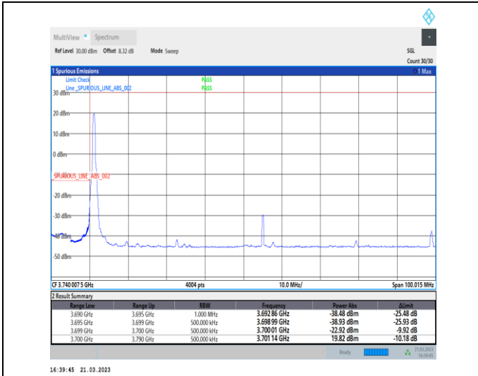
1-N77-3700-3980-30-90-L-4-CP-QPSK-Edge_1RB_Lef t-1@0-Ant0-1--PASS-see graph
