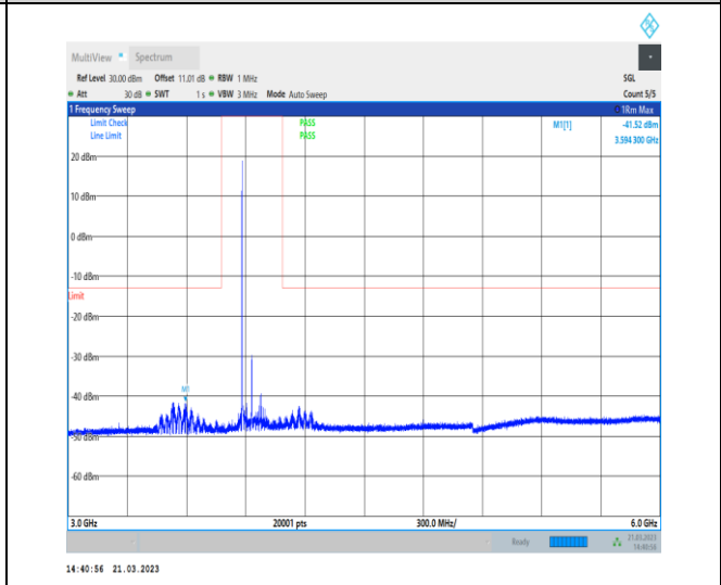
1-N77-3700-3980-30-100-M-1-DFT-QPSK-Edge_1R B_Left-1@0-3000-6000-Ant0-3465.75--39.26--13-PA SS
