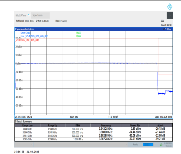
1-N77-3700-3980-30-100-H-6-CP-QPSK-Outer_F ull-273@0-Ant0-1--PASS-see graph
