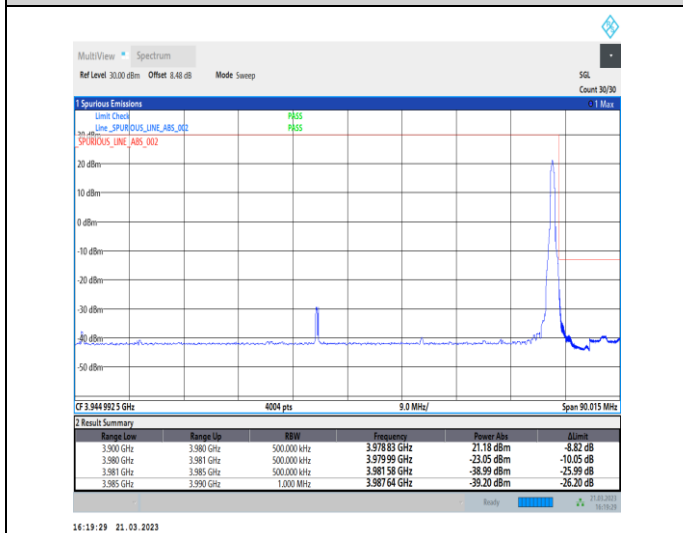
1-N77-3700-3980-30-80-H-5-CP-QPSK-Edge_1RB_Ri ght-1@216-Ant0-1--PASS-see graph
