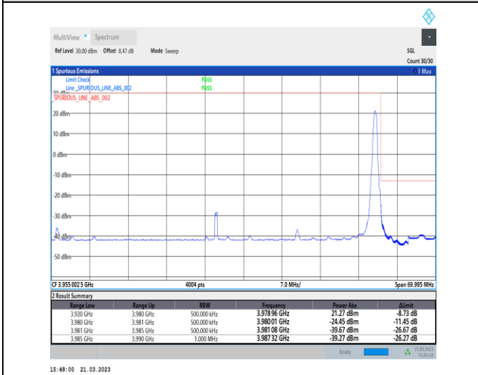
1-N77-3700-3980-30-60-H-5-CP-QPSK-Edge_1RB_Ri ght-1@161-Ant0-1--PASS-see graph
