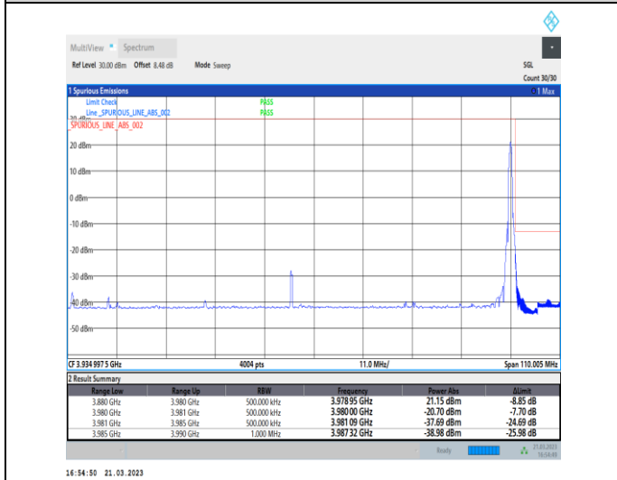
1-N77-3700-3980-30-100-H-5-CP-QPSK-Edge_1RB_R ight-1@272-Ant0-1--PASS-see graph
