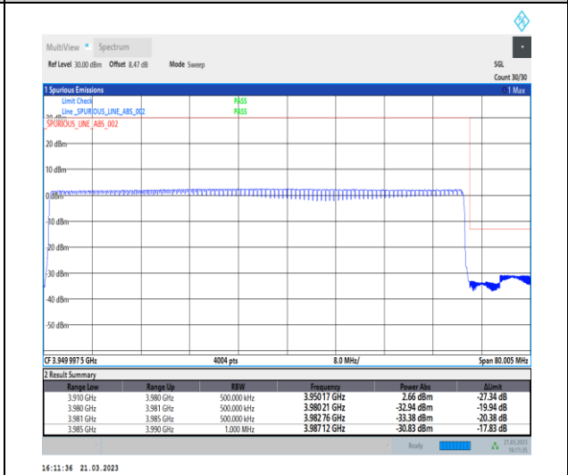
1-N77-3700-3980-30-70-H-6-CP-QPSK-Outer_Full -189@0-Ant0-1--PASS-see graph
