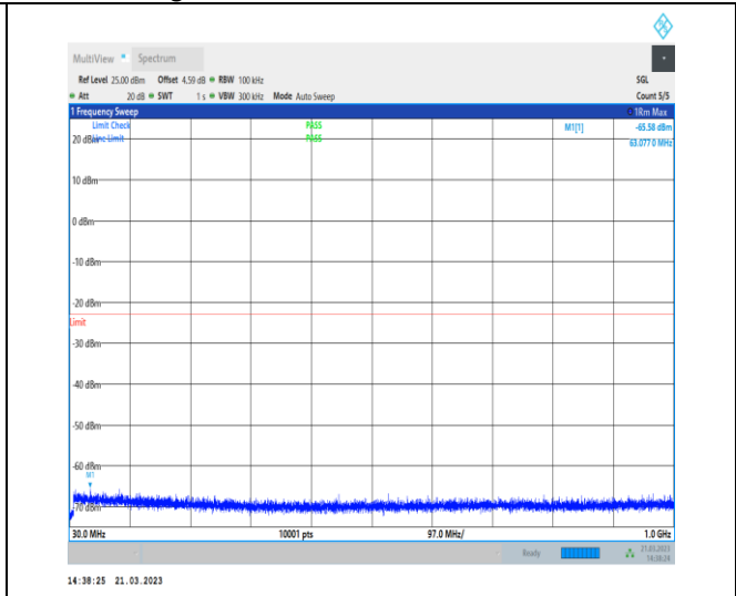
1-N77-3700-3980-30-100-M-1-DFT-QPSK-Edge_1R B_Left-1@0-30-1000-Ant0-63.08--65.58--23-PASS
