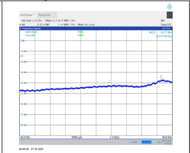
1-N77-3700-3980-30-100-M-1-DFT-QPSK-Edge_1R B_Left-1@0-26000-40000-Ant0-26000.00--45.07--13- -PASS
