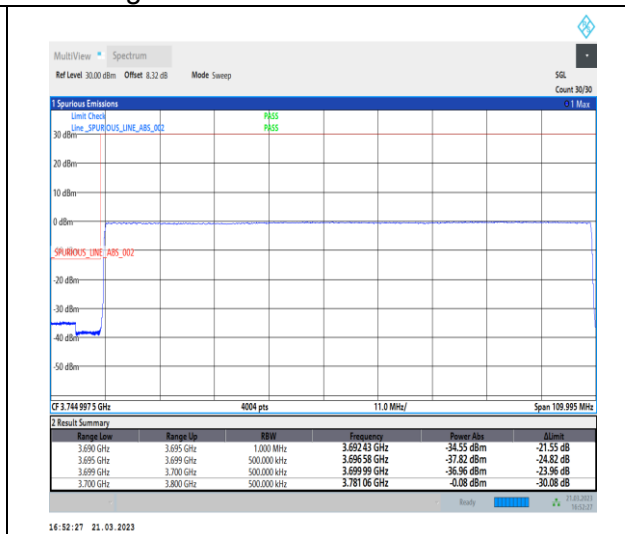
1-N77-3700-3980-30-100-L-6-CP-QPSK-Outer_Fu II-273@0-Ant0-1--PASS-see graph
