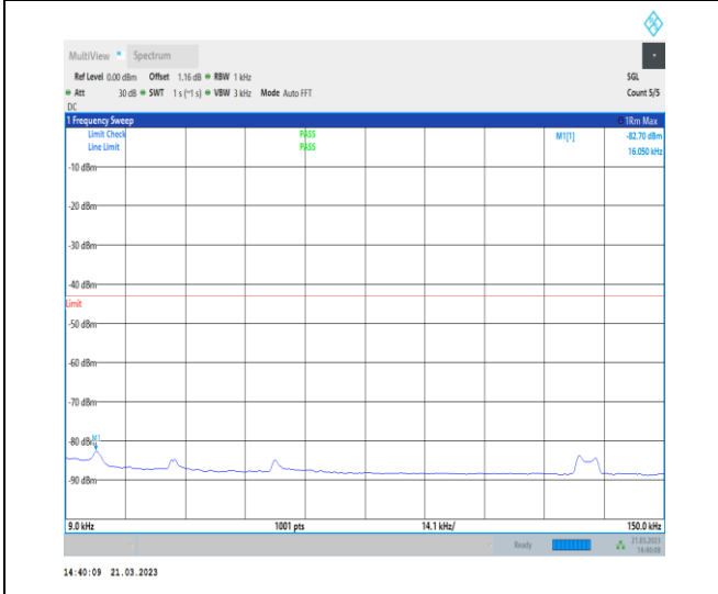
1-N77-3700-3980-30-100-H-1-DFT-QPSK-Edge_1R B_Left-1@0-0.009-0.15-Ant0-0.02--82.70--43-PASS
