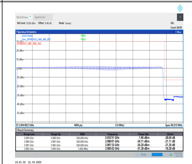
1-N77-3700-3980-30-80-H-6-CP-QPSK-Outer_Full -217@0-Ant0-1--PASS-see graph
