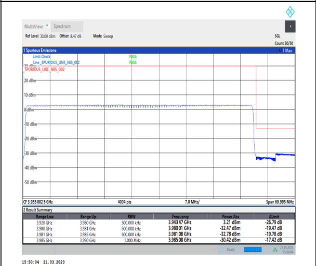
1-N77-3700-3980-30-60-H-6-CP-QPSK-Outer_Full -162@0-Ant0-1--PASS-see graph
