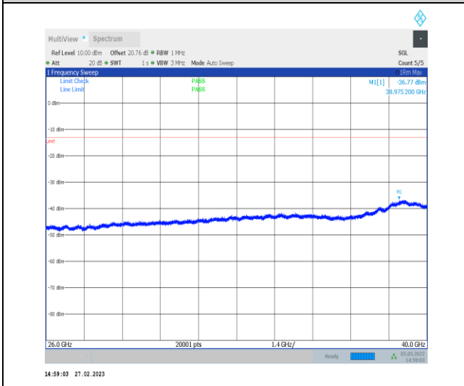
1-N77-3700-3980-30-100-L-1-DFT-QPSK-Edge_1R B_Left-1@0-26000-40000-Ant0-26000.00--45.23--13 -PASS
