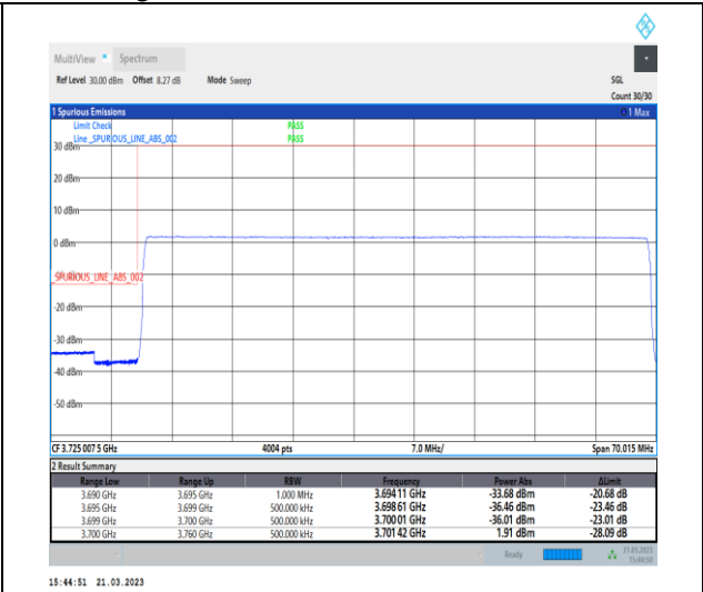
1-N77-3700-3980-30-60-L-6-CP-QPSK-Outer_Full -162@0-Ant0-1--PASS-see graph
