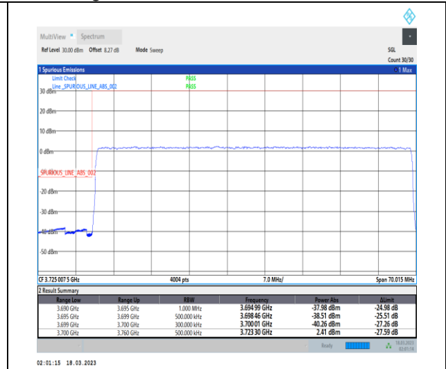
1-N77-3700-3980-30-60-L-3-DFT-PI2BPSK-Outer _Full-162@0-Ant0-1--PASS-see graph
