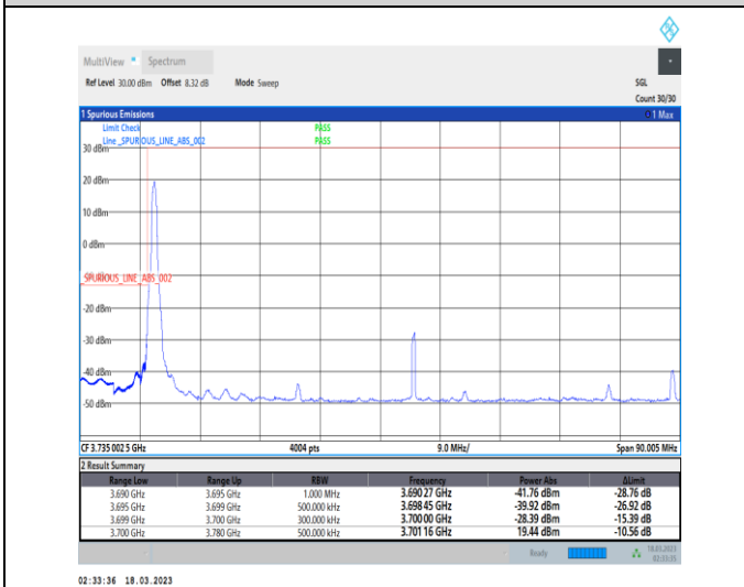
1-N77-3700-3980-30-80-L-4-CP-QPSK-Edge_1RB_Lef t-1@0-Ant0-1--PASS-see graph
