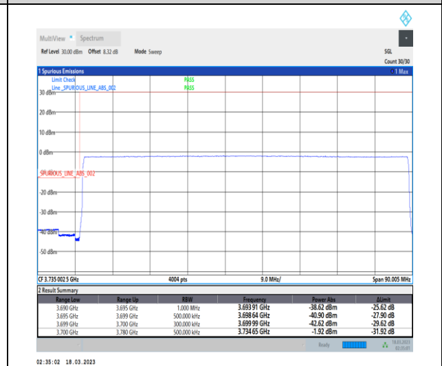
1-N77-3700-3980-30-80-L-6-CP-QPSK-Outer_Full -217@0-Ant0-1--PASS-see graph
