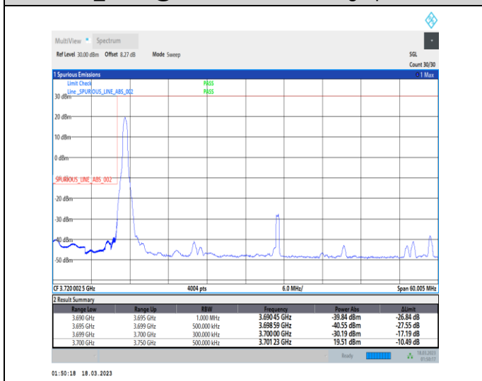
1-N77-3700-3980-30-50-L-4-CP-QPSK-Edge_1RB_Lef t-1@0-Ant0-1--PASS-see graph
