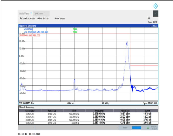
1-N77-3700-3980-30-40-H-5-CP-QPSK-Edge_1RB_Right-1@105-Ant0-1--PASS-see graph
