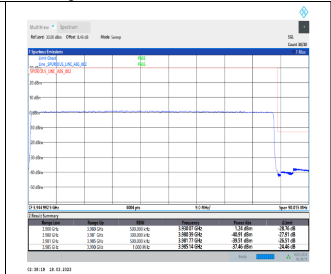
1-N77-3700-3980-30-80-H-3-DFT-PI2BPSK-Outer_Full-216@0-Ant0-1--PASS-see graph
