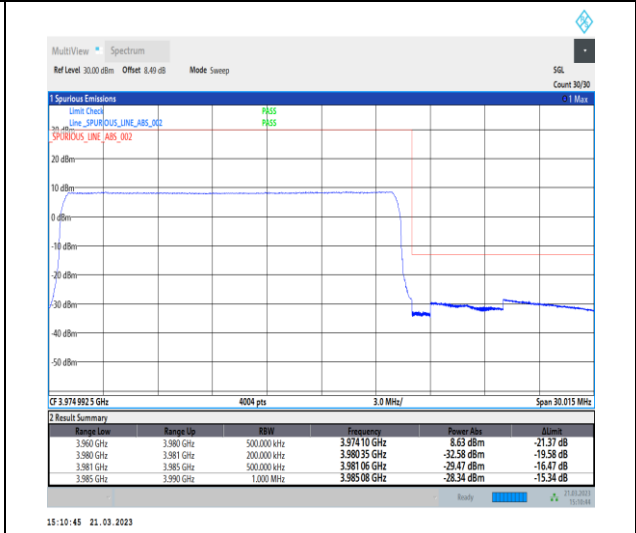
1-N77-3700-3980-30-20-H-6-CP-QPSK-Outer_Full -51@0-Ant0-1--PASS-see graph
