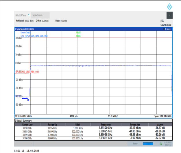
1-N77-3700-3980-30-100-L-6-CP-QPSK-Outer_Full-273@0-Ant0-1--PASS-see graph
