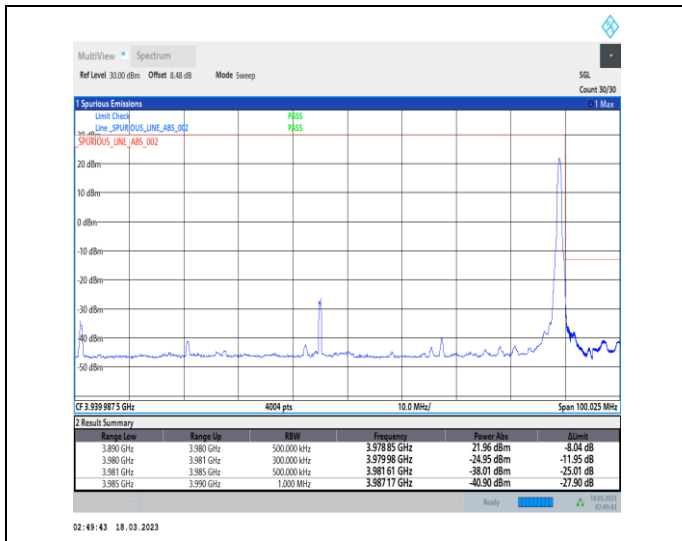
1-N77-3700-3980-30-90-H-2-DFT-PI2BPSK-Edge_1R_B_Right-1@244-Ant0-1--PASS-see graph
