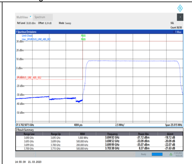
1-N77-3700-3980-30-15-L-6-CP-QPSK-Outer_Full -38@0-Ant0-1--PASS-see graph
