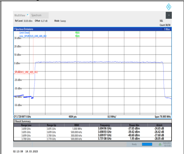
1-N77-3700-3980-30-70-L-3-DFT-PI2BPSK-Outer_Full-180@0-Ant0-1--PASS-see graph
