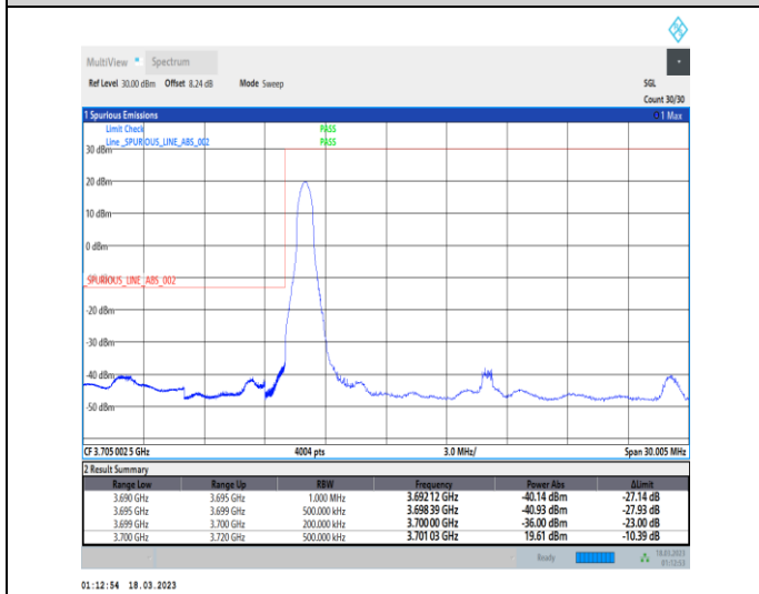
1-N77-3700-3980-30-20-L-4-CP-QPSK-Edge_1RB_Lef t-1@0-Ant0-1--PASS-see graph
