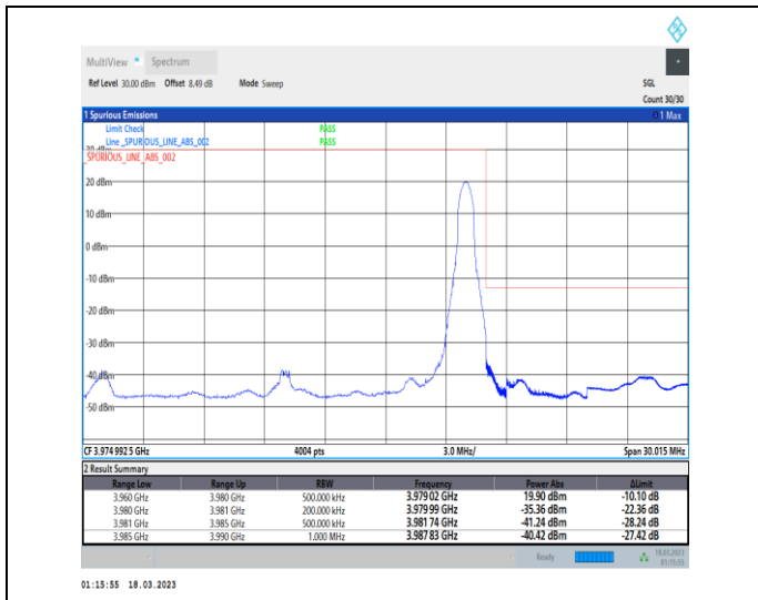
1-N77-3700-3980-30-20-H-2-DFT-PI2BPSK-Edge_1R_B_Right-1@50-Ant0-1--PASS-see graph
