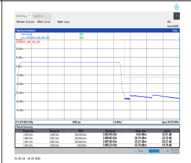
1-N77-3700-3980-30-20-H-6-CP-QPSK-Outer_Full-51@0-Ant0-1--PASS-see graph
