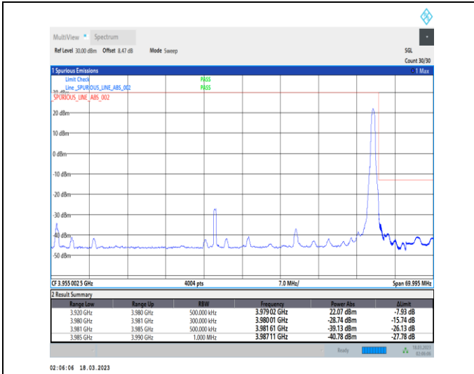
1-N77-3700-3980-30-60-H-2-DFT-PI2BPSK-Edge_1R_B_Right-1@161-Ant0-1--PASS-see graph
