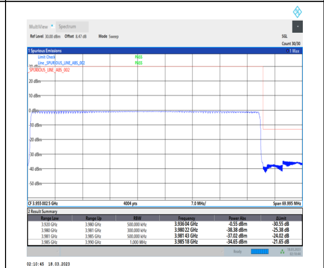
1-N77-3700-3980-30-60-H-6-CP-QPSK-Outer_Full-162@0-Ant0-1--PASS-see graph
