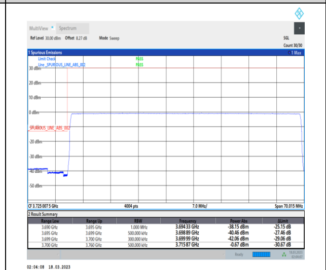
1-N77-3700-3980-30-60-L-6-CP-QPSK-Outer_Full -162@0-Ant0-1--PASS-see graph
