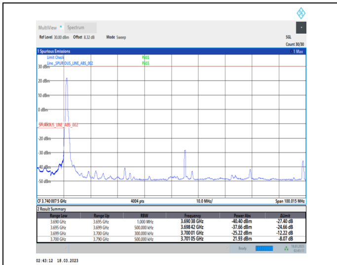
1-N77-3700-3980-30-90-L-1-DFT-PI2BPSK-Edge_1RB_Left-1@0-Ant0-1--PASS-see graph
