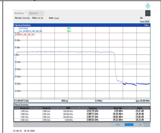
1-N77-3700-3980-30-40-H-3-DFT-PI2BPSK-Outer_Full-100@0-Ant0-1--PASS-see graph
