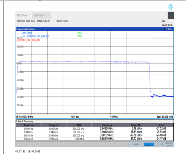
1-N77-3700-3980-30-60-H-3-DFT-PI2BPSK-Outer_Full-162@0-Ant0-1--PASS-see graph
