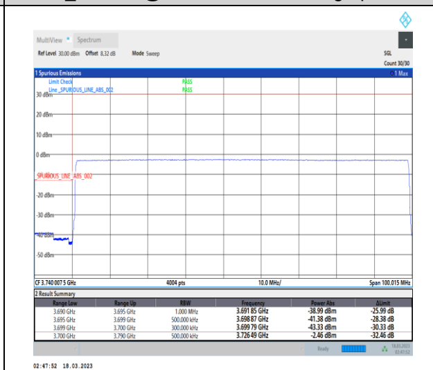
1-N77-3700-3980-30-90-L-6-CP-QPSK-Outer_Full -245@0-Ant0-1--PASS-see graph
