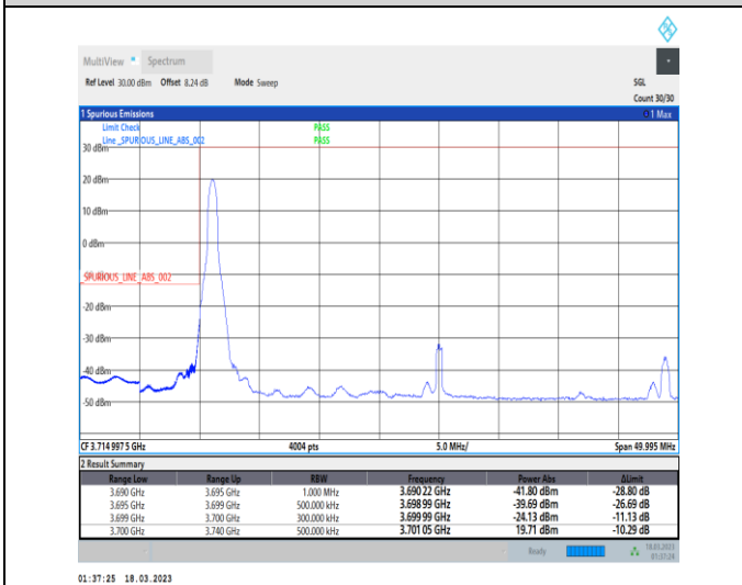
1-N77-3700-3980-30-40-L-4-CP-QPSK-Edge_1RB_Lef t-1@0-Ant0-1--PASS-see graph
