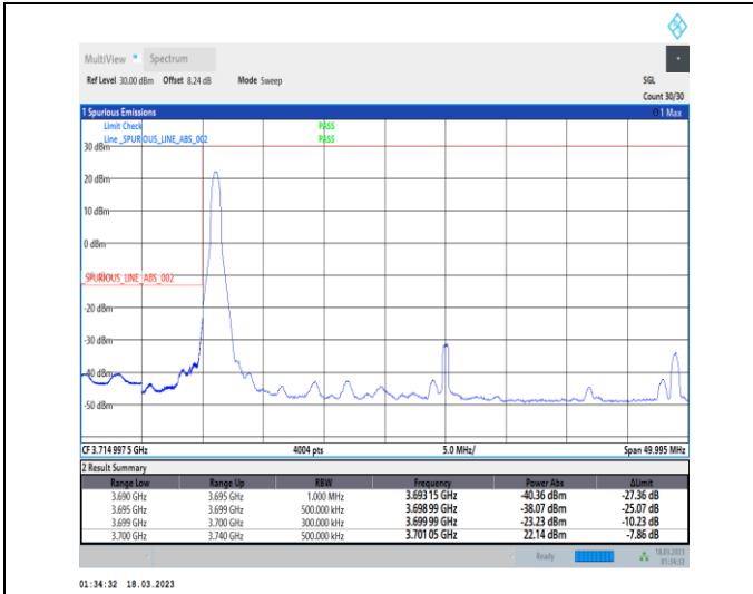
1-N77-3700-3980-30-40-L-1-DFT-PI2BPSK-Edge_1RB _Left-1@0-Ant0-1--PASS-see graph
