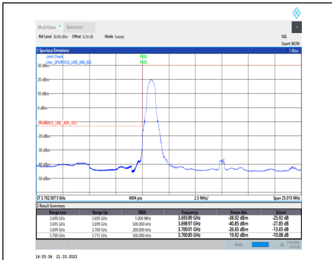
1-N77-3700-3980-30-15-L-4-CP-QPSK-Edge_1RB_Lef t-1@0-Ant0-1--PASS-see graph
