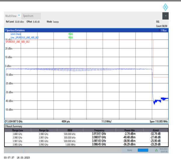
1-N77-3700-3980-30-100-H-6-CP-QPSK-Outer_Full-273@0-Ant0-1--PASS-see graph
