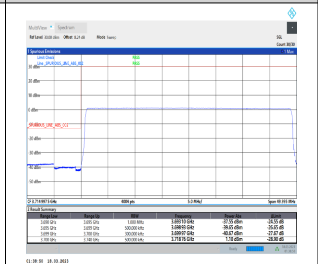
1-N77-3700-3980-30-40-L-6-CP-QPSK-Outer_Full -106@0-Ant0-1--PASS-see graph
