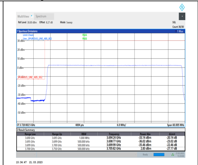
1-N77-3700-3980-30-50-L-6-CP-QPSK-Outer_Full -133@0-Ant0-1--PASS-see graph
