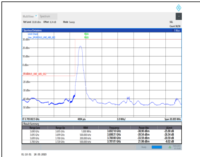
1-N77-3700-3980-30-20-L-1-DFT-PI2BPSK-Edge_1RB _Left-1@0-Ant0-1--PASS-see graph
