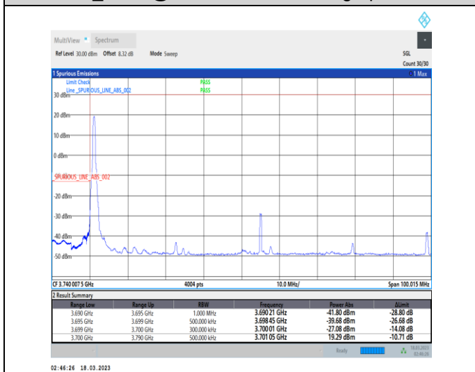
1-N77-3700-3980-30-90-L-4-CP-QPSK-Edge_1RB_Lef t-1@0-Ant0-1--PASS-see graph
