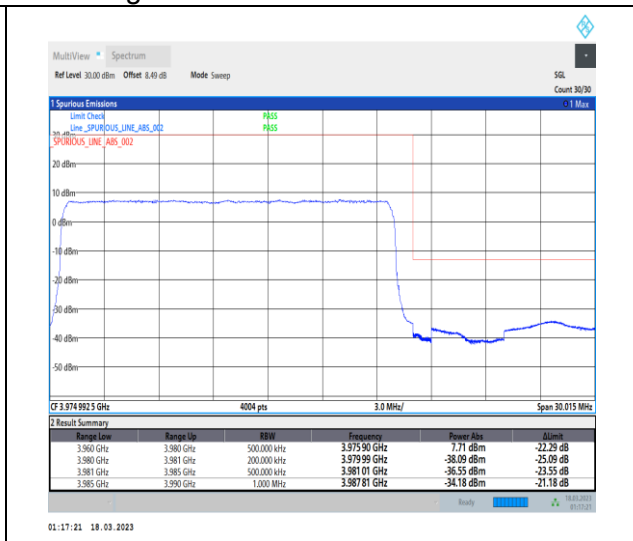
1-N77-3700-3980-30-20-H-3-DFT-PI2BPSK-Outer_Full-50@0-Ant0-1--PASS-see graph
