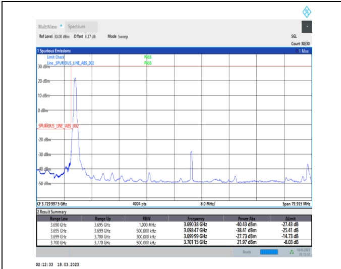
1-N77-3700-3980-30-70-L-1-DFT-PI2BPSK-Edge_1RB_Left-1@0-Ant0-1--PASS-see graph
