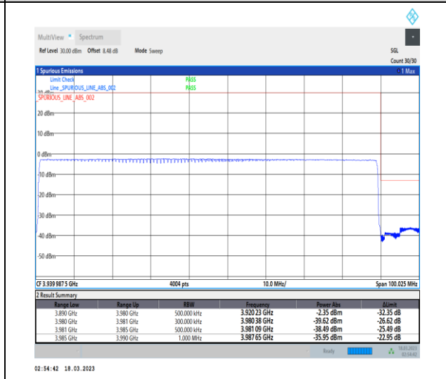
1-N77-3700-3980-30-90-H-6-CP-QPSK-Outer_Full-245@0-Ant0-1--PASS-see graph
