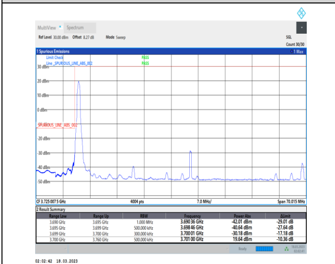
1-N77-3700-3980-30-60-L-4-CP-QPSK-Edge_1RB_Lef t-1@0-Ant0-1--PASS-see graph
