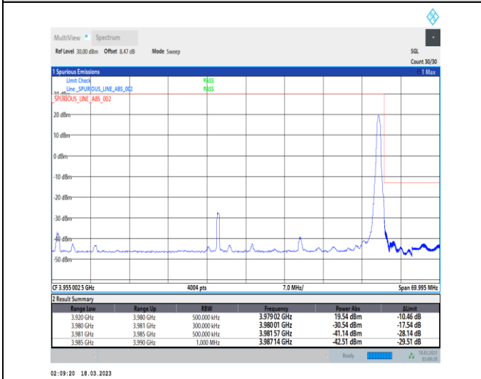
1-N77-3700-3980-30-60-H-5-CP-QPSK-Edge_1RB_Right-1@161-Ant0-1--PASS-see graph
