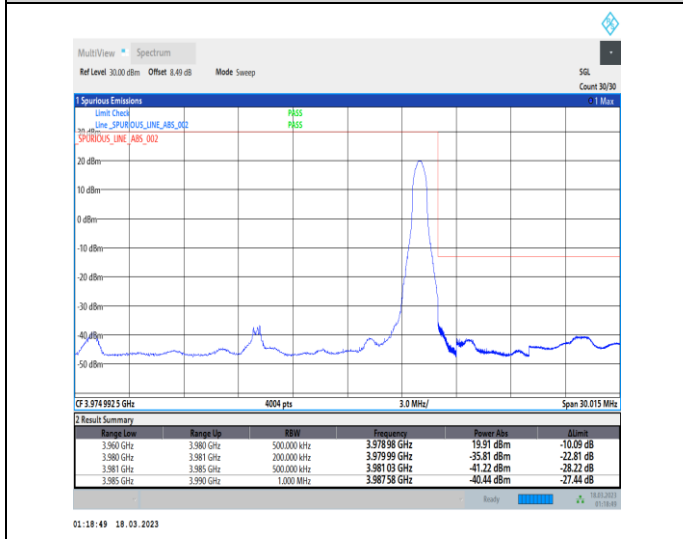
1-N77-3700-3980-30-20-H-5-CP-QPSK-Edge_1RB_Right-1@50-Ant0-1--PASS-see graph
