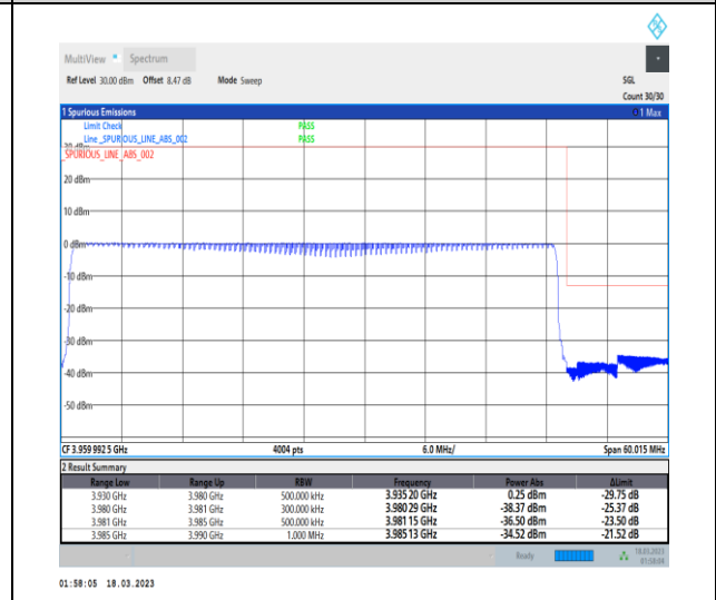
1-N77-3700-3980-30-50-H-6-CP-QPSK-Outer_Full-133@0-Ant0-1--PASS-see graph
