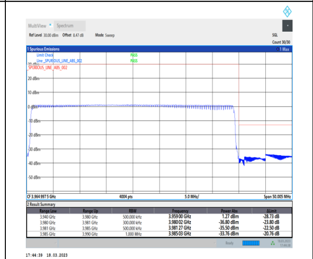
1-N77-3700-3980-30-40-H-6-CP-QPSK-Outer_Full-106@0-Ant0-1--PASS-see graph
