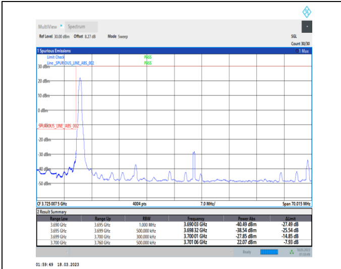
1-N77-3700-3980-30-60-L-1-DFT-PI2BPSK-Edge_1RB _Left-1@0-Ant0-1--PASS-see graph
