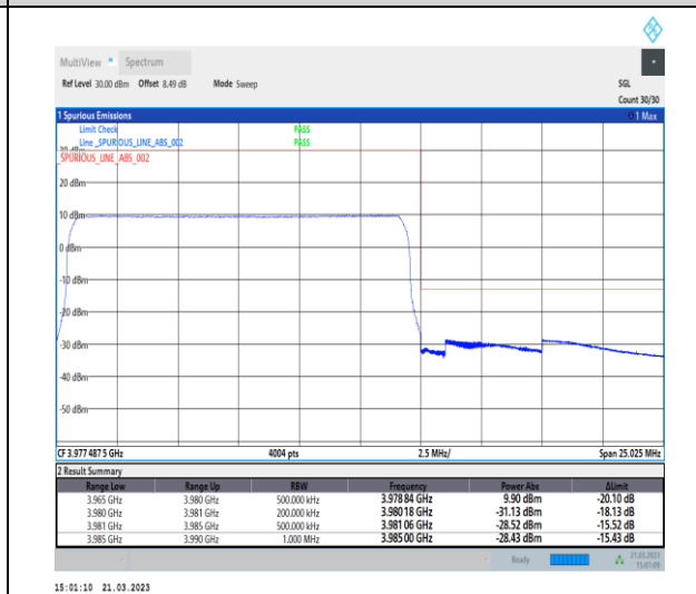
1-N77-3700-3980-30-15-H-6-CP-QPSK-Outer_Full -38@0-Ant0-1--PASS-see graph
