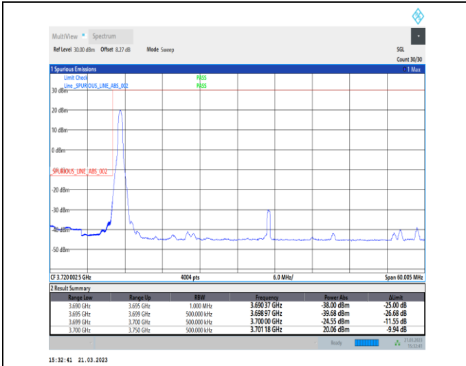
1-N77-3700-3980-30-50-L-4-CP-QPSK-Edge_1RB_Lef t-1@0-Ant0-1--PASS-see graph
