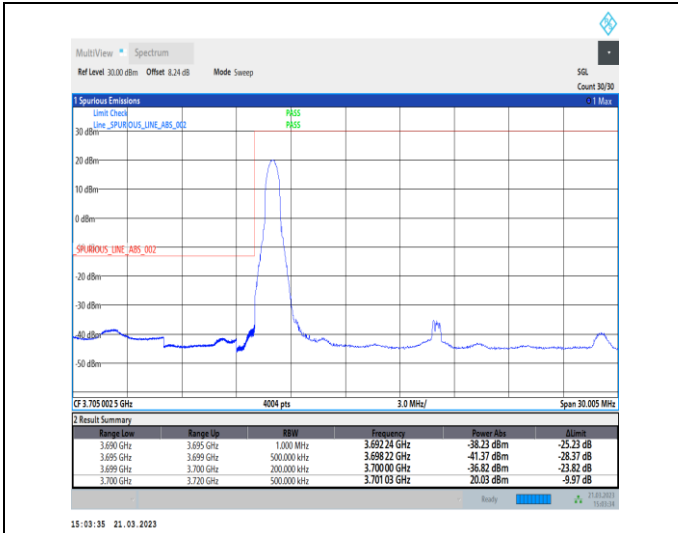
1-N77-3700-3980-30-20-L-4-CP-QPSK-Edge_1RB_Lef t-1@0-Ant0-1--PASS-see graph
