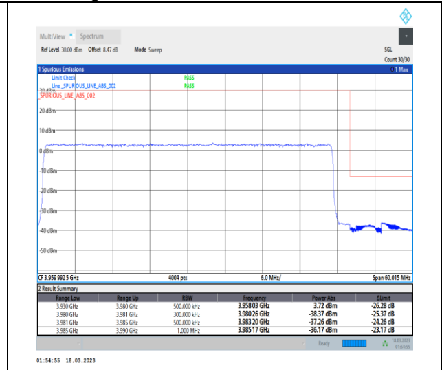
1-N77-3700-3980-30-50-H-3-DFT-PI2BPSK-Outer_Full-128@0-Ant0-1--PASS-see graph
