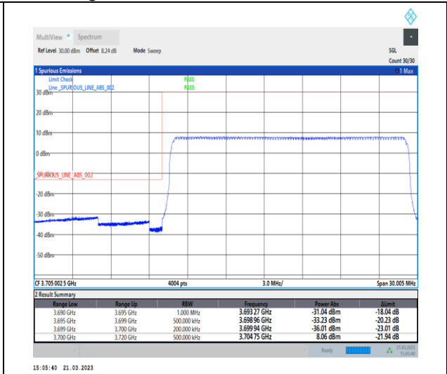
1-N77-3700-3980-30-20-L-6-CP-QPSK-Outer_Full -51@0-Ant0-1--PASS-see graph
