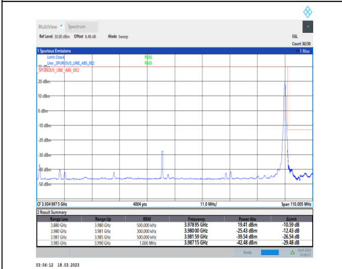
1-N77-3700-3980-30-100-H-5-CP-QPSK-Edge_1RB_Right-1@272-Ant0-1--PASS-see graph
