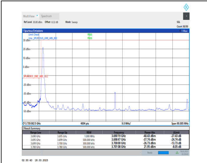
1-N77-3700-3980-30-80-L-1-DFT-PI2BPSK-Edge_1RB _Left-1@0-Ant0-1--PASS-see graph
