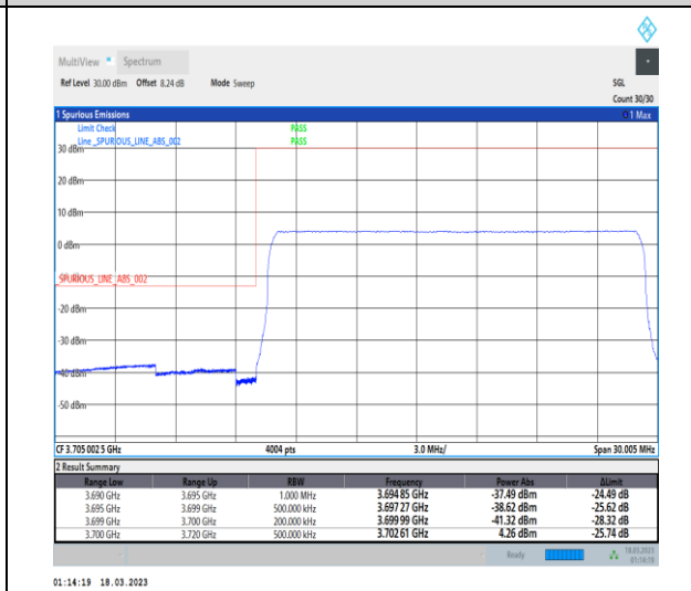
1-N77-3700-3980-30-20-L-6-CP-QPSK-Outer_Full -51@0-Ant0-1--PASS-see graph
