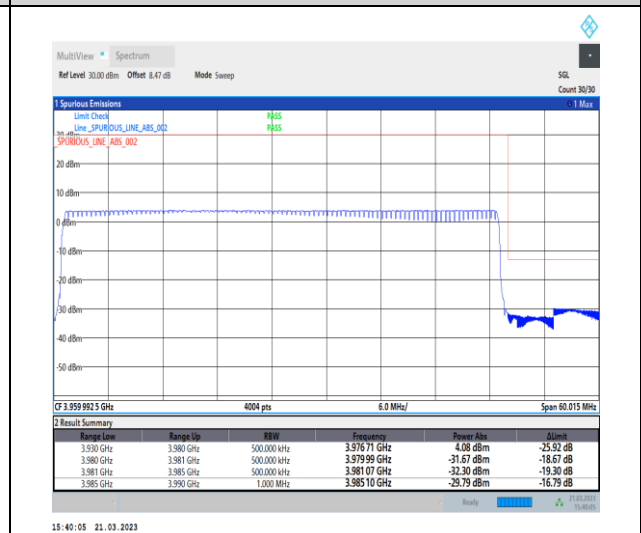
1-N77-3700-3980-30-50-H-6-CP-QPSK-Outer_Full -133@0-Ant0-1--PASS-see graph
