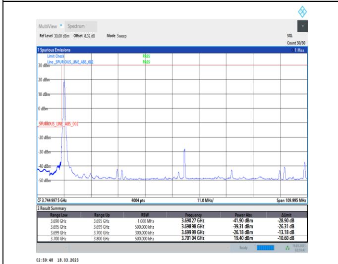
1-N77-3700-3980-30-100-L-4-CP-QPSK-Edge_1RB_Left-1@0-Ant0-1--PASS-see graph
