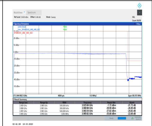
1-N77-3700-3980-30-80-H-6-CP-QPSK-Outer_Full-217@0-Ant0-1--PASS-see graph
