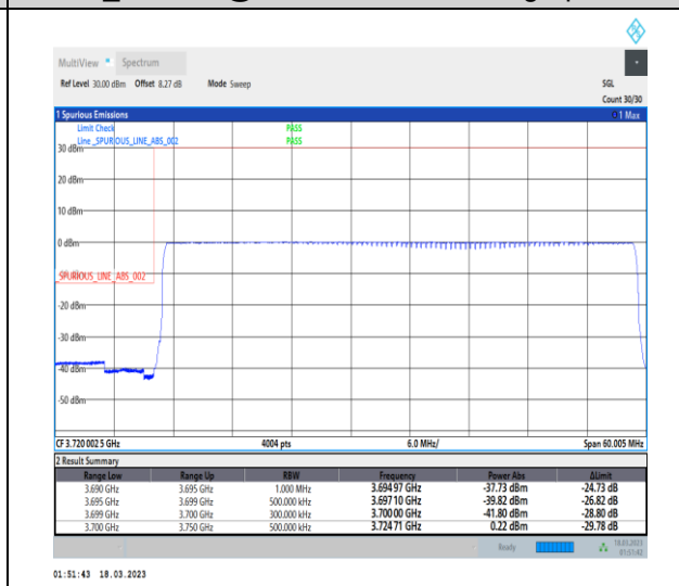
1-N77-3700-3980-30-50-L-6-CP-QPSK-Outer_Full -133@0-Ant0-1--PASS-see graph
