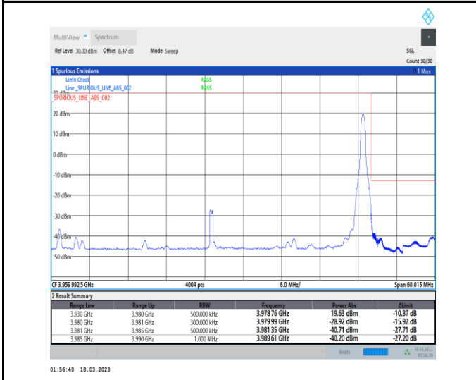
1-N77-3700-3980-30-50-H-5-CP-QPSK-Edge_1RB_Right-1@132-Ant0-1--PASS-see graph
