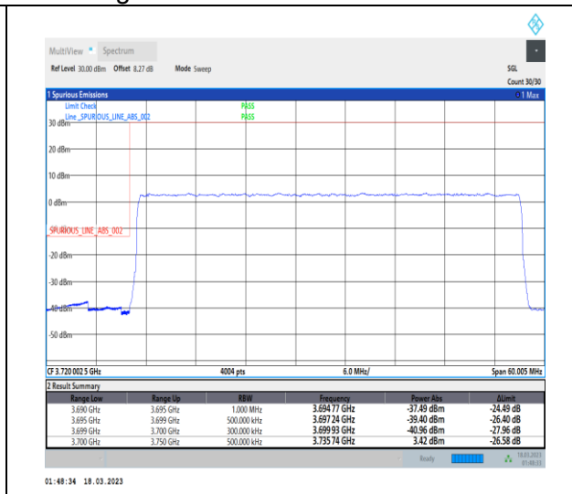
1-N77-3700-3980-30-50-L-3-DFT-PI2BPSK-Outer_Full-128@0-Ant0-1--PASS-see graph
