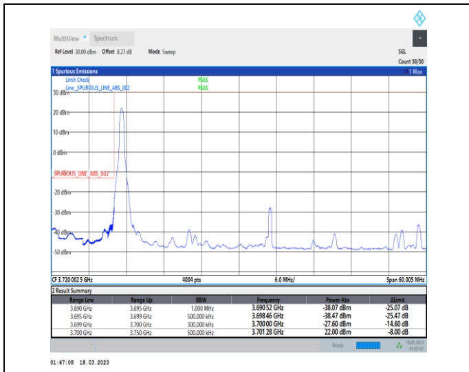
1-N77-3700-3980-30-50-L-1-DFT-PI2BPSK-Edge_1RB_Left-1@0-Ant0-1--PASS-see graph
