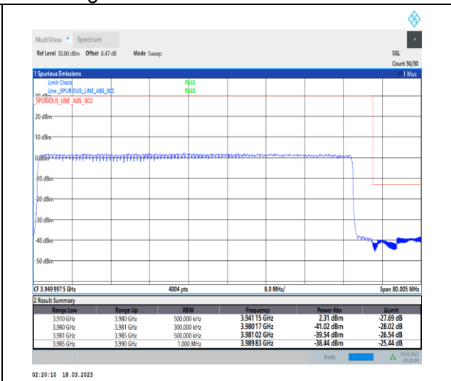
1-N77-3700-3980-30-70-H-3-DFT-PI2BPSK-Outer_Full-180@0-Ant0-1--PASS-see graph
