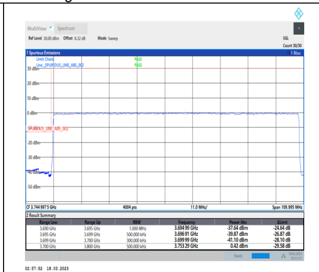
1-N77-3700-3980-30-100-L-3-DFT-PI2BPSK-Outer_Full-270@0-Ant0-1--PASS-see graph
