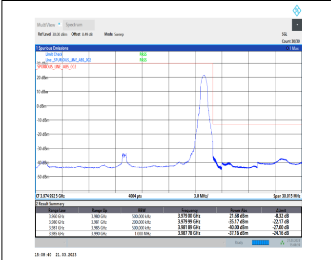
1-N77-3700-3980-30-20-H-5-CP-QPSK-Edge_1RB_Ri ght-1@50-Ant0-1--PASS-see graph
