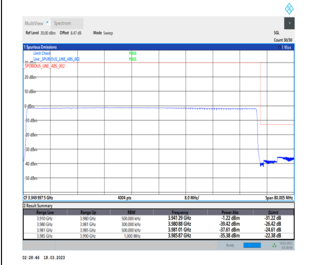
1-N77-3700-3980-30-70-H-6-CP-QPSK-Outer_Full-189@0-Ant0-1--PASS-see graph
