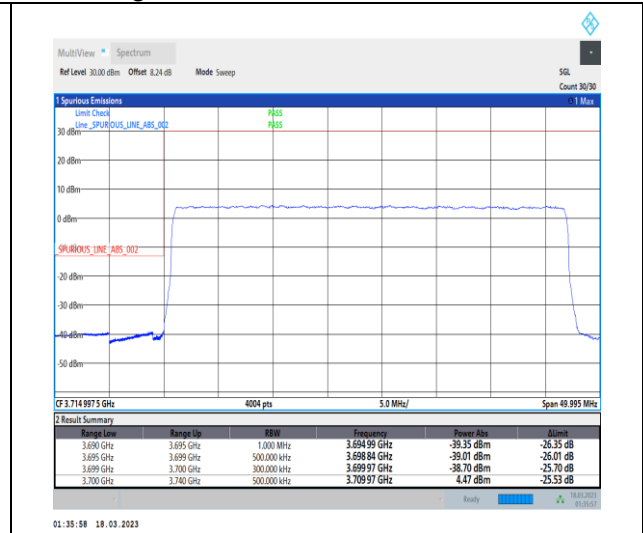
1-N77-3700-3980-30-40-L-3-DFT-PI2BPSK-Outer _Full-100@0-Ant0-1--PASS-see graph
