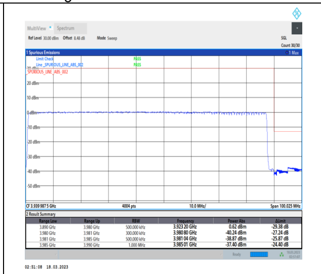
1-N77-3700-3980-30-90-H-3-DFT-PI2BPSK-Outer_Full-240@0-Ant0-1--PASS-see graph
