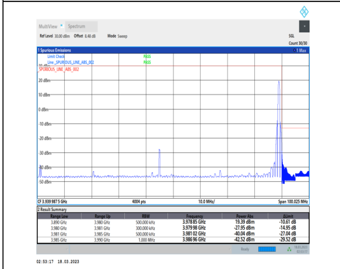
1-N77-3700-3980-30-90-H-5-CP-QPSK-Edge_1RB_Right-1@244-Ant0-1--PASS-see graph
