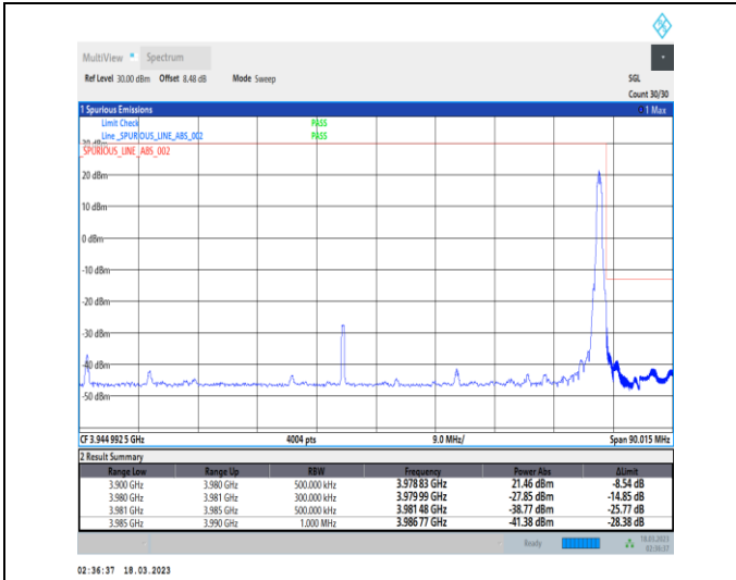
1-N77-3700-3980-30-80-H-2-DFT-PI2BPSK-Edge_1R_B_Right-1@216-Ant0-1--PASS-see graph
