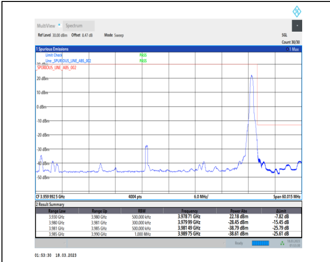
1-N77-3700-3980-30-50-H-2-DFT-PI2BPSK-Edge_1R_B_Right-1@132-Ant0-1--PASS-see graph
