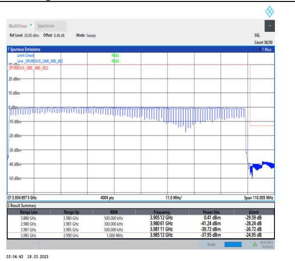
1-N77-3700-3980-30-100-H-3-DFT-PI2BPSK-Outer_Full-270@0-Ant0-1--PASS-see graph
