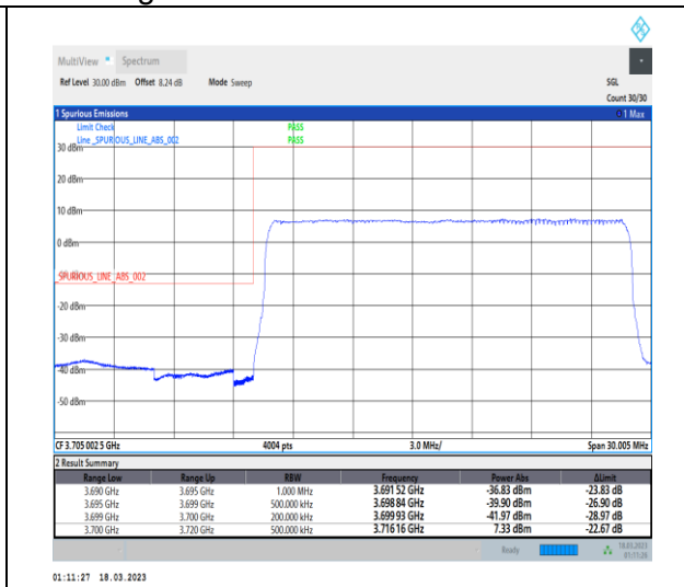
1-N77-3700-3980-30-20-L-3-DFT-PI2BPSK-Outer _Full-50@0-Ant0-1--PASS-see graph
