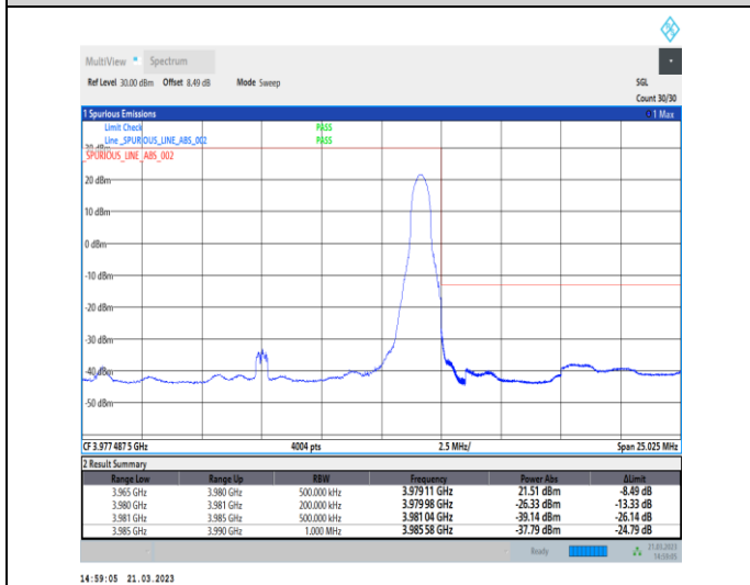
1-N77-3700-3980-30-15-H-5-CP-QPSK-Edge_1RB_Ri ght-1@37-Ant0-1--PASS-see graph
