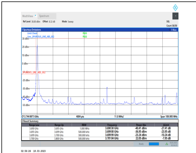
1-N77-3700-3980-30-100-L-1-DFT-PI2BPSK-Edge_1R_B_Left-1@0-Ant0-1--PASS-see graph
