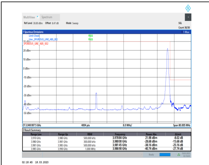
1-N77-3700-3980-30-70-H-2-DFT-PI2BPSK-Edge_1R_B_Right-1@188-Ant0-1--PASS-see graph
