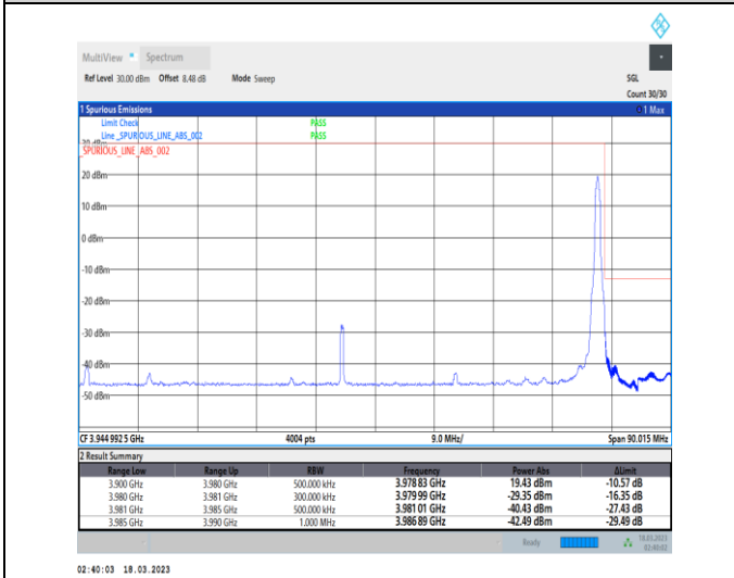
1-N77-3700-3980-30-80-H-5-CP-QPSK-Edge_1RB_Right-1@216-Ant0-1--PASS-see graph
