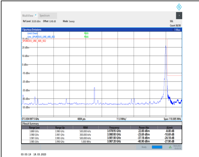
1-N77-3700-3980-30-100-H-2-DFT-PI2BPSK-Edge_1R_B_Right-1@272-Ant0-1--PASS-see graph
