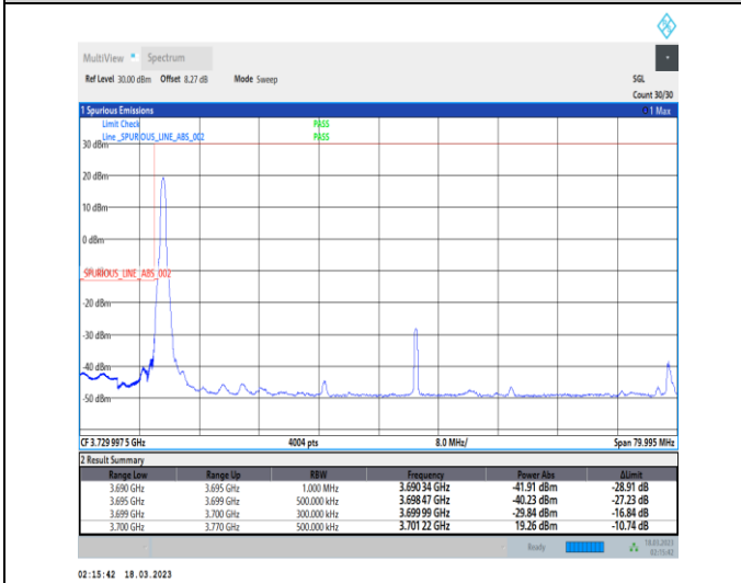
1-N77-3700-3980-30-70-L-4-CP-QPSK-Edge_1RB_Lef t-1@0-Ant0-1--PASS-see graph
