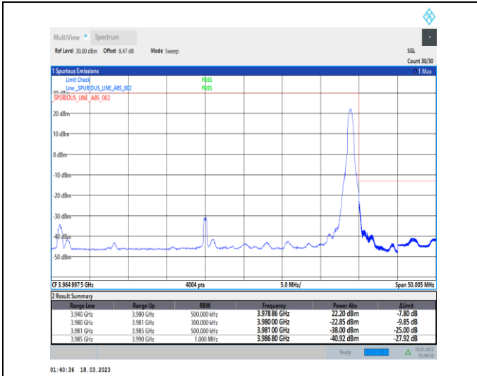
1-N77-3700-3980-30-40-H-2-DFT-PI2BPSK-Edge_1R_B_Right-1@105-Ant0-1--PASS-see graph
