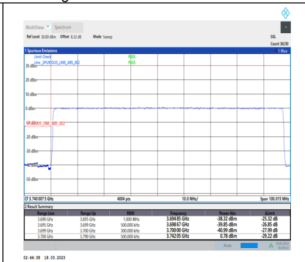
1-N77-3700-3980-30-90-L-3-DFT-PI2BPSK-Outer_Full-240@0-Ant0-1--PASS-see graph
