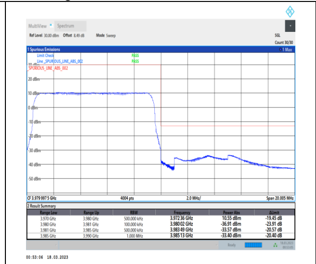
1-N77-3700-3980-30-10-H-3-DFT-PI2BPSK-Outer_Full-24@0-Ant0-1--PASS-see graph
