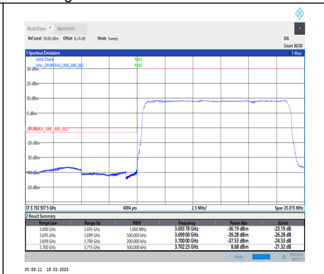
1-N77-3700-3980-30-15-L-3-DFT-PI2BPSK-Outer_Full-36@0-Ant0-1--PASS-see graph
