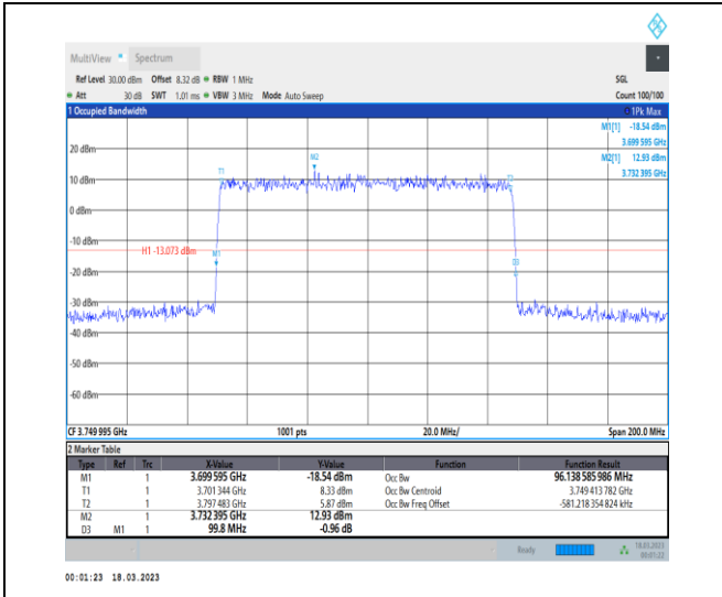
1-N77-3700-3980-30-100-L-1-DFT-QPSK-Outer_Full -270@0-Ant0-96.139-99.800-≤100-PASS
