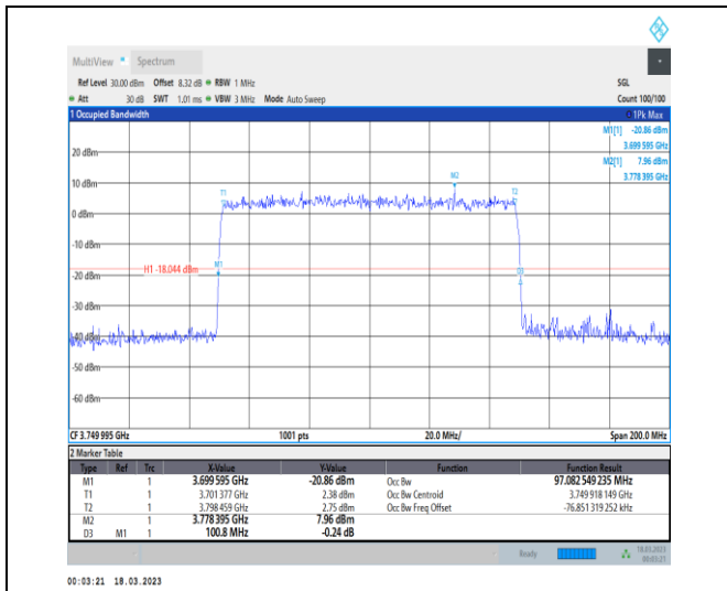
1-N77-3700-3980-30-100-L-9-CP-256QAM-Outer_F ull-273@0-Ant0-97.083-100.800-≤100-PASS
