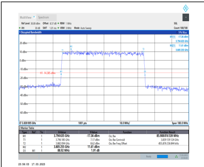
1-N77-3700-3980-30-90-M-3-DFT-16QAM-Outer_Ful I-240@0-Ant0-85.909-88.920-≤90-PASS
