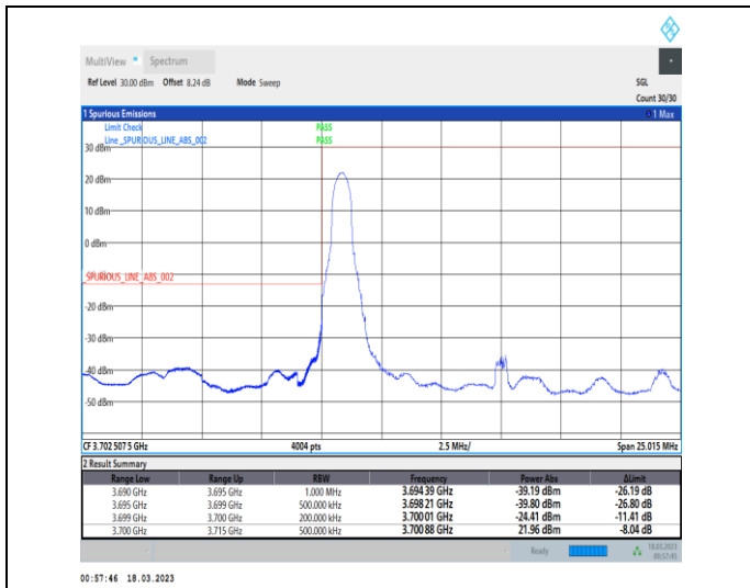
1-N77-3700-3980-30-15-L-1-DFT-PI2BPSK-Edge_1RB_Left-1@0-Ant0-1--PASS-see graph
