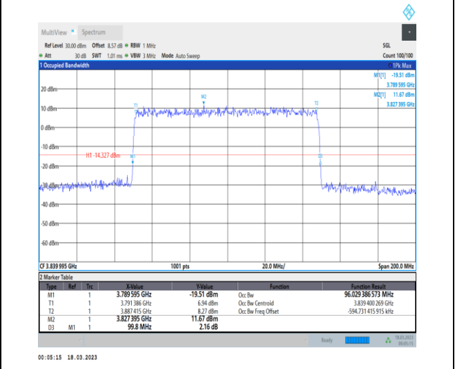
1-N77-3700-3980-30-100-M-3-DFT-16QAM-Outer_F ull-270@0-Ant0-96.029-99.800-≤100-PASS
