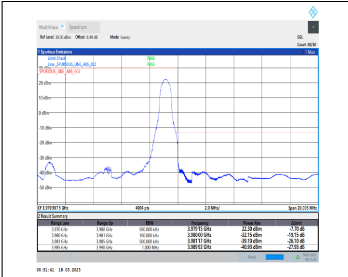
1-N77-3700-3980-30-10-H-2-DFT-PI2BPSK-Edge_1R_B_Right-1@23-Ant0-1--PASS-see graph
