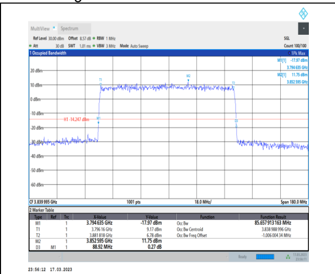
1-N77-3700-3980-30-90-M-4-DFT-64QAM-Outer_Ful I-240@0-Ant0-85.658-88.920-≤90-PASS
