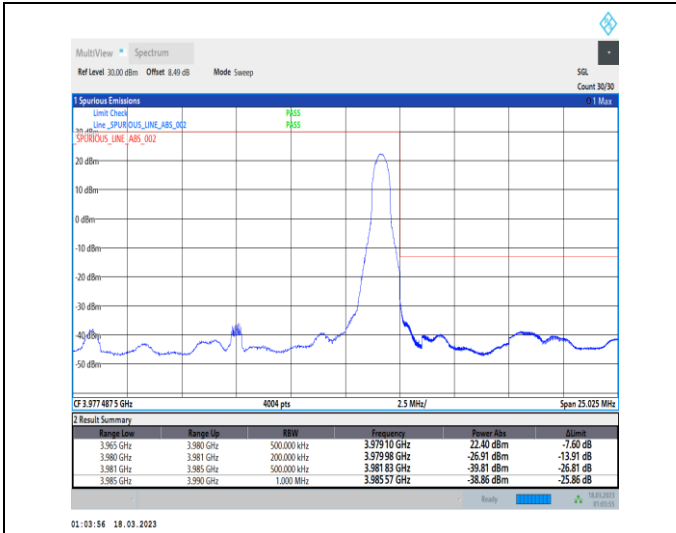
1-N77-3700-3980-30-15-H-2-DFT-PI2BPSK-Edge_1R_B_Right-1@37-Ant0-1--PASS-see graph
