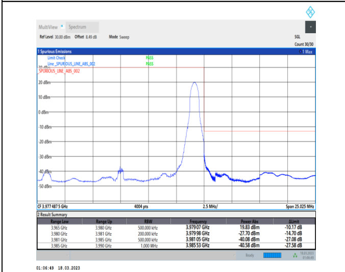
1-N77-3700-3980-30-15-H-5-CP-QPSK-Edge_1RB_Right-1@37-Ant0-1--PASS-see graph
