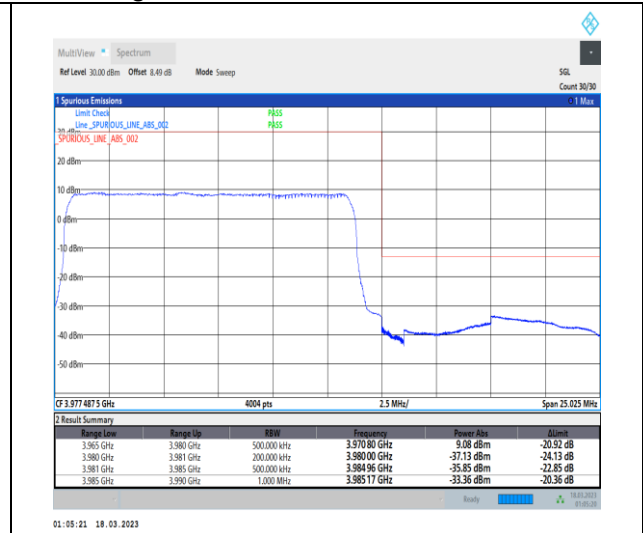
1-N77-3700-3980-30-15-H-3-DFT-PI2BPSK-Outer_Full-36@0-Ant0-1--PASS-see graph
