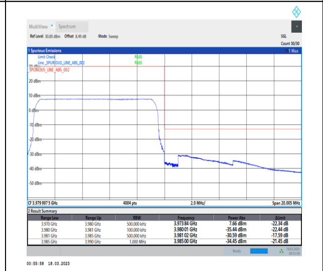
1-N77-3700-3980-30-10-H-6-CP-QPSK-Outer_Full-24@0-Ant0-1--PASS-see graph
