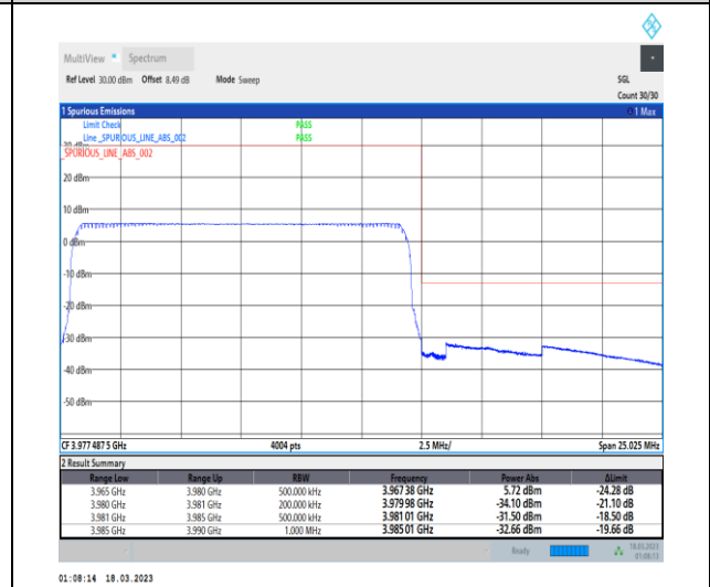
1-N77-3700-3980-30-15-H-6-CP-QPSK-Outer_Full-38@0-Ant0-1--PASS-see graph
