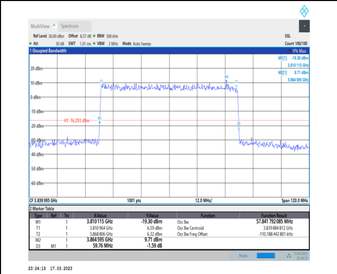
1-N77-3700-3980-30-60-M-3-DFT-16QAM-Outer_Full -162@0-Ant0-57.842-59.760-≤60-PASS
