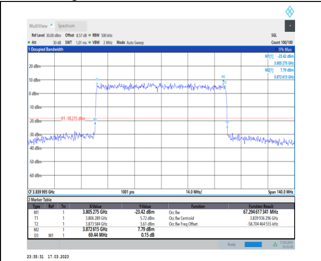
1-N77-3700-3980-30-70-M-6-CP-QPSK-Outer_Full-189@0-Ant0-67.295-69.440-≤70-PASS
