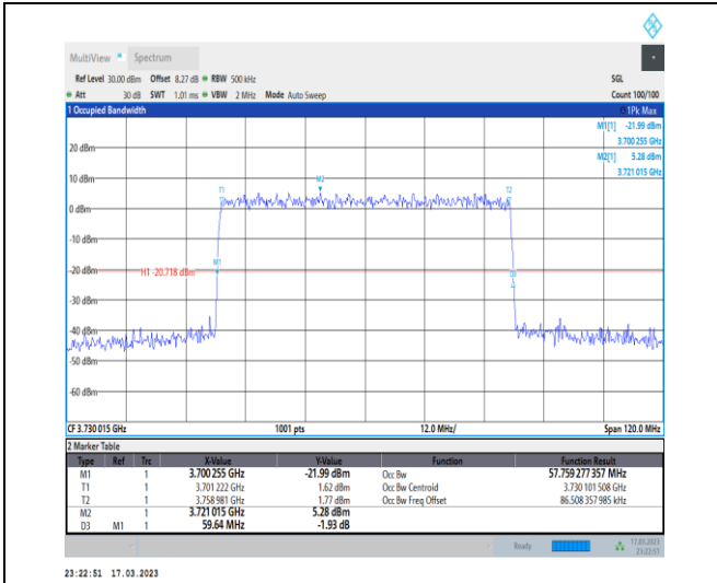
1-N77-3700-3980-30-60-L-9-CP-256QAM-Outer_Full -162@0-Ant0-57.759-59.640-≤60-PASS
