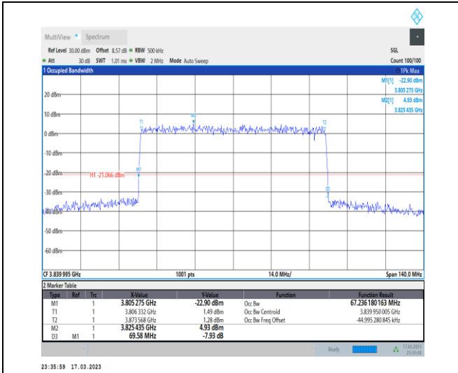
1-N77-3700-3980-30-70-M-9-CP-256QAM-Outer_Ful I-189@0-Ant0-67.236-69.580-≤70-PASS
