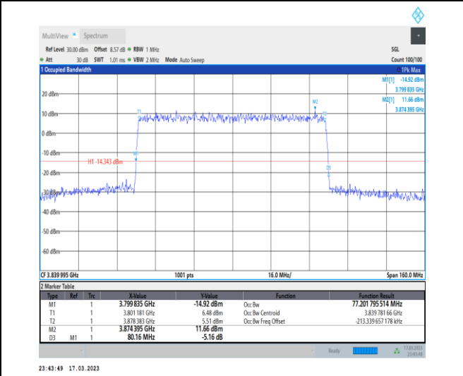
1-N77-3700-3980-30-80-M-1-DFT-QPSK-Outer_Full-216@0-Ant0-77.202-80.160-<math>\leq 80</math>-PASS
