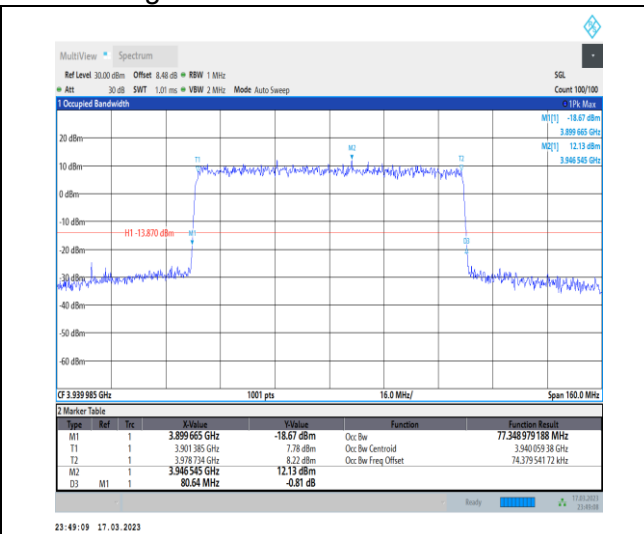
1-N77-3700-3980-30-80-H-6-CP-QPSK-Outer_Full-217@0-Ant0-77.349-80.640-≤80-PASS
