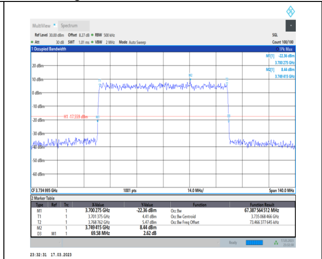
1-N77-3700-3980-30-70-L-7-CP-16QAM-Outer_Full-189@0-Ant0-67.388-69.580-≤70-PASS
