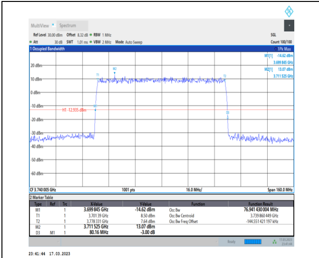
1-N77-3700-3980-30-80-L-3-DFT-16QAM-Outer_Full -216@0-Ant0-76.941-80.160-≤80-PASS
