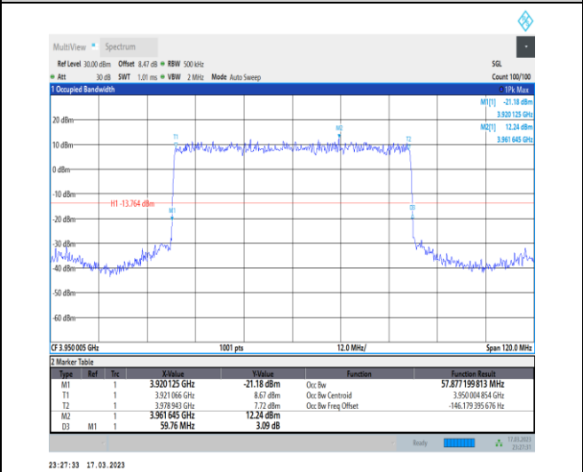
1-N77-3700-3980-30-60-H-2-DFT-PI2BPSK-Outer_Full-162@0-Ant0-57.877-59.760-≤60-PASS
