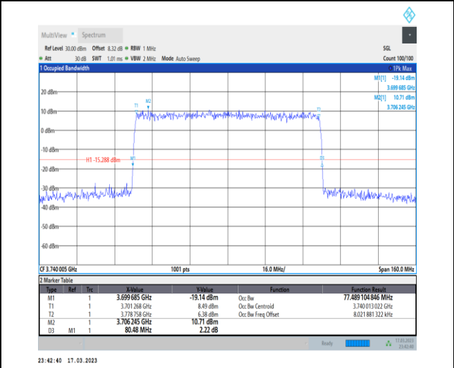
1-N77-3700-3980-30-80-L-6-CP-QPSK-Outer_Full-2 17@0-Ant0-77.489-80.480-≤80-PASS
