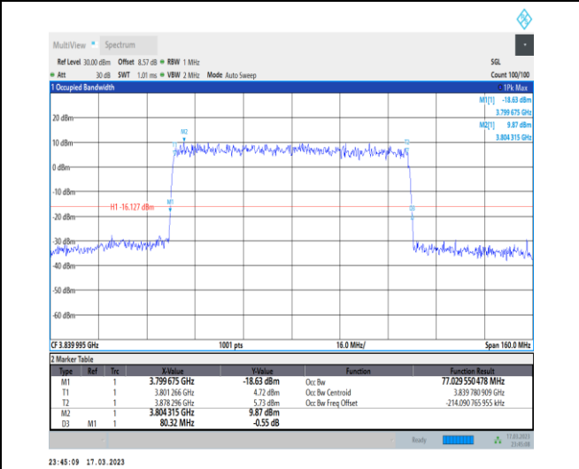
1-N77-3700-3980-30-80-M-5-DFT-256QAM-Outer_Full-216@0-Ant0-77.03-80.320-<math>\leq 80</math>-PASS
