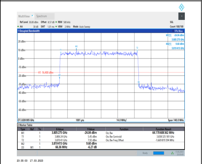
1-N77-3700-3980-30-70-M-4-DFT-64QAM-Outer_Full-180@0-Ant0-64.171-66.360-≤70-PASS
