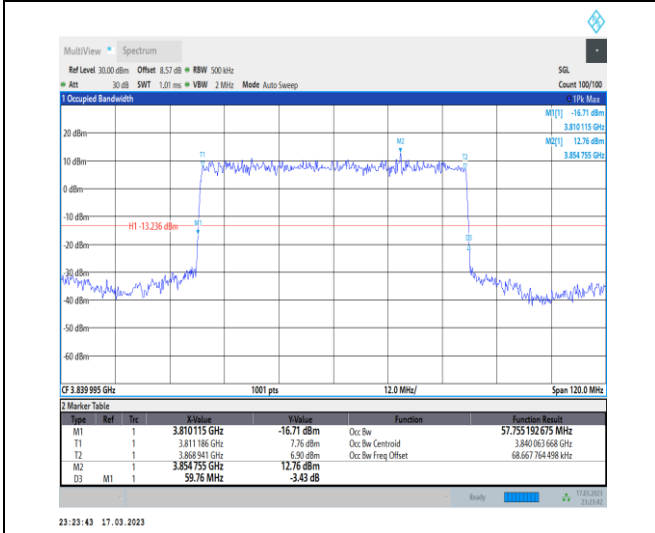
1-N77-3700-3980-30-60-M-2-DFT-PI2BPSK-Outer_Full -162@0-Ant0-57.755-59.760-≤60-PASS
