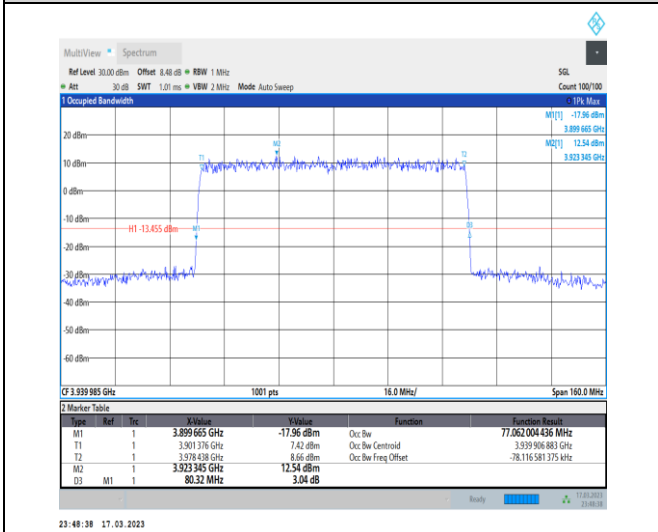
1-N77-3700-3980-30-80-H-3-DFT-16QAM-Outer_Full-216@0-Ant0-77.062-80.320-≤80-PASS
