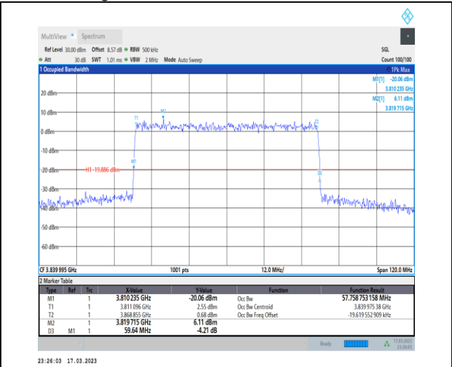
1-N77-3700-3980-30-60-M-9-CP-256QAM-Outer_FuII-162@0-Ant0-57.759-59.640-≤60-PASS
