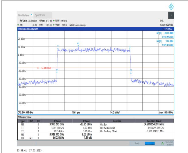
1-N77-3700-3980-30-70-H-4-DFT-64QAM-Outer_Full-180@0-Ant0-64.21-66.220-≤70-PASS
