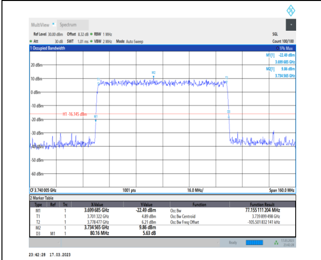
1-N77-3700-3980-30-80-L-5-DFT-256QAM-Outer_Fu ll-216@0-Ant0-77.155-80.160-≤80-PASS
