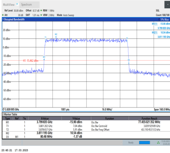
1-N77-3700-3980-30-80-M-6-CP-QPSK-Outer_Full-2 17@0-Ant0-77.455-80.480-≤80-PASS
