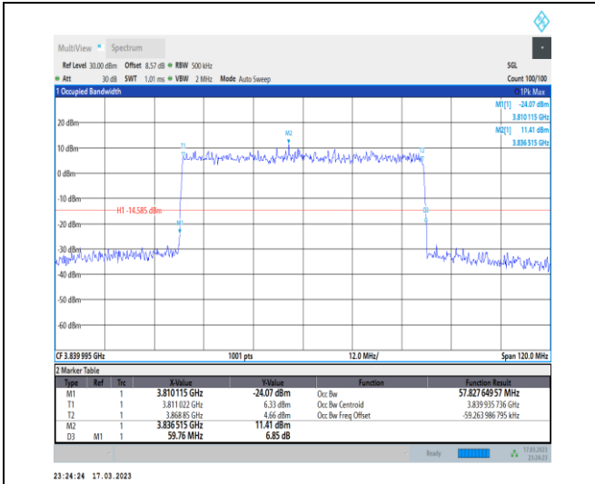
1-N77-3700-3980-30-60-M-4-DFT-64QAM-Outer_Full-162@0-Ant0-57.828-59.760-≤60-PASS
