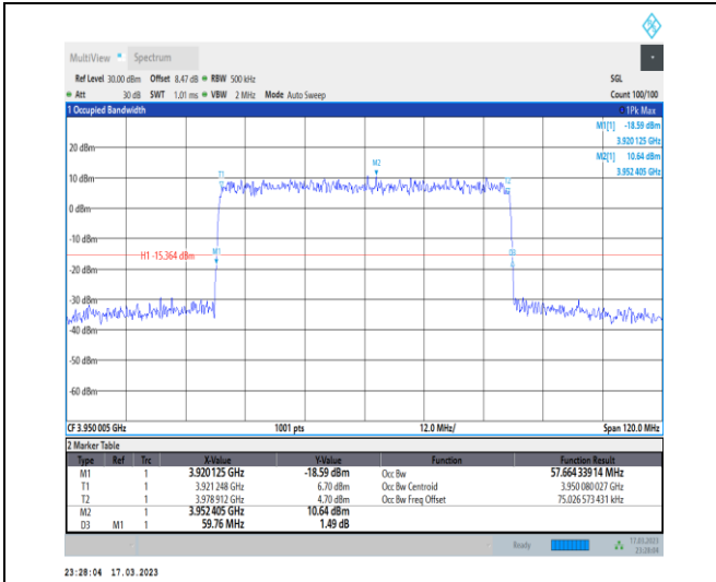
1-N77-3700-3980-30-60-H-3-DFT-16QAM-Outer_Ful I-162@0-Ant0-57.664-59.760-≤60-PASS
