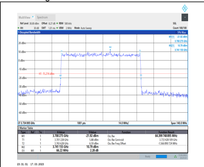
1-N77-3700-3980-30-70-L-3-DFT-16QAM-Outer_Full-180@0-Ant0-64.4-66.220-≤70-PASS
