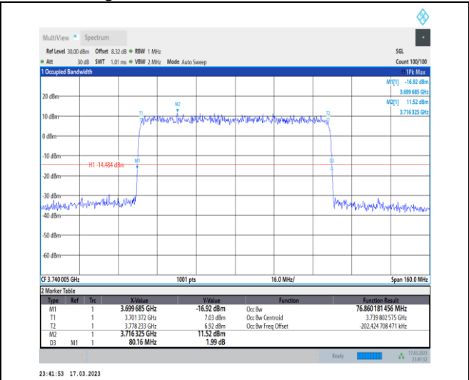
1-N77-3700-3980-30-80-L-4-DFT-64QAM-Outer_Full -216@0-Ant0-76.86-80.160-≤80-PASS
