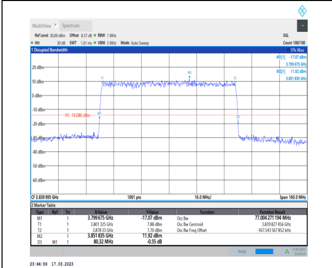
1-N77-3700-3980-30-80-M-4-DFT-64QAM-Outer_Full-216@0-Ant0-77.004-80.320-<math>\leq 80</math>-PASS
