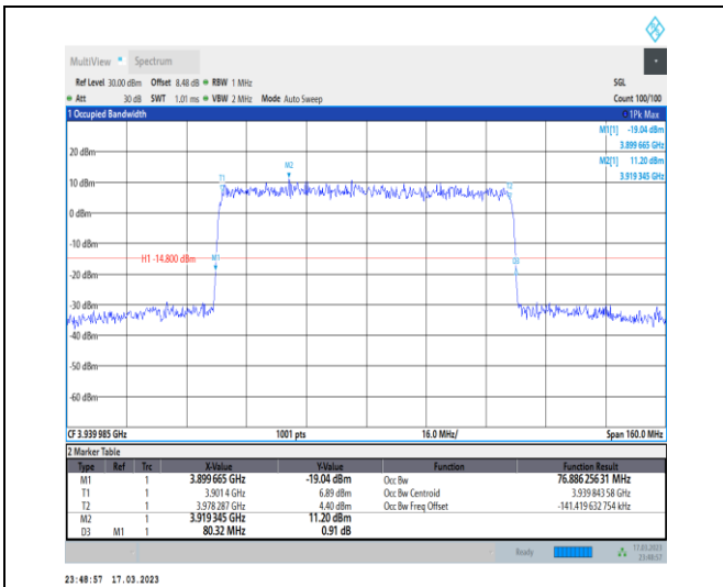
1-N77-3700-3980-30-80-H-5-DFT-256QAM-Outer_Full-216@0-Ant0-76.886-80.320-≤80-PASS
