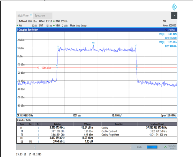
1-N77-3700-3980-30-60-M-1-DFT-QPSK-Outer_Full -162@0-Ant0-57.886-59.640-≤60-PASS
