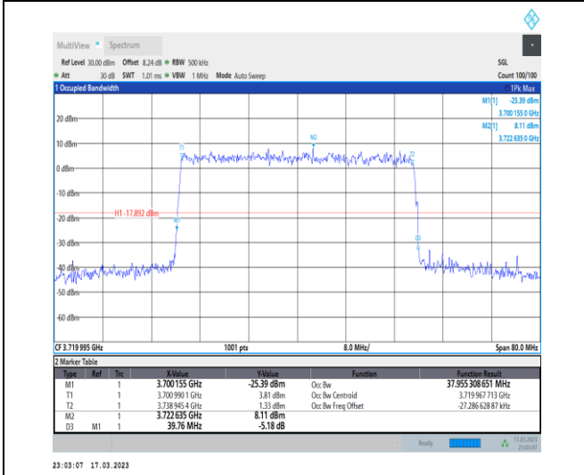
1-N77-3700-3980-30-40-L-9-CP-256QAM-Outer_Full-106@0-Ant0-37.955-39.760-≤40-PASS
