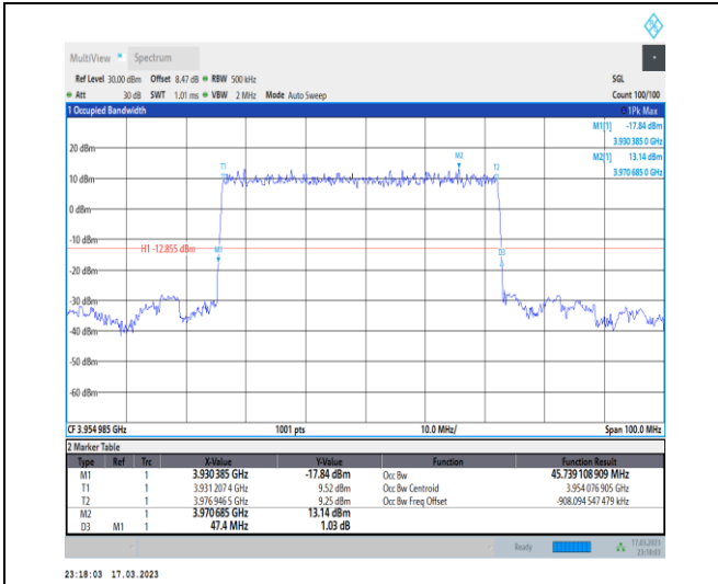
1-N77-3700-3980-30-50-H-2-DFT-PI2BPSK-Outer_Full-128@0-Ant0-45.739-47.400-≤50-PASS
