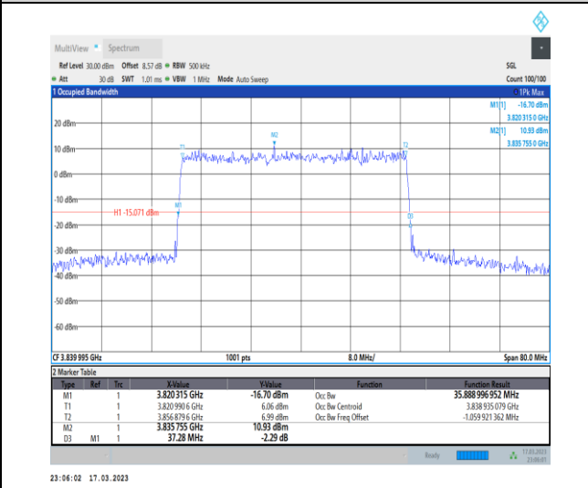
1-N77-3700-3980-30-40-M-5-DFT-256QAM-Outer_Full-100@0-Ant0-35.889-37.280-≤40-PASS
