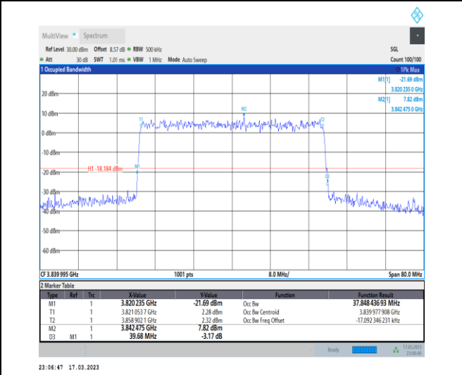
1-N77-3700-3980-30-40-M-9-CP-256QAM-Outer_Full-106@0-Ant0-37.848-39.680-≤40-PASS
