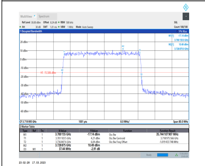
1-N77-3700-3980-30-40-L-5-DFT-256QAM-Outer_Fu II-100@0-Ant0-35.744-37.440-≤40-PASS
