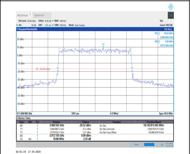
1-N77-3700-3980-30-20-H-8-CP-64QAM-Outer_Full-51@0-Ant0-18.143-18.880-≤20-PASS
