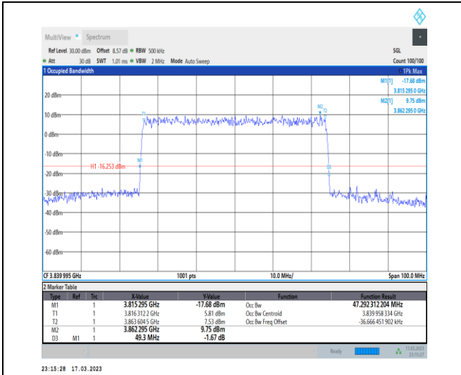
1-N77-3700-3980-30-50-M-7-CP-16QAM-Outer_Full-133@0-Ant0-47.292-49.300-≤50-PASS
