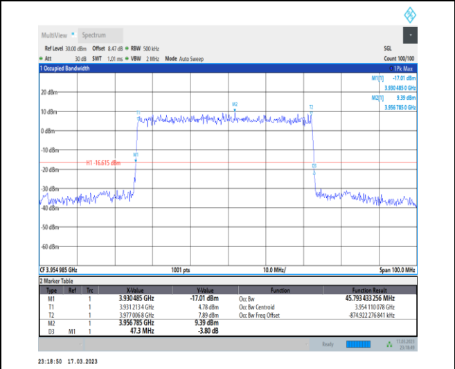
1-N77-3700-3980-30-50-H-5-DFT-256QAM-Outer_Full-128@0-Ant0-45.793-47.300-≤50-PASS
