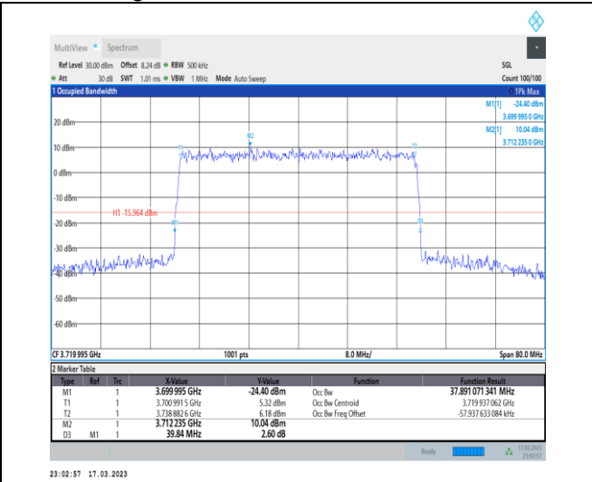
1-N77-3700-3980-30-40-L-8-CP-64QAM-Outer_Full-106@0-Ant0-37.891-39.840-≤40-PASS
