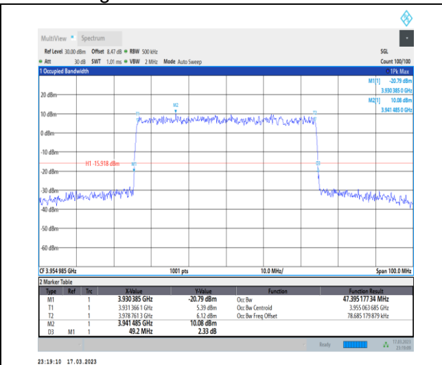
1-N77-3700-3980-30-50-H-7-CP-16QAM-Outer_Full-133@0-Ant0-47.395-49.200-≤50-PASS
