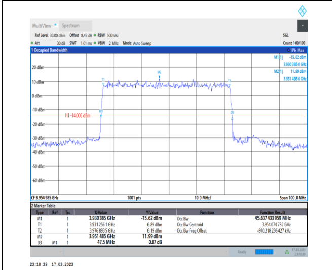
1-N77-3700-3980-30-50-H-4-DFT-64QAM-Outer_Full-128@0-Ant0-45.637-47.500-≤50-PASS
