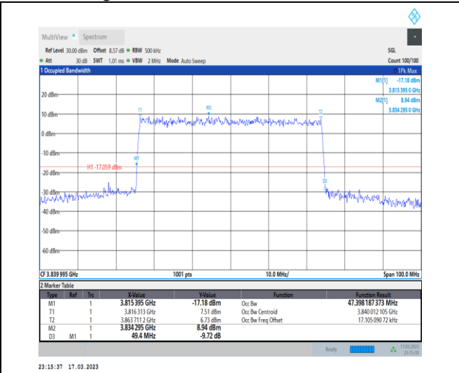
1-N77-3700-3980-30-50-M-8-CP-64QAM-Outer_Full-133@0-Ant0-47.398-49.400-≤50-PASS
