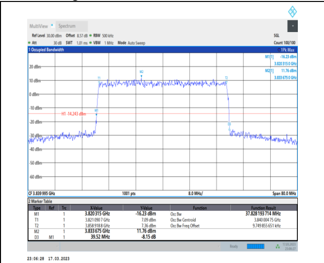
1-N77-3700-3980-30-40-M-7-CP-16QAM-Outer_Full-106@0-Ant0-37.828-39.520-≤40-PASS
