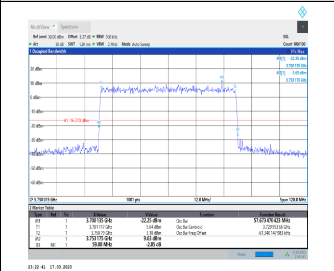
1-N77-3700-3980-30-60-L-8-CP-64QAM-Outer_Full-162@0-Ant0-57.673-59.880-≤60-PASS
