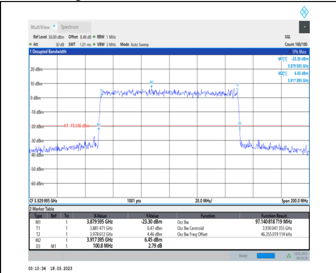
1-N77-3700-3980-30-100-H-9-CP-256QAM-Outer_Full-273@0-Ant0-97.141-100.800-≤100-PASS
