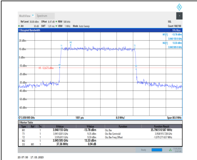
1-N77-3700-3980-30-40-H-1-DFT-QPSK-Outer_Full-100@0-Ant0-35.791-37.360-≤40-PASS
