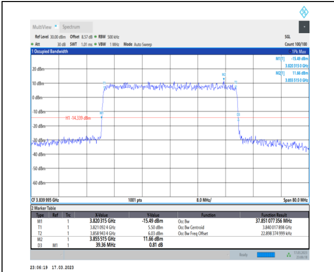
1-N77-3700-3980-30-40-M-6-CP-QPSK-Outer_Full-106@0-Ant0-37.851-39.360-≤40-PASS
