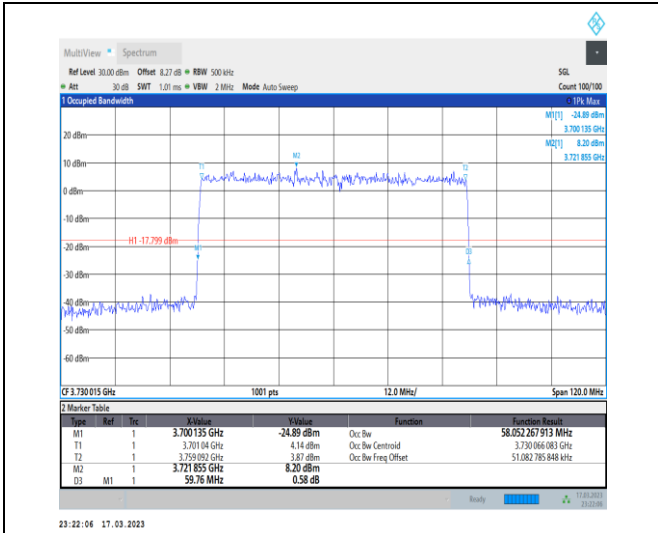
1-N77-3700-3980-30-60-L-5-DFT-256QAM-Outer_Fu II-162@0-Ant0-58.052-59.760-≤60-PASS
