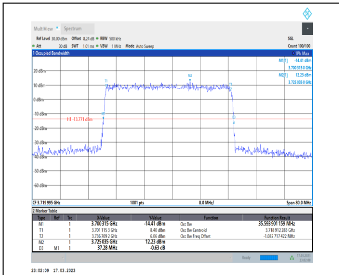
1-N77-3700-3980-30-40-L-3-DFT-16QAM-Outer_Full -100@0-Ant0-35.594-37.280-≤40-PASS
