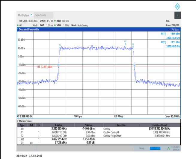
1-N77-3700-3980-30-40-M-1-DFT-QPSK-Outer_Full-100@0-Ant0-35.813-37.280-≤40-PASS
