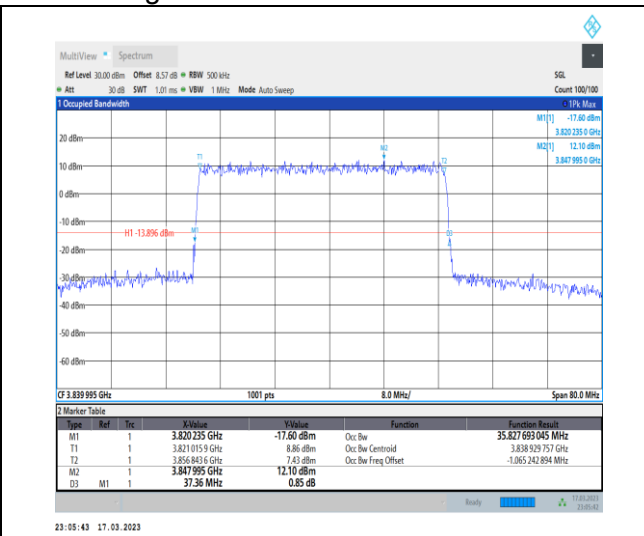
1-N77-3700-3980-30-40-M-3-DFT-16QAM-Outer_Full-100@0-Ant0-35.828-37.360-≤40-PASS
