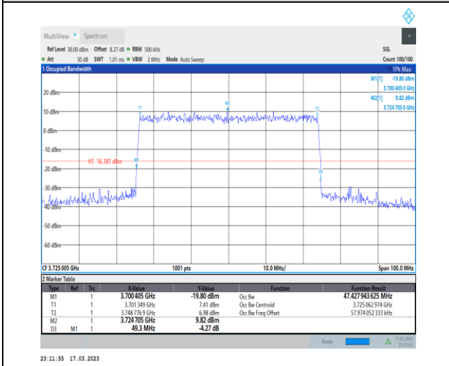
1-N77-3700-3980-30-50-L-6-CP-QPSK-Outer_Full-133@0-Ant0-47.428-49.300-≤50-PASS
