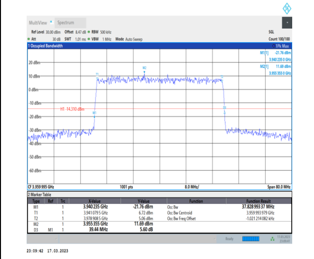
1-N77-3700-3980-30-40-H-8-CP-64QAM-Outer_Full-106@0-Ant0-37.829-39.440-≤40-PASS
