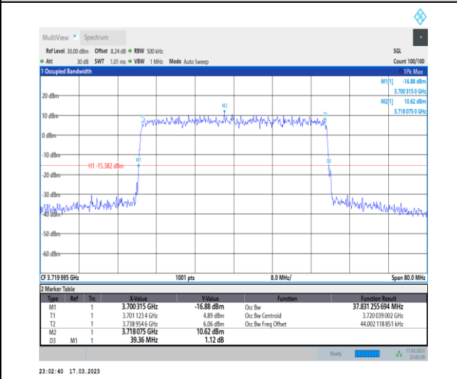
1-N77-3700-3980-30-40-L-6-CP-QPSK-Outer_Full-1 06@0-Ant0-37.831-39.360-≤40-PASS
