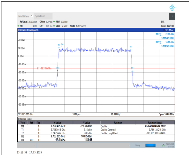
1-N77-3700-3980-30-50-L-4-DFT-64QAM-Outer_Full -128@0-Ant0-45.643-47.400-≤50-PASS
