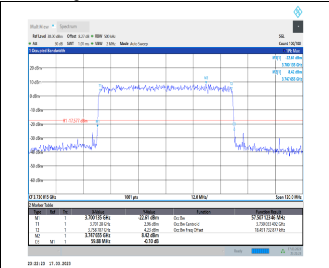
1-N77-3700-3980-30-60-L-6-CP-QPSK-Outer_Full-1 62@0-Ant0-57.507-59.880-≤60-PASS
