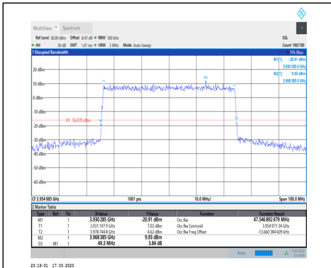
1-N77-3700-3980-30-50-H-6-CP-QPSK-Outer_Full-1 33@0-Ant0-47.547-49.300-≤50-PASS
