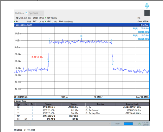
1-N77-3700-3980-30-50-H-3-DFT-16QAM-Outer_Full-128@0-Ant0-45.747-47.600-≤50-PASS
