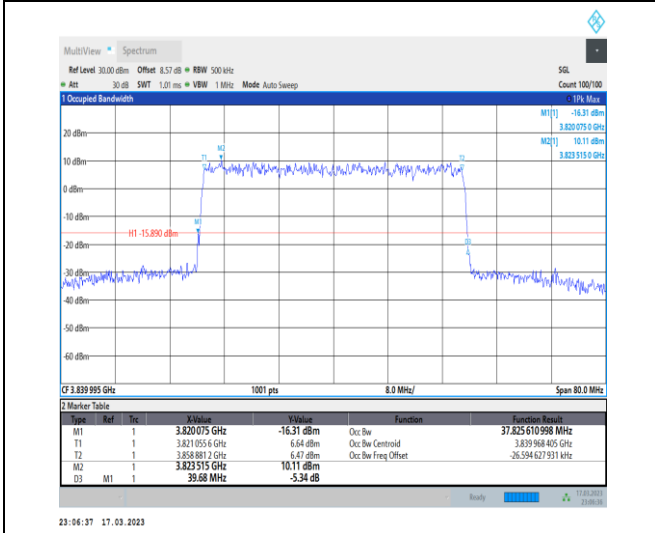
1-N77-3700-3980-30-40-M-8-CP-64QAM-Outer_Full-106@0-Ant0-37.826-39.680-≤40-PASS
