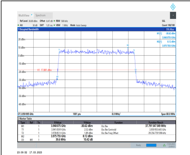
1-N77-3700-3980-30-40-H-9-CP-256QAM-Outer_Full-I-106@0-Ant0-37.792-39.600-≤40-PASS
