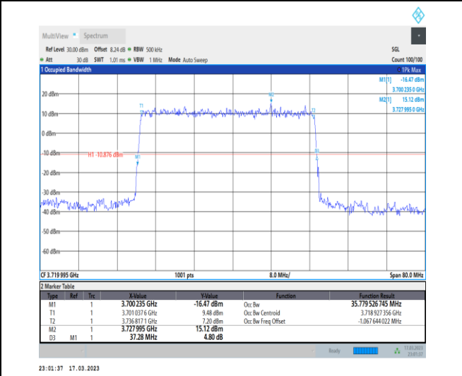
1-N77-3700-3980-30-40-L-2-DFT-PI2BPSK-Outer_Full-100@0-Ant0-35.78-37.280-≤40-PASS
