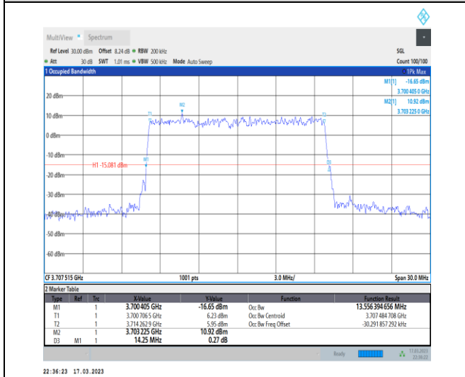
1-N77-3700-3980-30-15-L-8-CP-64QAM-Outer_Full-38@0-Ant0-13.556-14.250-≤15-PASS
