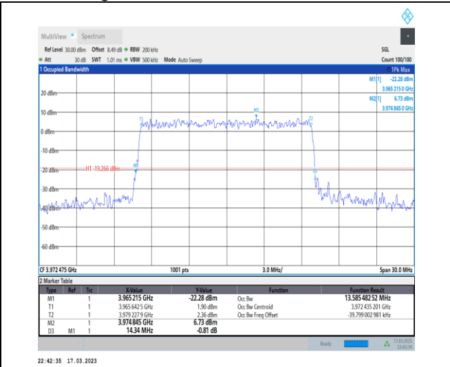
1-N77-3700-3980-30-15-H-9-CP-256QAM-Outer_Full-38@0-Ant0-13.585-14.340-≤15-PASS
