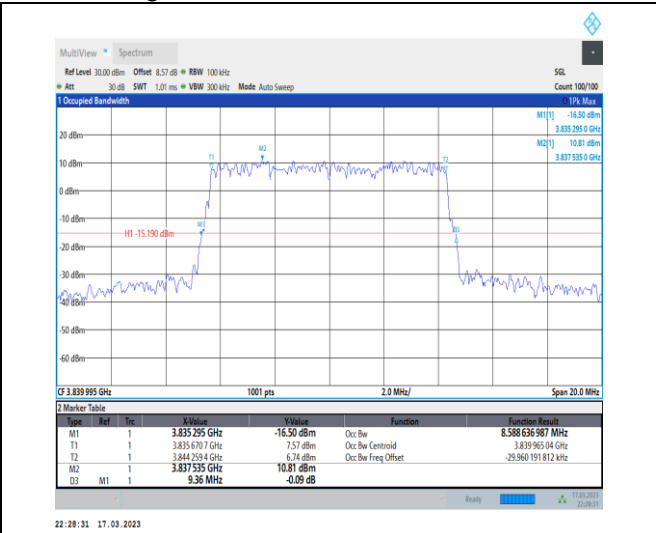
1-N77-3700-3980-30-10-M-1-DFT-QPSK-Outer_Full -24@0-Ant0-8.589-9.360-≤10-PASS
