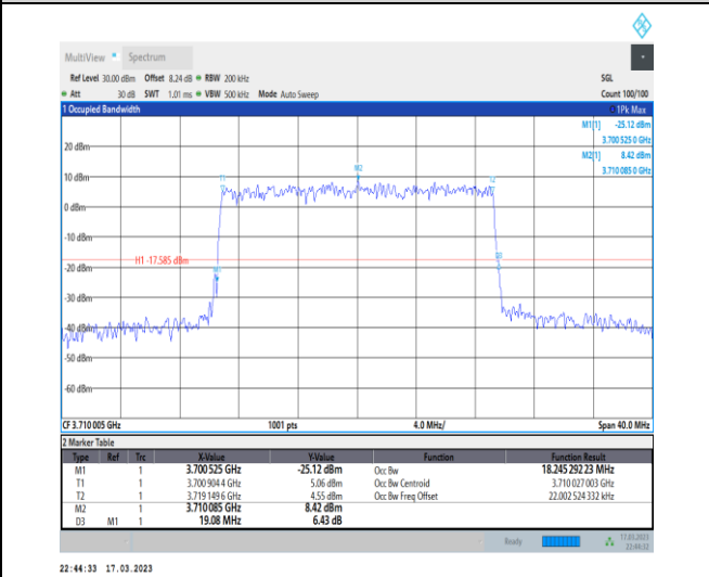
1-N77-3700-3980-30-20-L-6-CP-QPSK-Outer_Full-5 1@0-Ant0-18.245-19.080-≤20-PASS
