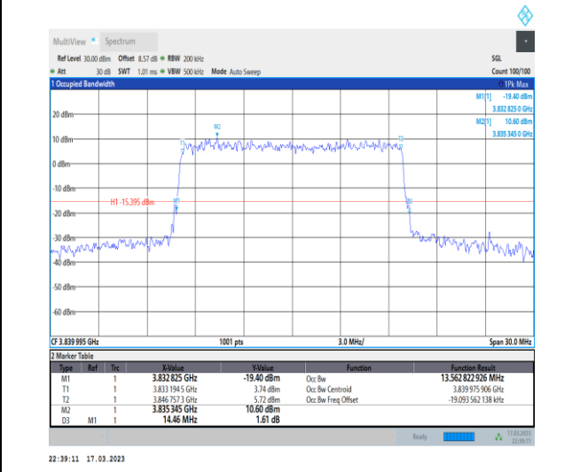
1-N77-3700-3980-30-15-M-8-CP-64QAM-Outer_Full-38@0-Ant0-13.563-14.460-≤15-PASS
