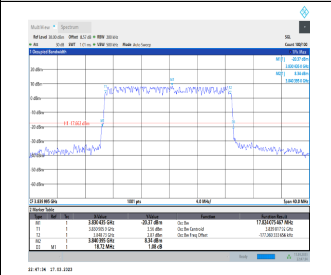
1-N77-3700-3980-30-20-M-5-DFT-256QAM-Outer_Full-50@0-Ant0-17.824-18.720-≤20-PASS
