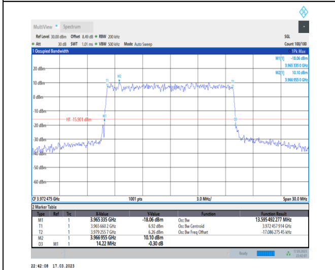
1-N77-3700-3980-30-15-H-6-CP-QPSK-Outer_Full-38@0-Ant0-13.595-14.220-≤15-PASS
