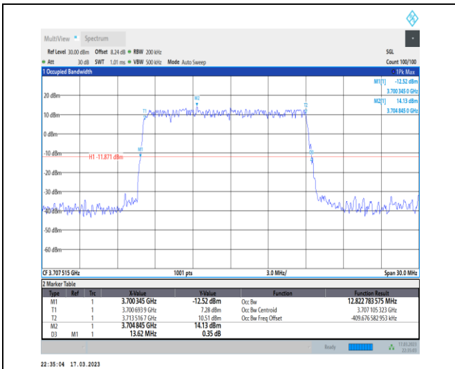
1-N77-3700-3980-30-15-L-2-DFT-PI2BPSK-Outer_Full-36@0-Ant0-12.823-13.620-≤15-PASS
