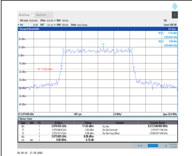
1-N77-3700-3980-30-10-H-5-DFT-256QAM-Outer_Full-24@0-Ant0-8.573-9.060-≤10-PASS
