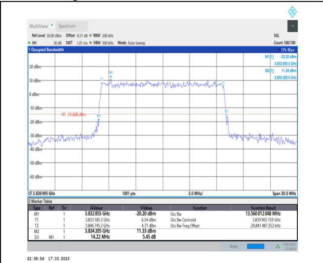
1-N77-3700-3980-30-15-M-6-CP-QPSK-Outer_Full-38@0-Ant0-13.56-14.220-≤15-PASS
