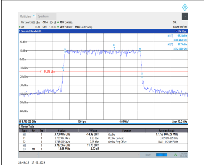
1-N77-3700-3980-30-20-L-1-DFT-QPSK-Outer_Full-50@0-Ant0-17.759-18.680-≤20-PASS
