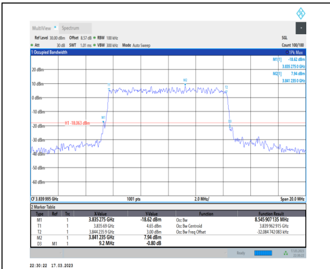
1-N77-3700-3980-30-10-M-8-CP-64QAM-Outer_Full-24@0-Ant0-8.546-9.200-≤10-PASS
