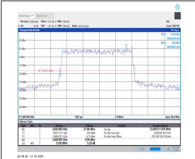
1-N77-3700-3980-30-15-M-5-DFT-256QAM-Outer_Full-36@0-Ant0-12.859-13.830-≤15-PASS
