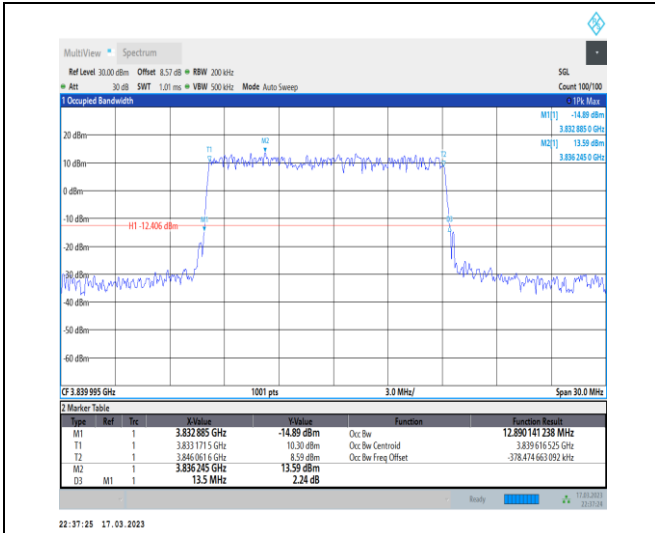
1-N77-3700-3980-30-15-M-1-DFT-QPSK-Outer_Full-36@0-Ant0-12.89-13.500-≤15-PASS
