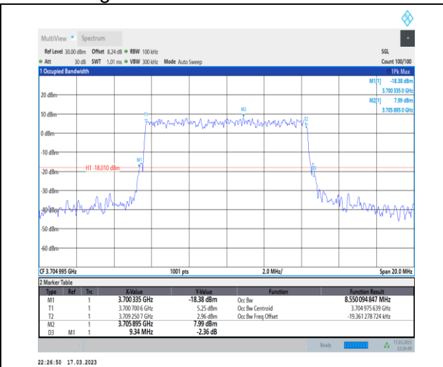
1-N77-3700-3980-30-10-L-6-CP-QPSK-Outer_Full-2 4@0-Ant0-8.55-9.340-≤10-PASS
