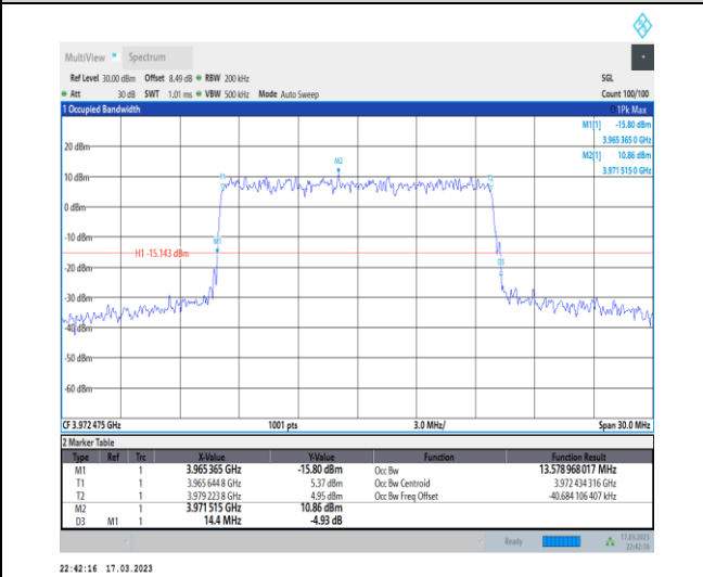
1-N77-3700-3980-30-15-H-7-CP-16QAM-Outer_Full-38@0-Ant0-13.579-14.400-≤15-PASS
