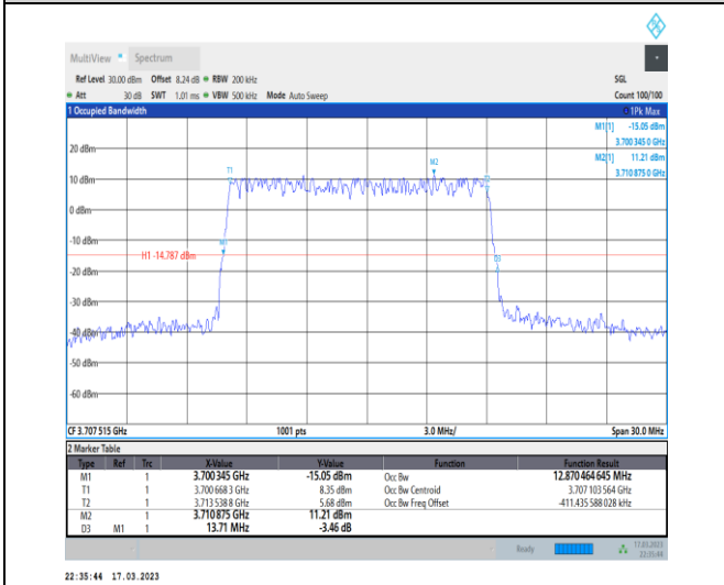
1-N77-3700-3980-30-15-L-4-DFT-64QAM-Outer_Full-36@0-Ant0-12.87-13.710-≤15-PASS
