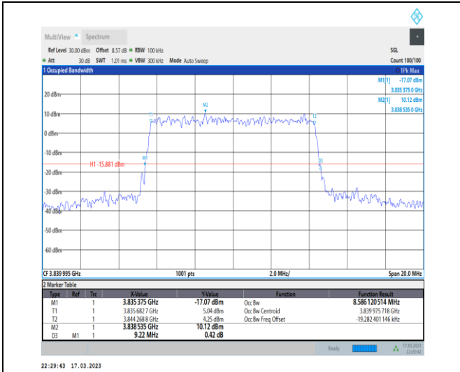
1-N77-3700-3980-30-10-M-4-DFT-64QAM-Outer_Ful I-24@0-Ant0-8.586-9.220-≤10-PASS
