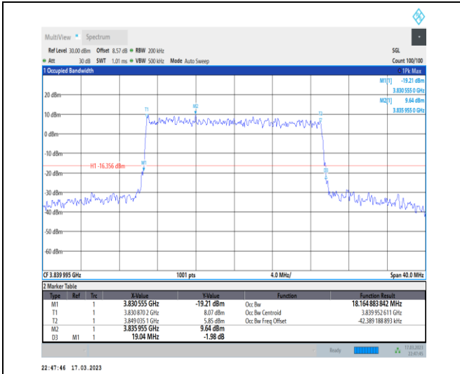
1-N77-3700-3980-30-20-M-6-CP-QPSK-Outer_Full-5 1@0-Ant0-18.165-19.040-≤20-PASS
