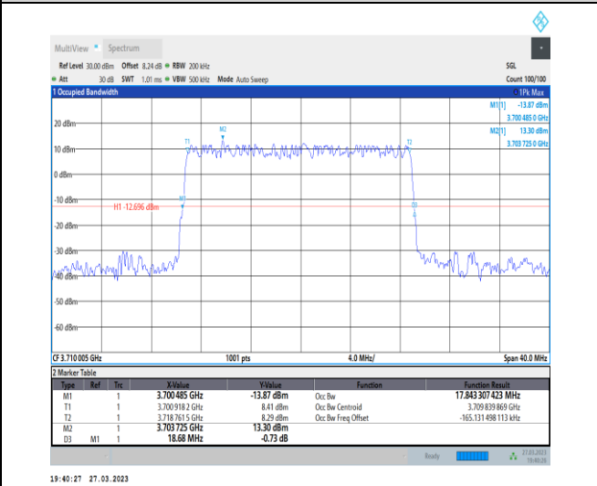
1-N77-3700-3980-30-20-L-2-DFT-PI2BPSK-Outer_Full-50@0-Ant0-17.843-18.680-≤20-PASS
