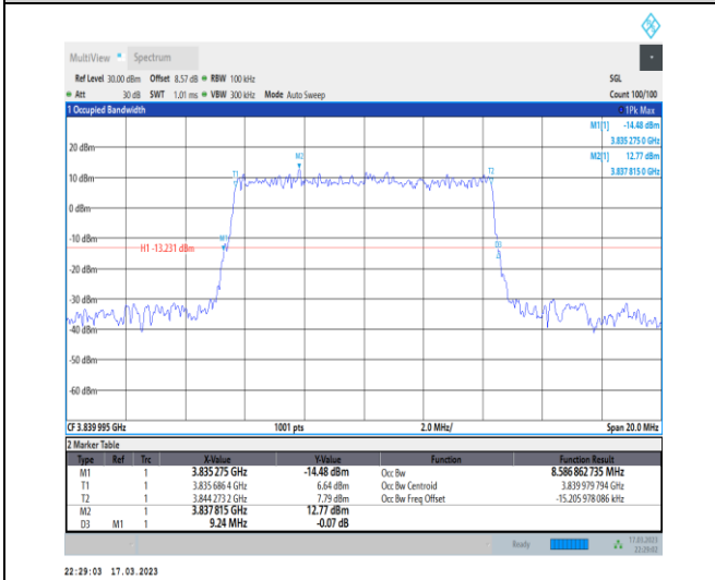
1-N77-3700-3980-30-10-M-2-DFT-PI2BPSK-Outer_F ull-24@0-Ant0-8.587-9.240-≤10-PASS
