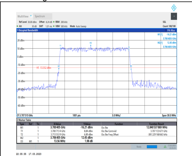
1-N77-3700-3980-30-15-L-3-DFT-16QAM-Outer_Full-36@0-Ant0-12.841-13.560-≤15-PASS
