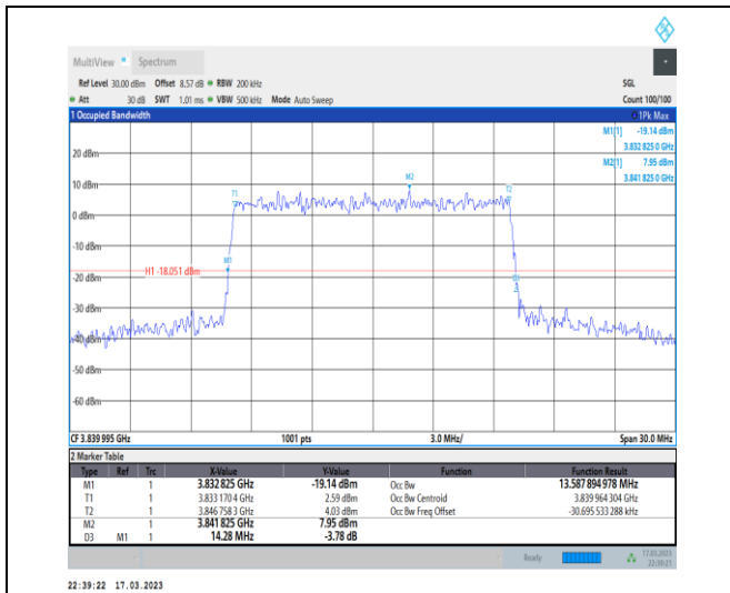
1-N77-3700-3980-30-15-M-9-CP-256QAM-Outer_Ful I-38@0-Ant0-13.588-14.280-≤15-PASS
