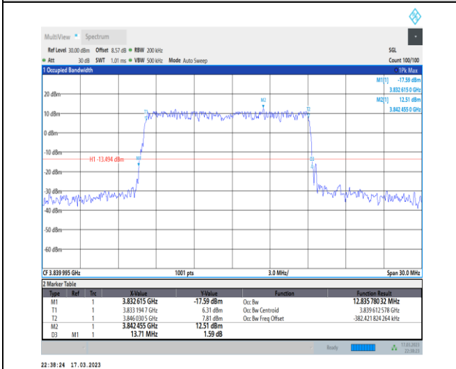
1-N77-3700-3980-30-15-M-3-DFT-16QAM-Outer_Full-36@0-Ant0-12.836-13.710-≤15-PASS
