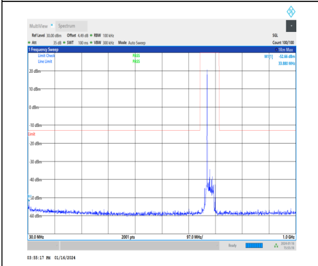
1-N71-15-20-H-1-DFT-PI2BPSK-Inner_1RB_Left-1 @ 1-30-1000-Ant7-34.85--52.66--13-PASS
