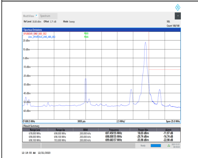
1-N71-15-20-H-5-CP-QPSK-Edge_1RB_Right-1@105-Ant7-1--PASS-see graph
