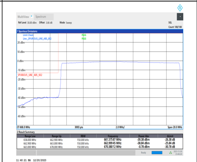
1-N71-15-15-L-6-CP-QPSK-Outer_Full-79@0-Ant7-1--PASS-see graph
