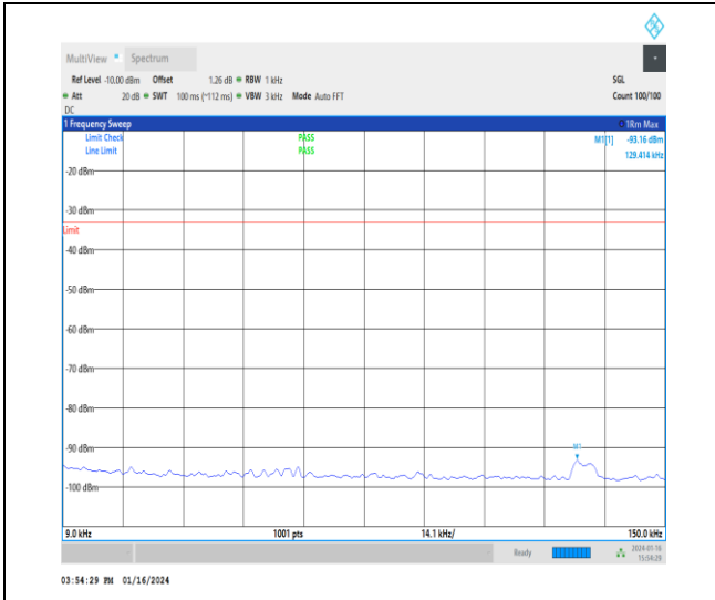
1-N71-15-20-H-1-DFT-PI2BPSK-Inner_1RB_Left-1 @ 1-0.009-0.15-Ant7-0.13--93.16--33-PASS
