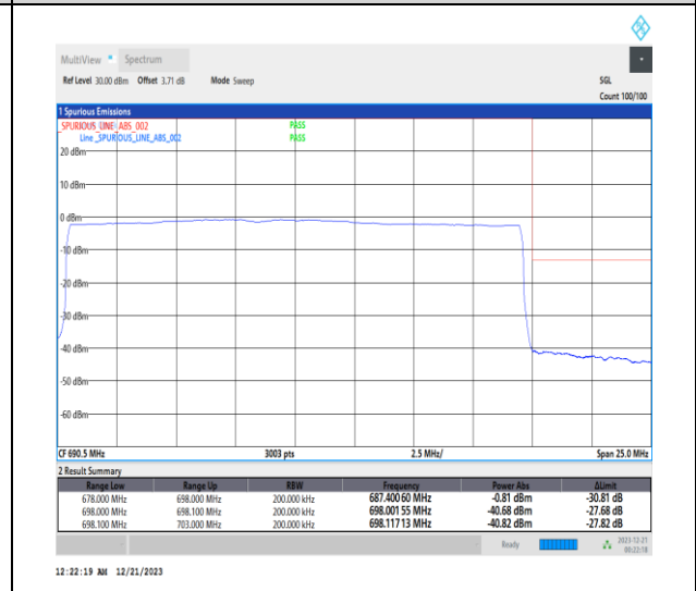
1-N71-15-20-H-6-CP-QPSK-Outer_Full-106@0-Ant7-1--PASS-see graph
