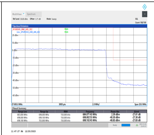
1-N71-15-15-H-3-DFT-PI2BPSK-Outer_Full-75@0-Ant7-1--PASS-see graph
