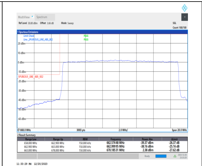
1-N71-15-15-L-3-DFT-PI2BPSK-Outer_Full-75@0-Ant7-1--PASS-see graph
