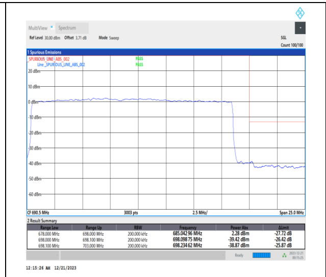
1-N71-15-20-H-3-DFT-PI2BPSK-Outer_Full-100@0-Ant7-1--PASS-see graph
