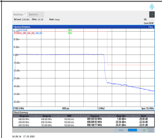
1-N71-PC3-15-10-H-6-CP-QPSK-Outer_Full-52@ 0-Ant7-1--PASS-see graph
