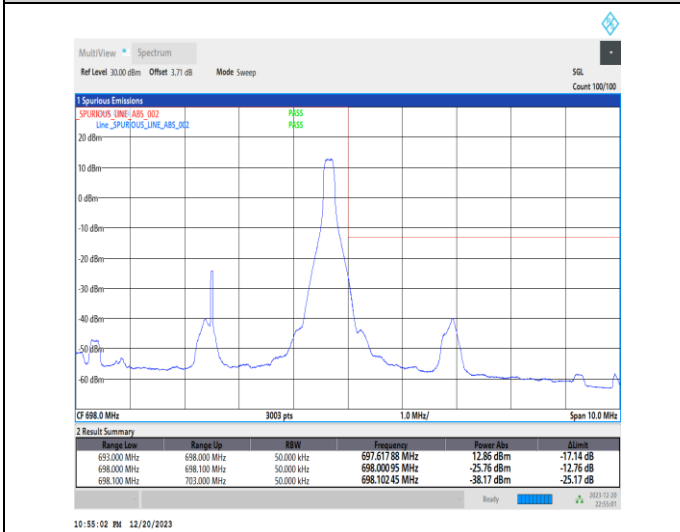
1-N71-15-5-H-5-CP-QPSK-Edge_1RB_Right-1@24-Ant7-1--PASS-see graph
