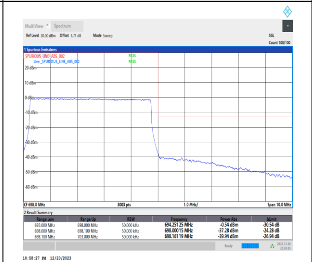
1-N71-15-5-H-6-CP-QPSK-Outer_Full-25@0-Ant7-1--PASS-see graph
