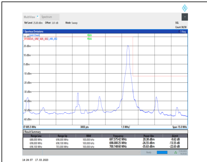
1-N71-PC3-15-10-H-2-DFT-PI2BPSK-Edge_1RB_Righ t-1@51-Ant7-1--PASS-see graph
