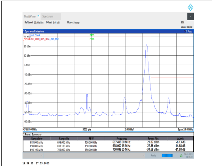
1-N71-PC3-15-15-H-2-DFT-PI2BPSK-Edge_1RB_Righ t-1@78-Ant7-1--PASS-see graph
