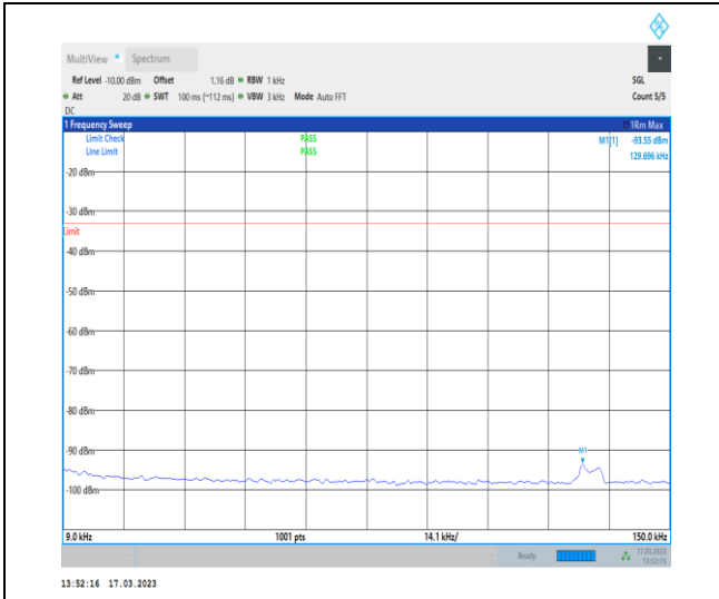
1-N71-PC3-15-20-H-1-DFT-PI2BPSK-Inner_1RB_L eft-1@1-0.009-0.15-Ant7-0.13--93.55--33-PASS
