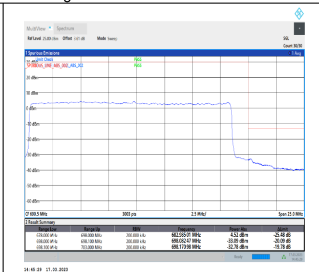
1-N71-PC3-15-20-H-3-DFT-PI2BPSK-Outer_Full-1 00@0-Ant7-1--PASS-see graph
