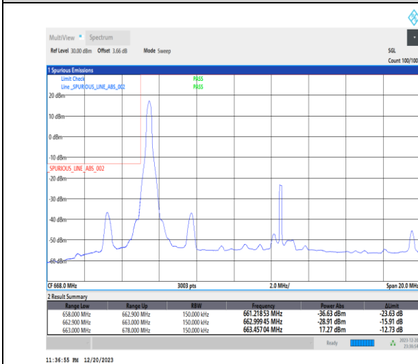
1-N71-15-15-L-4-CP-QPSK-Edge_1RB_Left-1@0-Ant7-1--PASS-see graph
