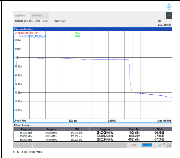
1-N71-15-15-H-6-CP-QPSK-Outer_Full-79@0-Ant7-1--PASS-see graph
