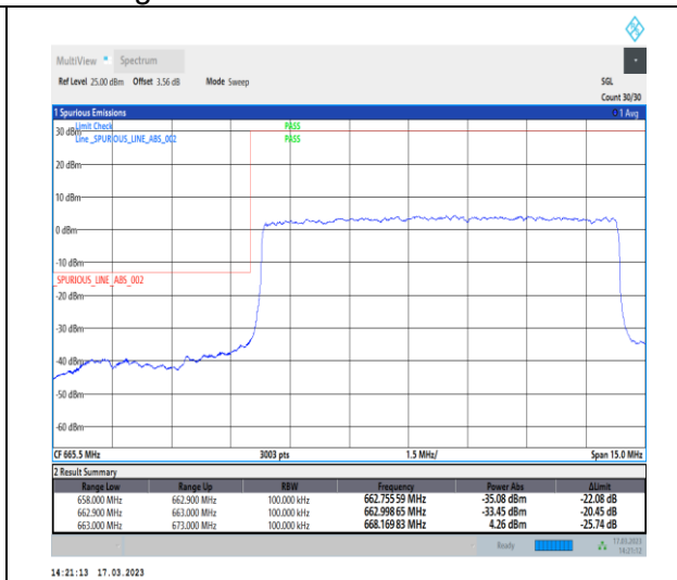
1-N71-PC3-15-10-L-3-DFT-PI2BPSK-Outer_Full-50@0-Ant7-1--PASS-see graph
