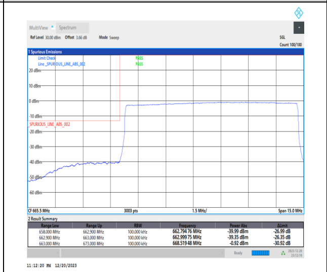
1-N71-15-10-L-6-CP-QPSK-Outer_Full-52@0-Ant7 -1--PASS-see graph
