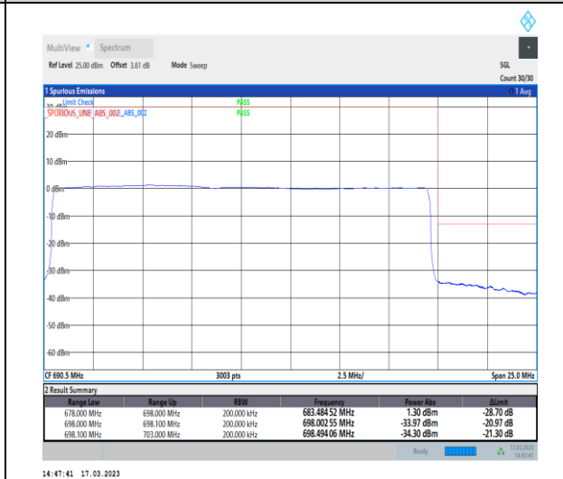
1-N71-PC3-15-20-H-6-CP-QPSK-Outer_Full-106 @0-Ant7-1--PASS-see graph
