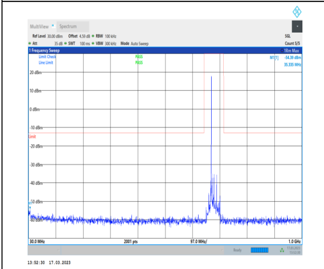
1-N71-PC3-15-20-H-1-DFT-PI2BPSK-Inner_1RB_L eft-1@1-30-1000-Ant7-35.34--54.39--13-PASS
