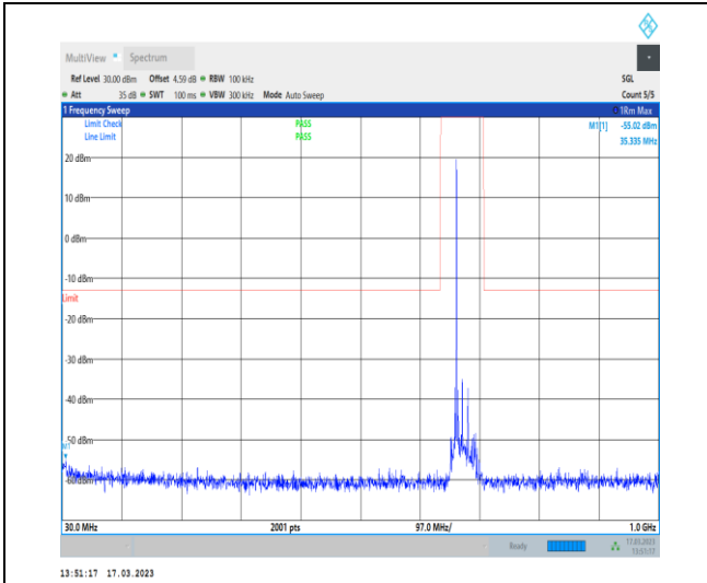
1-N71-PC3-15-20-M-1-DFT-PI2BPSK-Inner_1RB_L eft-1@1-30-1000-Ant7-35.34--55.02--13-PASS
