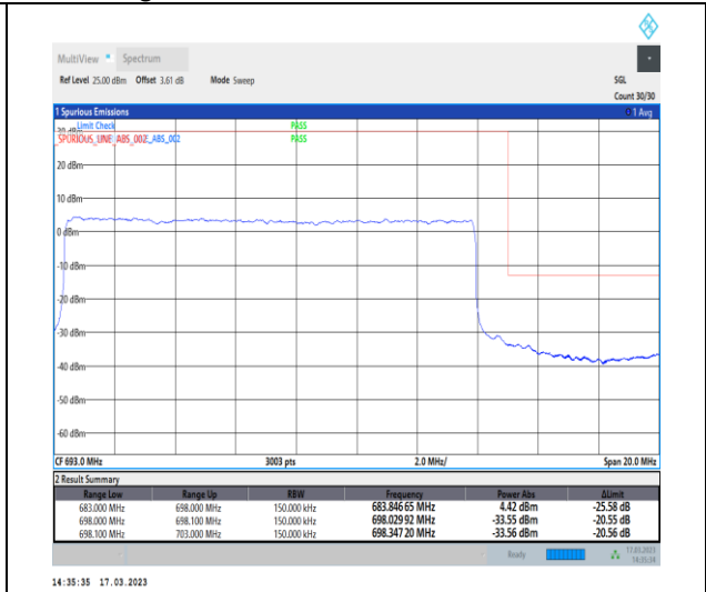
1-N71-PC3-15-15-H-3-DFT-PI2BPSK-Outer_Full-7 5@0-Ant7-1--PASS-see graph
