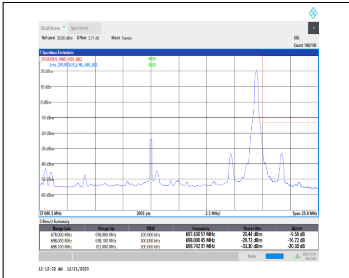
1-N71-15-20-H-2-DFT-PI2BPSK-Edge_1RB_Right-1@105-Ant7-1--PASS-see graph
