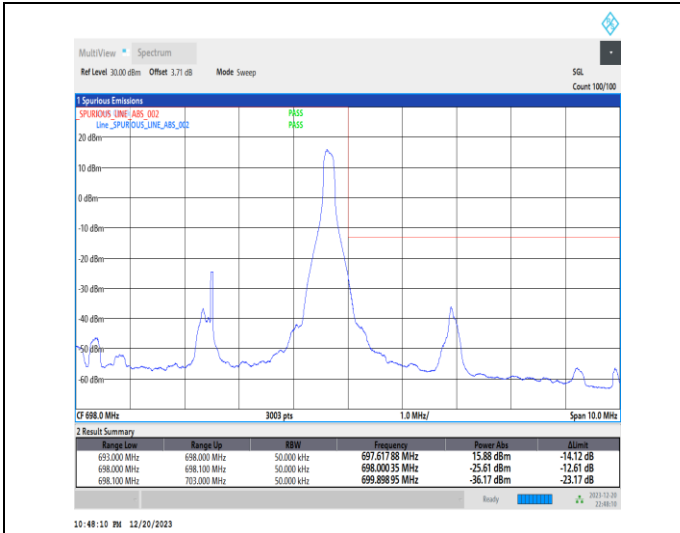
1-N71-15-5-H-2-DFT-PI2BPSK-Edge_1RB_Right-1@2 4-Ant7-1--PASS-see graph
