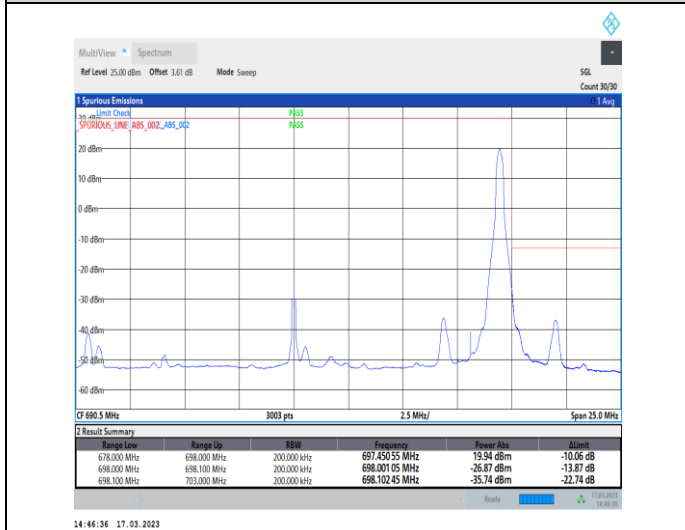
1-N71-PC3-15-20-H-5-CP-QPSK-Edge_1RB_Right-1 @105-Ant7-1--PASS-see graph
