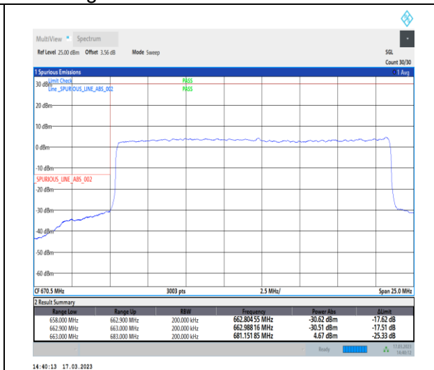
1-N71-PC3-15-20-L-3-DFT-PI2BPSK-Outer_Full-100@0-Ant7-1--PASS-see graph
