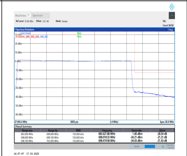
1-N71-PC3-15-15-H-6-CP-QPSK-Outer_Full-79@ 0-Ant7-1--PASS-see graph
