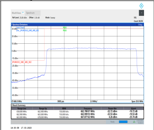
1-N71-PC3-15-15-L-3-DFT-PI2BPSK-Outer_Full-75@0-Ant7-1--PASS-see graph
