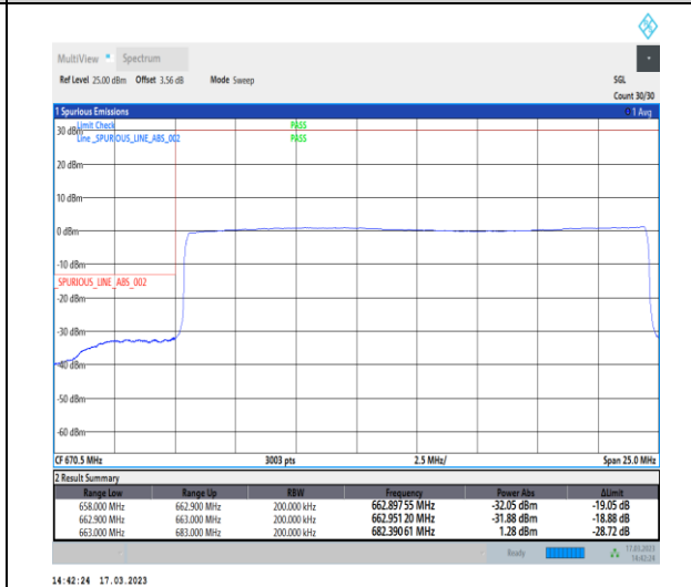
1-N71-PC3-15-20-L-6-CP-QPSK-Outer_Full-106@0-Ant7-1--PASS-see graph
