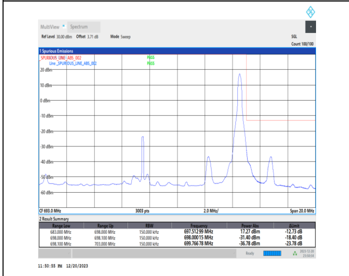
1-N71-15-15-H-5-CP-QPSK-Edge_1RB_Right-1@78-Ant7-1--PASS-see graph
