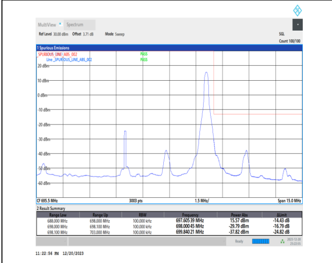
1-N71-15-10-H-5-CP-QPSK-Edge_1RB_Right-1@51-Ant7-1--PASS-see graph
