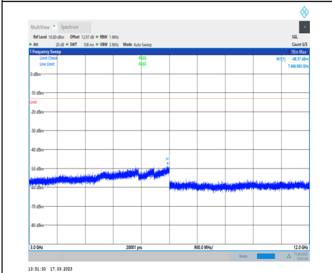
1-N71-PC3-15-20-M-1-DFT-PI2BPSK-Inner_1RB_L eft-1@1-3000-12000-Ant7-7446.45--48.37--13-PAS S
