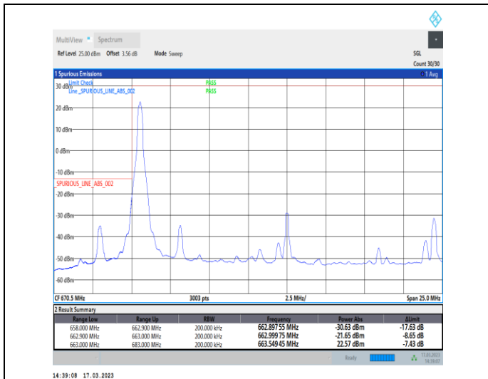
1-N71-PC3-15-20-L-1-DFT-PI2BPSK-Edge_1RB_Left-1@0-Ant7-1--PASS-see graph
