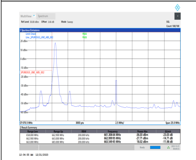
1-N71-15-20-L-4-CP-QPSK-Edge_1RB_Left-1@0-Ant 7-1--PASS-see graph
