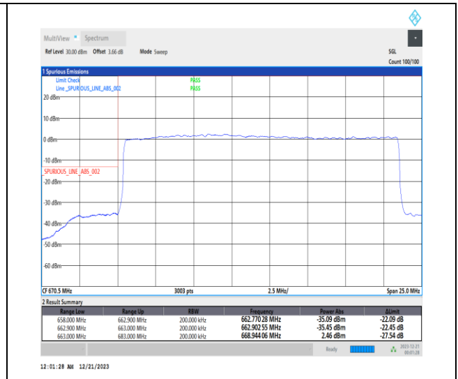
1-N71-15-20-L-3-DFT-PI2BPSK-Outer_Full-100@0 Ant7-1--PASS-see graph
