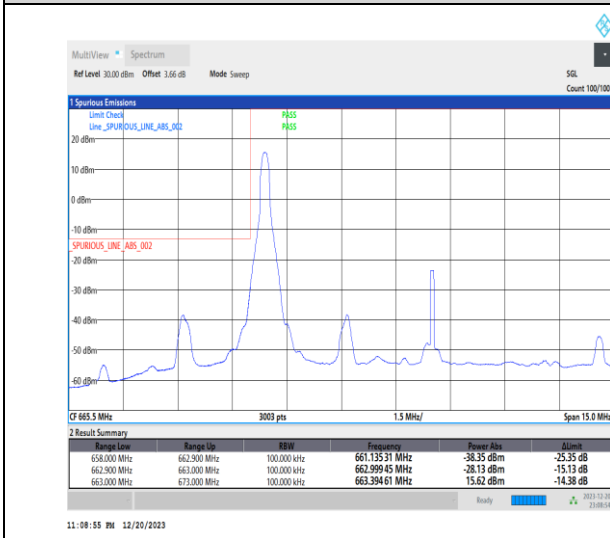
1-N71-15-10-L-4-CP-QPSK-Edge_1RB_Left-1@0-Ant 7-1--PASS-see graph
