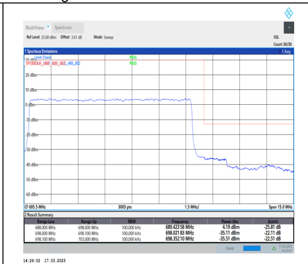
1-N71-PC3-15-10-H-3-DFT-PI2BPSK-Outer_Full-5 0@0-Ant7-1--PASS-see graph
