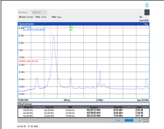
1-N71-PC3-15-15-L-4-CP-QPSK-Edge_1RB_Left-1@0-Ant7-1--PASS-see graph
