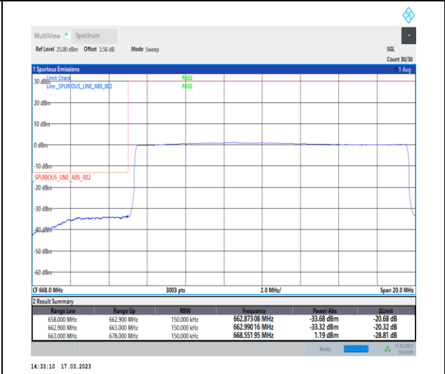
1-N71-PC3-15-15-L-6-CP-QPSK-Outer_Full-79@0-Ant7-1--PASS-see graph
