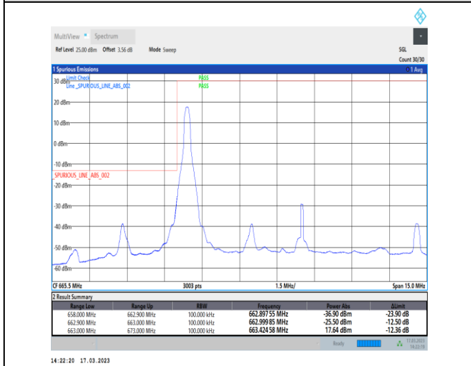
1-N71-PC3-15-10-L-4-CP-QPSK-Edge_1RB_Left-1@0-Ant7-1--PASS-see graph
