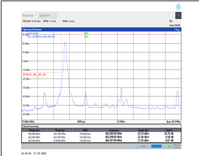
1-N71-PC3-15-15-L-1-DFT-PI2BPSK-Edge_1RB_Left-1@0-Ant7-1--PASS-see graph
