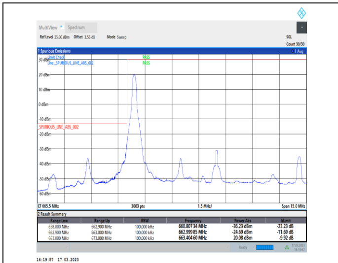
1-N71-PC3-15-10-L-1-DFT-PI2BPSK-Edge_1RB_Left-1@0-Ant7-1--PASS-see graph
