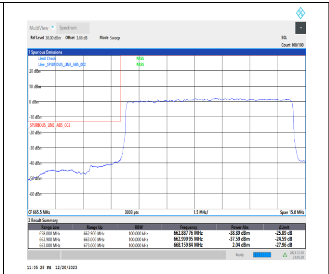
1-N71-15-10-L-3-DFT-PI2BPSK-Outer_Full-50@0- Ant7-1--PASS-see graph
