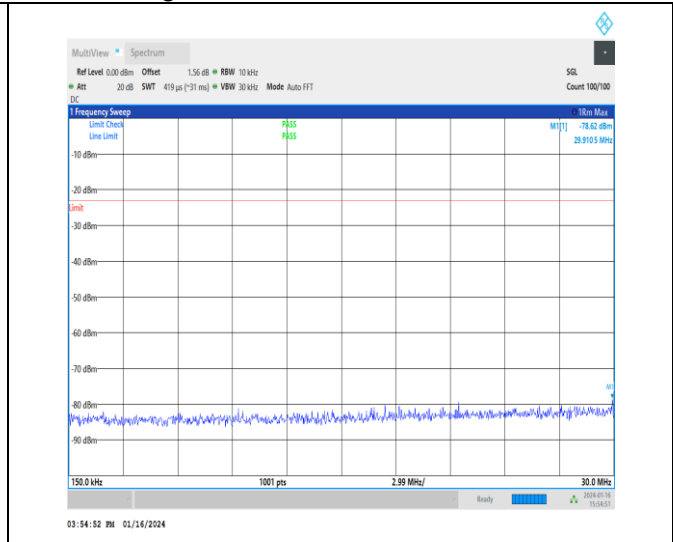
1-N71-15-20-H-1-DFT-PI2BPSK-Inner_1RB_Left-1 @ 1-0.15-30-Ant7-2.42--78.62--23-PASS
