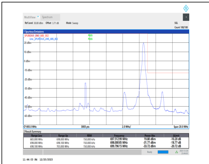
1-N71-15-15-H-2-DFT-PI2BPSK-Edge_1RB_Right-1@78-Ant7-1--PASS-see graph
