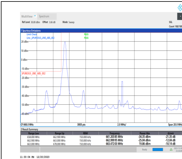
1-N71-15-15-L-1-DFT-PI2BPSK-Edge_1RB_Left-1@0-Ant7-1--PASS-see graph
