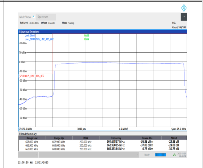
1-N71-15-20-L-6-CP-QPSK-Outer_Full-106@0-Ant 7-1--PASS-see graph
