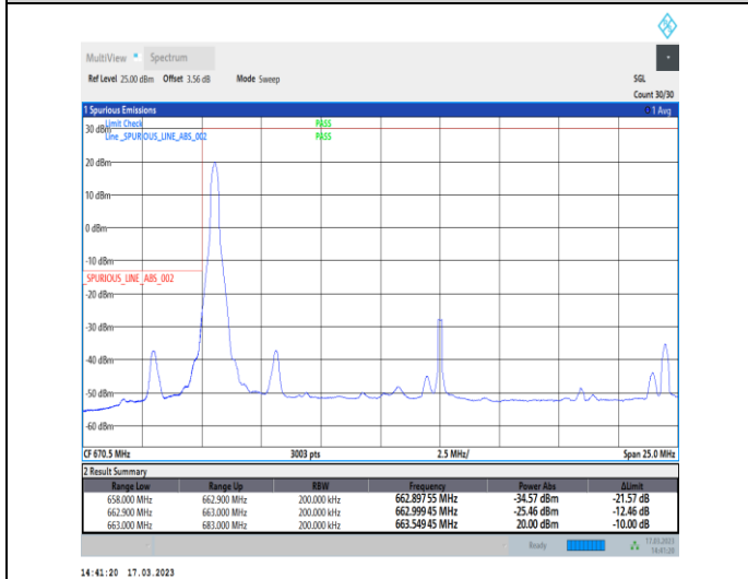
1-N71-PC3-15-20-L-4-CP-QPSK-Edge_1RB_Left-1@0-Ant7-1--PASS-see graph
