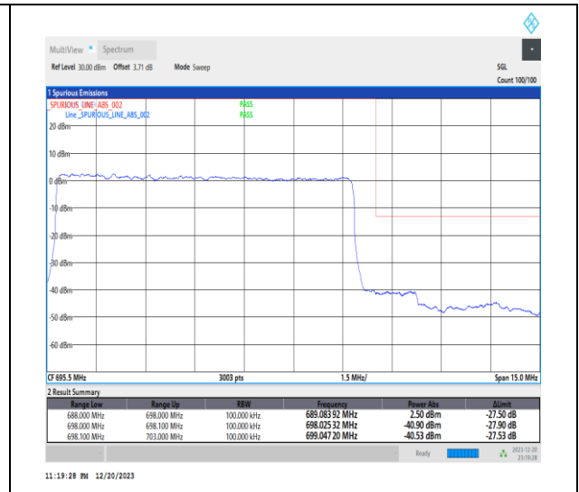
1-N71-15-10-H-3-DFT-PI2BPSK-Outer_Full-50@0-Ant7-1--PASS-see graph
