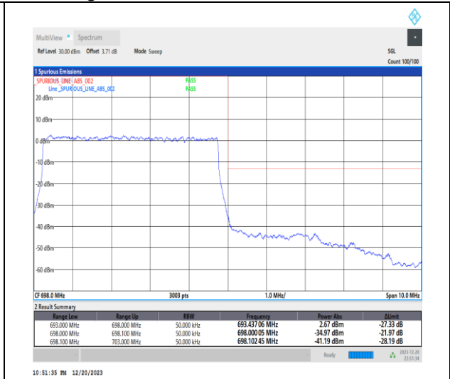
1-N71-15-5-H-3-DFT-PI2BPSK-Outer_Full-25@0-Ant7-1--PASS-see graph
