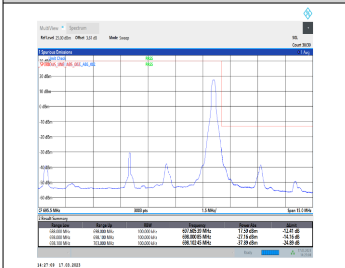
1-N71-PC3-15-10-H-5-CP-QPSK-Edge_1RB_Righ t-1@51-Ant7-1--PASS-see graph
