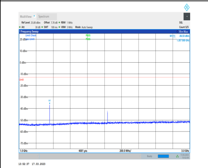
1-N71-PC3-15-20-H-1-DFT-PI2BPSK-Inner_1RB_Lef t-1@1-1000-3000-Ant7-1357.50--36.53--13-PASS
