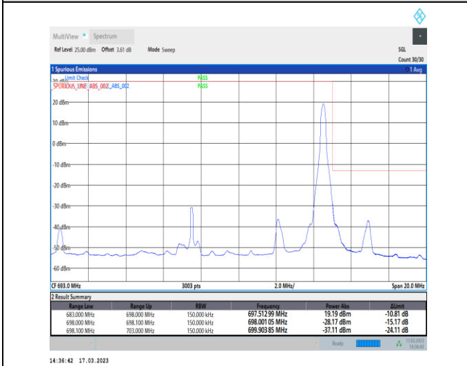
1-N71-PC3-15-15-H-5-CP-QPSK-Edge_1RB_Righ t-1@78-Ant7-1--PASS-see graph
