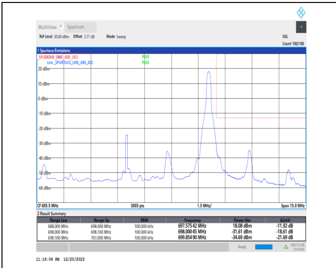
1-N71-15-10-H-2-DFT-PI2BPSK-Edge_1RB_Right-1@51-Ant7-1--PASS-see graph
