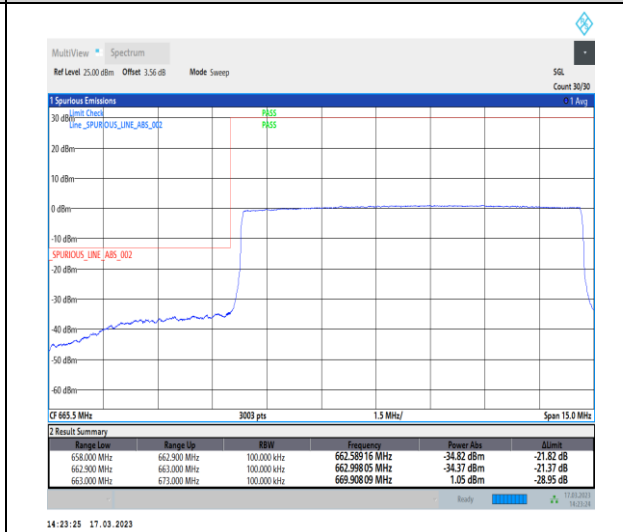
1-N71-PC3-15-10-L-6-CP-QPSK-Outer_Full-52@0-Ant7-1--PASS-see graph
