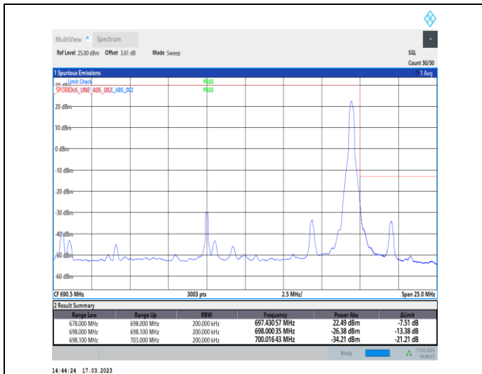
1-N71-PC3-15-20-H-2-DFT-PI2BPSK-Edge_1RB_Righ t-1@105-Ant7-1--PASS-see graph
