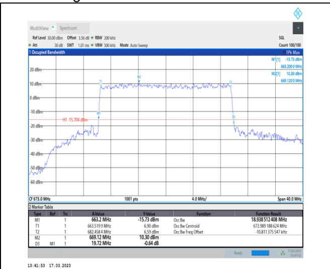
1-N71-PC3-15-20-L-6-CP-QPSK-Outer_Full-106@0-Ant7-18.939-19.720-≤20-PASS
