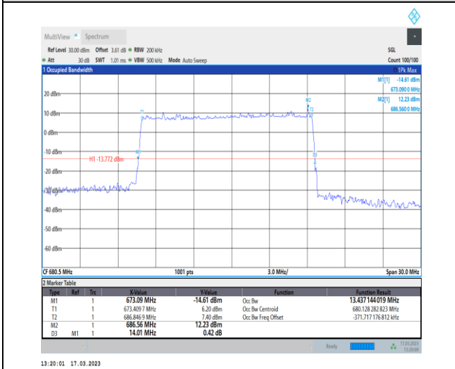
1-N71-PC3-15-15-M-5-DFT-256QAM-Outer_Full-75 @0-Ant7-13.437-14.010-≤15-PASS
