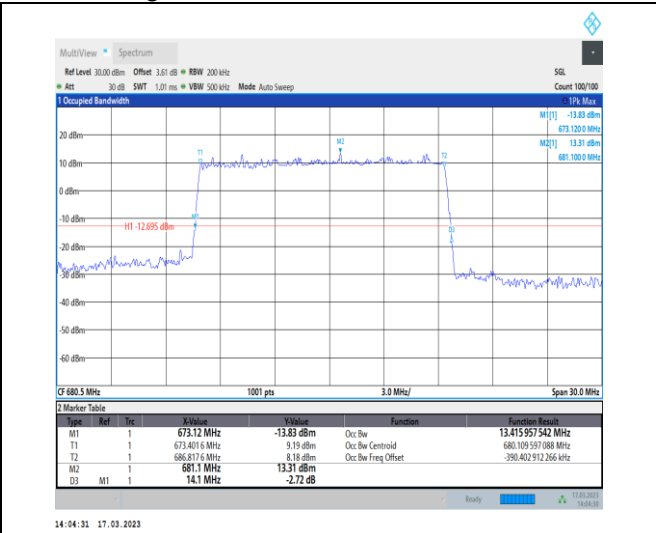
1-N71-PC3-15-15-M-8-CP-64QAM-Outer_Full-79@0 -Ant7-13.416-14.100-≤15-PASS
