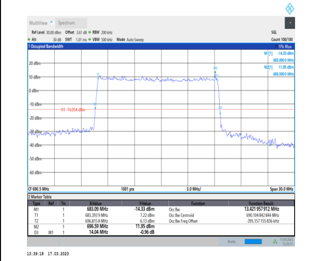
1-N71-PC3-15-15-H-5-DFT-256QAM-Outer_Full-75 @0-Ant7-13.422-14.040-≤15-PASS
