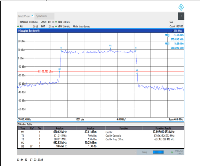
1-N71-PC3-15-20-M-5-DFT-256QAM-Outer_Full-100 @0-Ant7-17.897-18.600-≤20-PASS
