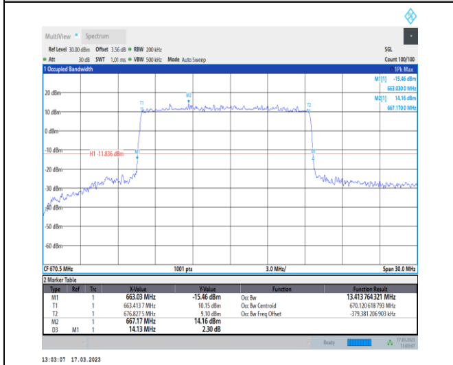
1-N71-PC3-15-15-L-1-DFT-QPSK-Outer_Full-75@0- Ant7-13.414-14.130-≤15-PASS
