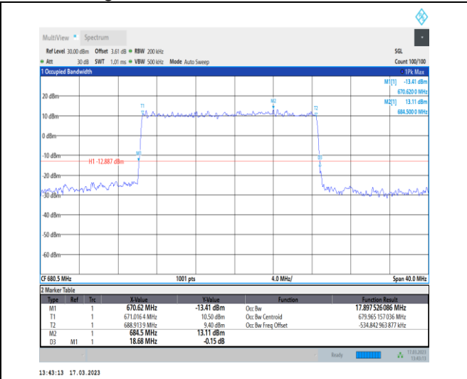
1-N71-PC3-15-20-M-1-DFT-QPSK-Outer_Full-100 @0-Ant7-17.898-18.680-≤20-PASS
