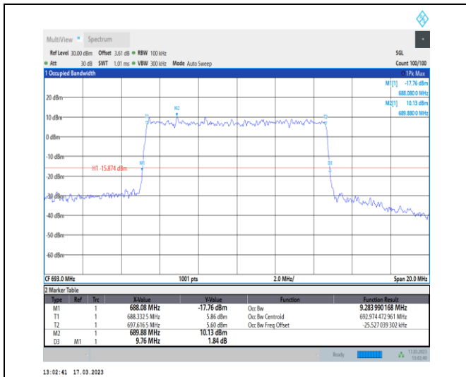
1-N71-PC3-15-10-H-8-CP-64QAM-Outer_Full-52@0 -Ant7-9.284-9.760-≤10-PASS
