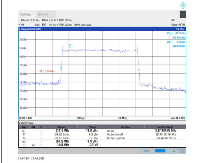
1-N71-PC3-15-20-H-5-DFT-256QAM-Outer_Full-100 @0-Ant7-17.872-18.640-≤20-PASS
