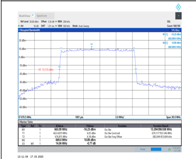
1-N71-PC3-15-15-L-5-DFT-256QAM-Outer_Full-75 @0-Ant7-13.394-14.040-≤15-PASS
