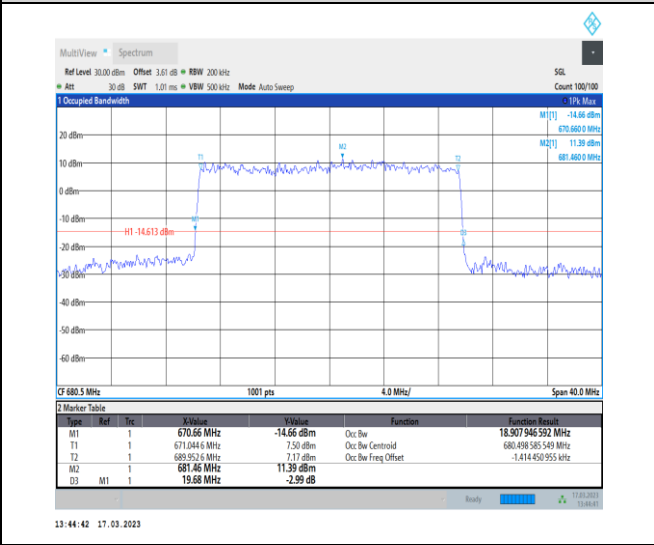
1-N71-PC3-15-20-M-7-CP-16QAM-Outer_Full-106@0 -Ant7-18.908-19.680-≤20-PASS
