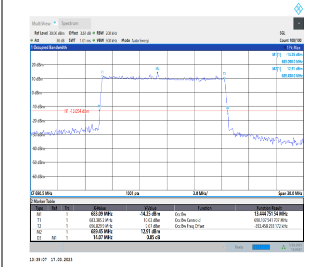
1-N71-PC3-15-15-H-4-DFT-64QAM-Outer_Full-75 @0-Ant7-13.445-14.070-≤15-PASS
