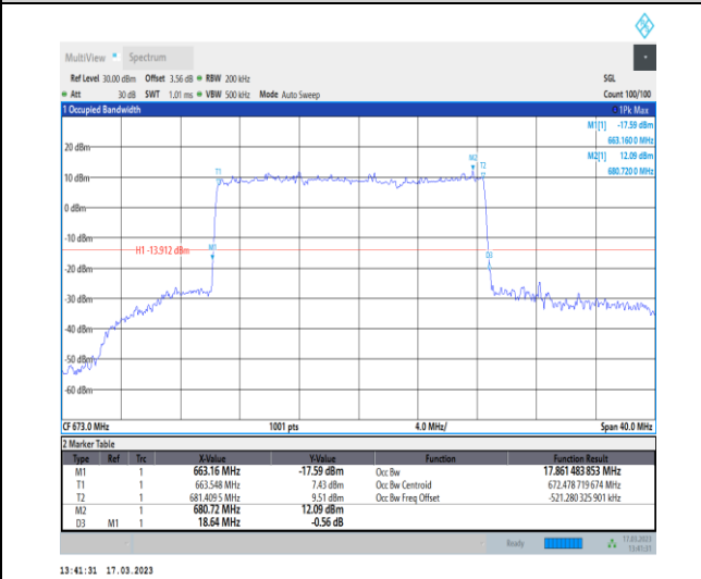
1-N71-PC3-15-20-L-4-DFT-64QAM-Outer_Full-100@0-Ant7-17.861-18.640-≤20-PASS
