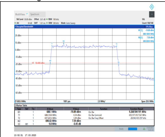
1-N71-PC3-15-10-H-9-CP-256QAM-Outer_Full-52@ 0-Ant7-9.269-9.800-≤10-PASS
