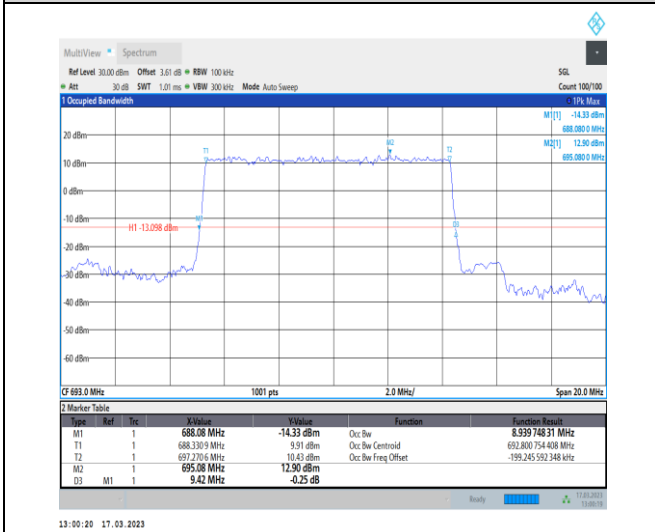
1-N71-PC3-15-10-H-2-DFT-PI2BPSK-Outer_Full-50 @0-Ant7-8.94-9.420-≤10-PASS
