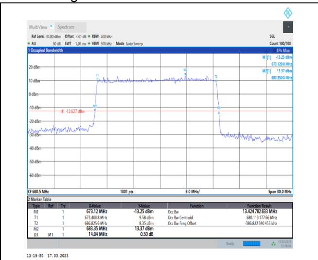
1-N71-PC3-15-15-M-4-DFT-64QAM-Outer_Full-75@ 0-Ant7-13.425-14.040-≤15-PASS
