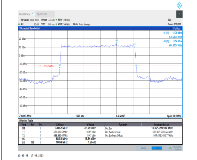
1-N71-PC3-15-20-M-2-DFT-PI2BPSK-Outer_Full-10 @0-Ant7-17.876-18.680-≤20-PASS
