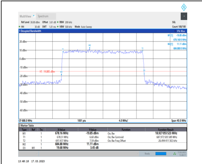
1-N71-PC3-15-20-H-7-CP-16QAM-Outer_Full-106@ 0-Ant7-18.927-19.680-≤20-PASS
