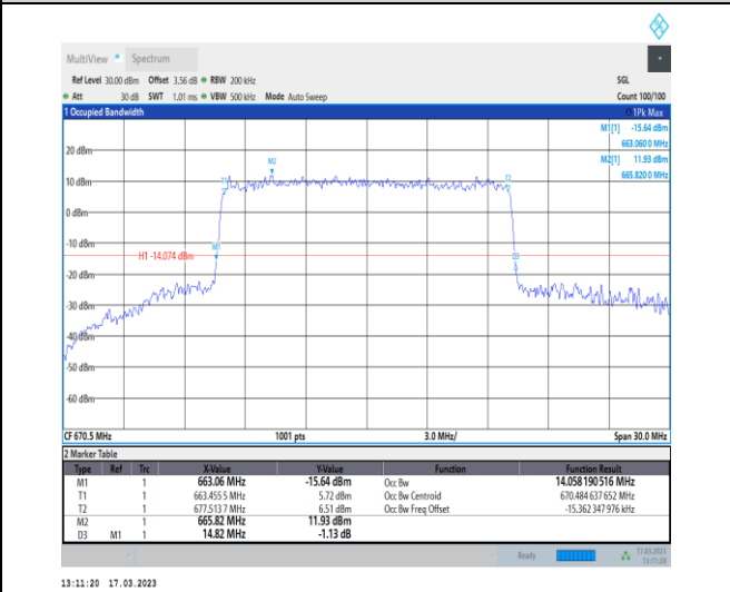
1-N71-PC3-15-15-L-6-CP-QPSK-Outer_Full-79@0- Ant7-14.058-14.820-≤15-PASS
