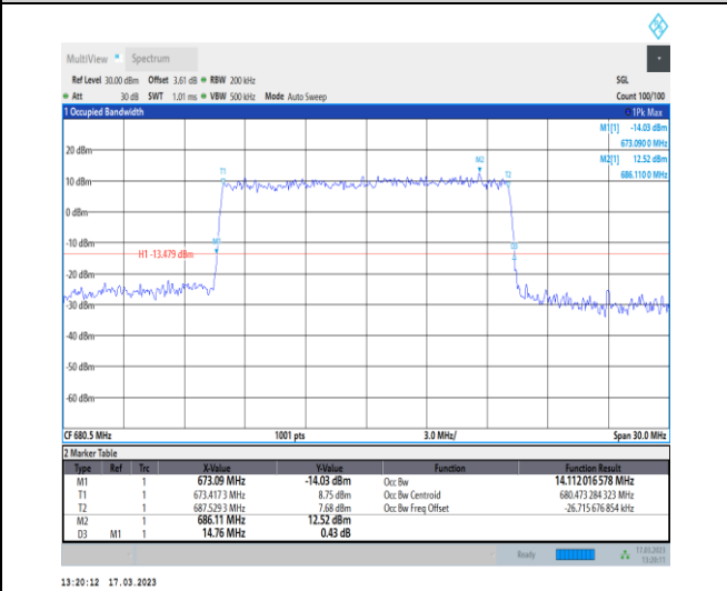
1-N71-PC3-15-15-M-6-CP-QPSK-Outer_Full-79@0- Ant7-14.112-14.760-≤15-PASS
