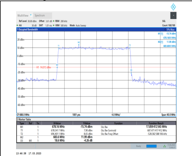
1-N71-PC3-15-20-H-4-DFT-64QAM-Outer_Full-100 @0-Ant7-17.859-18.600-≤20-PASS
