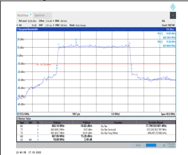
1-N71-PC3-15-20-L-2-DFT-PI2BPSK-Outer_Full-100@0-Ant7-17.8-18.680-≤20-PASS
