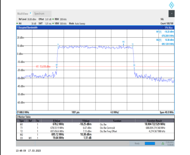
1-N71-PC3-15-20-H-6-CP-QPSK-Outer_Full-106@0 -Ant7-18.905-19.640-≤20-PASS
