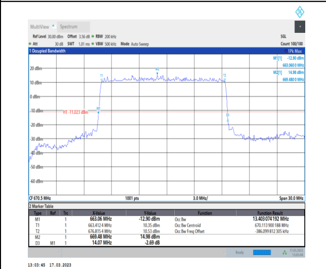
1-N71-PC3-15-15-L-2-DFT-PI2BPSK-Outer_Full-75 @0-Ant7-13.403-14.070-≤15-PASS
