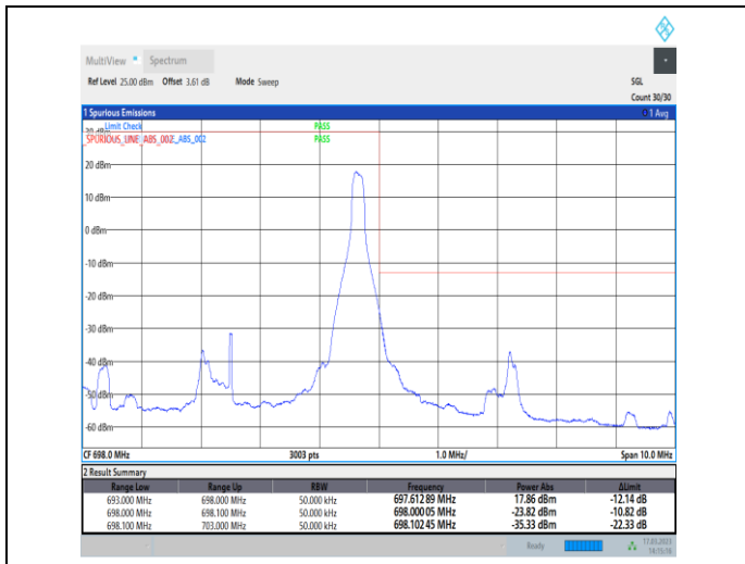
1-N71-PC3-15-5-H-2-DFT-PI2BPSK-Edge_1RB_Right-1@24-Ant7-1--PASS-see graph
