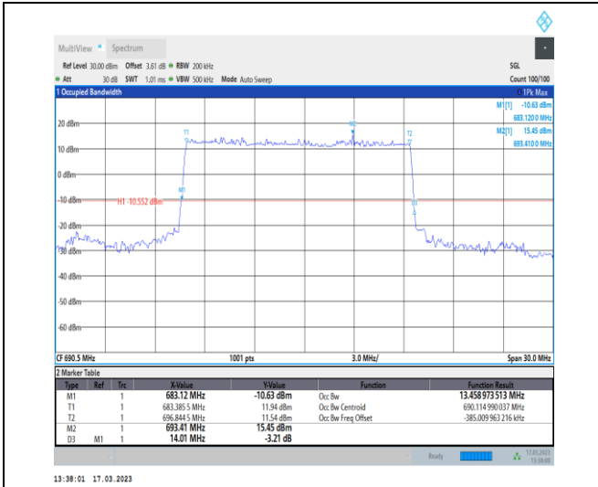
1-N71-PC3-15-15-H-2-DFT-PI2BPSK-Outer_Full-75 @0-Ant7-13.459-14.010-≤15-PASS
