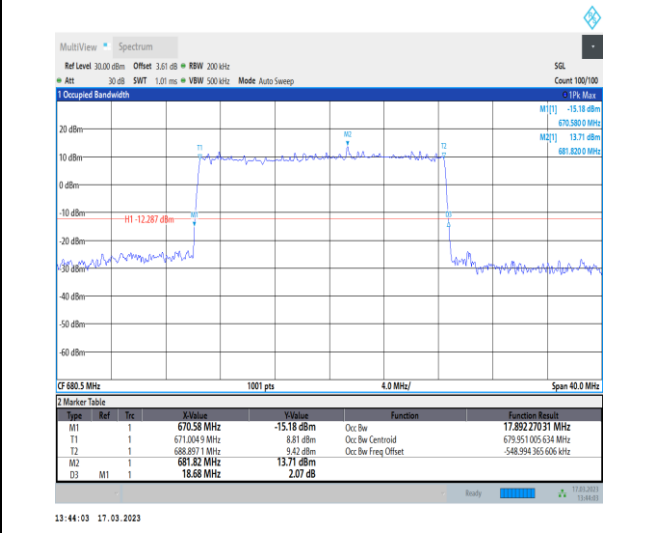
1-N71-PC3-15-20-M-3-DFT-16QAM-Outer_Full-100 @0-Ant7-17.892-18.680-≤20-PASS
