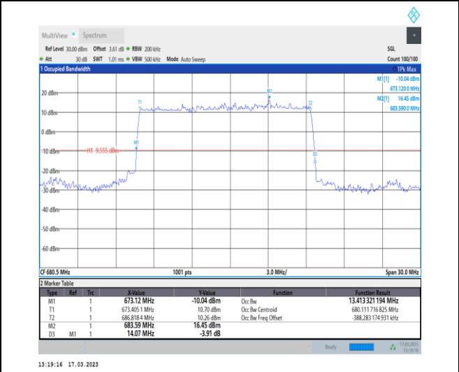
1-N71-PC3-15-15-M-2-DFT-PI2BPSK-Outer_Full-75@0-Ant7-13.413-14.070-≤15-PASS
