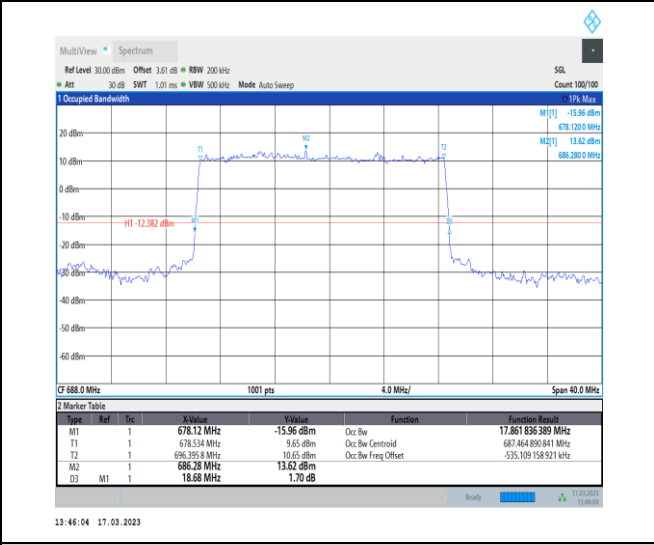
1-N71-PC3-15-20-H-2-DFT-PI2BPSK-Outer_Full-100 @0-Ant7-17.862-18.680-≤20-PASS
