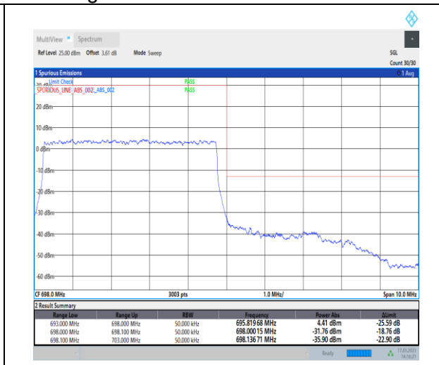
1-N71-PC3-15-5-H-3-DFT-PI2BPSK-Outer_Full-25@0-Ant7-1--PASS-see graph
