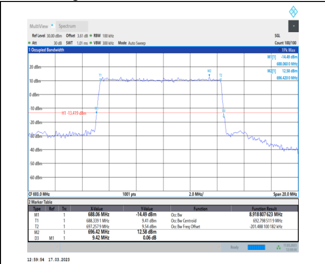
1-N71-PC3-15-10-H-1-DFT-QPSK-Outer_Full-50@ 0-Ant7-8.919-9.420-≤10-PASS
