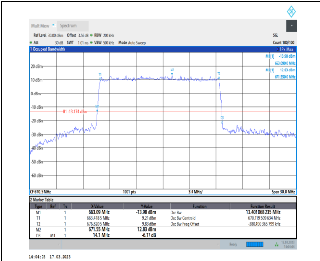
1-N71-PC3-15-15-L-3-DFT-16QAM-Outer_Full-75@ 0-Ant7-13.402-14.100-≤15-PASS
