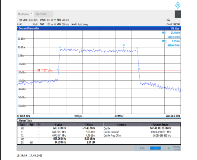
1-N71-PC3-15-15-H-9-CP-256QAM-Outer_Full-79@0-Ant7-14.142-14.790-≤15-PASS
