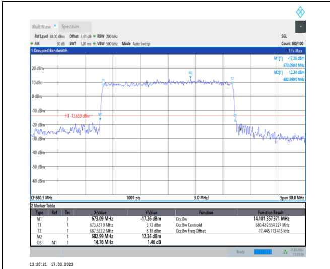
1-N71-PC3-15-15-M-7-CP-16QAM-Outer_Full-79@0 -Ant7-14.101-14.760-≤15-PASS
