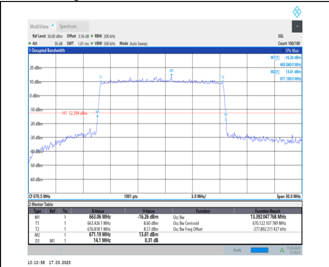
1-N71-PC3-15-15-L-4-DFT-64QAM-Outer_Full-75@ 0-Ant7-13.392-14.100-≤15-PASS
