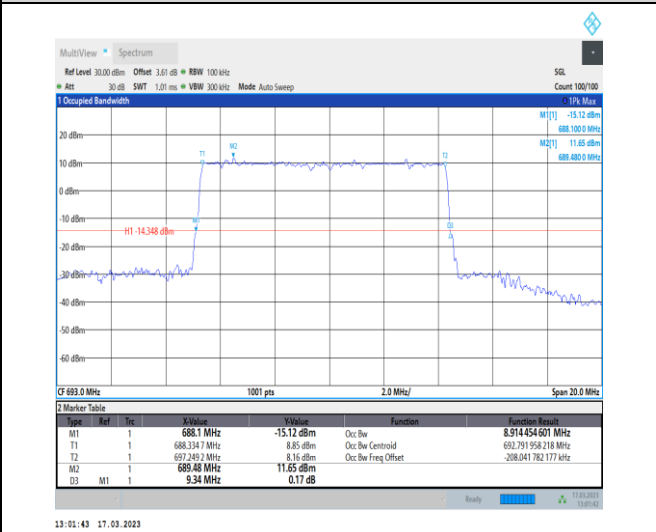
1-N71-PC3-15-10-H-3-DFT-16QAM-Outer_Full-50@ 0-Ant7-8.914-9.340-≤10-PASS
