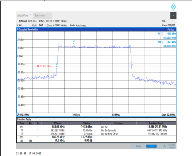
1-N71-PC3-15-15-H-3-DFT-16QAM-Outer_Full-75 @0-Ant7-13.436-14.100-≤15-PASS
