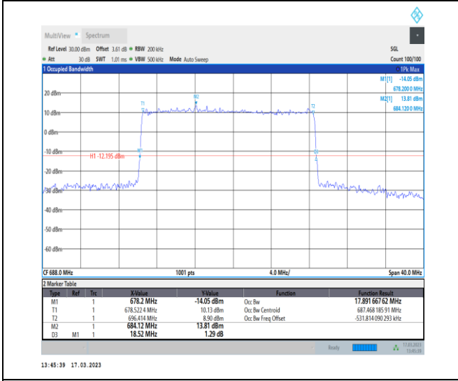
1-N71-PC3-15-20-H-1-DFT-QPSK-Outer_Full-100@ 0-Ant7-17.892-18.520-≤20-PASS
