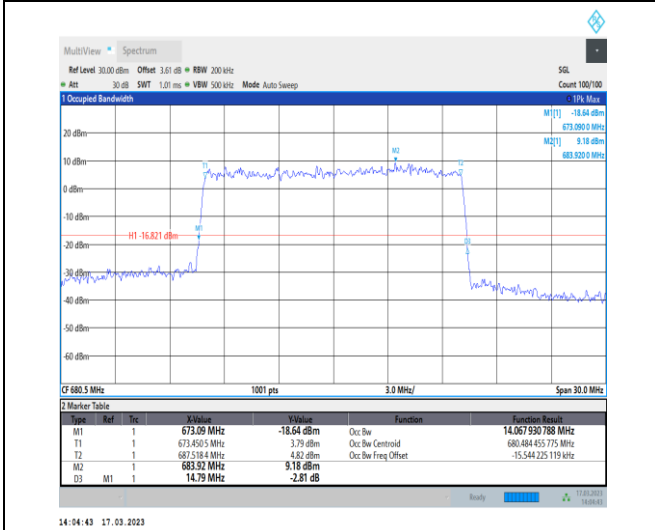
1-N71-PC3-15-15-M-9-CP-256QAM-Outer_Full-79@0 0-Ant7-14.068-14.790-≤15-PASS
