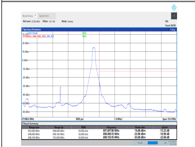
1-N71-PC3-15-5-H-2-DFT-PI2BPSK-Edge_1RB_Right-1@24-Ant7-1--PASS-see graph
