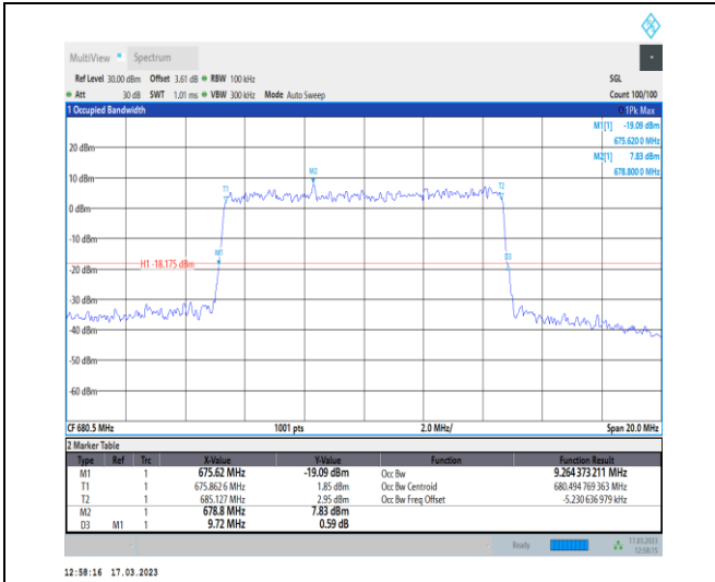
1-N71-PC3-15-10-M-9-CP-256QAM-Outer_Full-52@ 0-Ant7-9.264-9.720-≤10-PASS
