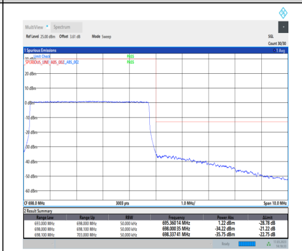
1-N71-PC3-15-5-H-3-DFT-PI2BPSK-Outer_Full-25@0-Ant7-1--PASS-see graph
