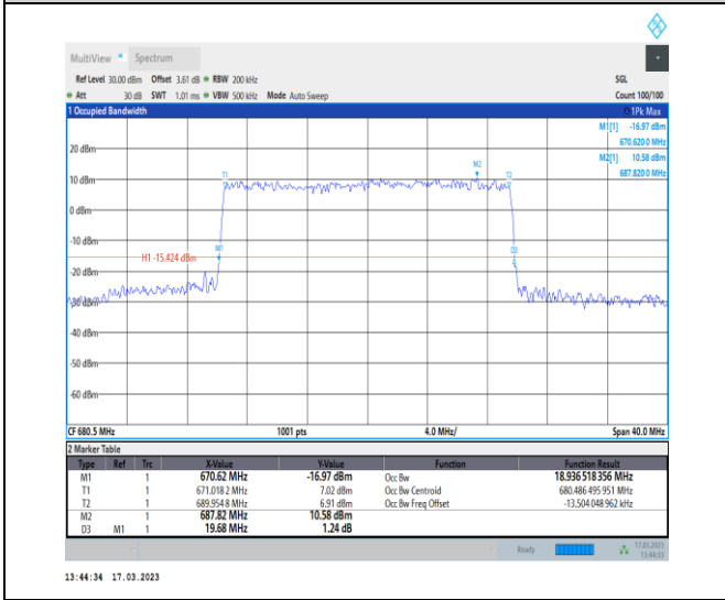
1-N71-PC3-15-20-M-6-CP-QPSK-Outer_Full-106@0 -Ant7-18.937-19.680-≤20-PASS
