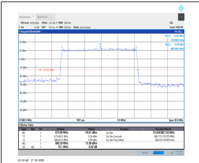
1-N71-PC3-15-15-M-3-DFT-16QAM-Outer_Full-75@ 0-Ant7-13.424-14.100-≤15-PASS
