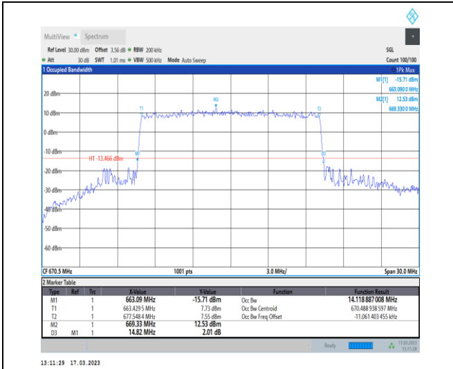
1-N71-PC3-15-15-L-7-CP-16QAM-Outer_Full-79@0-Ant7-14.119-14.820-≤15-PASS
