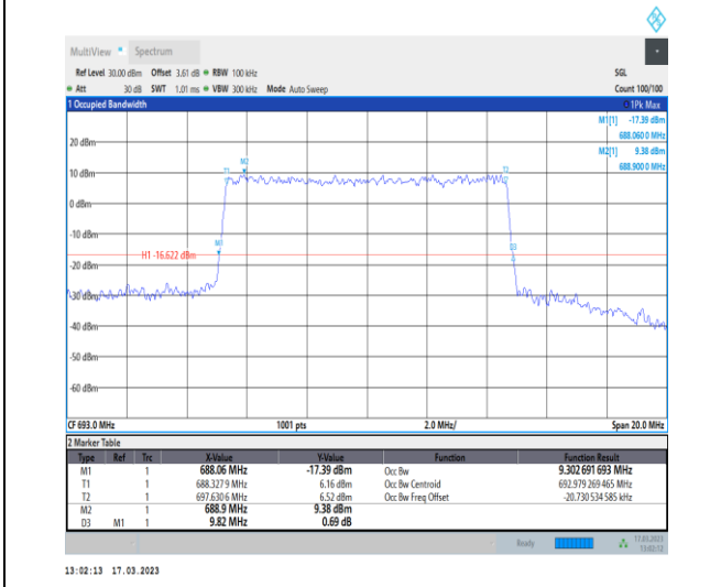
1-N71-PC3-15-10-H-6-CP-QPSK-Outer_Full-52@0-Ant7-9.303-9.820-≤10-PASS
