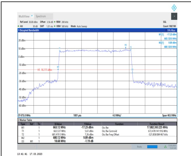
1-N71-PC3-15-20-L-5-DFT-256QAM-Outer_Full-100@0-Ant7-17.882-18.680-≤20-PASS
