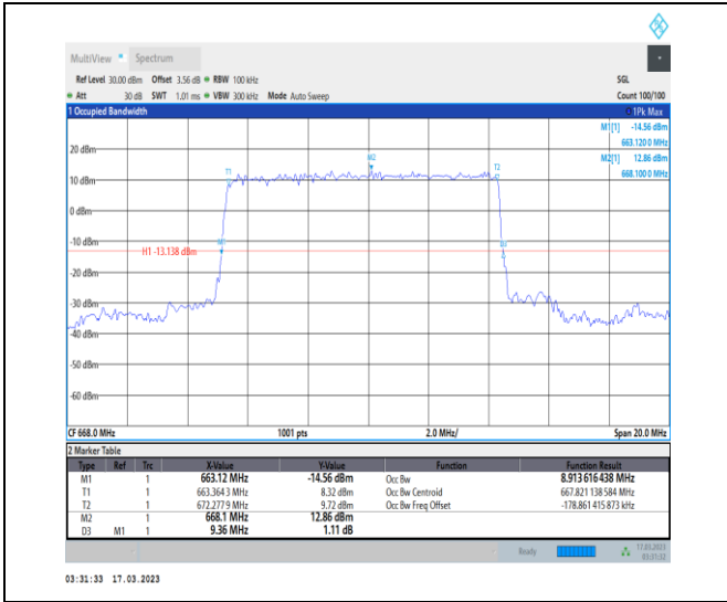
1-N71-PC3-15-10-L-2-DFT-PI2BPSK-Outer_Full-50 @0-Ant7-8.914-9.360-≤10-PASS
