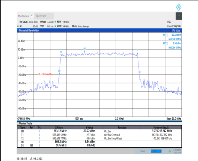
1-N71-PC3-15-10-L-9-CP-256QAM-Outer_Full-52@ 0-Ant7-9.27-9.760-≤10-PASS
