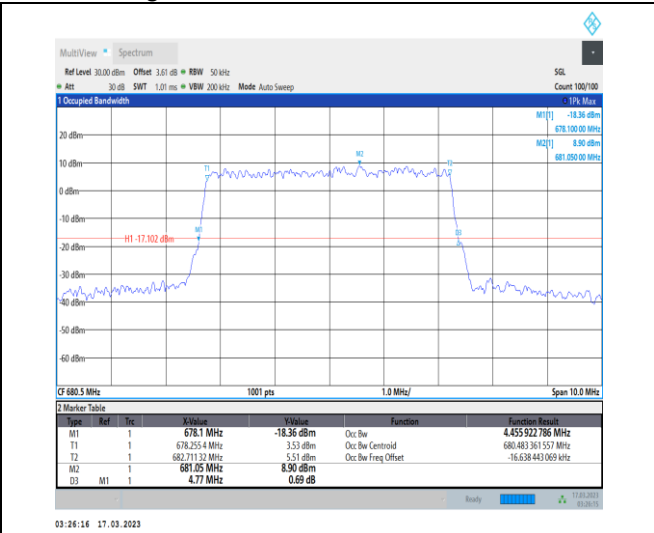
1-N71-PC3-15-5-M-5-DFT-256QAM-Outer_Full-25@0-Ant7-4.456-4.770-≤5-PASS
