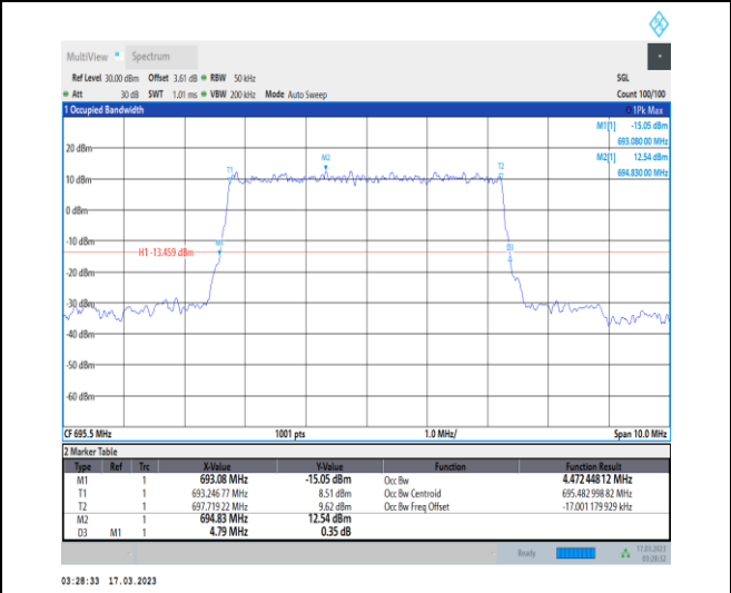
1-N71-PC3-15-5-H-2-DFT-PI2BPSK-Outer_Full-25@0-Ant7-4.472-4.790-≤5-PASS
