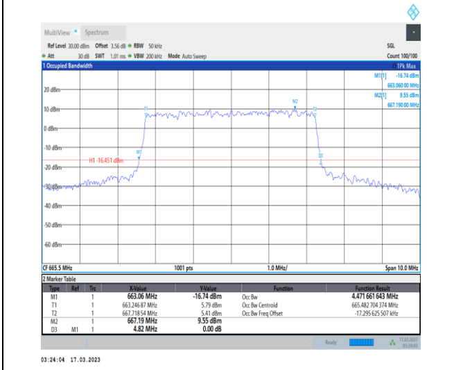
1-N71-PC3-15-5-L-7-CP-16QAM-Outer_Full-25@0-Ant7-4.472-4.820-<math>\leq</math>5-PASS
