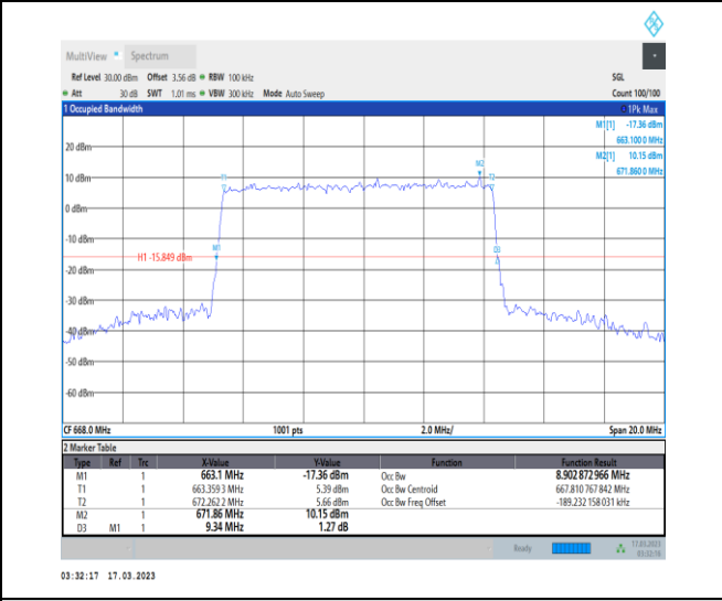
1-N71-PC3-15-10-L-5-DFT-256QAM-Outer_Full-50 @0-Ant7-8.903-9.340-≤10-PASS
