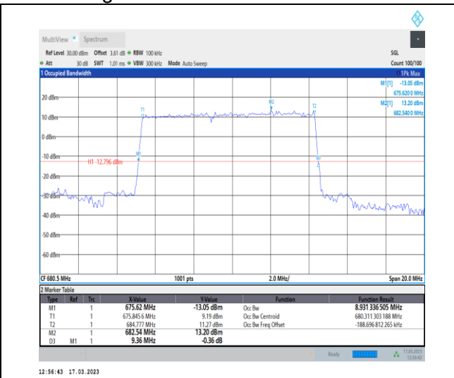
1-N71-PC3-15-10-M-2-DFT-PI2BPSK-Outer_Full-50@0-Ant7-8.931-9.360-≤10-PASS
