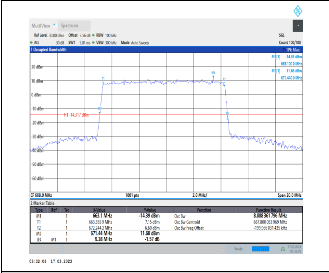
1-N71-PC3-15-10-L-4-DFT-64QAM-Outer_Full-50 @0-Ant7-8.888-9.380-≤10-PASS
