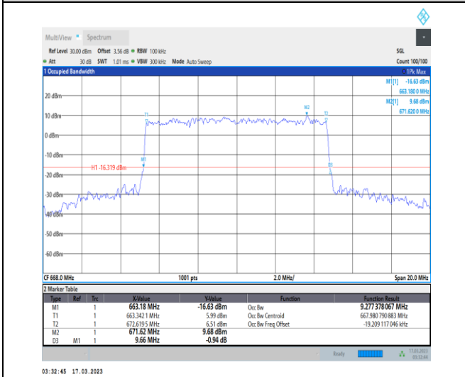
1-N71-PC3-15-10-L-8-CP-64QAM-Outer_Full-52@0- Ant7-9.277-9.660-≤10-PASS
