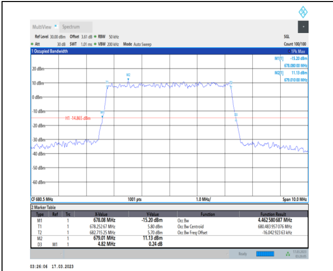
1-N71-PC3-15-5-M-4-DFT-64QAM-Outer_Full-25@0-Ant7-4.463-4.820-≤5-PASS
