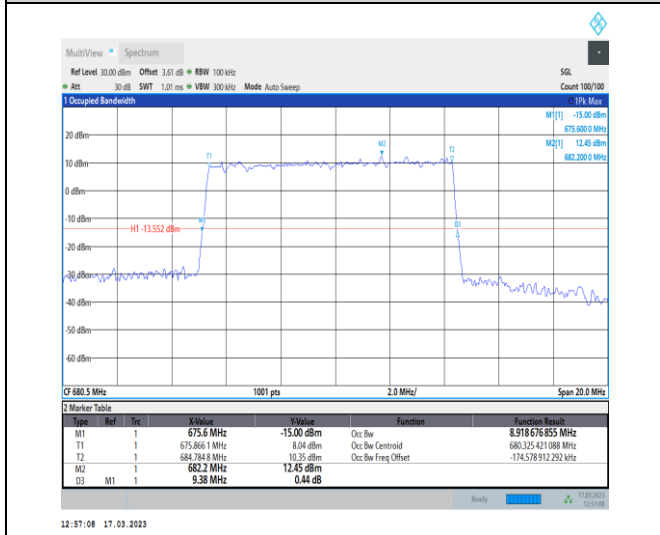
1-N71-PC3-15-10-M-3-DFT-16QAM-Outer_Full-50@0-Ant7-8.919-9.380-≤10-PASS
