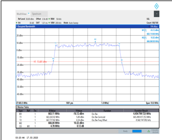
1-N71-PC3-15-5-L-5-DFT-256QAM-Outer_Full-25@0-Ant7-4.455-4.780-<math>\leq</math>5-PASS
