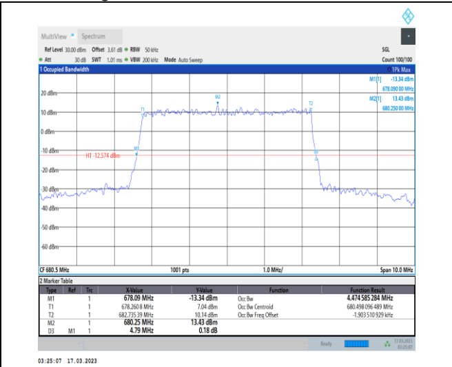
1-N71-PC3-15-5-M-1-DFT-QPSK-Outer_Full-25@0-Ant7-4.475-4.790-≤5-PASS
