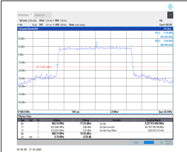
1-N71-PC3-15-10-L-6-CP-QPSK-Outer_Full-52@0-A Ant7-9.258-9.740-≤10-PASS
