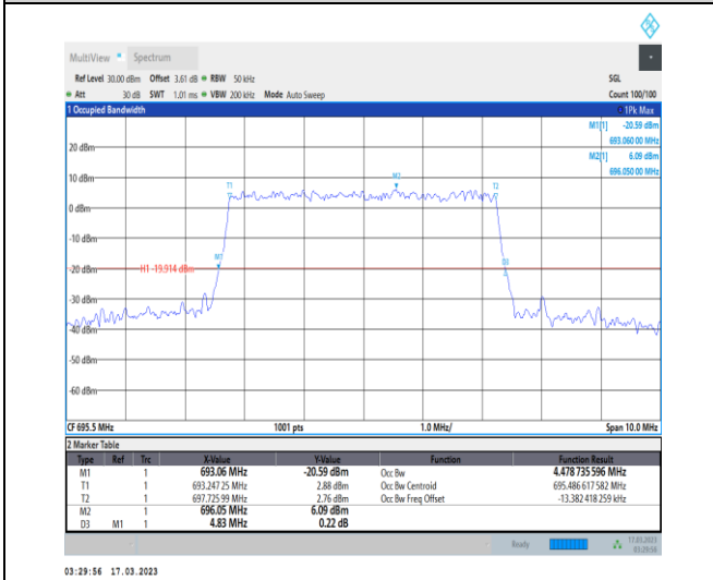
1-N71-PC3-15-5-H-9-CP-256QAM-Outer_Full-25@0-Ant7-4.479-4.830-≤5-PASS
