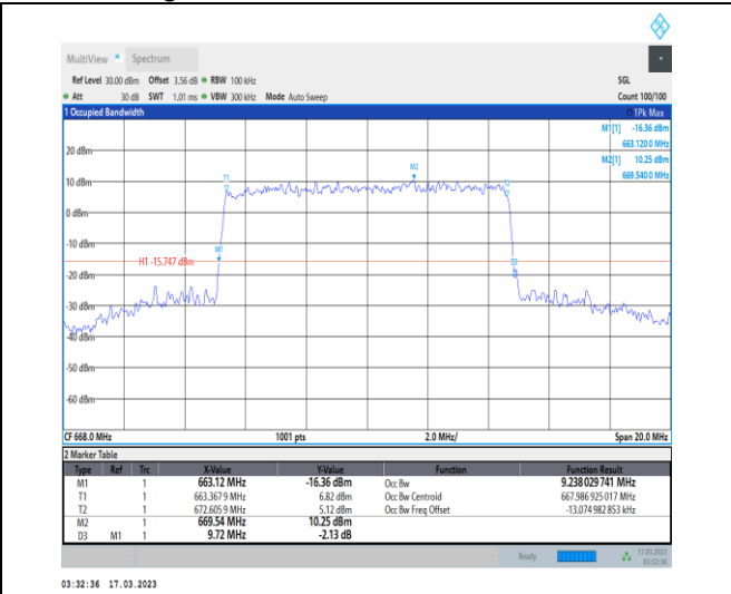
1-N71-PC3-15-10-L-7-CP-16QAM-Outer_Full-52@0- Ant7-9.238-9.720-≤10-PASS
