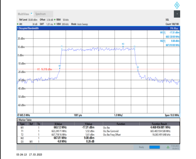
1-N71-PC3-15-5-L-8-CP-64QAM-Outer_Full-25@0-Ant7-4.468-4.800-<math>\leq</math>5-PASS
