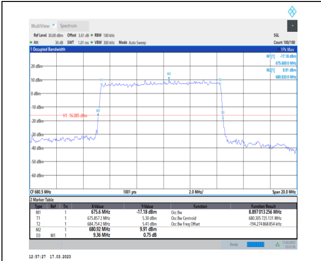
1-N71-PC3-15-10-M-5-DFT-256QAM-Outer_Full-50@0-Ant7-8.897-9.360-≤10-PASS
