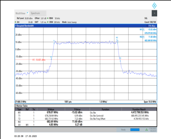
1-N71-PC3-15-5-M-3-DFT-16QAM-Outer_Full-25@0-Ant7-4.473-4.850-≤5-PASS
