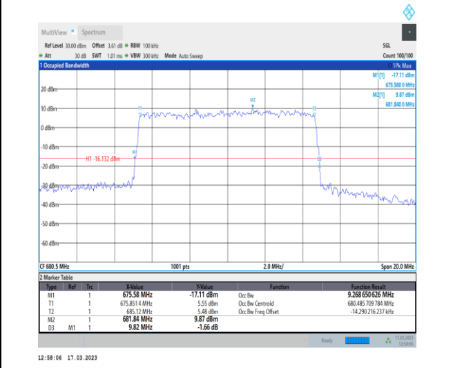
1-N71-PC3-15-10-M-8-CP-64QAM-Outer_Full-52@0-Ant7-9.269-9.820-≤10-PASS
