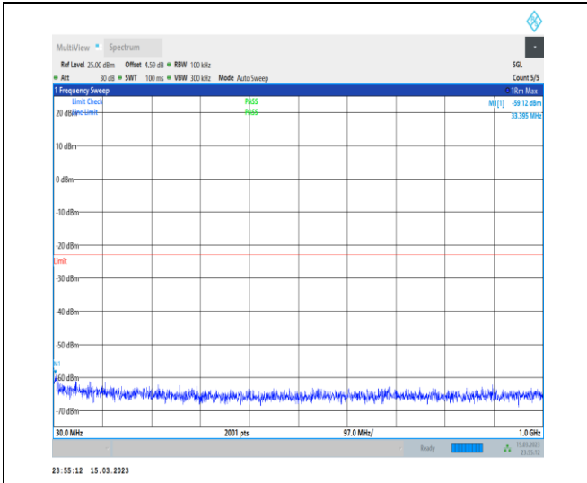
1-N70-PC3-15-15-H-1-DFT-PI2BPSK-Inner_1RB_Le ft-1@1-30-1000-Ant7-33.40--59.12--23-PASS
