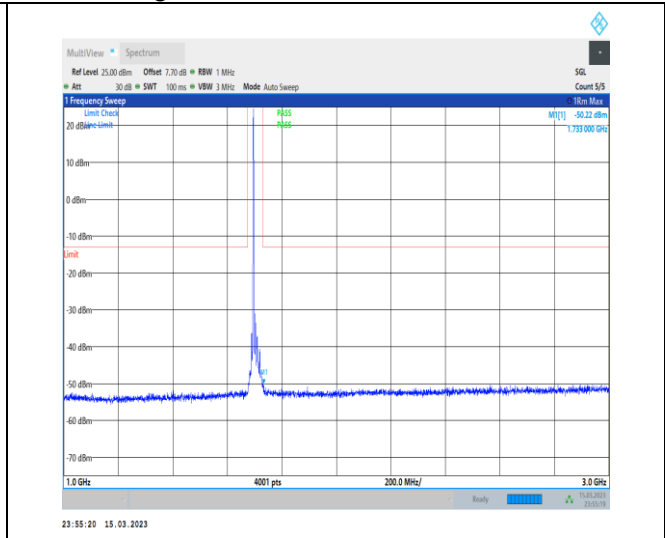
1-N70-PC3-15-15-H-1-DFT-PI2BPSK-Inner_1RB_Le ft-1@1-1000-3000-Ant7-1733.00--50.22--13-PASS
