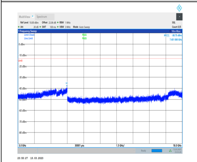
1-N70-PC3-15-15-H-1-DFT-PI2BPSK-Inner_1RB_Le ft-1@1-3000-18000-Ant7-7451.00--38.75--13-PASS
