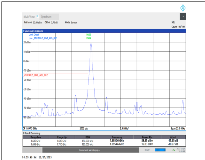
1-N70-15-15-L-1-DFT-PI2BPSK-Edge_1RB_Left-1@0-Ant7-1-seegraph-PASS-see graph
