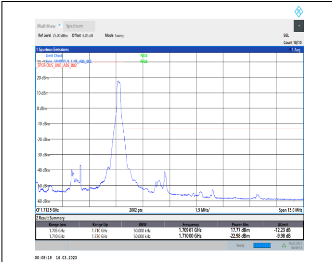
1-N70-PC3-15-5-H-2-DFT-PI2BPSK-Edge_1RB_Right-1@24-Ant7-1-seegraph-PASS-see graph
