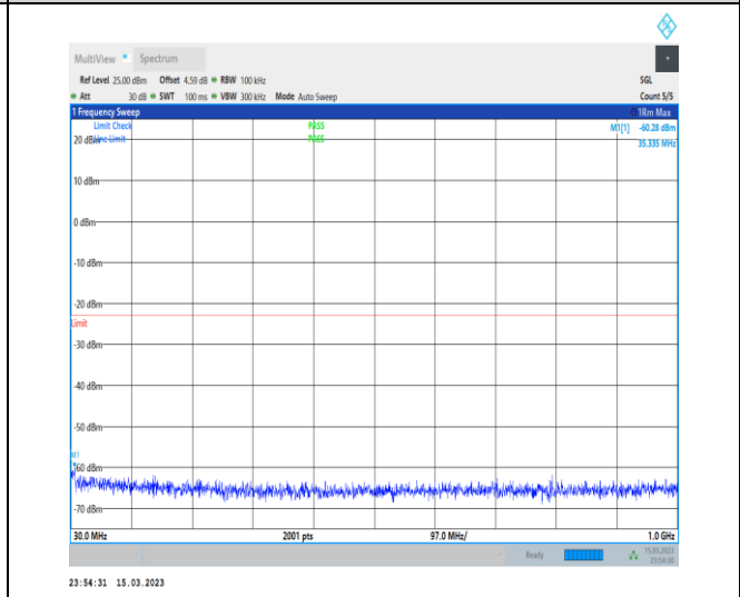
1-N70-PC3-15-15-M-1-DFT-PI2BPSK-Inner_1RB_Le ft-1@1-30-1000-Ant7-35.34--60.28--23-PASS
