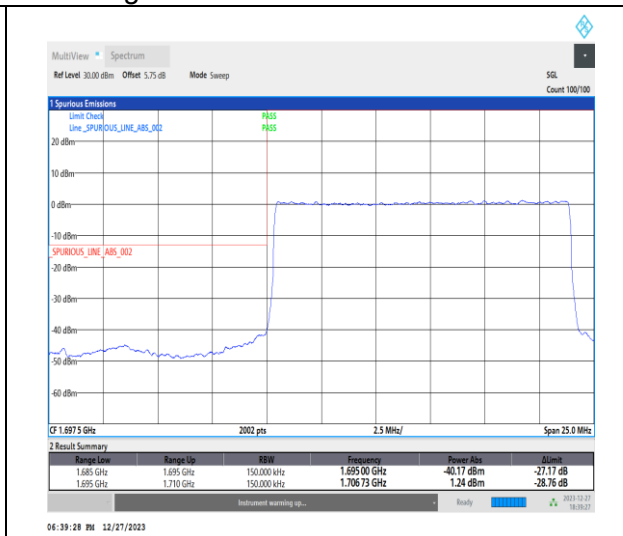
1-N70-15-15-L-3-DFT-PI2BPSK-Outer_Full-75@0-Ant7-1-seegraph-PASS-see graph
