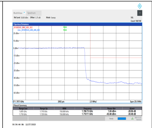
1-N70-15-15-H-3-DFT-PI2BPSK-Outer_Full-75@0-Ant7-1-seegraph-PASS-see graph
