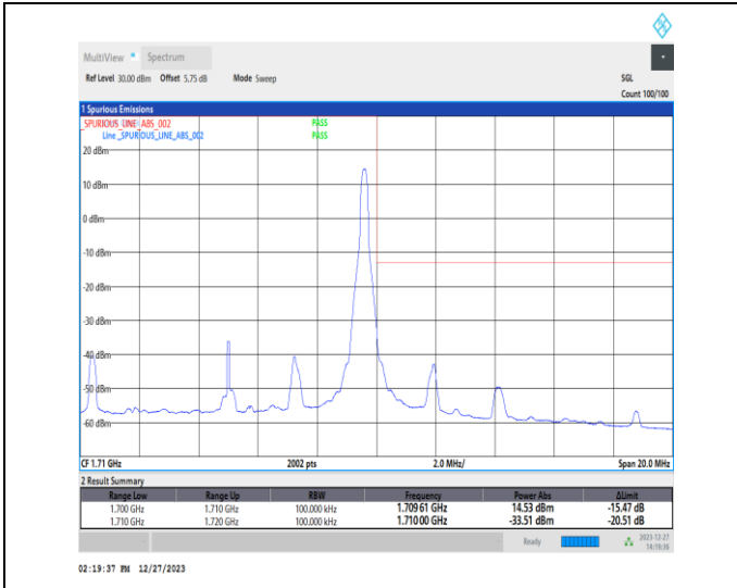
1-N70-15-10-H-2-DFT-PI2BPSK-Edge_1RB_Right-1@51-Ant7-1-seegraph-PASS-see graph
