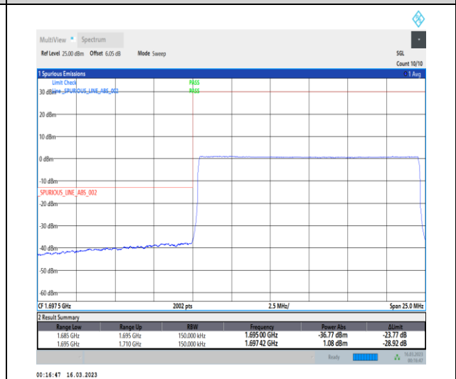
1-N70-PC3-15-15-L-6-CP-QPSK-Outer_Full-79@0-Ant7-1-seegraph-PASS-see graph
