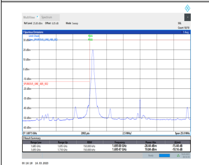
1-N70-PC3-15-15-L-4-CP-QPSK-Edge_1RB_Left-1@0-Ant7-1-seegraph-PASS-see graph
