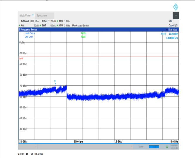
1-N70-PC3-15-15-M-1-DFT-PI2BPSK-Inner_1RB_Le ft-1@1-3000-18000-Ant7-6424.50--39.02--13-PASS
