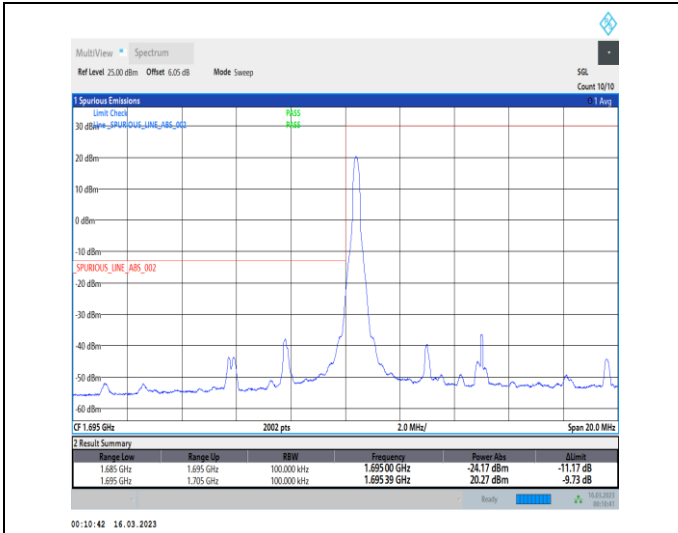
1-N70-PC3-15-10-L-1-DFT-PI2BPSK-Edge_1RB_Left-1@0-Ant7-1-seegraph-PASS-see graph
