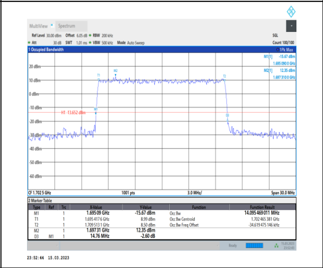
1-N70-PC3-15-15-H-8-CP-64QAM-Outer_Full-79@0 -Ant7-14.095-14.760-≤15-PASS
