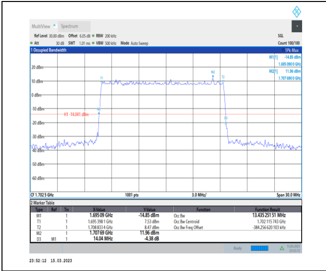
1-N70-PC3-15-15-H-5-DFT-256QAM-Outer_Full-75 @0-Ant7-13.435-14.040-≤15-PASS
