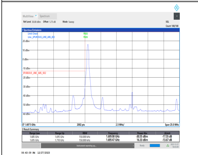
1-N70-15-15-L-4-CP-QPSK-Edge_1RB_Left-1@0-Ant7-1-seegraph-PASS-see graph
