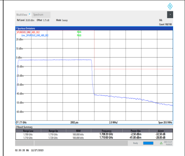
1-N70-15-10-H-6-CP-QPSK-Outer_Full-52@0-Ant7-1-seegraph-PASS-see graph
