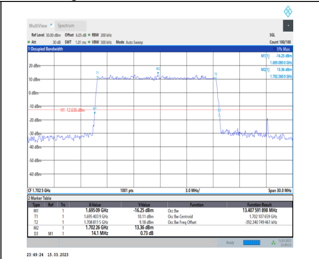
1-N70-PC3-15-15-M-3-DFT-16QAM-Outer_Full-75 @0-Ant7-13.408-14.100-≤15-PASS
