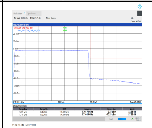
1-N70-15-15-H-6-CP-QPSK-Outer_Full-79@0-Ant7-1-seegraph-PASS-see graph
