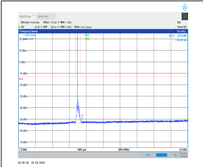
1-N70-PC3-15-15-M-1-DFT-PI2BPSK-Inner_1RB_Le ft-1@1-1000-3000-Ant7-1750.50--50.18--13-PASS
