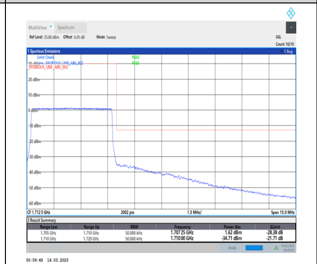
1-N70-PC3-15-5-H-6-CP-QPSK-Outer_Full-25@0-Ant7-1-seegraph-PASS-see graph
