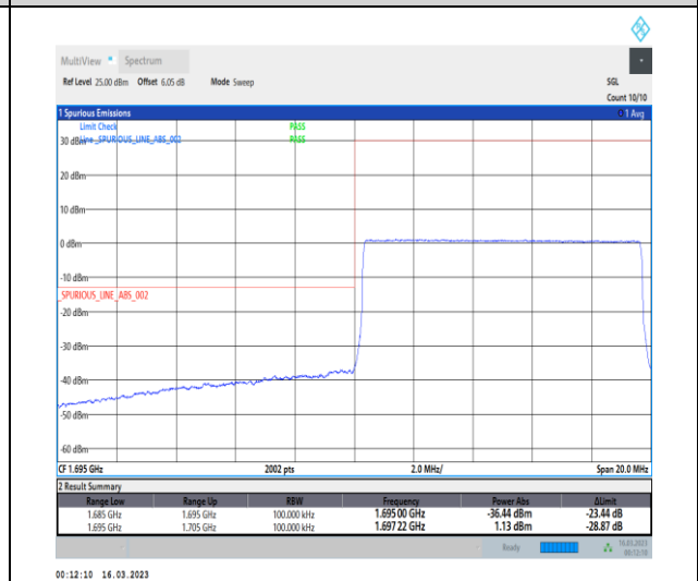
1-N70-PC3-15-10-L-6-CP-QPSK-Outer_Full-52@0-Ant7-1-seegraph-PASS-see graph
