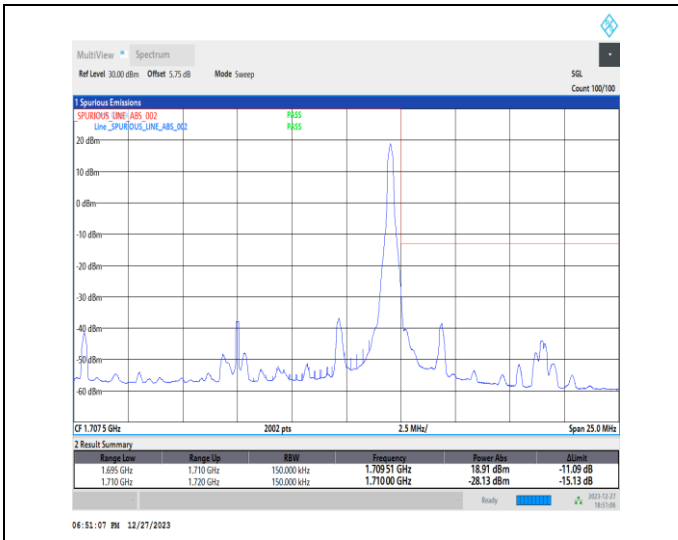
1-N70-15-15-H-2-DFT-PI2BPSK-Edge_1RB_Right-1@78-Ant7-1-seegraph-PASS-see graph
