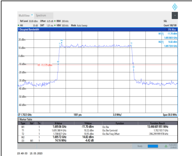
1-N70-PC3-15-15-M-2-DFT-PI2BPSK-Outer_Full-75 @0-Ant7-13.447-14.160-≤15-PASS
