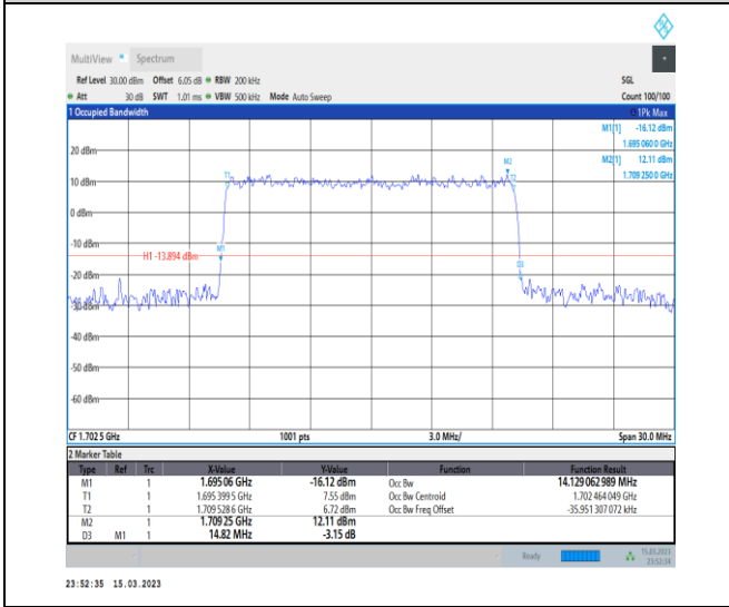
1-N70-PC3-15-15-H-7-CP-16QAM-Outer_Full-79@0 -Ant7-14.129-14.820-≤15-PASS
