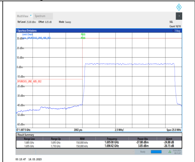
1-N70-PC3-15-15-L-3-DFT-PI2BPSK-Outer_Full-75@0-Ant7-1-seegraph-PASS-see graph
