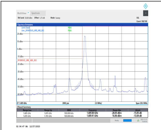
1-N70-15-10-L-1-DFT-PI2BPSK-Edge_1RB_Left-1@0-Ant7-1-seegraph-PASS-see graph
