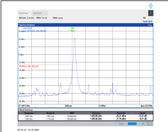
1-N70-PC3-15-15-L-1-DFT-PI2BPSK-Edge_1RB_Left-1@0-Ant7-1-seegraph-PASS-see graph
