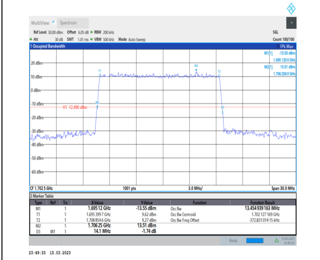
1-N70-PC3-15-15-M-4-DFT-64QAM-Outer_Full-75 @0-Ant7-13.455-14.100-≤15-PASS
