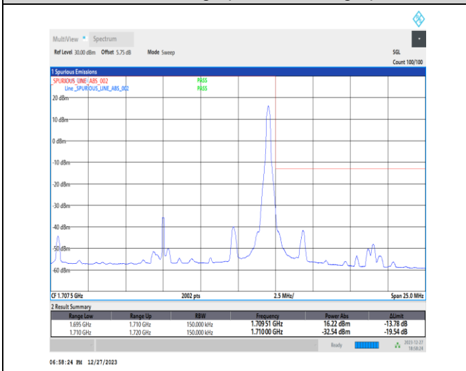
1-N70-15-15-H-5-CP-QPSK-Edge_1RB_Right-1@78-Ant7-1-seegraph-PASS-see graph
