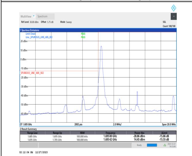
1-N70-15-10-L-4-CP-QPSK-Edge_1RB_Left-1@0-Ant7-1-seegraph-PASS-see graph
