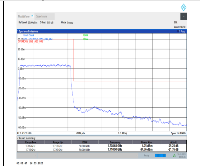
1-N70-PC3-15-5-H-3-DFT-PI2BPSK-Outer_Full-25@0-Ant7-1-seegraph-PASS-see graph
