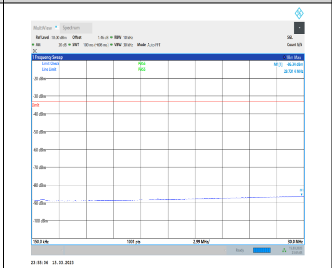
1-N70-PC3-15-15-H-1-DFT-PI2BPSK-Inner_1RB_Le ft-1@1-0.15-30-Ant7-29.73--86.34--33-PASS
