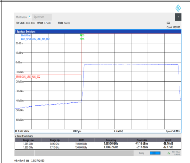
1-N70-15-15-L-6-CP-QPSK-Outer_Full-79@0-Ant7-1-seegraph-PASS-see graph
