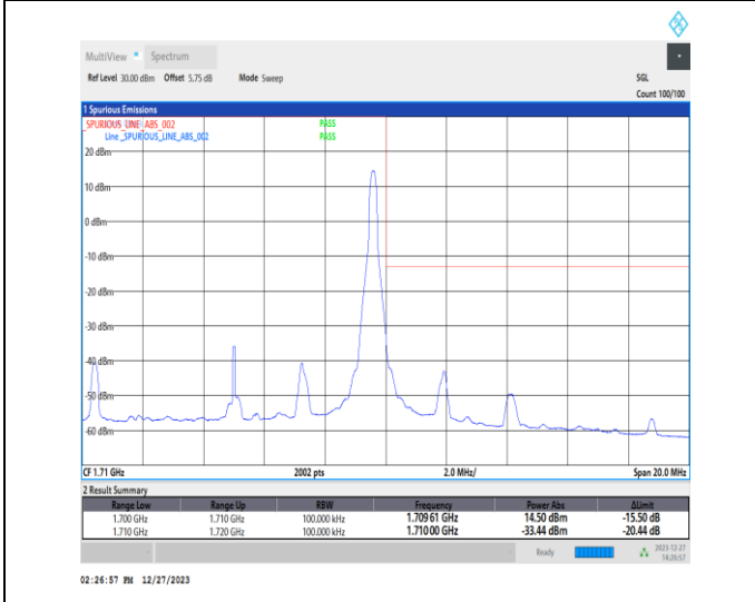
1-N70-15-10-H-5-CP-QPSK-Edge_1RB_Right-1@51-Ant7-1-seegraph-PASS-see graph
