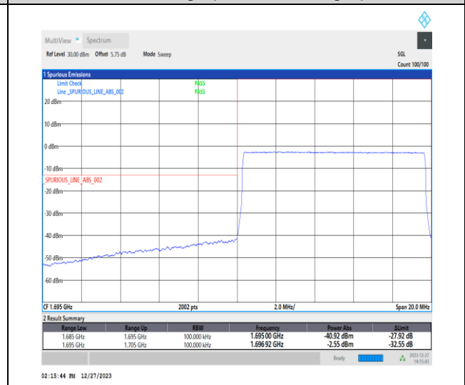
1-N70-15-10-L-6-CP-QPSK-Outer_Full-52@0-Ant7-1-seegraph-PASS-see graph
