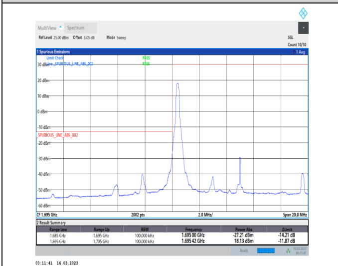
1-N70-PC3-15-10-L-4-CP-QPSK-Edge_1RB_Left-1@0-Ant7-1-seegraph-PASS-see graph
