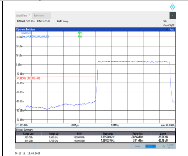
1-N70-PC3-15-10-L-3-DFT-PI2BPSK-Outer_Full-50@0-Ant7-1-seegraph-PASS-see graph
