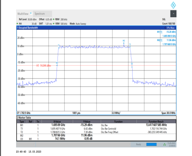
1-N70-PC3-15-15-M-5-DFT-256QAM-Outer_Full-75 @0-Ant7-13.418-14.100-≤15-PASS
