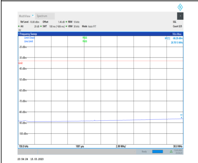
1-N70-PC3-15-15-M-1-DFT-PI2BPSK-Inner_1RB_Le ft-1@1-0.15-30-Ant7-29.70--86.28--33-PASS
