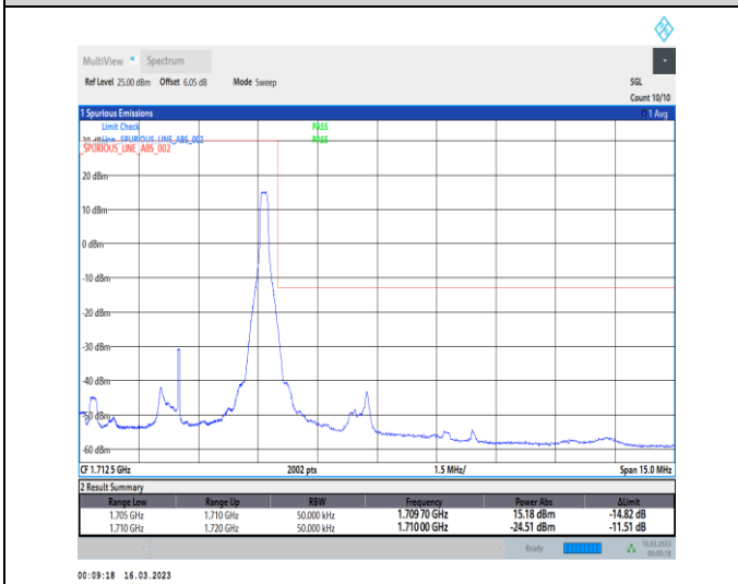
1-N70-PC3-15-5-H-5-CP-QPSK-Edge_1RB_Right-1@24-Ant7-1-seegraph-PASS-see graph
