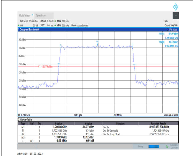
1-N70-PC3-15-10-H-2-DFT-PI2BPSK-Outer_Full-50 @0-Ant7-8.914-9.420-≤10-PASS
