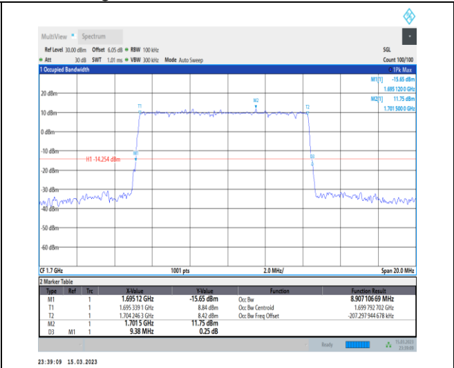
1-N70-PC3-15-10-L-3-DFT-16QAM-Outer_Full-50 @0-Ant7-8.907-9.380-≤10-PASS
