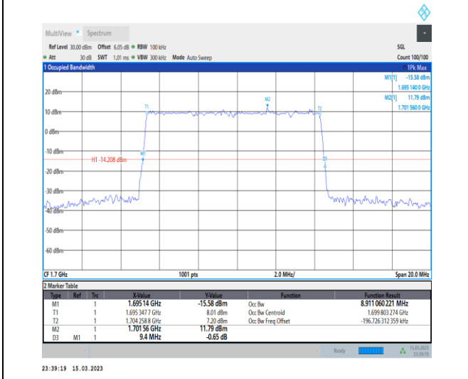
1-N70-PC3-15-10-L-4-DFT-64QAM-Outer_Full-50 @0-Ant7-8.911-9.400-≤10-PASS
