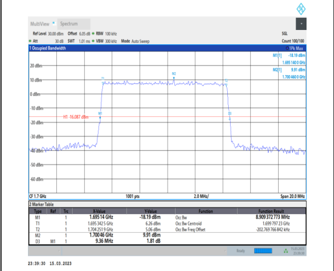
1-N70-PC3-15-10-L-5-DFT-256QAM-Outer_Full-50 @0-Ant7-8.909-9.360-≤10-PASS
