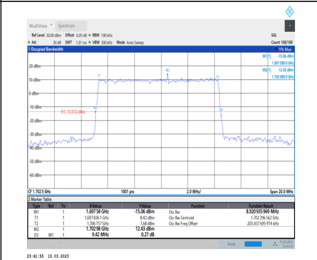
1-N70-PC3-15-10-M-4-DFT-64QAM-Outer_Full-50@0-Ant7-8.921-9.420-≤10-PASS
