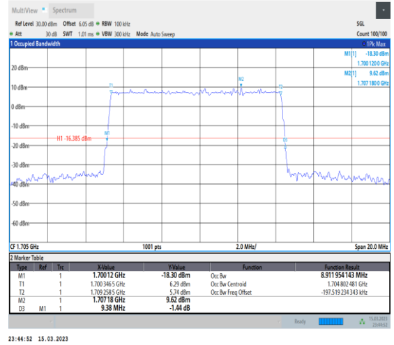
1-N70-PC3-15-10-H-5-DFT-256QAM-Outer_Full-50 @0-Ant7-8.912-9.380-≤10-PASS
