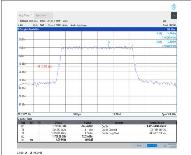
1-N70-PC3-15-5-H-1-DFT-QPSK-Outer_Full-25@0-Ant7-4.466-4.790-≤5-PASS
