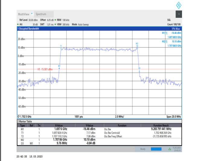
1-N70-PC3-15-10-M-8-CP-64QAM-Outer_Full-52@0-Ant7-9.284-9.760-≤10-PASS
