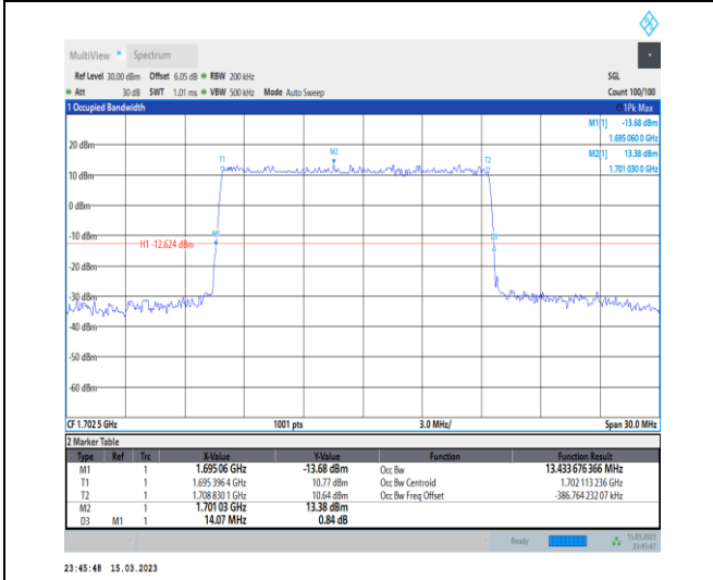
1-N70-PC3-15-15-L-1-DFT-QPSK-Outer_Full-75@0- Ant7-13.434-14.070-≤15-PASS
