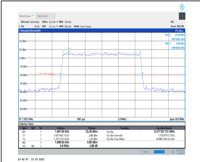
1-N70-PC3-15-10-M-9-CP-256QAM-Outer_Full-52@ 0-Ant7-9.272-9.800-≤10-PASS
