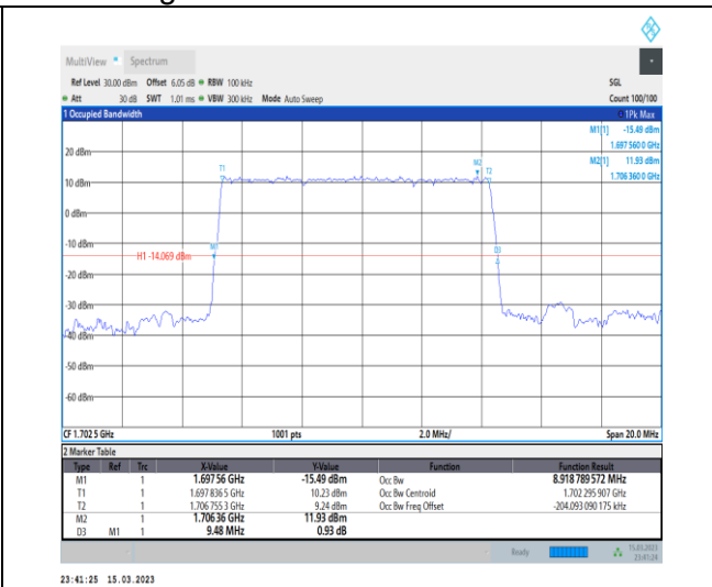
1-N70-PC3-15-10-M-2-DFT-PI2BPSK-Outer_Full-50@0-Ant7-8.919-9.480-≤10-PASS
