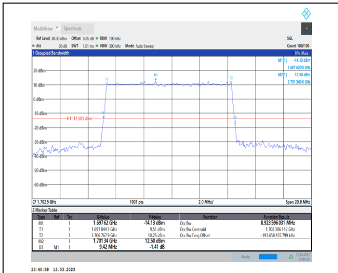
1-N70-PC3-15-10-M-1-DFT-QPSK-Outer_Full-50@0-Ant7-8.924-9.420-≤10-PASS
