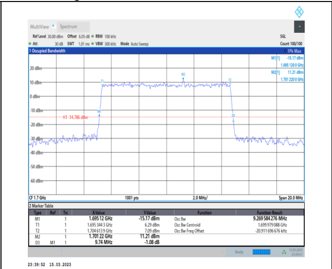
1-N70-PC3-15-10-L-7-CP-16QAM-Outer_Full-52@0- Ant7-9.27-9.740-≤10-PASS
