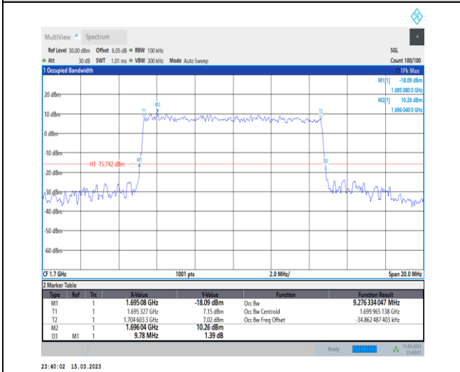
1-N70-PC3-15-10-L-8-CP-64QAM-Outer_Full-52@0- Ant7-9.276-9.780-≤10-PASS
