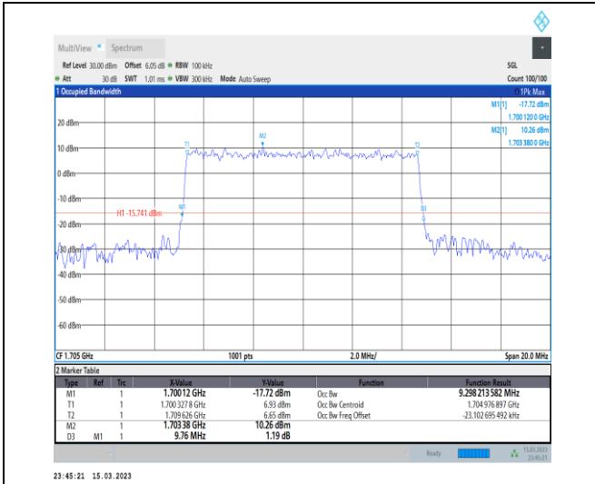
1-N70-PC3-15-10-H-8-CP-64QAM-Outer_Full-52@0 -Ant7-9.298-9.760-≤10-PASS
