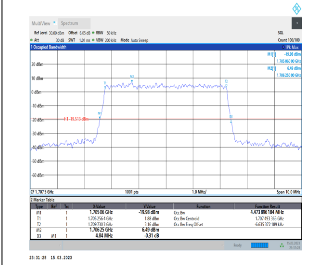
1-N70-PC3-15-5-H-9-CP-256QAM-Outer_Full-25@0-Ant7-4.474-4.840-≤5-PASS
