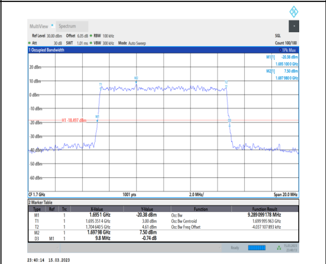
1-N70-PC3-15-10-L-9-CP-256QAM-Outer_Full-52@ 0-Ant7-9.289-9.800-≤10-PASS
