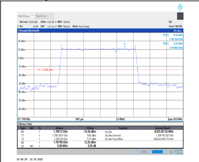
1-N70-PC3-15-10-H-1-DFT-QPSK-Outer_Full-50@ 0-Ant7-8.925-9.380-≤10-PASS
