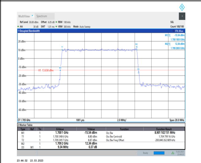
1-N70-PC3-15-10-H-3-DFT-16QAM-Outer_Full-50@ 0-Ant7-8.901-9.340-≤10-PASS
