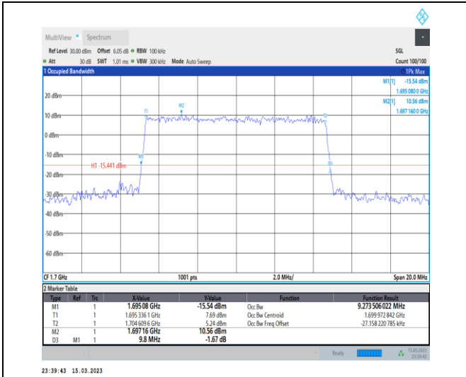
1-N70-PC3-15-10-L-6-CP-QPSK-Outer_Full-52@0-A Ant7-9.274-9.800-≤10-PASS
