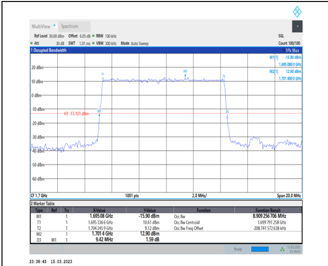
1-N70-PC3-15-10-L-2-DFT-PI2BPSK-Outer_Full-50 @0-Ant7-8.909-9.420-≤10-PASS
