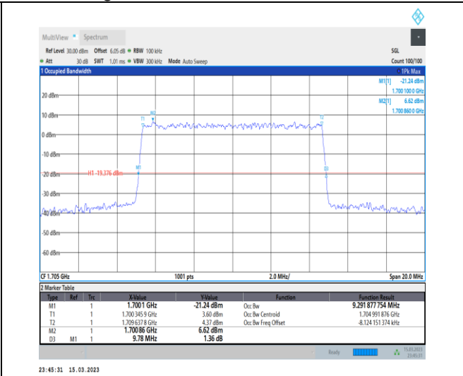
1-N70-PC3-15-10-H-9-CP-256QAM-Outer_Full-52@ 0-Ant7-9.292-9.780-≤10-PASS
