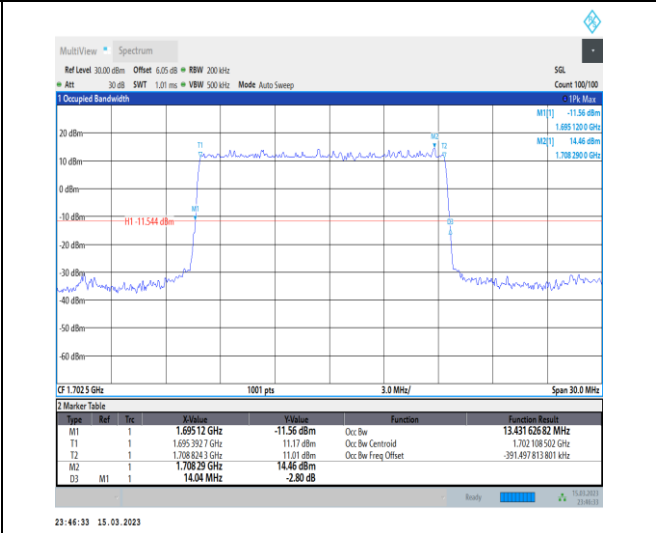
1-N70-PC3-15-15-L-2-DFT-PI2BPSK-Outer_Full-75 @0-Ant7-13.432-14.040-≤15-PASS
