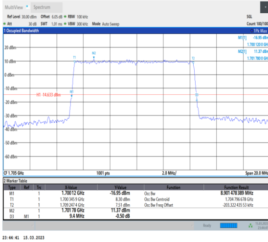
1-N70-PC3-15-10-H-4-DFT-64QAM-Outer_Full-50@ 0-Ant7-8.901-9.400-≤10-PASS
