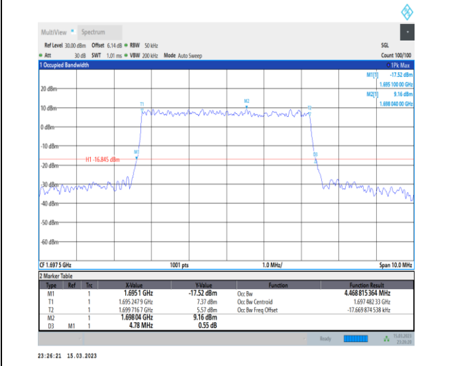
1-N70-PC3-15-5-L-8-CP-64QAM-Outer_Full-25@0-Ant7-4.469-4.780-≤5-PASS
