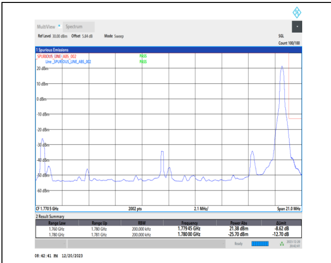
1-N66-15-20-H-2-DFT-PI2BPSK-Edge_1RB_Right-1@105-Ant1-1-seegraph-PASS-see graph
