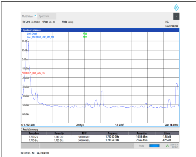
1-N66-15-40-L-1-DFT-PI2BPSK-Edge_1RB_Left-1@0-Ant1-1-seegraph-PASS-see graph
