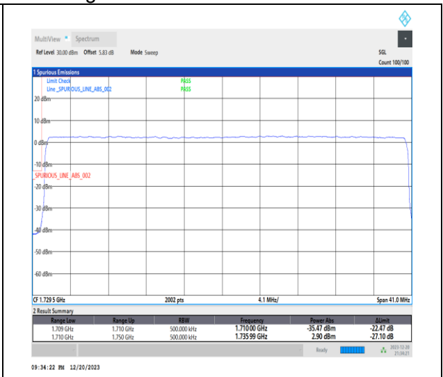
1-N66-15-40-L-3-DFT-PI2BPSK-Outer_Full-216@0-Ant1-1-seegraph-PASS-see graph
