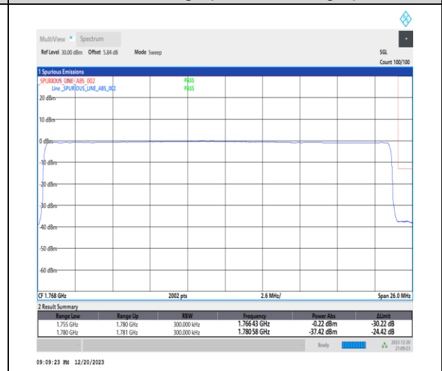
1-N66-15-25-H-6-CP-QPSK-Outer_Full-133@0-Ant1-1-seegraph-PASS-see graph
