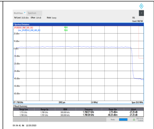
1-N66-15-25-H-3-DFT-PI2BPSK-Outer_Full-128@0-Ant1-1-seegraph-PASS-see graph
