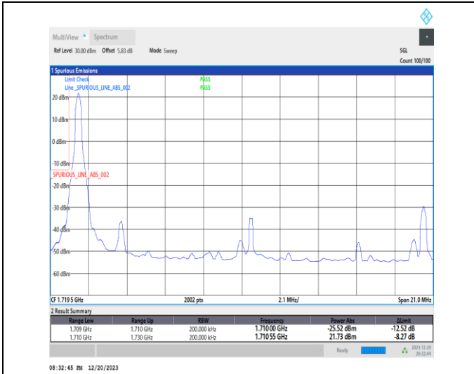
1-N66-15-20-L-1-DFT-PI2BPSK-Edge_1RB_Left-1@0-Ant1-1-seegraph-PASS-see graph
