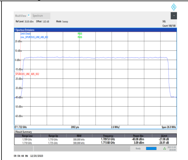
1-N66-15-25-L-3-DFT-PI2BPSK-Outer_Full-128@0-Ant1-1-seegraph-PASS-see graph
