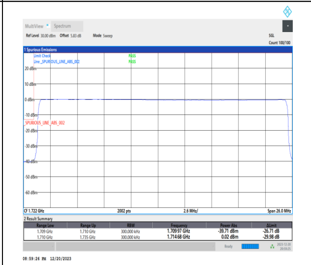
1-N66-15-25-L-6-CP-QPSK-Outer_Full-133@0-Ant1-1-seegraph-PASS-see graph
