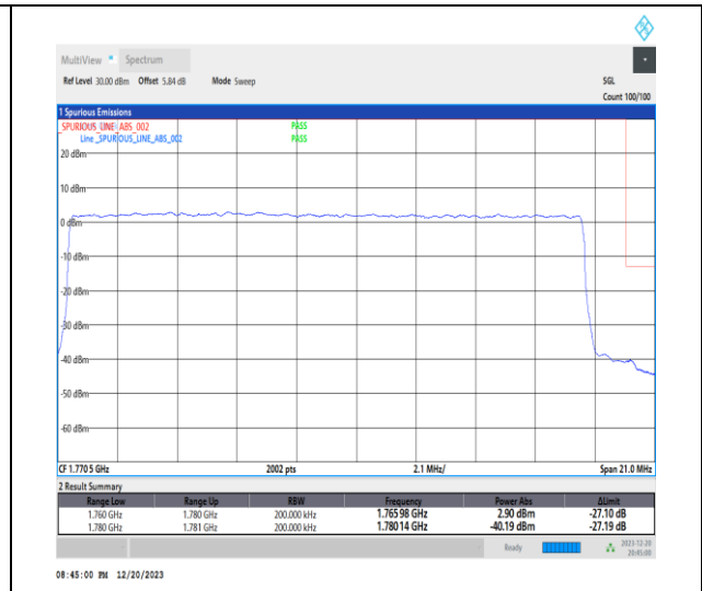
1-N66-15-20-H-3-DFT-PI2BPSK-Outer_Full-100@0-Ant1-1-seegraph-PASS-see graph
