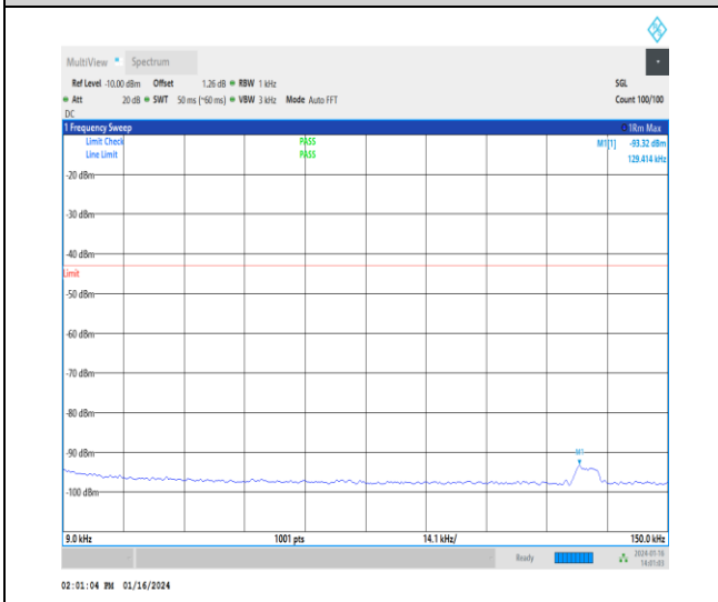
1-N66-15-40-M-1-DFT-PI2BPSK-Inner_1RB_Left-1 @ 1-0.009-0.15-Ant1-0.13--93.32--43-PASS
