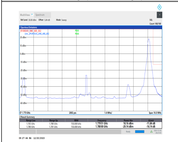
1-N66-15-15-H-5-CP-QPSK-Edge_1RB_Right-1@78-Ant1-1-seegraph-PASS-see graph
