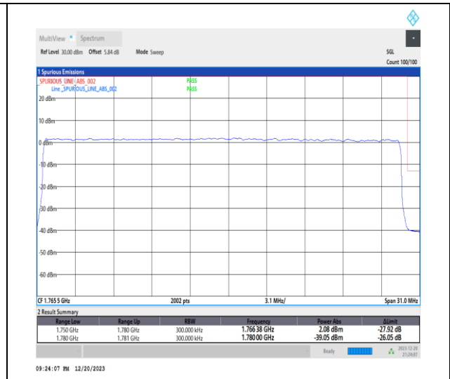
1-N66-15-30-H-3-DFT-PI2BPSK-Outer_Full-160@0-Ant1-1-seegraph-PASS-see graph
