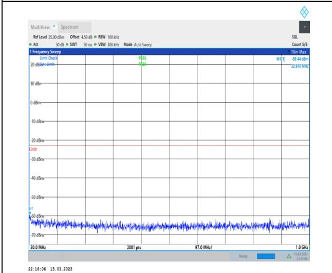
1-N66-PC3-15-40-H-1-DFT-PI2BPSK-Inner_1RB_L eft-1@1-30-1000-Ant1-32.91--59.44--23-PASS
