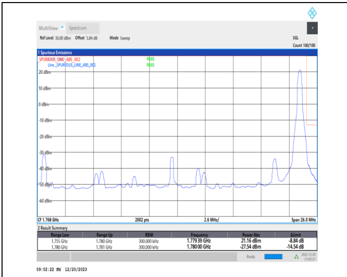
1-N66-15-25-H-2-DFT-PI2BPSK-Edge_1RB_Right-1@132-Ant1-1-seegraph-PASS-see graph
