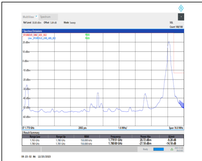
1-N66-15-15-H-2-DFT-PI2BPSK-Edge_1RB_Right-1@78-Ant1-1-seegraph-PASS-see graph
