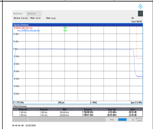
1-N66-15-20-H-6-CP-QPSK-Outer_Full-106@0-Ant1-1-seegraph-PASS-see graph
