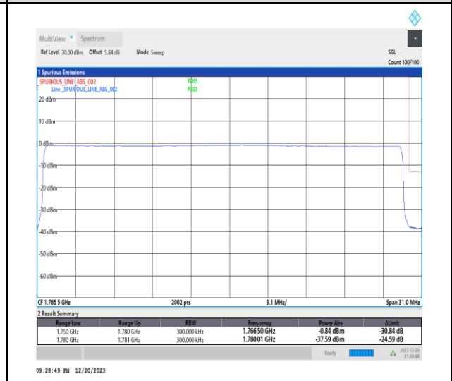
1-N66-15-30-H-6-CP-QPSK-Outer_Full-160@0-Ant1-1-seegraph-PASS-see graph
