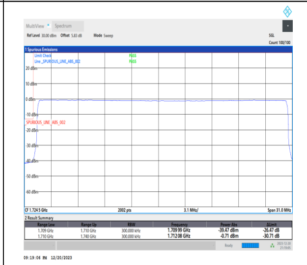
1-N66-15-30-L-6-CP-QPSK-Outer_Full-160@0-Ant1-1-seegraph-PASS-see graph
