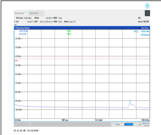
1-N66-15-40-H-1-DFT-PI2BPSK-Inner_1RB_Left-1 @1-0.009-0.15-Ant1-0.13--93.41--43-PASS
