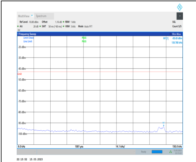
1-N66-PC3-15-40-H-1-DFT-PI2BPSK-Inner_1RB_L eft-1@1-0.009-0.15-Ant1-0.13--93.43--43-PASS
