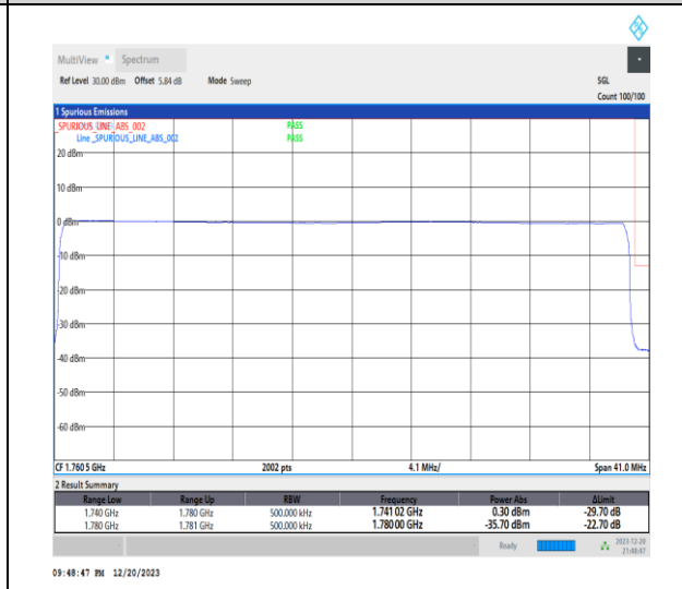
1-N66-15-40-H-6-CP-QPSK-Outer_Full-216@0-Ant1-1-seegraph-PASS-see graph
