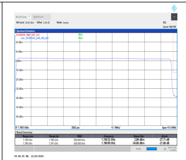
1-N66-15-40-H-3-DFT-PI2BPSK-Outer_Full-216@0-Ant1-1-seegraph-PASS-see graph
