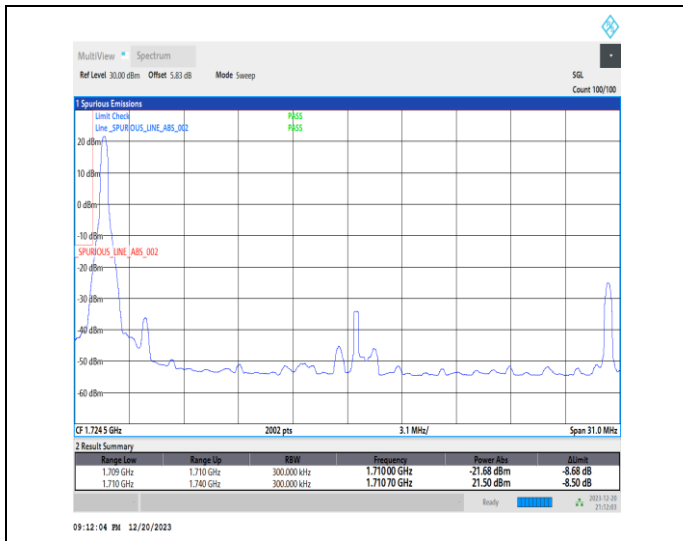
1-N66-15-30-L-1-DFT-PI2BPSK-Edge_1RB_Left-1@0-Ant1-1-seegraph-PASS-see graph
