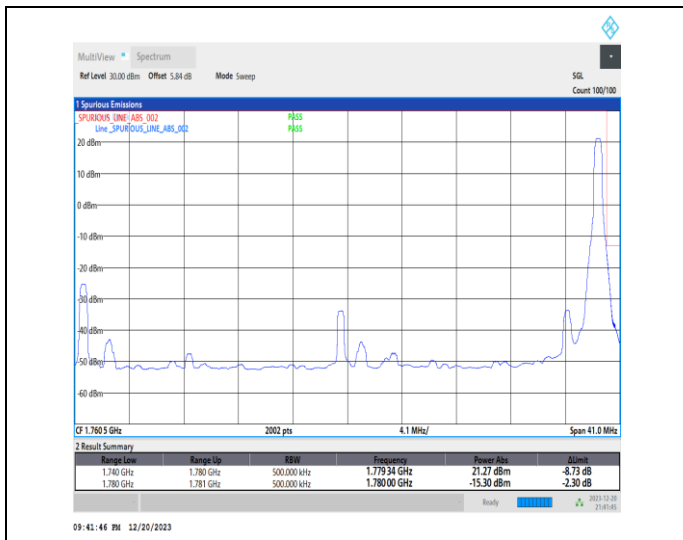
1-N66-15-40-H-2-DFT-PI2BPSK-Edge_1RB_Right-1@215-Ant1-1-seegraph-PASS-see graph
