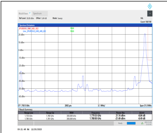
1-N66-15-30-H-2-DFT-PI2BPSK-Edge_1RB_Right-1@159-Ant1-1-seegraph-PASS-see graph
