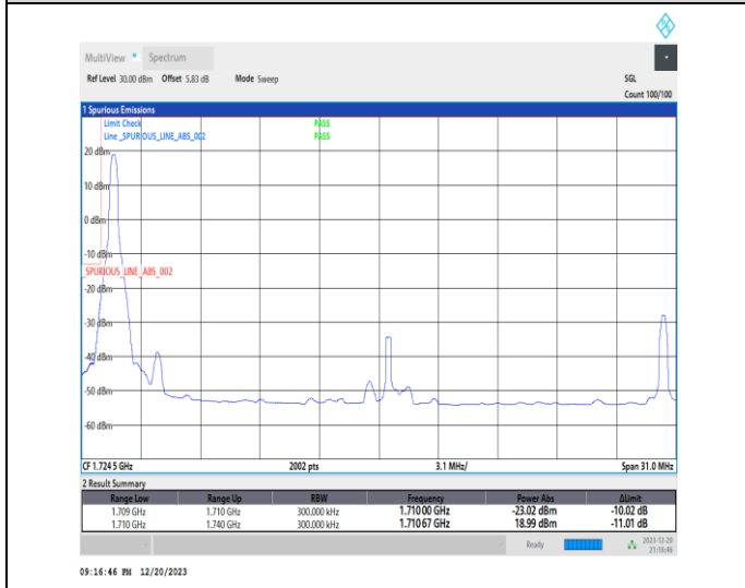
1-N66-15-30-L-4-CP-QPSK-Edge_1RB_Left-1@0-Ant1-1-seegraph-PASS-see graph
