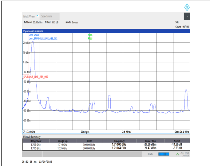
1-N66-15-25-L-1-DFT-PI2BPSK-Edge_1RB_Left-1@0-Ant1-1-seegraph-PASS-see graph
