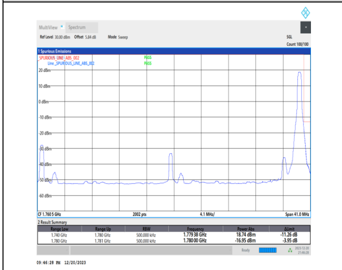
1-N66-15-40-H-5-CP-QPSK-Edge_1RB_Right-1@215-Ant1-1-seegraph-PASS-see graph
