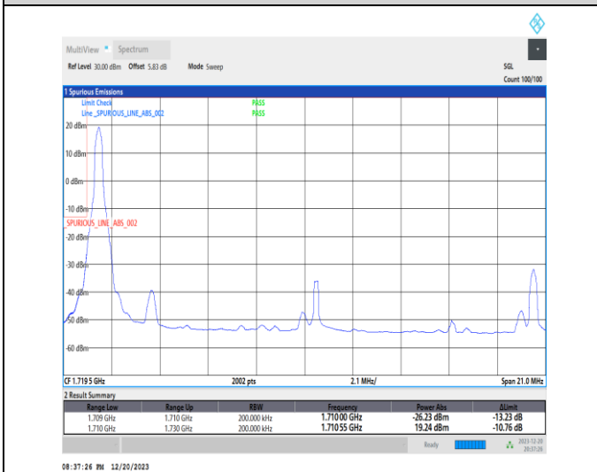
1-N66-15-20-L-4-CP-QPSK-Edge_1RB_Left-1@0-Ant1-1-seegraph-PASS-see graph
