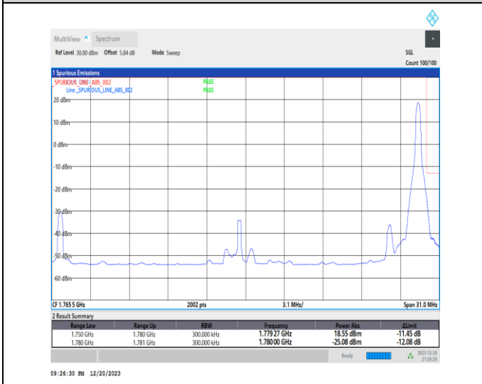
1-N66-15-30-H-5-CP-QPSK-Edge_1RB_Right-1@159-Ant1-1-seegraph-PASS-see graph
