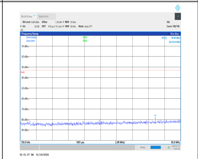
1-N66-15-40-M-1-DFT-PI2BPSK-Inner_1RB_Left-1@ 1-0.15-30-Ant1-28.93--79.69--33-PASS
