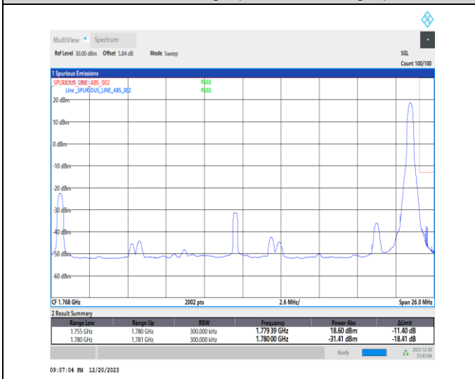
1-N66-15-25-H-5-CP-QPSK-Edge_1RB_Right-1@132-Ant1-1-seegraph-PASS-see graph
