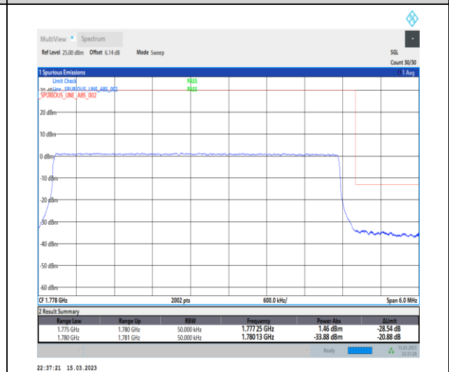
1-N66-PC3-15-5-H-6-CP-QPSK-Outer_Full-25@0-Ant1-1-seegraph-PASS-see graph
