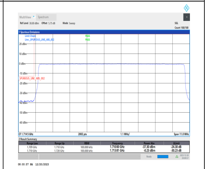
1-N66-15-10-L-6-CP-QPSK-Outer_Full-52@0-Ant1-1-seegraph-PASS-see graph
