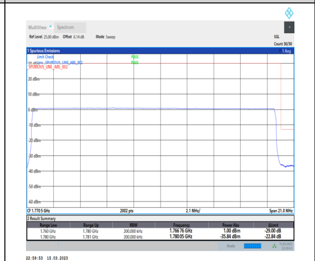
1-N66-PC3-15-20-H-6-CP-QPSK-Outer_Full-106@0-Ant1-1-seegraph-PASS-see graph
