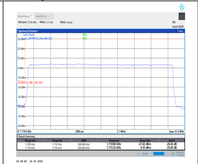
1-N66-PC3-15-20-L-3-DFT-PI2BPSK-Outer_Full-100@0-Ant1-1-seegraph-PASS-see graph
