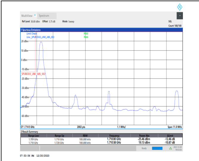
1-N66-15-10-L-1-DFT-PI2BPSK-Edge_1RB_Left-1@0-Ant1-1-seegraph-PASS-see graph
