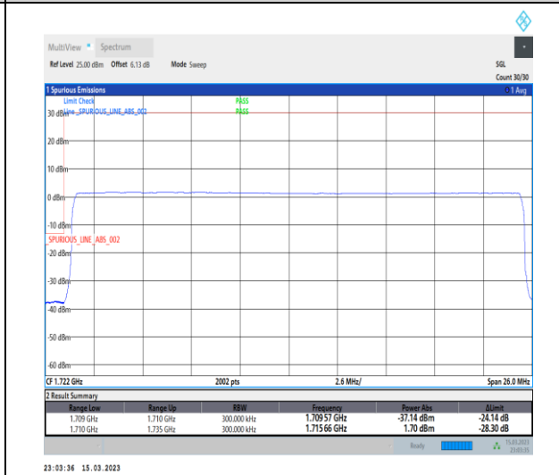
1-N66-PC3-15-25-L-6-CP-QPSK-Outer_Full-133@0-Ant1-1-seegraph-PASS-see graph
