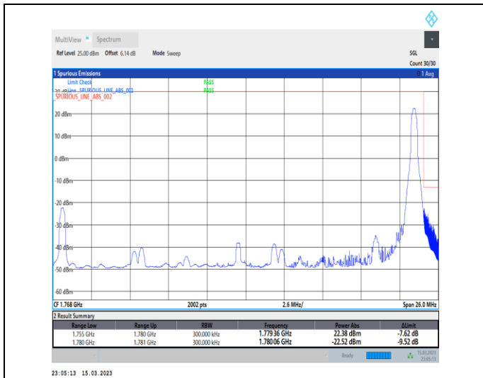
1-N66-PC3-15-25-H-2-DFT-PI2BPSK-Edge_1RB_Right-t-1@132-Ant1-1-seegraph-PASS-see graph
