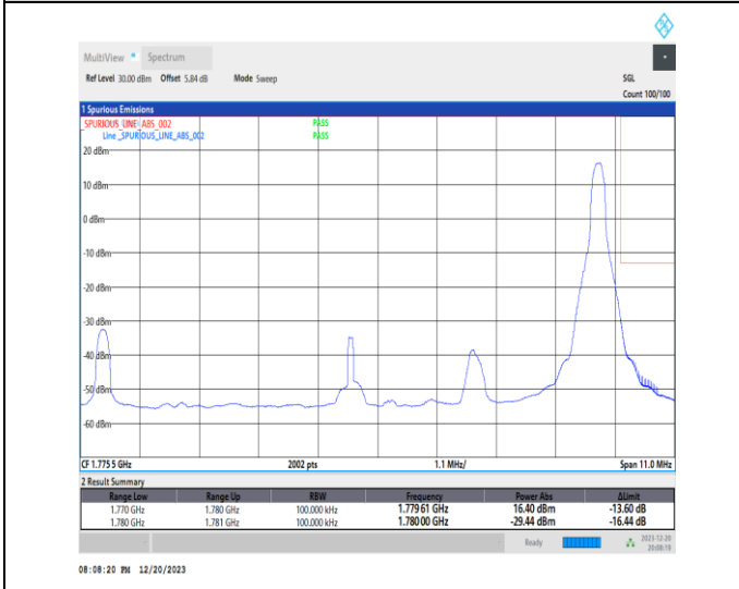
1-N66-15-10-H-5-CP-QPSK-Edge_1RB_Right-1@51-Ant1-1-seegraph-PASS-see graph
