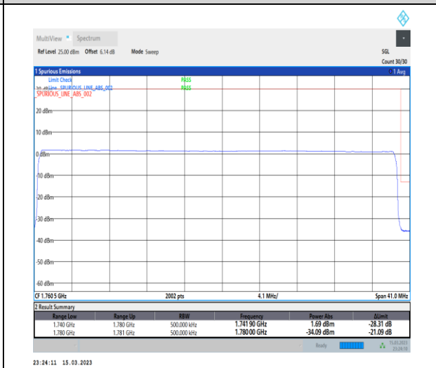
1-N66-PC3-15-40-H-6-CP-QPSK-Outer_Full-216@0-Ant1-1-seegraph-PASS-see graph
