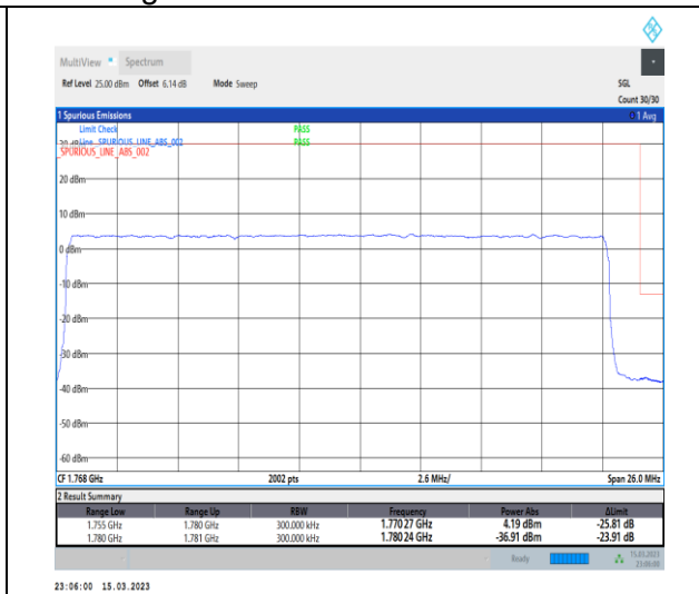
1-N66-PC3-15-25-H-3-DFT-PI2BPSK-Outer_Full-1-28@0-Ant1-1-seegraph-PASS-see graph
