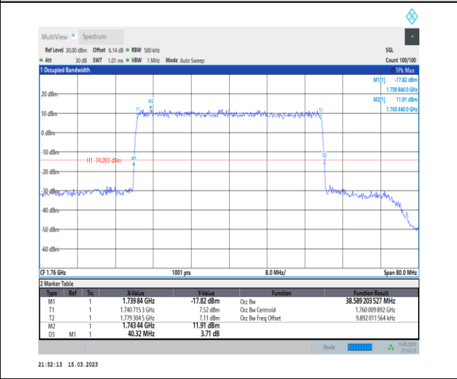
1-N66-PC3-15-40-H-4-DFT-64QAM-Outer_Full-216@0-Ant1-38.589-40.320-≤40-PASS
