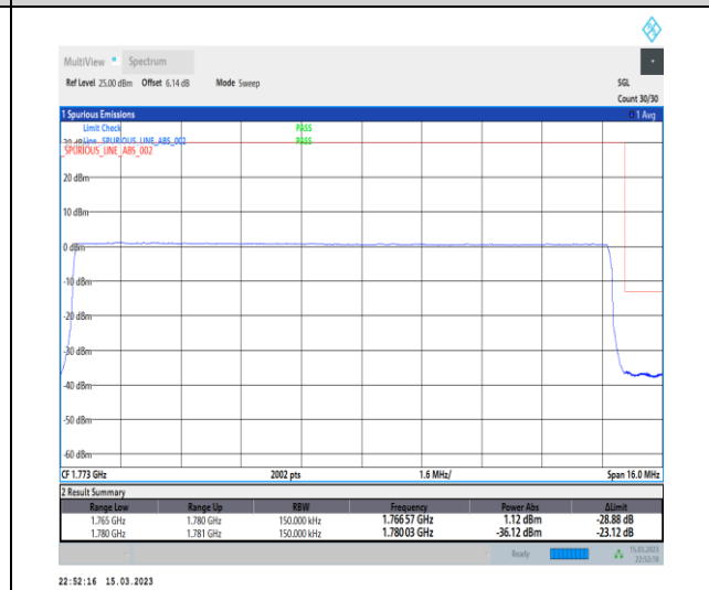
1-N66-PC3-15-15-H-6-CP-QPSK-Outer_Full-79@ 0-Ant1-1-seegraph-PASS-see graph
