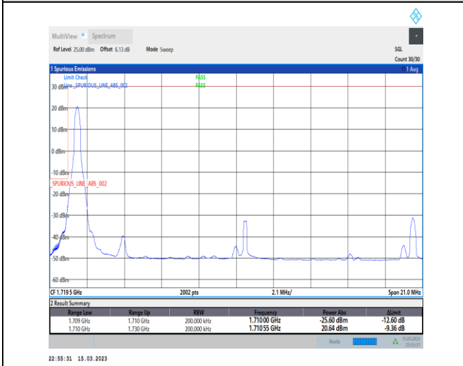
1-N66-PC3-15-20-L-4-CP-QPSK-Edge_1RB_Left-1@0-Ant1-1-seegraph-PASS-see graph
