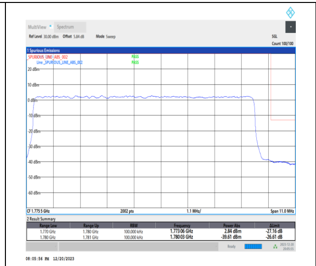
1-N66-15-10-H-3-DFT-PI2BPSK-Outer_Full-50@0-Ant1-1-seegraph-PASS-see graph
