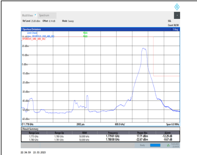
1-N66-PC3-15-5-H-2-DFT-PI2BPSK-Edge_1RB_Right-1@24-Ant1-1-seegraph-PASS-see graph
