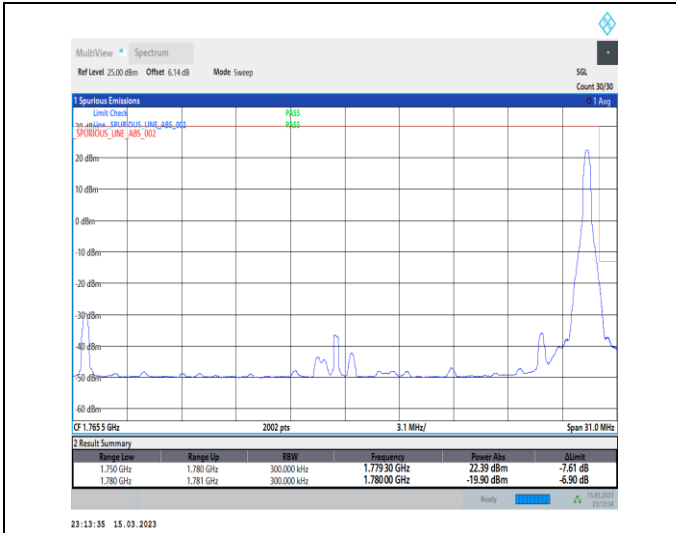
1-N66-PC3-15-30-H-2-DFT-PI2BPSK-Edge_1RB_Right-t-1@159-Ant1-1-seegraph-PASS-see graph
