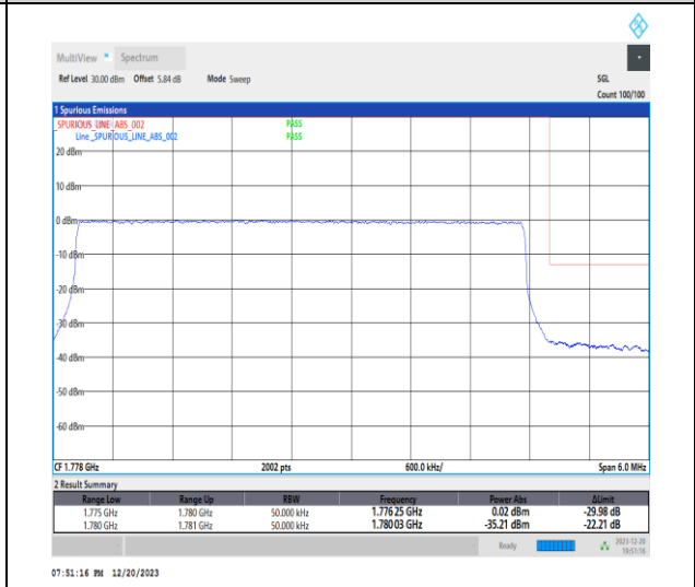
1-N66-15-5-H-6-CP-QPSK-Outer_Full-25@0-Ant1-1-seegraph-PASS-see graph
