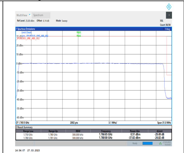
1-N66-PC3-15-30-H-3-DFT-PI2BPSK-Outer_Full-160@0-Ant1-1-seegraph-PASS-see graph
