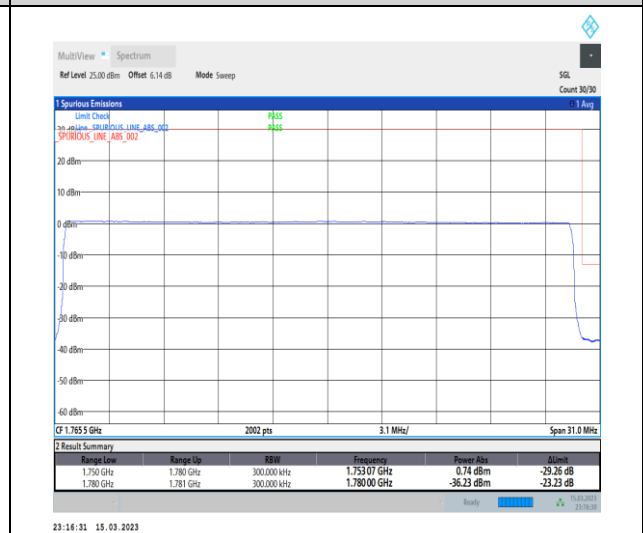
1-N66-PC3-15-30-H-6-CP-QPSK-Outer_Full-160@0-Ant1-1-seegraph-PASS-see graph
