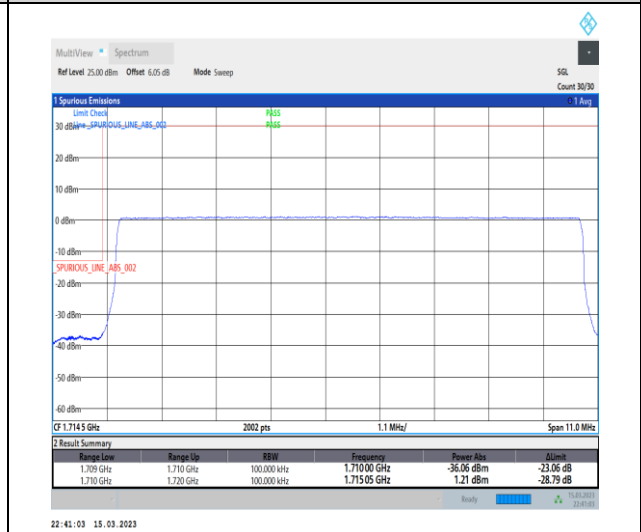
1-N66-PC3-15-10-L-6-CP-QPSK-Outer_Full-52@0-Ant1-1-seegraph-PASS-see graph
