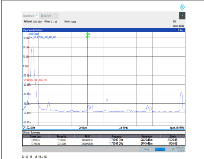
1-N66-PC3-15-25-L-4-CP-QPSK-Edge_1RB_Left-1@0-Ant1-1-seegraph-PASS-see graph
