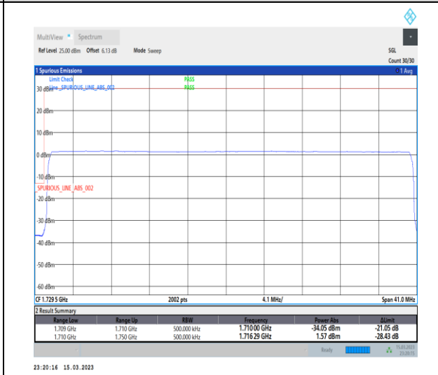
1-N66-PC3-15-40-L-6-CP-QPSK-Outer_Full-216@0-Ant1-1-seegraph-PASS-see graph
