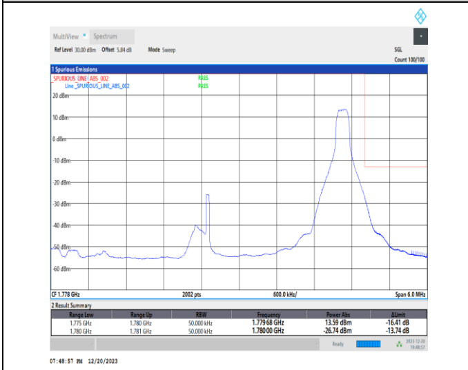
1-N66-15-5-H-5-CP-QPSK-Edge_1RB_Right-1@24-Ant1-1-seegraph-PASS-see graph
