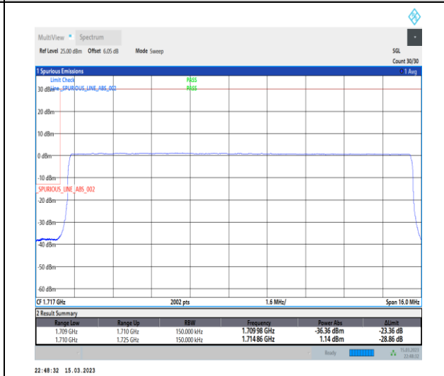
1-N66-PC3-15-15-L-6-CP-QPSK-Outer_Full-79@0-Ant1-1-seegraph-PASS-see graph
