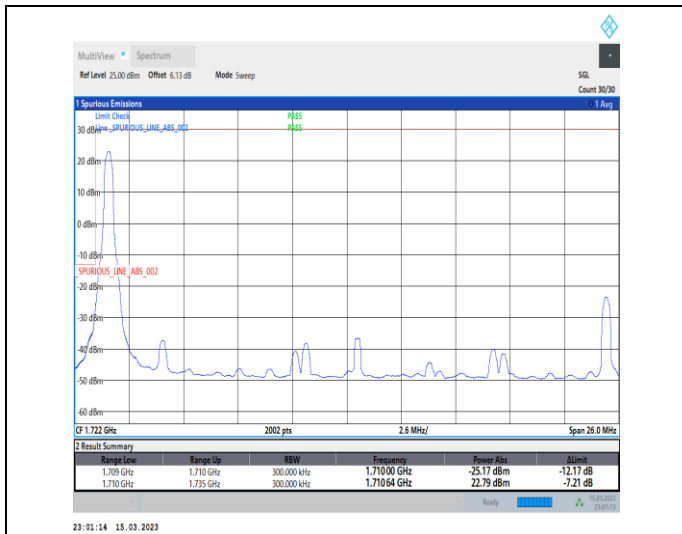
1-N66-PC3-15-25-L-1-DFT-PI2BPSK-Edge_1RB_Left-1@0-Ant1-1-seegraph-PASS-see graph
