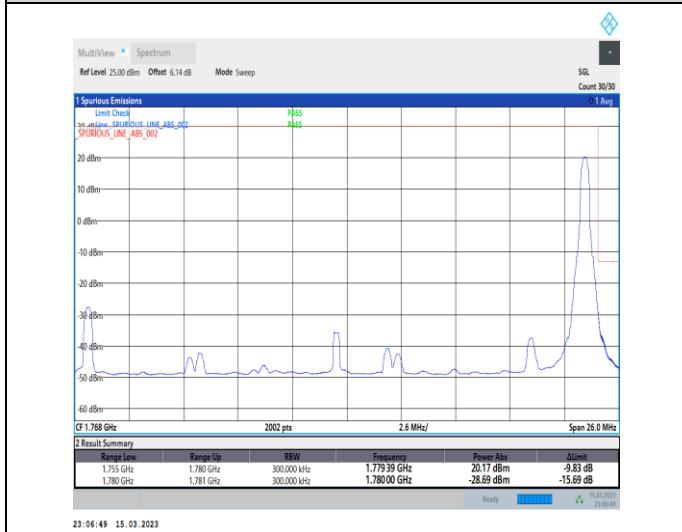
1-N66-PC3-15-25-H-5-CP-QPSK-Edge_1RB_Right-1@132-Ant1-1-seegraph-PASS-see graph
