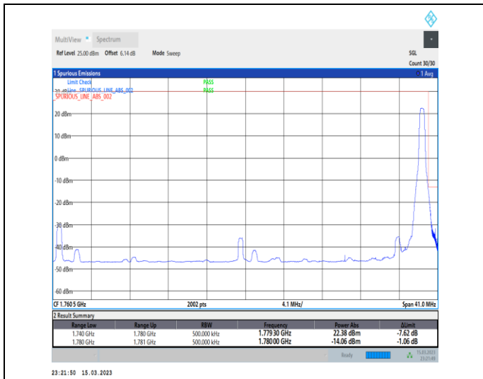
1-N66-PC3-15-40-H-2-DFT-PI2BPSK-Edge_1RB_Right-t-1@215-Ant1-1-seegraph-PASS-see graph
