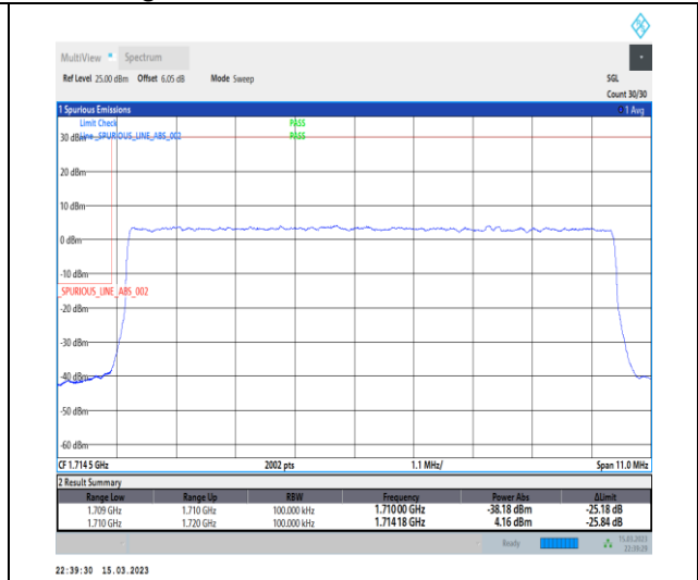
1-N66-PC3-15-10-L-3-DFT-PI2BPSK-Outer_Full-50@0-Ant1-1-seegraph-PASS-see graph
