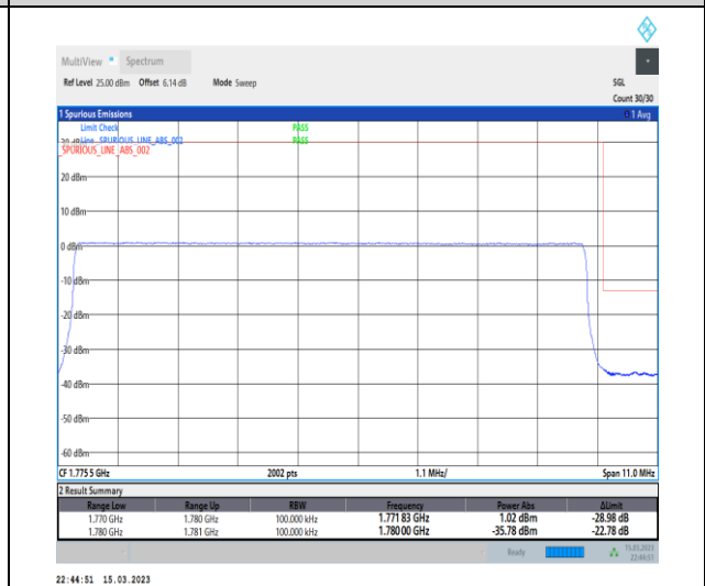
1-N66-PC3-15-10-H-6-CP-QPSK-Outer_Full-52@0-Ant1-1-seegraph-PASS-see graph
