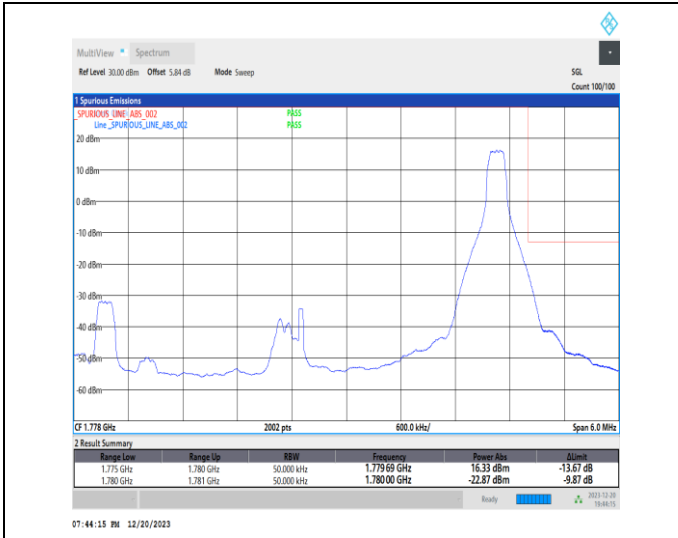
1-N66-15-5-H-2-DFT-PI2BPSK-Edge_1RB_Right-1@2 4-Ant1-1-seegraph-PASS-see graph
