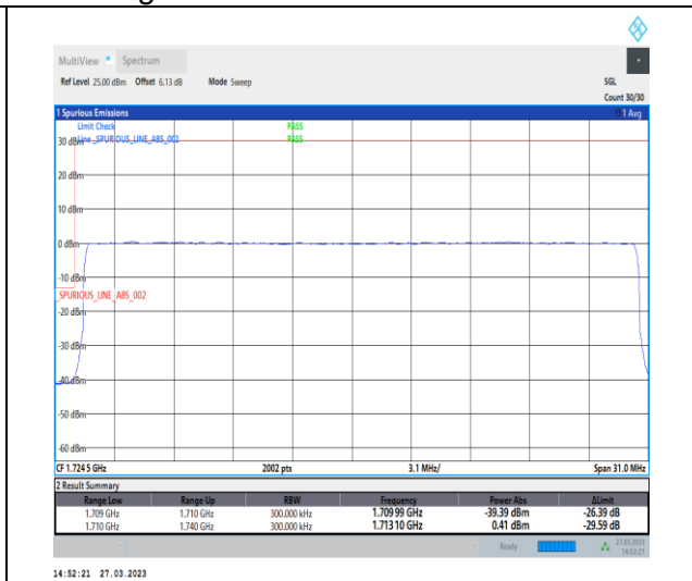
1-N66-PC3-15-30-L-3-DFT-PI2BPSK-Outer_Full-160@0-Ant1-1-seegraph-PASS-see graph
