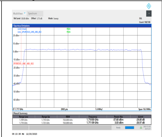
1-N66-15-15-L-3-DFT-PI2BPSK-Outer_Full-75@0-Ant1-1-seegraph-PASS-see graph
