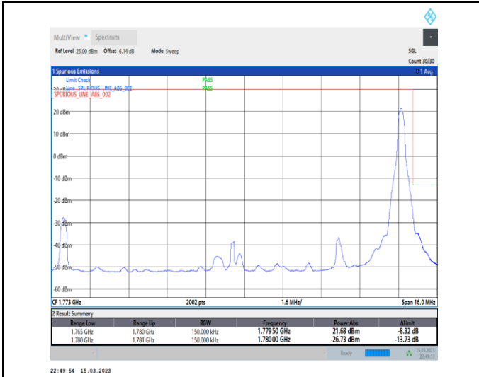
1-N66-PC3-15-15-H-2-DFT-PI2BPSK-Edge_1RB_Righ t-1@78-Ant1-1-seegraph-PASS-see graph
