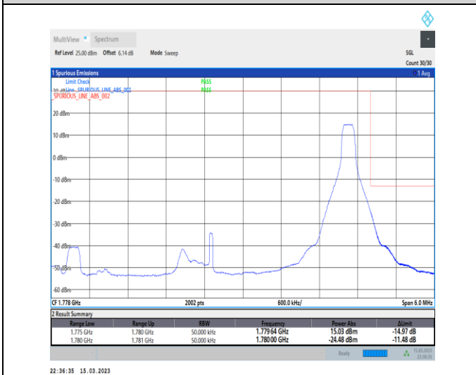
1-N66-PC3-15-5-H-5-CP-QPSK-Edge_1RB_Right-1@24-Ant1-1-seegraph-PASS-see graph
