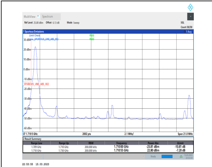
1-N66-PC3-15-20-L-1-DFT-PI2BPSK-Edge_1RB_Left-1@0-Ant1-1-seegraph-PASS-see graph
