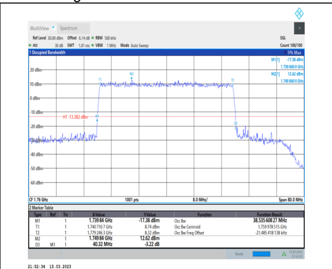
1-N66-PC3-15-40-H-6-CP-QPSK-Outer_Full-216@0 -Ant1-38.536-40.320-≤40-PASS
