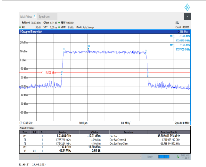
1-N66-PC3-15-40-M-8-CP-64QAM-Outer_Full-216@0 -Ant1-38.503-40.240-≤40-PASS
