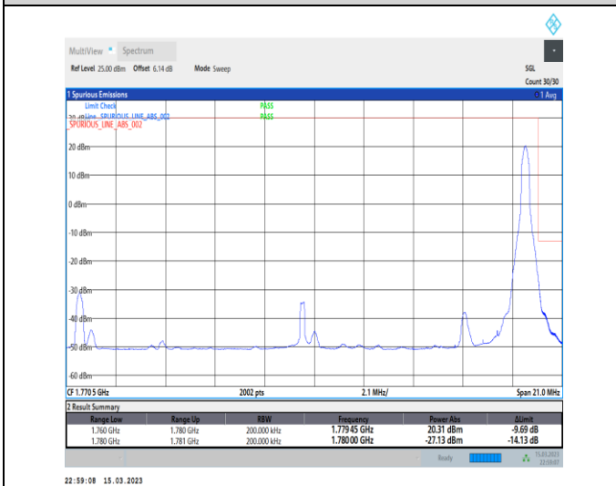
1-N66-PC3-15-20-H-5-CP-QPSK-Edge_1RB_Right-1@105-Ant1-1-seegraph-PASS-see graph
