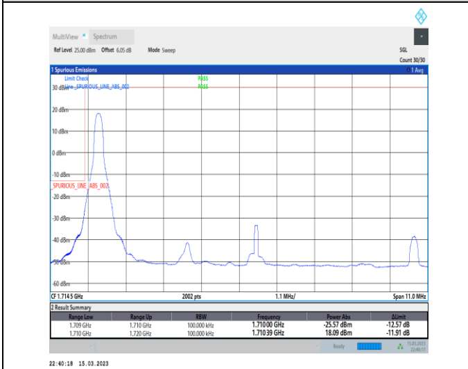
1-N66-PC3-15-10-L-4-CP-QPSK-Edge_1RB_Left-1@0-Ant1-1-seegraph-PASS-see graph
