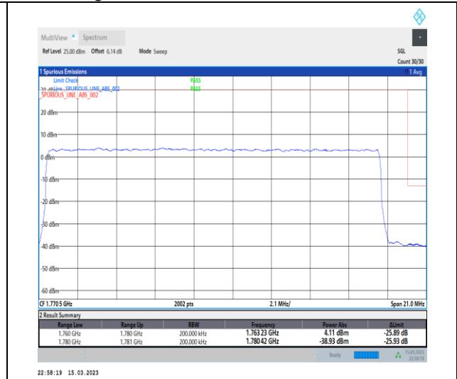
1-N66-PC3-15-20-H-3-DFT-PI2BPSK-Outer_Full-100@0-Ant1-1-seegraph-PASS-see graph
