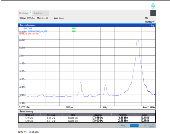
1-N66-PC3-15-10-H-2-DFT-PI2BPSK-Edge_1RB_Right-t@51-Ant1-1-seegraph-PASS-see graph
