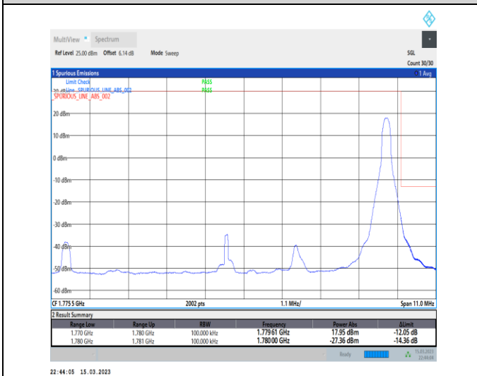
1-N66-PC3-15-10-H-5-CP-QPSK-Edge_1RB_Right-1@51-Ant1-1-seegraph-PASS-see graph
