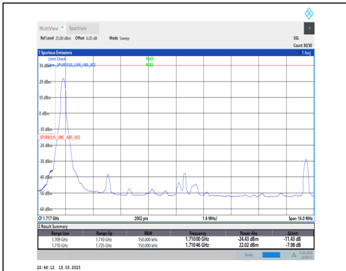
1-N66-PC3-15-15-L-1-DFT-PI2BPSK-Edge_1RB_Left-1@0-Ant1-1-seegraph-PASS-see graph
