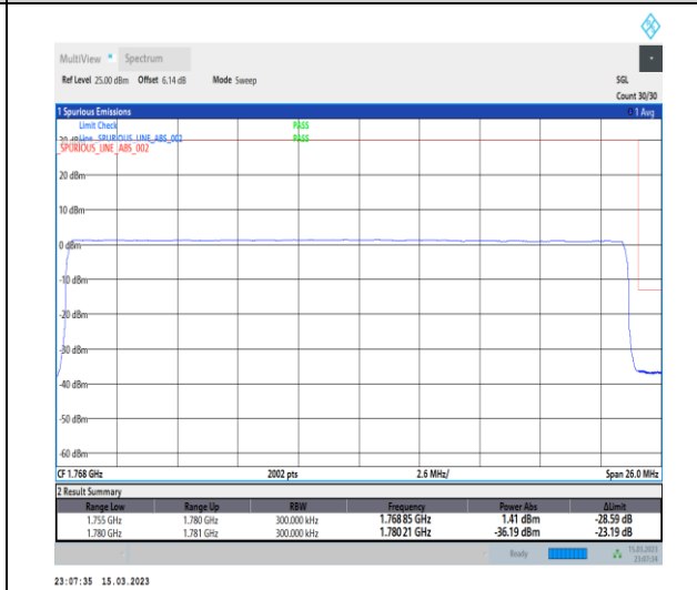
1-N66-PC3-15-25-H-6-CP-QPSK-Outer_Full-133@0-Ant1-1-seegraph-PASS-see graph
