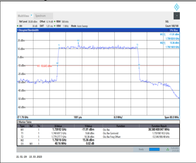
1-N66-PC3-15-40-H-2-DFT-PI2BPSK-Outer_Full-216@0-Ant1-38.58-40.160-≤40-PASS
