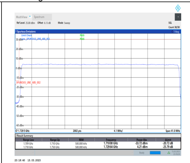
1-N66-PC3-15-40-L-3-DFT-PI2BPSK-Outer_Full-216@0-Ant1-1-seegraph-PASS-see graph
