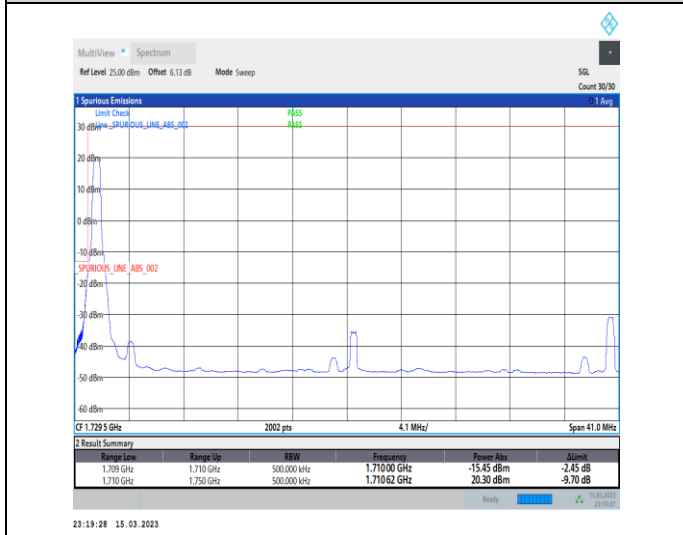
1-N66-PC3-15-40-L-4-CP-QPSK-Edge_1RB_Left-1@0-Ant1-1-seegraph-PASS-see graph
