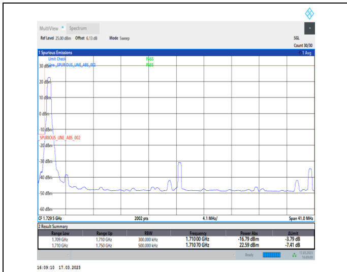
1-N66-PC3-15-40-L-1-DFT-PI2BPSK-Edge_1RB_Left-1@0-Ant1-1-seegraph-PASS-see graph
