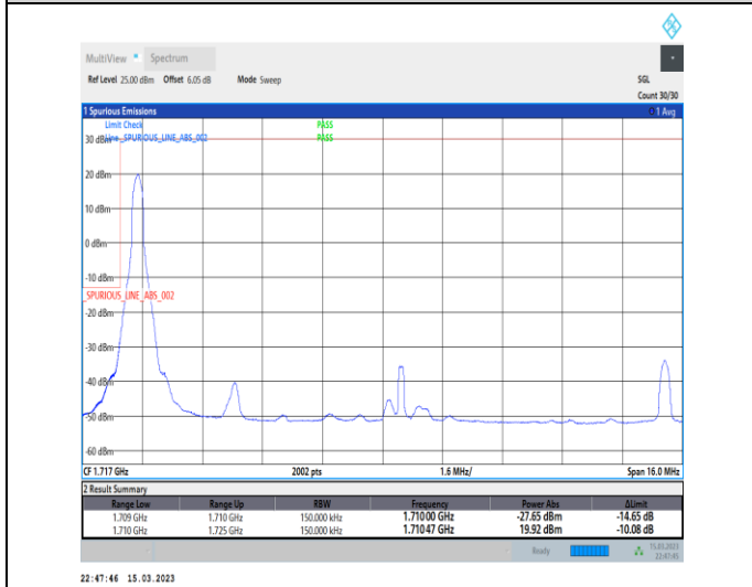
1-N66-PC3-15-15-L-4-CP-QPSK-Edge_1RB_Left-1@0-Ant1-1-seegraph-PASS-see graph
