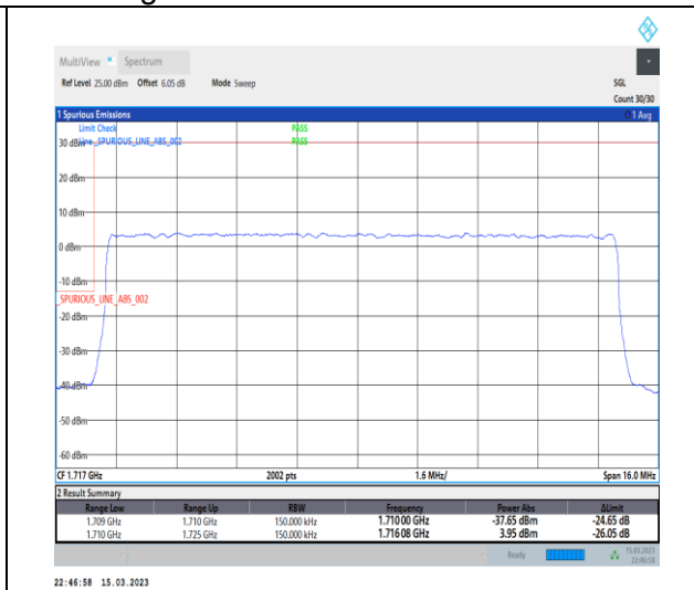
1-N66-PC3-15-15-L-3-DFT-PI2BPSK-Outer_Full-75@0-Ant1-1-seegraph-PASS-see graph
