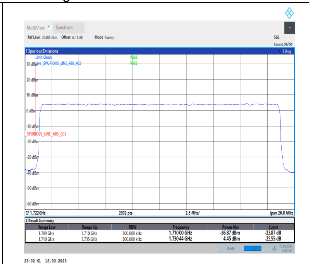
1-N66-PC3-15-25-L-3-DFT-PI2BPSK-Outer_Full-128@0-Ant1-1-seegraph-PASS-see graph
