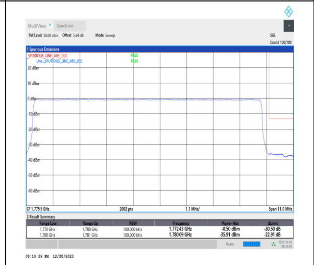
1-N66-15-10-H-6-CP-QPSK-Outer_Full-52@0-Ant1-1-seegraph-PASS-see graph
