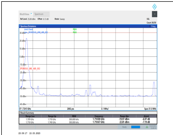
1-N66-PC3-15-30-L-1-DFT-PI2BPSK-Edge_1RB_Left-1@0-Ant1-1-seegraph-PASS-see graph
