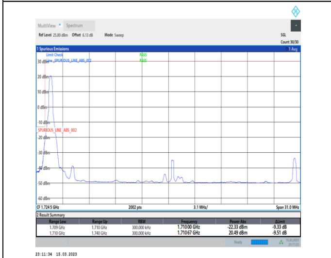
1-N66-PC3-15-30-L-4-CP-QPSK-Edge_1RB_Left-1@0-Ant1-1-seegraph-PASS-see graph
