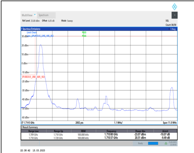
1-N66-PC3-15-10-L-1-DFT-PI2BPSK-Edge_1RB_Left-1@0-Ant1-1-seegraph-PASS-see graph
