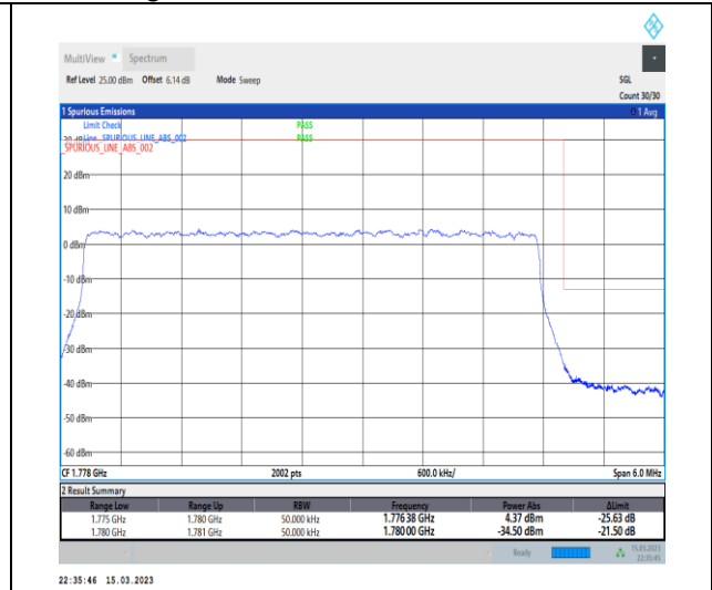
1-N66-PC3-15-5-H-3-DFT-PI2BPSK-Outer_Full-25@0-Ant1-1-seegraph-PASS-see graph
