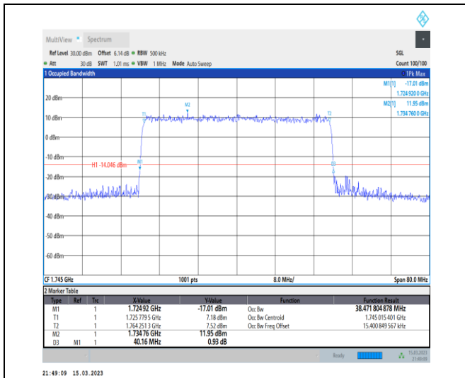
1-N66-PC3-15-40-M-6-CP-QPSK-Outer_Full-216@0 -Ant1-38.472-40.160-≤40-PASS
