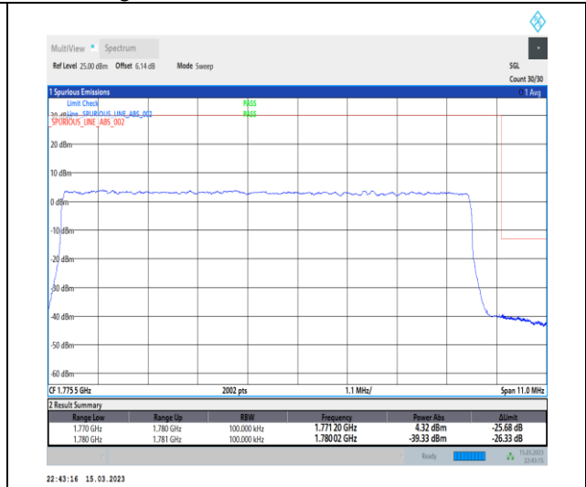
1-N66-PC3-15-10-H-3-DFT-PI2BPSK-Outer_Full-50@0-Ant1-1-seegraph-PASS-see graph
