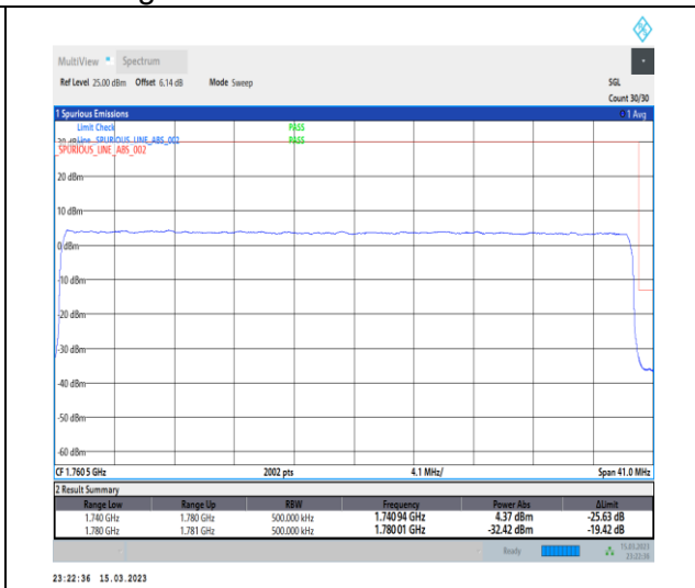
1-N66-PC3-15-40-H-3-DFT-PI2BPSK-Outer_Full-216@0-Ant1-1-seegraph-PASS-see graph
