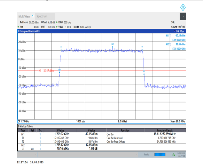
1-N66-PC3-15-40-L-4-DFT-64QAM-Outer_Full-216 @0-Ant1-38.612-40.160-≤40-PASS
