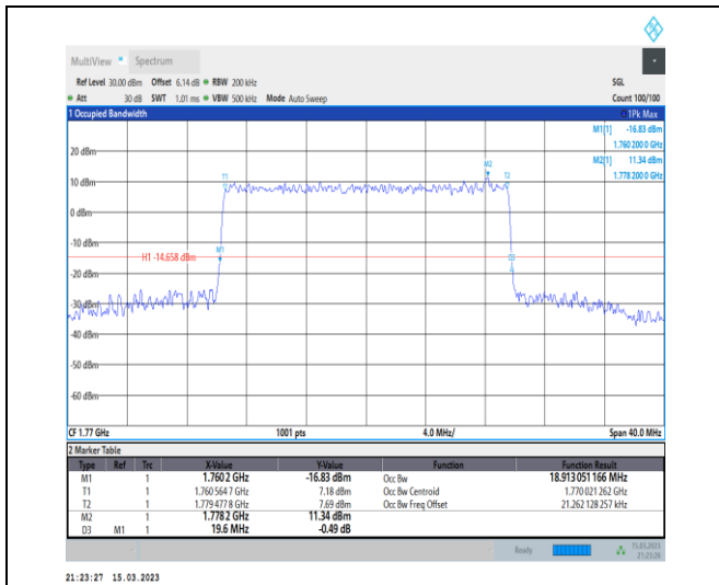
1-N66-PC3-15-20-H-6-CP-QPSK-Outer_Full-106@0 -Ant1-18.913-19.600-≤20-PASS
