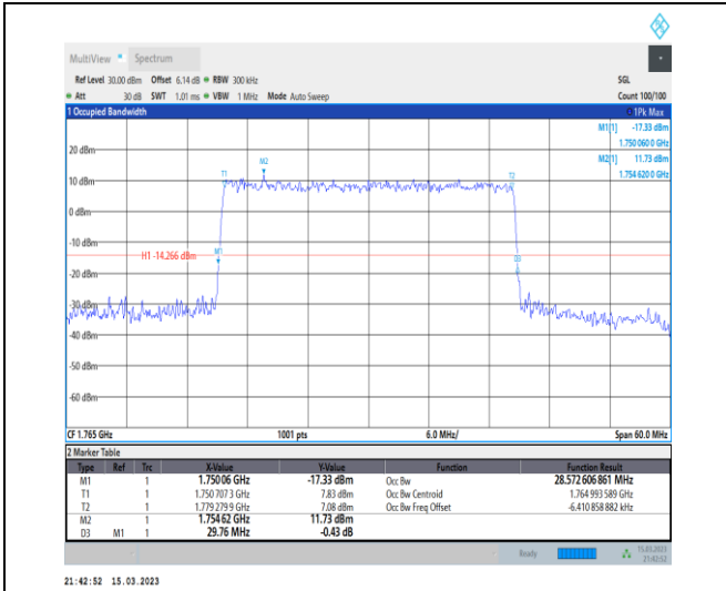
1-N66-PC3-15-30-H-4-DFT-64QAM-Outer_Full-160 @0-Ant1-28.573-29.760-≤30-PASS
