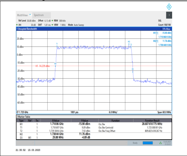
1-N66-PC3-15-30-L-3-DFT-16QAM-Outer_Full-160 @0-Ant1-28.608-29.880-≤30-PASS
