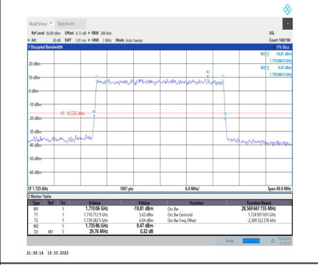
1-N66-PC3-15-30-L-5-DFT-256QAM-Outer_Full-160 @0-Ant1-28.57-29.760-≤30-PASS
