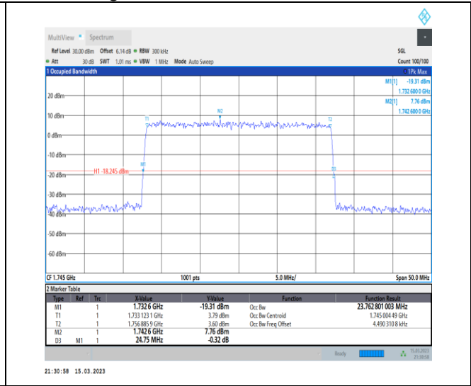
1-N66-PC3-15-25-M-9-CP-256QAM-Outer_Full-133 @0-Ant1-23.762-24.750-<=25-PASS
