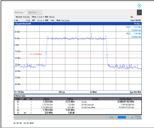
1-N66-PC3-15-25-M-4-DFT-64QAM-Outer_Full-128 @0-Ant1-22.887-23.900-≤25-PASS
