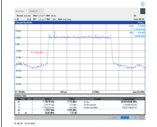
1-N66-PC3-15-30-H-2-DFT-PI2BPSK-Outer_Full-160 @0-Ant1-28.506-29.640-≤30-PASS
