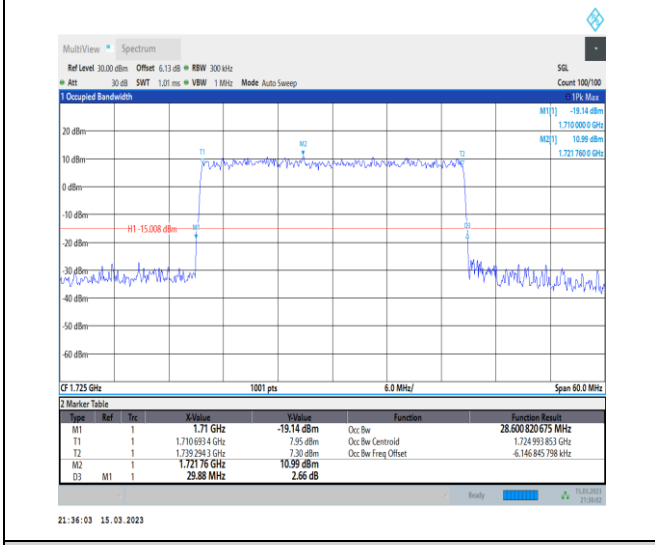
1-N66-PC3-15-30-L-4-DFT-64QAM-Outer_Full-160 @0-Ant1-28.601-29.880-≤30-PASS
