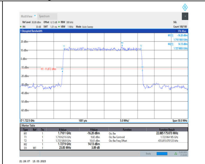
1-N66-PC3-15-25-L-2-DFT-PI2BPSK-Outer_Full-128 @0-Ant1-22.885-23.850- \leq 25 -PASS
