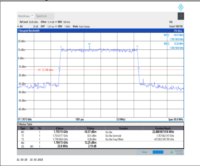
1-N66-PC3-15-25-H-4-DFT-64QAM-Outer_Full-128 @0-Ant1-22.889-23.800-≤25-PASS
