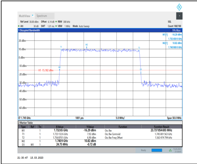
1-N66-PC3-15-25-M-8-CP-64QAM-Outer_Full-133@ 0-Ant1-23.738-24.750-<=25-PASS
