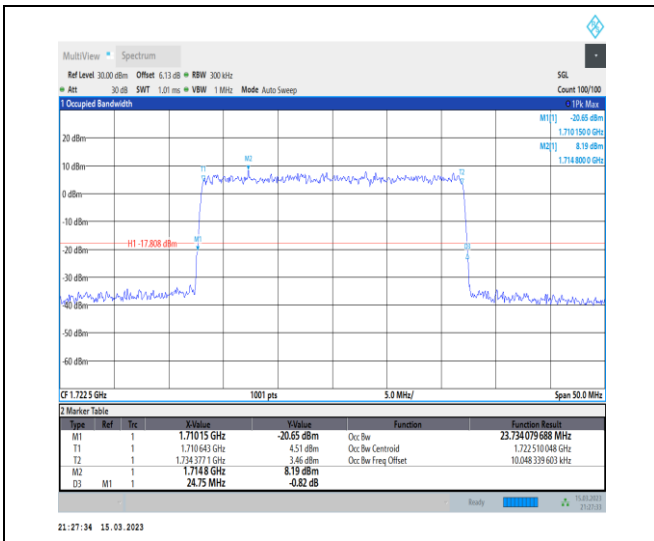
1-N66-PC3-15-25-L-9-CP-256QAM-Outer_Full-133 @0-Ant1-23.734-24.750-≤25-PASS
