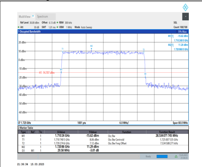
1-N66-PC3-15-30-L-7-CP-16QAM-Outer_Full-160@0-Ant1-28.534-29.580-≤30-PASS
