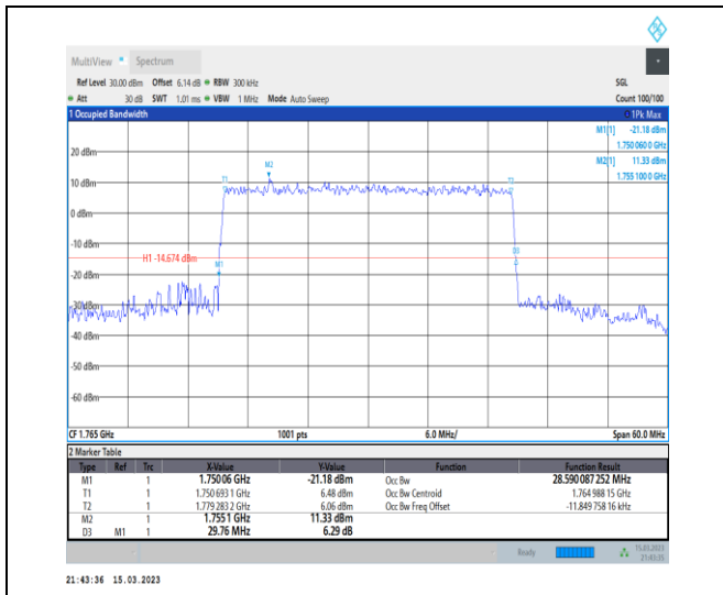
1-N66-PC3-15-30-H-8-CP-64QAM-Outer_Full-160@ 0-Ant1-28.59-29.760-≤30-PASS
