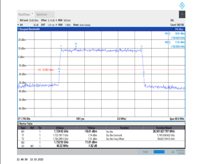
1-N66-PC3-15-40-M-5-DFT-256QAM-Outer_Full-216 @0-Ant1-38.502-40.320-≤40-PASS
