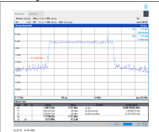
1-N66-PC3-15-20-H-7-CP-16QAM-Outer_Full-106@0 -Ant1-18.909-19.720-≤20-PASS
