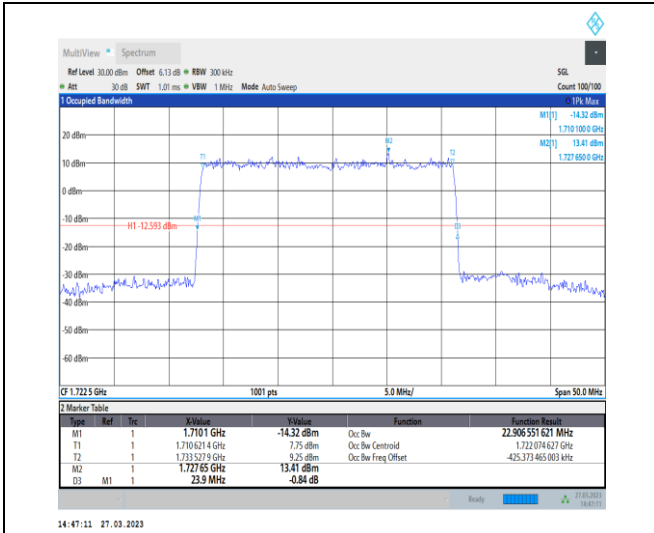
1-N66-PC3-15-25-L-1-DFT-QPSK-Outer_Full-128@ 0-Ant1-22.907-23.900- \leq 25 -PASS
