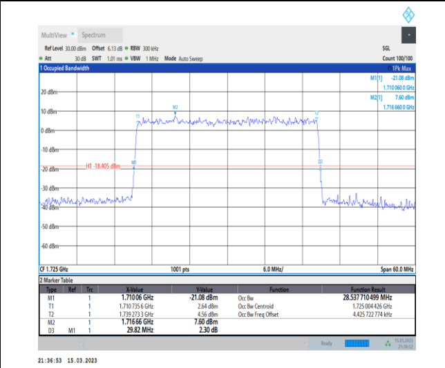
1-N66-PC3-15-30-L-9-CP-256QAM-Outer_Full-160@0-Ant1-28.538-29.820-≤30-PASS
