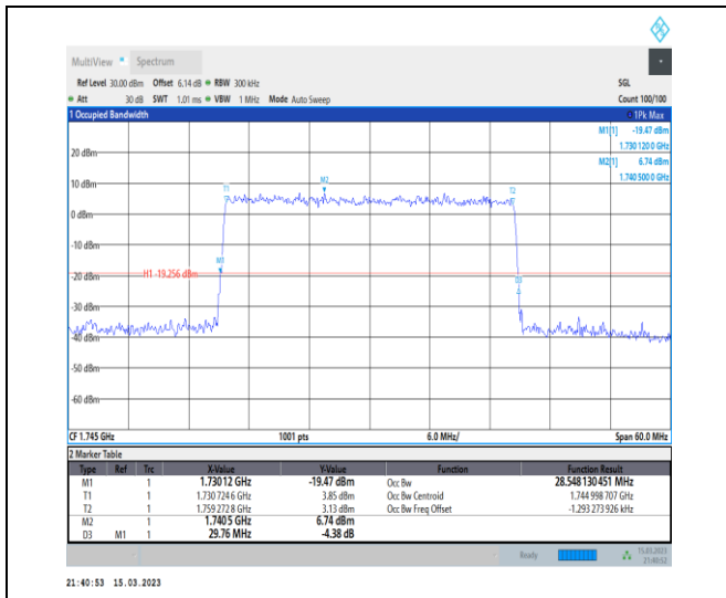
1-N66-PC3-15-30-M-9-CP-256QAM-Outer_Full-160 @0-Ant1-28.548-29.760-≤30-PASS
