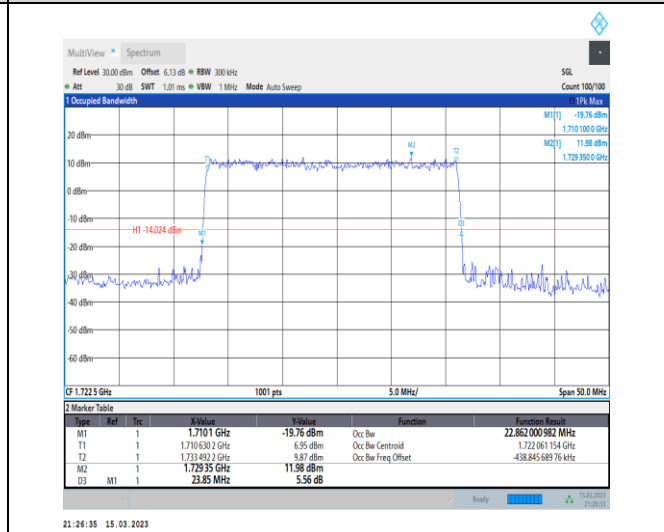
1-N66-PC3-15-25-L-4-DFT-64QAM-Outer_Full-128 @0-Ant1-22.862-23.850- \leq 25 -PASS
