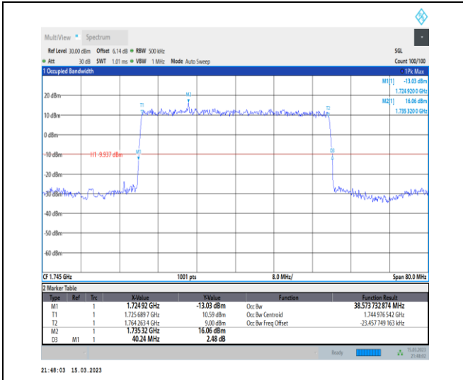
1-N66-PC3-15-40-M-2-DFT-PI2BPSK-Outer_Full-21 @0-Ant1-38.574-40.240-≤40-PASS
