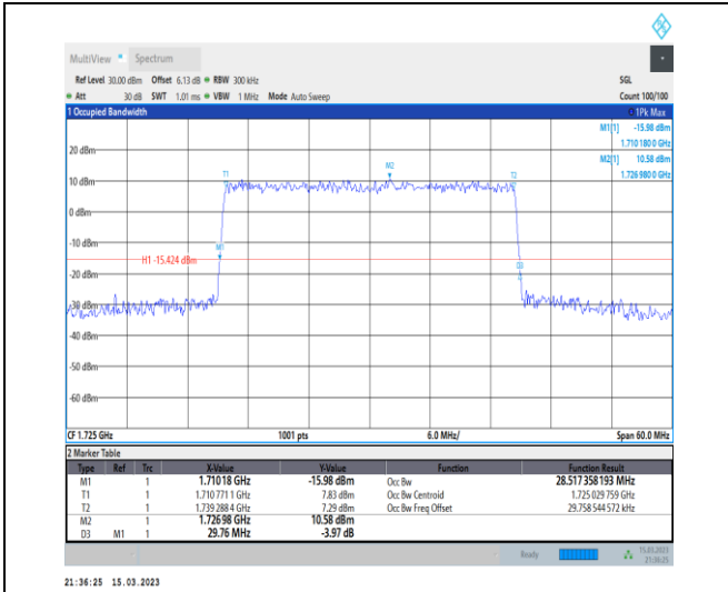
1-N66-PC3-15-30-L-6-CP-QPSK-Outer_Full-160@0-Ant1-28.517-29.760-≤30-PASS
