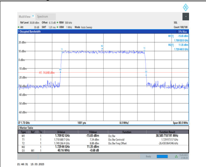
1-N66-PC3-15-40-L-8-CP-64QAM-Outer_Full-216@0-Ant1-38.586-40.160-≤40-PASS
