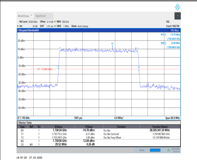
1-N66-PC3-15-30-M-4-DFT-64QAM-Outer_Full-160@0-Ant1-28.505-29.520-≤30-PASS
