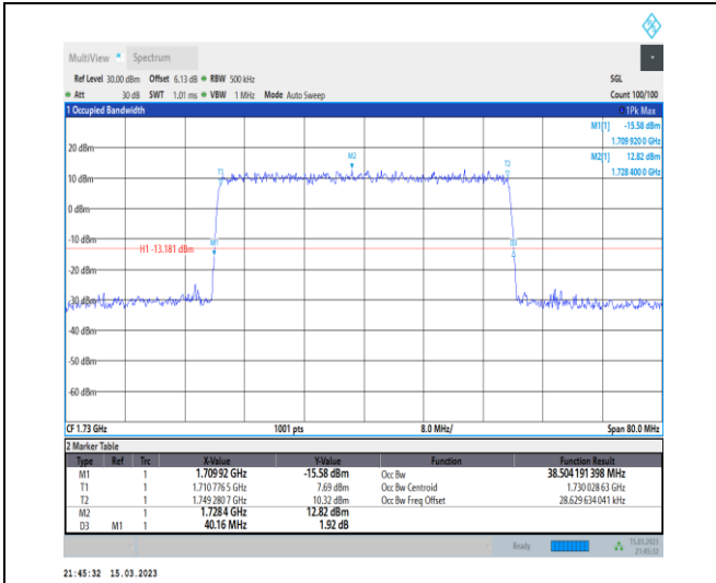
1-N66-PC3-15-40-L-3-DFT-16QAM-Outer_Full-216 @0-Ant1-38.504-40.160-≤40-PASS
