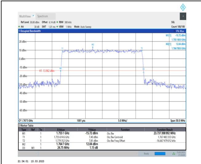
1-N66-PC3-15-25-H-7-CP-16QAM-Outer_Full-133@ 0-Ant1-23.737-24.750-≤25-PASS
