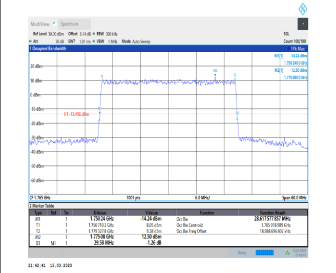
1-N66-PC3-15-30-H-3-DFT-16QAM-Outer_Full-160 @0-Ant1-28.618-29.580-≤30-PASS
