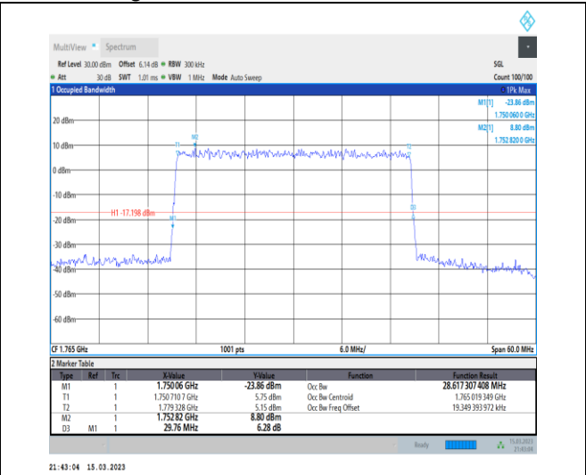
1-N66-PC3-15-30-H-5-DFT-256QAM-Outer_Full-160 @0-Ant1-28.617-29.760-≤30-PASS
