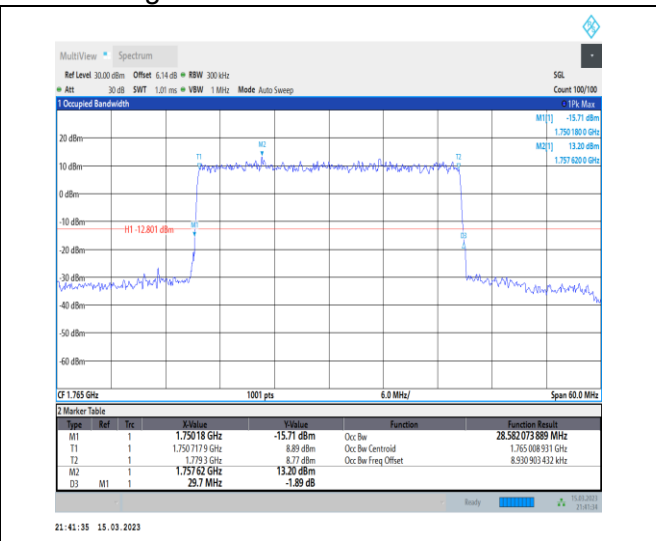
1-N66-PC3-15-30-H-1-DFT-QPSK-Outer_Full-160 @0-Ant1-28.582-29.700-≤30-PASS
