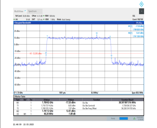
1-N66-PC3-15-40-L-6-CP-QPSK-Outer_Full-216 @0-Ant1-38.598-40.240-≤40-PASS
