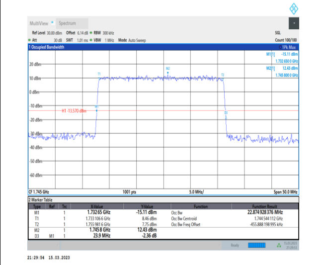
1-N66-PC3-15-25-M-3-DFT-16QAM-Outer_Full-128 @0-Ant1-22.875-23.900-≤25-PASS
