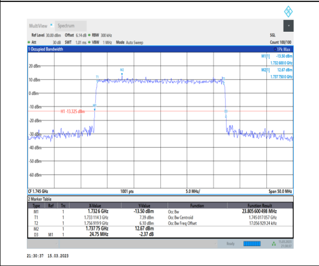
1-N66-PC3-15-25-M-7-CP-16QAM-Outer_Full-133@0 -Ant1-23.806-24.750-≤25-PASS
