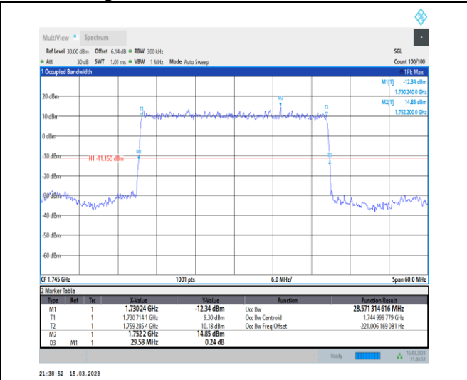
1-N66-PC3-15-30-M-2-DFT-PI2BPSK-Outer_Full-160@0-Ant1-28.571-29.580-≤30-PASS
