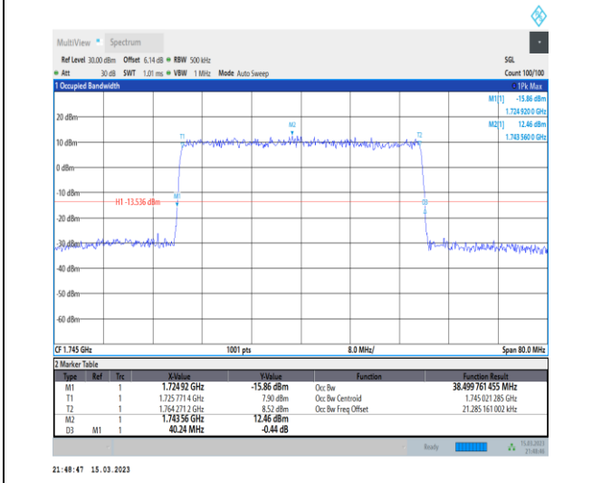
1-N66-PC3-15-40-M-4-DFT-64QAM-Outer_Full-216 @0-Ant1-38.5-40.240-≤40-PASS
