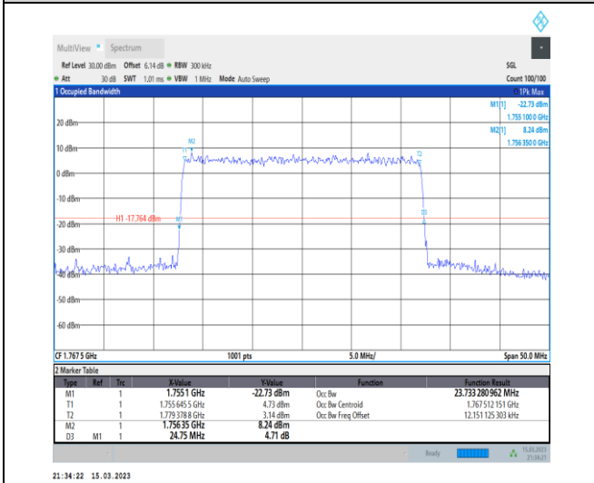
1-N66-PC3-15-25-H-9-CP-256QAM-Outer_Full-133 @0-Ant1-23.733-24.750-≤25-PASS
