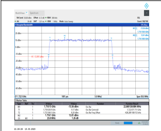
1-N66-PC3-15-25-L-3-DFT-16QAM-Outer_Full-128 @0-Ant1-22.87-23.800- \leq 25 -PASS
