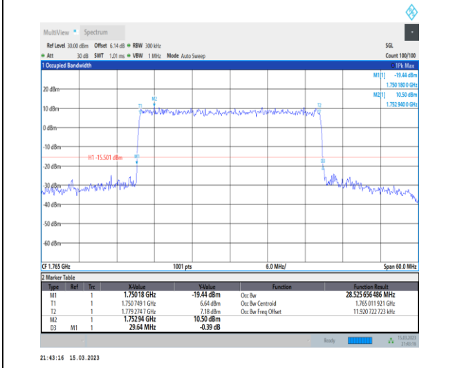
1-N66-PC3-15-30-H-6-CP-QPSK-Outer_Full-160@0 -Ant1-28.526-29.640-≤30-PASS
