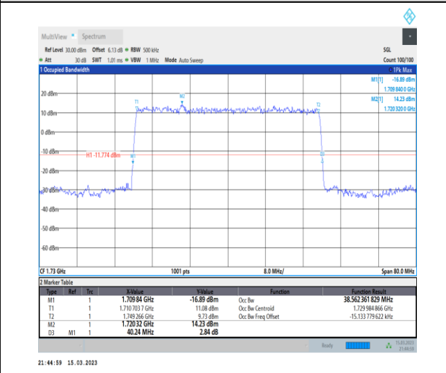
1-N66-PC3-15-40-L-2-DFT-PI2BPSK-Outer_Full-216 @0-Ant1-38.562-40.240-≤40-PASS
