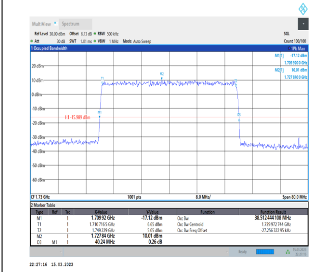
1-N66-PC3-15-40-L-5-DFT-256QAM-Outer_Full-216 @0-Ant1-38.512-40.240-≤40-PASS
