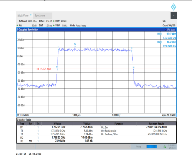
1-N66-PC3-15-25-M-5-DFT-256QAM-Outer_Full-128 @0-Ant1-22.835-23.900-≤25-PASS
