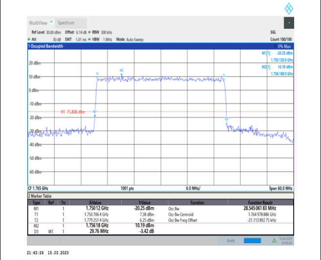
1-N66-PC3-15-30-H-7-CP-16QAM-Outer_Full-160@0 -Ant1-28.545-29.760-≤30-PASS
