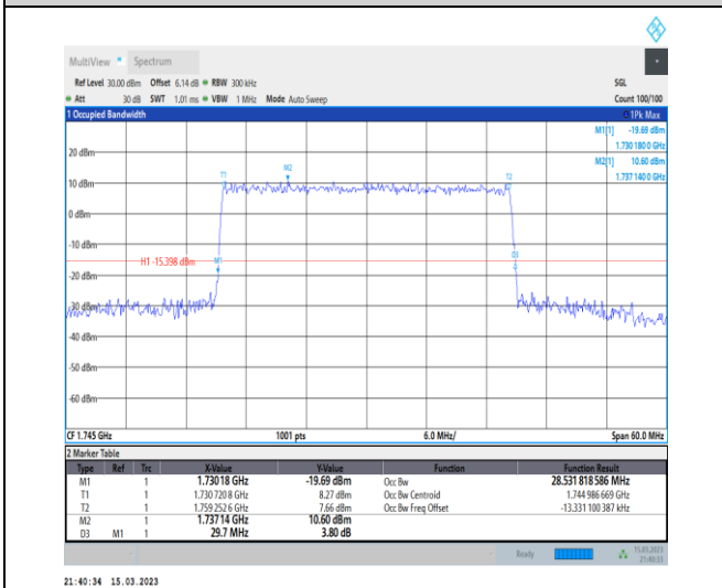
1-N66-PC3-15-30-M-7-CP-16QAM-Outer_Full-160@0-Ant1-28.532-29.700-≤30-PASS
