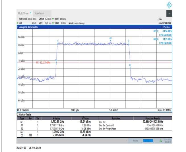
1-N66-PC3-15-25-M-2-DFT-PI2BPSK-Outer_Full-12 @0-Ant1-22.88-23.850-≤25-PASS
