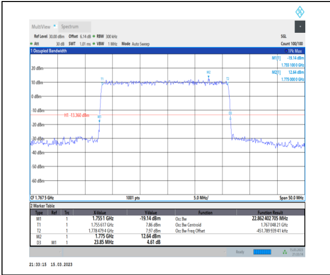
1-N66-PC3-15-25-H-3-DFT-16QAM-Outer_Full-128 @0-Ant1-22.862-23.850-≤25-PASS
