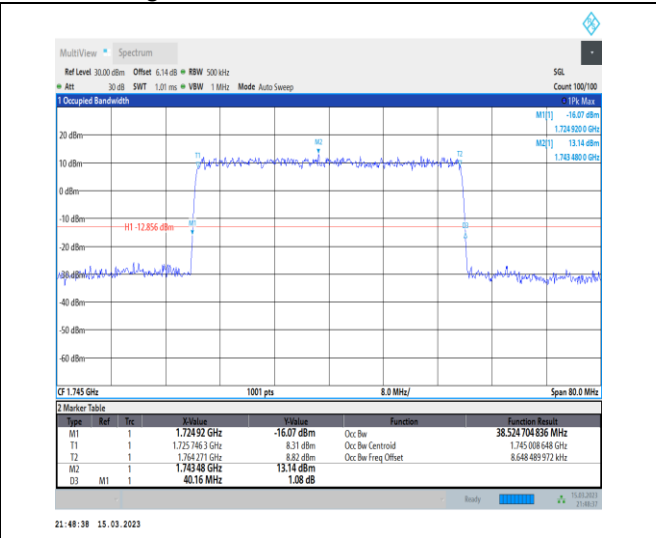
1-N66-PC3-15-40-M-3-DFT-16QAM-Outer_Full-216 @0-Ant1-38.525-40.160-≤40-PASS
