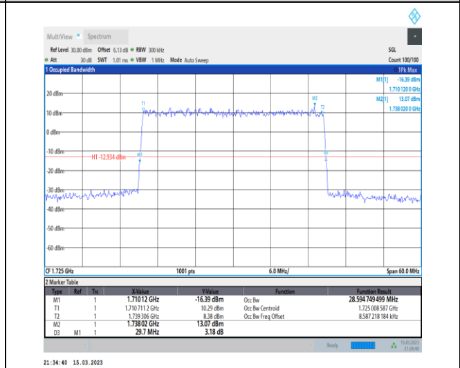
1-N66-PC3-15-30-L-1-DFT-QPSK-Outer_Full-160@ 0-Ant1-28.595-29.700-≤30-PASS
