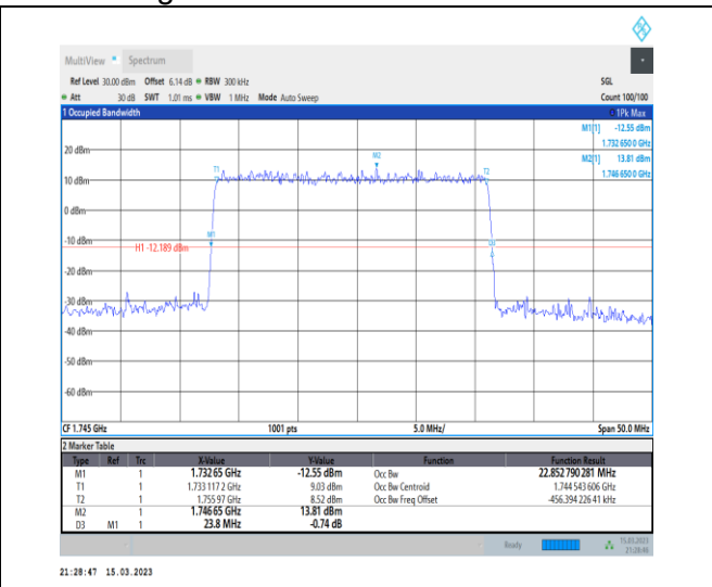
1-N66-PC3-15-25-M-1-DFT-QPSK-Outer_Full-128 @0-Ant1-22.853-23.800-≤25-PASS
