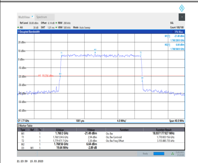
1-N66-PC3-15-20-H-9-CP-256QAM-Outer_Full-106@0 -Ant1-18.937-19.640-≤20-PASS
