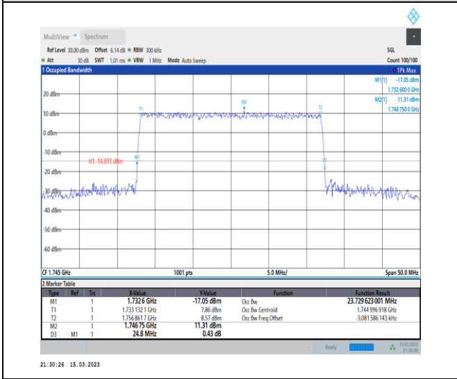
1-N66-PC3-15-25-M-6-CP-QPSK-Outer_Full-133@0 -Ant1-23.73-24.800-≤25-PASS
