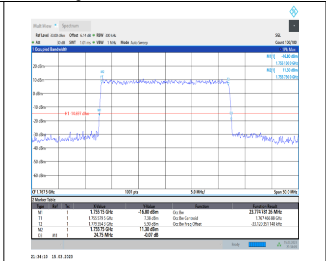
1-N66-PC3-15-25-H-8-CP-64QAM-Outer_Full-133@ 0-Ant1-23.775-24.750-≤25-PASS
