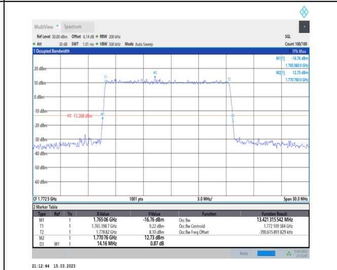
1-N66-PC3-15-15-H-4-DFT-64QAM-Outer_Full-75@0-Ant1-13.421-14.160-≤15-PASS
