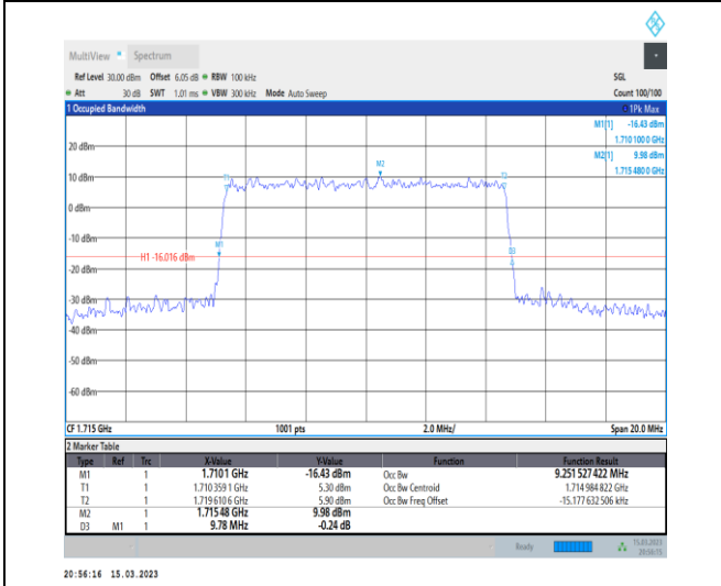
1-N66-PC3-15-10-L-8-CP-64QAM-Outer_Full-52@0-A Ant1-9.252-9.780-≤10-PASS
