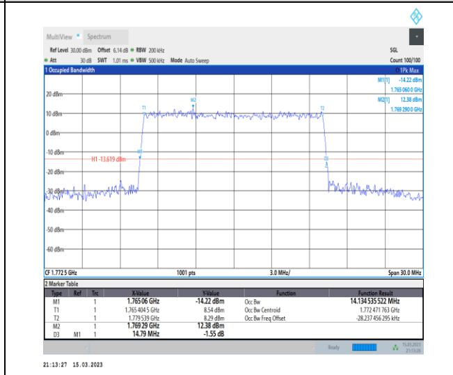
1-N66-PC3-15-15-H-8-CP-64QAM-Outer_Full-79@0-Ant1-14.135-14.790-≤15-PASS
