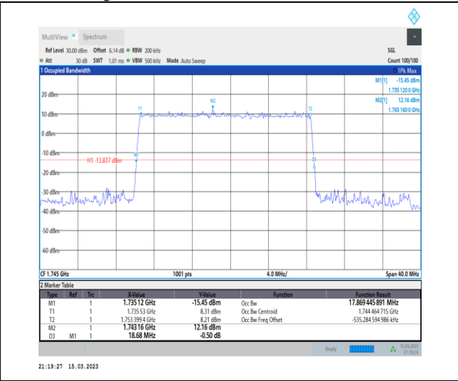
1-N66-PC3-15-20-M-4-DFT-64QAM-Outer_Full-100 @0-Ant1-17.869-18.680-≤20-PASS
