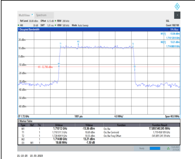
1-N66-PC3-15-20-L-2-DFT-PI2BPSK-Outer_Full-100 @0-Ant1-17.894-18.680-≤20-PASS
