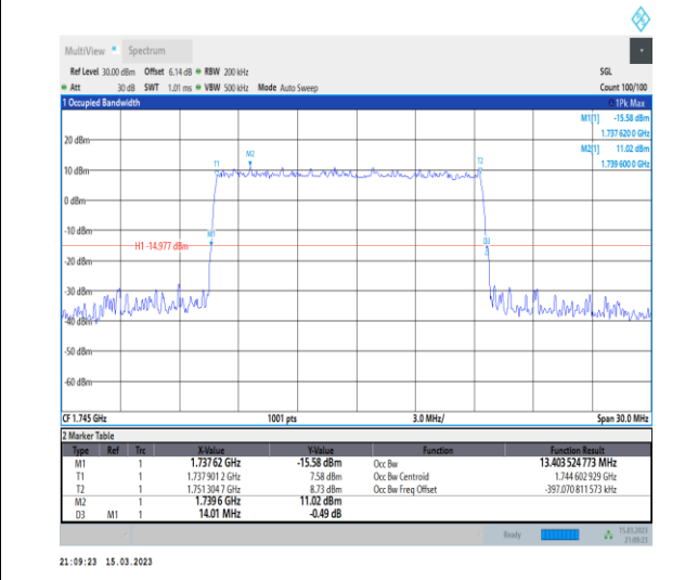
1-N66-PC3-15-15-M-5-DFT-256QAM-Outer_Full-75 @0-Ant1-13.404-14.010-≤15-PASS
