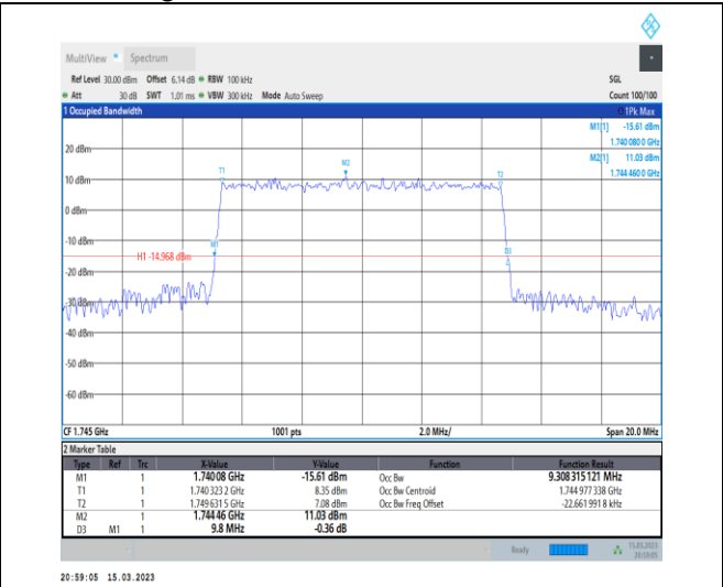
1-N66-PC3-15-10-M-6-CP-QPSK-Outer_Full-52@0-Ant1-9.308-9.800-≤10-PASS
