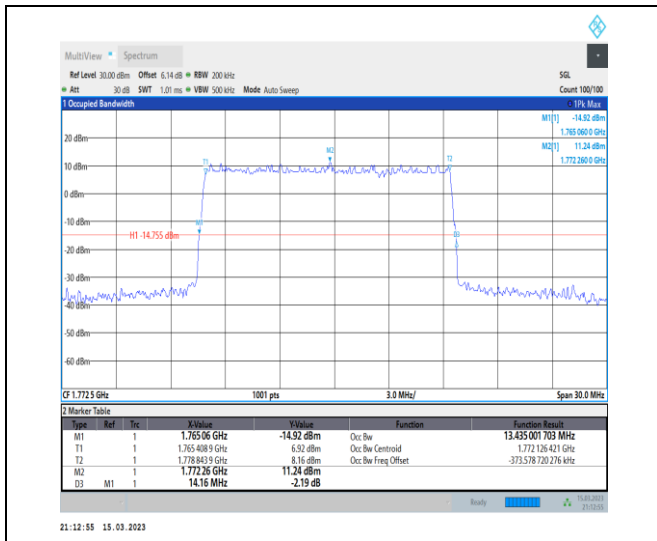
1-N66-PC3-15-15-H-5-DFT-256QAM-Outer_Full-75 @0-Ant1-13.435-14.160-≤15-PASS
