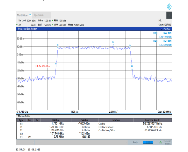
1-N66-PC3-15-10-L-7-CP-16QAM-Outer_Full-52@0-A Ant1-9.272-9.780-≤10-PASS
