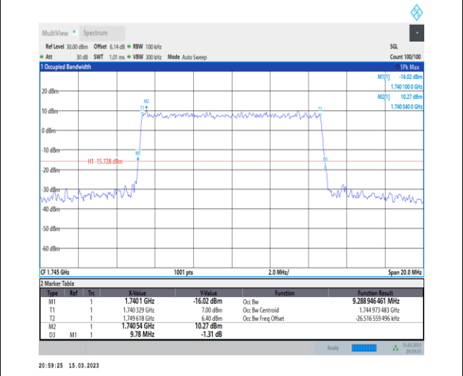
1-N66-PC3-15-10-M-8-CP-64QAM-Outer_Full-52@0-Ant1-9.289-9.780-≤10-PASS
