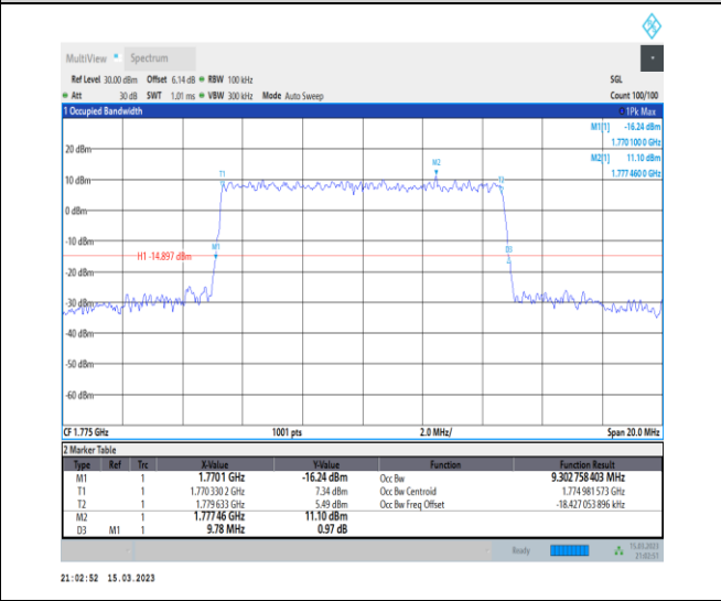
1-N66-PC3-15-10-H-7-CP-16QAM-Outer_Full-52@0-Ant1-9.303-9.780-≤10-PASS
