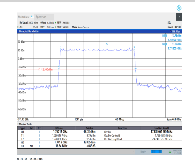
1-N66-PC3-15-20-H-1-DFT-QPSK-Outer_Full-100@ 0-Ant1-17.882-18.640-≤20-PASS
