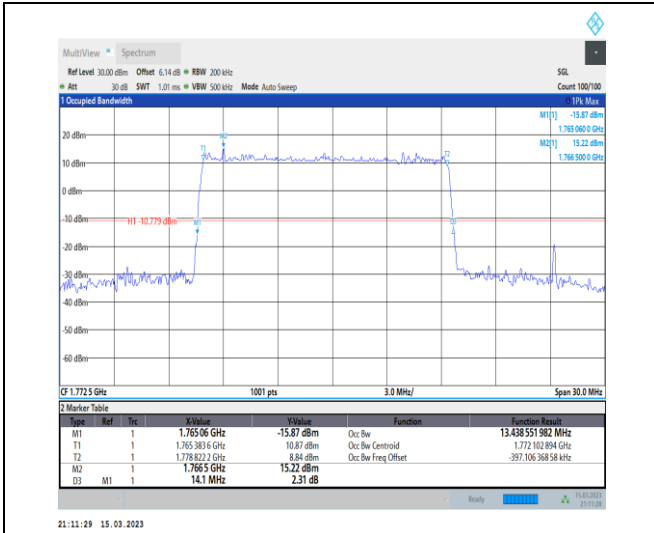
1-N66-PC3-15-15-H-1-DFT-QPSK-Outer_Full-75@0-Ant1-13.439-14.100-≤15-PASS
