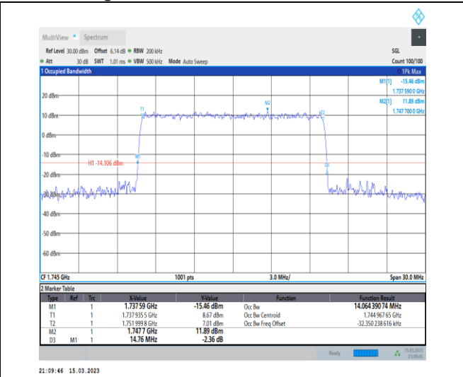
1-N66-PC3-15-15-M-7-CP-16QAM-Outer_Full-79@0-Ant1-14.064-14.760-≤15-PASS
