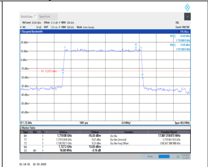
1-N66-PC3-15-20-L-1-DFT-QPSK-Outer_Full-100@ 0-Ant1-17.861-18.680-≤20-PASS
