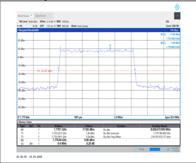
1-N66-PC3-15-10-H-5-DFT-256QAM-Outer_Full-50@0-Ant1-8.927-9.400-≤10-PASS
