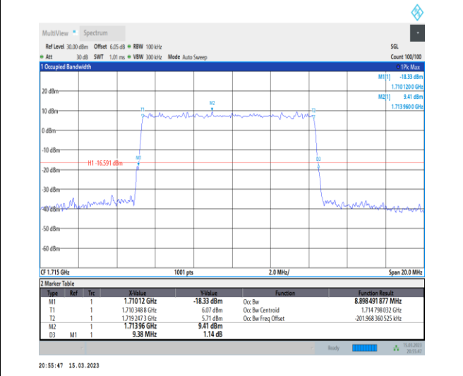
1-N66-PC3-15-10-L-5-DFT-256QAM-Outer_Full-50 @0-Ant1-8.898-9.380-≤10-PASS
