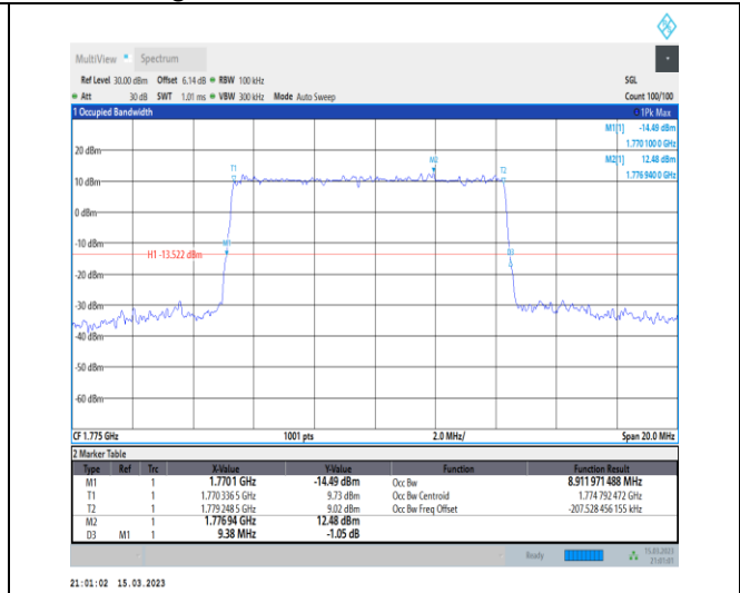
1-N66-PC3-15-10-H-1-DFT-QPSK-Outer_Full-50@0- Ant1-8.912-9.380-≤10-PASS
