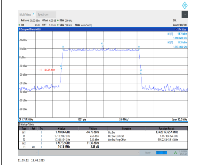
1-N66-PC3-15-15-L-5-DFT-256QAM-Outer_Full-75@0-Ant1-13.423-14.130-≤15-PASS
