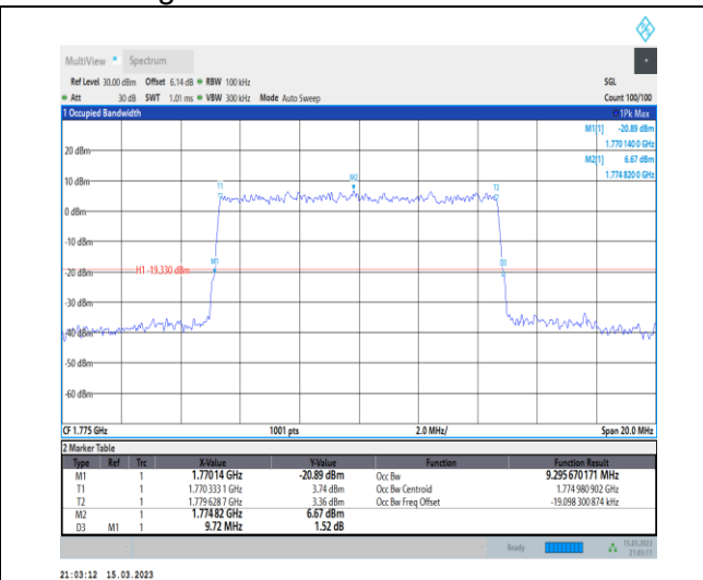
1-N66-PC3-15-10-H-9-CP-256QAM-Outer_Full-52@ 0-Ant1-9.296-9.720-≤10-PASS
