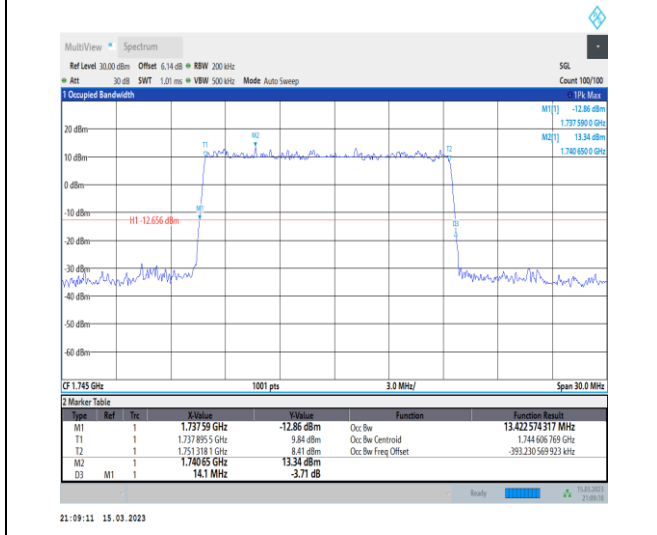
1-N66-PC3-15-15-M-4-DFT-64QAM-Outer_Full-75 @0-Ant1-13.423-14.100-≤15-PASS
