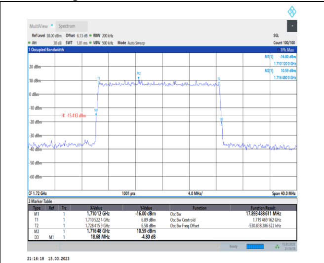
1-N66-PC3-15-20-L-5-DFT-256QAM-Outer_Full-100 @0-Ant1-17.893-18.680-≤20-PASS
