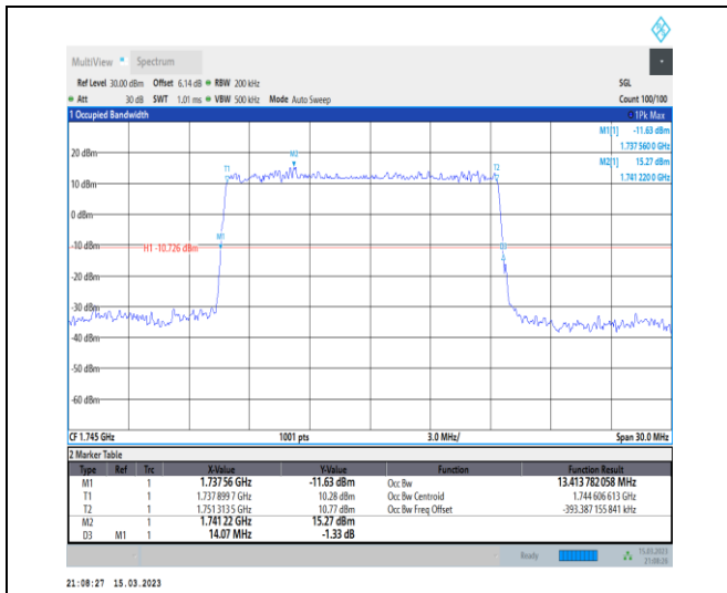
1-N66-PC3-15-15-M-2-DFT-PI2BPSK-Outer_Full-75 @0-Ant1-13.414-14.070-≤15-PASS
