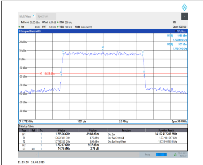
1-N66-PC3-15-15-H-9-CP-256QAM-Outer_Full-79@ 0-Ant1-14.102-14.760-≤15-PASS
