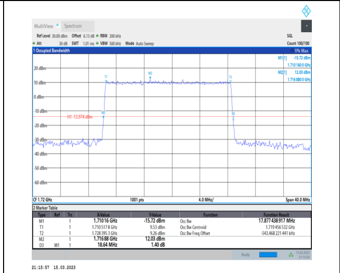
1-N66-PC3-15-20-L-3-DFT-16QAM-Outer_Full-100 @0-Ant1-17.877-18.640-≤20-PASS
