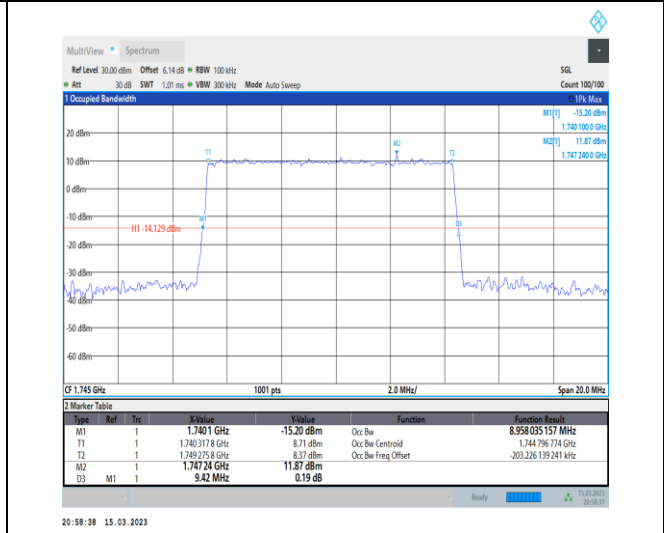
1-N66-PC3-15-10-M-4-DFT-64QAM-Outer_Full-50@0-Ant1-8.958-9.420-≤10-PASS
