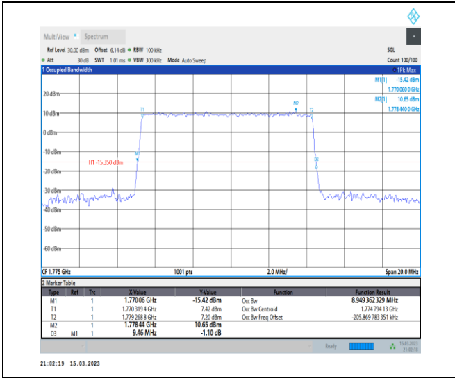
1-N66-PC3-15-10-H-4-DFT-64QAM-Outer_Full-50@0-Ant1-8.949-9.460-≤10-PASS
