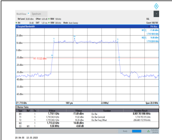
1-N66-PC3-15-10-L-2-DFT-PI2BPSK-Outer_Full-50 @0-Ant1-8.902-9.360-≤10-PASS
