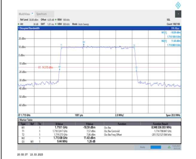
1-N66-PC3-15-10-L-4-DFT-64QAM-Outer_Full-50 @0-Ant1-8.948-9.440-≤10-PASS
