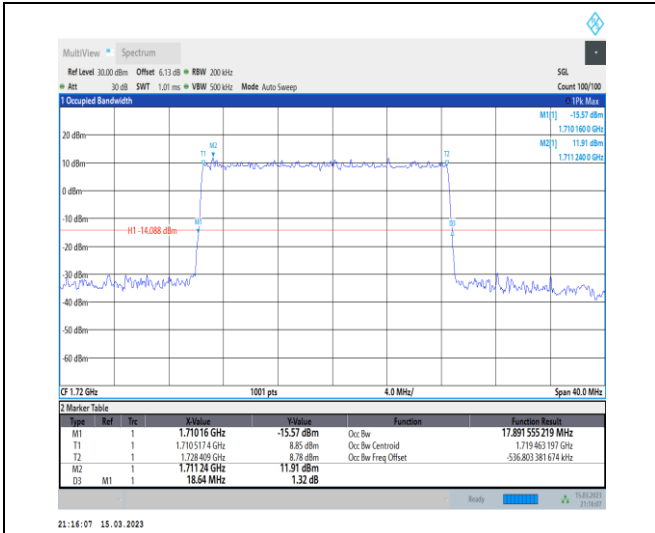
1-N66-PC3-15-20-L-4-DFT-64QAM-Outer_Full-100 @0-Ant1-17.892-18.640-≤20-PASS
