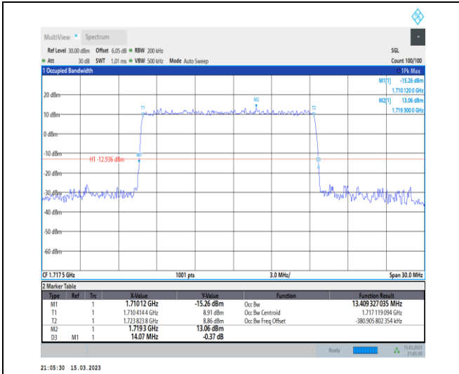
1-N66-PC3-15-15-L-3-DFT-16QAM-Outer_Full-75@0-Ant1-13.409-14.070-≤15-PASS
