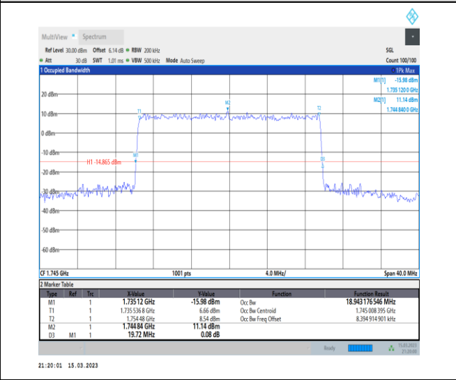
1-N66-PC3-15-20-M-6-CP-QPSK-Outer_Full-106@0 -Ant1-18.943-19.720-≤20-PASS
