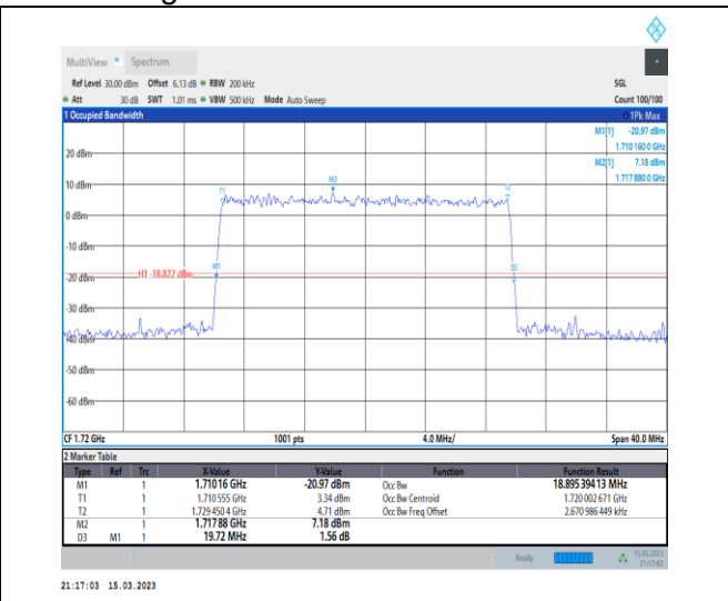
1-N66-PC3-15-20-L-9-CP-256QAM-Outer_Full-106@0-Ant1-18.895-19.720-≤20-PASS
