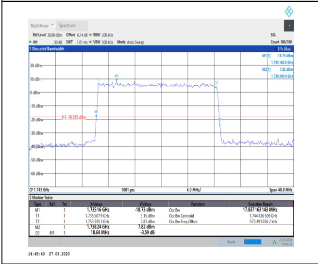
1-N66-PC3-15-20-M-5-DFT-256QAM-Outer_Full-100 @0-Ant1-17.837-18.640-≤20-PASS
