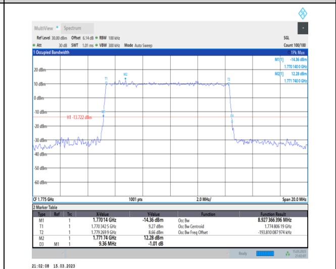
1-N66-PC3-15-10-H-3-DFT-16QAM-Outer_Full-50@ 0-Ant1-8.927-9.360-≤10-PASS
