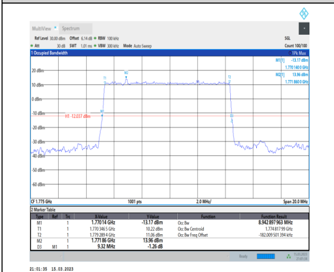
1-N66-PC3-15-10-H-2-DFT-PI2BPSK-Outer_Full-50 @0-Ant1-8.943-9.320-≤10-PASS
