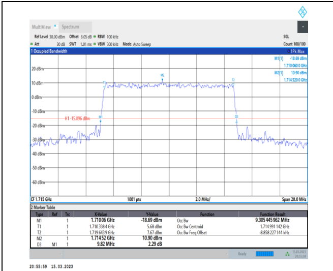
1-N66-PC3-15-10-L-6-CP-QPSK-Outer_Full-52@0-A Ant1-9.305-9.820-≤10-PASS
