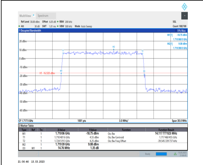
1-N66-PC3-15-15-L-9-CP-256QAM-Outer_Full-79@0-Ant1-14.118-14.760-≤15-PASS
