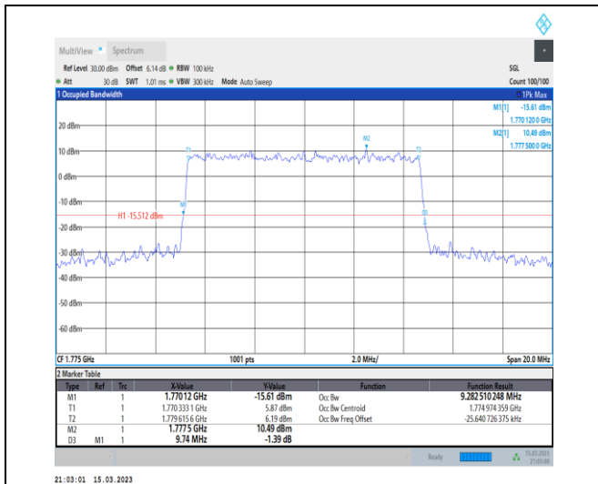
1-N66-PC3-15-10-H-8-CP-64QAM-Outer_Full-52@0 -Ant1-9.283-9.740-≤10-PASS
