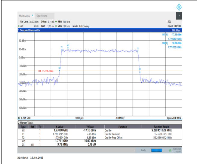
1-N66-PC3-15-10-H-6-CP-QPSK-Outer_Full-52@0-Ant1-9.28-9.780-≤10-PASS
