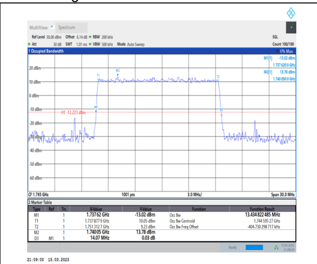
1-N66-PC3-15-15-M-3-DFT-16QAM-Outer_Full-75 @0-Ant1-13.435-14.070-≤15-PASS
