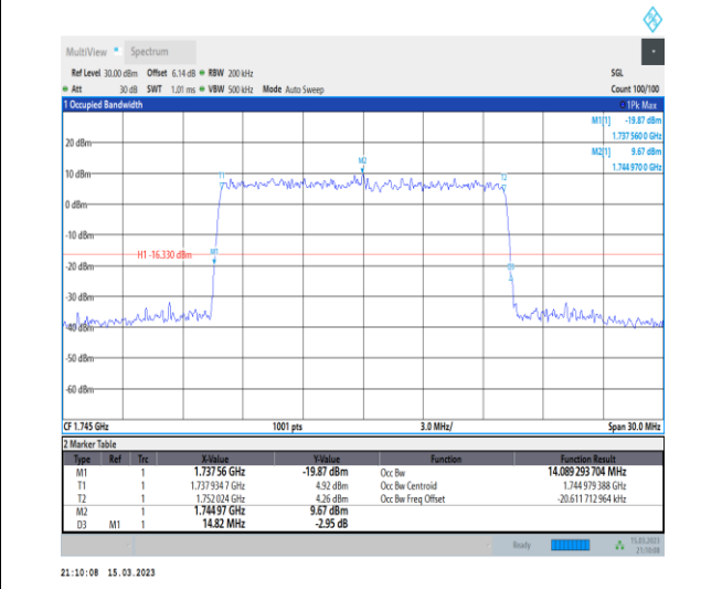
1-N66-PC3-15-15-M-9-CP-256QAM-Outer_Full-79@0-Ant1-14.089-14.820-≤15-PASS
