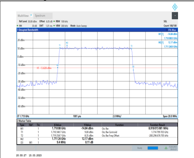
1-N66-PC3-15-10-L-3-DFT-16QAM-Outer_Full-50 @0-Ant1-8.918-9.400-≤10-PASS
