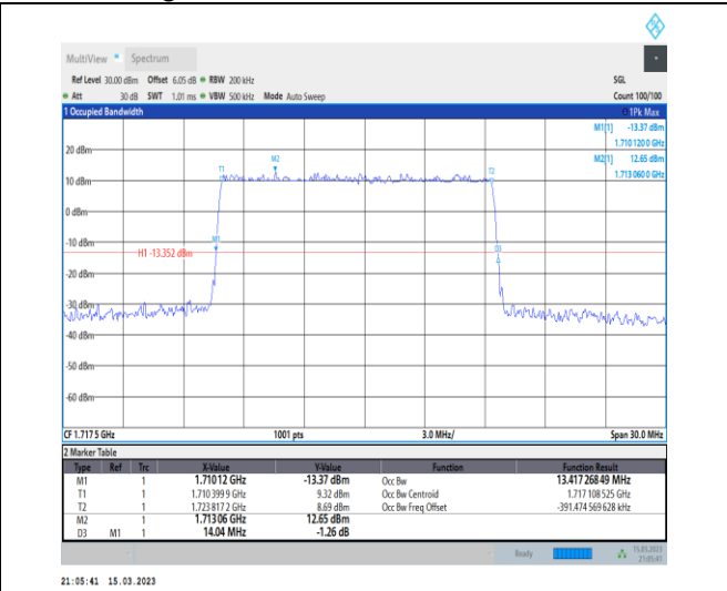
1-N66-PC3-15-15-L-4-DFT-64QAM-Outer_Full-75@0-Ant1-13.417-14.040-≤15-PASS
