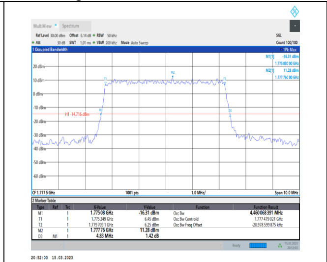
1-N66-PC3-15-5-H-4-DFT-64QAM-Outer_Full-25@0 -Ant1-4.46-4.830-≤5-PASS
