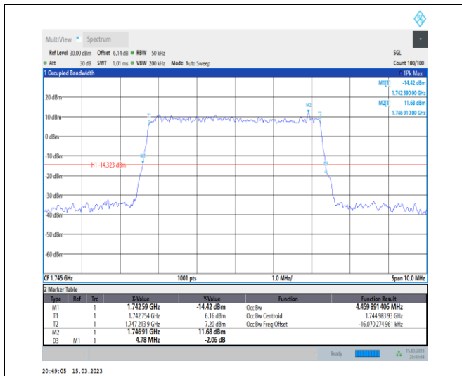
1-N66-PC3-15-5-M-4-DFT-64QAM-Outer_Full-25@0 -Ant1-4.46-4.780-≤5-PASS
