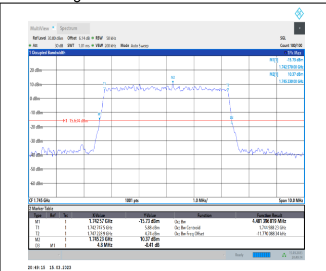
1-N66-PC3-15-5-M-5-DFT-256QAM-Outer_Full-25@0 -Ant1-4.481-4.800-≤5-PASS
