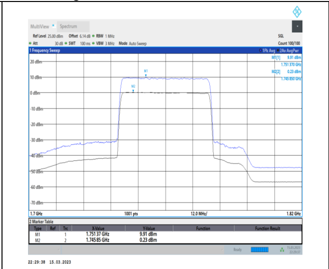
1-N66-PC3-15-40-H-2-CP-256QAM-Outer_Full-216 @0-Ant1-9.68-100%-0.00-9.68-PASS-≤13
