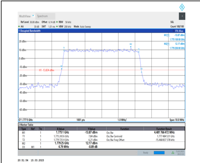
1-N66-PC3-15-5-H-3-DFT-16QAM-Outer_Full-25@0 -Ant1-4.482-4.790-≤5-PASS
