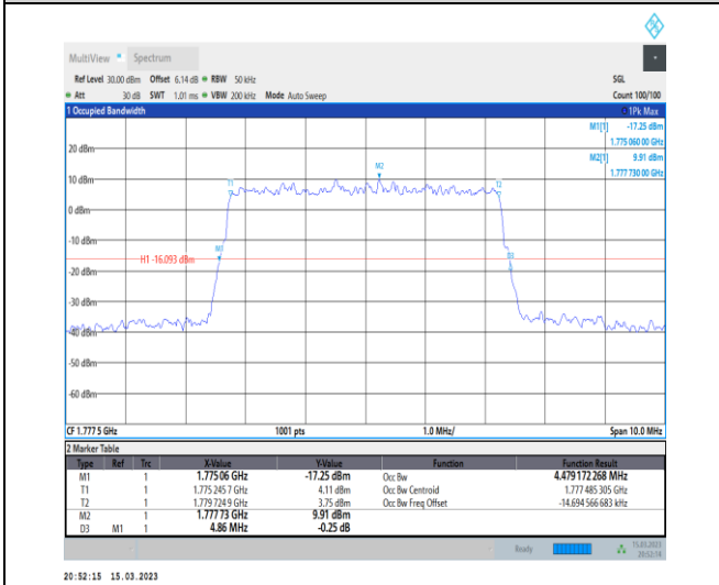
1-N66-PC3-15-5-H-5-DFT-256QAM-Outer_Full-25@0 -Ant1-4.479-4.860-≤5-PASS
