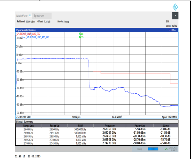
1-N41-30-50-H-3-DFT-PI2BPSK-Outer_Full-128@0-Ant1-1--PASS-see graph
