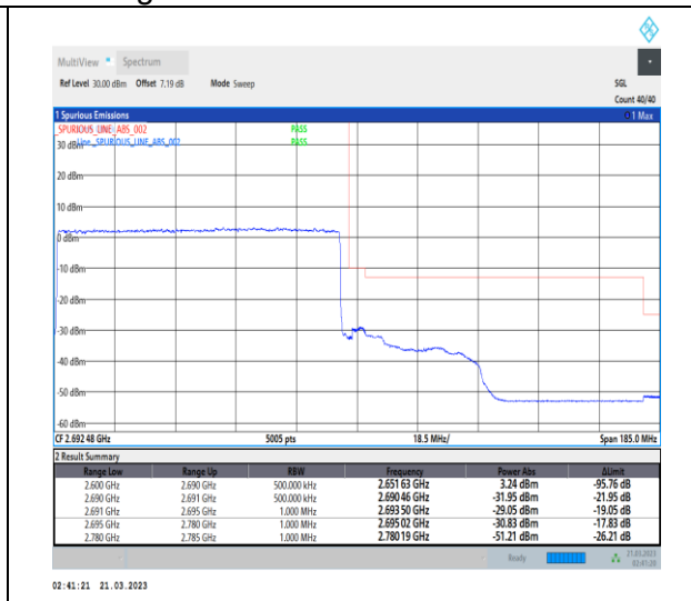
1-N41-30-90-H-3-DFT-PI2BPSK-Outer_Full-240@0-Ant1-1--PASS-see graph
