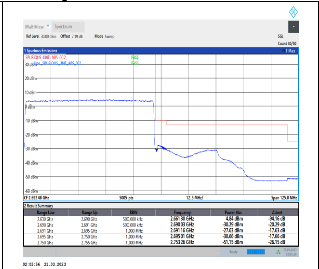
1-N41-30-60-H-3-DFT-PI2BPSK-Outer_Full-162@0-Ant1-1--PASS-see graph
