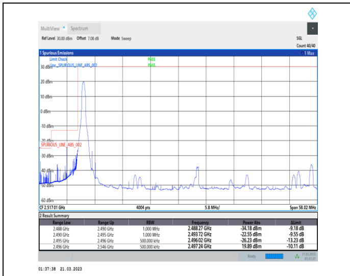
1-N41-30-50-L-1-DFT-PI2BPSK-Edge_1RB_Left-1@0-Ant1-1--PASS-see graph
