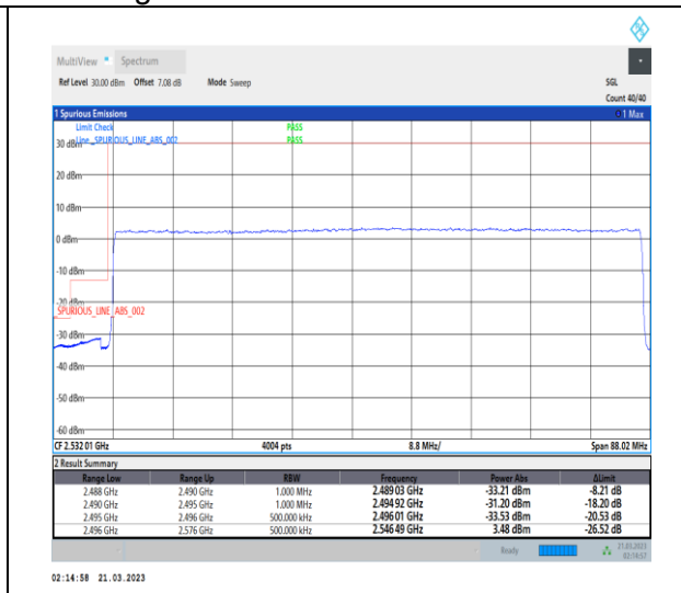
1-N41-30-80-L-3-DFT-PI2BPSK-Outer_Full-216@0-Ant1-1--PASS-see graph
