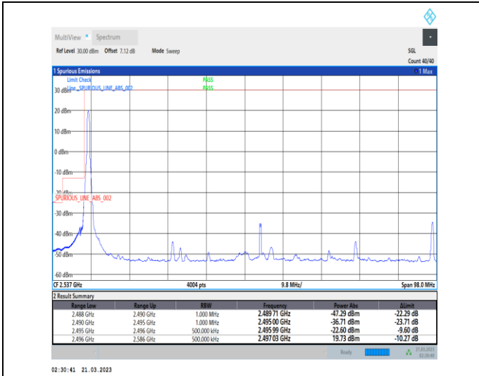
1-N41-30-90-L-1-DFT-PI2BPSK-Edge_1RB_Left-1@0-Ant1-1--PASS-see graph
