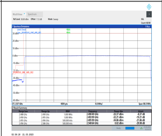
1-N41-30-90-L-6-CP-QPSK-Outer_Full-245@0-Ant1-1--PASS-see graph
