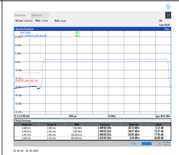
1-N41-30-40-L-6-CP-QPSK-Outer_Full-106@0-Ant1-1--PASS-see graph
