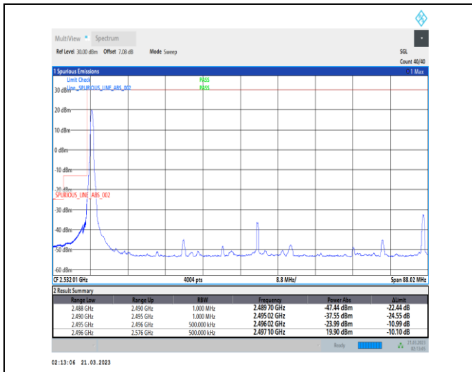
1-N41-30-80-L-1-DFT-PI2BPSK-Edge_1RB_Left-1@0-Ant1-1--PASS-see graph
