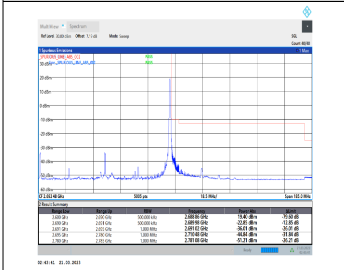
1-N41-30-90-H-5-CP-QPSK-Edge_1RB_Right-1@244-Ant1-1--PASS-see graph
