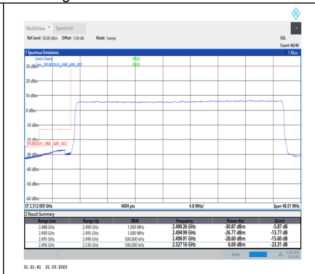
1-N41-30-40-L-3-DFT-PI2BPSK-Outer_Full-100@0-Ant1-1--PASS-see graph
