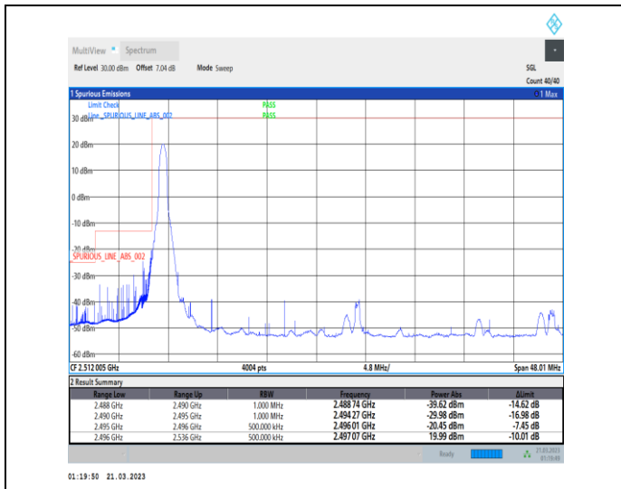
1-N41-30-40-L-1-DFT-PI2BPSK-Edge_1RB_Left-1@0-Ant1-1--PASS-see graph
