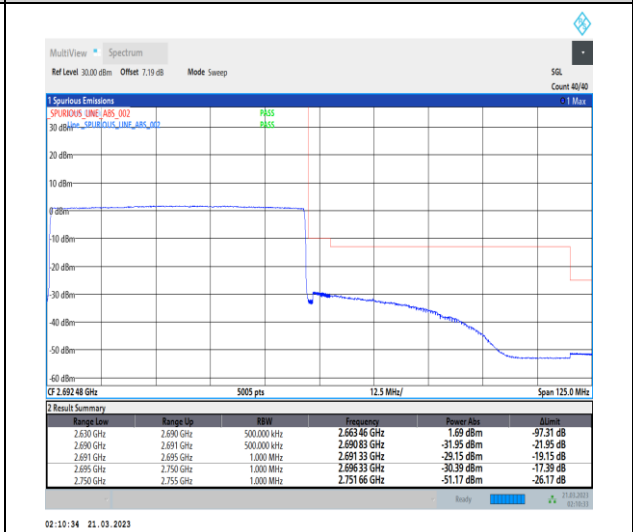
1-N41-30-60-H-6-CP-QPSK-Outer_Full-162@0-Ant1-1--PASS-see graph
