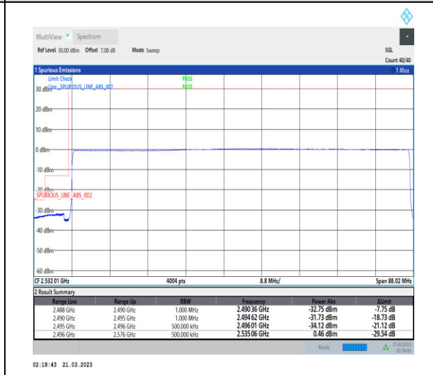
1-N41-30-80-L-6-CP-QPSK-Outer_Full-217@0-Ant1-1--PASS-see graph
