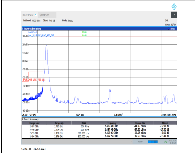
1-N41-30-50-L-4-CP-QPSK-Edge_1RB_Left-1@0-Ant1-1--PASS-see graph
