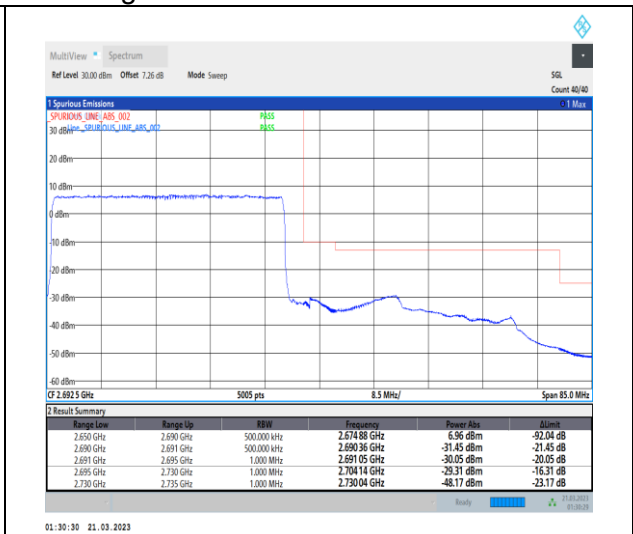
1-N41-30-40-H-3-DFT-PI2BPSK-Outer_Full-100@0-Ant1-1--PASS-see graph
