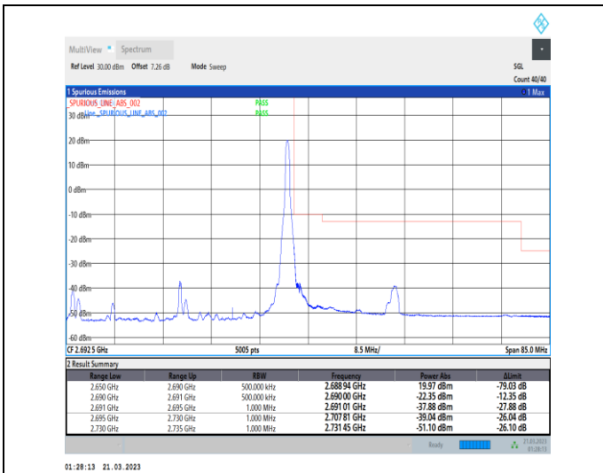
1-N41-30-40-H-2-DFT-PI2BPSK-Edge_1RB_Right-1@105-Ant1-1--PASS-see graph
