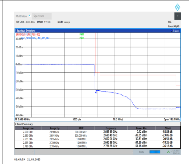
1-N41-30-90-H-6-CP-QPSK-Outer_Full-245@0-Ant1-1--PASS-see graph
