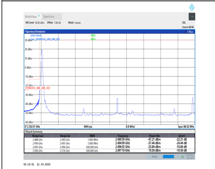
1-N41-30-80-L-4-CP-QPSK-Edge_1RB_Left-1@0-Ant1-1--PASS-see graph
