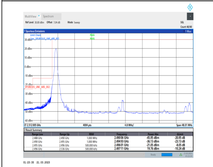
1-N41-30-40-L-4-CP-QPSK-Edge_1RB_Left-1@0-Ant1-1--PASS-see graph
