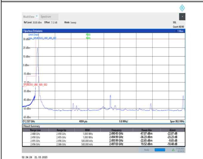
1-N41-30-90-L-4-CP-QPSK-Edge_1RB_Left-1@0-Ant1-1--PASS-see graph
