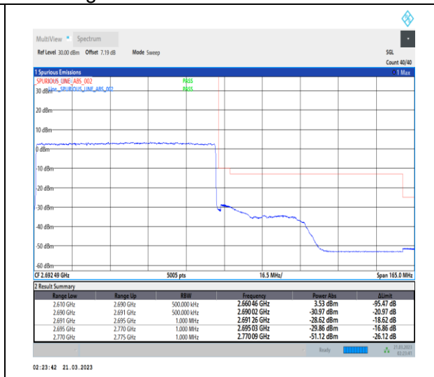
1-N41-30-80-H-3-DFT-PI2BPSK-Outer_Full-216@0-Ant1-1--PASS-see graph
