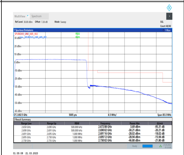
1-N41-30-40-H-6-CP-QPSK-Outer_Full-106@0-Ant1-1--PASS-see graph
