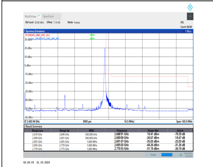
1-N41-30-80-H-5-CP-QPSK-Edge_1RB_Right-1@216-Ant1-1--PASS-see graph
