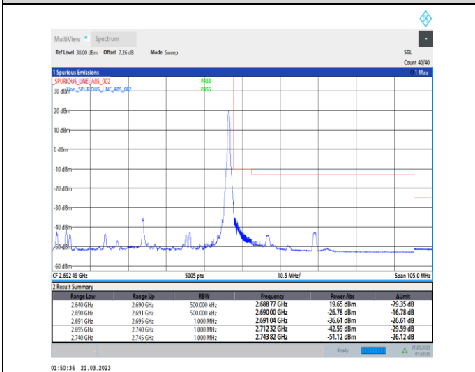
1-N41-30-50-H-5-CP-QPSK-Edge_1RB_Right-1@132-Ant1-1--PASS-see graph
