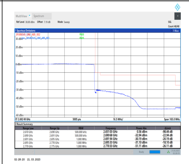
1-N41-30-80-H-6-CP-QPSK-Outer_Full-217@0-Ant1-1--PASS-see graph
