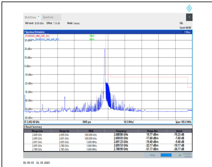
1-N41-30-90-H-2-DFT-PI2BPSK-Edge_1RB_Right-1@244-Ant1-1--PASS-see graph
