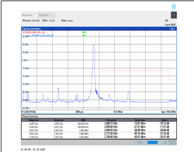
1-N41-30-50-H-2-DFT-PI2BPSK-Edge_1RB_Right-1@132-Ant1-1--PASS-see graph
