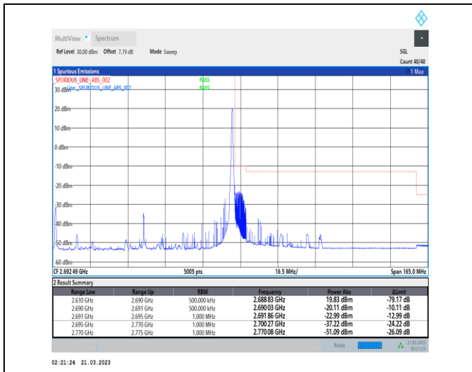
1-N41-30-80-H-2-DFT-PI2BPSK-Edge_1RB_Right-1@216-Ant1-1--PASS-see graph
