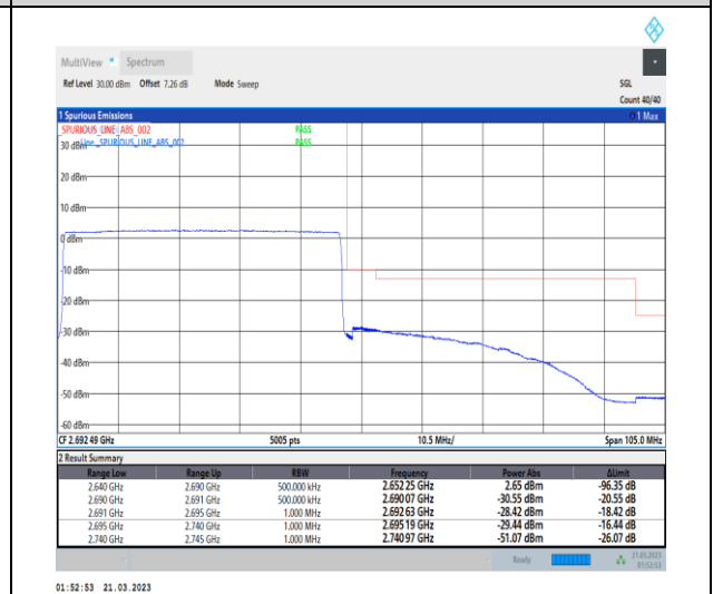
1-N41-30-50-H-6-CP-QPSK-Outer_Full-133@0-Ant1-1--PASS-see graph
