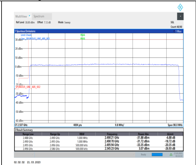
1-N41-30-90-L-3-DFT-PI2BPSK-Outer_Full-240@0-Ant1-1--PASS-see graph
