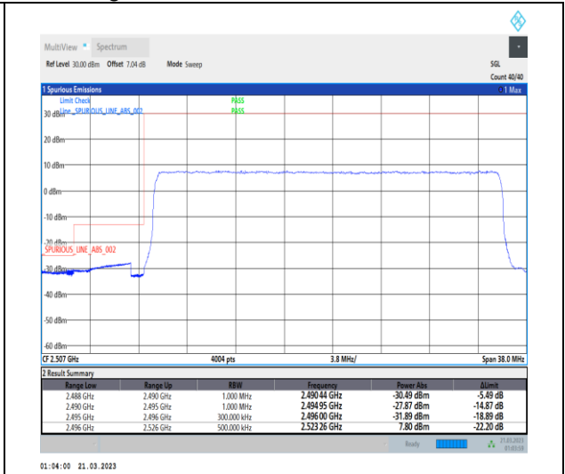
1-N41-30-30-L-3-DFT-PI2BPSK-Outer_Full-75@0-Ant1-1--PASS-see graph
