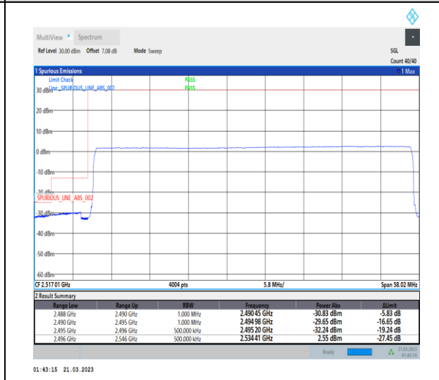
1-N41-30-50-L-6-CP-QPSK-Outer_Full-133@0-Ant1-1--PASS-see graph
