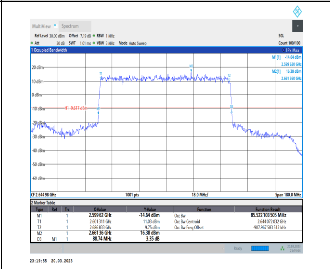
1-N41-30-90-H-2-DFT-PI2BPSK-Outer_Full-240@0-Ant Ant1-85.522-88.740-<90-PASS
