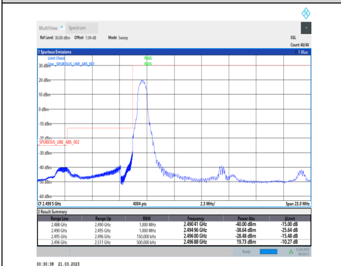
1-N41-30-15-L-4-CP-QPSK-Edge_1RB_Left-1@0-Ant1-1--PASS-see graph
