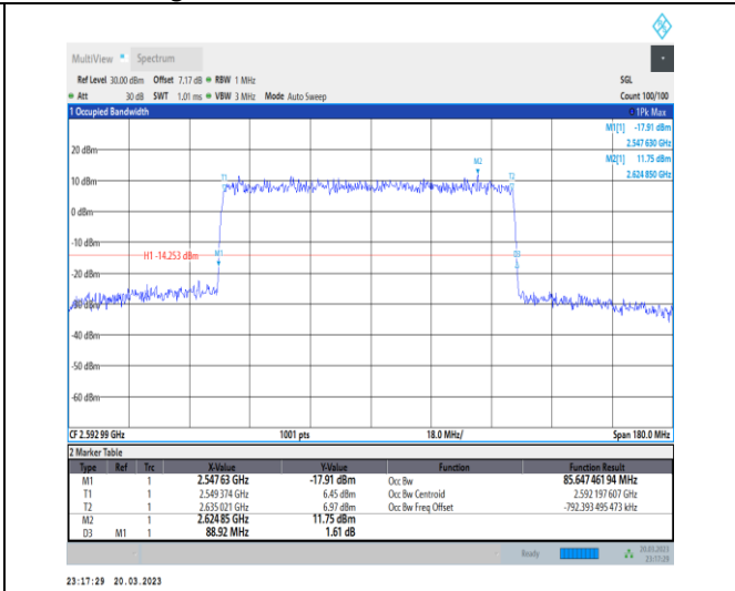
1-N41-30-90-M-5-DFT-256QAM-Outer_Full-240@0-Ant1-85.647-88.920-≤90-PASS
