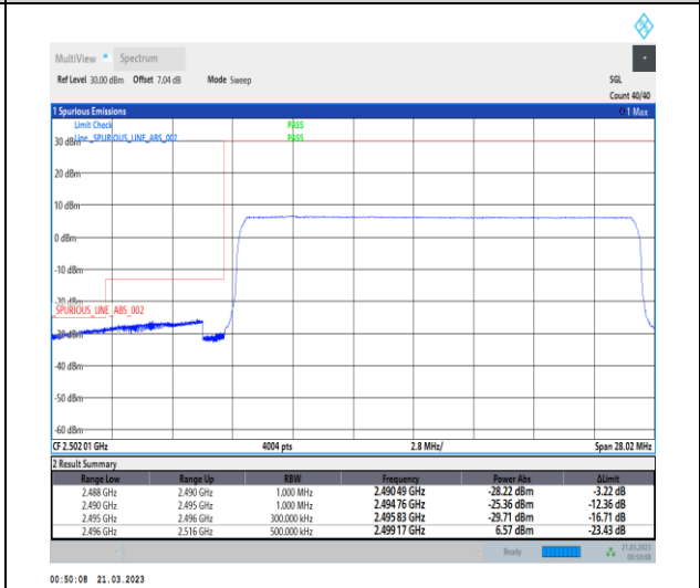
1-N41-30-20-L-6-CP-QPSK-Outer_Full-51@0-Ant1-1--PASS-see graph
