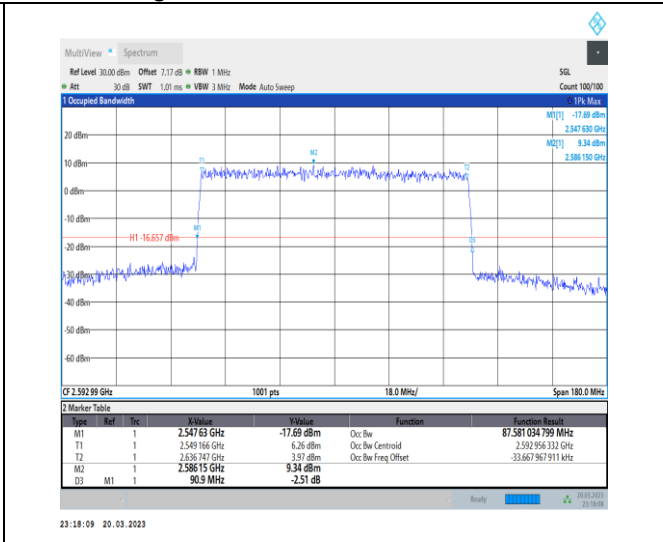
1-N41-30-90-M-9-CP-256QAM-Outer_Full-245@0-A nt1-87.581-90.900-<90-PASS
