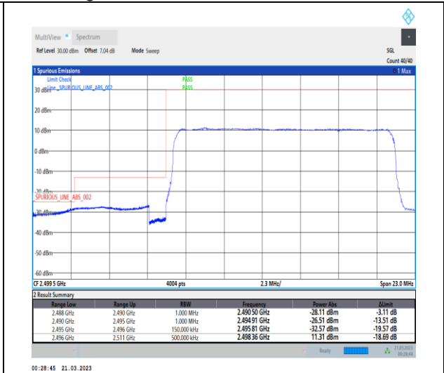
1-N41-30-15-L-3-DFT-PI2BPSK-Outer_Full-36@0-Ant1-1--PASS-see graph
