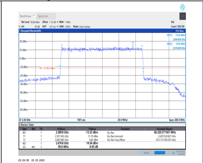
1-N41-30-100-H-1-DFT-QPSK-Outer_Full-270@0-An t1-96.32-99.600-≤100-PASS
