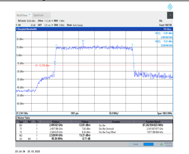
1-N41-30-90-L-6-CP-QPSK-Outer_Full-245@0-Ant1-87.243-90.360-≤90-PASS
