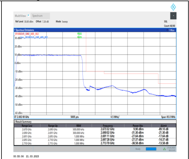
1-N41-30-20-H-3-DFT-PI2BPSK-Outer_Full-50@0-Ant1-1--PASS-see graph
