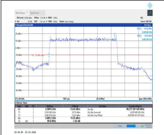
1-N41-30-100-H-2-DFT-PI2BPSK-Outer_Full-270@0-Ant1-96.272-99.800-≤100-PASS
