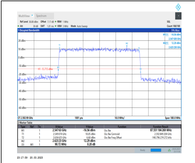
1-N41-30-90-M-8-CP-64QAM-Outer_Full-245@0-An t1-87.551-90.720-<90-PASS
