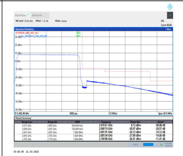
1-N41-30-15-H-6-CP-QPSK-Outer_Full-38@0-Ant1-1--PASS-see graph
