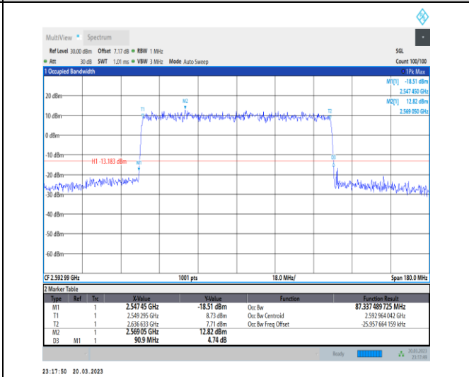
1-N41-30-90-M-7-CP-16QAM-Outer_Full-245@0-Ant 1-87.337-90.900-≤90-PASS
