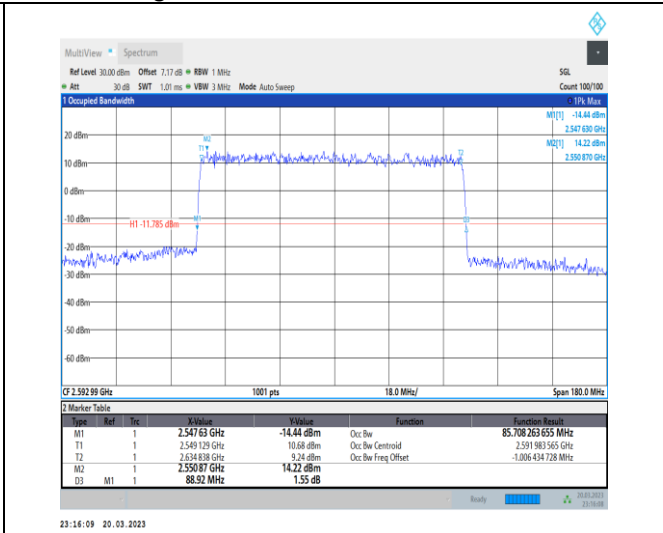
1-N41-30-90-M-1-DFT-QPSK-Outer_Full-240@0-Ant 1-85.708-88.920-≤90-PASS
