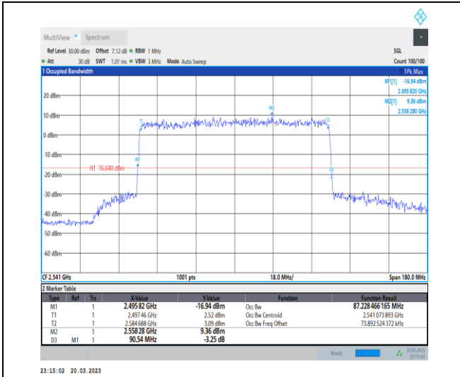
1-N41-30-90-L-9-CP-256QAM-Outer_Full-245@0-A nt1-87.228-90.540-≤90-PASS
