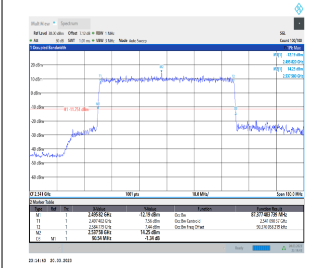
1-N41-30-90-L-7-CP-16QAM-Outer_Full-245@0-Ant1-87.377-90.540-≤90-PASS
