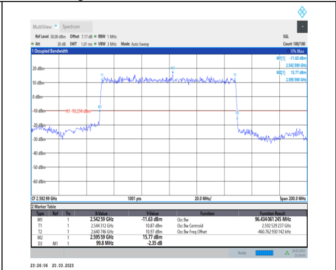
1-N41-30-100-M-2-DFT-PI2BPSK-Outer_Full-270@0-A -Ant1-96.434-99.800-≤100-PASS
