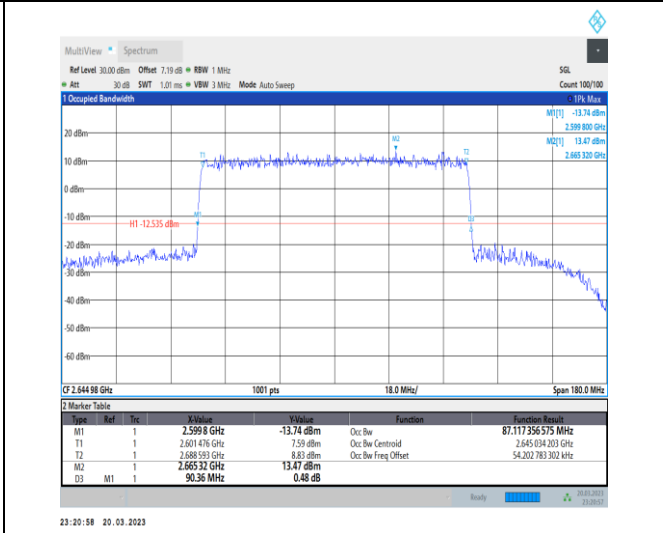
1-N41-30-90-H-6-CP-QPSK-Outer_Full-245@0-Ant1 -87.117-90.360-≤90-PASS
