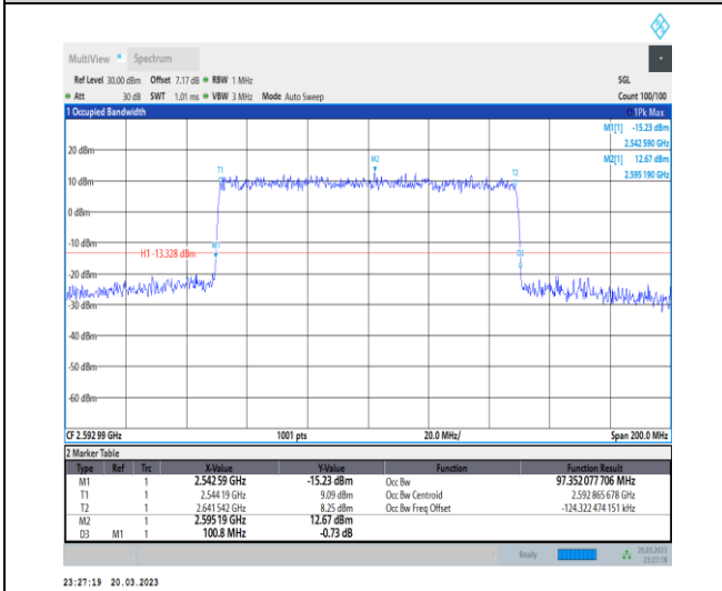
1-N41-30-100-M-7-CP-16QAM-Outer_Full-273@0-Ant1-97.352-100.800-≤100-PASS
