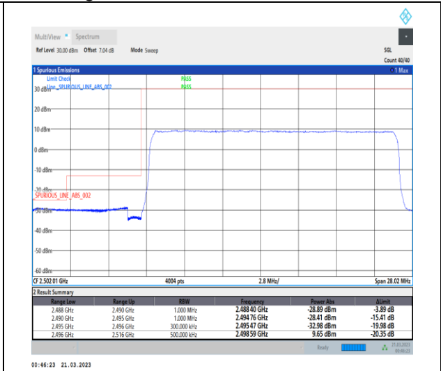
1-N41-30-20-L-3-DFT-PI2BPSK-Outer_Full-50@0-Ant1-1--PASS-see graph
