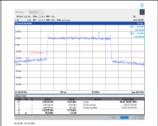
1-N41-30-100-M-4-DFT-64QAM-Outer_Full-270@0-A Ant1-96.242-99.800-≤100-PASS
