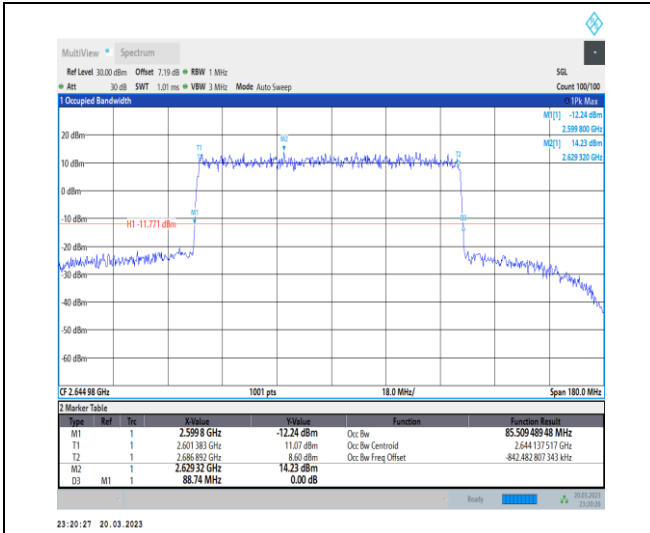
1-N41-30-90-H-3-DFT-16QAM-Outer_Full-240@0-A nt1-85.509-88.740-≤90-PASS
