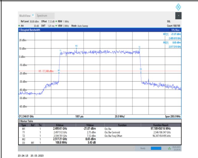
1-N41-30-100-L-9-CP-256QAM-Outer_Full-273@0-A nt1-97.189-100.800-≤100-PASS
