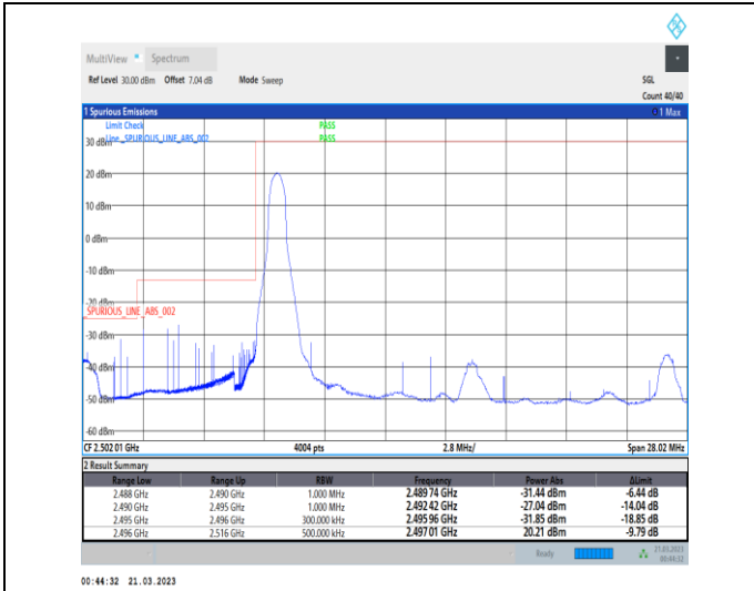
1-N41-30-20-L-1-DFT-PI2BPSK-Edge_1RB_Left-1@0-Ant1-1--PASS-see graph
