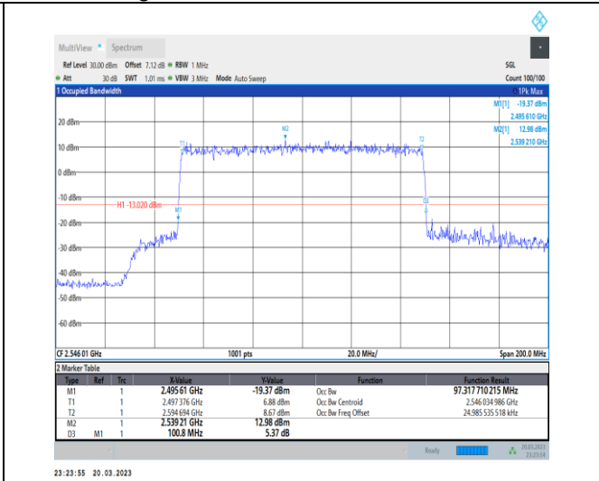
1-N41-30-100-L-7-CP-16QAM-Outer_Full-273@0-An t1-97.318-100.800-≤100-PASS
