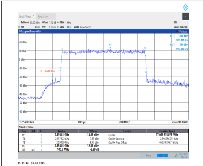
1-N41-30-100-L-6-CP-QPSK-Outer_Full-273@0-Ant 1-97.069-100.600-≤100-PASS
