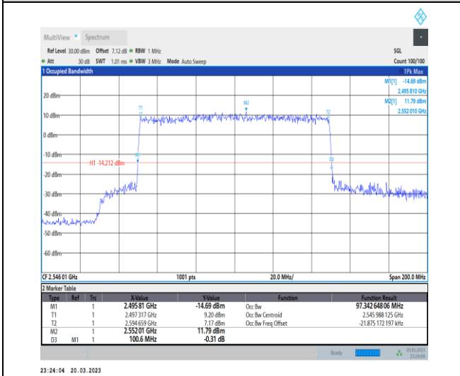
1-N41-30-100-L-8-CP-64QAM-Outer_Full-273@0-A nt1-97.343-100.600-≤100-PASS
