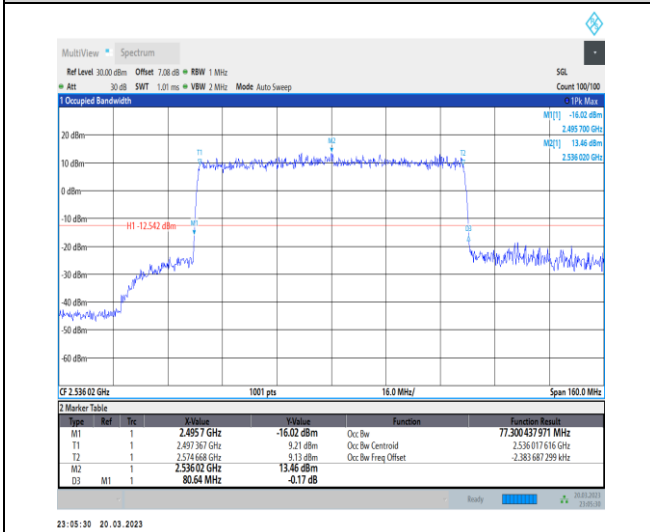
1-N41-30-80-L-6-CP-QPSK-Outer_Full-217@0-Ant1 -77.3-80.640-<math>\leq 80</math>-PASS
