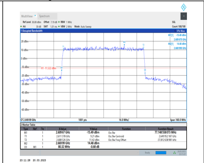
1-N41-30-80-H-3-DFT-16QAM-Outer_Full-216@0-Ant1-77.149-80.320-≤80-PASS
