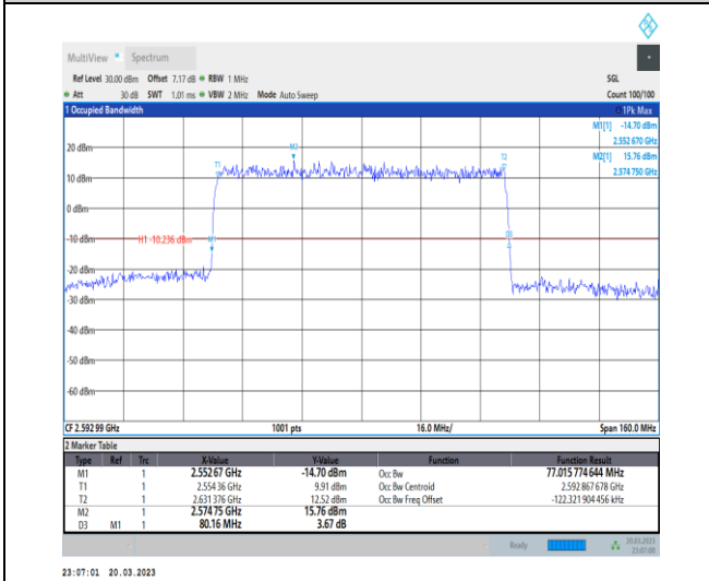
1-N41-30-80-M-1-DFT-QPSK-Outer_Full-216@0-Ant 1-77.016-80.160-≤80-PASS
