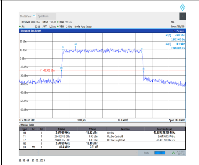
1-N41-30-50-H-7-CP-16QAM-Outer_Full-133@0-Ant 1-47.339-49.400-≤50-PASS
