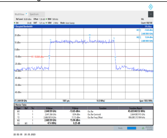
1-N41-30-50-H-1-DFT-QPSK-Outer_Full-128@0-Ant 1-45.636-47.400-≤50-PASS
