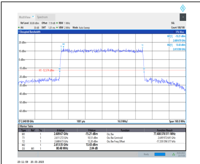
1-N41-30-80-H-6-CP-QPSK-Outer_Full-217@0-Ant1 -77.4-80.480-≤80-PASS
