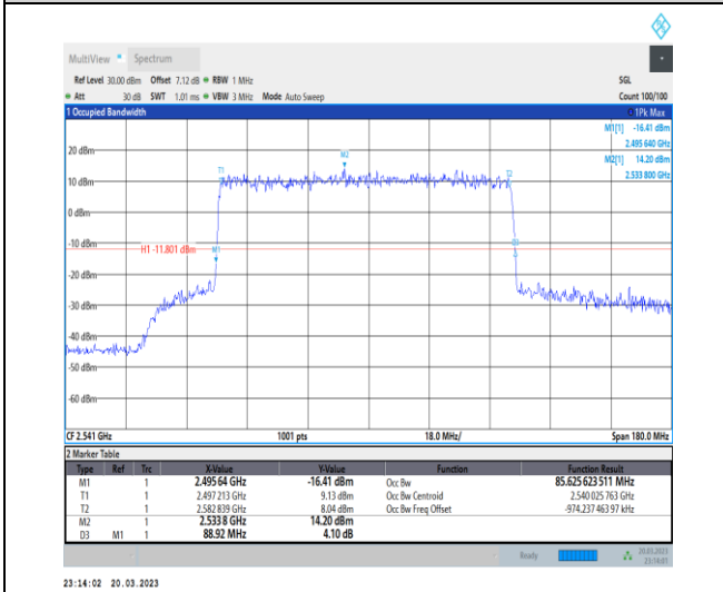
1-N41-30-90-L-3-DFT-16QAM-Outer_Full-240@0-Ant1-85.626-88.920-≤90-PASS
