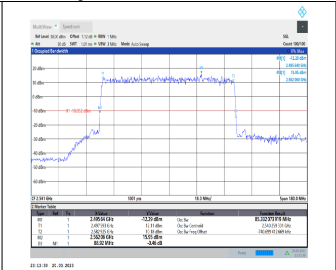
1-N41-30-90-L-2-DFT-PI2BPSK-Outer_Full-240@0-Ant1-85.332-88.920-≤90-PASS
