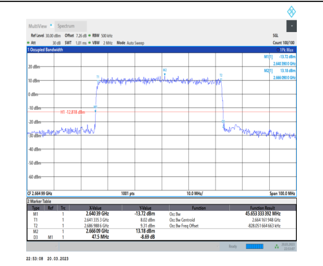
1-N41-30-50-H-3-DFT-16QAM-Outer_Full-128@0-Ant 1-45.653-47.500-≤50-PASS
