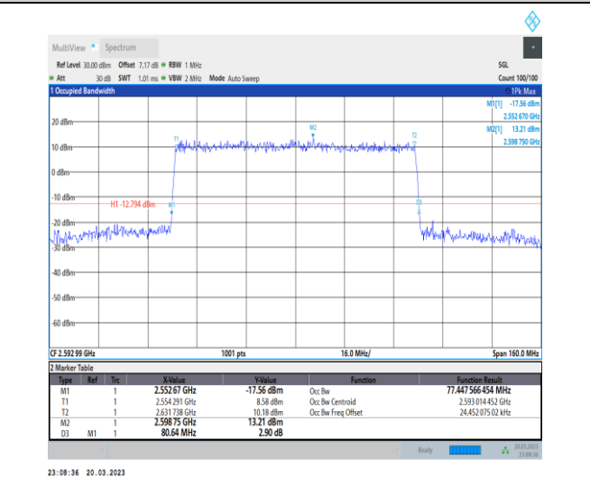
1-N41-30-80-M-6-CP-QPSK-Outer_Full-217@0-Ant1 -77.448-80.640-≤80-PASS
