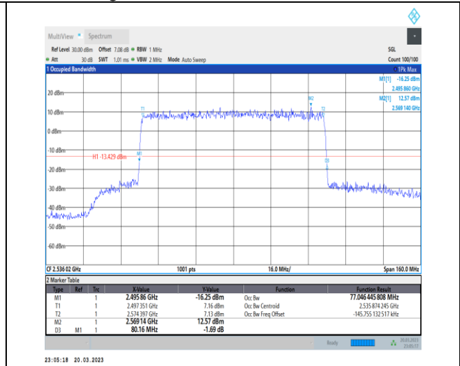
1-N41-30-80-L-5-DFT-256QAM-Outer_Full-216@0-A nt1-77.046-80.160-<math>\leq 80</math>-PASS
