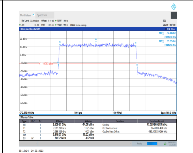
1-N41-30-80-H-1-DFT-QPSK-Outer_Full-216@0-Ant 1-77.04-80.320-<=80-PASS
