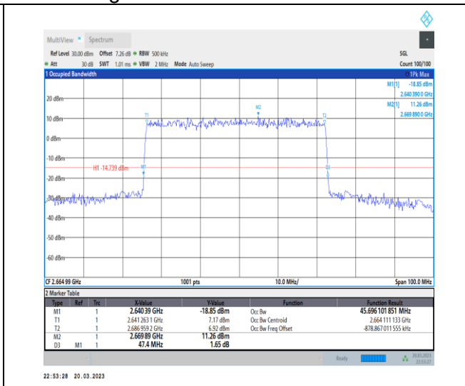
1-N41-30-50-H-5-DFT-256QAM-Outer_Full-128@0-A nt1-45.696-47.400-≤50-PASS
