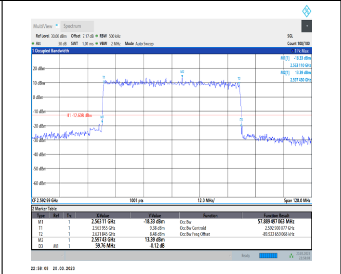
1-N41-30-60-M-1-DFT-QPSK-Outer_Full-162@0-Ant 1-57.889-59.760-≤60-PASS
