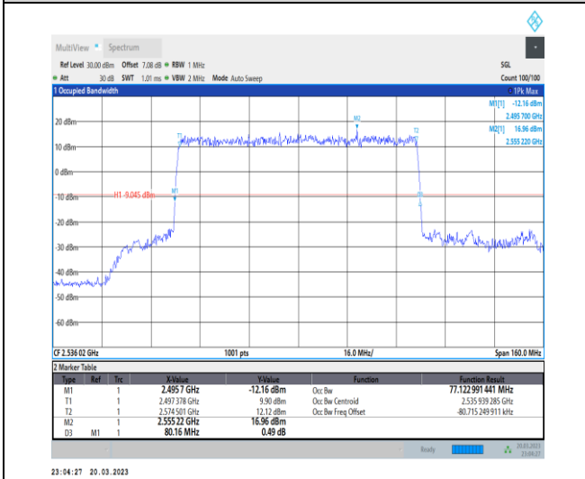
1-N41-30-80-L-2-DFT-PI2BPSK-Outer_Full-216@0-Ant1 Ant1-77.123-80.160-≤80-PASS
