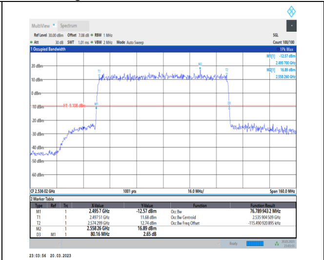
1-N41-30-80-L-1-DFT-QPSK-Outer_Full-216@0-Ant 1-76.79-80.160-≤80-PASS
