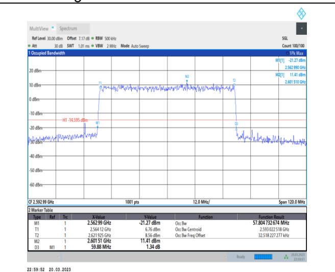
1-N41-30-60-M-7-CP-16QAM-Outer_Full-162@0-Ant 1-57.805-59.880-≤60-PASS
