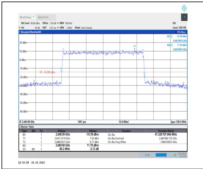
1-N41-30-50-H-8-CP-64QAM-Outer_Full-133@0-Ant 1-47.321-49.200-≤50-PASS
