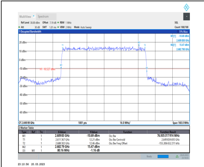
1-N41-30-80-H-2-DFT-PI2BPSK-Outer_Full-216@0-Ant1-76.935-80.160-≤80-PASS
