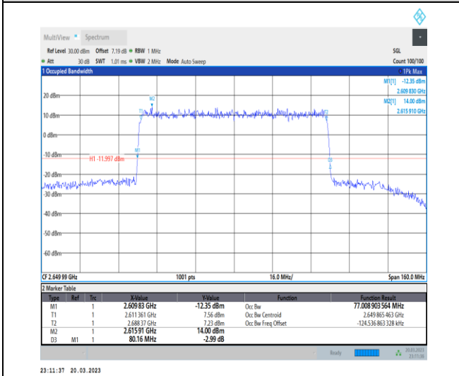
1-N41-30-80-H-4-DFT-64QAM-Outer_Full-216@0-Ant1-77.009-80.160-≤80-PASS
