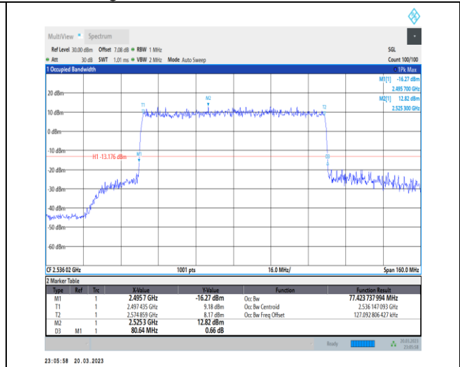
1-N41-30-80-L-9-CP-256QAM-Outer_Full-217@0-Ant t1-77.424-80.640-≤80-PASS
