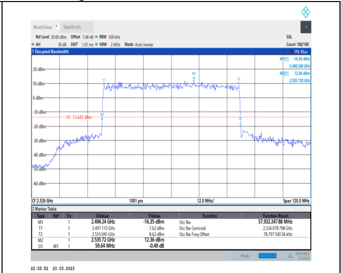
1-N41-30-60-L-4-DFT-64QAM-Outer_Full-162@0-Ant1-57.932-59.640-≤60-PASS
