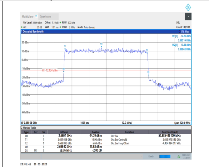
1-N41-30-60-H-2-DFT-PI2BPSK-Outer_Full-162@0-Ant 1-57.835-59.760-≤60-PASS
