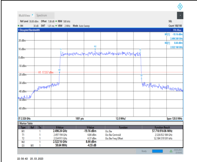
1-N41-30-60-L-9-CP-256QAM-Outer_Full-162@0-A nt1-57.717-59.640-≤60-PASS
