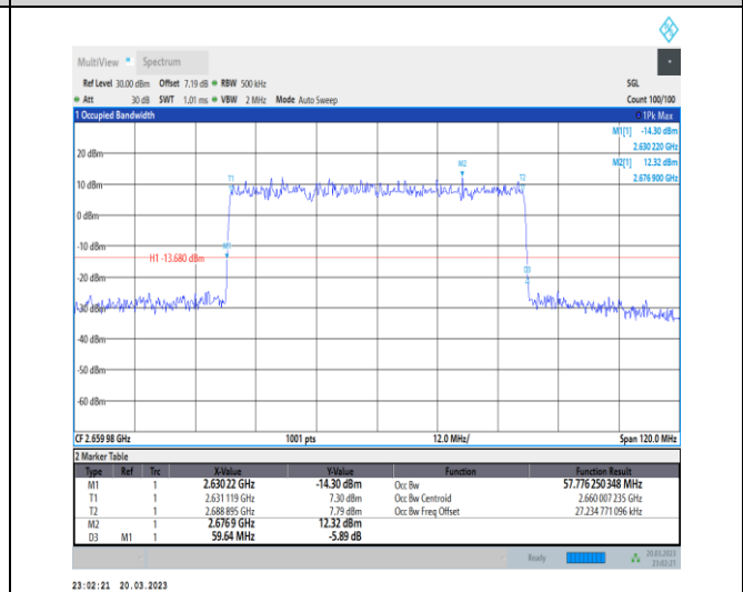
1-N41-30-60-H-4-DFT-64QAM-Outer_Full-162@0-Ant 1-57.776-59.640-≤60-PASS
