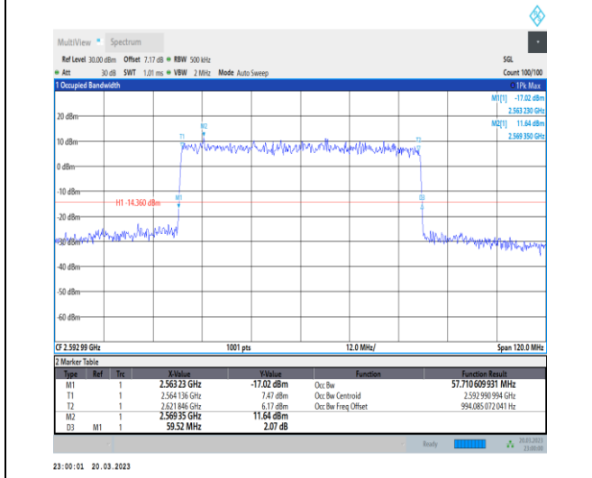
1-N41-30-60-M-8-CP-64QAM-Outer_Full-162@0-Ant t1-57.711-59.520-≤60-PASS
