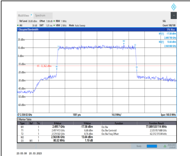
1-N41-30-80-L-4-DFT-64QAM-Outer_Full-216@0-A nt1-77.09-80.320-<math>\leq 80</math>-PASS
