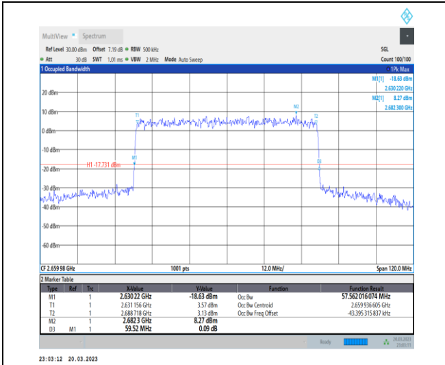
1-N41-30-60-H-9-CP-256QAM-Outer_Full-162@0-A nt1-57.562-59.520-≤60-PASS
