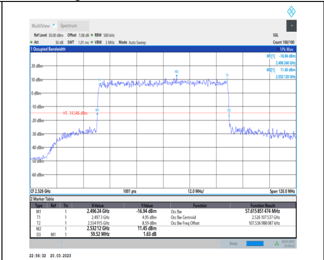
1-N41-30-60-L-8-CP-64QAM-Outer_Full-162@0-Ant 1-57.616-59.520-≤60-PASS
