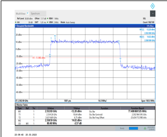
1-N41-30-80-M-7-CP-16QAM-Outer_Full-217@0-An t1-77.409-80.480-<=80-PASS
