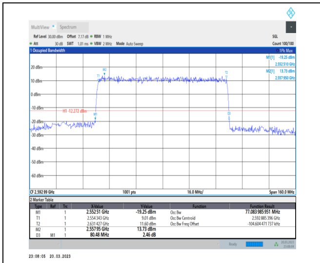
1-N41-30-80-M-3-DFT-16QAM-Outer_Full-216@0-A nt1-77.084-80.480-≤80-PASS
