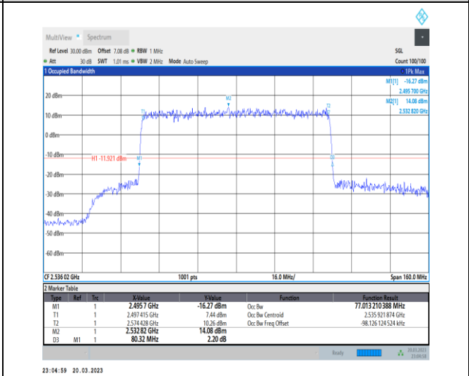
1-N41-30-80-L-3-DFT-16QAM-Outer_Full-216@0-Ant t1-77.013-80.320-≤80-PASS
