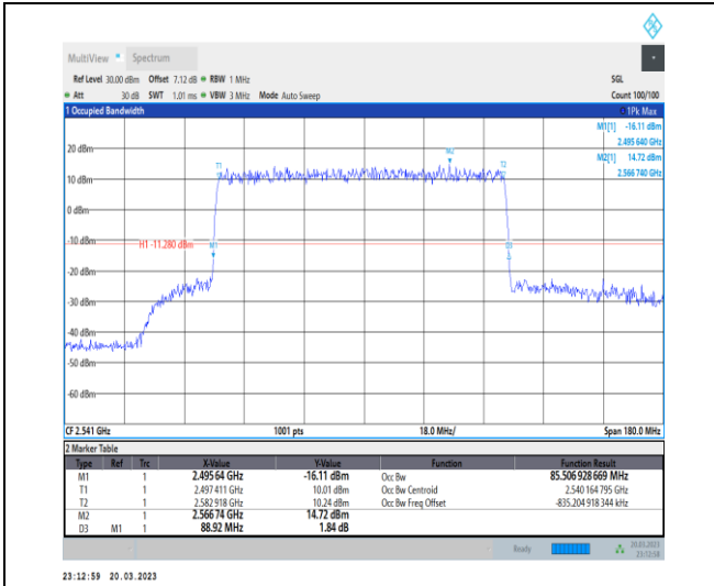
1-N41-30-90-L-1-DFT-QPSK-Outer_Full-240@0-Ant 1-85.507-88.920-≤90-PASS
