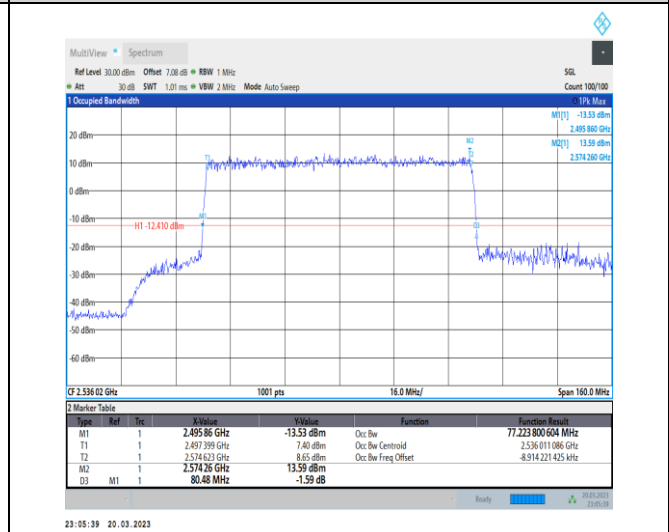
1-N41-30-80-L-7-CP-16QAM-Outer_Full-217@0-Ant1 -77.224-80.480-<math>\leq 80</math>-PASS
