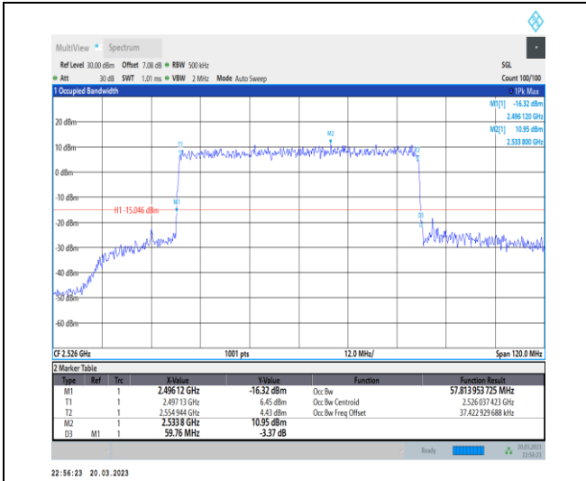
1-N41-30-60-L-7-CP-16QAM-Outer_Full-162@0-Ant 1-57.814-59.760-≤60-PASS
