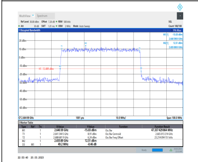
1-N41-30-50-H-6-CP-QPSK-Outer_Full-133@0-Ant1 -47.337-49.200-≤50-PASS
