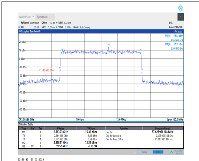
1-N41-30-60-M-6-CP-QPSK-Outer_Full-162@0-Ant 1-57.627-59.520-≤60-PASS
