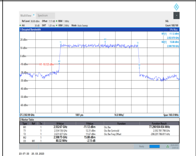
1-N41-30-80-M-2-DFT-PI2BPSK-Outer_Full-216@0-Ant Ant1-77.291-80.320-≤80-PASS
