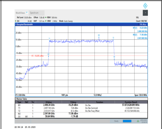
1-N41-30-60-L-6-CP-QPSK-Outer_Full-162@0-Ant1-57.873-59.640-≤60-PASS
