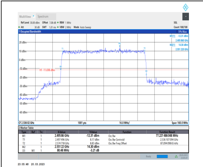
1-N41-30-80-L-8-CP-64QAM-Outer_Full-217@0-Ant 1-77.221-80.480-≤80-PASS
