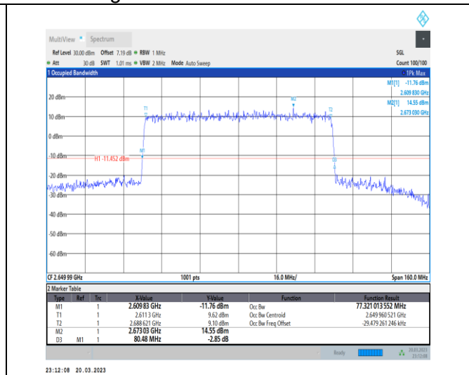
1-N41-30-80-H-7-CP-16QAM-Outer_Full-217@0-Ant 1-77.321-80.480-≤80-PASS
