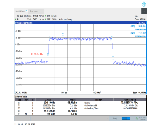
1-N41-30-50-M-8-CP-64QAM-Outer_Full-133@0-Ant1-47.415-49.500-≤50-PASS
