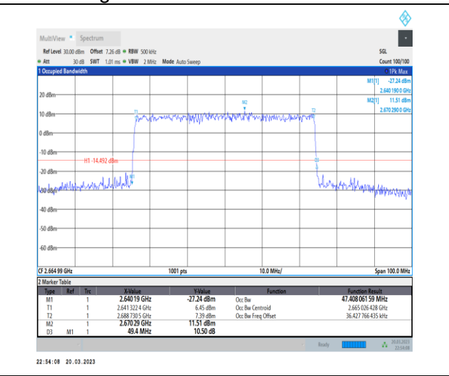
1-N41-30-50-H-9-CP-256QAM-Outer_Full-133@0-A nt1-47.408-49.400-≤50-PASS
