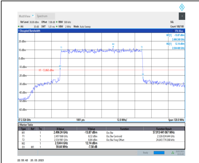
1-N41-30-60-L-3-DFT-16QAM-Outer_Full-162@0-Ant1-57.913-59.640-≤60-PASS
