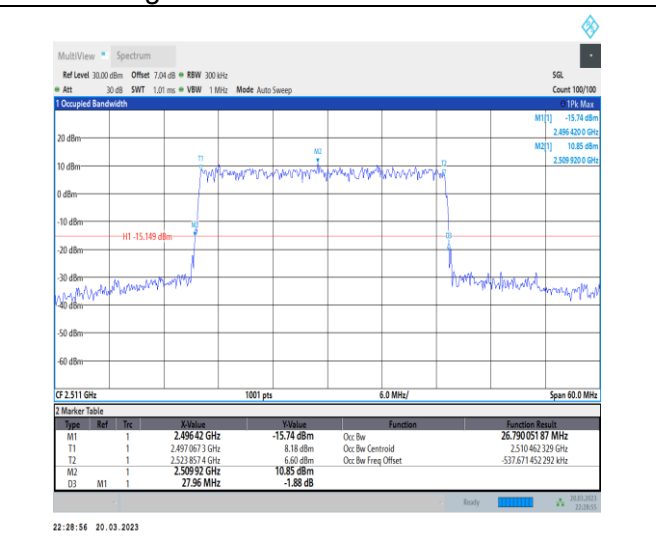
1-N41-30-30-L-5-DFT-256QAM-Outer_Full-75@0-An t1-26.79-27.960-≤30-PASS
