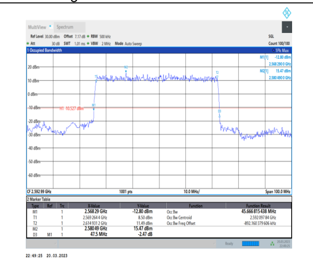
1-N41-30-50-M-2-DFT-PI2BPSK-Outer_Full-128@0-Ant 1-45.667-47.500-≤50-PASS
