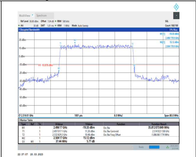
1-N41-30-40-L-2-DFT-PI2BPSK-Outer_Full-100@0-Ant 1-35.812-37.440-≤40-PASS
