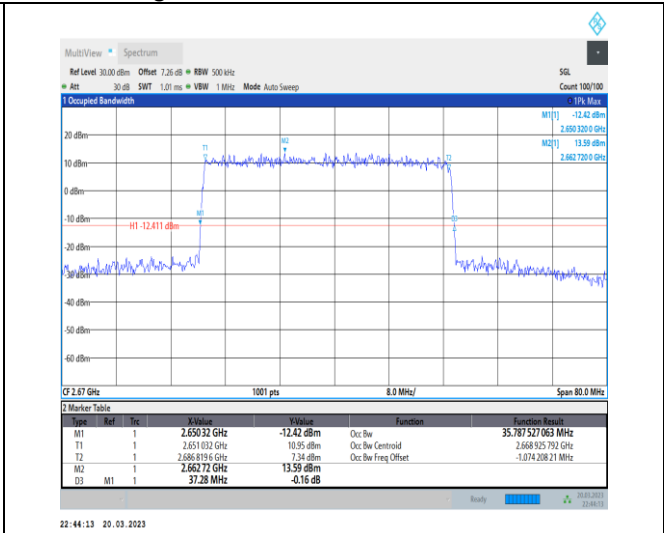
1-N41-30-40-H-4-DFT-64QAM-Outer_Full-100@0-A t1-35.788-37.280-≤40-PASS
