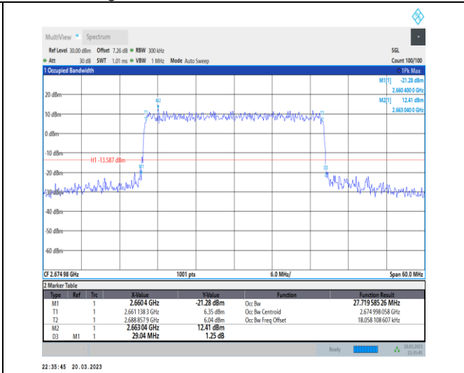
1-N41-30-30-H-7-CP-16QAM-Outer_Full-78@0-Ant1-27.72-29.040-<30-PASS
