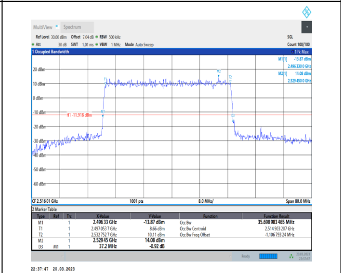
1-N41-30-40-L-4-DFT-64QAM-Outer_Full-100@0-Ant 1-35.699-37.200-≤40-PASS
