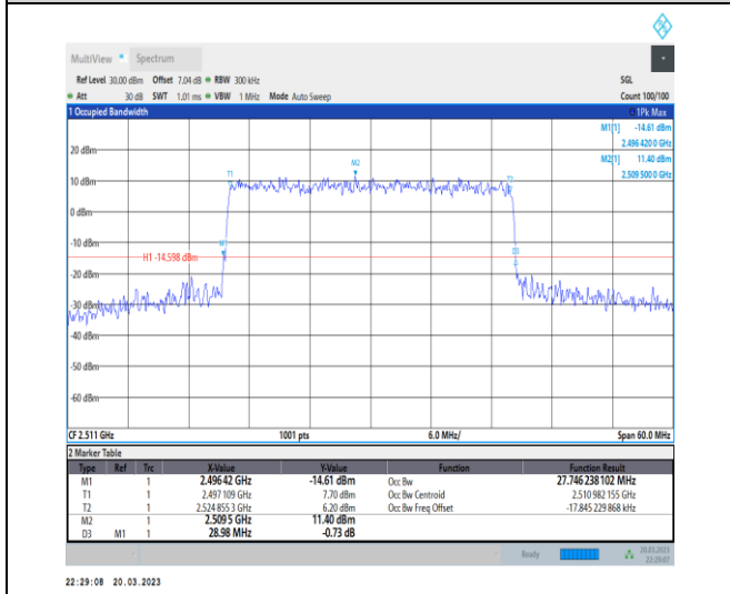
1-N41-30-30-L-6-CP-QPSK-Outer_Full-78@0-Ant1- 27.746-28.980-≤30-PASS
