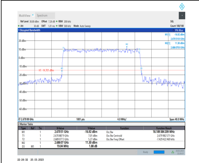
1-N41-30-20-H-7-CP-16QAM-Outer_Full-51@0-Ant1 -18.189-19.040-≤20-PASS
