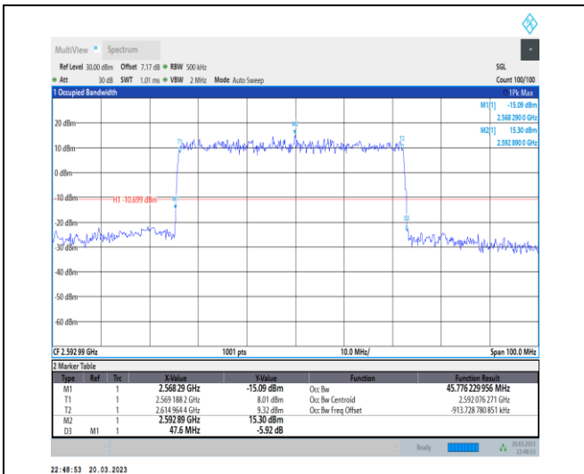
1-N41-30-50-M-1-DFT-QPSK-Outer_Full-128@0-Ant 1-45.776-47.600-≤50-PASS
