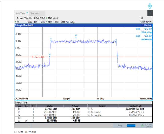
1-N41-30-40-M-8-CP-64QAM-Outer_Full-106@0-An t1-37.848-39.360-<40-PASS
