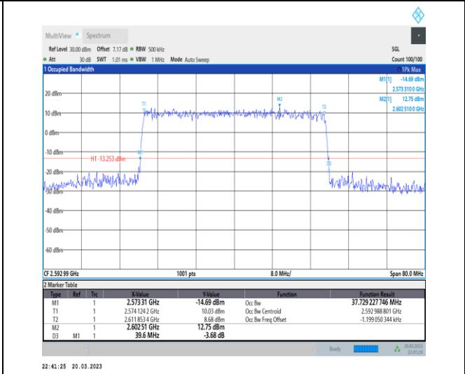
1-N41-30-40-M-7-CP-16QAM-Outer_Full-106@0-Ant 1-37.729-39.600-≤40-PASS
