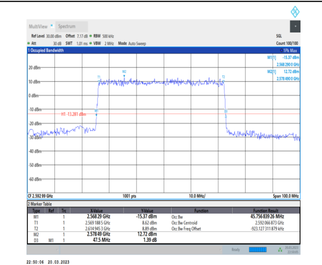
1-N41-30-50-M-4-DFT-64QAM-Outer_Full-128@0-Ant 1-45.757-47.500-≤50-PASS
