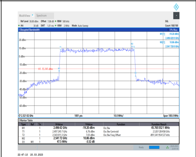
1-N41-30-50-L-5-DFT-256QAM-Outer_Full-128@0-Ant1-45.766-47.500-≤50-PASS
