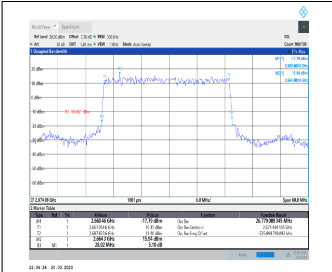
1-N41-30-30-H-2-DFT-PI2BPSK-Outer_Full-75@0-A nt1-26.779-28.020-≤30-PASS
