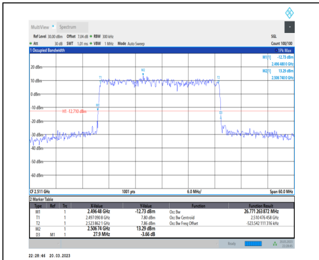
1-N41-30-30-L-4-DFT-64QAM-Outer_Full-75@0-Ant 1-26.771-27.900-≤30-PASS
