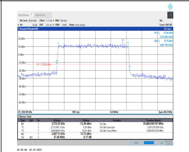
1-N41-30-40-M-3-DFT-16QAM-Outer_Full-100@0-A nt1-35.869-37.360-≤40-PASS
