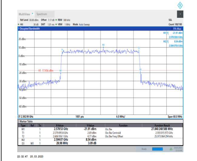
1-N41-30-30-M-9-CP-256QAM-Outer_Full-78@0-An t1-27.84-28.980-≤30-PASS
