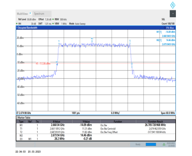
1-N41-30-30-H-1-DFT-QPSK-Outer_Full-75@0-Ant1 26.706-28.200-≤30-PASS
