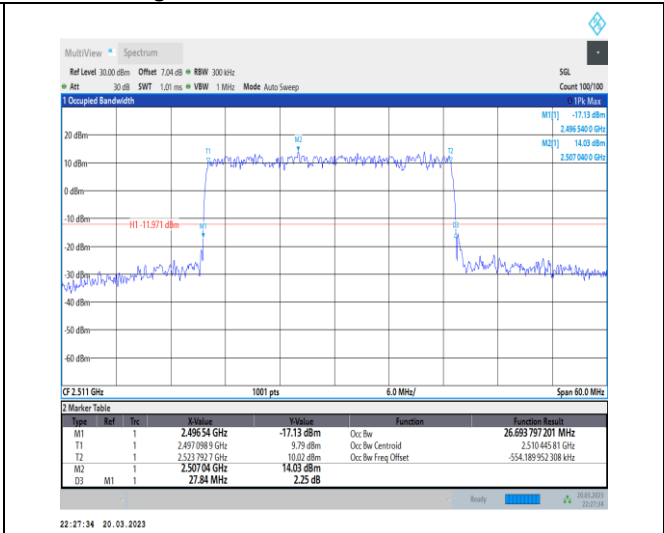
1-N41-30-30-L-1-DFT-QPSK-Outer_Full-75@0-Ant1 26.694-27.840-≤30-PASS
