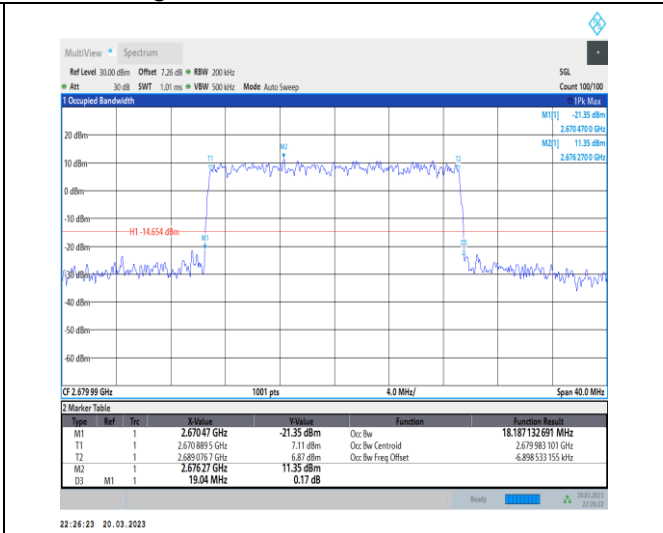
1-N41-30-20-H-6-CP-QPSK-Outer_Full-51@0-Ant1 18.187-19.040-≤20-PASS
