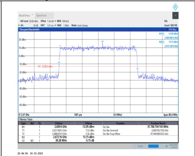
1-N41-30-40-H-8-CP-64QAM-Outer_Full-106@0-Ant 1-37.767-39.280-≤40-PASS
