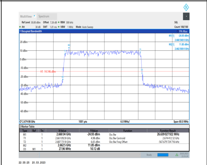
1-N41-30-30-H-5-DFT-256QAM-Outer_Full-75@0-Ant 1-26.639-27.960-≤30-PASS
