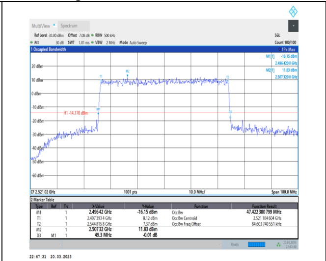
1-N41-30-50-L-7-CP-16QAM-Outer_Full-133@0-Ant 1-47.422-49.300-≤50-PASS
