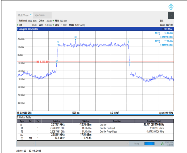
1-N41-30-40-M-2-DFT-PI2BPSK-Outer_Full-100@0-Ant1 Ant1-35.771-37.200-≤40-PASS
