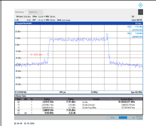
1-N41-30-20-H-8-CP-64QAM-Outer_Full-51@0-Ant1 -18.1-18.960-≤20-PASS
