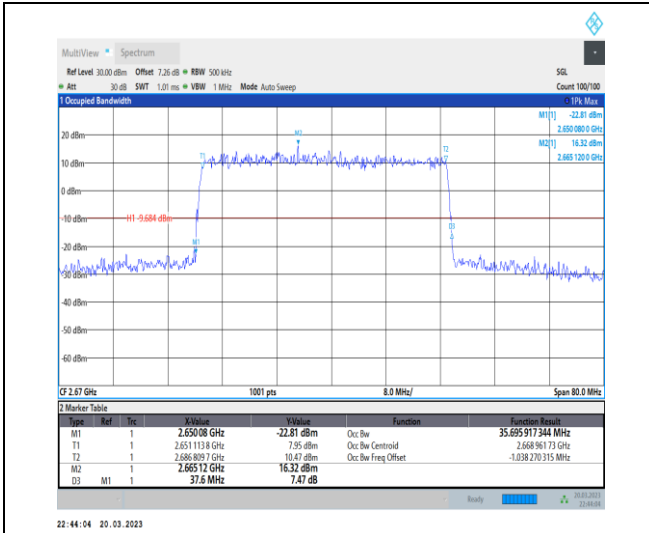
1-N41-30-40-H-3-DFT-16QAM-Outer_Full-100@0-A nt1-35.696-37.600-≤40-PASS
