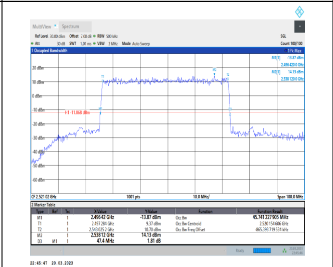
1-N41-30-50-L-1-DFT-QPSK-Outer_Full-128@0-Ant 1-45.741-47.400-≤50-PASS
