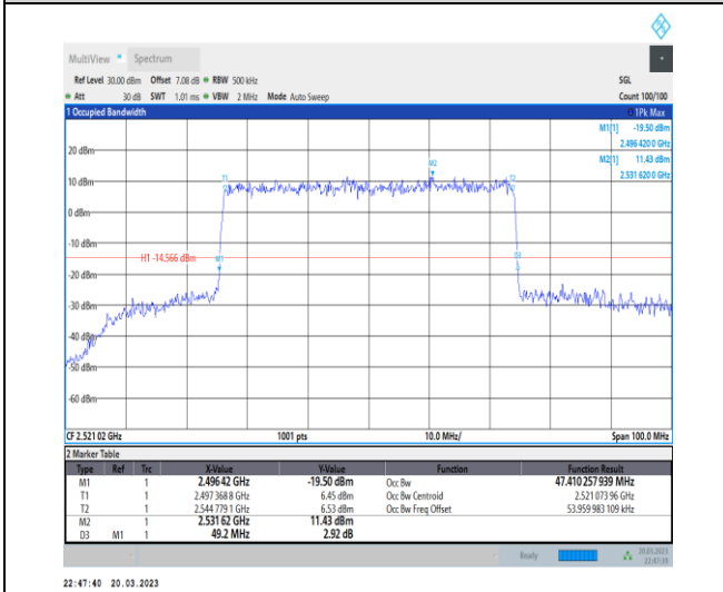
1-N41-30-50-L-8-CP-64QAM-Outer_Full-133@0-Ant 1-47.41-49.200-≤50-PASS
