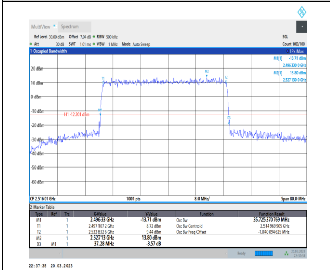
1-N41-30-40-L-3-DFT-16QAM-Outer_Full-100@0-Ant 1-35.725-37.280-≤40-PASS
