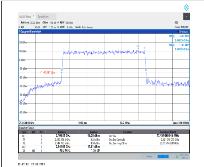
1-N41-30-50-L-6-CP-QPSK-Outer_Full-133@0-Ant1 -47.457-49.300-≤50-PASS
