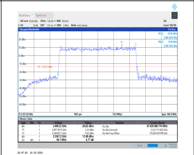
1-N41-30-50-L-9-CP-256QAM-Outer_Full-133@0-Ant t1-47.439-49.700-≤50-PASS
