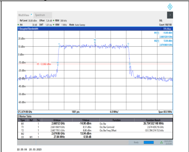
1-N41-30-30-H-3-DFT-16QAM-Outer_Full-75@0-Ant 1-26.735-27.840-≤30-PASS
