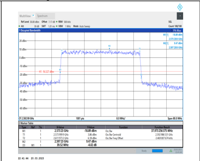
1-N41-30-40-M-9-CP-256QAM-Outer_Full-106@0-A nt1-37.973-39.520-<40-PASS
