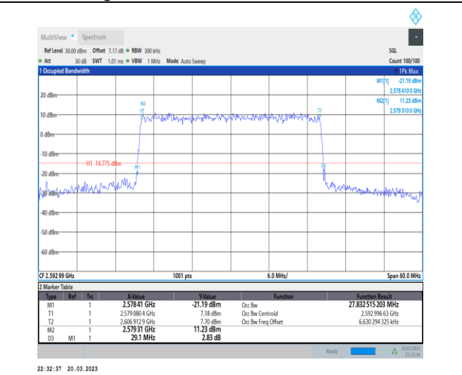
1-N41-30-30-M-8-CP-64QAM-Outer_Full-78@0-Ant1 -27.833-29.100-≤30-PASS
