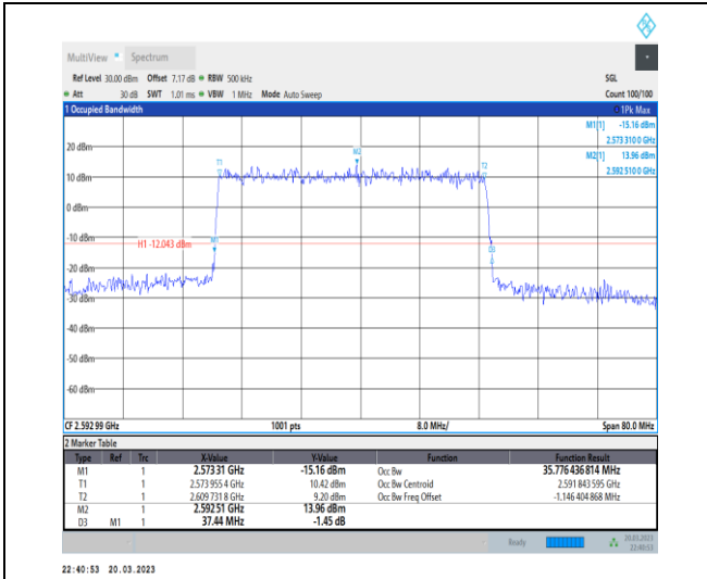
1-N41-30-40-M-4-DFT-64QAM-Outer_Full-100@0-A nt1-35.776-37.440-≤40-PASS
