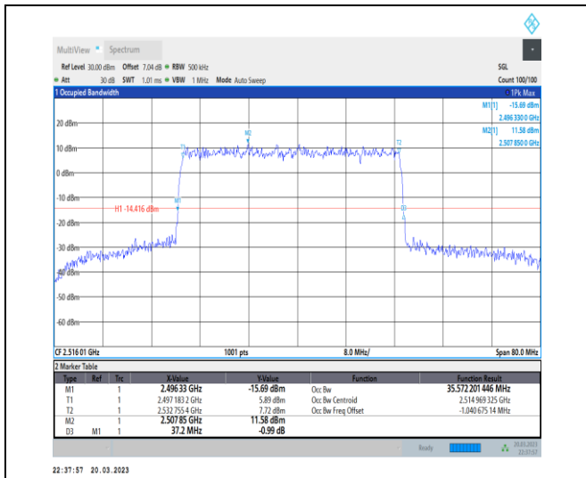
1-N41-30-40-L-5-DFT-256QAM-Outer_Full-100@0-Ant1-35.572-37.200-≤40-PASS
