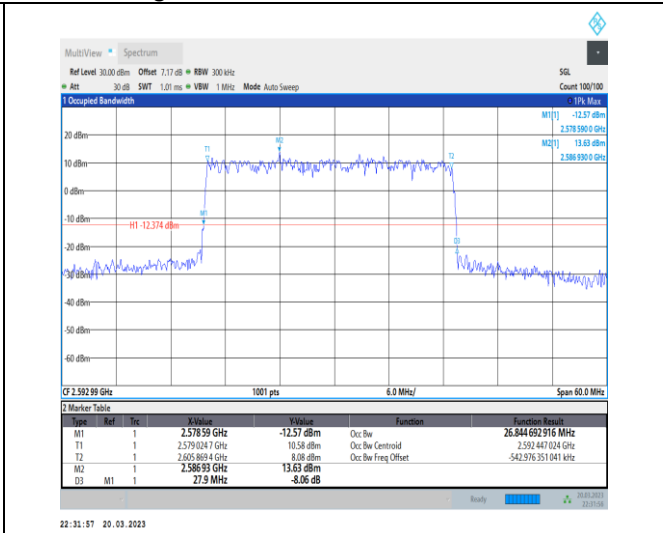
1-N41-30-30-M-4-DFT-64QAM-Outer_Full-75@0-Ant 1-26.845-27.900-≤30-PASS
