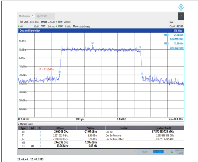
1-N41-30-40-H-7-CP-16QAM-Outer_Full-106@0-Ant 1-37.871-39.760-≤40-PASS
