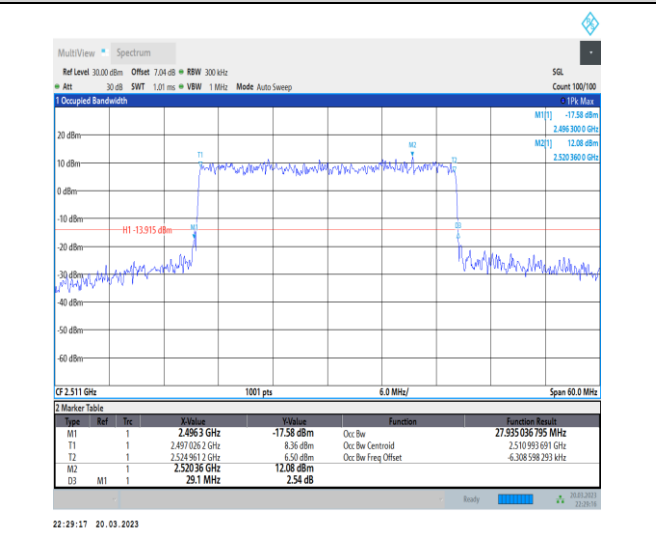
1-N41-30-30-L-7-CP-16QAM-Outer_Full-78@0-Ant1- 27.935-29.100-≤30-PASS
