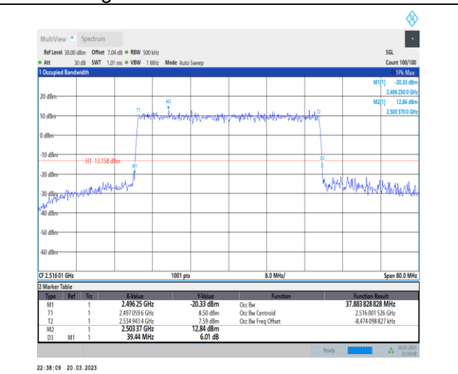
1-N41-30-40-L-6-CP-QPSK-Outer_Full-106@0-Ant1-37.884-39.440-≤40-PASS
