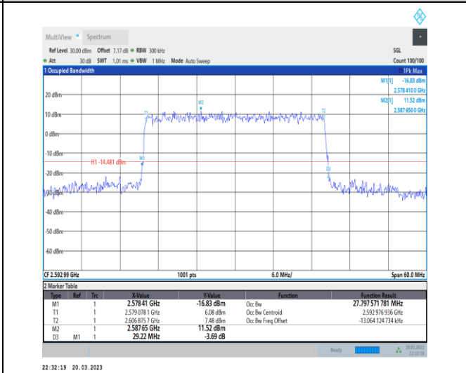
1-N41-30-30-M-6-CP-QPSK-Outer_Full-78@0-Ant1 27.798-29.220-≤30-PASS
