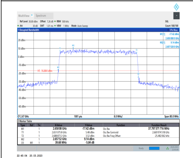
1-N41-30-40-H-9-CP-256QAM-Outer_Full-106@0-A nt1-37.797-39.680-≤40-PASS
