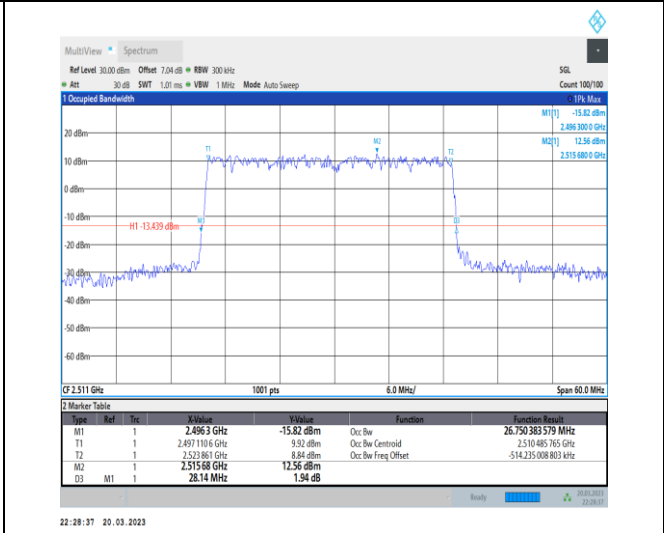
1-N41-30-30-L-3-DFT-16QAM-Outer_Full-75@0-Ant 1-26.75-28.140-≤30-PASS
