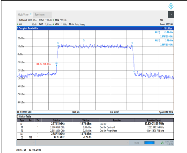
1-N41-30-40-M-6-CP-QPSK-Outer_Full-106@0-Ant 1-37.879-39.760-≤40-PASS
