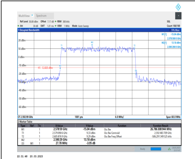
1-N41-30-30-M-3-DFT-16QAM-Outer_Full-75@0-Ant t1-26.786-27.780-≤30-PASS
