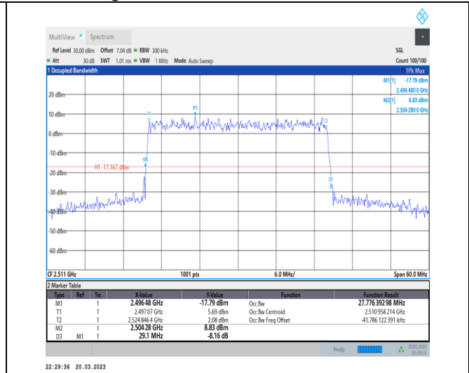
1-N41-30-30-L-9-CP-256QAM-Outer_Full-78@0-Ant1 1-27.776-29.100-≤30-PASS
