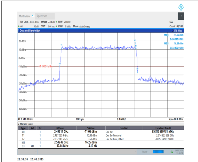
1-N41-30-40-L-1-DFT-QPSK-Outer_Full-100@0-Ant 1-35.816-37.440-≤40-PASS
