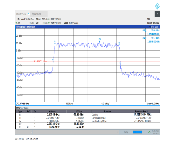
1-N41-30-20-H-5-DFT-256QAM-Outer_Full-50@0-A nt1-17.823-18.640-≤20-PASS
