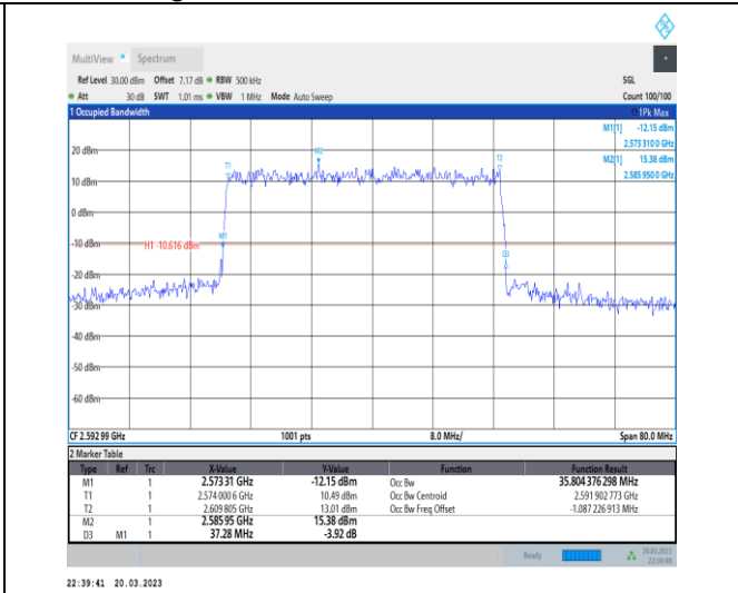
1-N41-30-40-M-1-DFT-QPSK-Outer_Full-100@0-Ant 1-35.804-37.280-≤40-PASS
