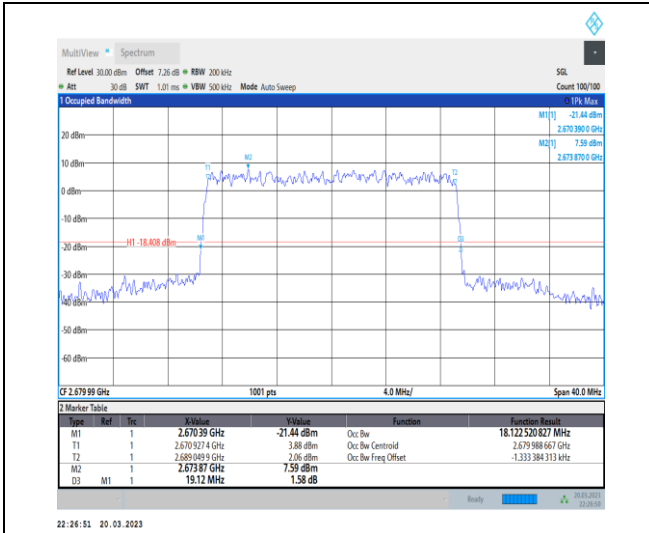
1-N41-30-20-H-9-CP-256QAM-Outer_Full-51@0-Ant 1-18.123-19.120-≤20-PASS
