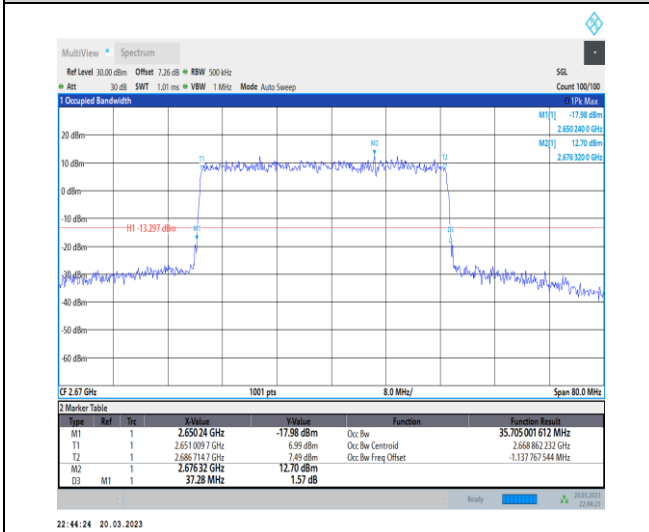
1-N41-30-40-H-5-DFT-256QAM-Outer_Full-100@0-A Ant1-35.705-37.280-≤40-PASS
