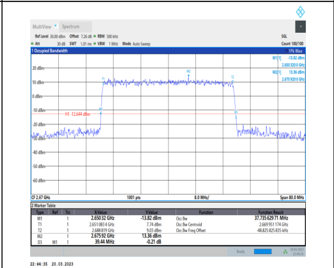
1-N41-30-40-H-6-CP-QPSK-Outer_Full-106@0-A Ant1-37.736-39.440-≤40-PASS
