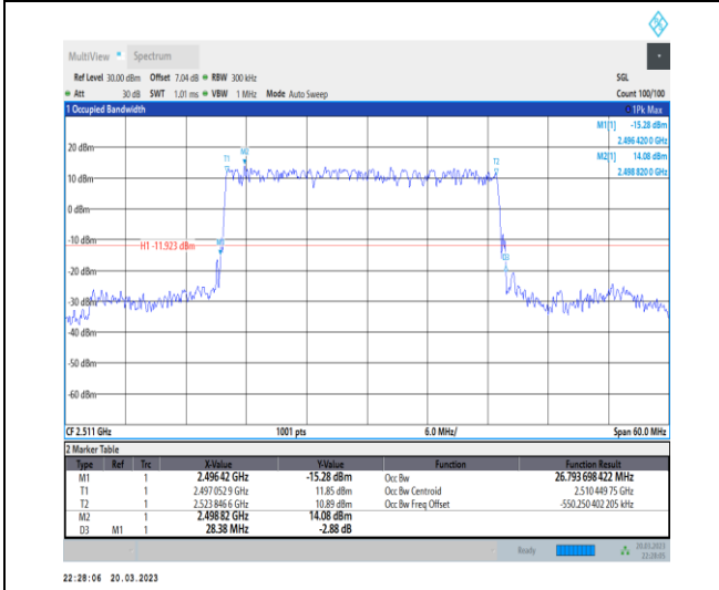
1-N41-30-30-L-2-DFT-PI2BPSK-Outer_Full-75@0-Ant nt1-26.794-28.380-≤30-PASS
