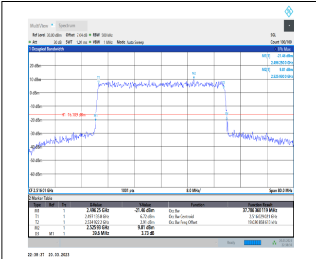
1-N41-30-40-L-9-CP-256QAM-Outer_Full-106@0-A nt1-37.786-39.600-≤40-PASS
