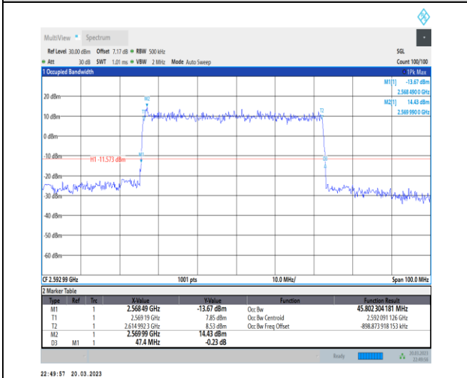
1-N41-30-50-M-3-DFT-16QAM-Outer_Full-128@0-Ant 1-45.802-47.400-≤50-PASS
