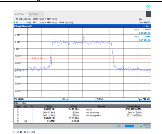
1-N41-30-10-H-4-DFT-64QAM-Outer_Full-24@0-Ant 1-8.57-9.160-≤10-PASS
