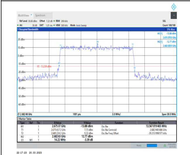
1-N41-30-15-H-6-CP-QPSK-Outer_Full-38@0-Ant1 13.567-14.220-≤15-PASS
