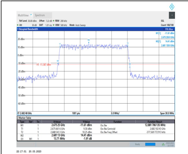
1-N41-30-15-H-4-DFT-64QAM-Outer_Full-36@0-Ant 1-12.882-13.710-≤15-PASS
