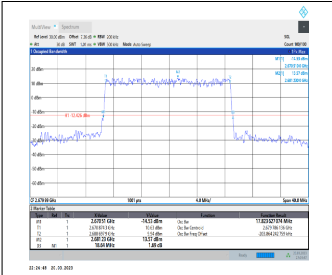
1-N41-30-20-H-1-DFT-QPSK-Outer_Full-50@0-Ant1 -17.824-18.640-≤20-PASS
