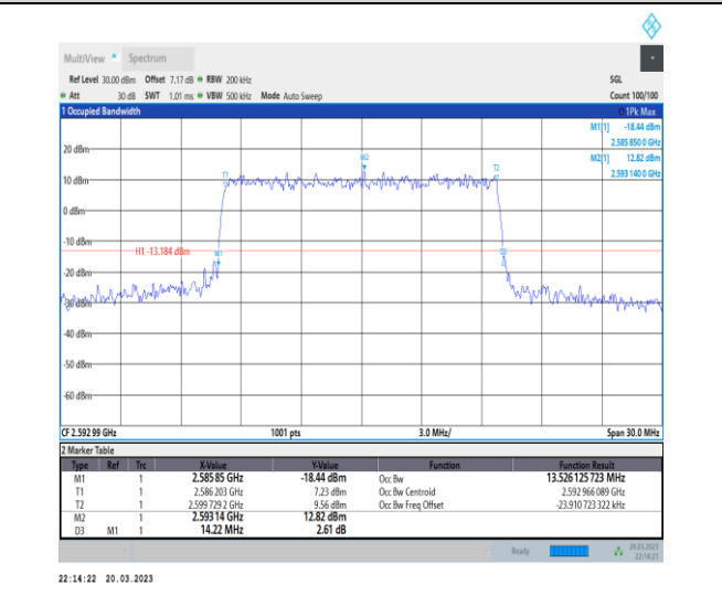
1-N41-30-15-M-8-CP-64QAM-Outer_Full-38@0-Ant1 -13.526-14.220-≤15-PASS
