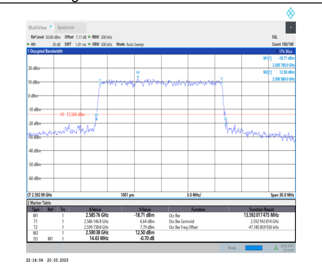
1-N41-30-15-M-6-CP-QPSK-Outer_Full-38@0-Ant1 13.592-14.430-≤15-PASS
