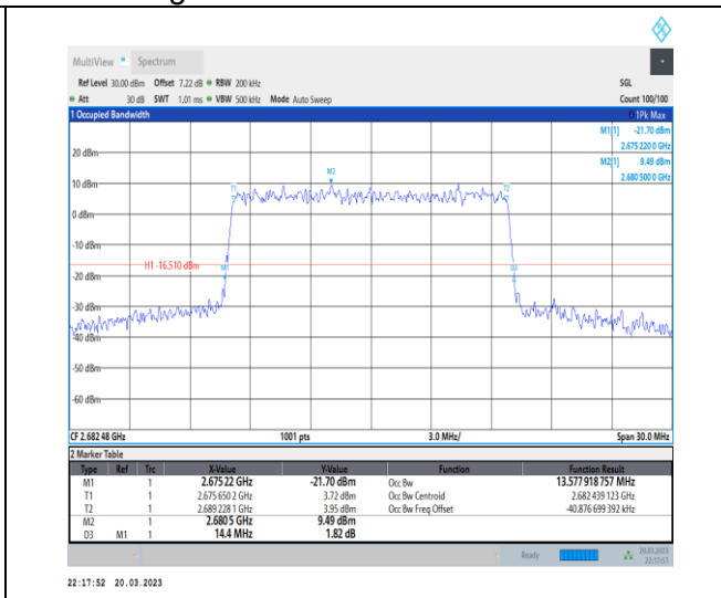
1-N41-30-15-H-9-CP-256QAM-Outer_Full-38@0-Ant1 -13.578-14.400-≤15-PASS
