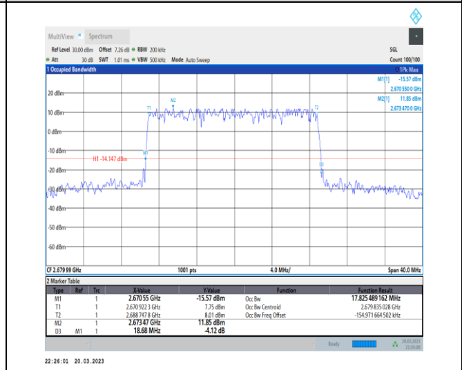
1-N41-30-20-H-4-DFT-64QAM-Outer_Full-50@0-Ant1 1-17.825-18.680-≤20-PASS
