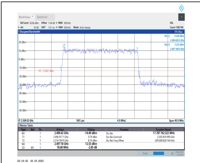
1-N41-30-20-L-3-DFT-16QAM-Outer_Full-50@0-Ant 1-17.788-18.680-≤20-PASS
