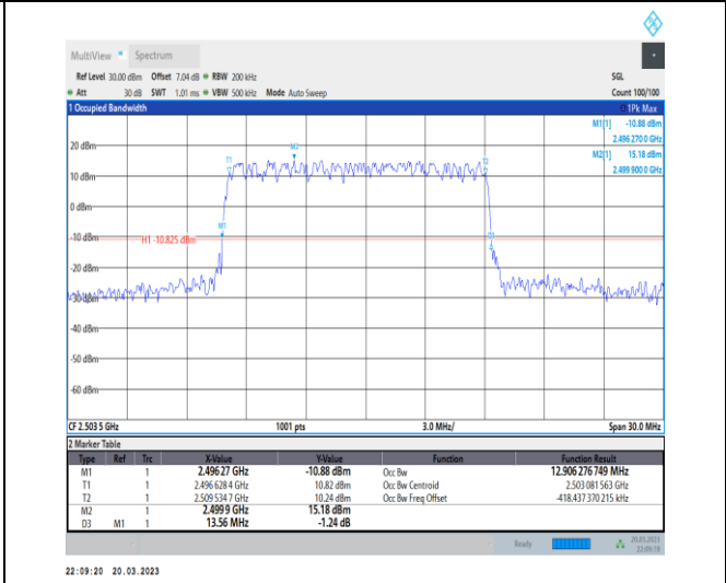
1-N41-30-15-L-1-DFT-QPSK-Outer_Full-36@0-Ant1 12.906-13.560≤15-PASS
