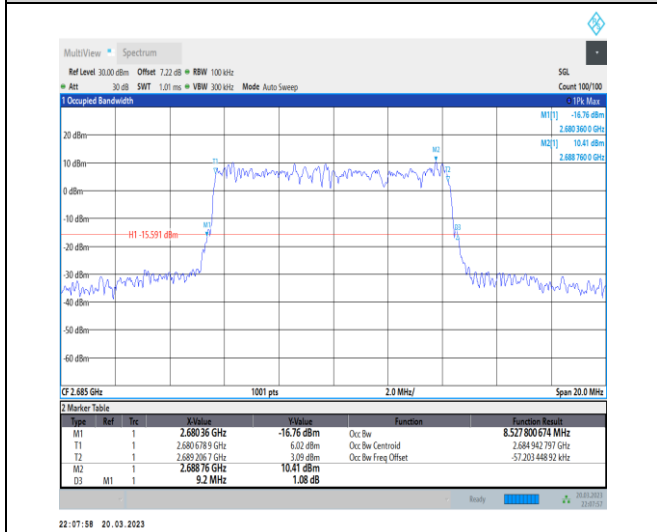
1-N41-30-10-H-5-DFT-256QAM-Outer_Full-24@0-Ant nt1-8.528-9.200-≤10-PASS
