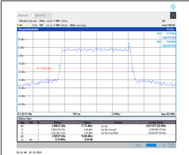
1-N41-30-10-L-5-DFT-256QAM-Outer_Full-24@0-A nt1-8.612-9.160-≤10-PASS
