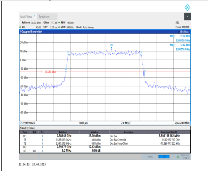
1-N41-30-10-M-5-DFT-256QAM-Outer_Full-24@0-A nt1-8.546-9.200-≤10-PASS
