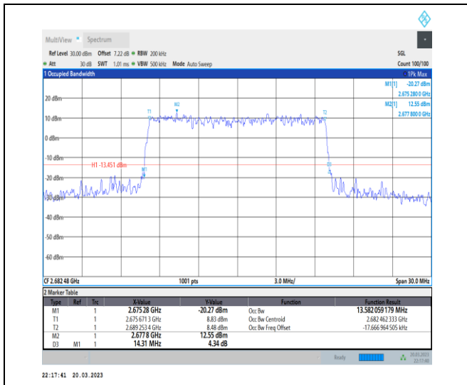
1-N41-30-15-H-8-CP-64QAM-Outer_Full-38@0-Ant1 -13.582-14.310-≤15-PASS
