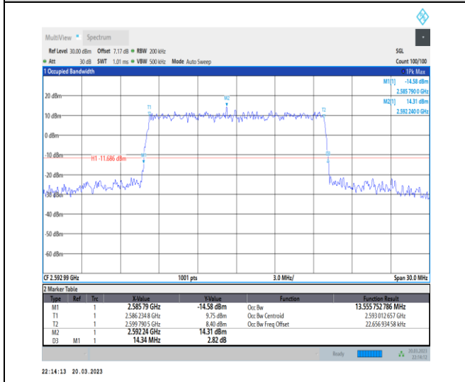
1-N41-30-15-M-7-CP-16QAM-Outer_Full-38@0-Ant 1-13.556-14.340-≤15-PASS
