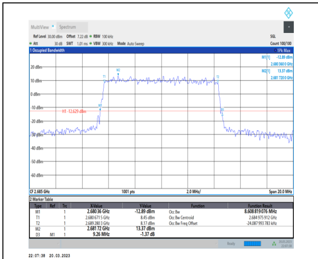
1-N41-30-10-H-3-DFT-16QAM-Outer_Full-24@0-Ant 1-8.609-9.260-≤10-PASS
