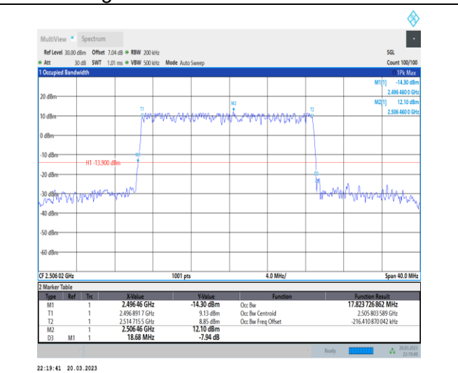
1-N41-30-20-L-4-DFT-64QAM-Outer_Full-50@0-Ant 1-17.824-18.680-≤20-PASS
