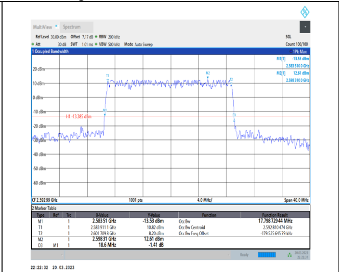
1-N41-30-20-M-3-DFT-16QAM-Outer_Full-50@0-Ant 1-17.799-18.600-≤20-PASS
