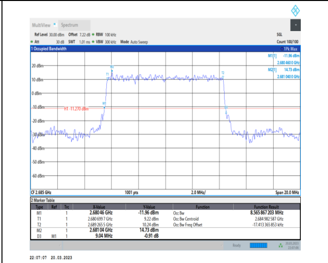
1-N41-30-10-H-2-DFT-PI2BPSK-Outer_Full-24@0-A nt1-8.566-9.040-≤10-PASS
