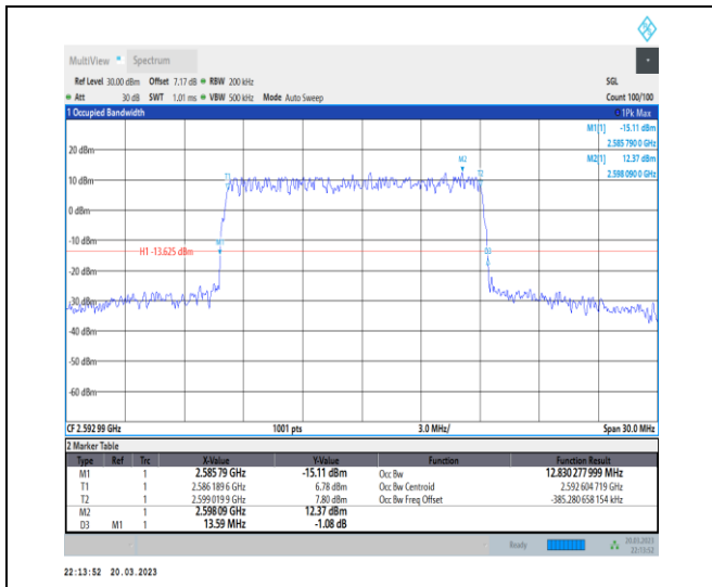
1-N41-30-15-M-5-DFT-256QAM-Outer_Full-36@0-A nt1-12.83-13.590-≤15-PASS
