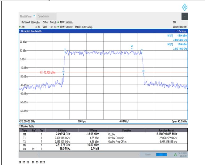
1-N41-30-20-L-8-CP-64QAM-Outer_Full-51@0-Ant1 18.16-19.000-≤20-PASS
