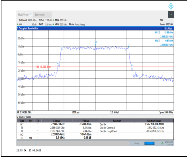
1-N41-30-10-M-6-CP-QPSK-Outer_Full-24@0-Ant1- 8.593-9.400-≤10-PASS
