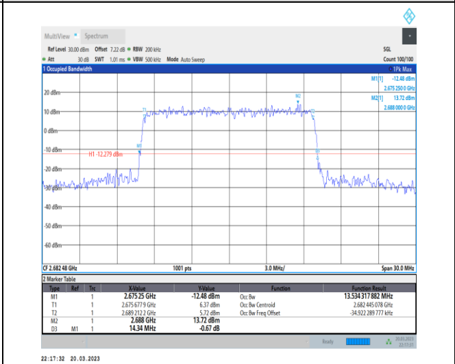
1-N41-30-15-H-7-CP-16QAM-Outer_Full-38@0-Ant1 -13.534-14.340-≤15-PASS
