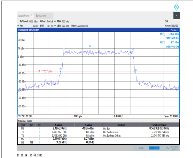
1-N41-30-10-L-9-CP-256QAM-Outer_Full-24@0-Ant 1-8.564-9.280-≤10-PASS
