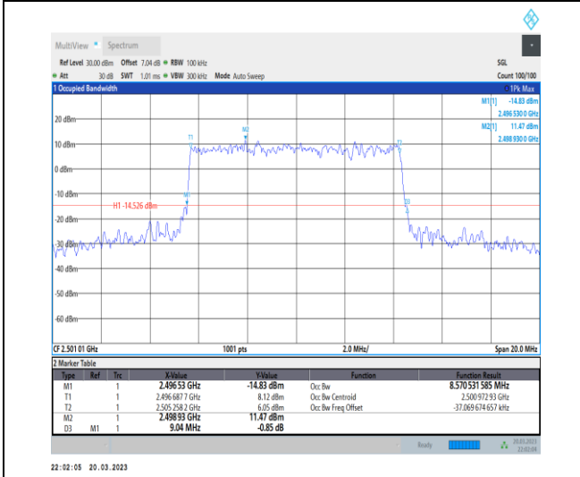
1-N41-30-10-L-7-CP-16QAM-Outer_Full-24@0-Ant1 -8.571-9.040-≤10-PASS
