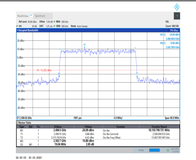
1-N41-30-20-L-6-CP-QPSK-Outer_Full-51@0-Ant1-1 8.194-19.040-≤20-PASS
