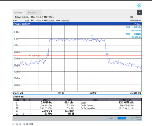
1-N41-30-10-H-6-CP-QPSK-Outer_Full-24@0-Ant 1-8.586-9.300-≤10-PASS
