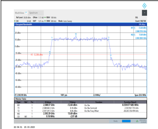
1-N41-30-10-M-2-DFT-PI2BPSK-Outer_Full-24@0-A nt1-8.559-9.180-≤10-PASS
