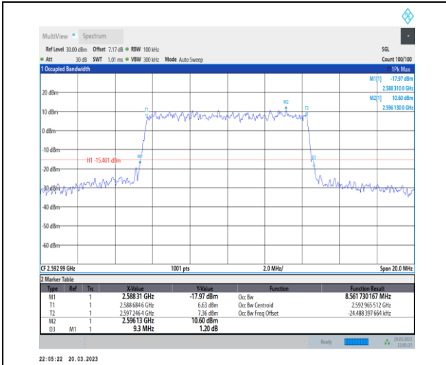
1-N41-30-10-M-8-CP-64QAM-Outer_Full-24@0-Ant 1-8.562-9.300-≤10-PASS
