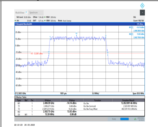
1-N41-30-15-L-3-DFT-16QAM-Outer_Full-36@0-Ant 1-12.853-13.590-≤15-PASS
