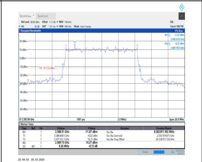
1-N41-30-10-M-3-DFT-16QAM-Outer_Full-24@0-Ant 1-8.583-9.260-≤10-PASS
