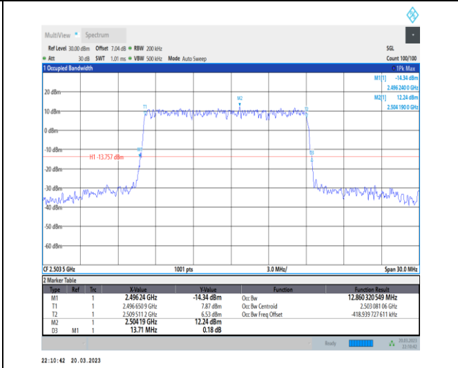
1-N41-30-15-L-5-DFT-256QAM-Outer_Full-36@0-Ant t1-12.86-13.710-≤15-PASS
