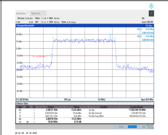
1-N41-30-20-M-1-DFT-QPSK-Outer_Full-50@0-Ant1 -17.856-18.560-≤20-PASS
