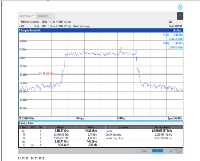
1-N41-30-10-M-9-CP-256QAM-Outer_Full-24@0-Ant 1-8.565-9.260-≤10-PASS
