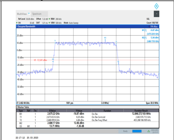
1-N41-30-15-H-5-DFT-256QAM-Outer_Full-36@0-Ant t1-12.846-13.710-≤15-PASS
