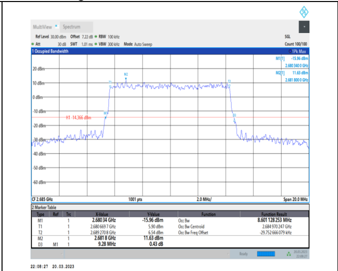
1-N41-30-10-H-8-CP-64QAM-Outer_Full-24@0-Ant1 -8.601-9.280≤10-PASS
