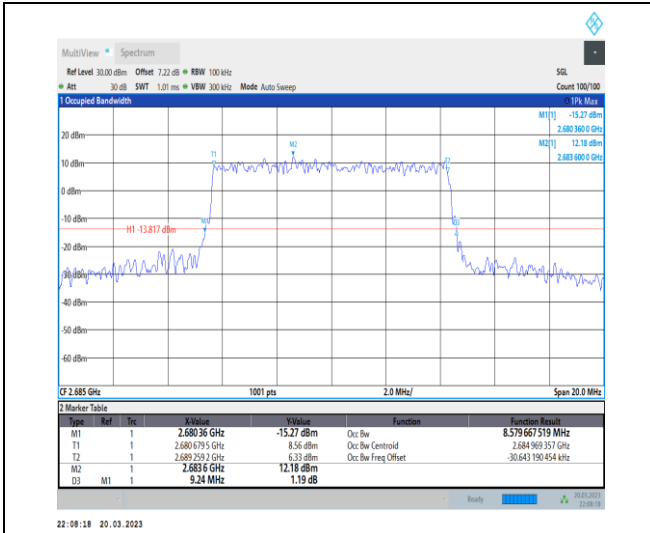
1-N41-30-10-H-7-CP-16QAM-Outer_Full-24@0-Ant1 -8.58-9.240≤10-PASS
