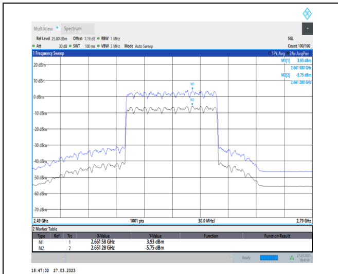
1-N41-30-100-H-1-DFT-256QAM-Outer_Full-270@0-Ant1-9.68-19.56%-7.09-2.59-PASS-≤13
