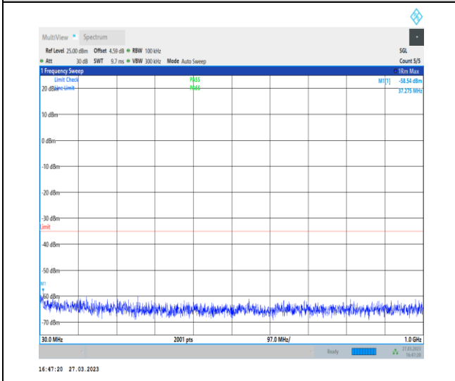
1-N38-30-40-H-1-DFT-PI2BPSK-Inner_1RB_Left-1 @ 1-30-1000-Ant1-48.92--58.54--35-PASS
