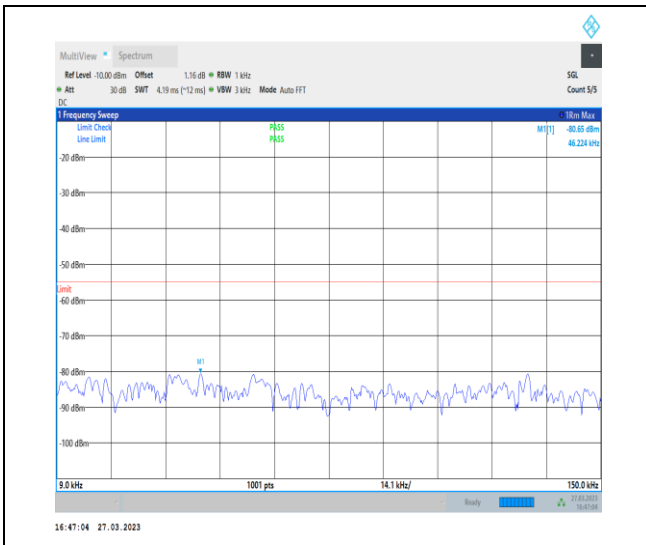
1-N38-30-40-H-1-DFT-PI2BPSK-Inner_1RB_Left-1 @ 1-0.009-0.15-Ant1-0.13--80.65--55-PASS
