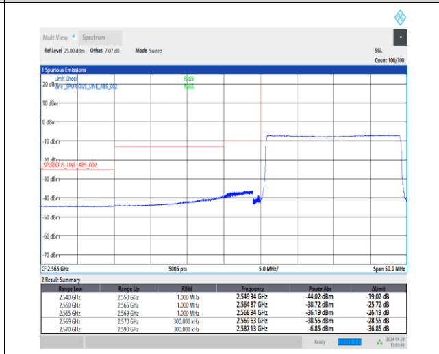
1-N38-30-20-L-6-CP-QPSK-Outer_Full-51@0-Ant1-1--PASS-see graph
