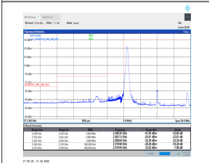
1-N38-30-20-L-4-CP-QPSK-Edge_1RB_Left-1@0-Ant1-1--PASS-see graph
