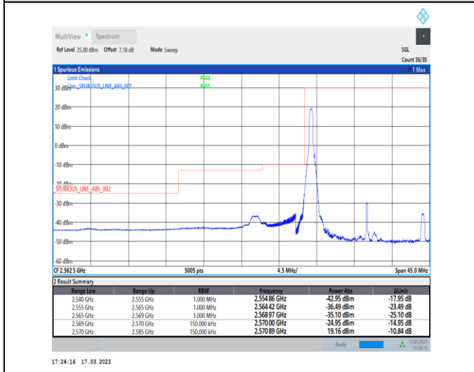
1-N38-30-15-L-4-CP-QPSK-Edge_1RB_Left-1@0-Ant1-1--PASS-see graph
