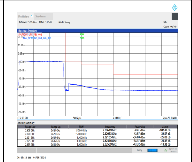
1-N38-30-15-H-6-CP-QPSK-Outer_Full-38@0-Ant1-1--PASS-see graph
