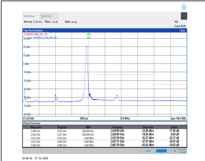
1-N38-30-40-H-2-DFT-PI2BPSK-Edge_1RB_Right-1@105-Ant1-1--PASS-see graph
