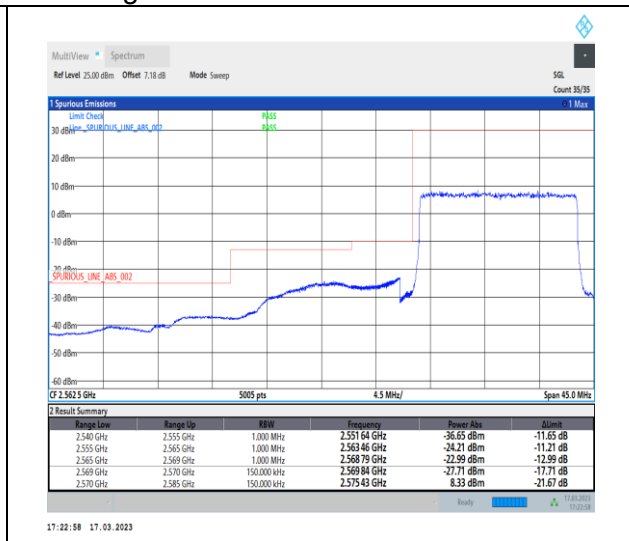
1-N38-30-15-L-3-DFT-PI2BPSK-Outer_Full-36@0-Ant1-1--PASS-see graph
