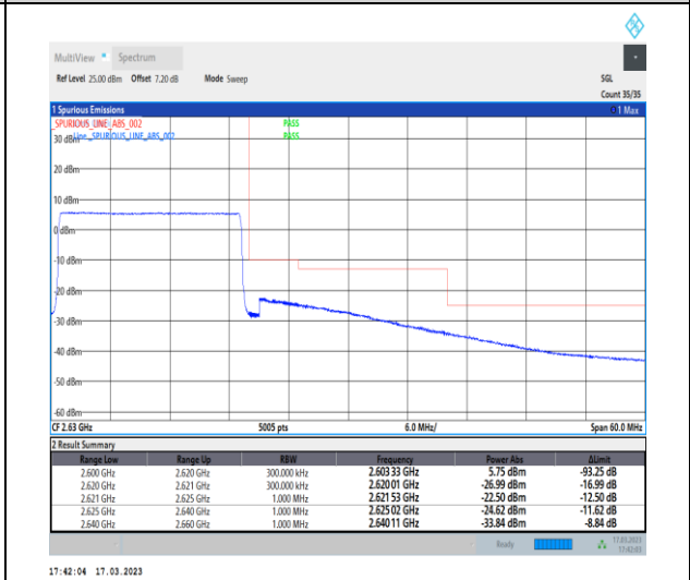
1-N38-30-20-H-6-CP-QPSK-Outer_Full-51@0-Ant1-1--PASS-see graph
