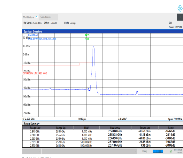
1-N38-30-40-L-1-DFT-PI2BPSK-Edge_1RB_Left-1@0-Ant1-1--PASS-see graph
