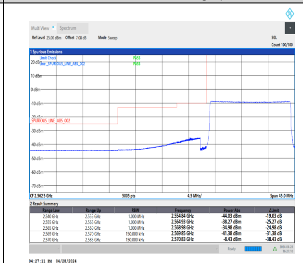
1-N38-30-15-L-6-CP-QPSK-Outer_Full-38@0-Ant1-1--PASS-see graph
