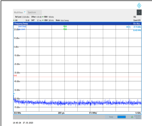
1-N38-30-40-M-1-DFT-PI2BPSK-Inner_1RB_Left-1 @ 1-30-1000-Ant1-32.43--57.74--35-PASS
