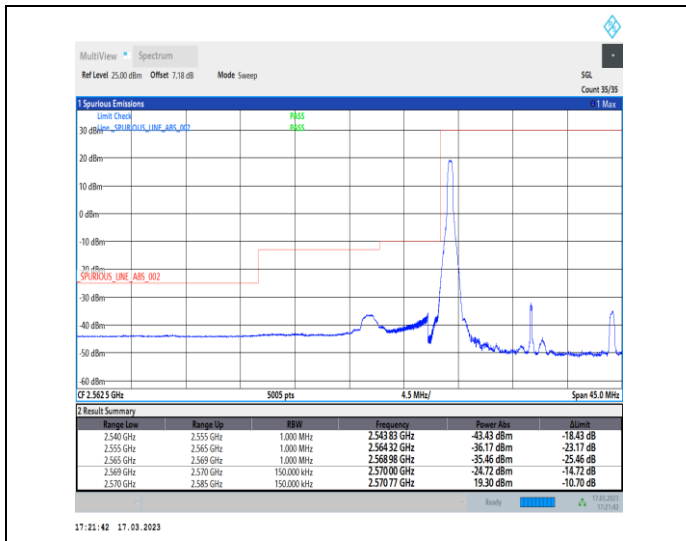
1-N38-30-15-L-1-DFT-PI2BPSK-Edge_1RB_Left-1@0-Ant1-1--PASS-see graph
