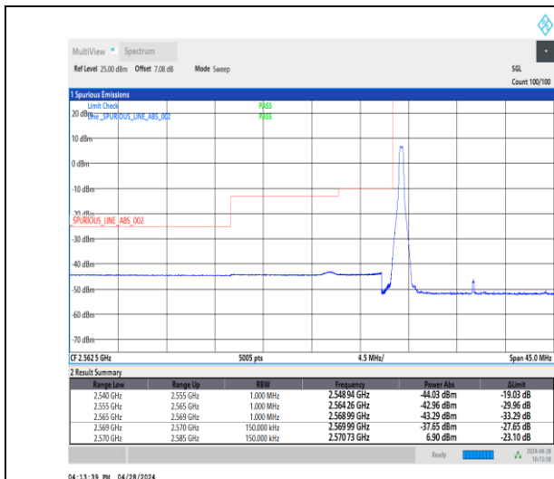
1-N38-30-15-L-1-DFT-PI2BPSK-Edge_1RB_Left-1@0-Ant1-1--PASS-see graph
