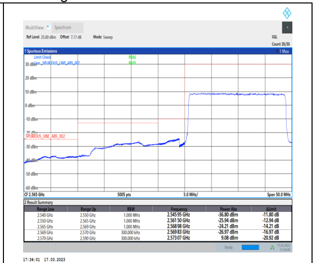
1-N38-30-20-L-3-DFT-PI2BPSK-Outer_Full-50@0-Ant1-1--PASS-see graph
