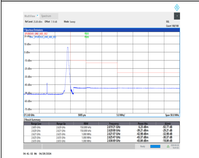
1-N38-30-15-H-5-CP-QPSK-Edge_1RB_Right-1@37-Ant1-1--PASS-see graph
