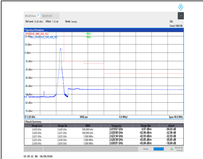
1-N38-30-10-H-2-DFT-PI2BPSK-Edge_1RB_Right-1@23-Ant1-1--PASS-see graph
