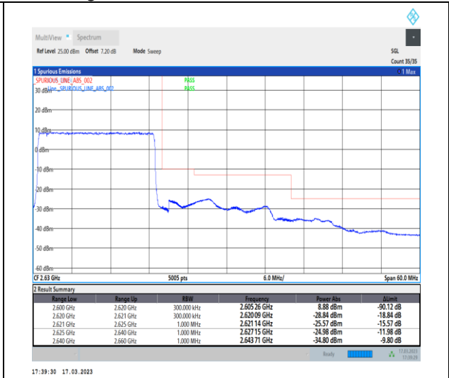
1-N38-30-20-H-3-DFT-PI2BPSK-Outer_Full-50@0-Ant1-1--PASS-see graph
