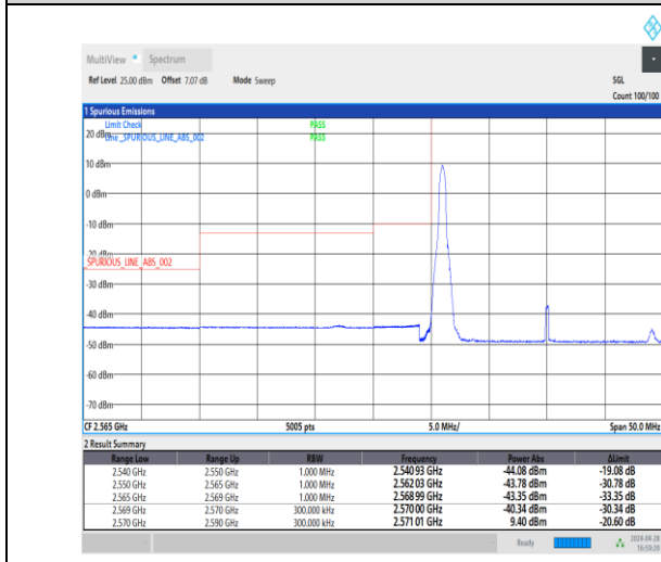
1-N38-30-20-L-4-CP-QPSK-Edge_1RB_Left-1@0-Ant1-1--PASS-see graph
