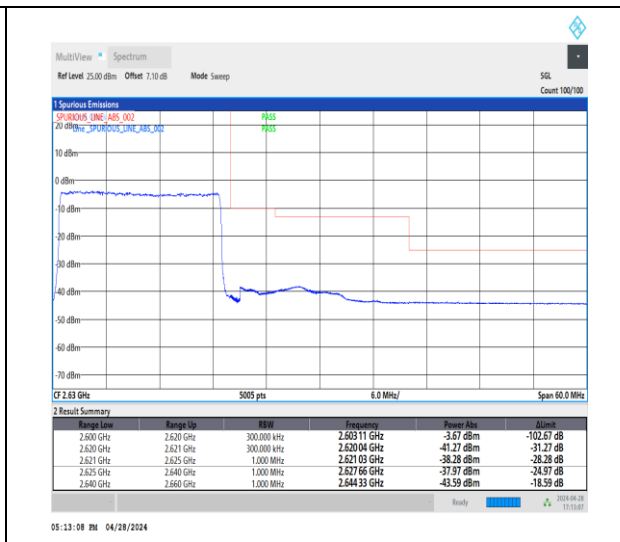
1-N38-30-20-H-3-DFT-PI2BPSK-Outer_Full-50@0-Ant1-1--PASS-see graph
