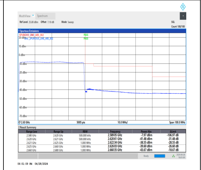
1-N38-30-40-H-6-CP-QPSK-Outer_Full-106@0-Ant1-1--PASS-see graph
