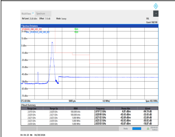
1-N38-30-10-H-5-CP-QPSK-Edge_1RB_Right-1@23-Ant1-1--PASS-see graph
