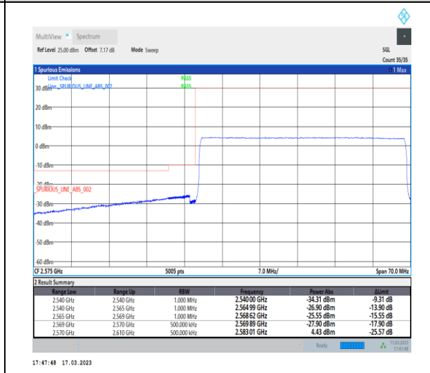
1-N38-30-40-L-6-CP-QPSK-Outer_Full-106@0-Ant1-1--PASS-see graph
