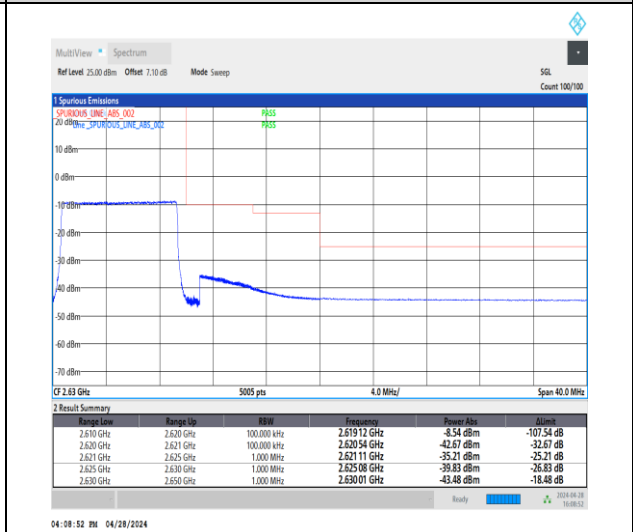
1-N38-30-10-H-6-CP-QPSK-Outer_Full-24@0-Ant1-1--PASS-see graph
