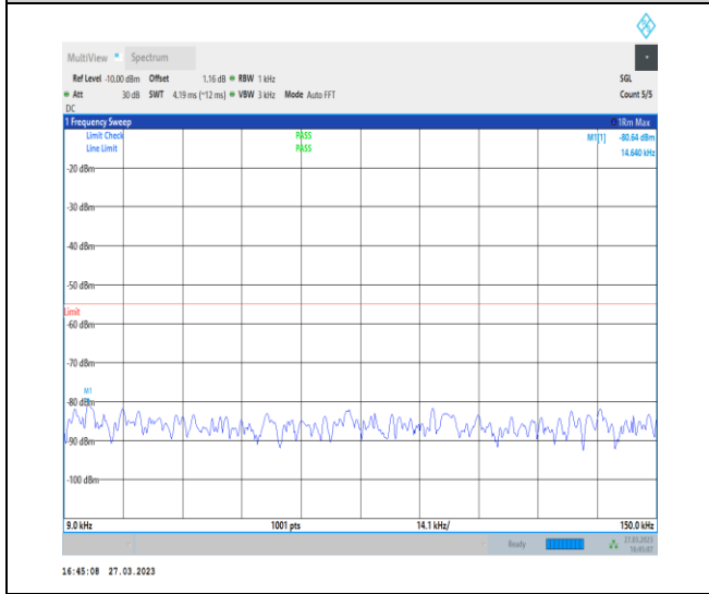
1-N38-30-40-M-1-DFT-PI2BPSK-Inner_1RB_Left-1 @ 1-0.009-0.15-Ant1-0.09--80.64--55-PASS
