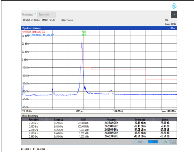
1-N38-30-40-H-5-CP-QPSK-Edge_1RB_Right-1@105-Ant1-1--PASS-see graph
