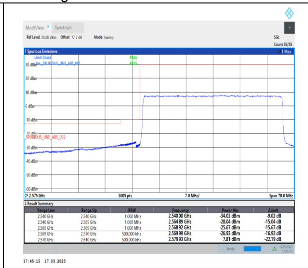
1-N38-30-40-L-3-DFT-PI2BPSK-Outer_Full-100@0-Ant1-1--PASS-see graph
