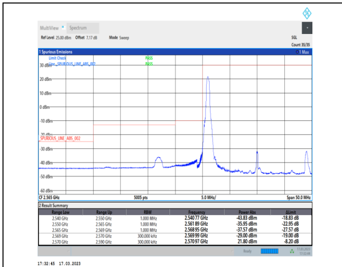
1-N38-30-20-L-1-DFT-PI2BPSK-Edge_1RB_Left-1@0-Ant1-1--PASS-see graph
