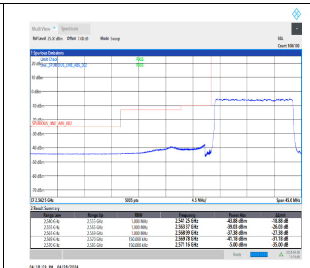
1-N38-30-15-L-3-DFT-PI2BPSK-Outer_Full-36@0-Ant1-1--PASS-see graph
