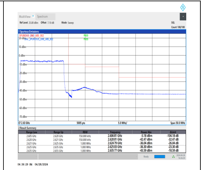
1-N38-30-15-H-3-DFT-PI2BPSK-Outer_Full-36@0-Ant1-1--PASS-see graph
