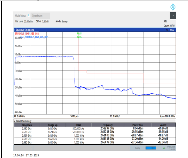
1-N38-30-40-H-3-DFT-PI2BPSK-Outer_Full-100@0-Ant1-1--PASS-see graph
