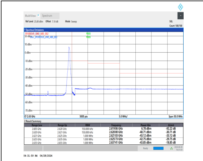
1-N38-30-15-H-2-DFT-PI2BPSK-Edge_1RB_Right-1@37-Ant1-1--PASS-see graph
