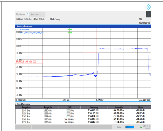
1-N38-30-20-L-3-DFT-PI2BPSK-Outer_Full-50@0-Ant1-1--PASS-see graph
