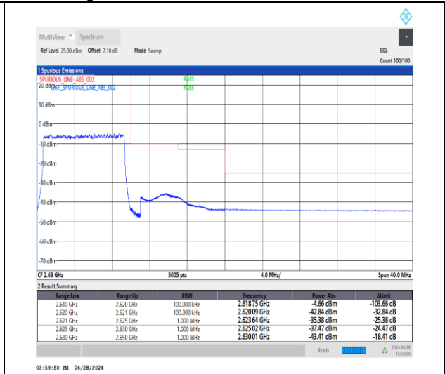
1-N38-30-10-H-3-DFT-PI2BPSK-Outer_Full-24@0-Ant1-1--PASS-see graph
