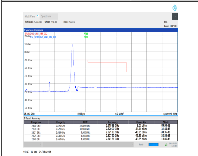
1-N38-30-20-H-5-CP-QPSK-Edge_1RB_Right-1@50-Ant1-1--PASS-see graph
