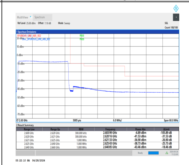
1-N38-30-20-H-6-CP-QPSK-Outer_Full-51@0-Ant1-1--PASS-see graph
