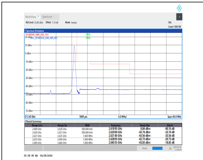
1-N38-30-20-H-2-DFT-PI2BPSK-Edge_1RB_Right-1@50-Ant1-1--PASS-see graph
