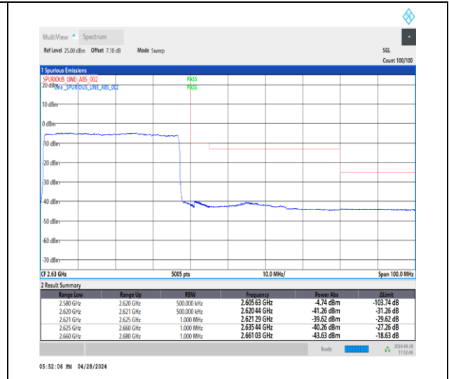
1-N38-30-40-H-3-DFT-PI2BPSK-Outer_Full-100@0-Ant1-1--PASS-see graph
