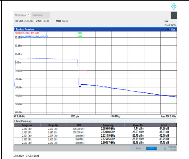
1-N38-30-40-H-6-CP-QPSK-Outer_Full-106@0-Ant1-1--PASS-see graph
