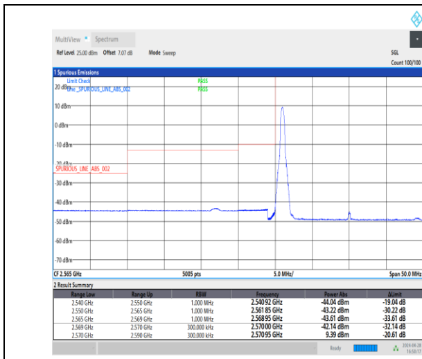
1-N38-30-20-L-1-DFT-PI2BPSK-Edge_1RB_Left-1@0-Ant1-1--PASS-see graph
