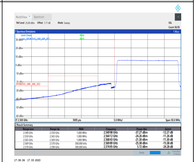
1-N38-30-20-L-6-CP-QPSK-Outer_Full-51@0-Ant1-1--PASS-see graph
