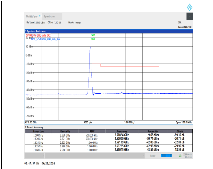
1-N38-30-40-H-2-DFT-PI2BPSK-Edge_1RB_Right-1@105-Ant1-1--PASS-see graph
