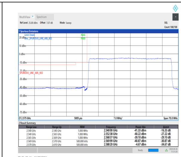
1-N38-30-40-L-3-DFT-PI2BPSK-Outer_Full-100@0-Ant1-1--PASS-see graph
