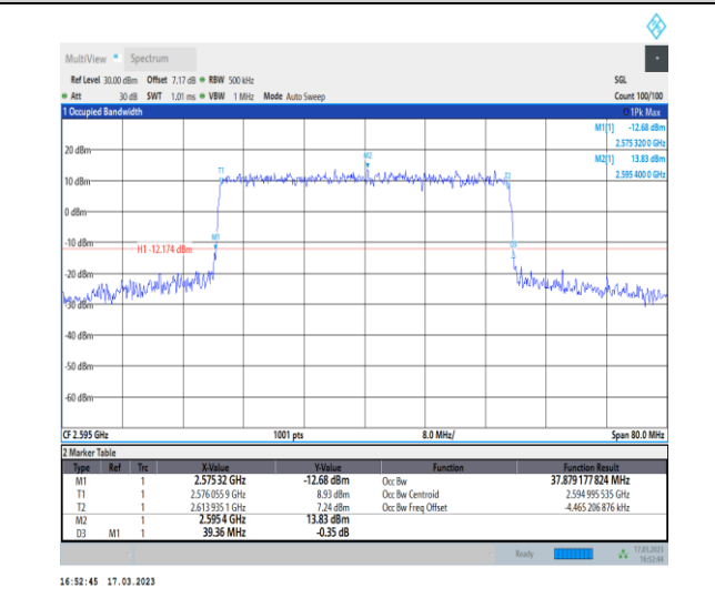
1-N38-30-40-M-6-CP-QPSK-Outer_Full-106@0-Ant1 -37.879-39.360-≤40-PASS
