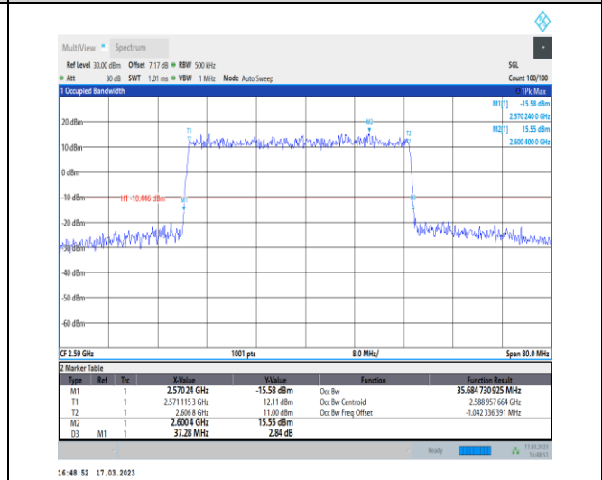
1-N38-30-40-L-3-DFT-16QAM-Outer_Full-100@0-An t1 1-35.685-37.280-≤40-PASS
