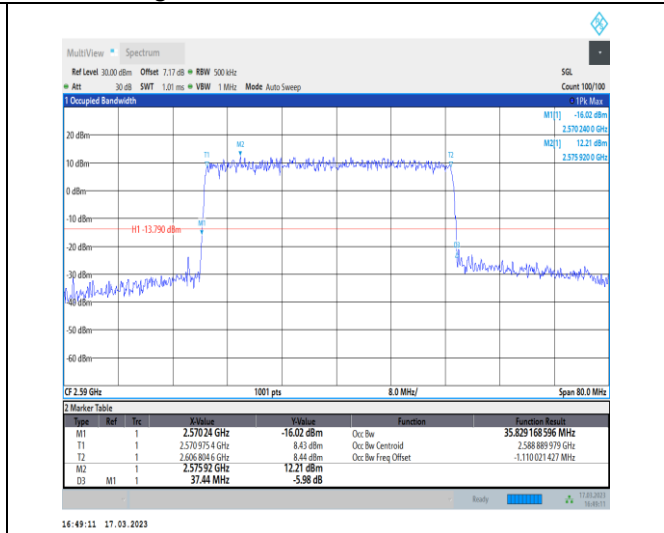
1-N38-30-40-L-5-DFT-256QAM-Outer_Full-100@0-A nt1-35.829-37.440-<40-PASS
