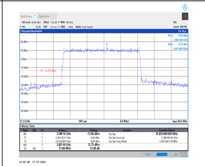
1-N38-30-40-H-5-DFT-256QAM-Outer_Full-100@0-Ant1-35.836-37.680-≤40-PASS
