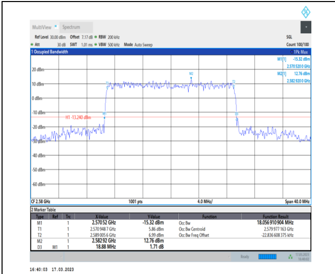
1-N38-30-20-L-7-CP-16QAM-Outer_Full-51@0-Ant1 -18.057-18.880-≤20-PASS
