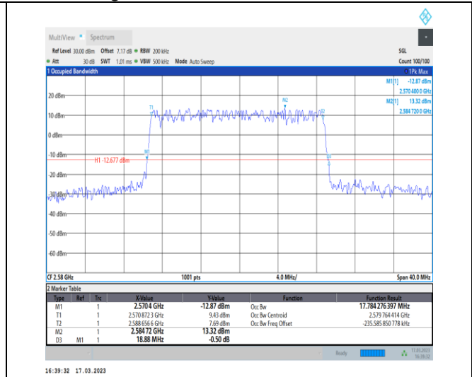
1-N38-30-20-L-4-DFT-64QAM-Outer_Full-50@0-Ant 1-17.784-18.880-≤20-PASS
