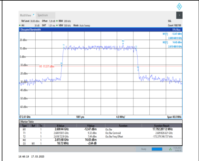
1-N38-30-20-H-4-DFT-64QAM-Outer_Full-50@0-Ant 1-17.792-18.720-≤20-PASS
