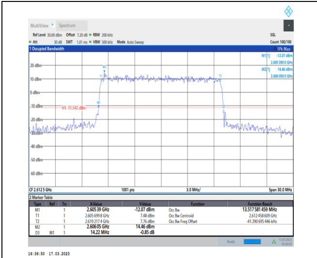
1-N38-30-15-H-8-CP-64QAM-Outer_Full-38@0-Ant1 -13.518-14.220-≤15-PASS
