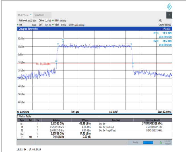
1-N38-30-40-M-7-CP-16QAM-Outer_Full-106@0-An t1-37.832-39.440-<math>\leq 40</math>-PASS
