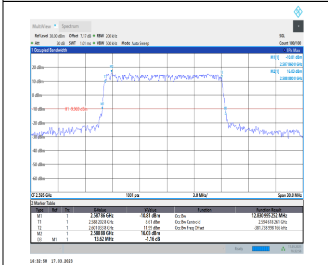
1-N38-30-15-M-3-DFT-16QAM-Outer_Full-36@0-Ant 1-12.831-13.620-≤15-PASS
