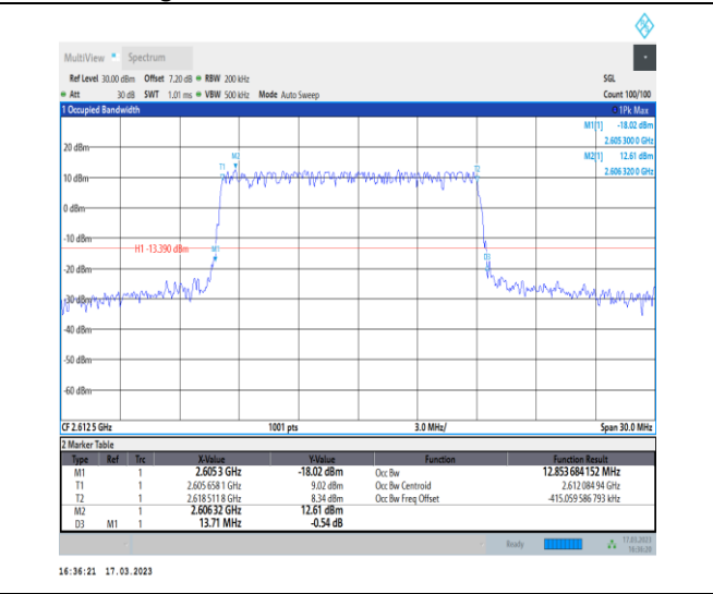
1-N38-30-15-H-5-DFT-256QAM-Outer_Full-36@0-A nt1-12.854-13.710-≤15-PASS
