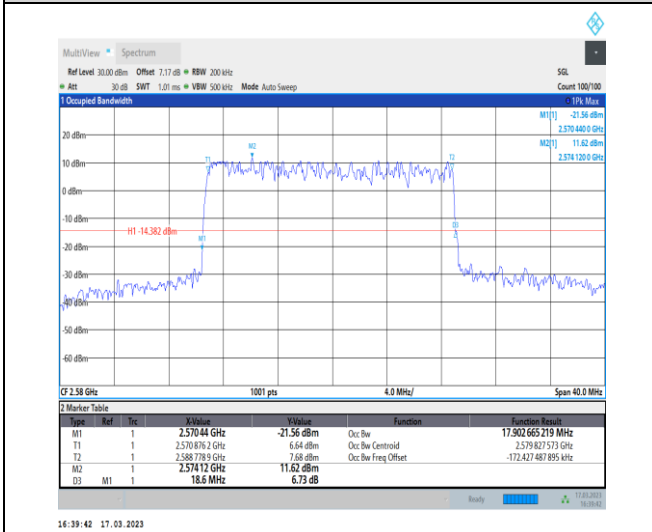
1-N38-30-20-L-5-DFT-256QAM-Outer_Full-50@0-Ant t1-17.903-18.600-≤20-PASS
