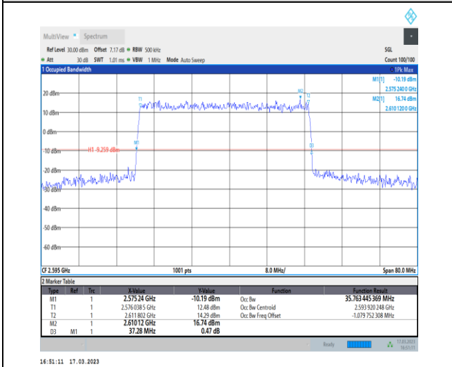
1-N38-30-40-M-1-DFT-QPSK-Outer_Full-100@0-Ant 1-35.763-37.280-≤40-PASS
