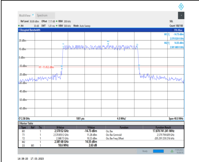
1-N38-30-20-L-1-DFT-QPSK-Outer_Full-50@0-Ant1- 17.871-18.600-≤20-PASS
