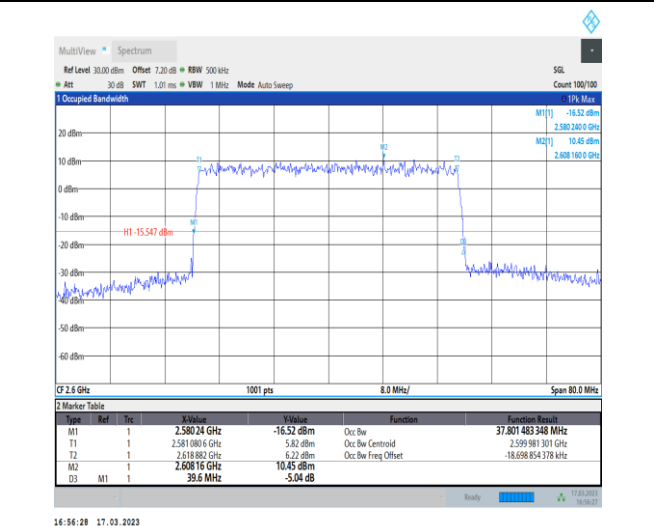
1-N38-30-40-H-9-CP-256QAM-Outer_Full-106@0-A nt1-37.801-39.600-≤40-PASS
