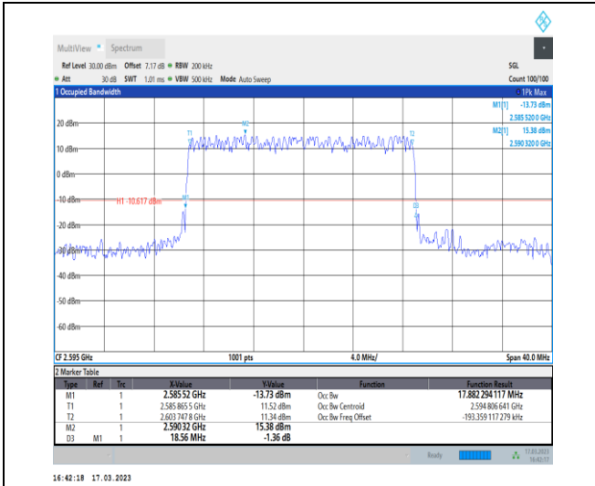
1-N38-30-20-M-2-DFT-PI2BPSK-Outer_Full-50@0-A nt1-17.882-18.560-≤20-PASS
