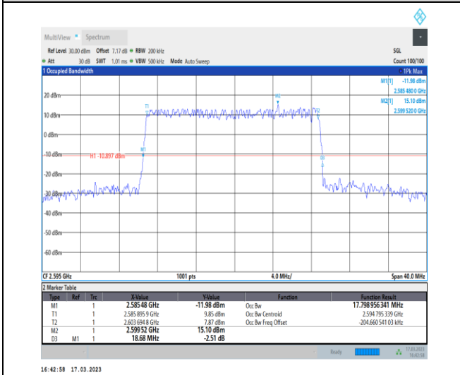
1-N38-30-20-M-4-DFT-64QAM-Outer_Full-50@0-Ant 1-17.799-18.680-≤20-PASS
