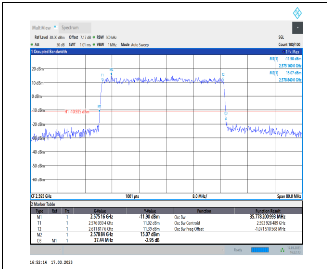
1-N38-30-40-M-3-DFT-16QAM-Outer_Full-100@0-A nt1-35.778-37.440-≤40-PASS
