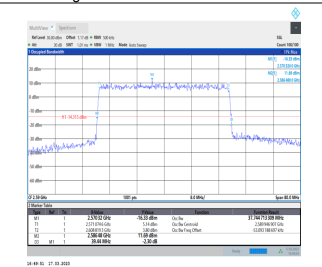
1-N38-30-40-L-9-CP-256QAM-Outer_Full-106@0-An t1-37.745-39.440-≤40-PASS
