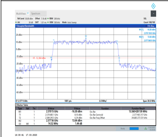
1-N38-30-15-L-8-CP-64QAM-Outer_Full-38@0-Ant1-13.56-14.520-≤15-PASS
