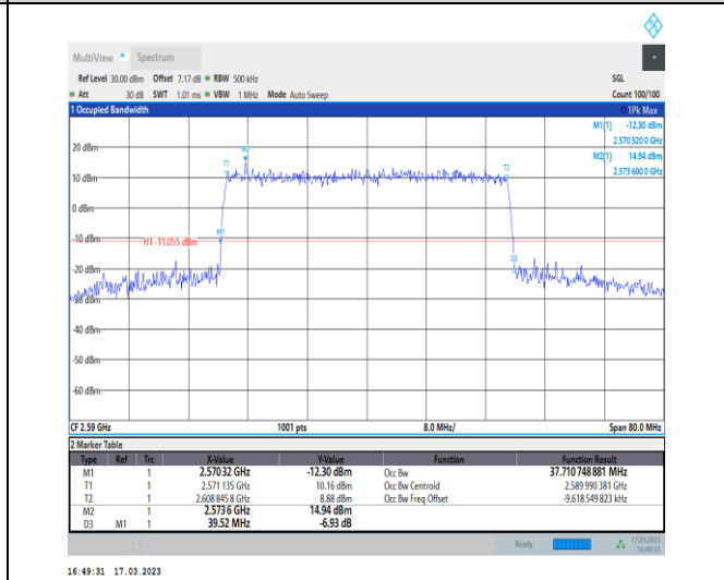
1-N38-30-40-L-7-CP-16QAM-Outer_Full-106@0-Ant 1-37.711-39.520-<40-PASS
