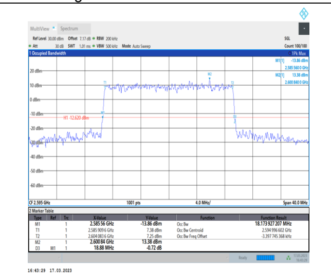
1-N38-30-20-M-7-CP-16QAM-Outer_Full-51@0-Ant1-18.174-18.880-≤20-PASS
