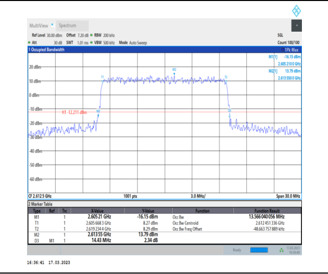
1-N38-30-15-H-7-CP-16QAM-Outer_Full-38@0-Ant1 -13.566-14.430-≤15-PASS
