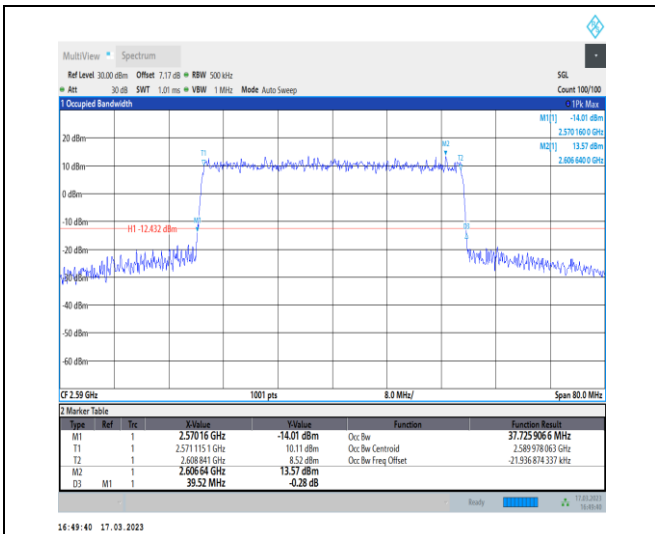
1-N38-30-40-L-8-CP-64QAM-Outer_Full-106@0-Ant 1-37.726-39.520-≤40-PASS
