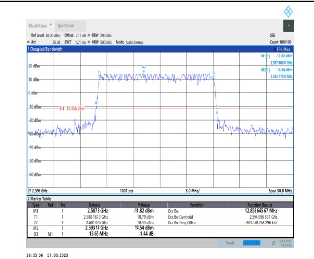
1-N38-30-15-M-4-DFT-64QAM-Outer_Full-36@0-Ant 1-12.859-13.650-≤15-PASS
