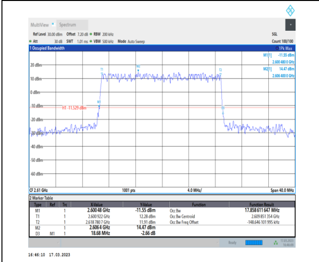
1-N38-30-20-H-3-DFT-16QAM-Outer_Full-50@0-Ant 1-17.859-18.680-≤20-PASS
