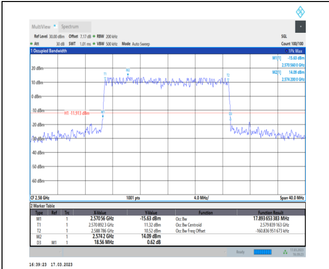
1-N38-30-20-L-3-DFT-16QAM-Outer_Full-50@0-Ant 1-17.894-18.560-≤20-PASS
