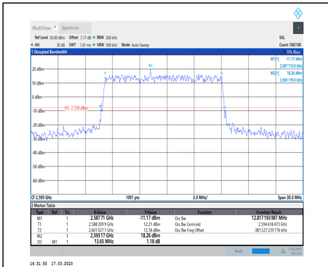
1-N38-30-15-M-1-DFT-QPSK-Outer_Full-36@0-Ant1 -12.817-13.650-≤15-PASS
