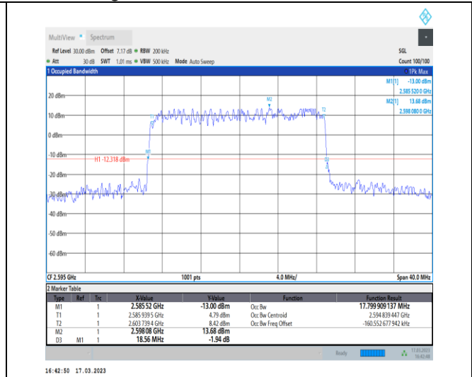
1-N38-30-20-M-3-DFT-16QAM-Outer_Full-50@0-Ant 1-17.8-18.560-≤20-PASS
