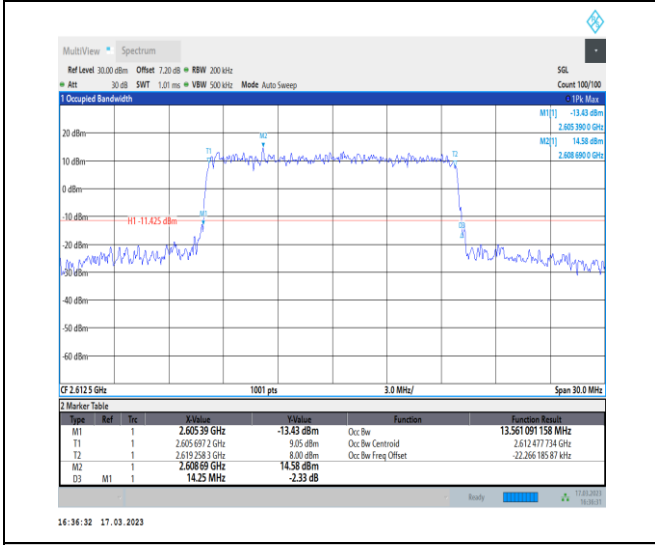
1-N38-30-15-H-6-CP-QPSK-Outer_Full-38@0-Ant1 13.561-14.250-≤15-PASS
