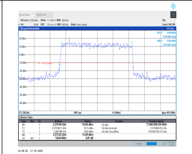
1-N38-30-20-L-2-DFT-PI2BPSK-Outer_Full-50@0-A nt1-17.846-18.640-≤20-PASS
