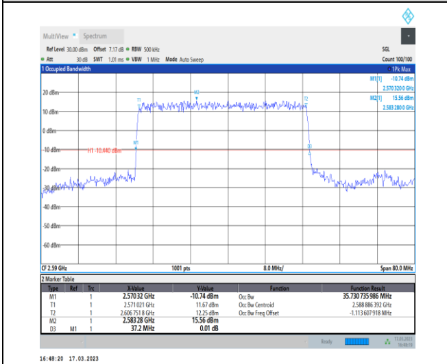
1-N38-30-40-L-2-DFT-PI2BPSK-Outer_Full-100@0-Ant1 1-35.731-37.200-≤40-PASS
