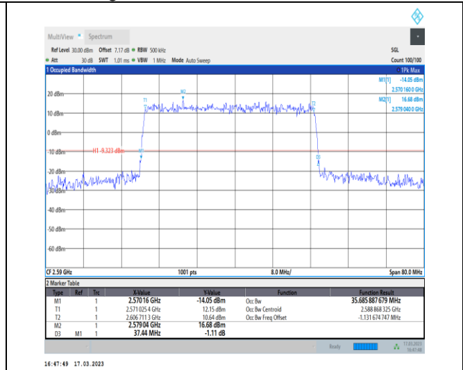
1-N38-30-40-L-1-DFT-QPSK-Outer_Full-100@0-Ant 1-35.686-37.440-≤40-PASS
