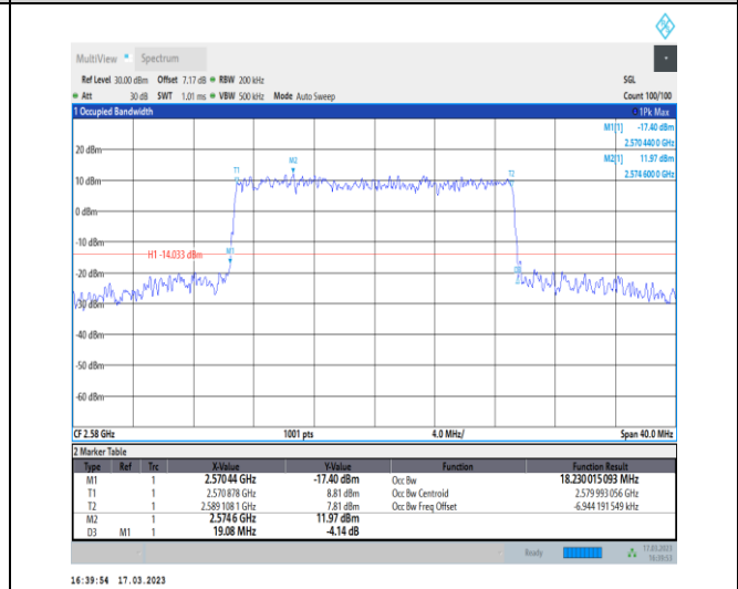
1-N38-30-20-L-6-CP-QPSK-Outer_Full-51@0-Ant1-1 8.23-19.080-≤20-PASS
