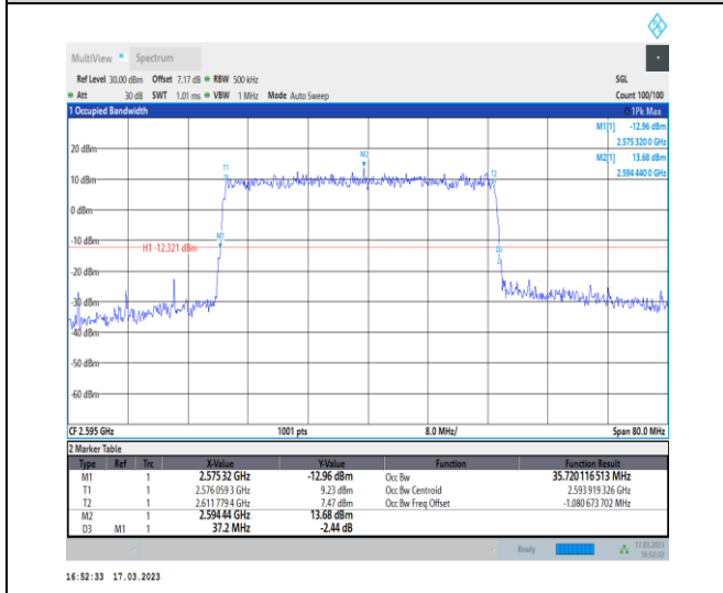
1-N38-30-40-M-5-DFT-256QAM-Outer_Full-100@0-A Ant1-35.72-37.200-≤40-PASS
