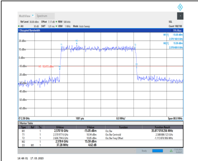
1-N38-30-40-L-4-DFT-64QAM-Outer_Full-100@0-An t1-35.817-37.280-<40-PASS
