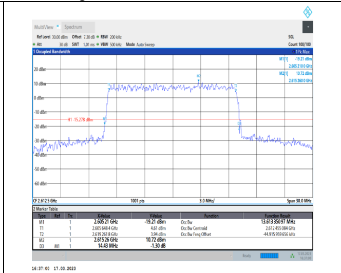
1-N38-30-15-H-9-CP-256QAM-Outer_Full-38@0-Ant 1-13.613-14.430-≤15-PASS
