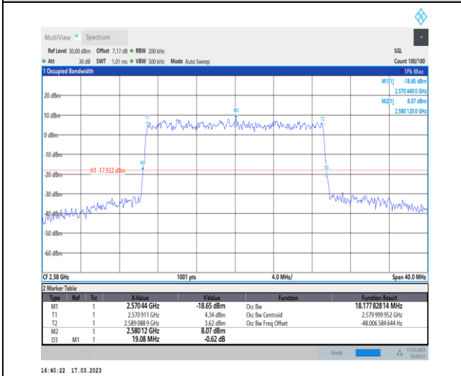
1-N38-30-20-L-9-CP-256QAM-Outer_Full-51@0-Ant 1-18.178-19.080-≤20-PASS
