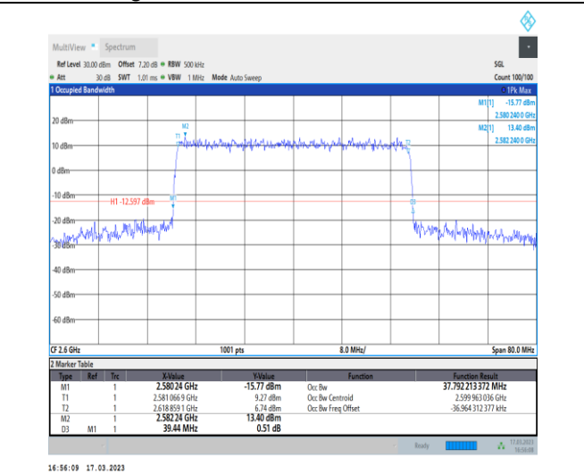
1-N38-30-40-H-7-CP-16QAM-Outer_Full-106@0-Ant 1-37.792-39.440-≤40-PASS
