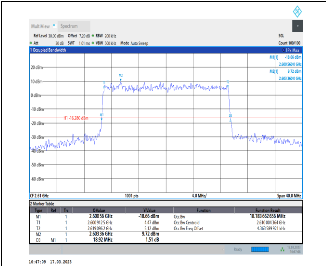
1-N38-30-20-H-9-CP-256QAM-Outer_Full-51@0-Ant 1-18.184-18.920-≤20-PASS
