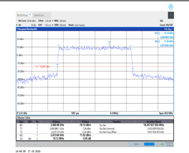
1-N38-30-20-H-8-CP-64QAM-Outer_Full-51@0-Ant1-18.248-19.120-≤20-PASS
