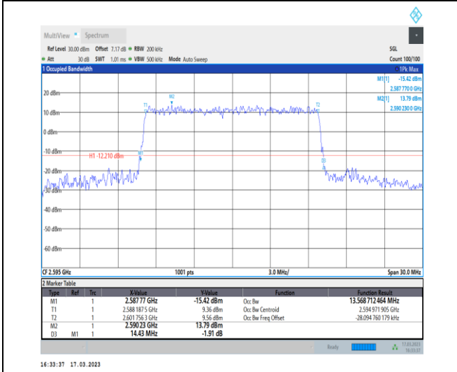
1-N38-30-15-M-7-CP-16QAM-Outer_Full-38@0-Ant1-13.569-14.430-≤15-PASS
