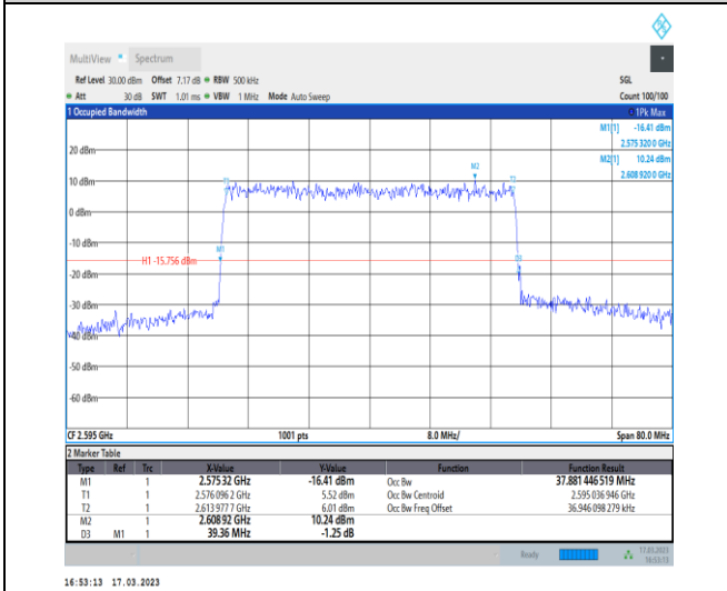
1-N38-30-40-M-9-CP-256QAM-Outer_Full-106@0-A nt1-37.881-39.360-<math>\leq 40</math>-PASS
