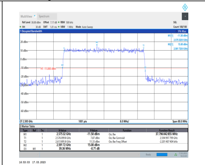
1-N38-30-40-M-8-CP-64QAM-Outer_Full-106@0-Ant 1-37.796-39.360-<math>\leq 40</math>-PASS
