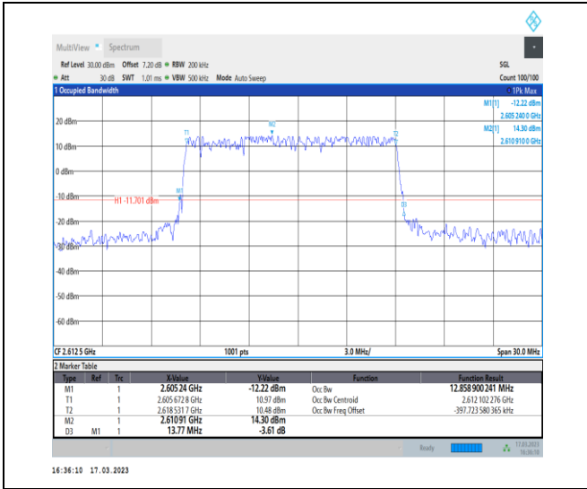
1-N38-30-15-H-4-DFT-64QAM-Outer_Full-36@0-Ant 1-12.859-13.770-≤15-PASS
